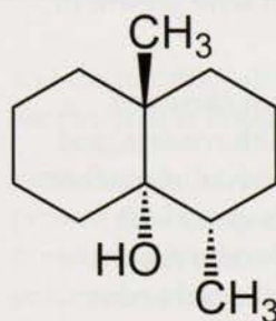
Figure 2. Chemical structures of geosmin (left) and 2-MIB (right)
