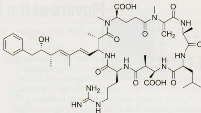
Figure 3. Chemical structure of microcystin-LR
