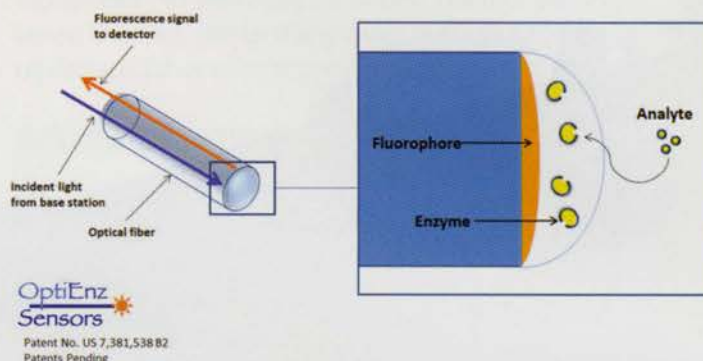
Figure 2. Schematic of the OptiEnz biosensing concept. Enzymes on the biosensor tip catalyze a reaction of the analyte (the chemical of interest), and the change in the levels of reaction products and reactants alters the fluorescence of a chemical layered on the tip.
