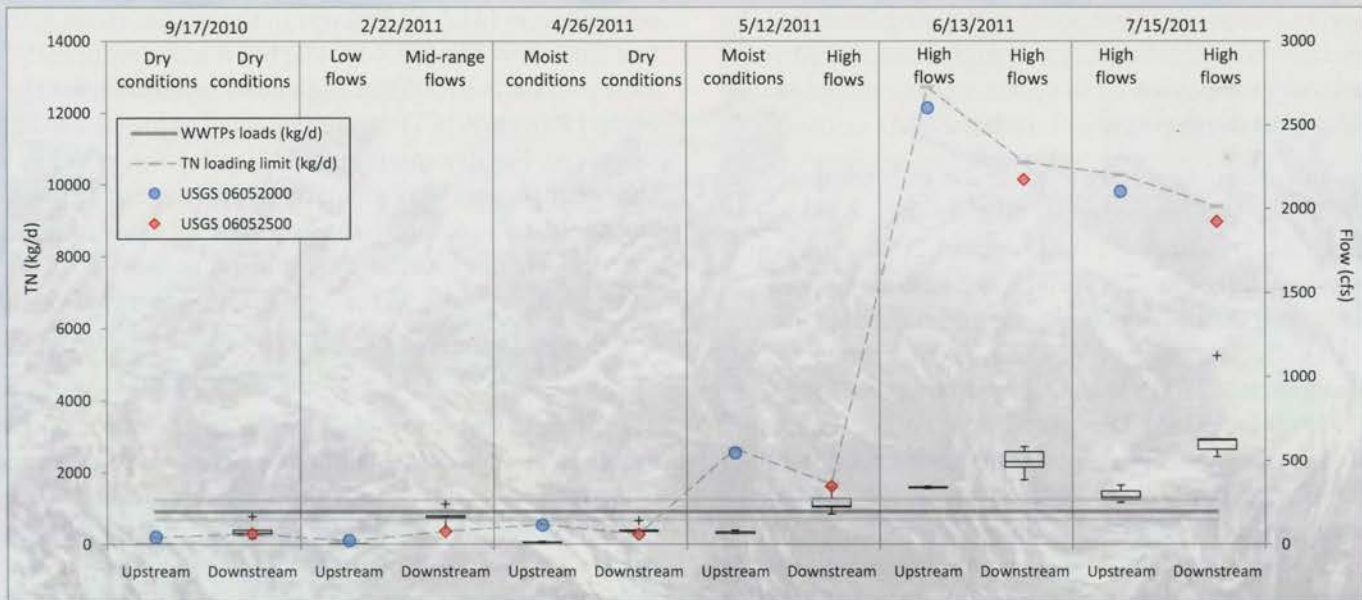
Figure 5. Hydrologic conditions, flows (cfs), the proposed TN loading limit (kg/d), TN loads from WWTPs (kg/d), and estimated TN loads (kg/d) upstream and downstream in the Cache la Poudre River on each event date.
