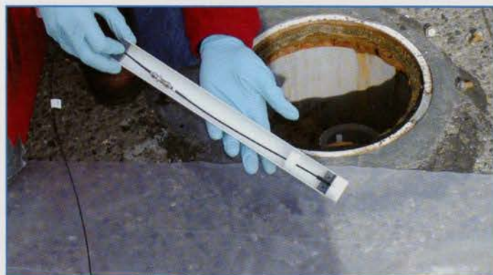
Figure 3. This device was developed to enable the biosensors to be used in groundwater monitoring wells. The plastic housing protects the sensor tip and weights in the bottom, allowing the assembly to be lowered. This apparatus has been used to measure contaminant concentrations at different depths, revealing unexpected stratifications of contamination in an aquifer.
