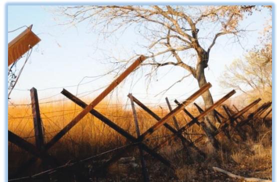
Kellner jetty jacks were installed along the banks and through the floodplain to stabilize and prevent lateral movement of the river channel.
