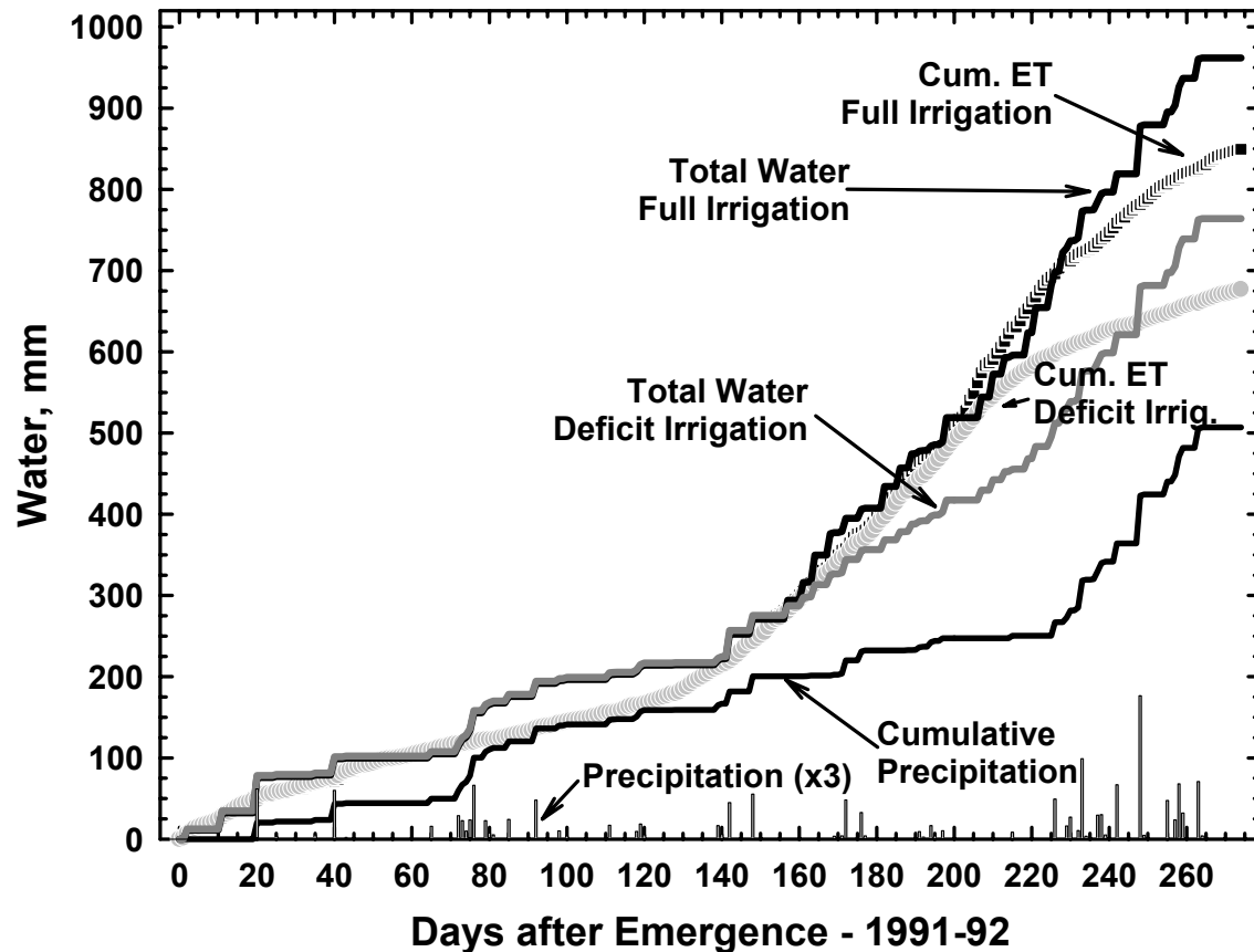
Figure 1. Water balance parameters for the 1991-92 winter wheat growing season (note the rainfall bars were multiplied by 3 to be more visible on the scale).
