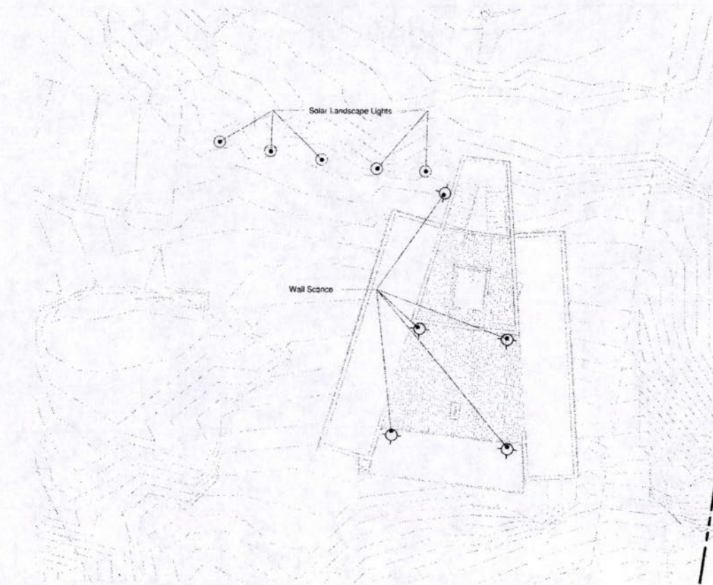
3 EXTERIOR LIGHTING PLAN 1" = 10'-0"
