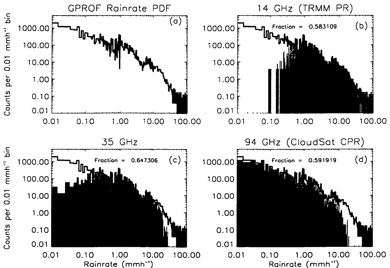
Figure D.5: (a) PDF of near-surface rainrate for the entire GPROF algorithm. (b)-(d) Fraction of profiles for which the reflectivity return from near-surface rainfall exceeds the radar minimum detectable signal for the TRMM PR, a hypothetical second frequency (35 GHz) on GPM, and the CloudSat CPR.
