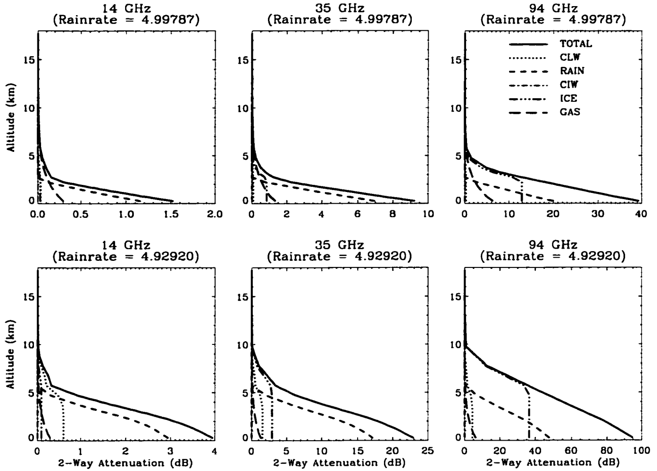
Figure D.11: Profiles of attenuation at 14, 35, and 94 GHz from each of the GPROF hydrometeor classes for two distinct profiles of rainfall both characterized by the same surface rainrate ( 5 \text{ mmh}^{-1} ).
