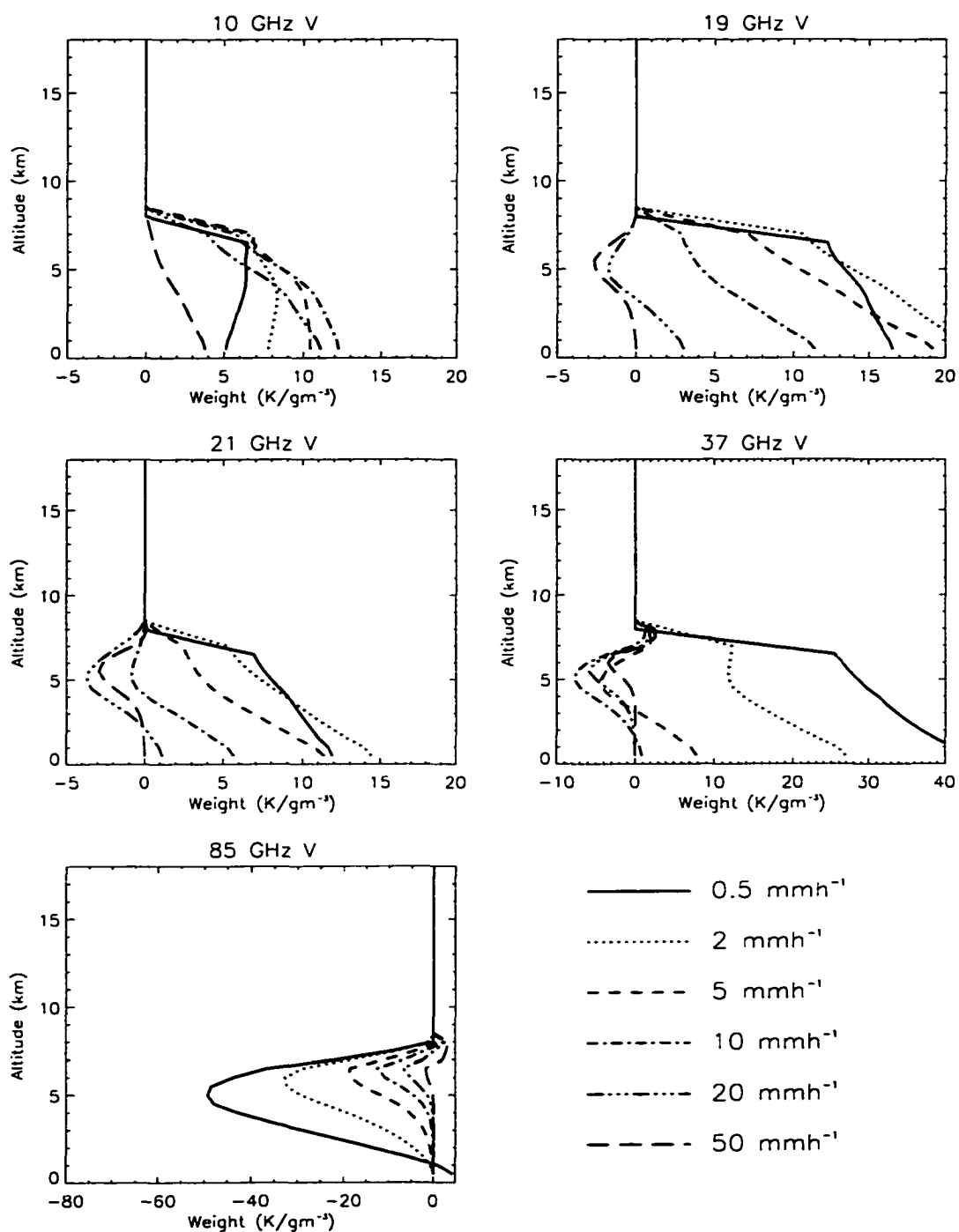
Figure 2.13: Liquid water weighting functions for each vertically polarized TMI channel as a function of rainrate over an ocean background.
