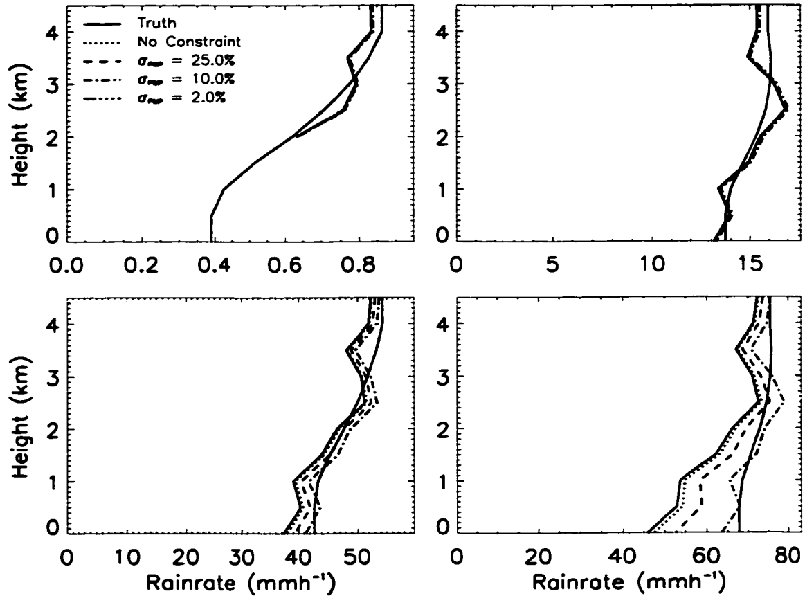
Figure D.25: Sample rainfall retrievals at 14 GHz.
