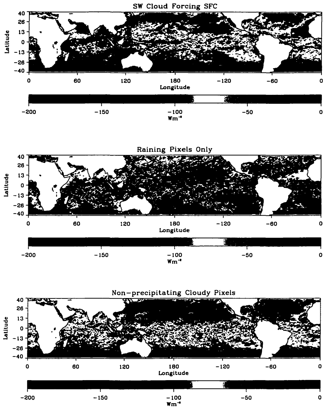
Figure 5.33: As in Figure 5.32 but for surface shortwave cloud forcing.
