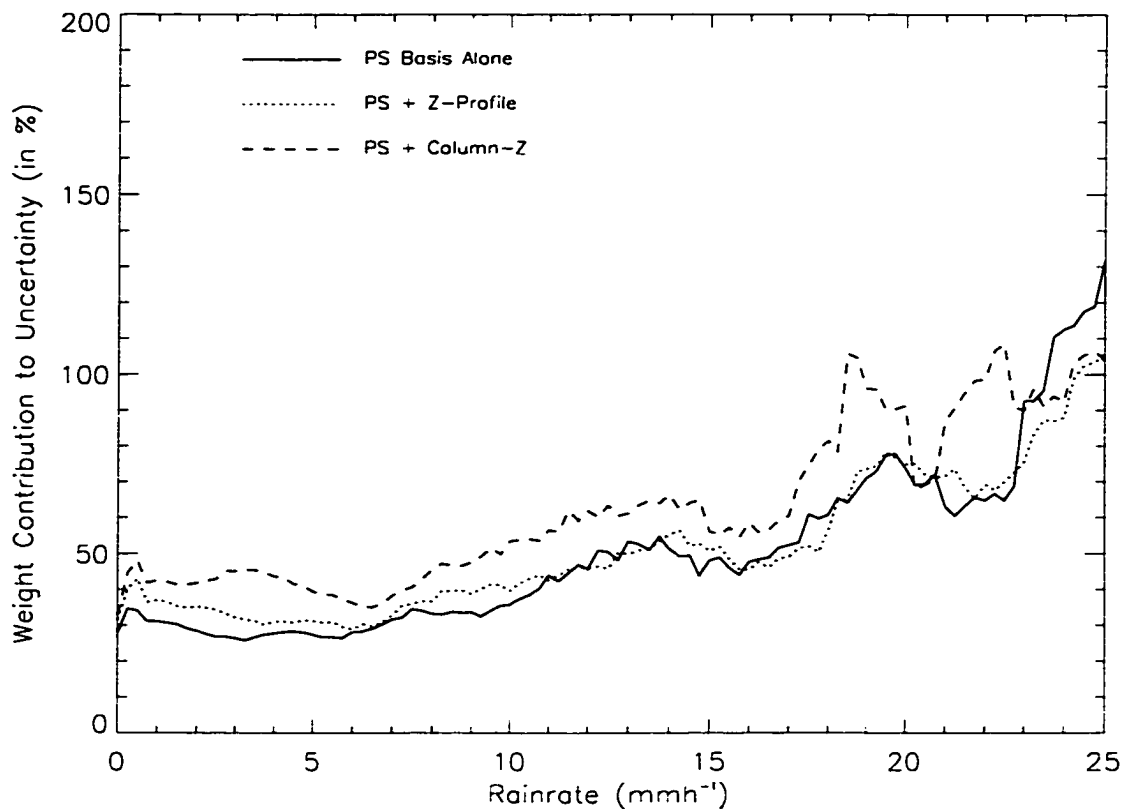
Figure 3.27: As in Figure 3.25 but for the weight component to the uncertainty.
