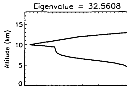
Figure 2.26: As in Figure 2.25 but at a rainrate of 20 \text{ mmh}^{-1} .
