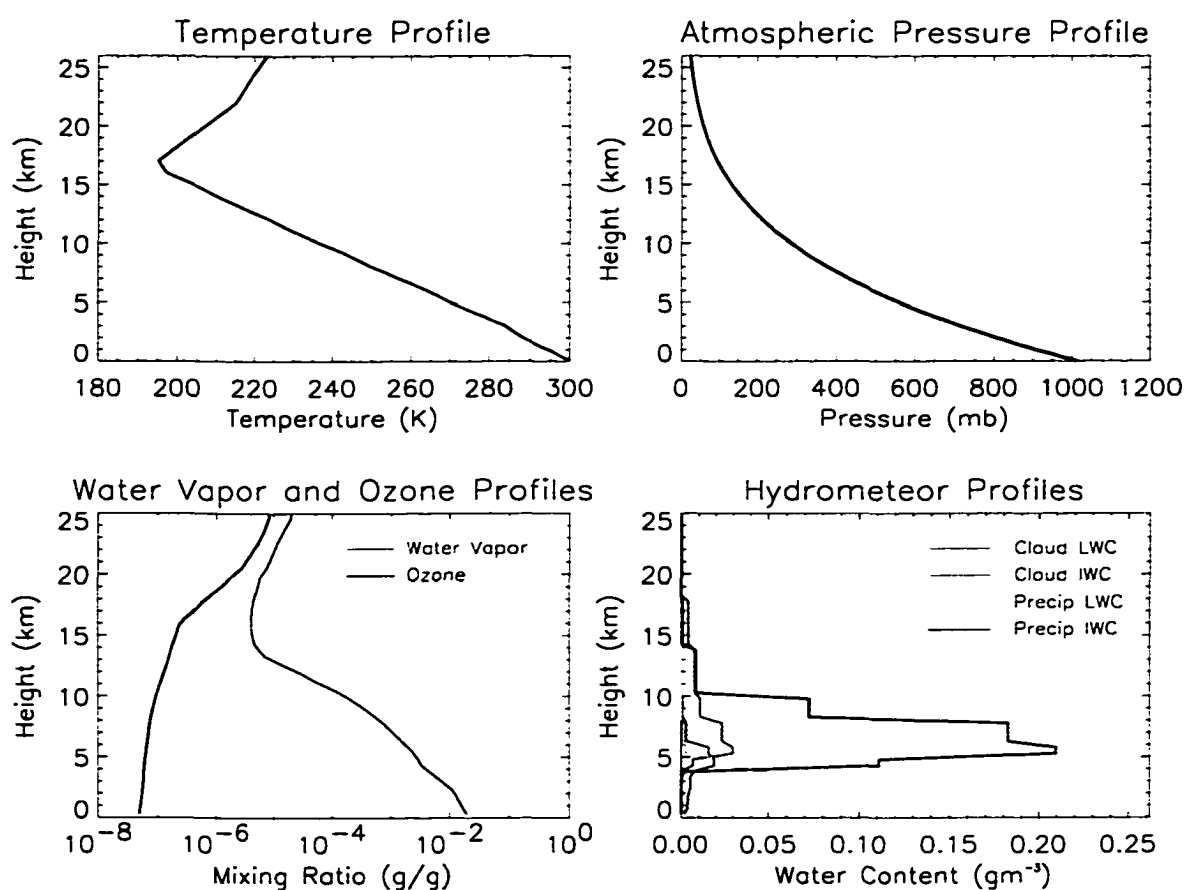
Figure 5.15: Inputs to the radiative transfer model for the light rain case.
