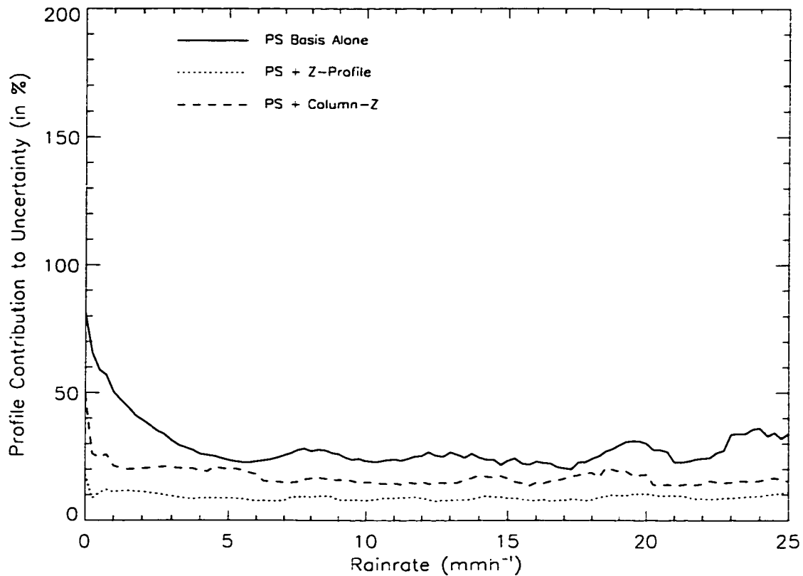
Figure 3.26: As in Figure 3.25 but for the profile database component to the uncertainty.
