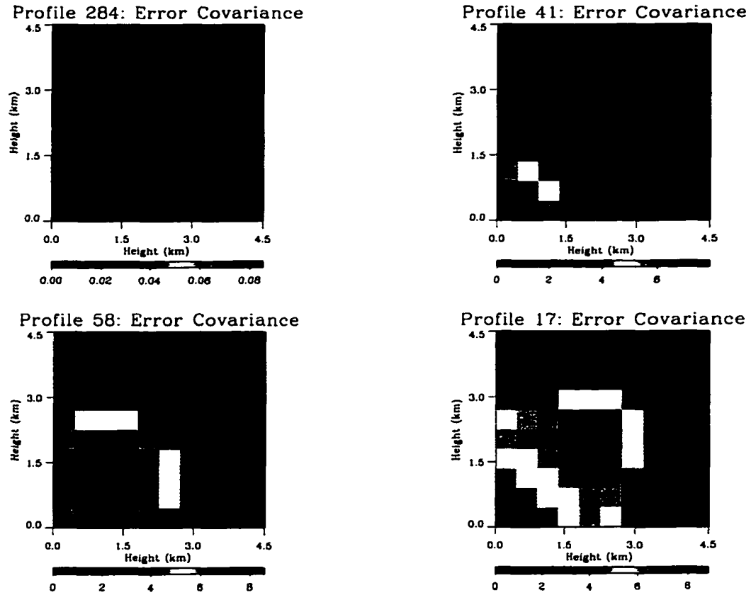
Figure D.27: Retrieval covariance matrices for synthetic retrievals at 94 GHz. All elements have been normalized by the appropriate retrieved rainrate and therefore represent fractional uncertainties.
