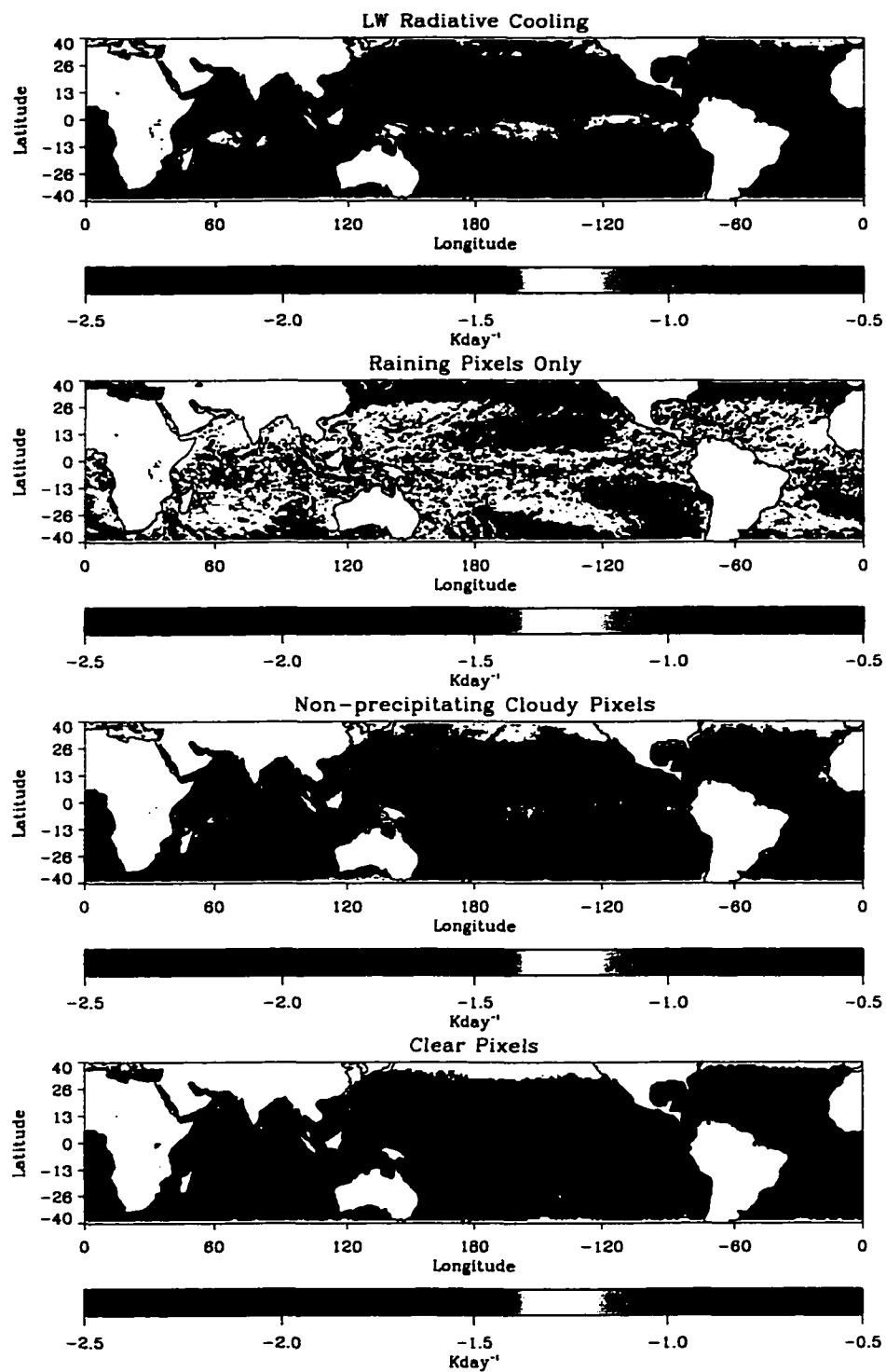
Figure 5.30: Monthly mean column-integrated longwave cooling for February 1998.
