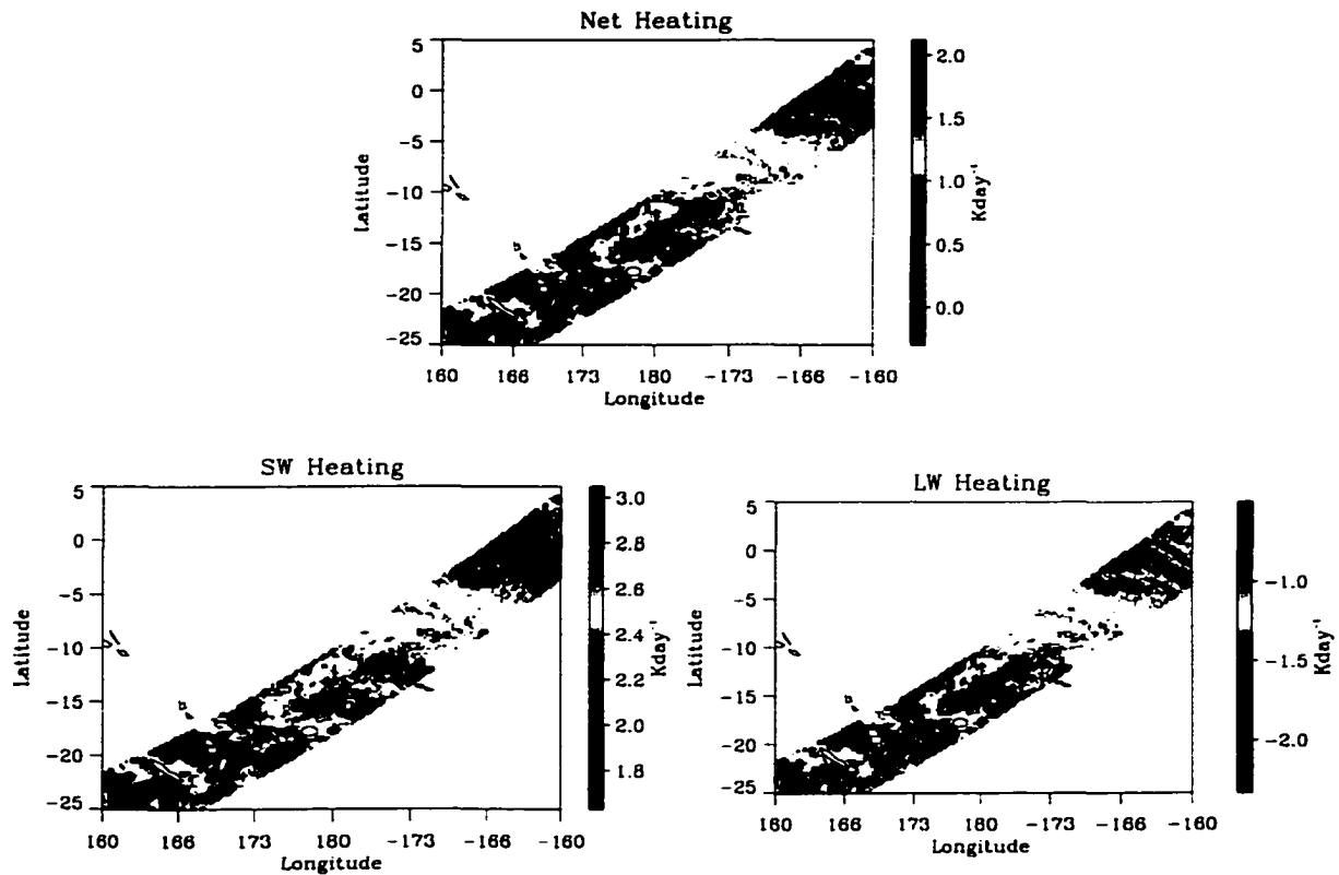
Figure 5.10: As in Figure 5.8 but for column-integrated SW, LW, and Net radiative heating.
