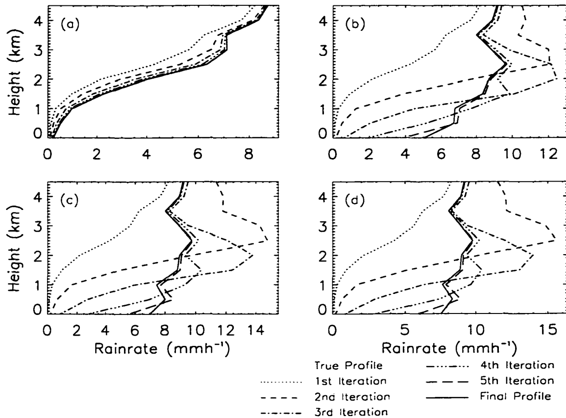
Figure D.33: Iterations in a synthetic retrieval at 94 GHz with (a) no constraint, (b) a constraint with \sigma_{PWP} = 25.0 , (c) a constraint with \sigma_{PWP} = 10.0 , and (d) a constraint with \sigma_{PWP} = 2.0 .
