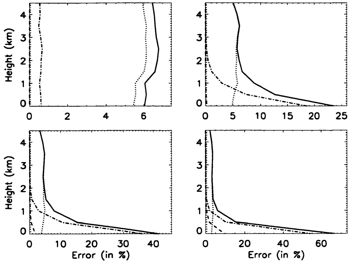
Figure D.29: The measurement (dotted line), a priori (dashed line), and PWP constraint (dot-dashed line) contributions to the total error (solid line) in the retrievals from Figure D.26 assuming a constraint accuracy of 10%.
