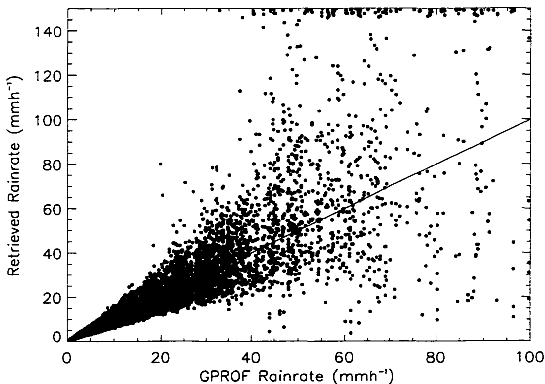
Figure D.35: Synthetic retrievals at 14 GHz as in Figure D.15 but assuming 6 dB errors.
