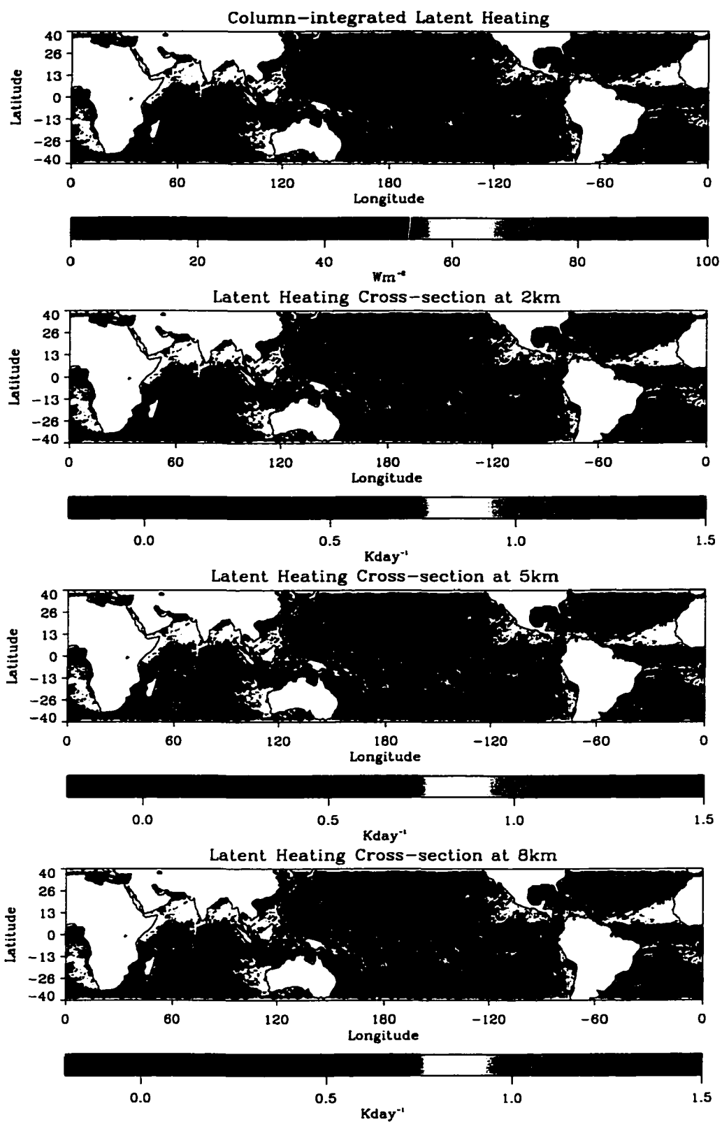
Figure C.2: Monthly mean column latent heating and cross-sections at 2.0, 5.0, and 8.0 km as retrieved by GPROF.
