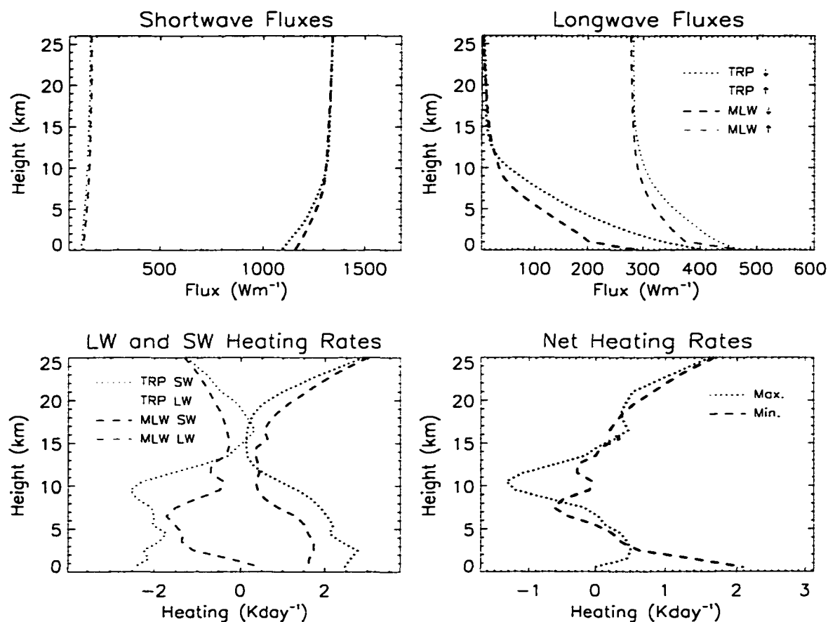
Figure 5.4: Clear-sky radiative flux and heating rate profiles for a standard tropical (TRP) and midlatitude winter (MLW) profiles of temperature and relative humidity.
