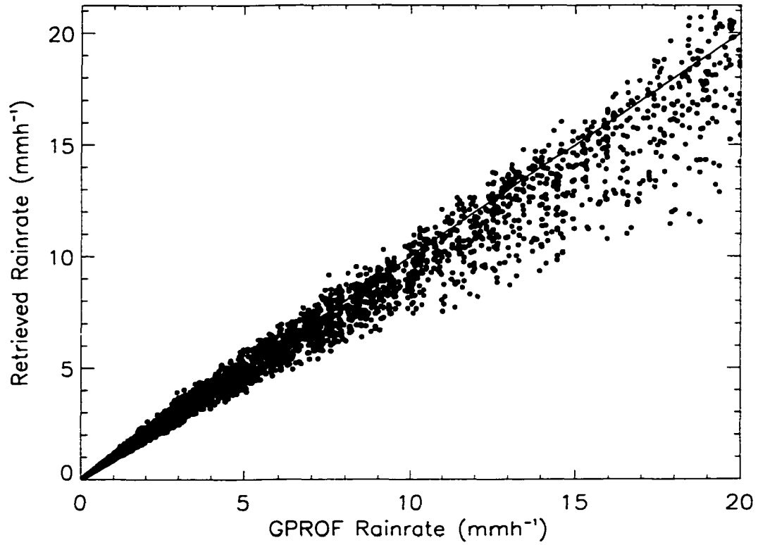
Figure D.21: As in Figure D.16 but at an altitude of 4.0 km.
