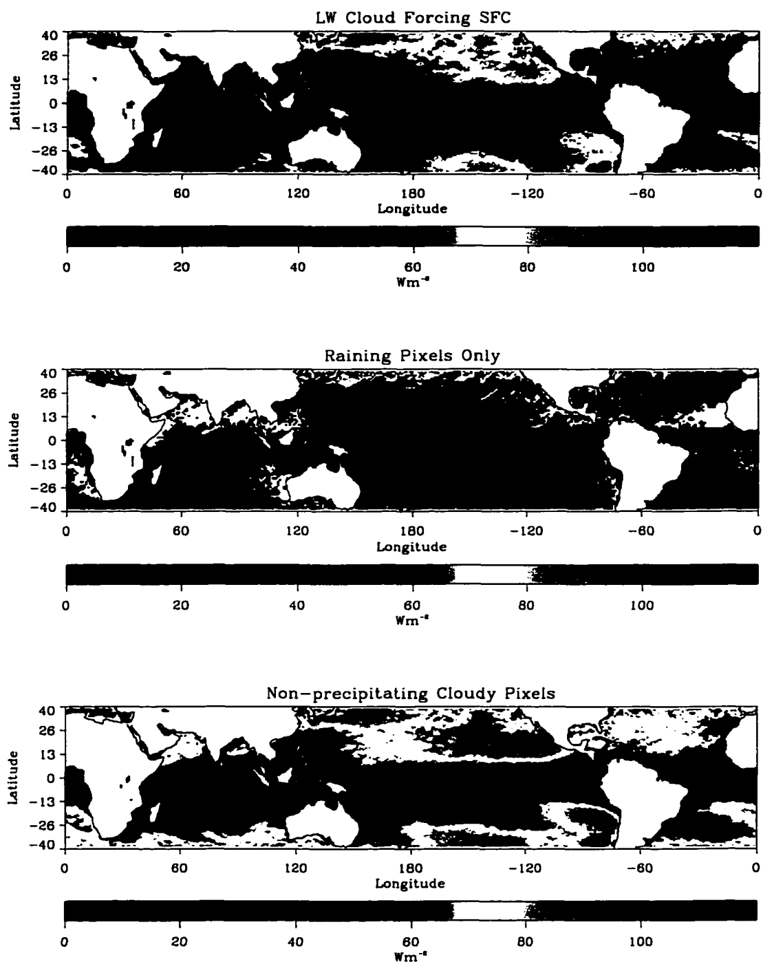
Figure 5.29: As in Figure 5.28 but for surface longwave cloud forcing.
