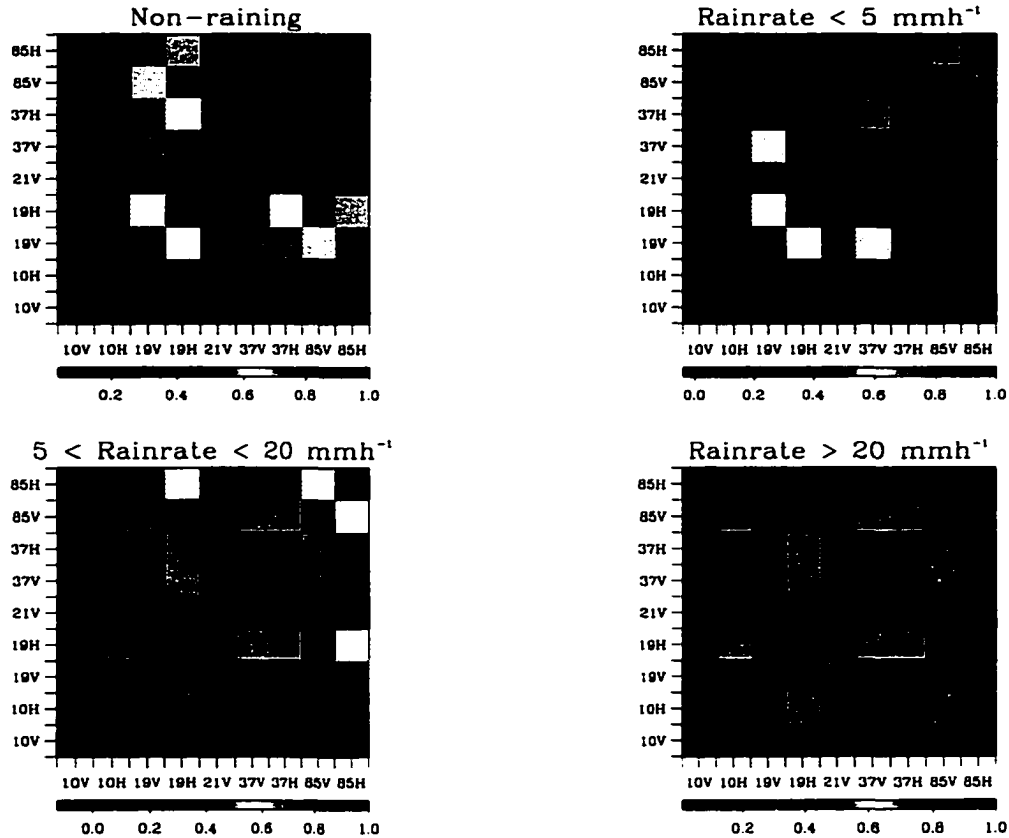
Figure 3.4: Correlation matrix for the 9 TMI channels.
