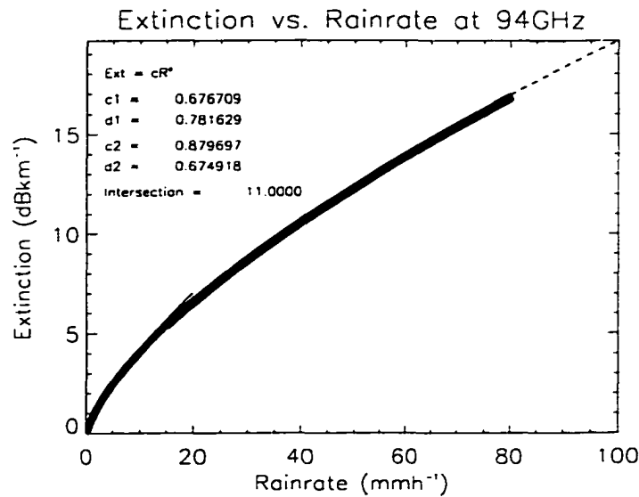
Figure D.13: Extinction vs. rainrate for a MP distribution of spherical raindrops.
