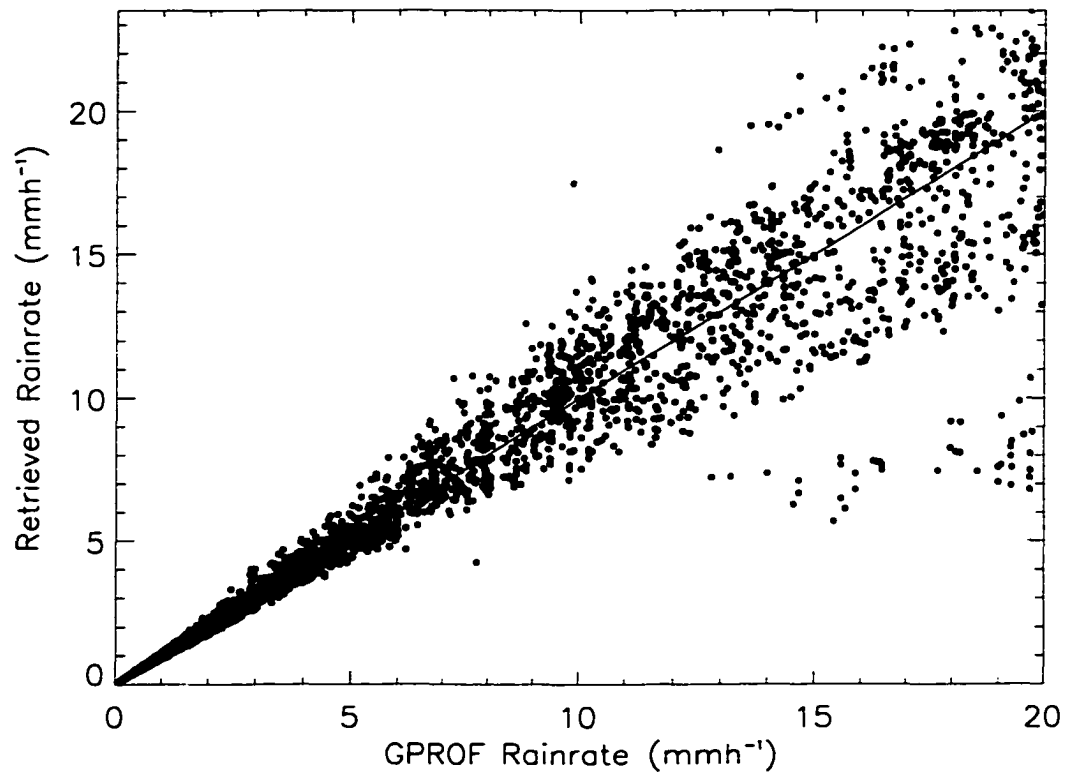
Figure D.24: Constrained synthetic near-surface rainfall retrievals at 14 GHz.
