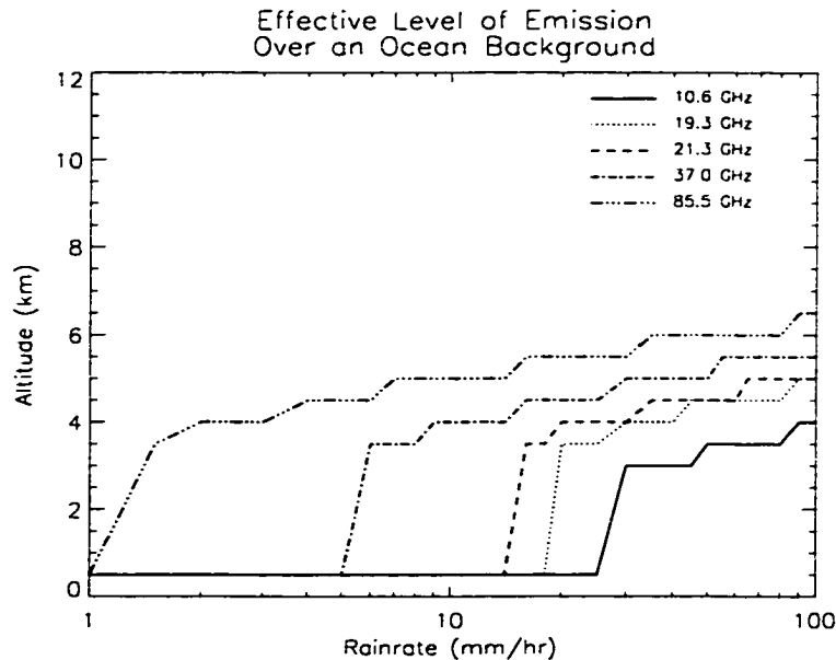
Figure 2.11: TMI effective levels of emission as a function of rainrate over an ocean background.
