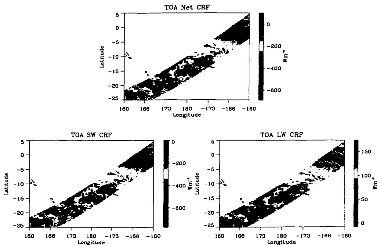
Figure 5.8: LW, SW, and net cloud radiative forcing at the TOA for a small section of orbit.
