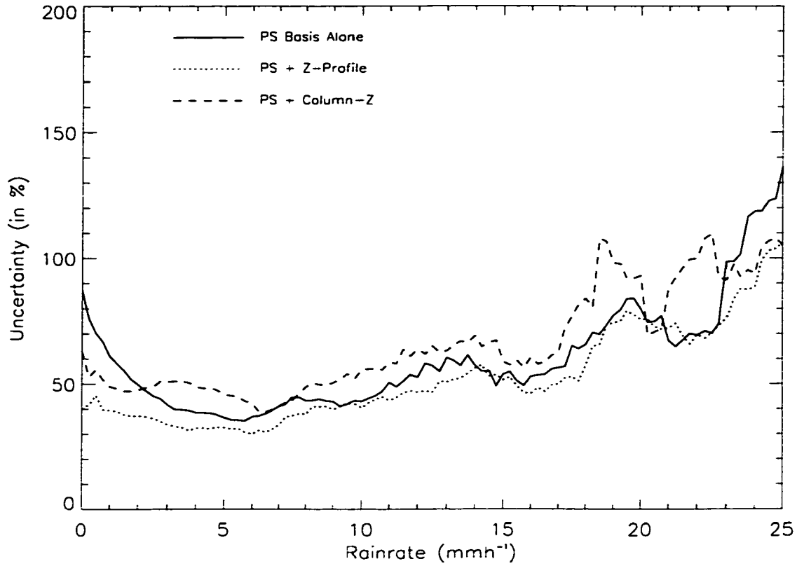
Figure 3.25: Total error in retrieved surface rainrate without PR data (solid), with the addition of a full PR reflectivity profile (dotted), and with the addition of a column-integrated reflectivity (dashed).
