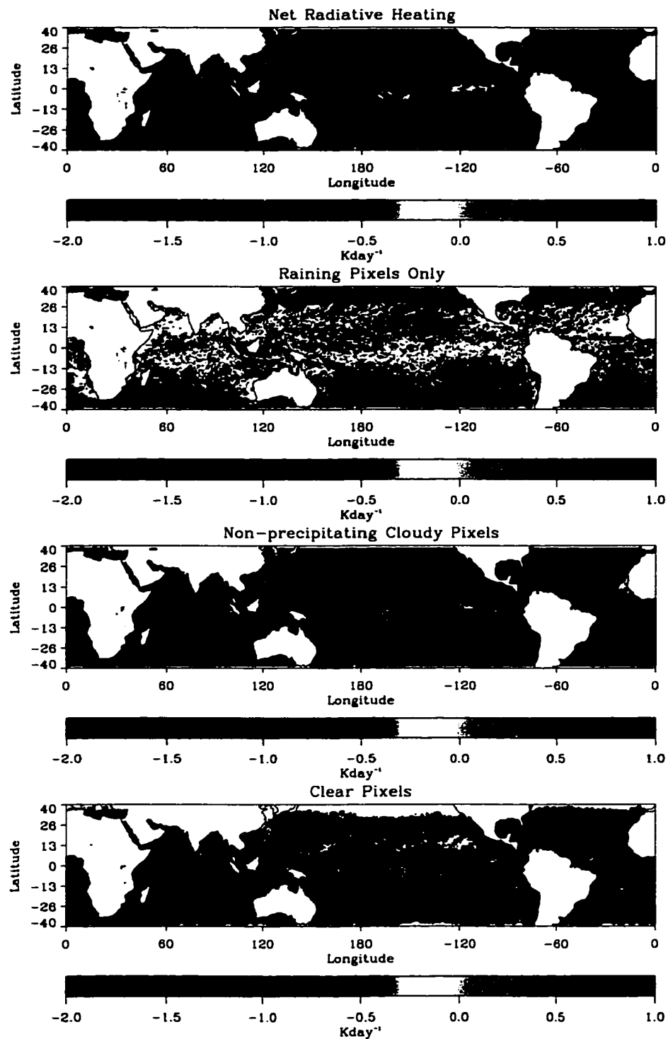
Figure 5.37: As in Figure 5.30 but for net heating.
