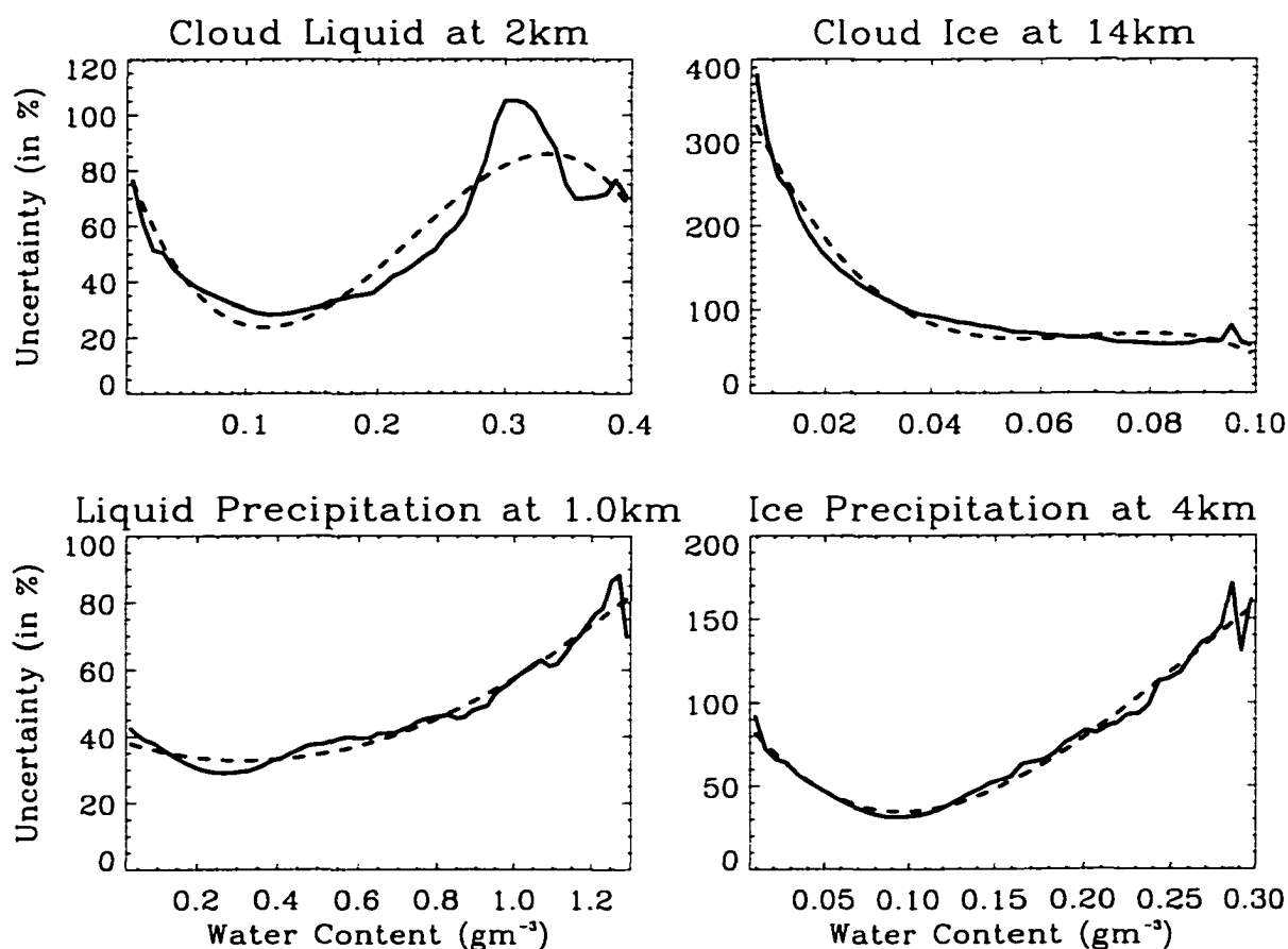
Figure 3.16: Sample third order polynomial fits to GPROF retrieval error for all four hydrometeor classes.
