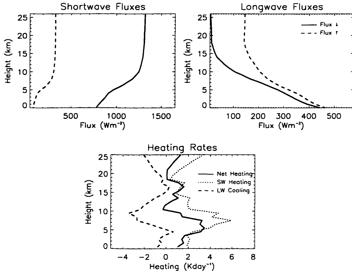
Figure 5.16: Flux and radiative heating rate profiles derived from the input shown in Figure 5.15.
