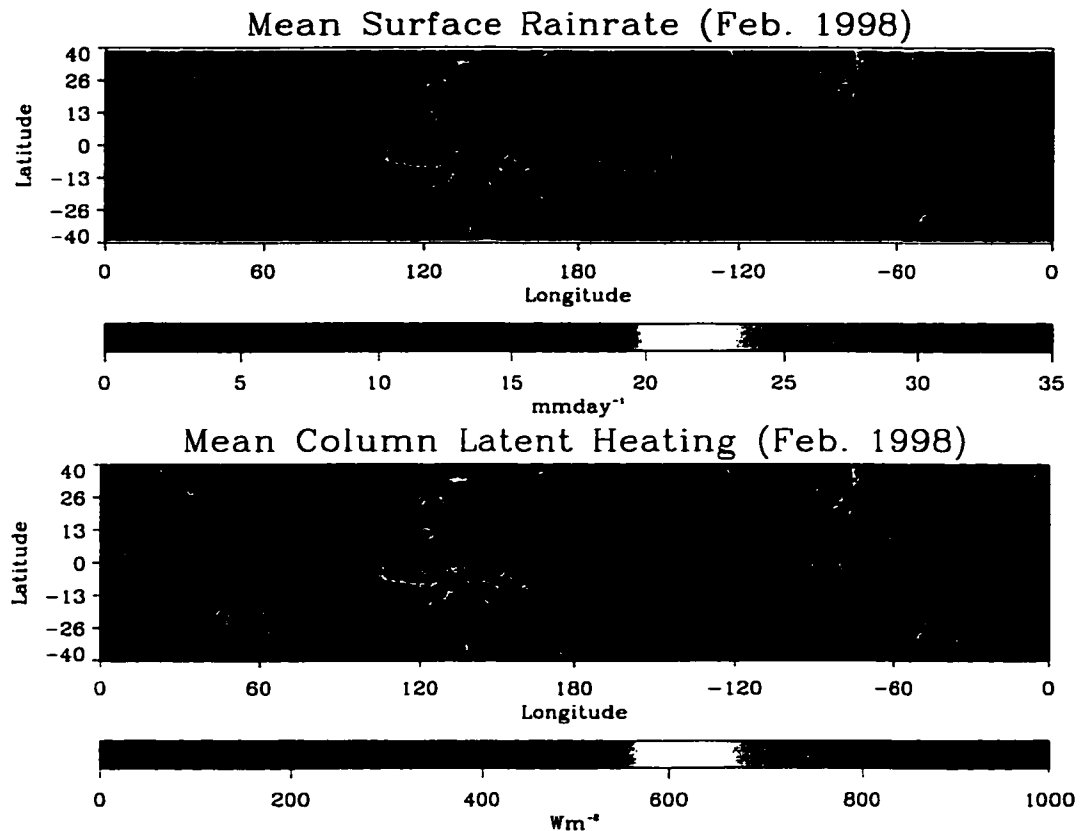
Figure C.3: GPROF monthly mean rainfall and associated column-integrated latent heat release for February 1998.
