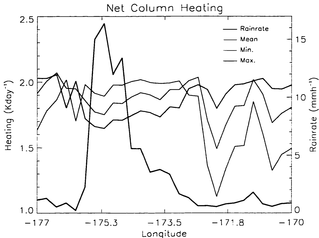
Figure 5.25: Range in estimates of column heating induced by GPROF retrieval uncertainties. Max. and Min. refer to the maximum and minimum perturbations in liquid and ice water contents, respectively.
