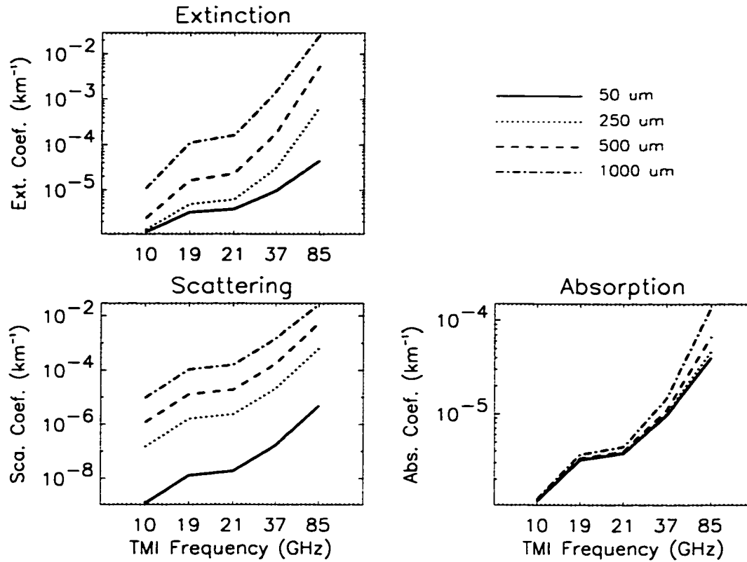
Figure 2.3: As in Figure 2.2 but for ice spheres.
