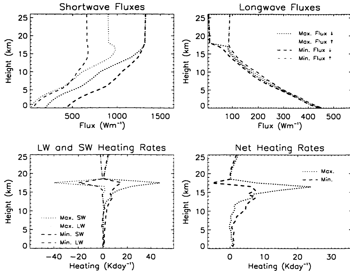
Figure 5.24: As in Figure 5.23 but in moderate rainfall.
