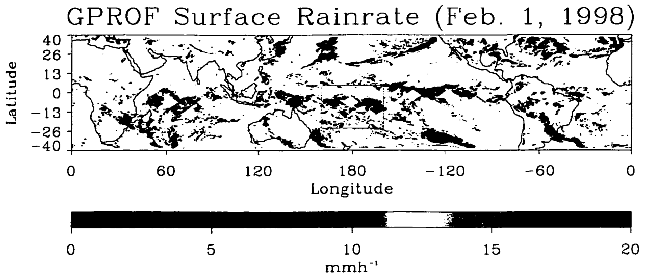
Figure 4.1: GPROF surface rainrate estimates from February 1, 1998. Results from the remainder of this chapter will focus on the region indicated by the gray box.
