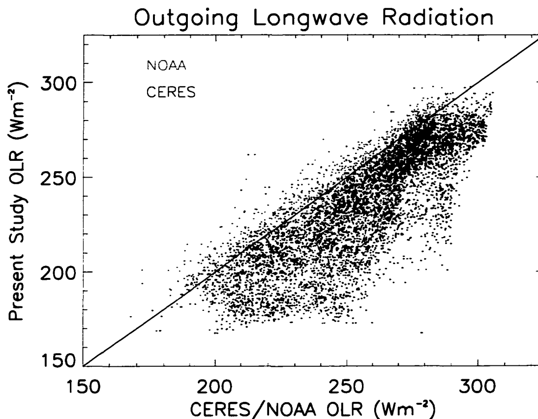
Figure 5.41: Scatter plot of derived monthly-mean OLR versus equivalent NOAA and CERES products.
