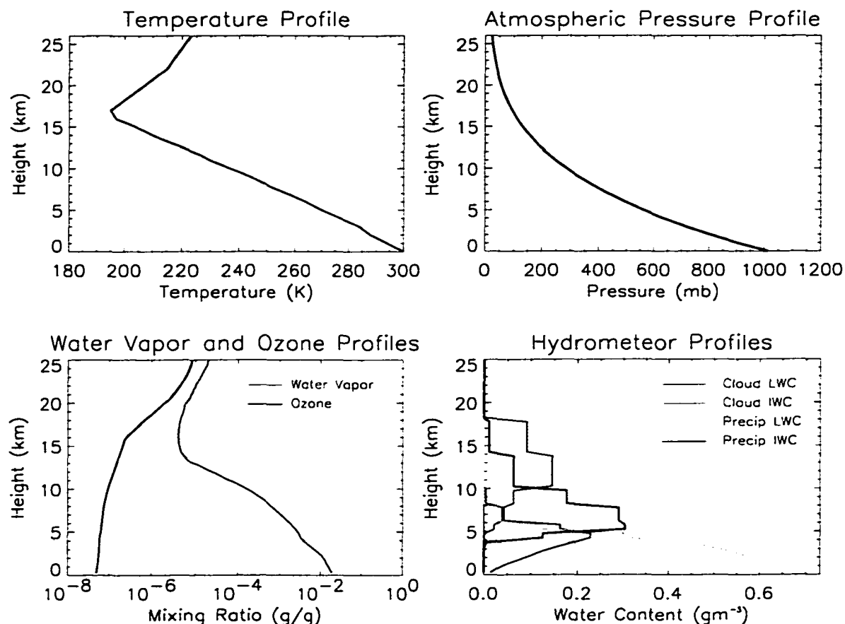
Figure 5.17: Inputs to the radiative transfer model for the moderate rain case.
