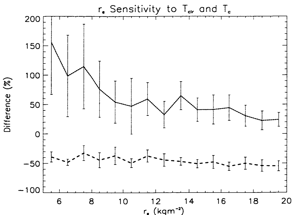
Figure 4.11: Expected range of uncertainty in r_e estimates resulting from required assumptions on T_{clr} and T_c .
