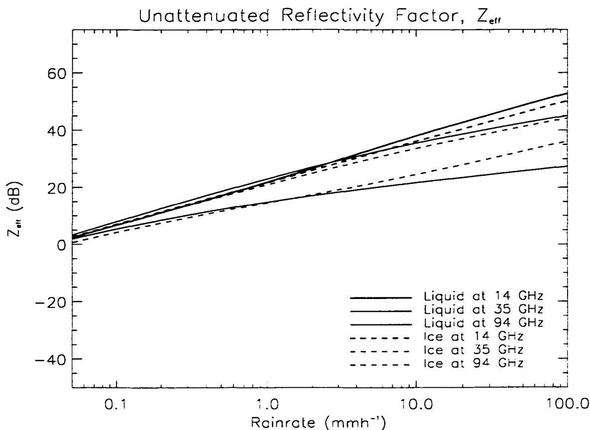
Figure D.2: Effective reflectivity factors as a function of rainrate at 14, 35, and 94 GHz in the absence of attenuation.
