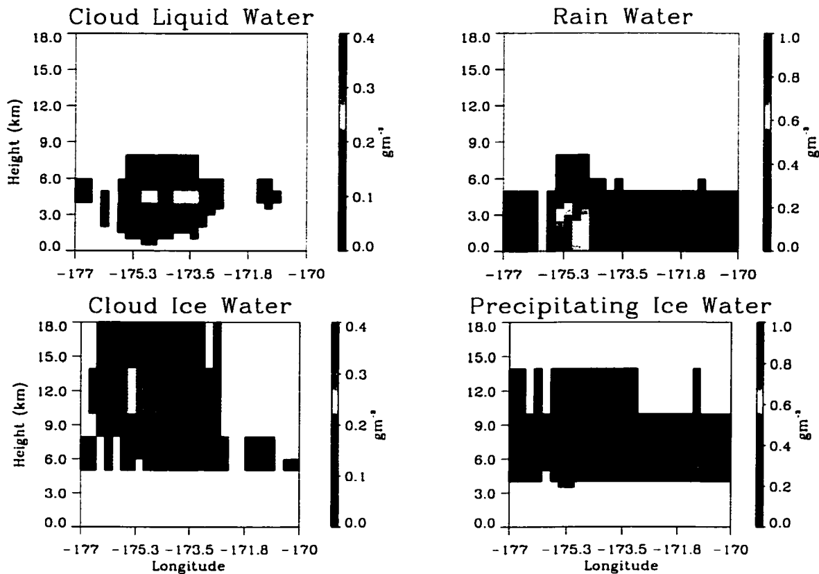
Figure 4.3: Longitude-height cross-sections of cloud liquid, cloud ice, precipitating liquid, and precipitating ice at 8°S from the GPROF algorithm.
