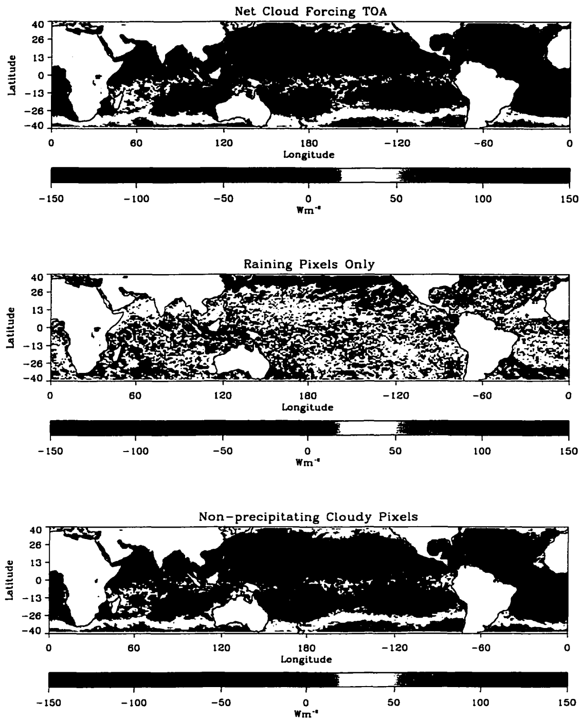
Figure 5.35: Monthly-mean net cloud forcing at the top of the atmosphere for February 1998.
