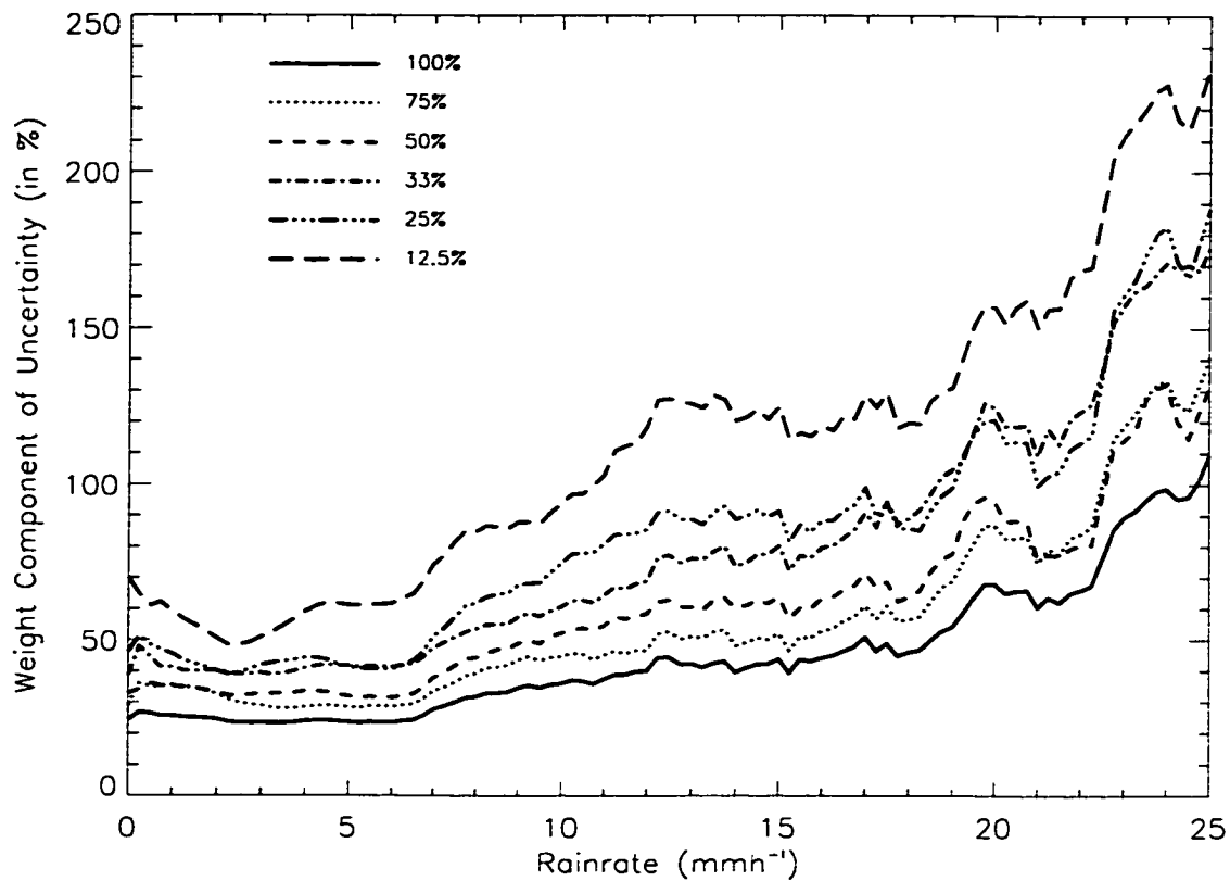
Figure 3.29: The component of the uncertainties plotted in Figure 3.28 owing to errors in measurement and radiative transfer modeling.
