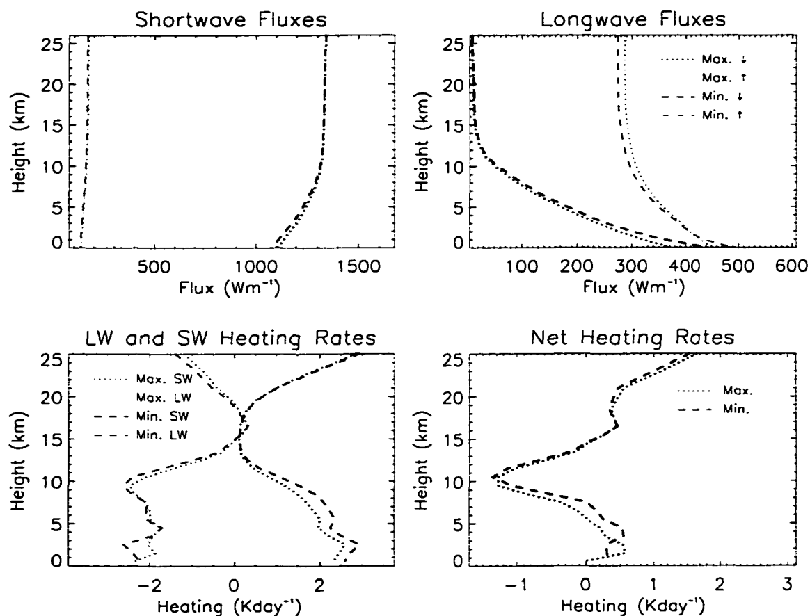
Figure 5.3: Sensitivity of radiative flux and heating rate profiles to errors in CWV and SST under cloud-free conditions.
