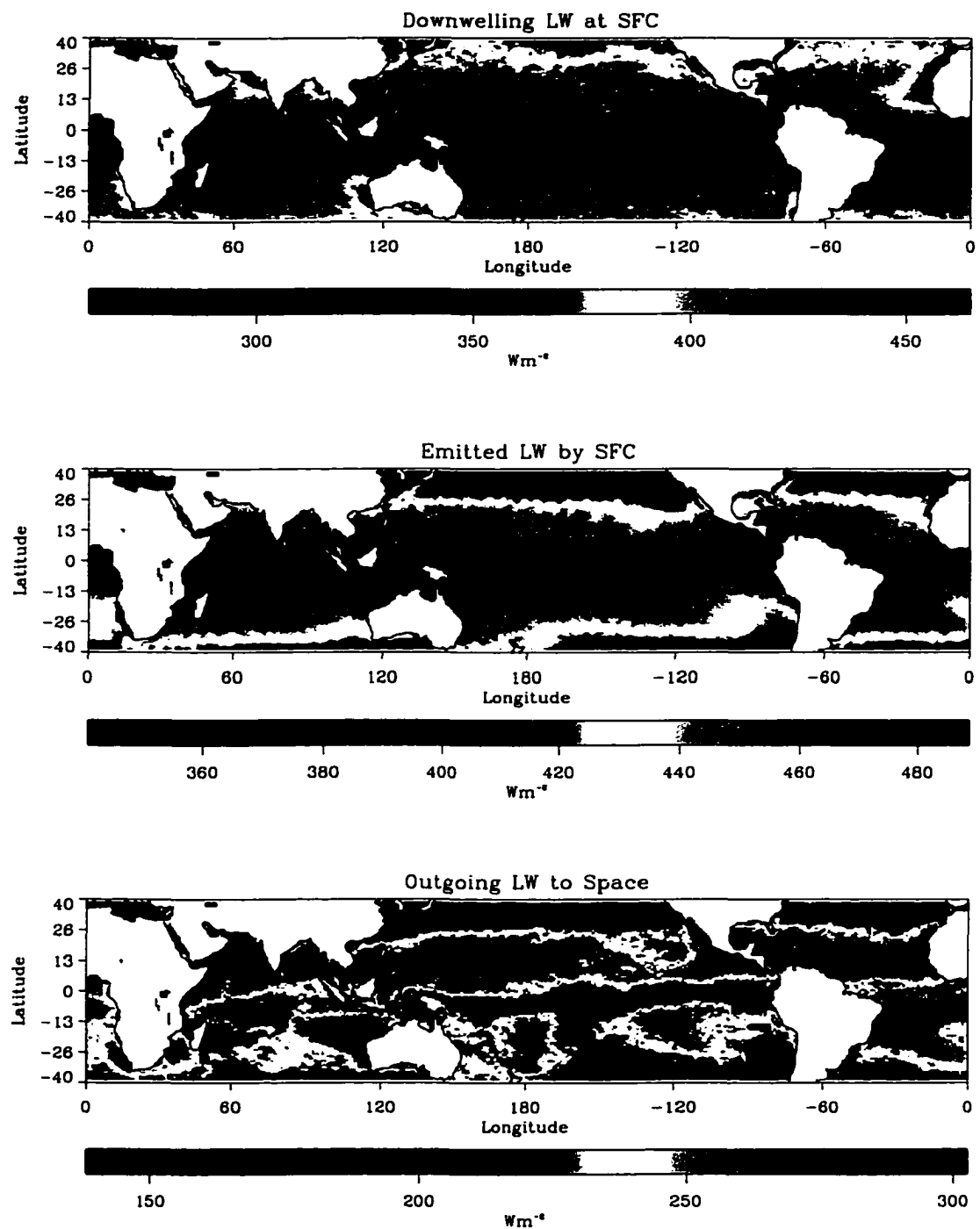
Figure 5.27: Monthly-mean LW fluxes for February 1998.
