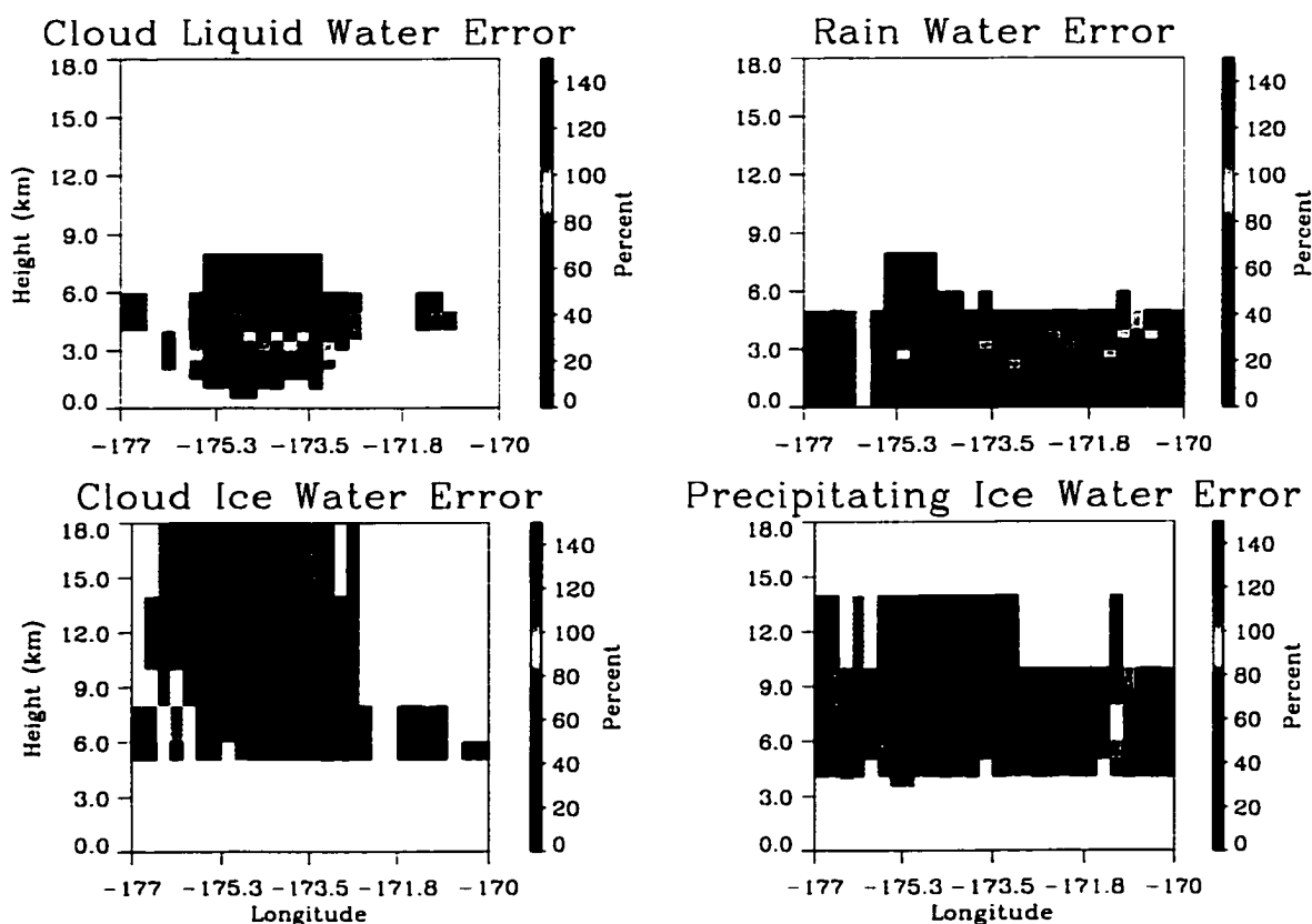
Figure 4.4: Uncertainties in the hydrometeor cross-sections presented in Figure 4.3.
