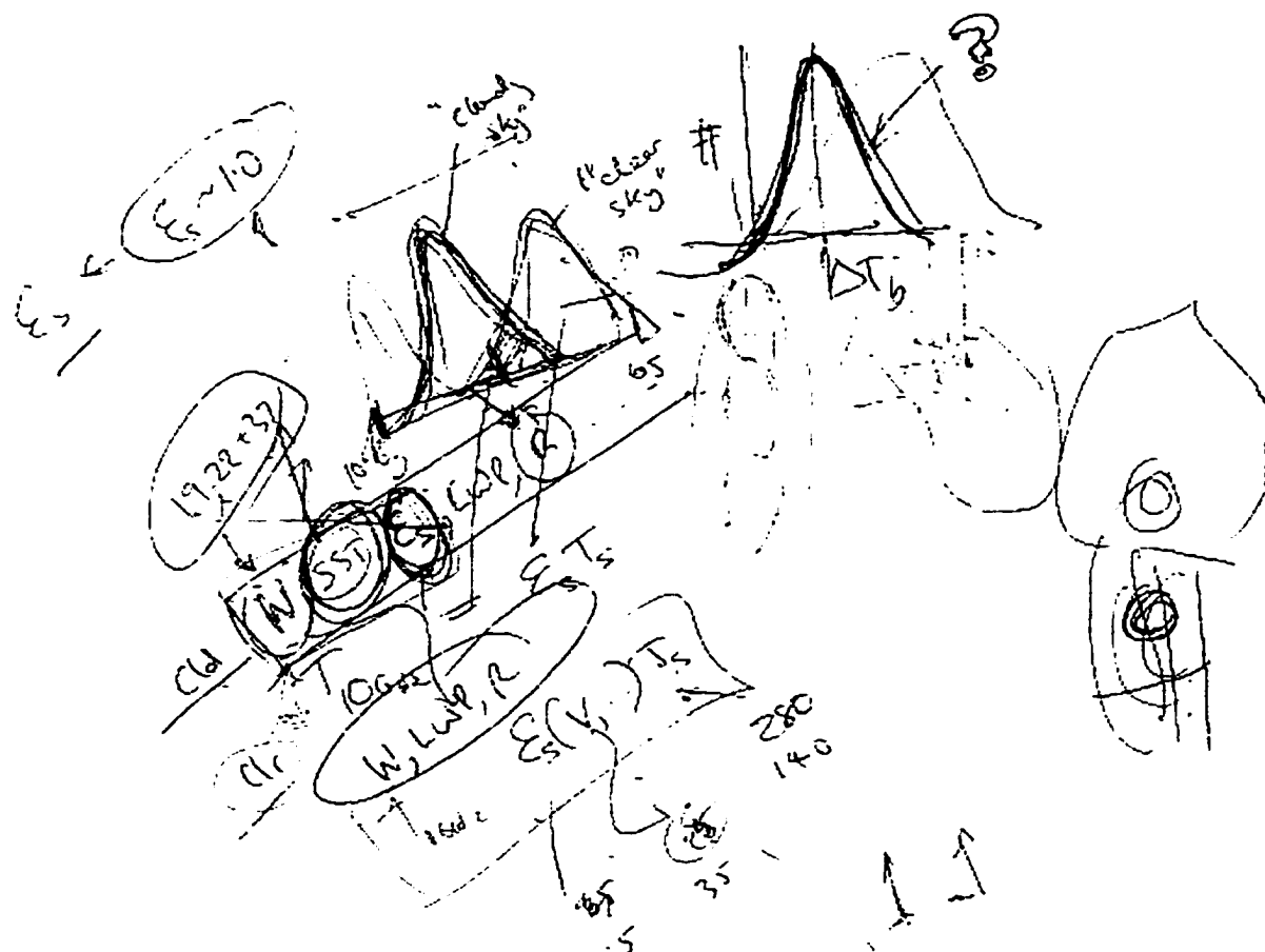
Figure 1.3: Schematic outline of the dissertation (from a personal communication with Dr. Graeme Stephens, early 1998).
