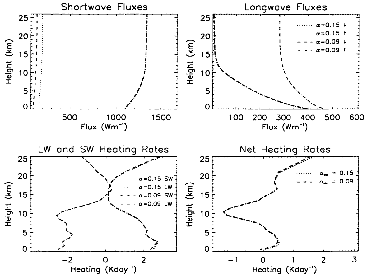
Figure 5.2: Sensitivity of clear-sky radiative fluxes and heating rates to ocean albedo.
