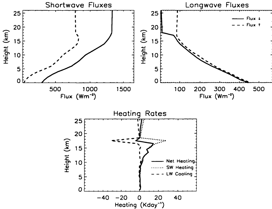
Figure 5.18: Flux and radiative heating rate profiles derived from the input shown in Figure 5.17.
