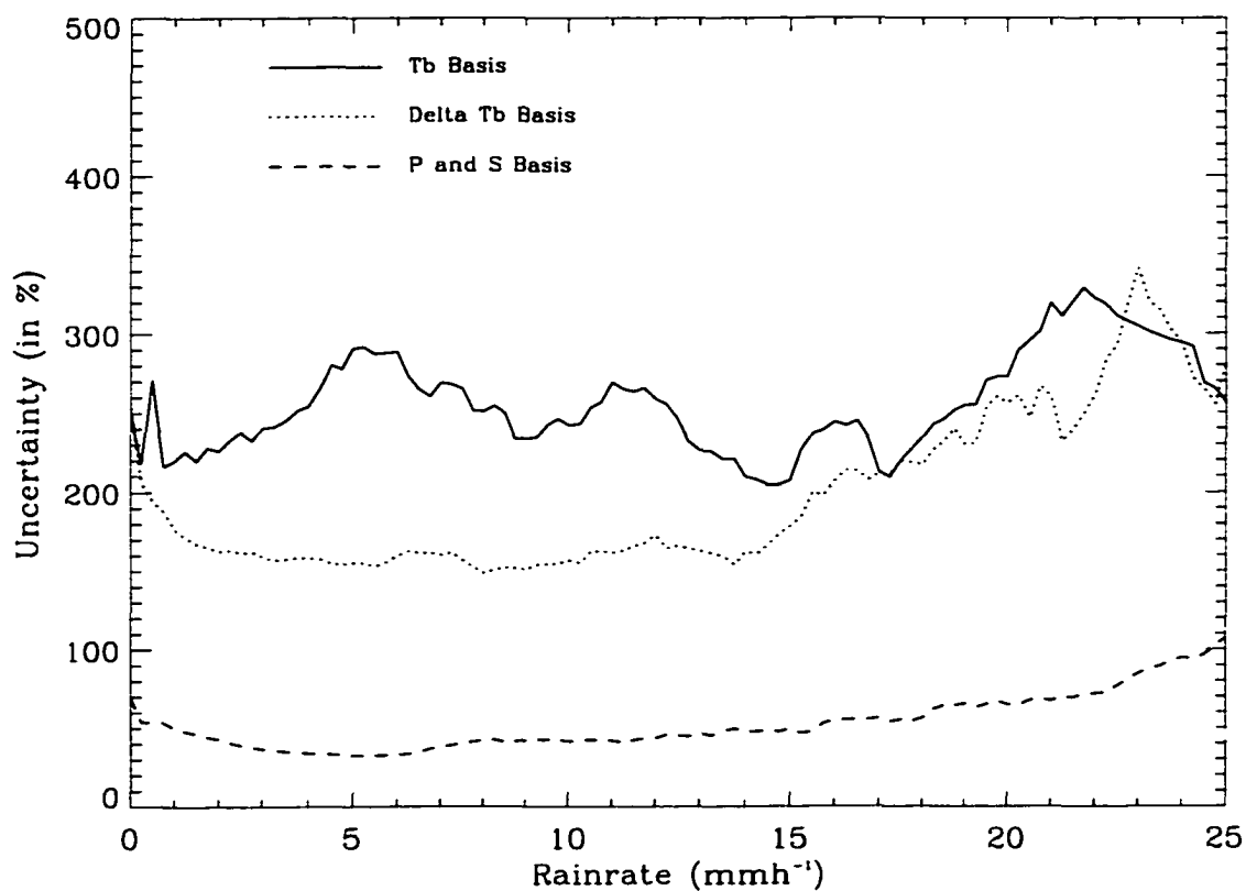
Figure 3.20: Comparison of retrieval uncertainty as a function of rainrate using raw T_B s (solid), vertical minus horizontal T_B differences (dotted), and emission and scattering indices (dashed).
