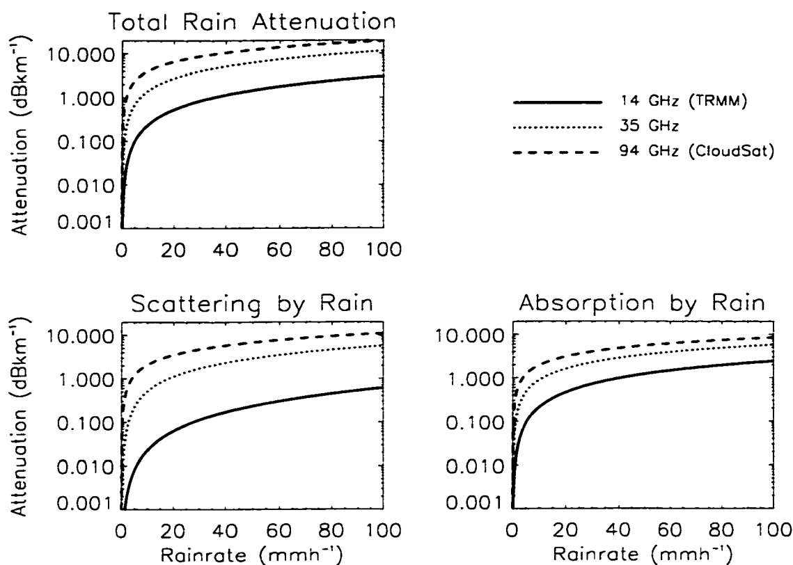
Figure D.3: Attenuation and its scattering and absorption components in \text{dBkm}^{-1} for liquid rain assuming a Marshall-Palmer DSD at 14, 35, and 94 GHz.
