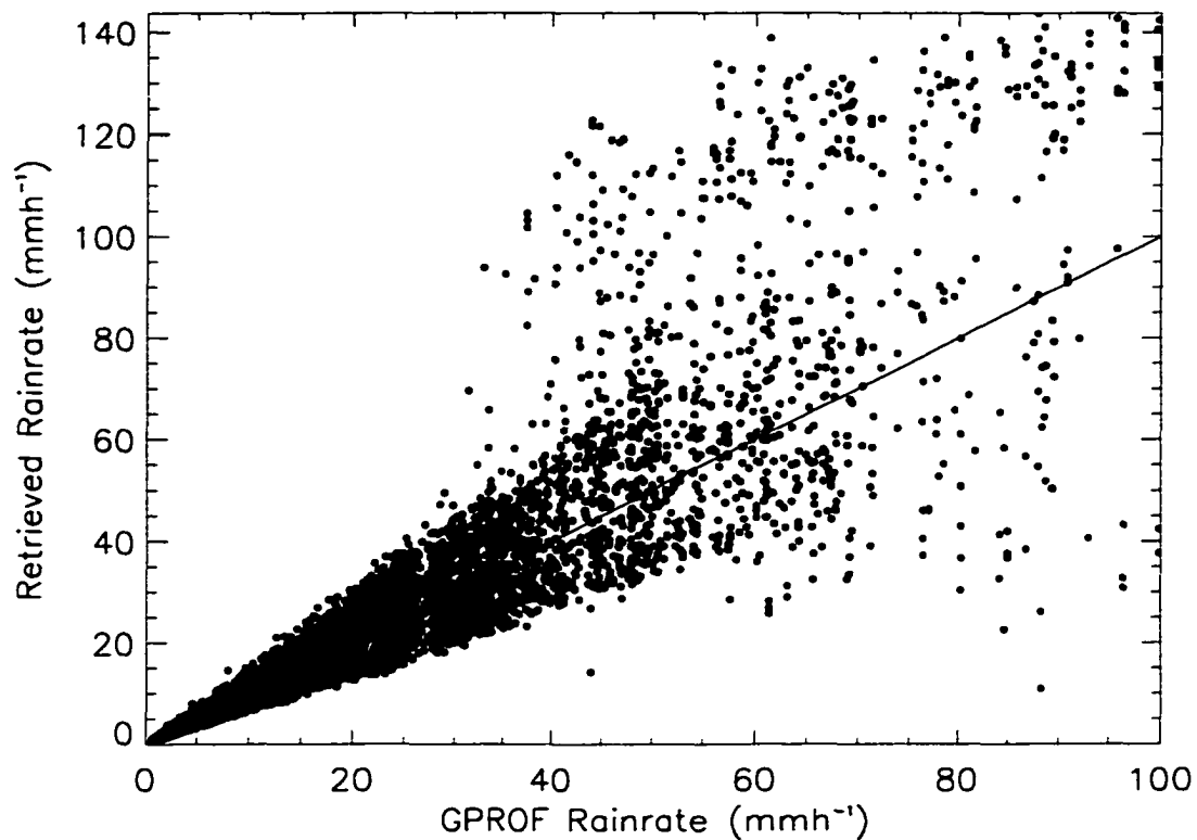
Figure D.36: As in Figure D.35 but with a PIA estimate accurate to 10 %.
