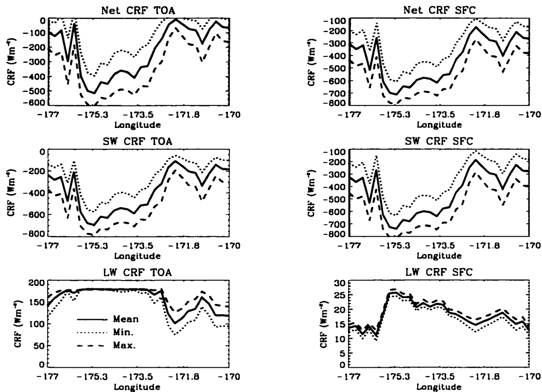
Figure 5.26: As in Figure 5.25 but corresponding to CRF estimates.
