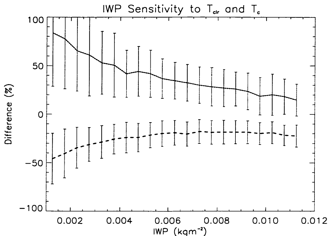
Figure 4.12: As in Figure 4.11 but for IWP.
