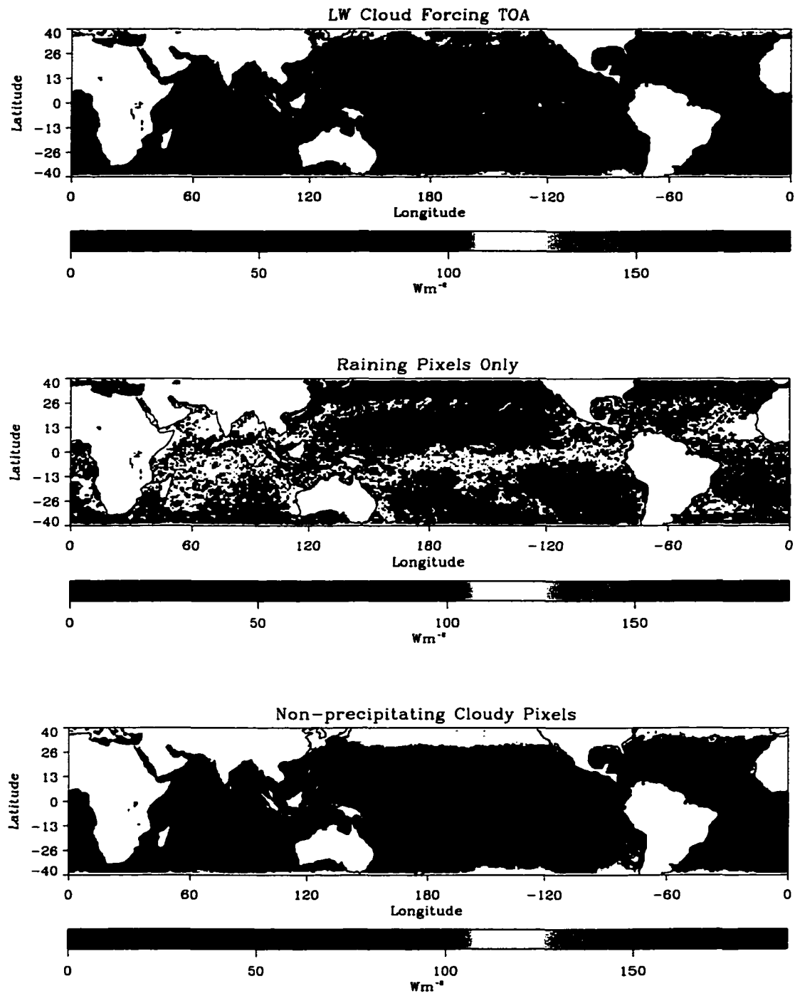
Figure 5.28: Monthly-mean longwave cloud forcing at the top of the atmosphere for February 1998.
