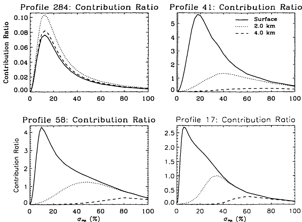
Figure D.32: As in Figure D.30 but for varying strengths of PIA constraint.
