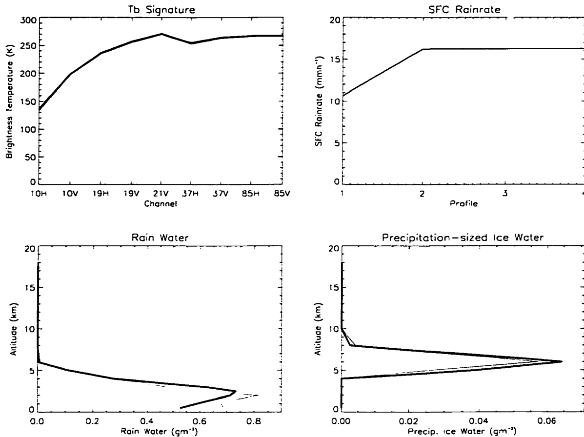
Figure 3.24: As in Figure 3.8 after including the corresponding PR reflectivity profile.
