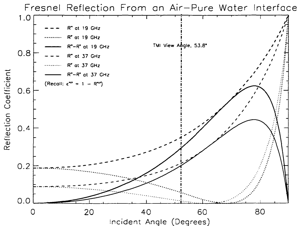
Figure 4.13: Reflection coefficients, R^{V,H} , at 19 and 37 GHz for reflection from a horizontal, smooth air-pure water interface at 295 K.
