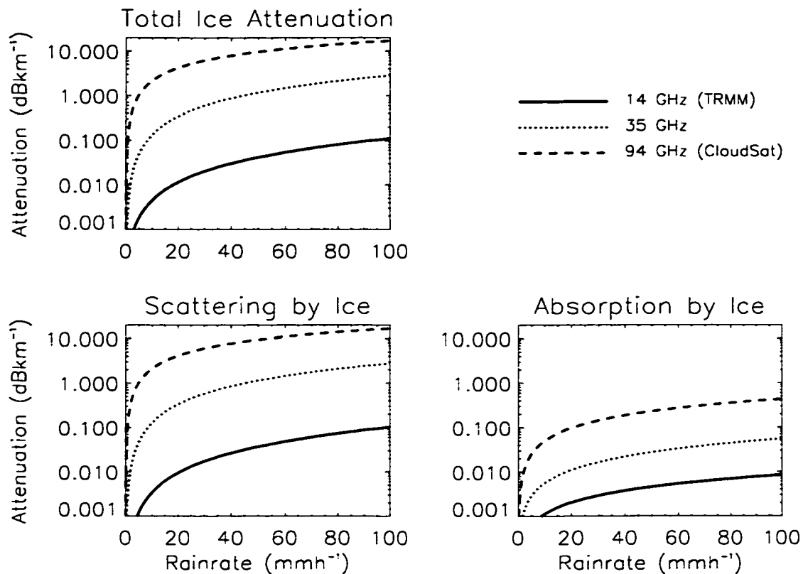
Figure D.4: As in Figure D.3 but for frozen hydrometeors.
