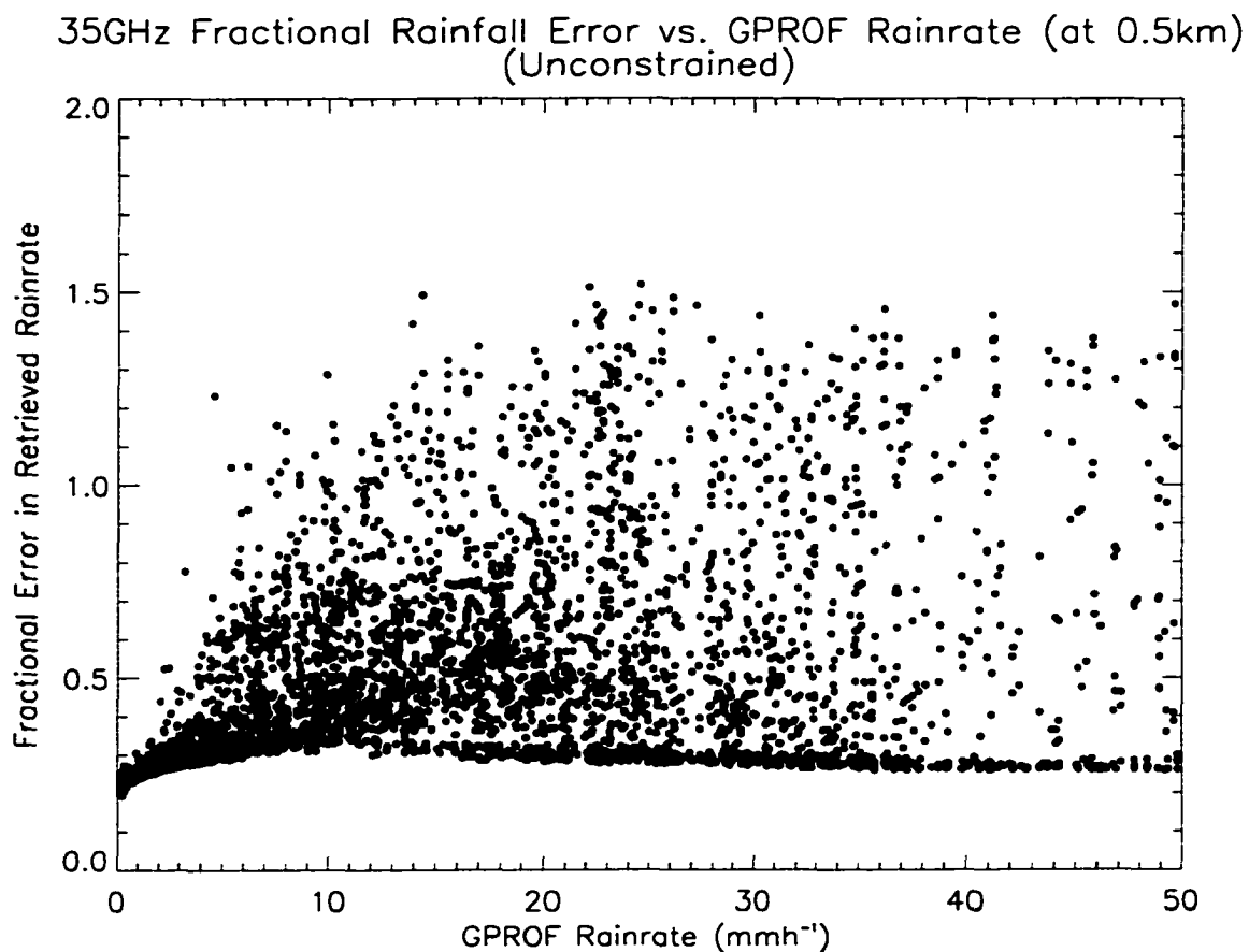
Figure E.2: Error in retrieved rainrate as a function of rainrate for the 35 GHz synthetic retrievals.
