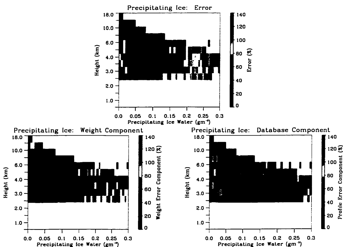
Figure 3.15: As in Figure 3.12 but for profiles of precipitating ice.
