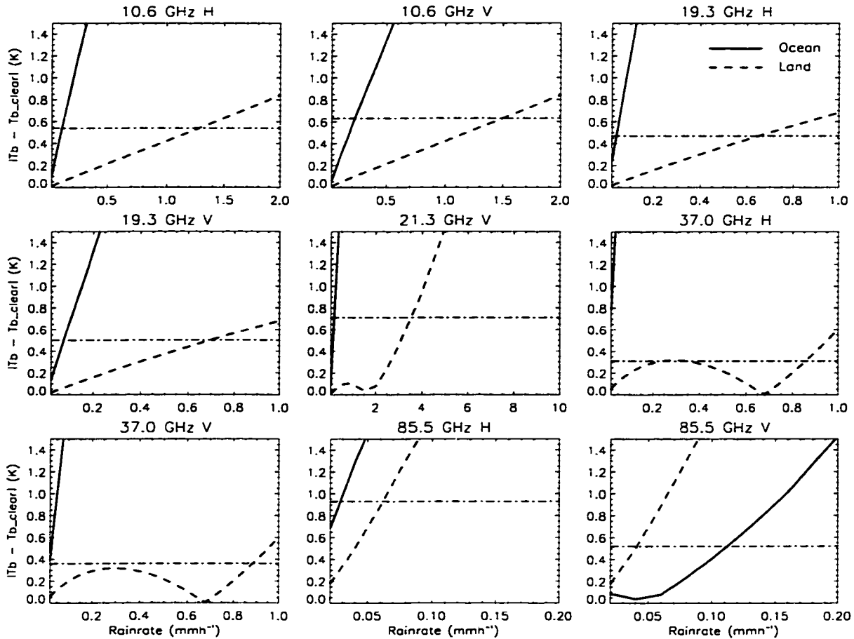
Figure 2.7: T_B difference between raining and clear sky scenes as a function of rainrate for each TMI channel. The horizontal dashed lines indicate the corresponding instrument sensitivity from Table 2.1.
