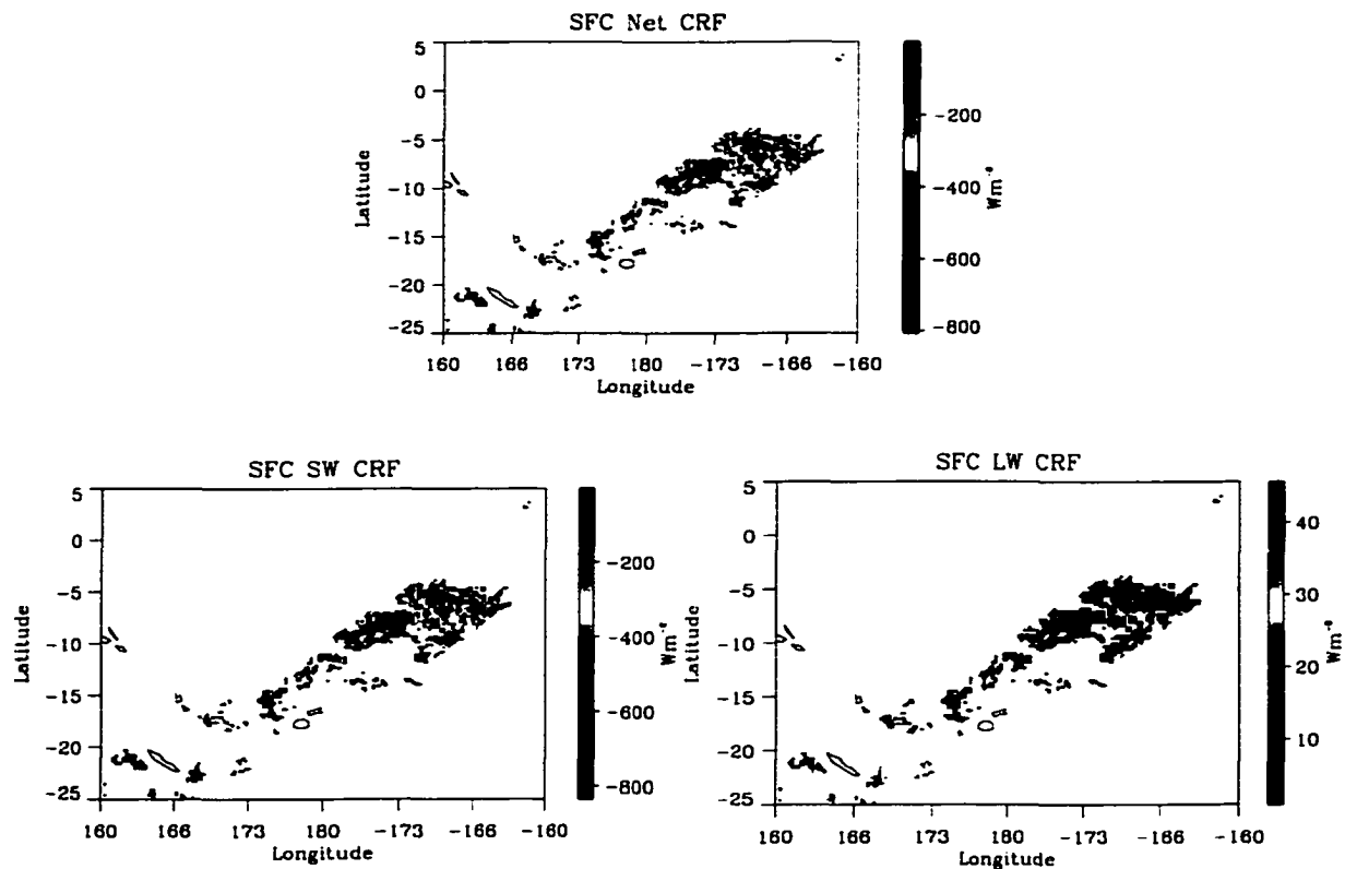
Figure 5.20: As in Figure 5.19 but illustrating CRF at the Earth's surface.
