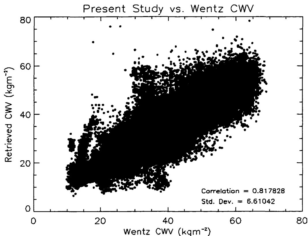
Figure 4.16: Comparison of precipitable water estimates from the present study with those from Wentz et al at RSS.
