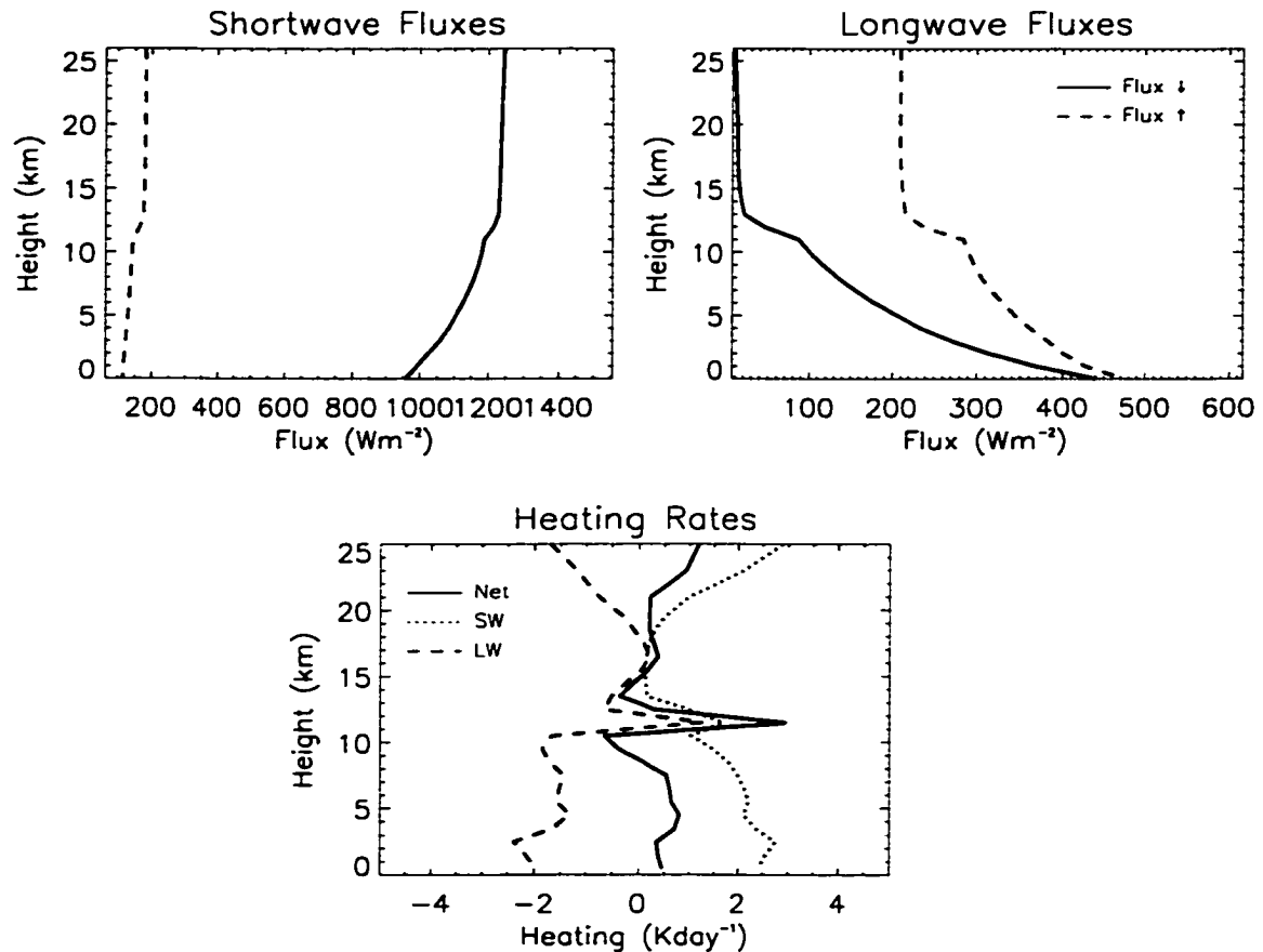
Figure 5.5: As in Figure 5.1 but for a pixel containing a cirrus cloud with an IR optical depth of 0.4, located between 11.5 and 13 km.
