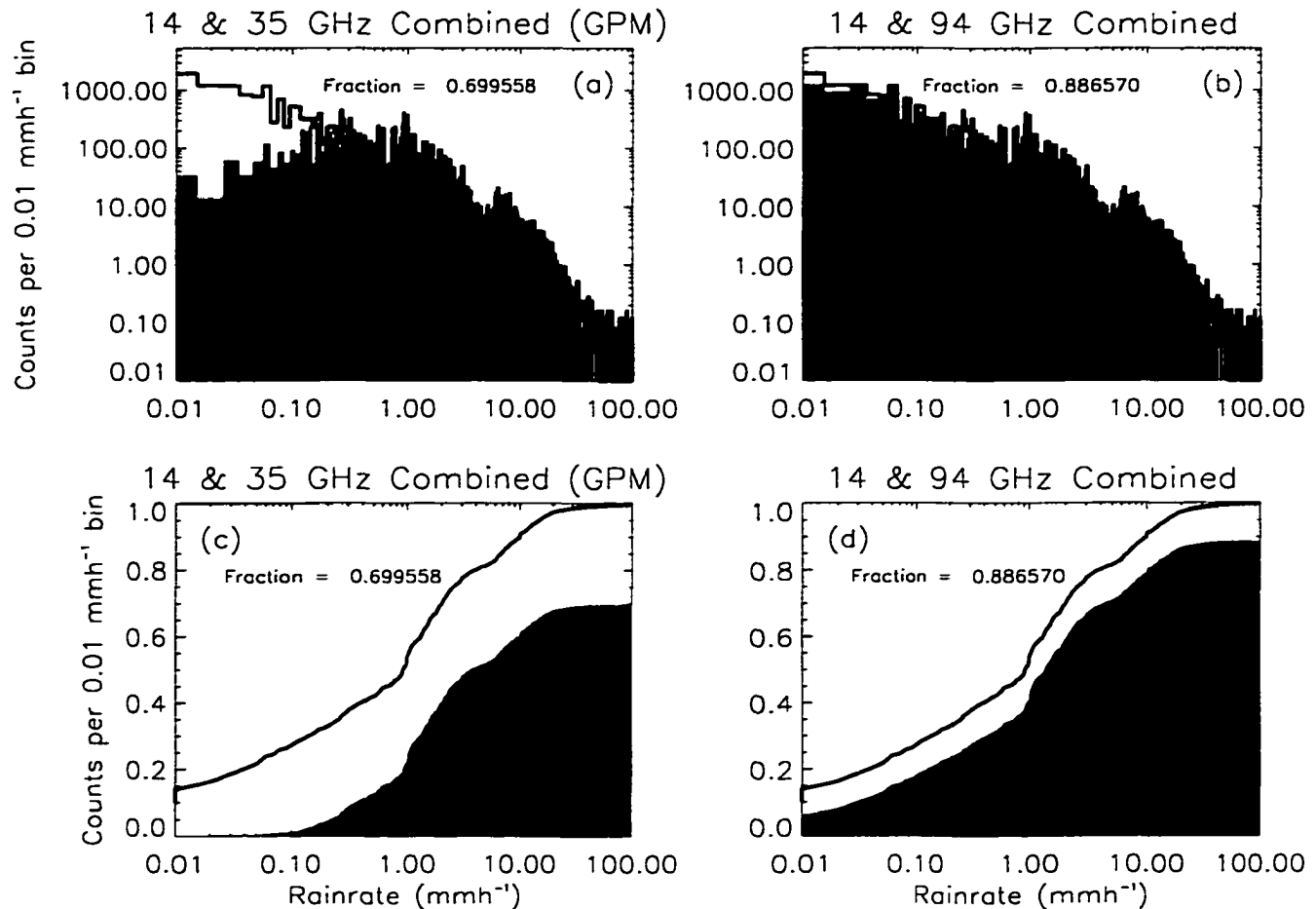
Figure E.6: As in Figures D.5 and D.6 but for hypothetical combinations of radars.
