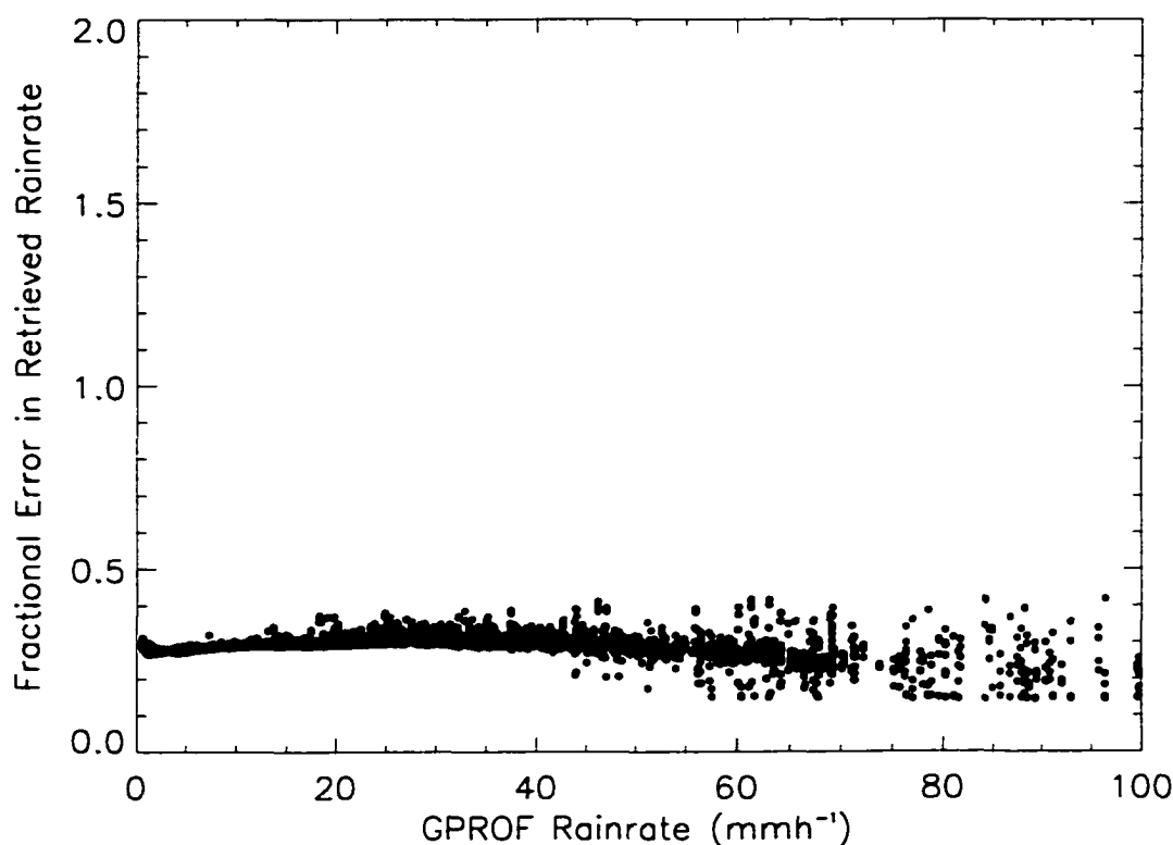
Figure D.17: Error in retrieved rainrate as a function of rainrate for the 14 GHz synthetic retrievals.
