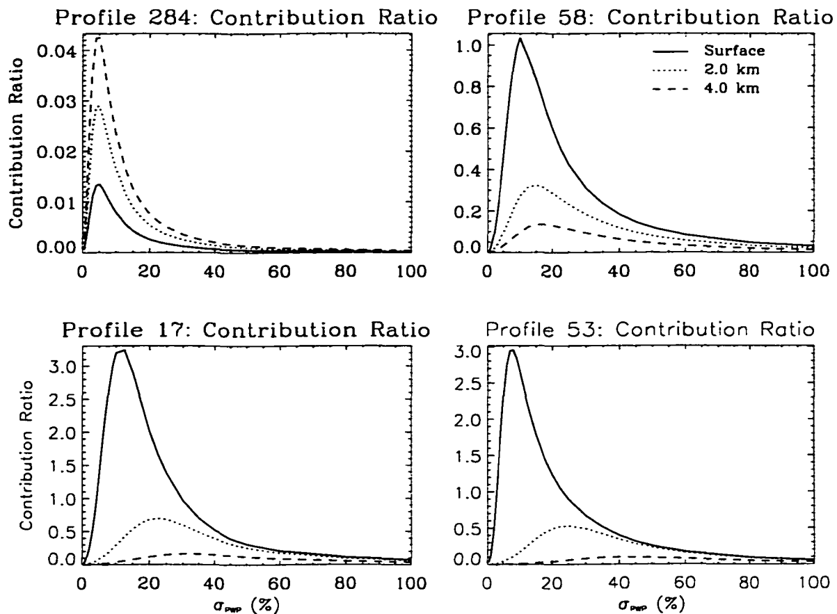
Figure E.5: Ratio of the constraint contribution to the total error to the sum of the corresponding measurement and a priori contributions as a function of constraint strength for the rainfall retrievals in Figure E.3.
