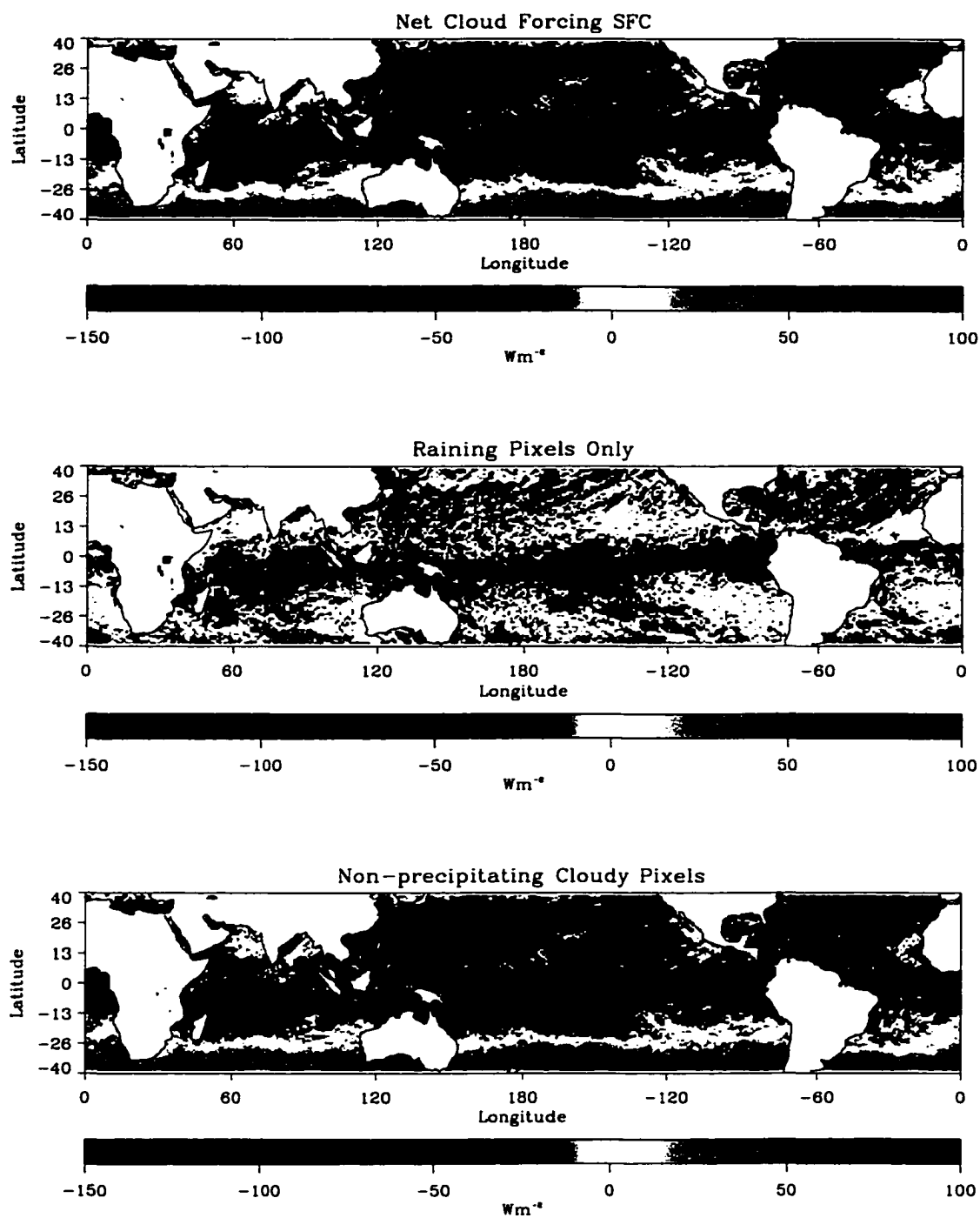
Figure 5.36: As in Figure 5.35 but for net cloud forcing at the surface.
