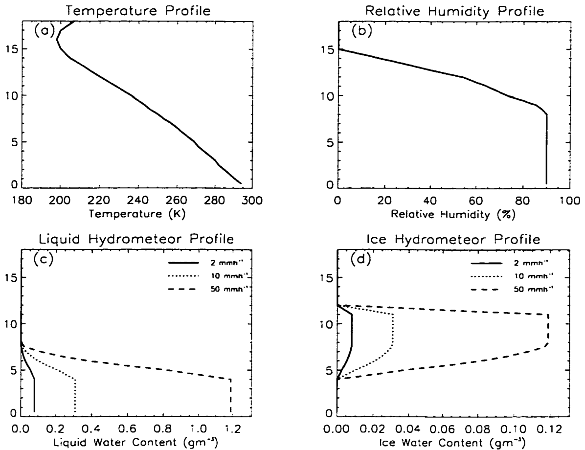
Figure 2.5: Profiles of (a) temperature, (b) relative humidity, (c) cloud liquid water, and (d) cloud ice water for selected rainrates.
