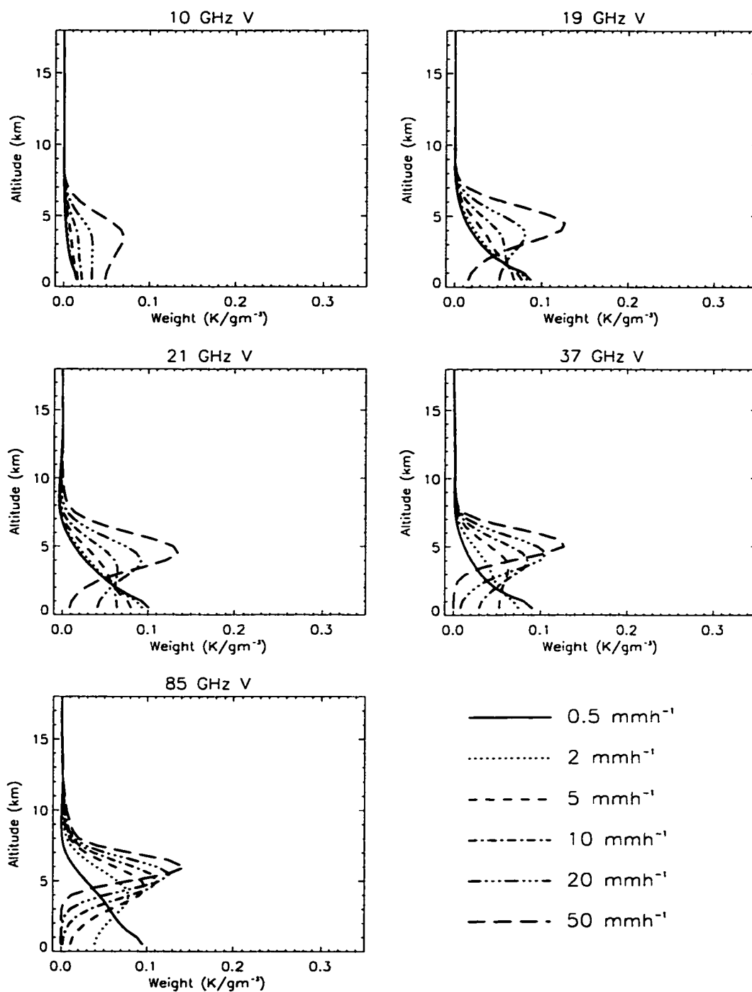
Figure 2.9: Temperature weighting functions for each vertically polarized TMI channel as a function of rainrate over a land background.
