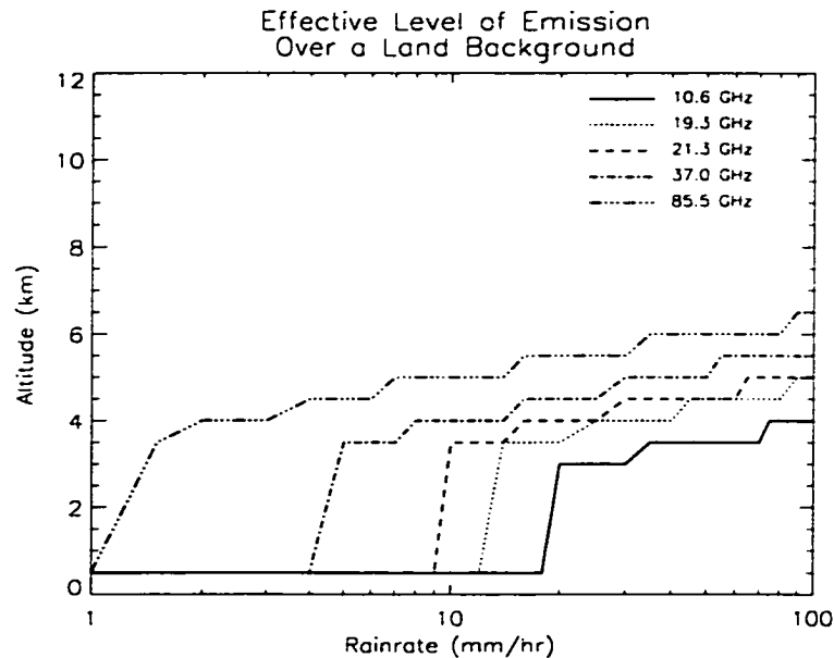
Figure 2.12: TMI effective levels of emission as a function of rainrate over a land background.
