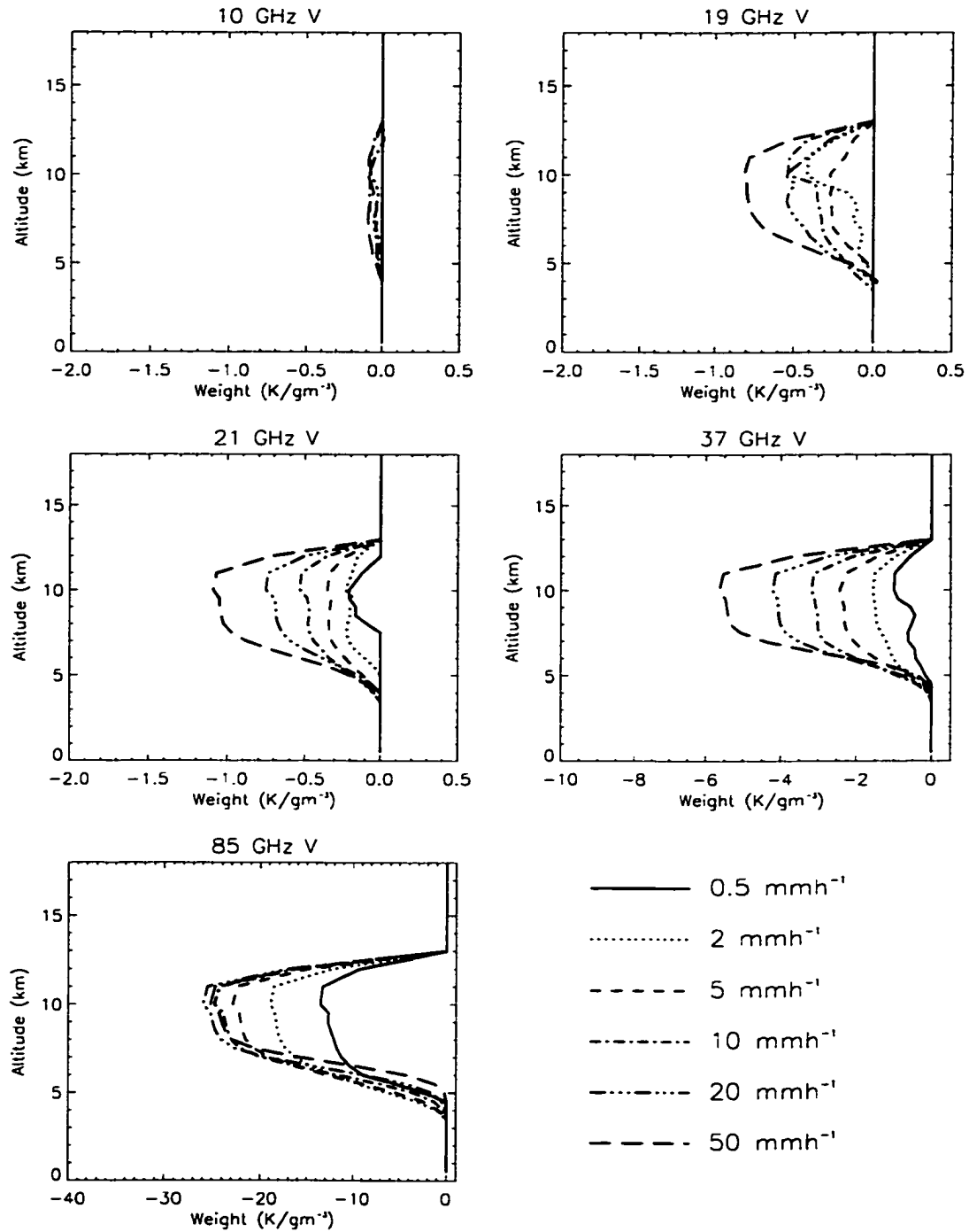
Figure 2.16: Ice water weighting functions for each vertically polarized TMI channel as a function of rainrate over a land background.
