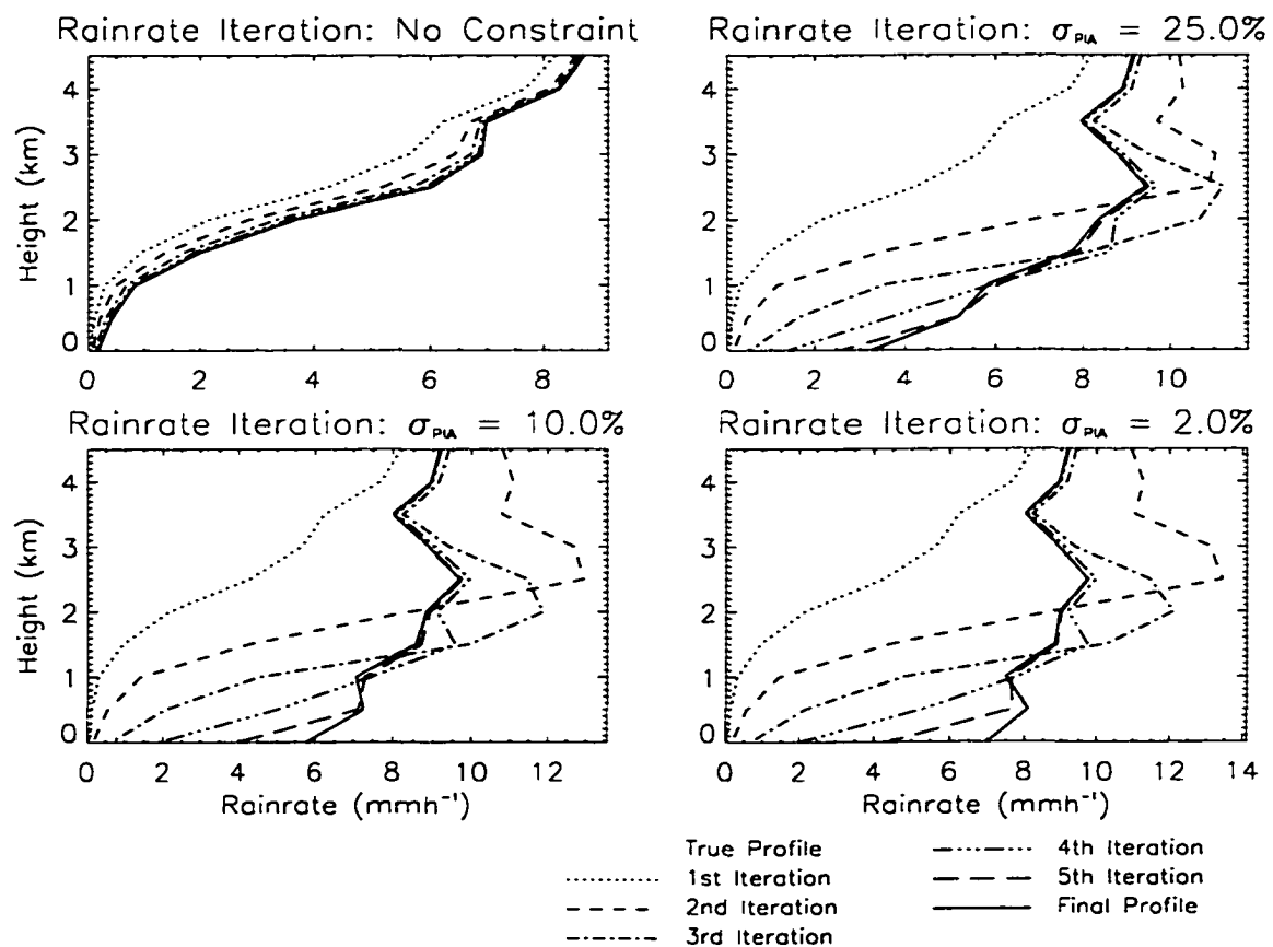
Figure D.34: As in Figure D.33 but using a PIA constraint as opposed to a PWP constraint.
