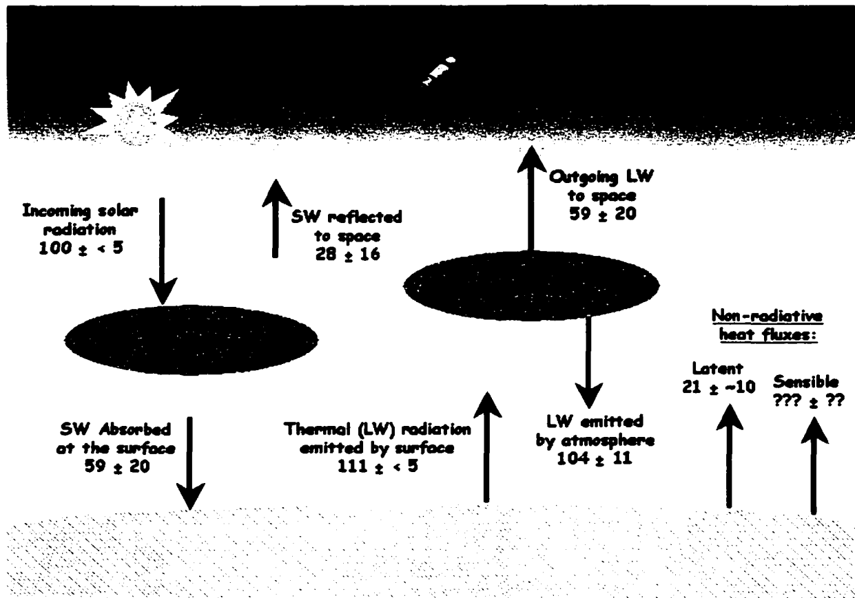
Figure 5.42: February 1998 tropical energy budget from TRMM. All quantities are expressed as a percentage of the total incoming solar radiation at the top of the atmosphere, 393.6 \text{ Wm}^{-2} .
