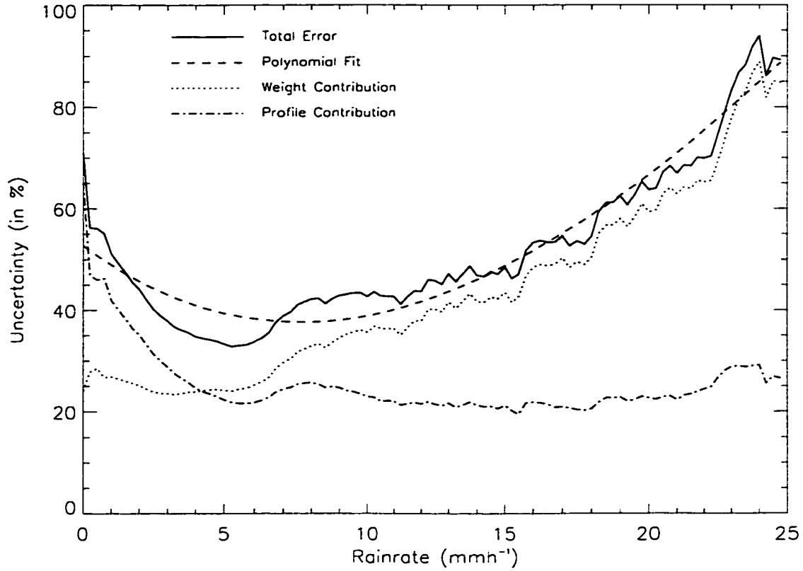
Figure 3.11: Cloud database and weight components to total uncertainty as a function of rainrate.
