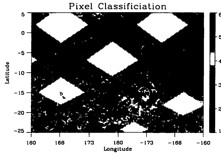
Figure 4.19: Pixel classification used to specify the locations of cloud and rainfall for future radiative transfer modeling. Flags are defined in Table 4.3.
