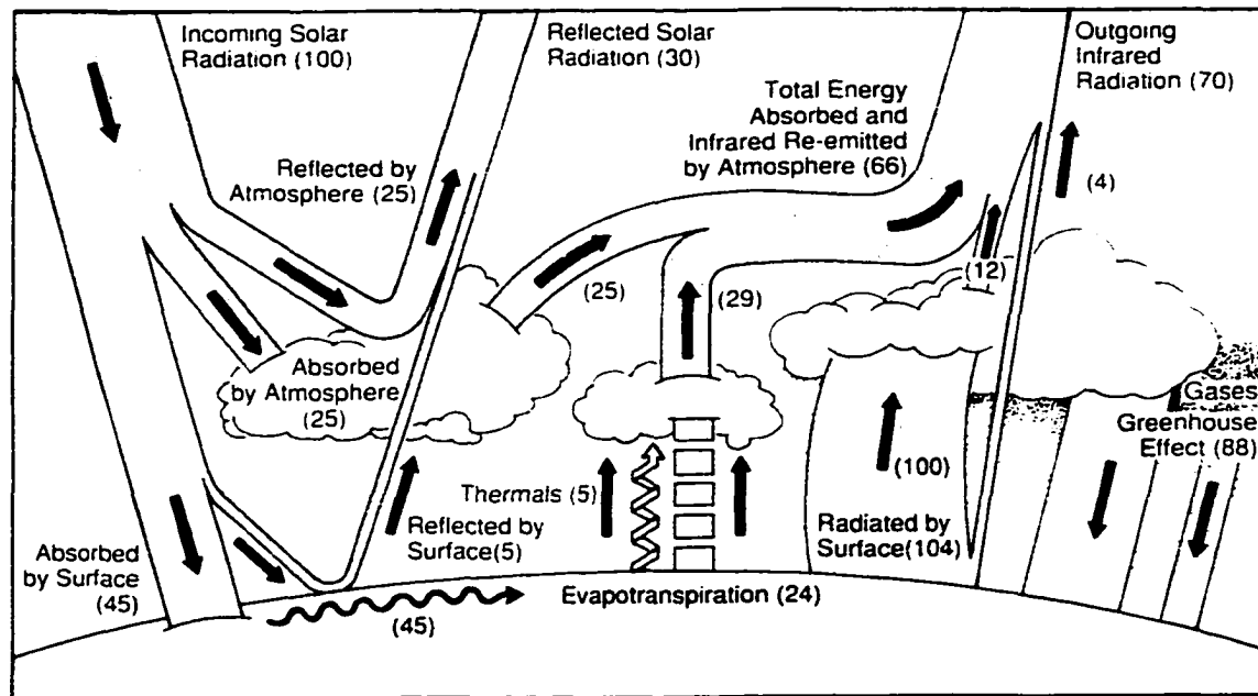
Figure 1.1: Principal components of the Earth's energy budget (adapted from Trenberth, 1992).
