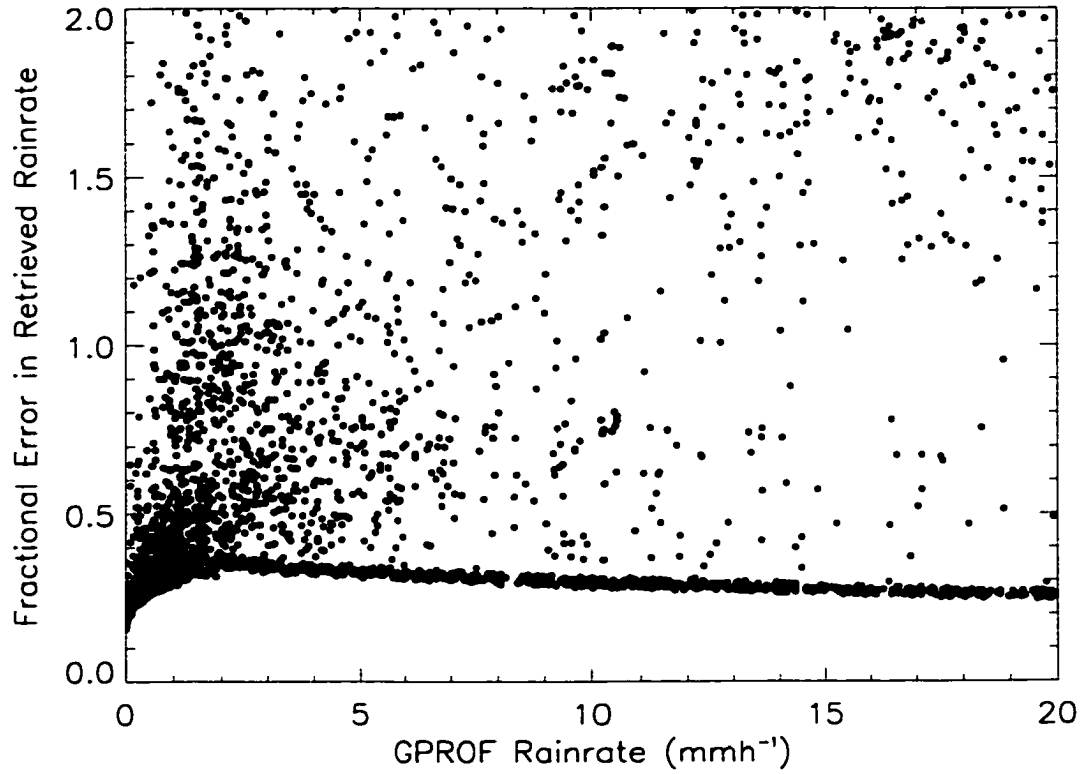
Figure D.19: As in Figure D.17 but at 94 GHz.
