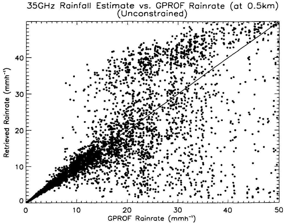
Figure E.1: Comparison of near-surface rainfall estimates using reflectivities at 35 GHz with truth.
