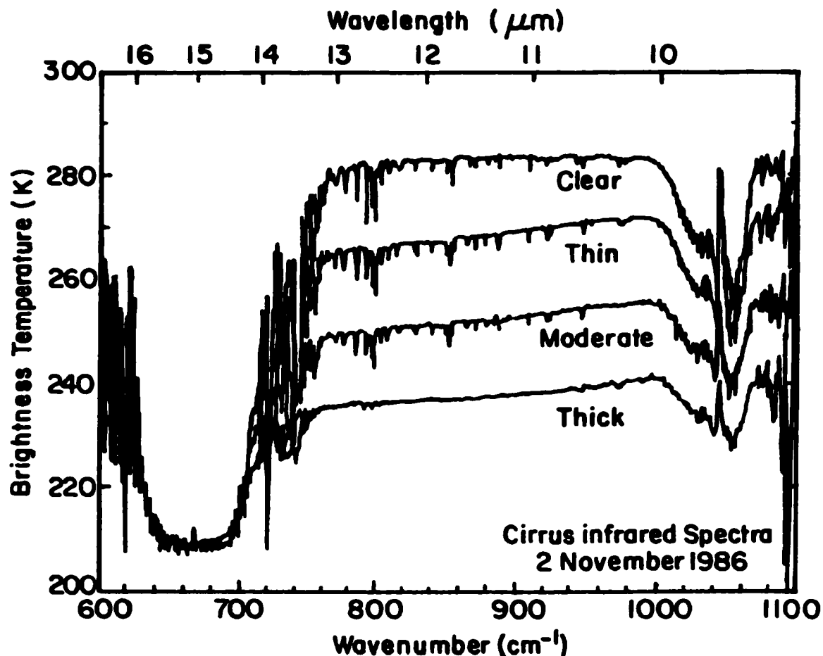
Figure 4.6: Emission spectra in the 8-12 \mu\text{m} atmospheric window due to clear-sky, thin, moderate, and thick cirrus scenes (from Stephens (1994)).
