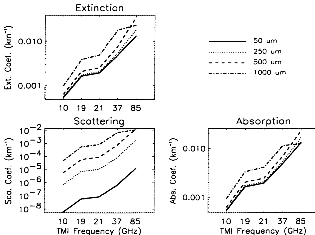
Figure 2.2: Extinction, scattering and absorption coefficients for liquid spheres at each TMI channel.
