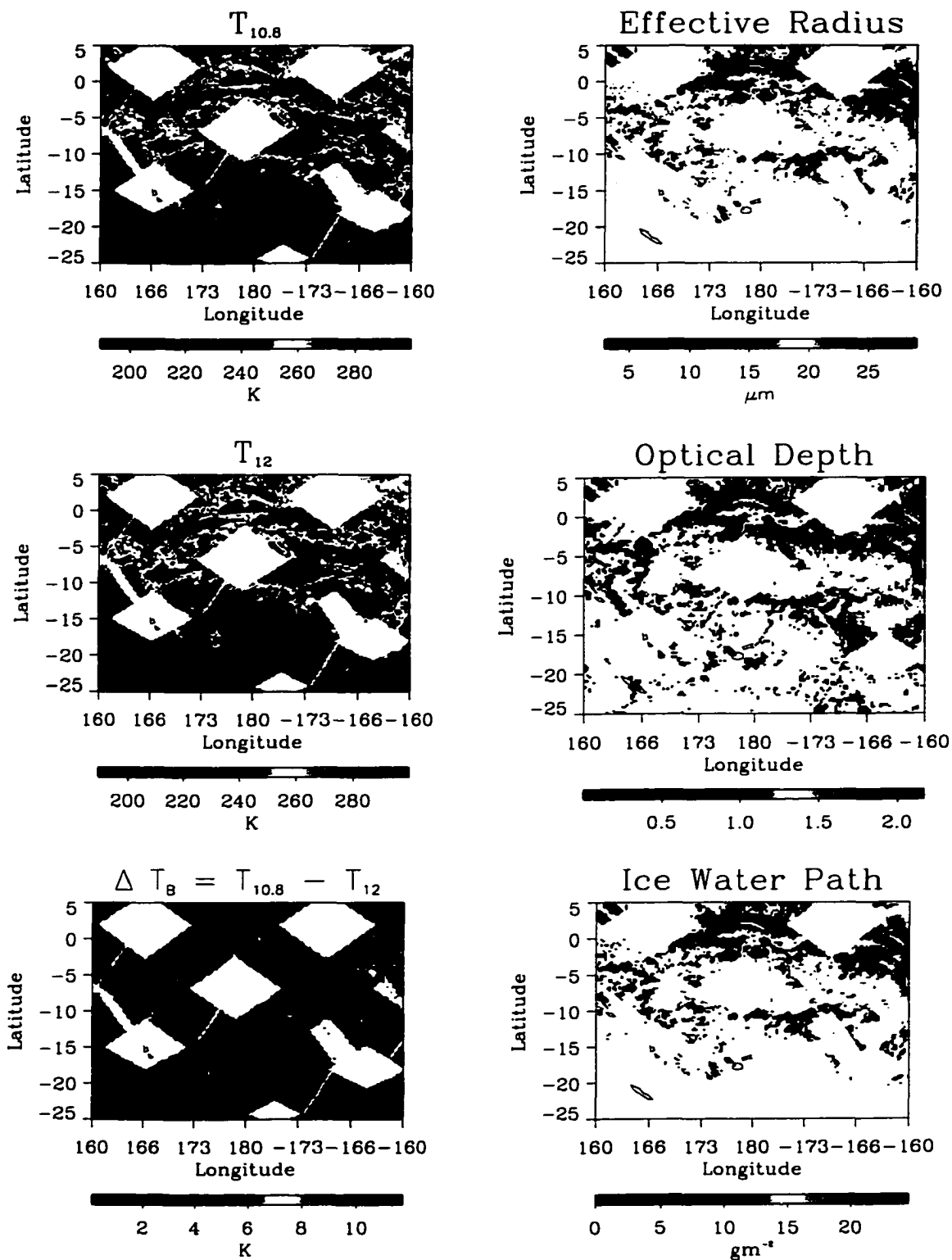
Figure 4.9: VIRS channel 4 and 5 input and resulting effective radius and IWP estimates from the sample region on February 1, 1998.
