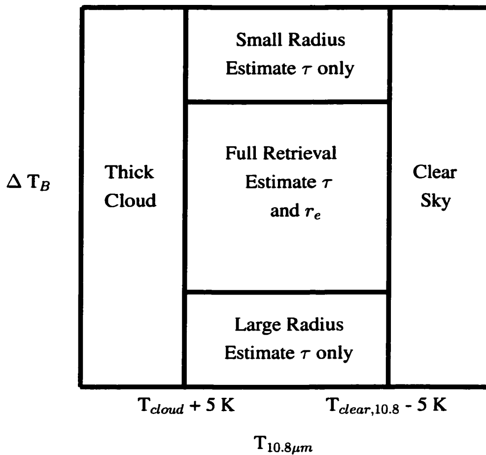
Figure 4.8: Cloud classification scheme used in VIRS-based retrievals of ice cloud optical properties. In the standard retrieval, pixels with T_{10.8} > T_{clear,10.8} - 5 \text{ K} are designated as clear-sky and those with T_{10.8} > T_{cloud} + 5 \text{ K} as thick cloud.
