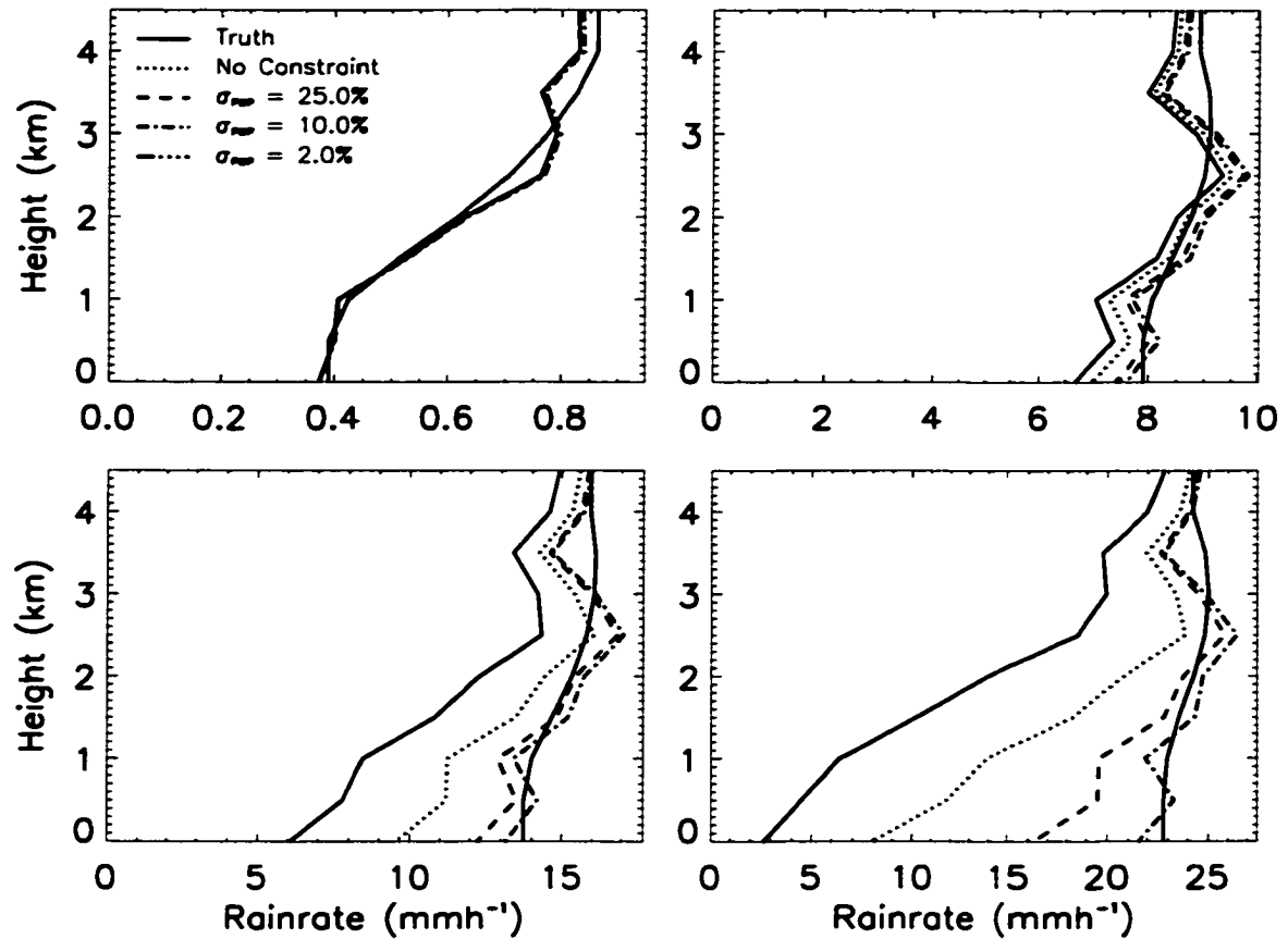
Figure E.3: Sample rainfall retrievals at 35 GHz. Profiles are chosen to reflect the range of rainfall retrievable at 35 GHz and therefore include some of those shown to represent 14 GHz retrievals in Figure D.25 at some shown in Figure D.26 illustrating 94 GHz retrievals.
