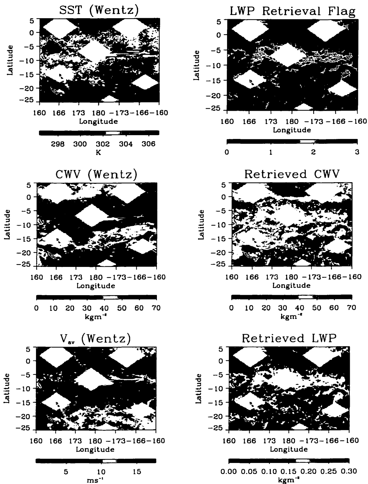
Figure 4.15: LWP retrievals from the sample region on February 1, 1998.
