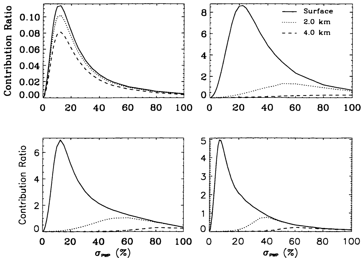
Figure D.30: Ratio of the constraint contribution to the total error to the sum of the corresponding measurement and a priori contributions as a function of constraint strength for the rainfall retrievals in Figure D.26.
