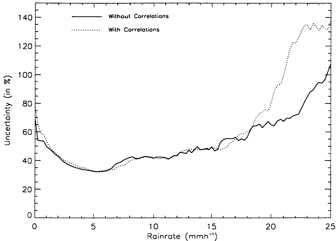
Figure 3.18: Retrieval errors assuming a diagonal covariance matrix (solid) and those using the full covariance matrix (dotted).
