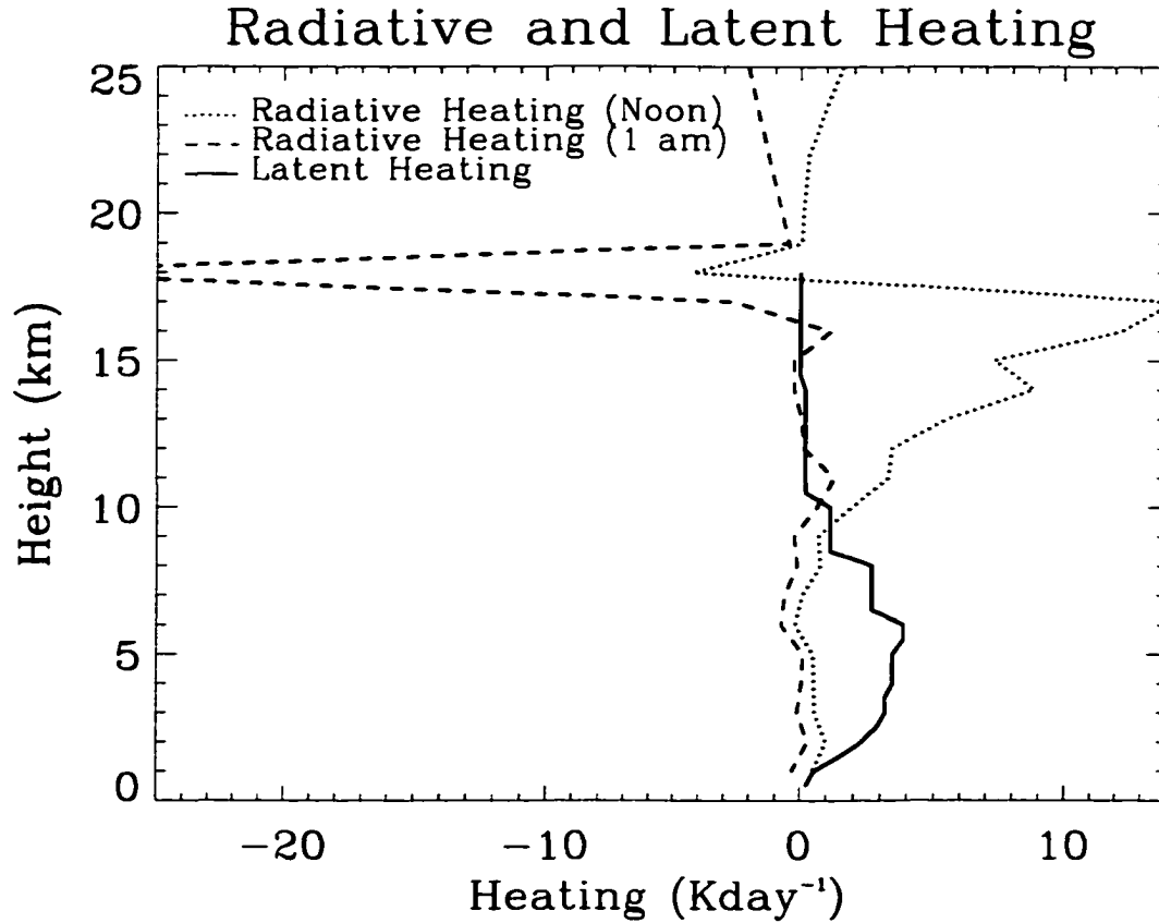
Figure C.1: Profiles of radiative and latent heating for a single precipitating pixel ( R = 11 \text{ mmh}^{-1} ).
