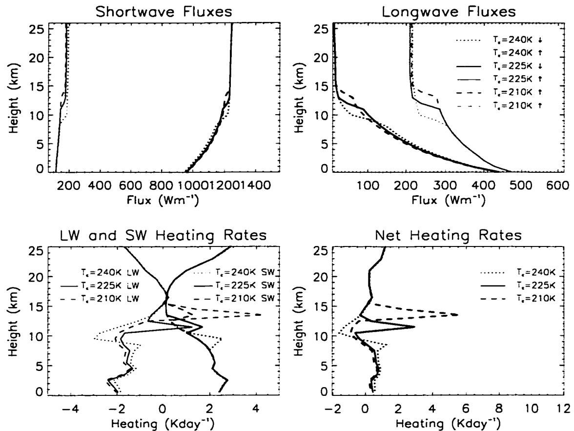
Figure 5.11: Sensitivity of radiative fluxes and heating rates to assumed cloud emitting temperature for thin cirrus case.
