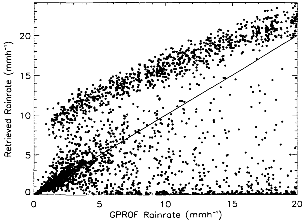
Figure D.16: As in Figure D.15 but for retrievals at 94 GHz.
