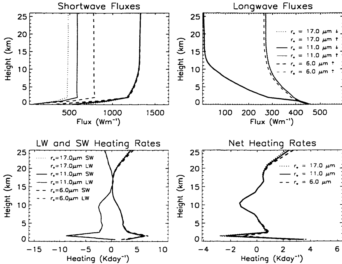
Figure 5.13: Sensitivity of radiative flux and heating rate profiles for liquid clouds with different r_e .
