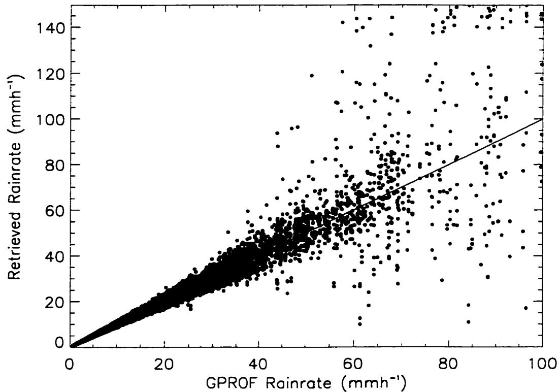
Figure D.15: Synthetic near-surface rainfall retrievals at 14 GHz.
