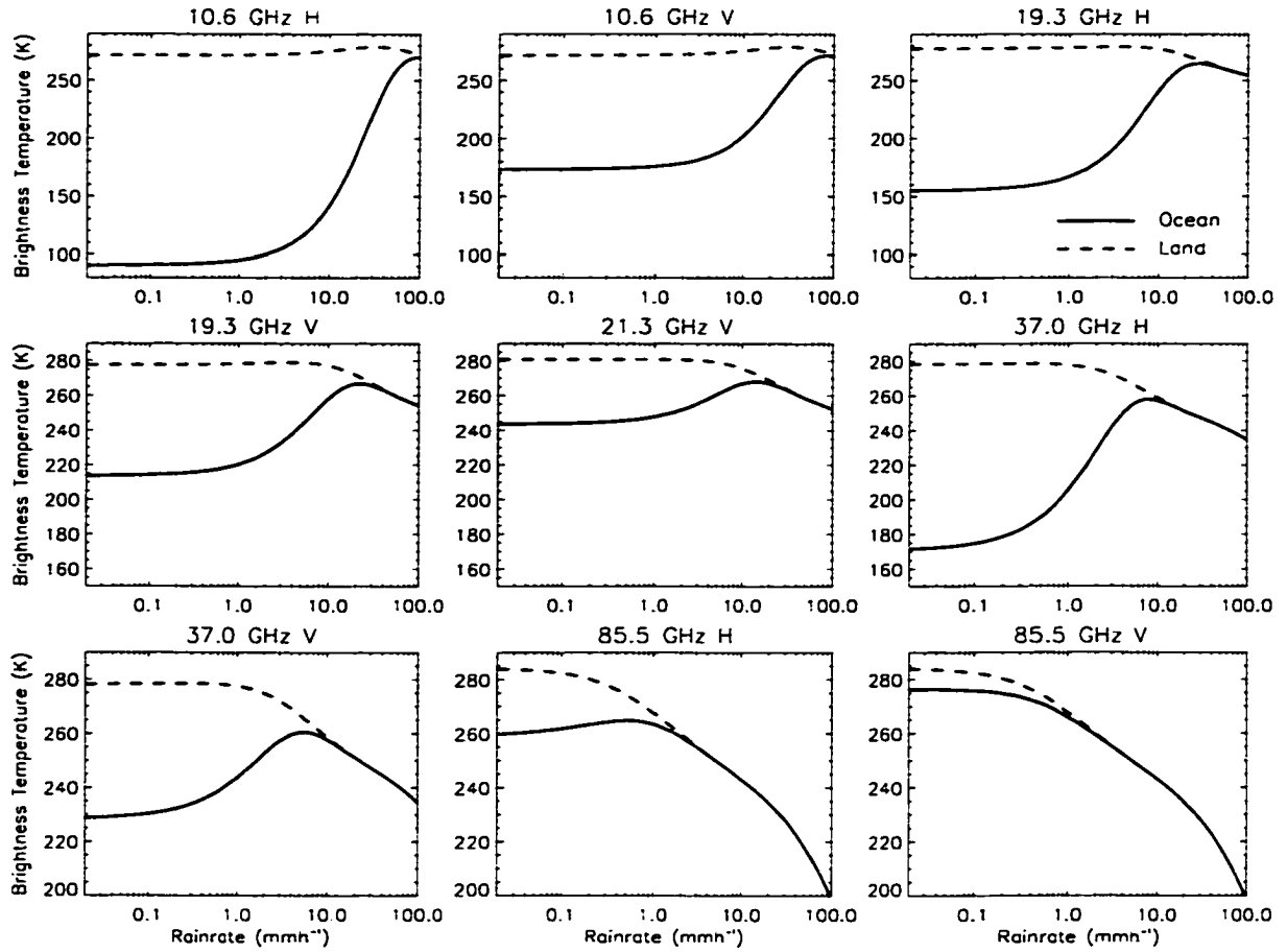
Figure 2.6: T_B as a function of rainrate for each TMI channel over both ocean and land backgrounds.
