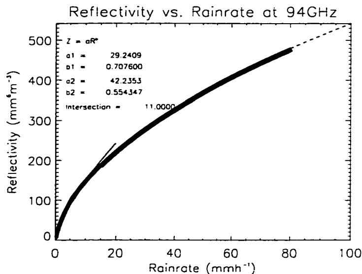
Figure D.12: Reflectivity vs. rainrate for a MP distribution of spherical raindrops.
