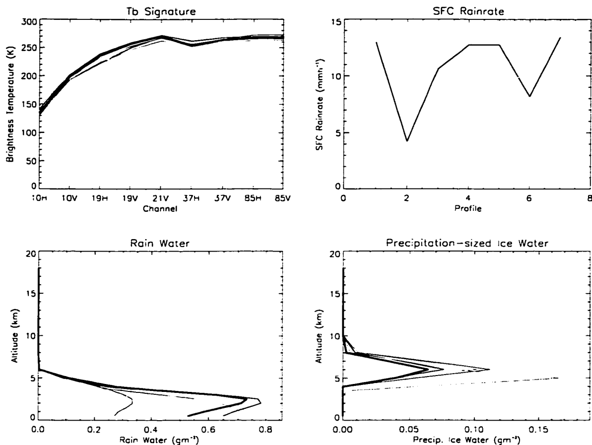
Figure 3.23: As in Figure 3.8 after including a column-integrated PR reflectivity profile.
