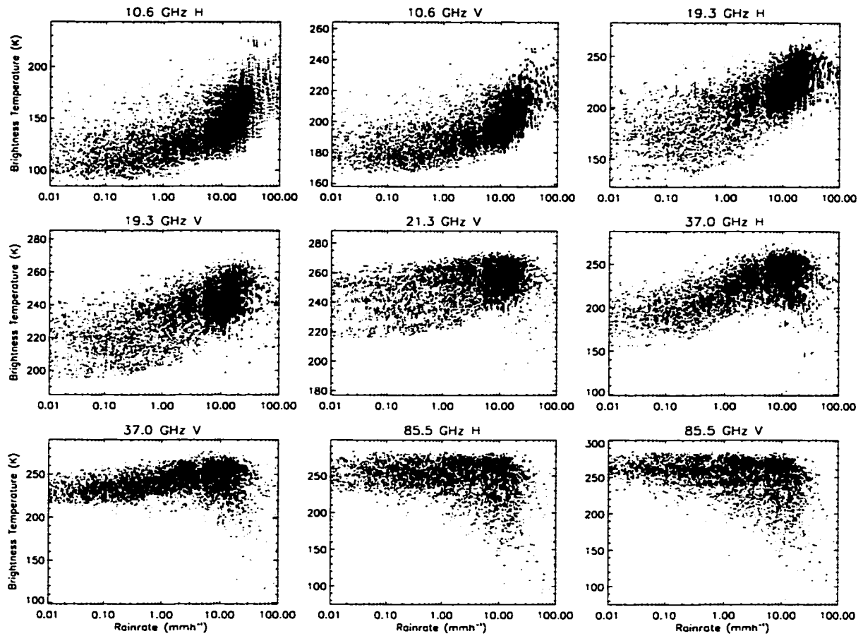
Figure 2.27: Scatter plots of TMI T_B s as a function of rainrate for the entire GPROF database.
