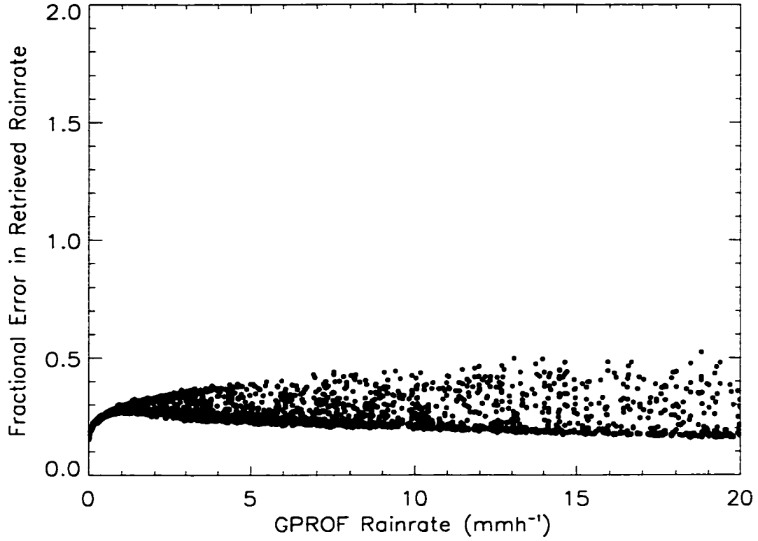
Figure D.22: As in Figure D.19 but at an altitude of 4.0 km.
