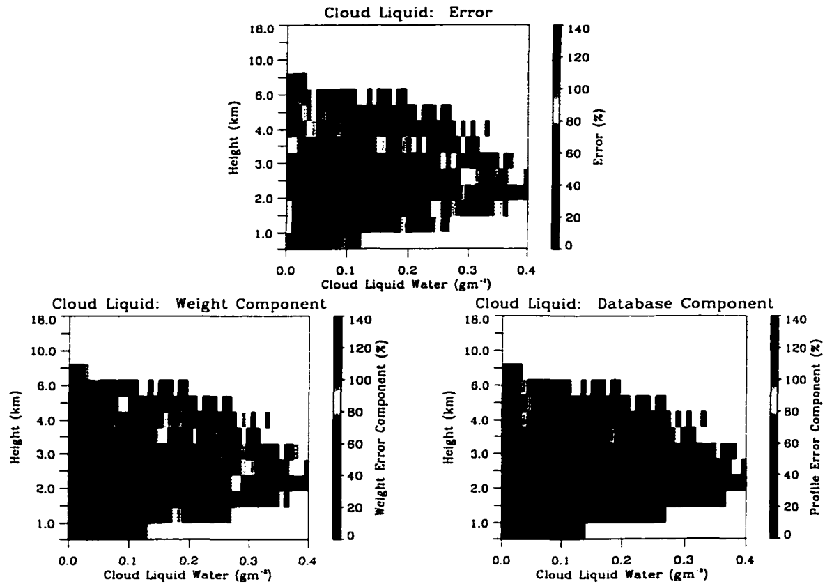
Figure 3.12: Uncertainties in cloud bin liquid water profile estimates and their corresponding weight and database components as a function of height and retrieved liquid water content. The irregular vertical axis accounts for the fact that cloud model levels are not equally spaced. See Table B.1 for model level heights.
