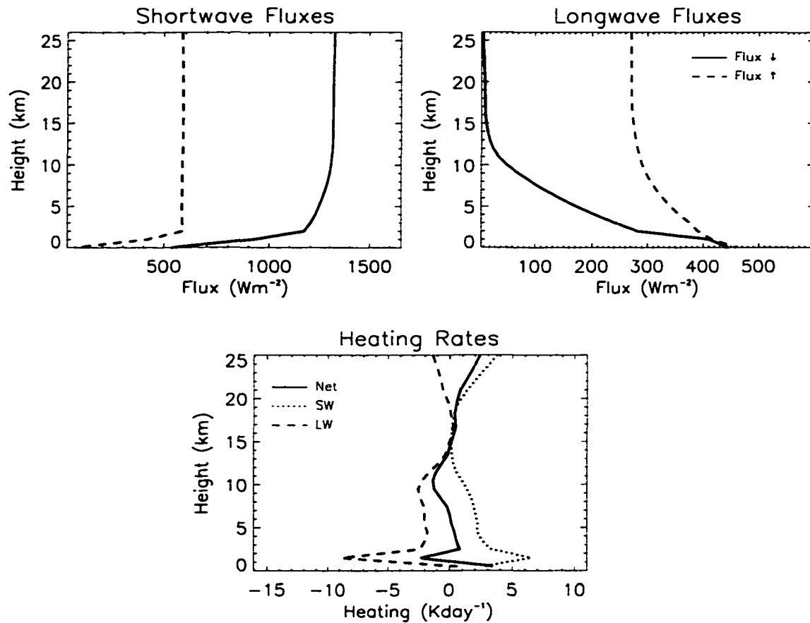
Figure 5.7: As in Figure 5.1 but for a pixel containing a 1 km stratus cloud with IR optical depth of 15 centered at 1.5 km.
