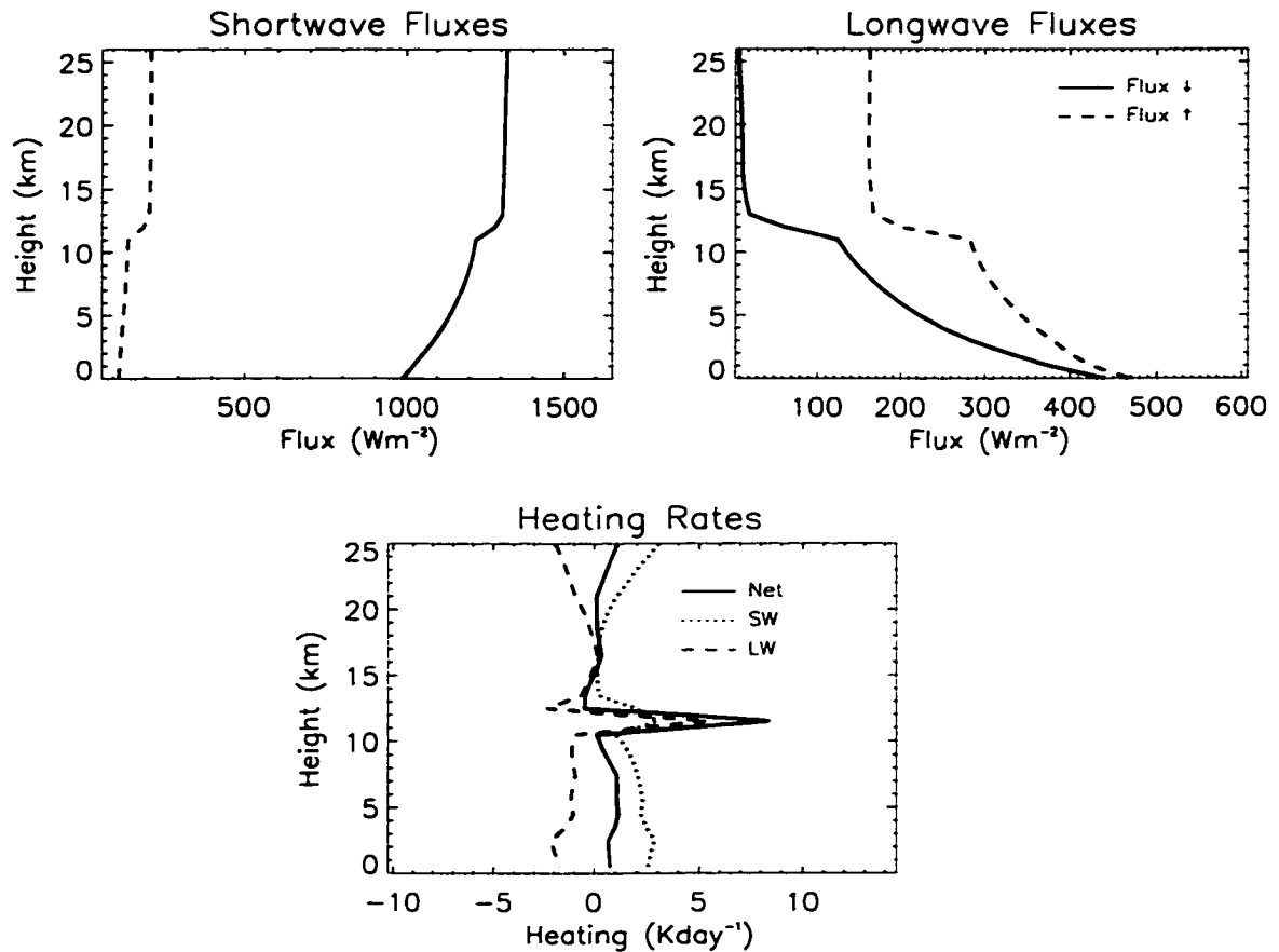
Figure 5.6: As in Figure 5.5 for a cirrus cloud with an IR optical depth of 1.2.
