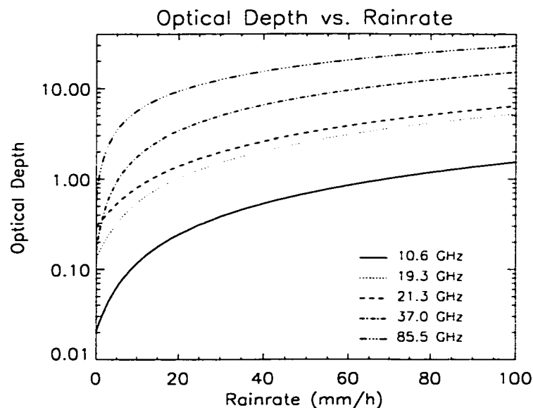
Figure 2.10: Optical depth as a function of rainrate at each TMI frequency.
