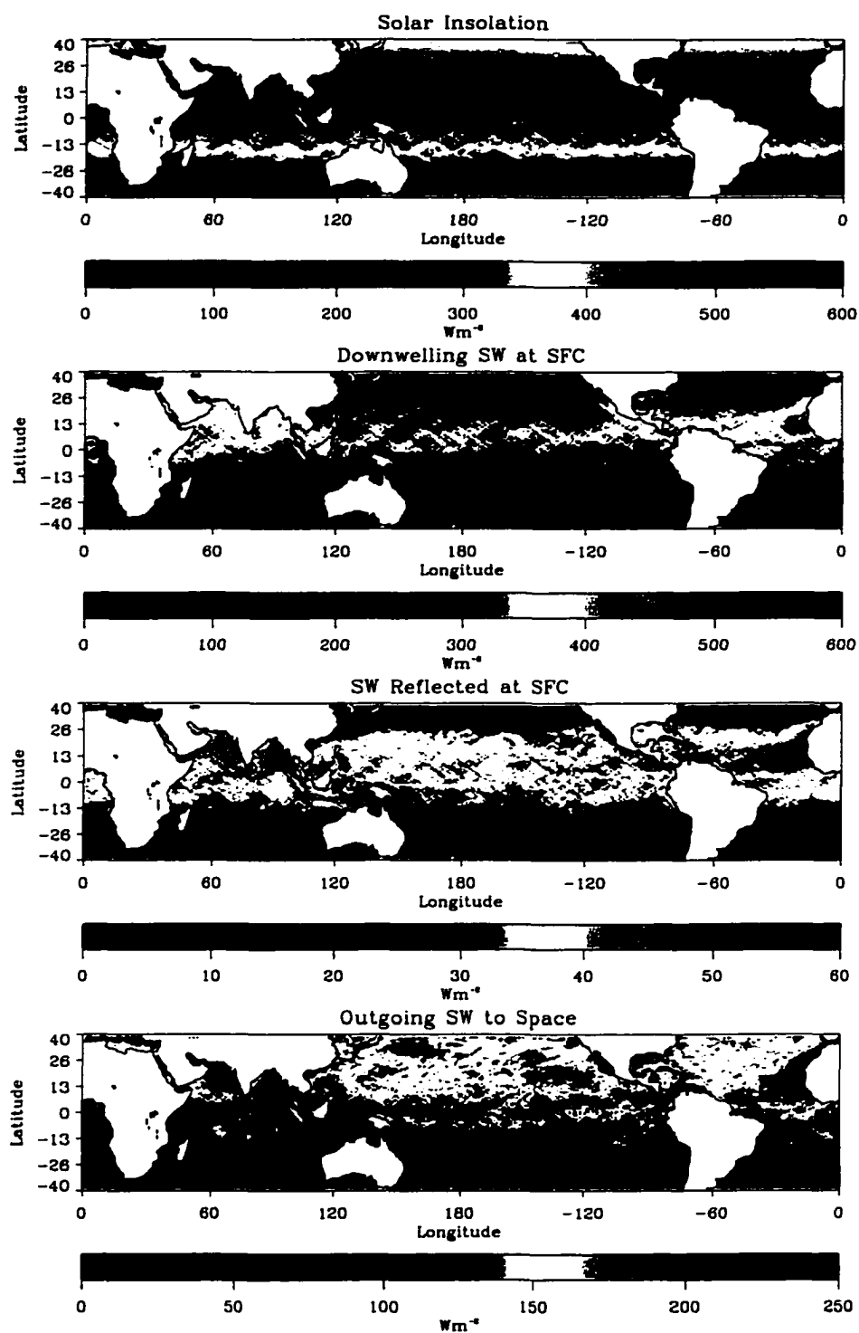
Figure 5.31: Monthly-mean SW fluxes for February 1998.
