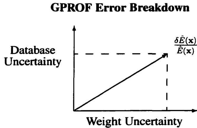
Figure 3.2: Reconstruction of the retrieval error from it's two components, the uncertainty associated with calculating the weights and that due to the cloud database.
