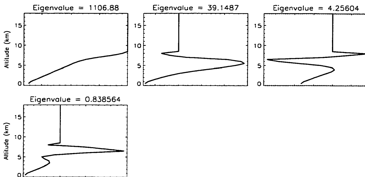
Figure 2.21: As in Figure 2.19 but at a rainrate of 20 \text{ mmh}^{-1} .
