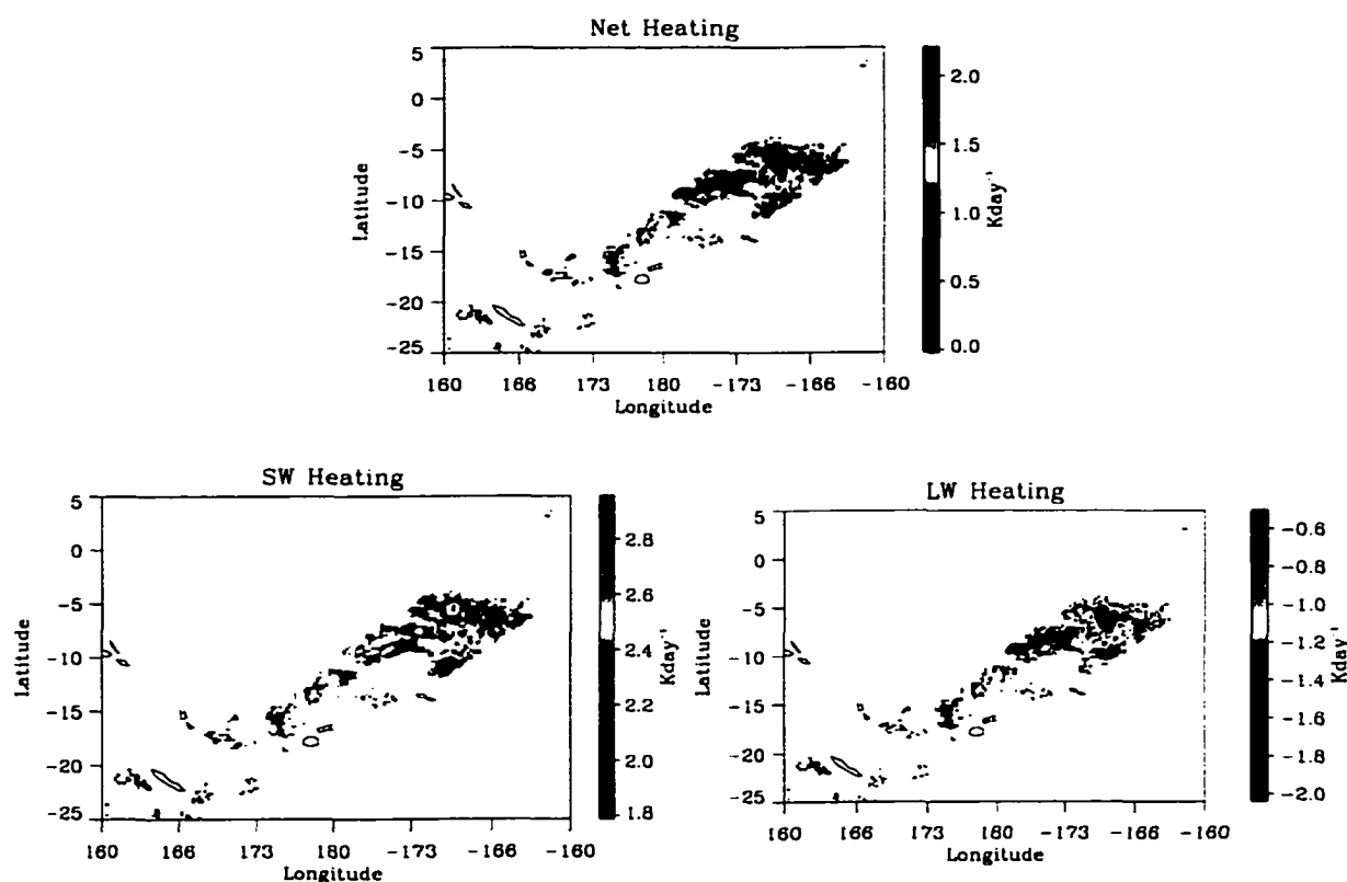
Figure 5.21: Column-integrated radiative heating rates for in precipitating pixels corresponding to a TRMM overpass at local noon.
