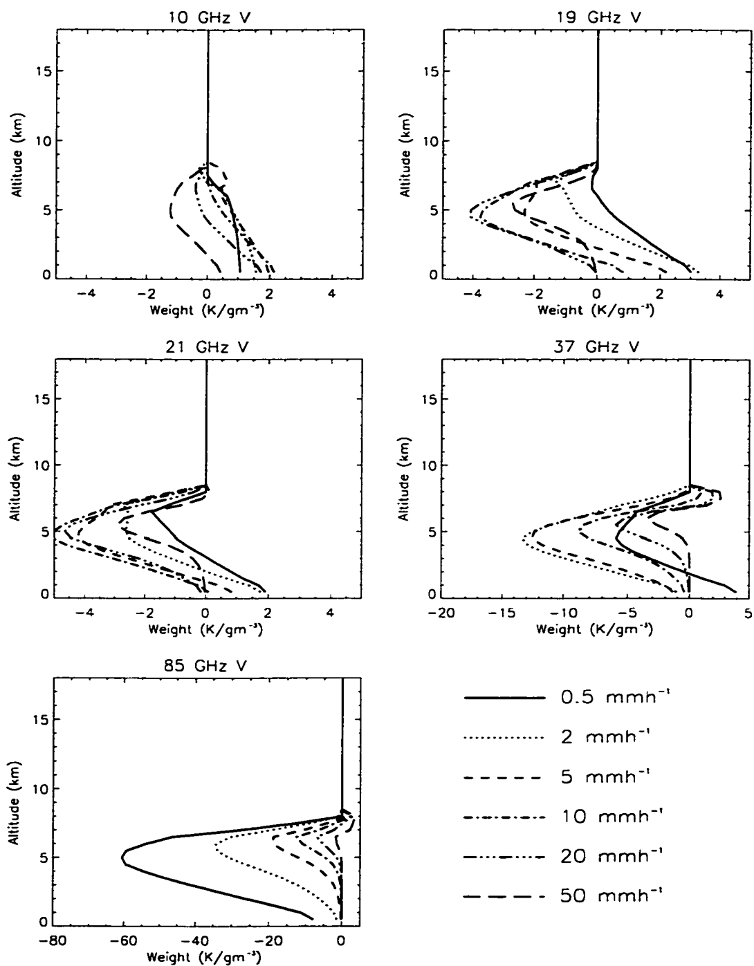
Figure 2.14: Liquid water weighting functions for each vertically polarized TMI channel as a function of rainrate over a land background.
