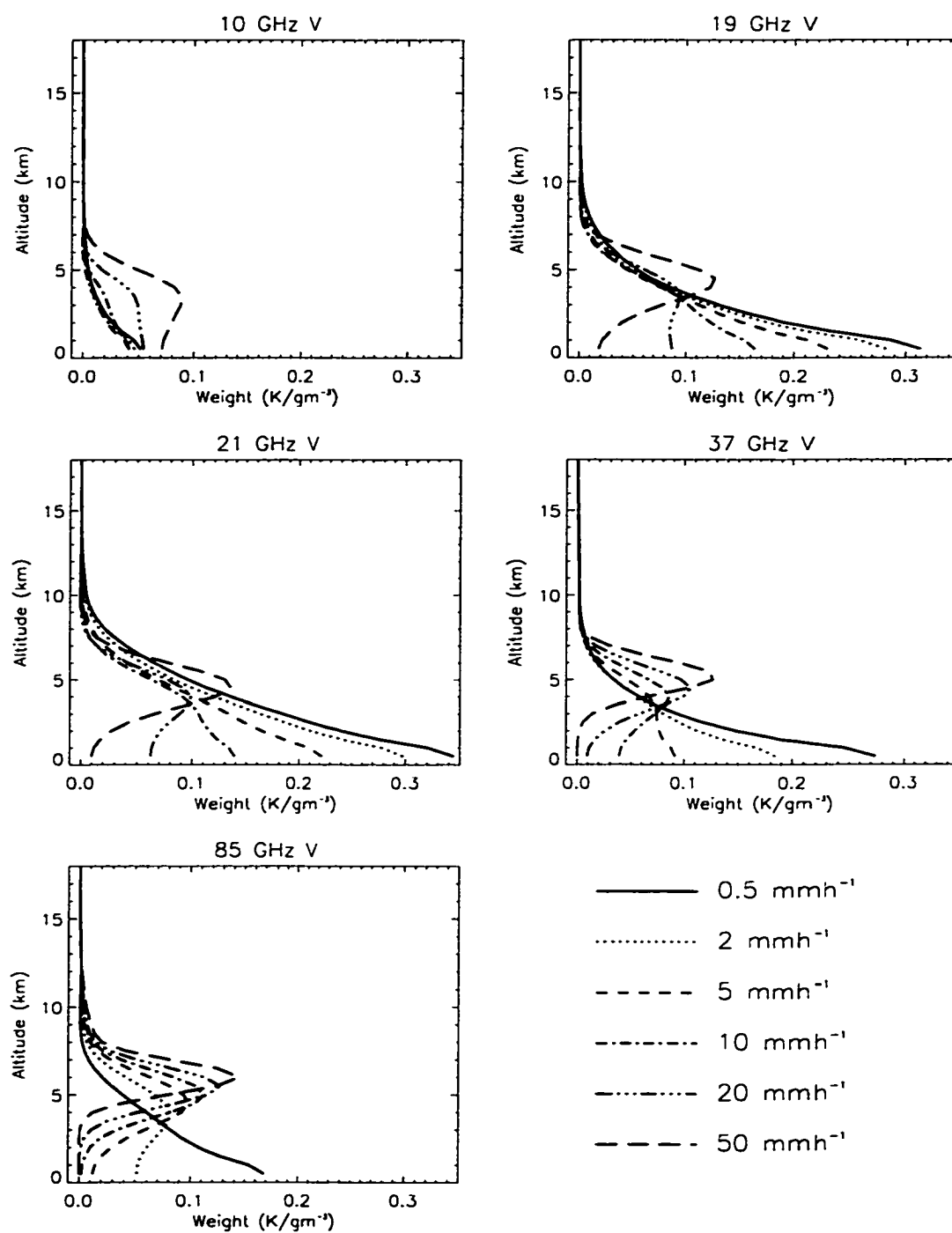
Figure 2.8: Temperature weighting functions for each vertically polarized TMI channel as a function of rainrate over an ocean background.
