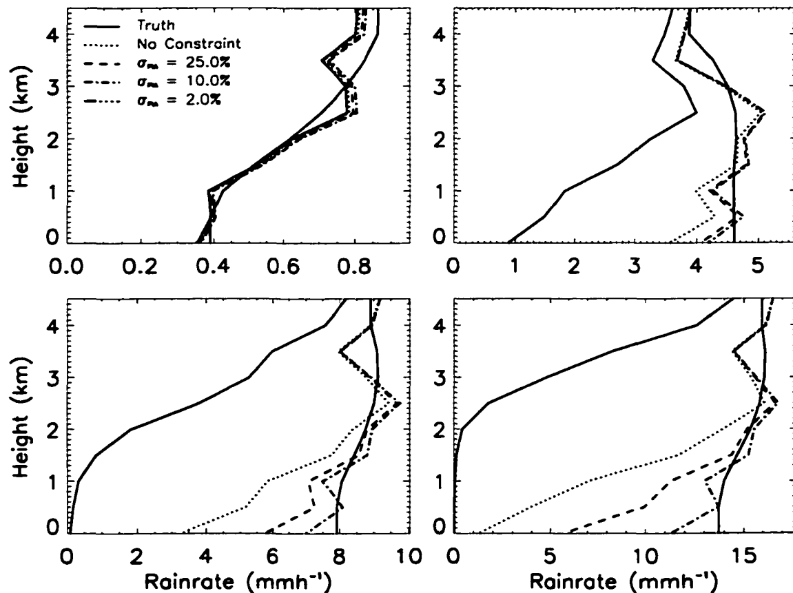
Figure D.31: As in Figure D.26 but with PIA constraints.
