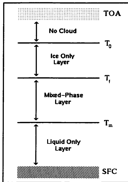
Figure 2.4: Schematic diagram of the cloud model.
