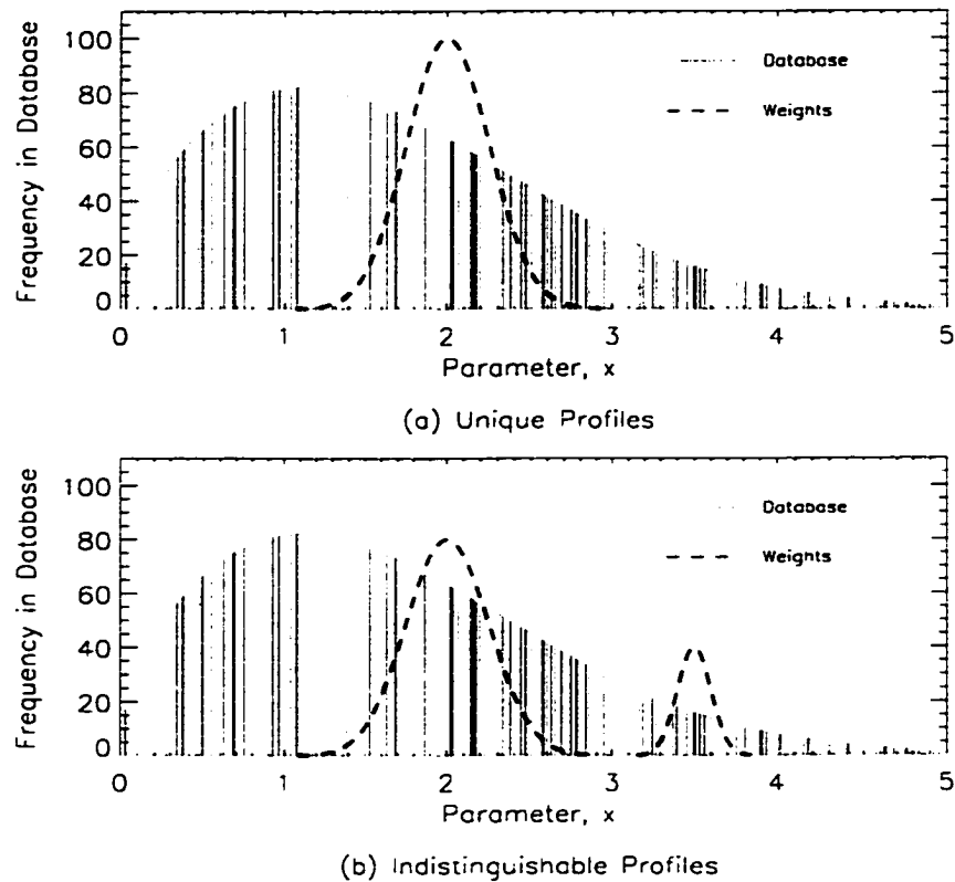
Figure 3.3: Graphical representation of retrieval process.
