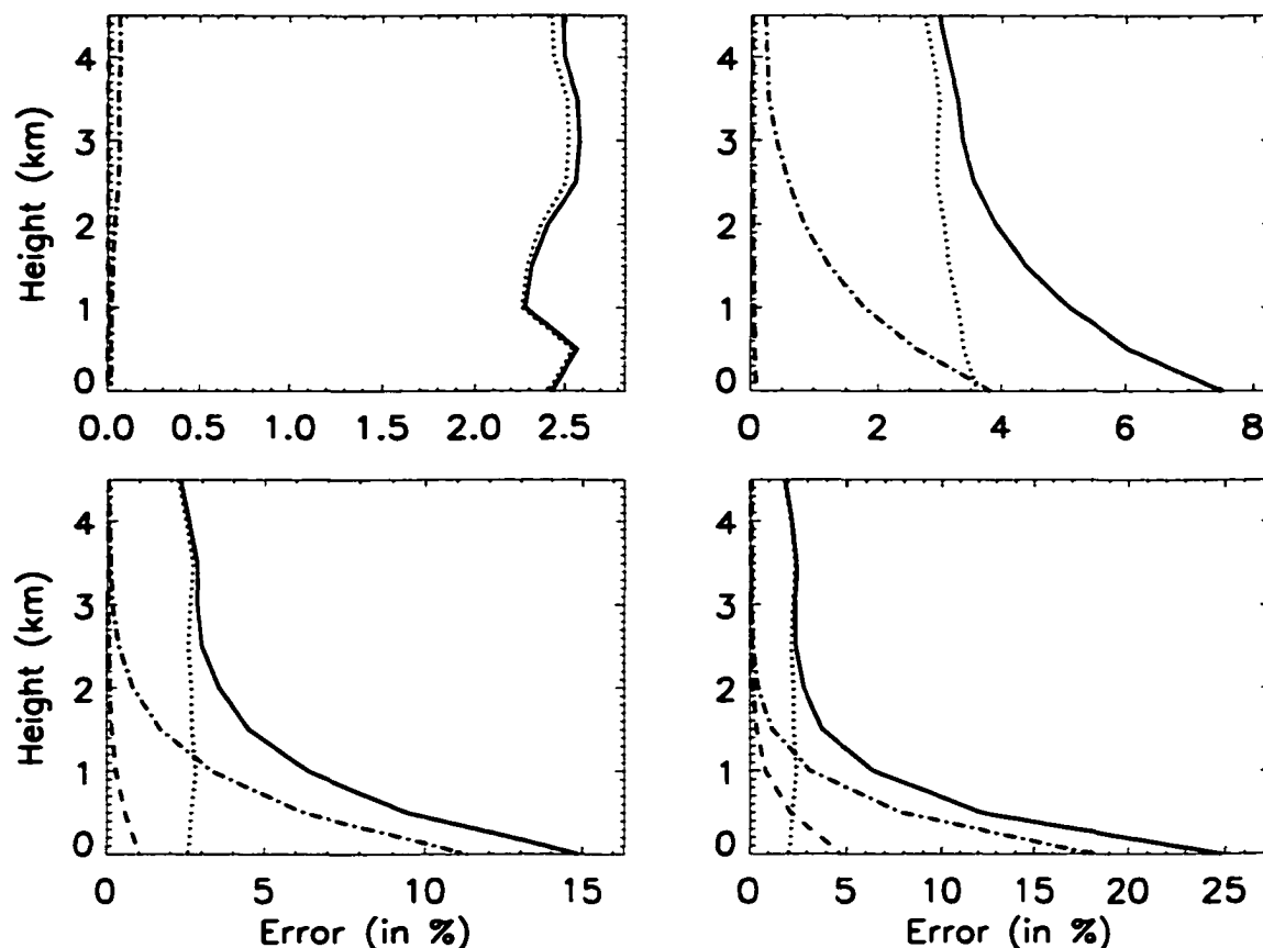
Figure E.4: The measurement (dotted line), a priori (dashed line), and PWP constraint (dot-dashed line) contributions to the total error (solid line) in the retrievals from Figure E.3 assuming a constraint accuracy of 10%.
