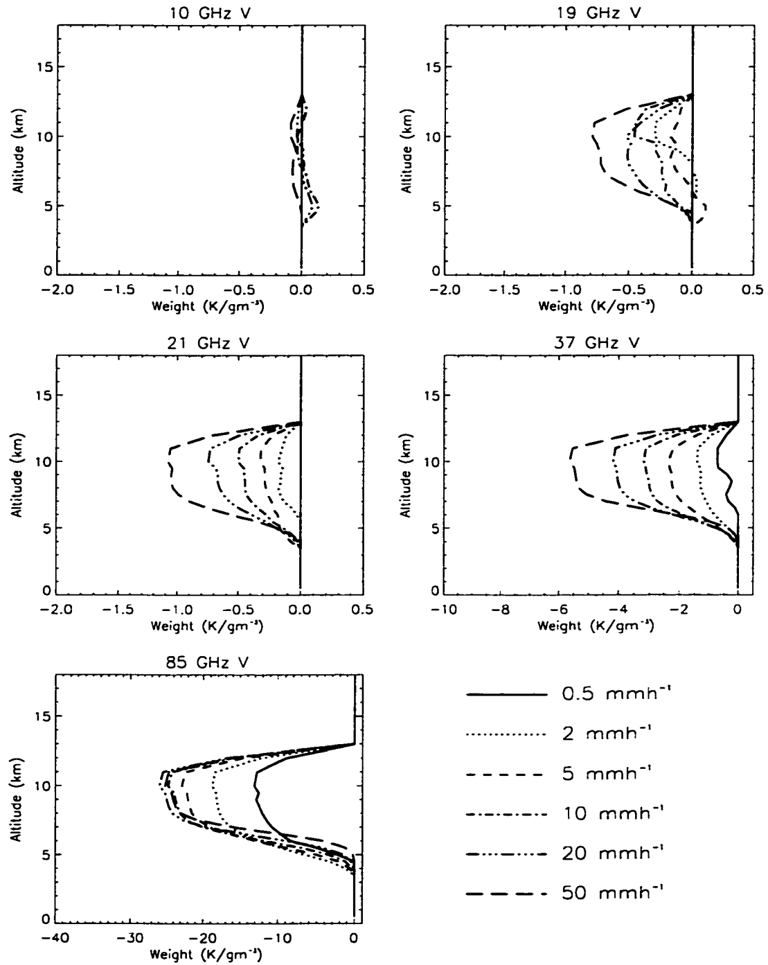
Figure 2.15: Ice water weighting functions for each vertically polarized TMI channel as a function of rainrate over an ocean background.
