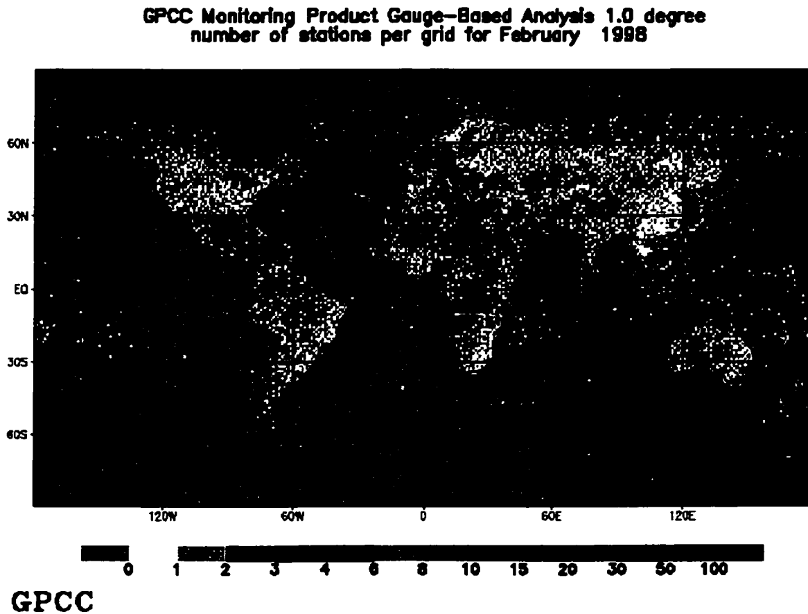
Figure 1.2: Global distribution of rainfall monitoring stations supplying data for the Global Precipitation Climatology Centre's gridded monthly total precipitation product (courtesy of The Global Precipitation Climatology Centre. HTTP://www.dwd.de/research/gpcc ).
