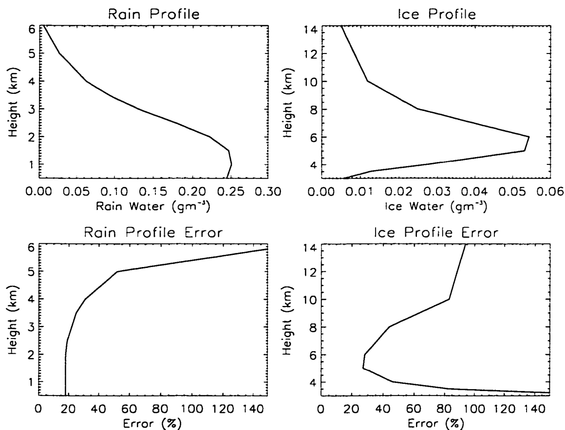
Figure 3.9: Example of retrieved rainfall and precipitation-sized ice hydrometeors and the resulting error profile estimated using our error model for a single pixel of a TRMM orbit.
