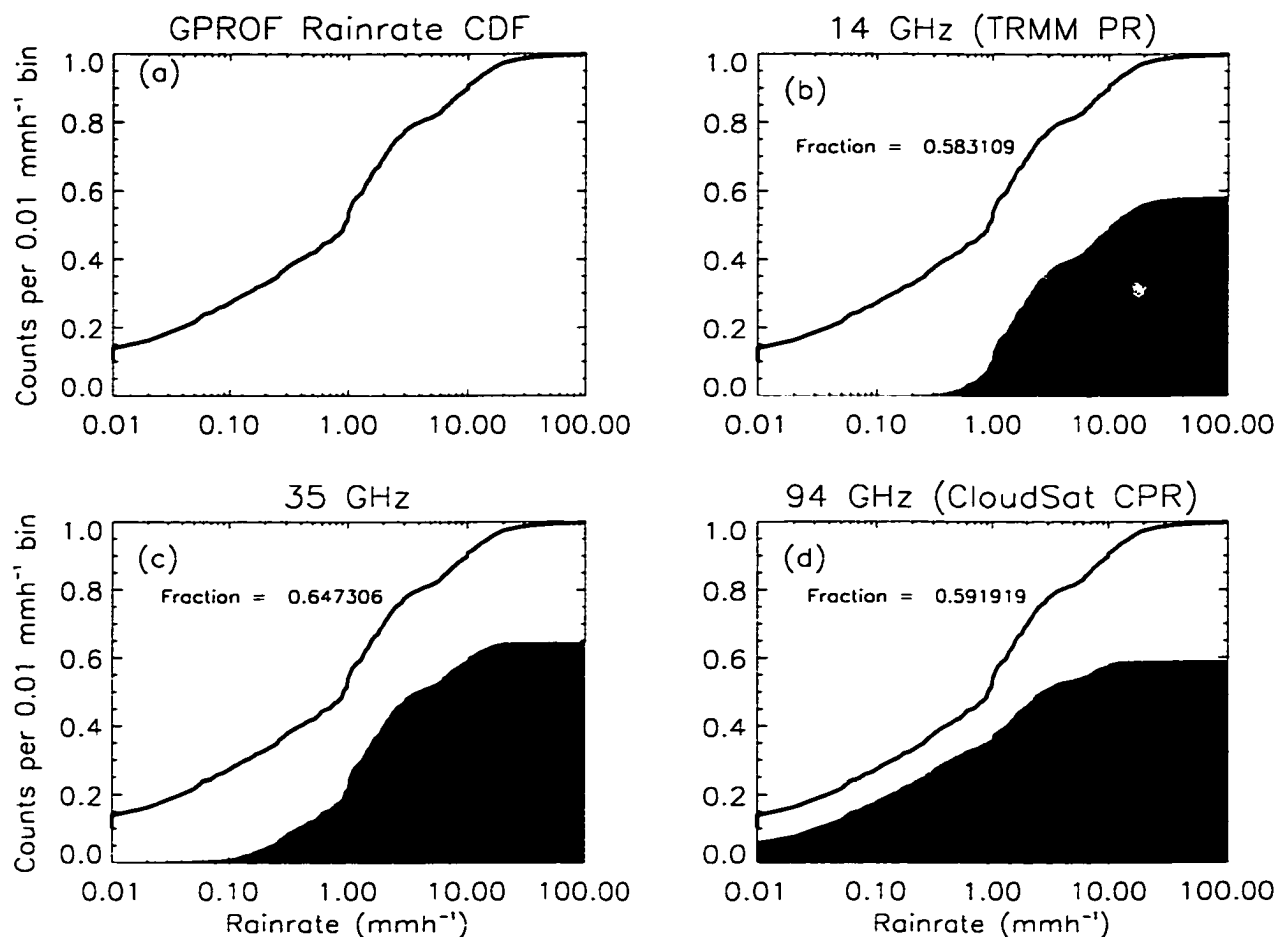
Figure D.6: The results displayed in Figure D.5 expressed in terms of normalized CDFs.
