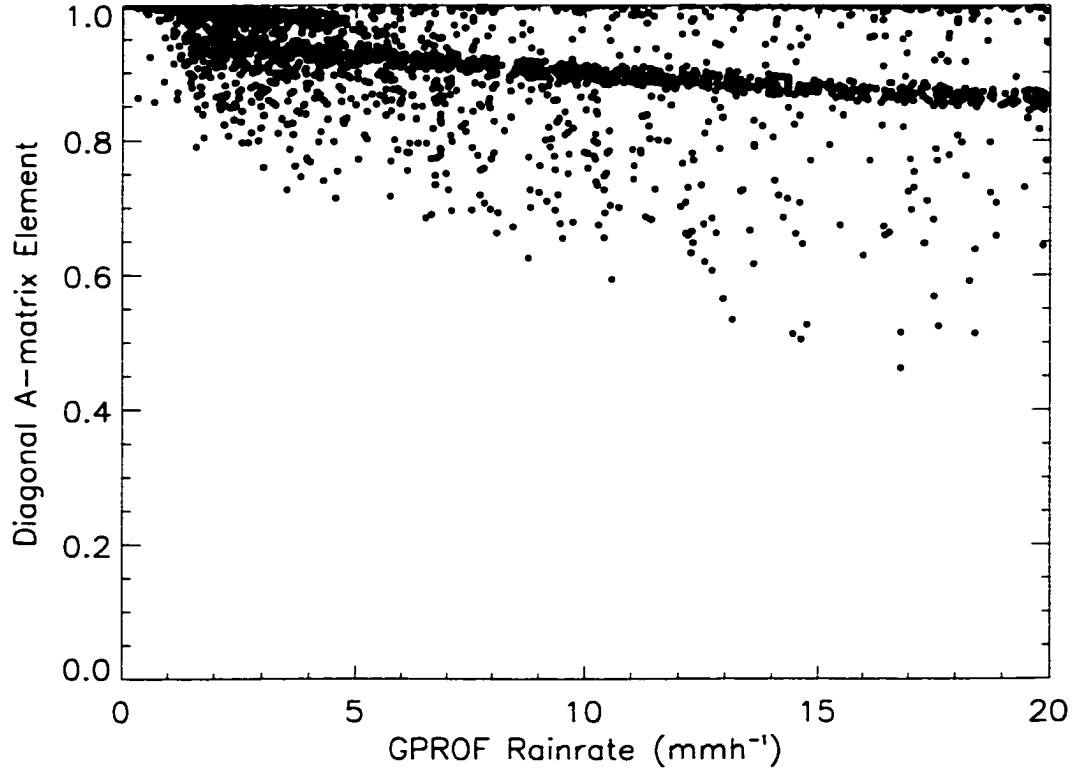
Figure D.20: As in Figure D.18 but at 94 GHz.
