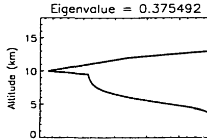
Figure 2.25: Statistically significant orthonormal weighting functions for retrieving ice water profiles at a rainrate of 2.0 \text{ mmh}^{-1} over an ocean background.
