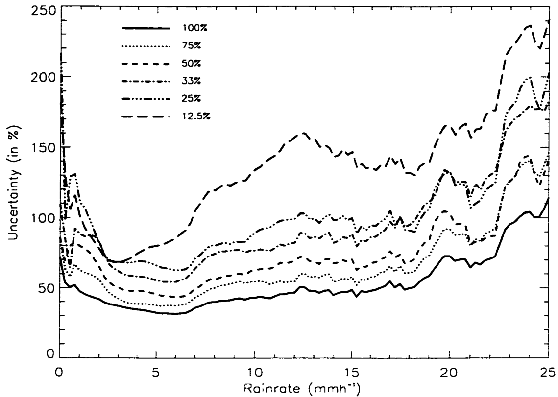
Figure 3.28: Uncertainty in retrieved surface rainrate as a function of database fraction used in the retrieval. The legend provides the percentage of the cloud database which gives rise to each curve.
