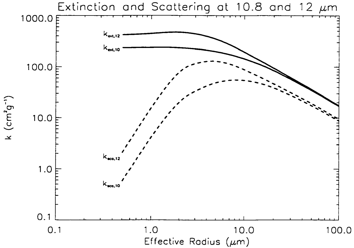
Figure 4.5: Mass extinction (solid curves) and scattering coefficients (dashed curves) at 10.8 and 12 \mu\text{m} plotted as a function of radius for monodispersed spherical ice particles.
