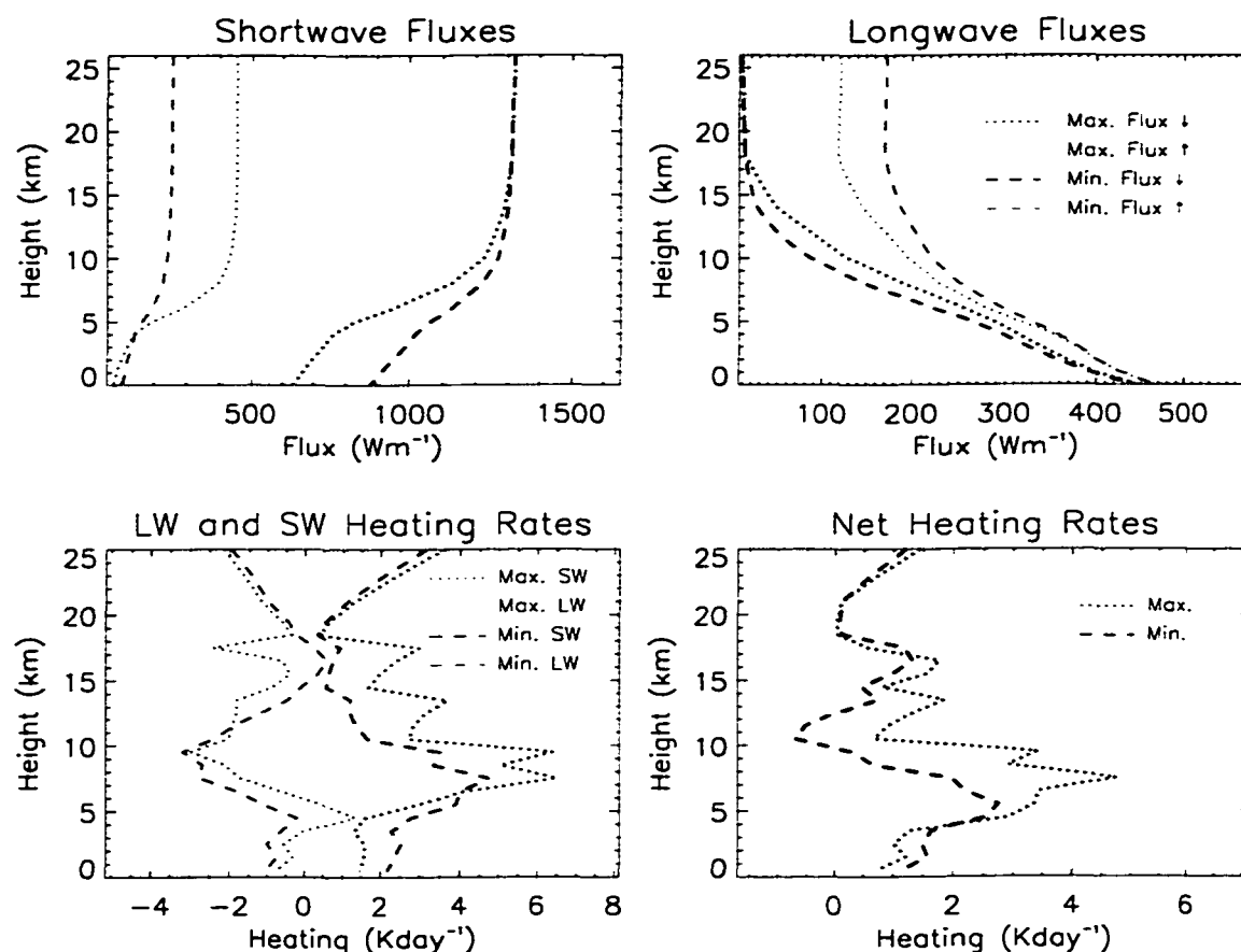
Figure 5.23: Sensitivity of flux and heating rate profiles in light rain to errors in retrieved water contents.
