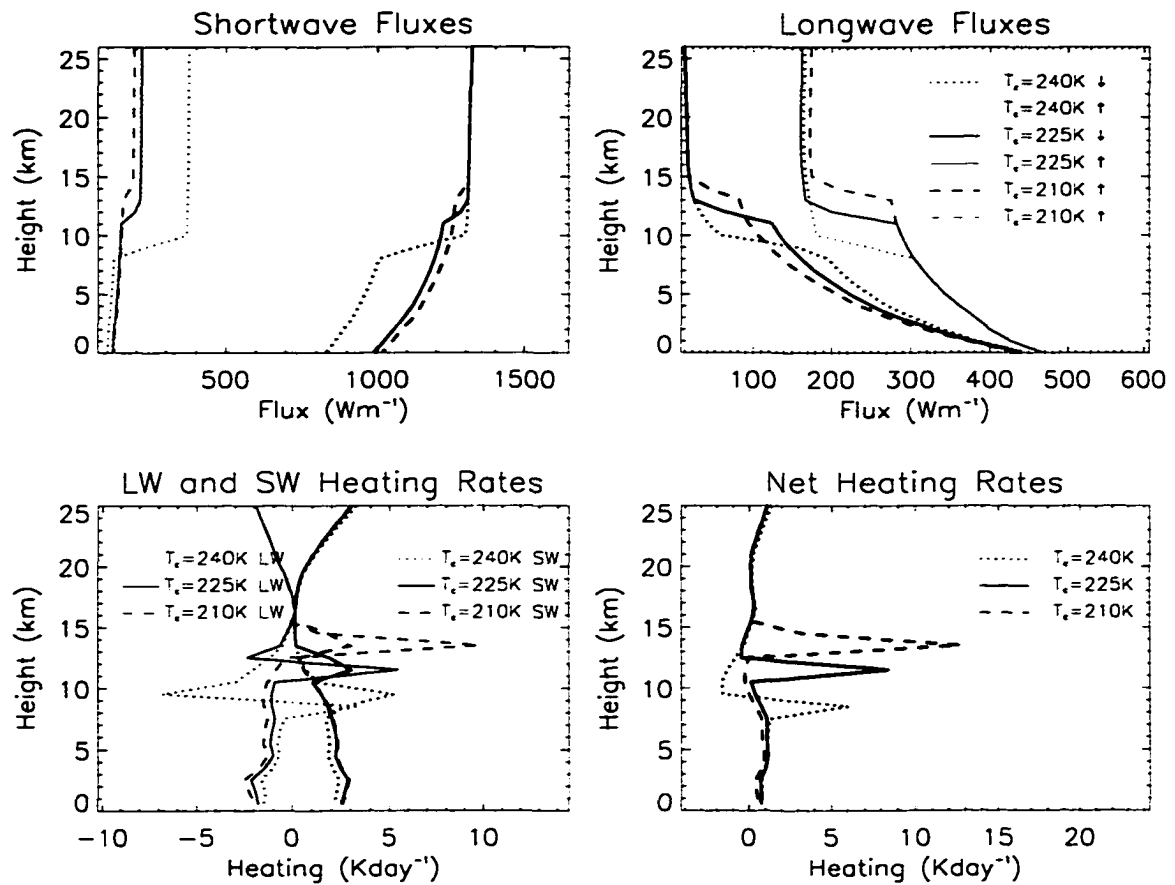
Figure 5.12: As in Figure 5.11 but for a cloud with an IR optical depth three times greater.
