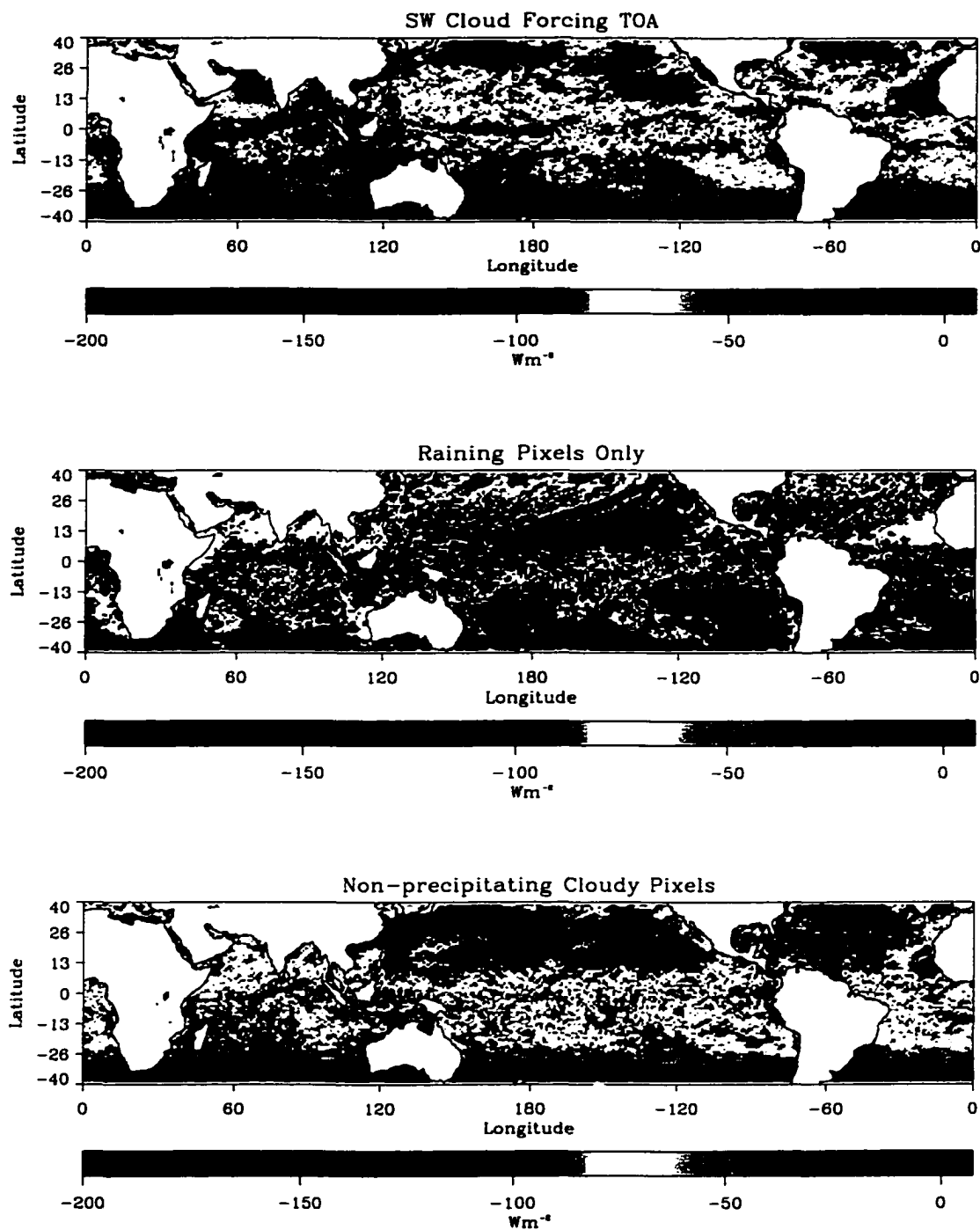
Figure 5.32: Monthly-mean shortwave cloud forcing at the top of the atmosphere for February 1998.
