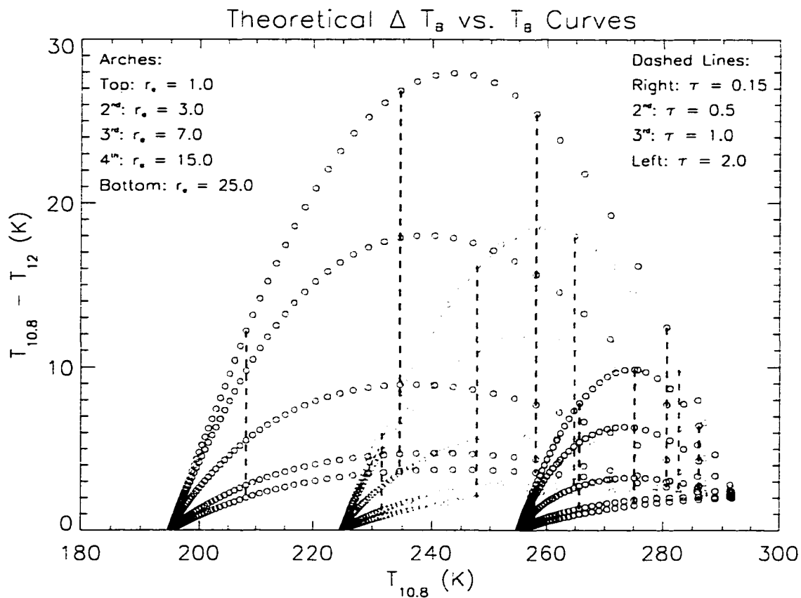
Figure 4.7: 10.8 - 12 \mu\text{m} brightness temperature differences as a function of 10.8 \mu\text{m} T_B for cirrus clouds containing spherical ice particles at 255 K (red), 225 K (green), and 195 K (blue). Radii assumed for each arch are indicated in the left-hand legend while optical depths corresponding to the vertical lines on the figure appear on the right.
