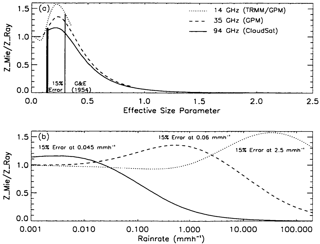
Figure D.1: Ratio of effective reflectivity computed using Mie theory to Rayleigh reflectivity as a function of: (a) effective size parameter, and (b) rainrate.
