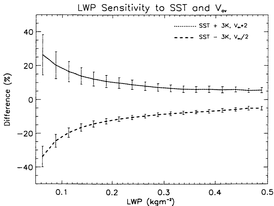
Figure 4.17: Expected range of uncertainty in LWP estimates resulting from errors in assumed SST and surface wind speed, V_{av} .
