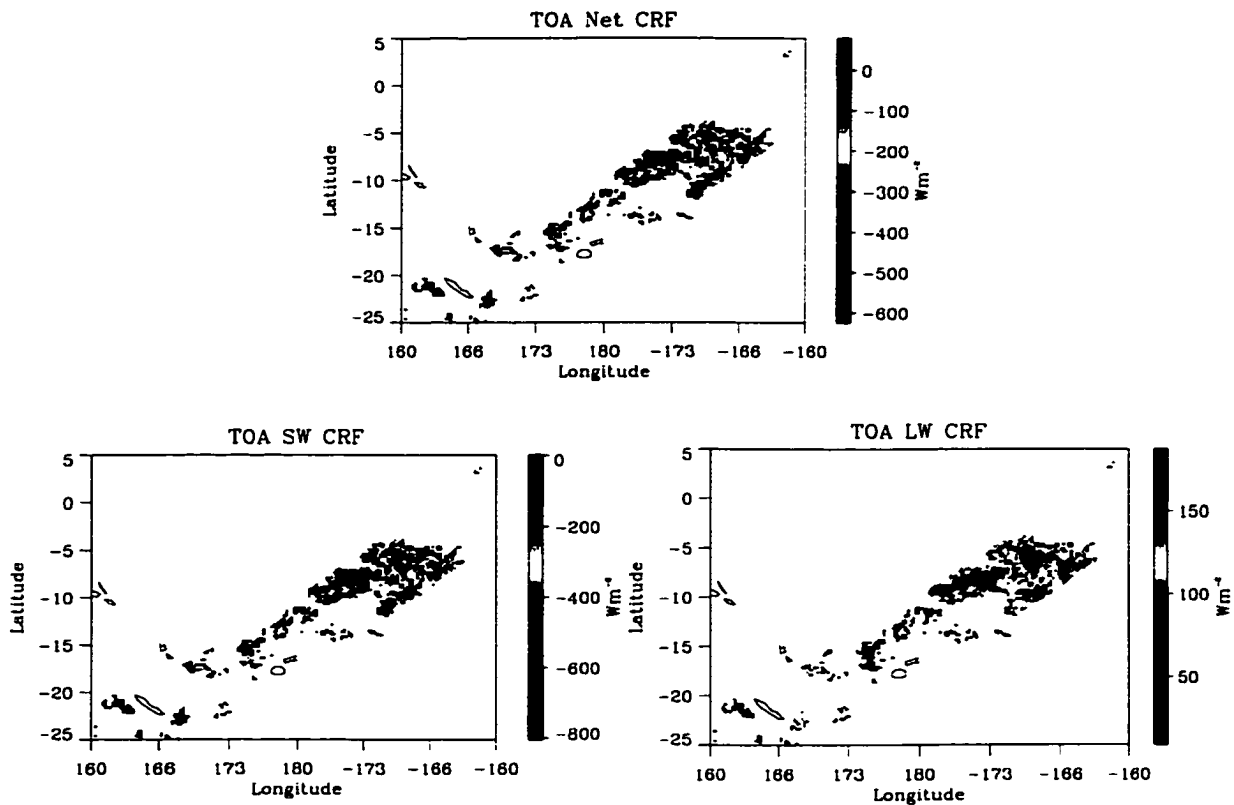
Figure 5.19: Cloud radiative forcing at TOA for precipitating pixels in a section of orbit.
