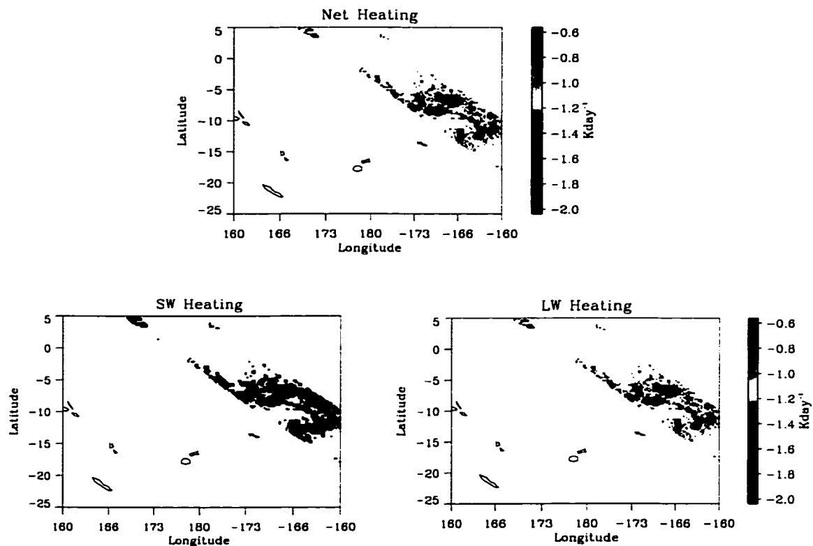
Figure 5.22: As in figure 5.21 but for an overpass at 1:00 am local time.
