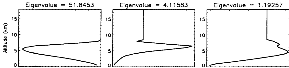
Figure 2.23: As in Figure 2.22 but at a rainrate of 5 \text{ mmh}^{-1} .
