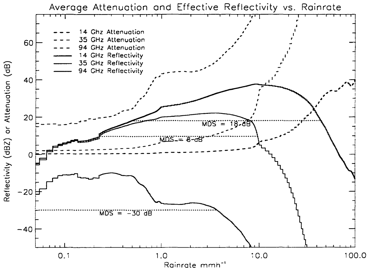
Figure D.7: Average attenuation and attenuation-corrected reflectivity from near surface rainfall plotted as a function of rainrate at 14, 35, and 94 GHz. Black dotted lines indicate the minimum detectable signals of each radar.
