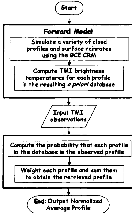
Figure 3.1: Flow chart representation of the 2A12 retrieval algorithm.
