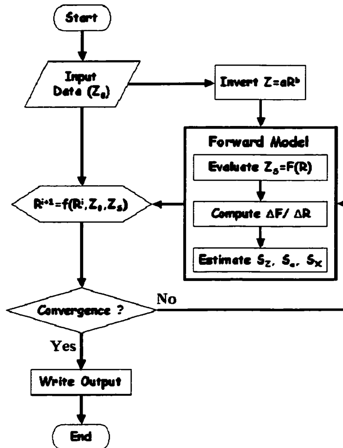
Figure D.14: The CORRAL retrieval algorithm.
