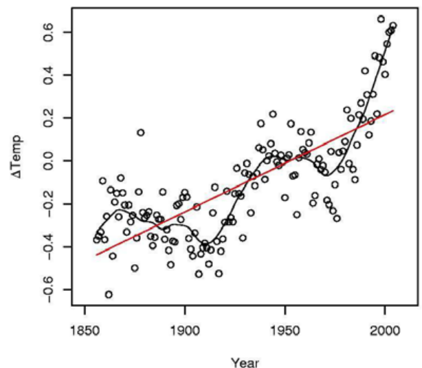
Figure 2. Annual departures from the period-of-record mean northern hemisphere temperature in degrees C, 1856–2004, with least squares fit (red line) and loess smooth (black line). From Cohn and Lins, 2005.
