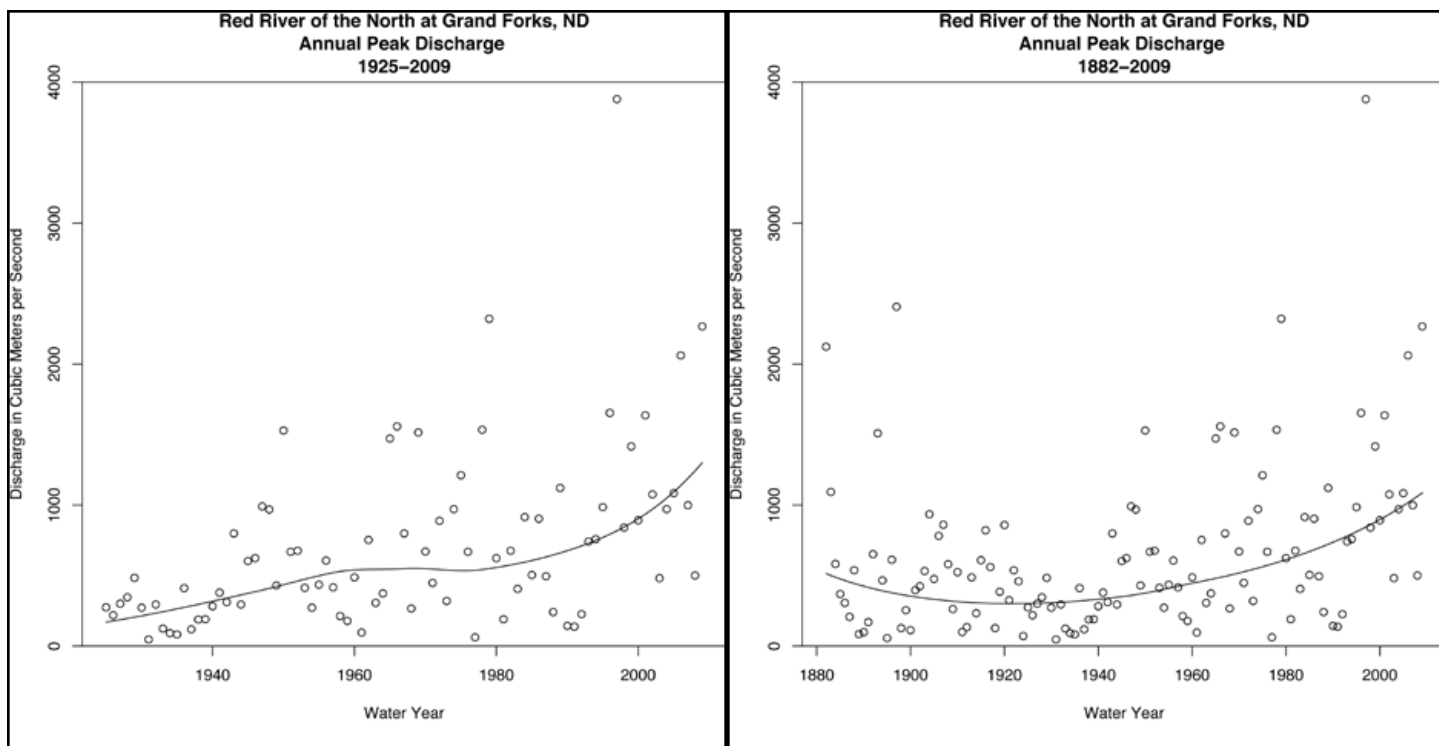
Figure 4. Annual Peak Discharge, Red River of the North at Grand Forks, ND. Solid line is a local polynomial regression fit. Left panel is 1925–2009. Right panel is 1882–2009.
