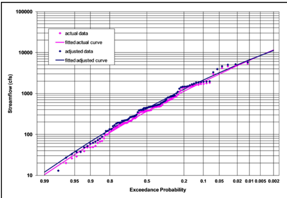
Figure 2b. Frequency analysis with peak flows adjusted for urbanization
