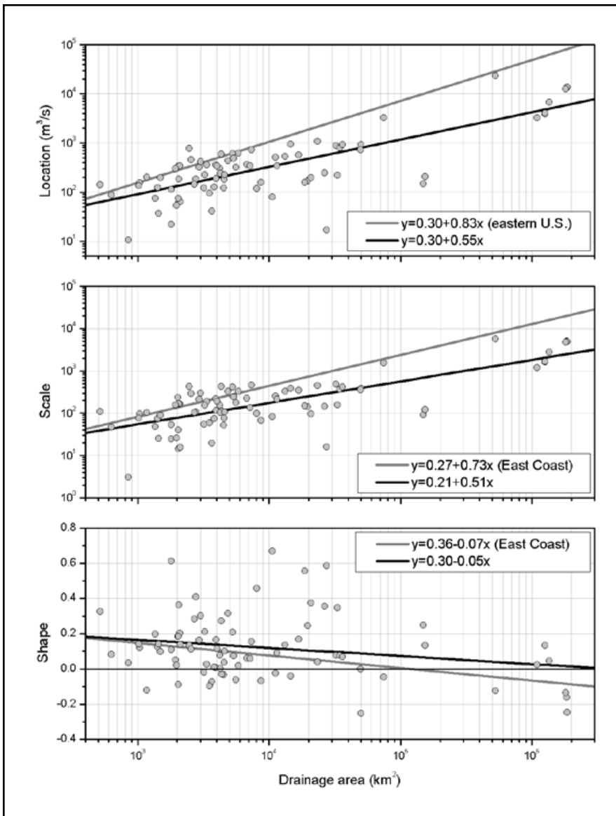
Figure 9. Plot of the parameters of the GEV distribution as a function of drainage area for the series without change-points (in mean and variance) or linear trends. The results for the eastern U.S. are based on the work by Villarini and Smith (2010).
