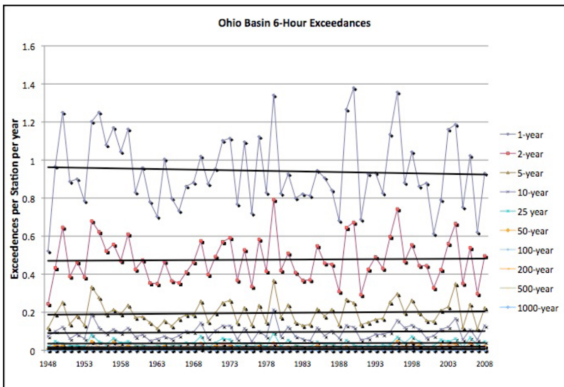
Figure 9. Ohio Basin 6-Hour Exceedances.
