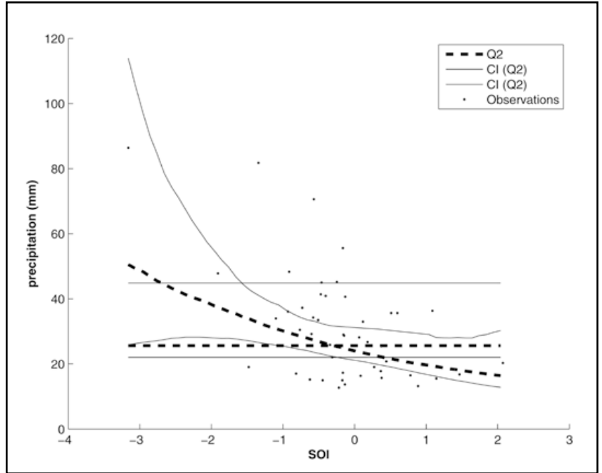
Figure 5. LN3-ML estimates of the medians (quantiles corresponding to the 2-year return period), and 95% confidence intervals conditional on the values of SOI, obtained with the LN3 3,1,1 and LN3 1,1,1 models.
