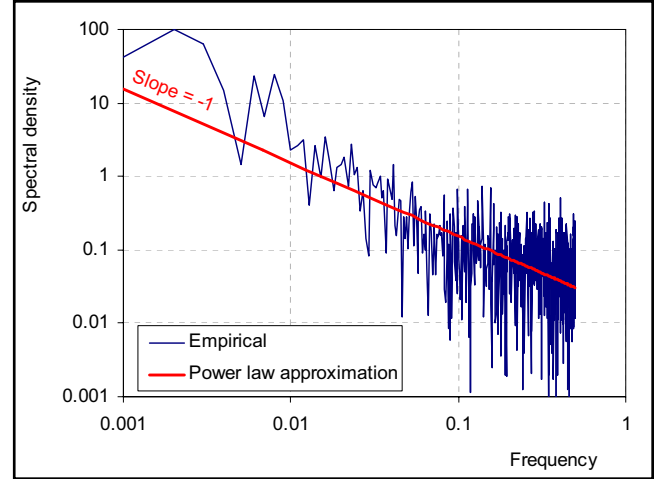
Figure 7. Empirical power spectrum of the time series of Figure 3.
