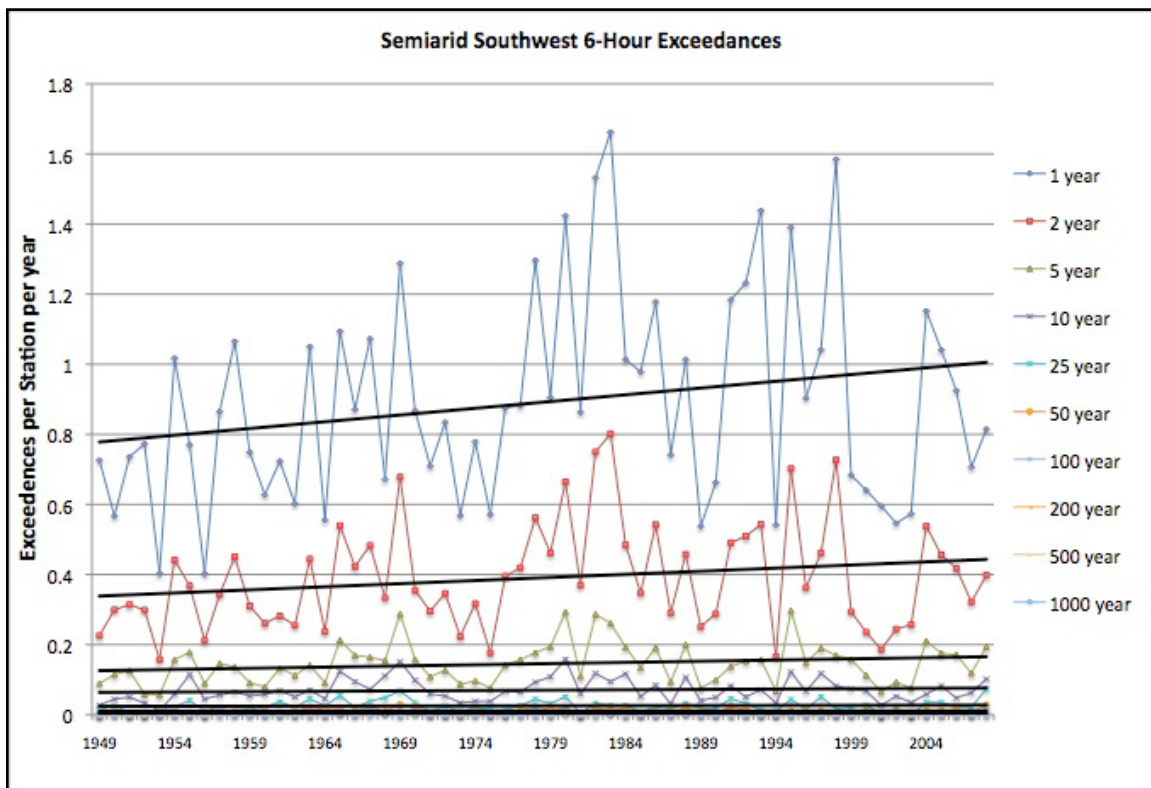
Figure 2. Semi-arid Southwest 6-Hour Exceedances.
