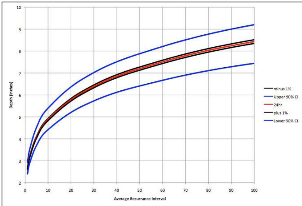
Figure 18. The effect of a 1% increase or decrease in exceedances per station per century is very small compared with the upper and lower 90% confidence intervals about the precipitation frequency estimates.
