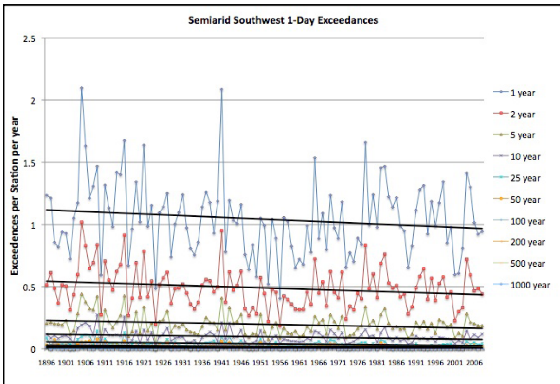
Figure 3. Semi-arid Southwest 1-Day Exceedances.
