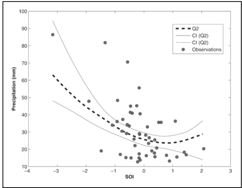
Figure 3. GML estimates of the medians and 95% credible intervals conditional on the values of SOI, obtained with the GEV_{3,1} model.
