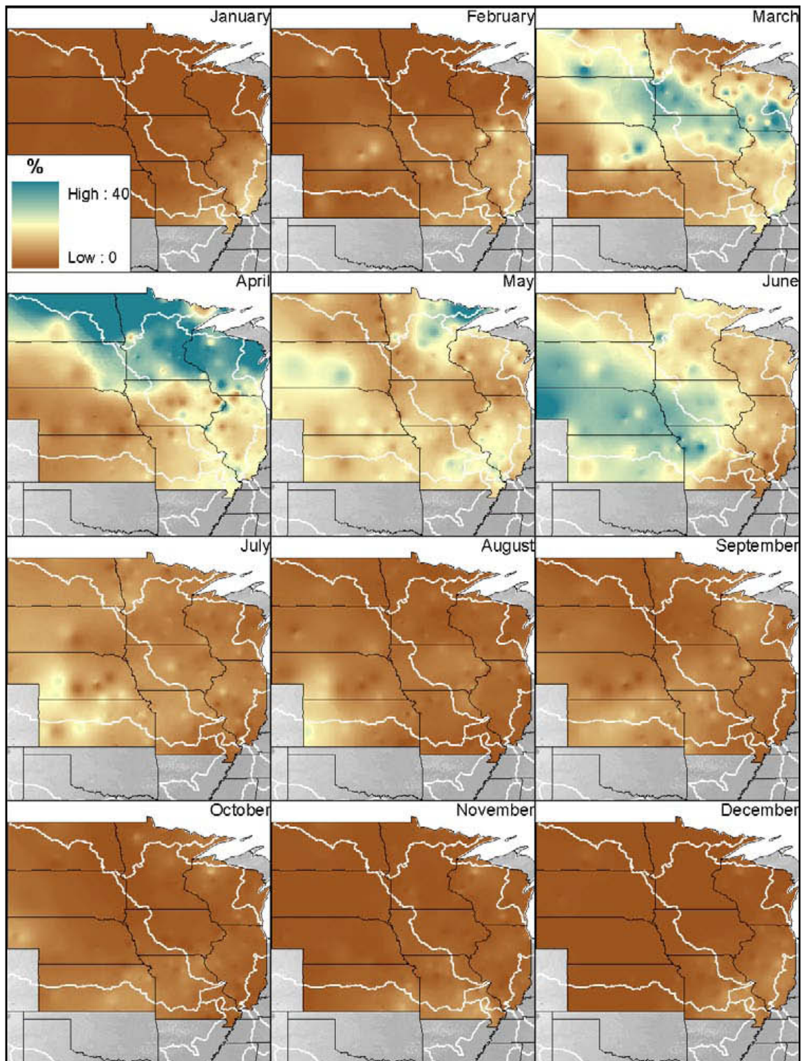
Figure 6. Maps showing the frequency of the annual maximum peak discharge for each month of the year.
