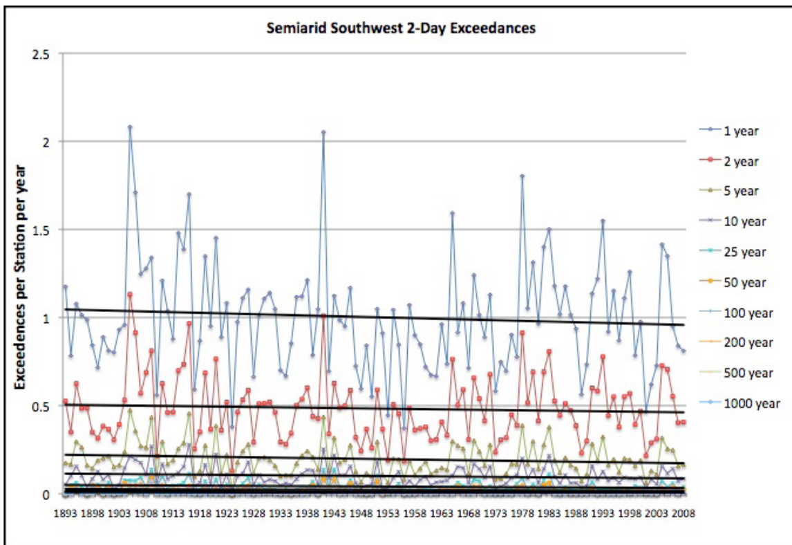
Figure 4. Semiarid Southwest 2-Day Exceedances.
