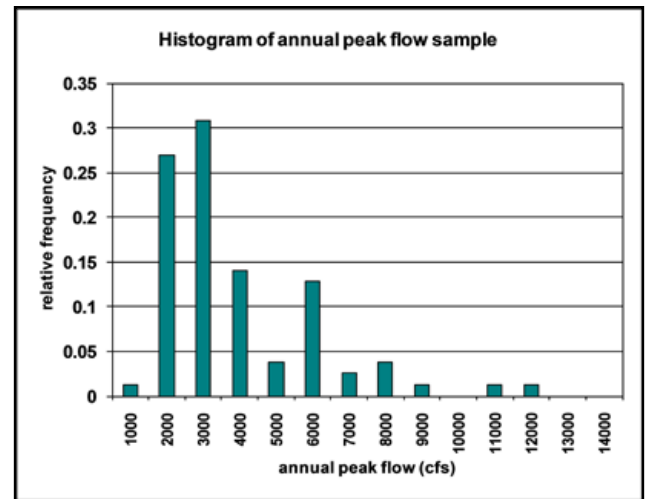
Figure 1b. Histogram of annual peak flow
