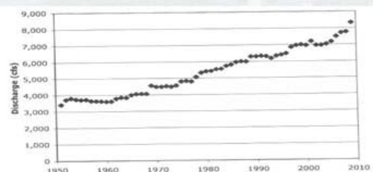
Figure 2. Retrospective 50-year moving average of natural annual maximum mean daily flow - Red River at Fargo
