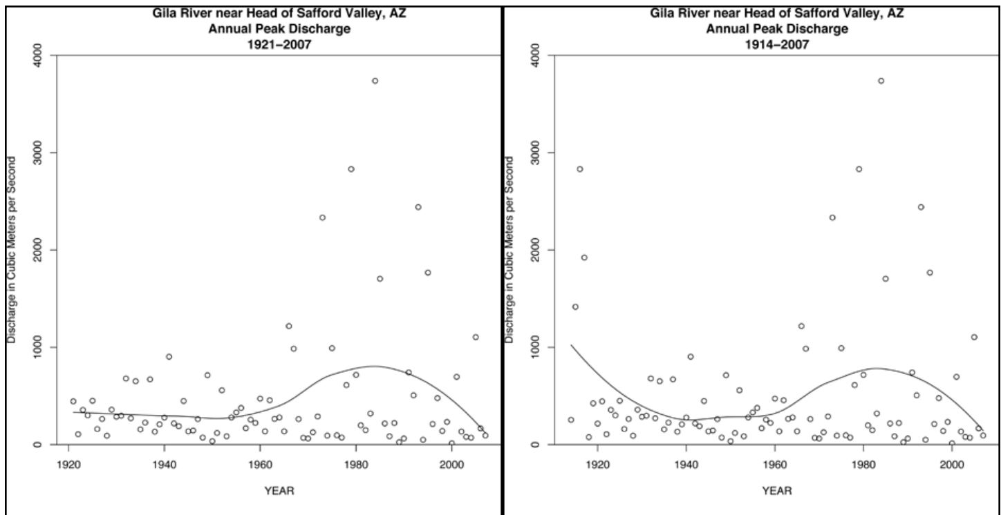
Figure 5. Annual Peak Discharge, Gila River near Head of Safford Valley, AZ. Solid line is a local polynomial regression fit. Left panel is 1921-2007. Right panel is 1914-2007
