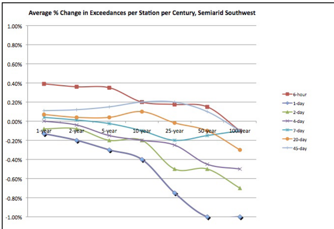
Figure 16. Average Percentage Change in Exceedances per Station per Century for the Semiarid Southwest Study Area.
