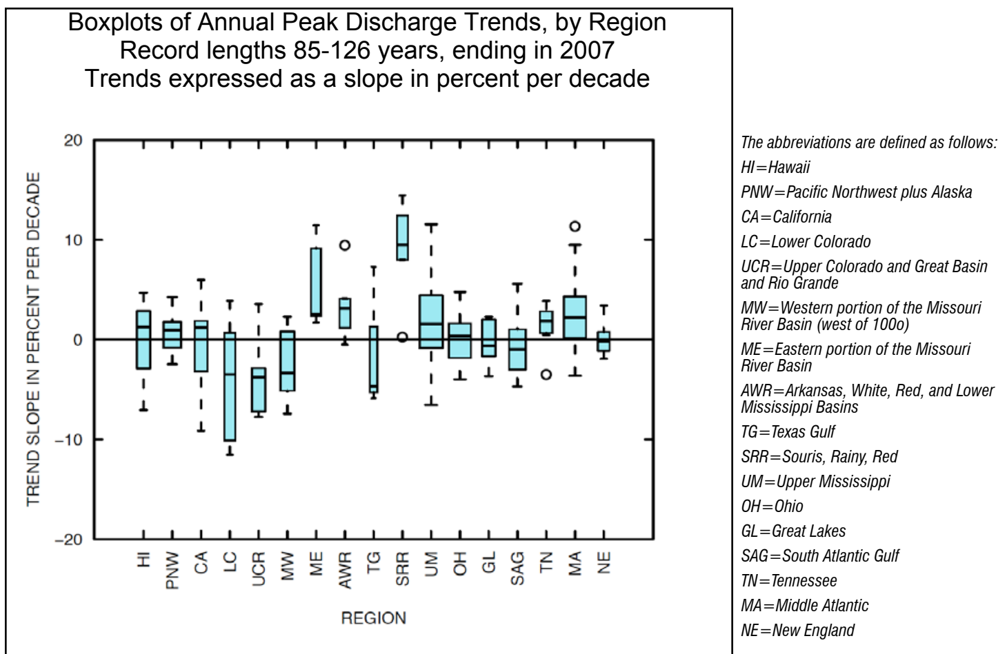
Figure 7. Boxplots of Annual Peak Discharge Trends, by Region. Record lengths range from 85-126 years, all ending in Water Year 2007. Trend slopes are expressed as percentage change per decade, based on a linear regression of the log of the annual peak discharge versus Water Year. Box widths are proportional to the square root of the sample size. The Regions are based on the Water Resources Regions of the US, with some modifications.
