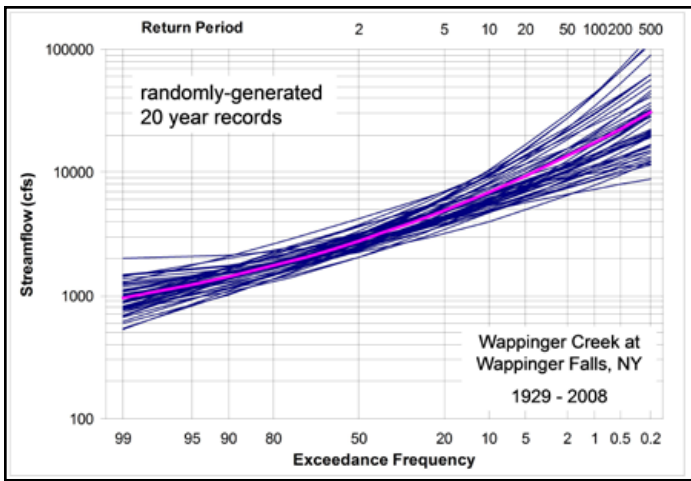
Figure 5c. Frequency curves fit to random 20-member samples from assumed frequency curve
