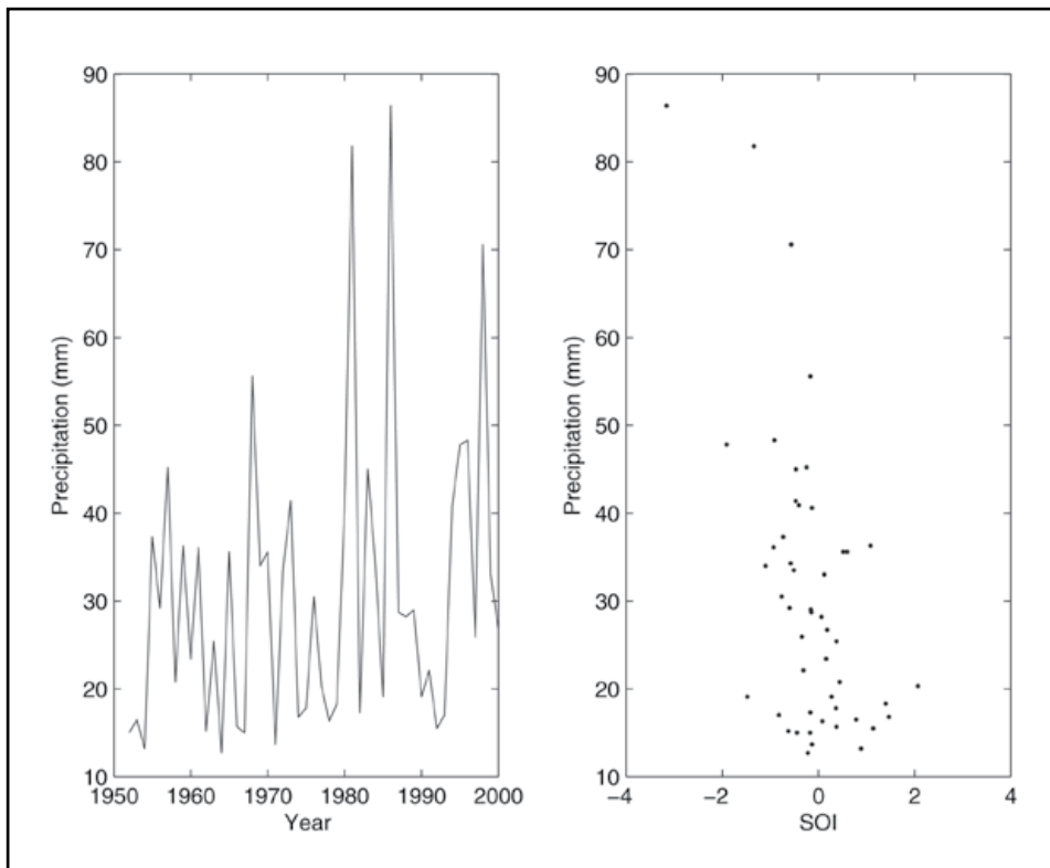
Figure 1. a) Annual maximum precipitation time series at Tehachapi station, and b) scatter plot of observed annual maximum precipitations and corresponding SOI values.
