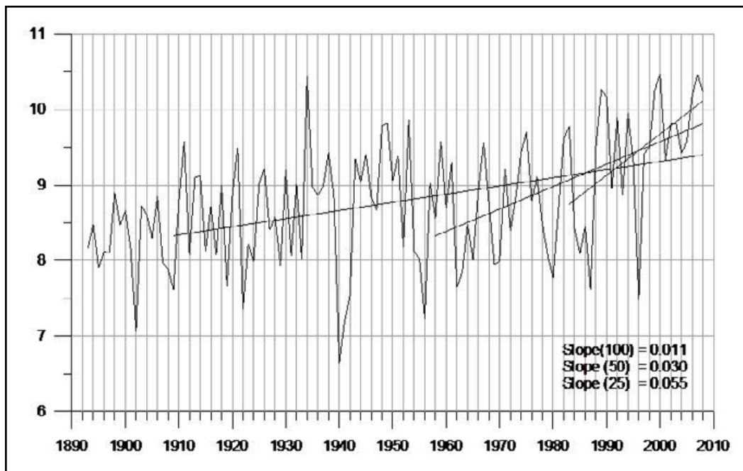
Figure 1. Changes in mean annual temperature in Potsdam.
