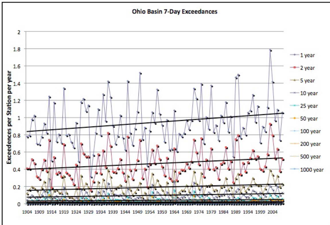
Figure 13. Ohio Basin 7-Day Exceedances.
