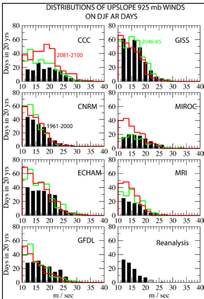
Figure 5. Same as Figure 4, except for upslope winds on AR days.
