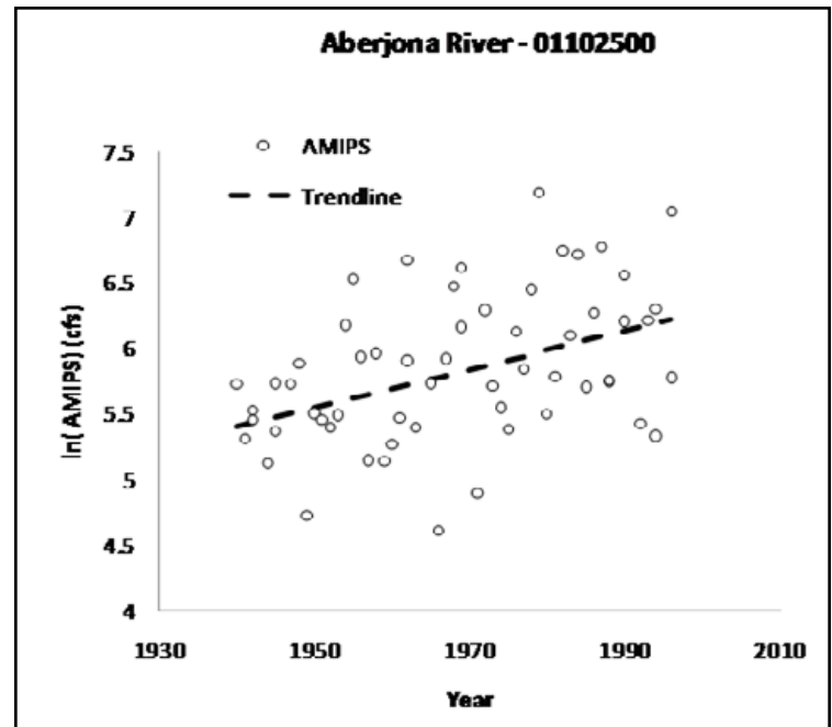
Figure 1. Example of trend in the logarithms of the AMIPS for Aberjona River in Massachusetts ( \hat{\beta} = 0.0146 )
