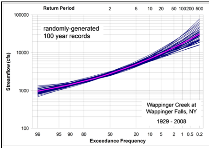
Figure 5e. Frequency curves fit to random 100-member samples from assumed frequency curve
