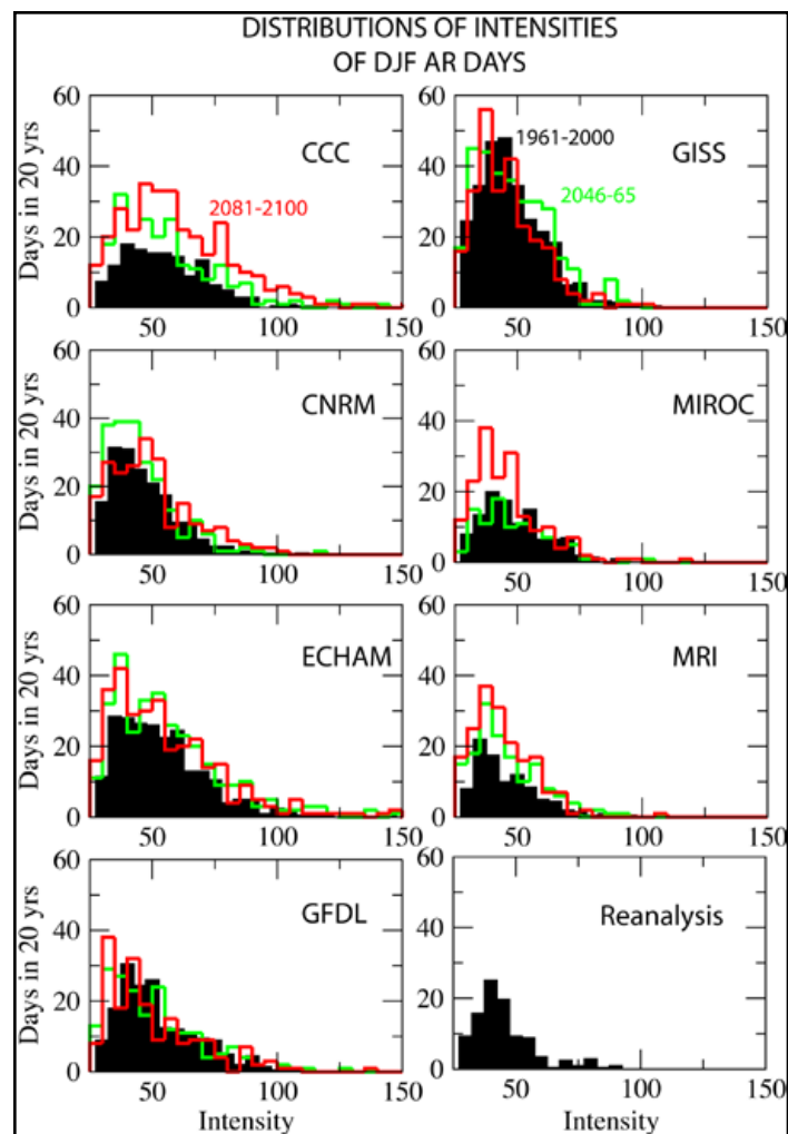
Figure 6. Same as Figure 4, except for intensities (IWW * upslope wind) on AR days.
