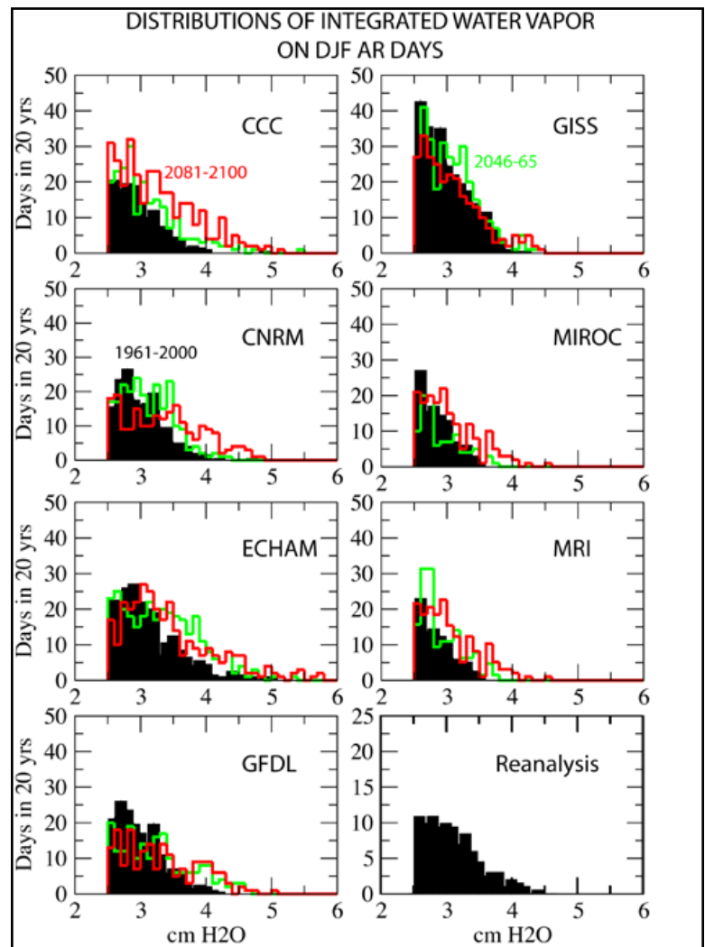
Figure 4. Histograms of simulated historical (20c3m, black) and future (A2, green and red) distributions of integrated water vapor values associated with AR-days in seven climate models and the NCAR-NCEP Reanalysis of historical observations.
