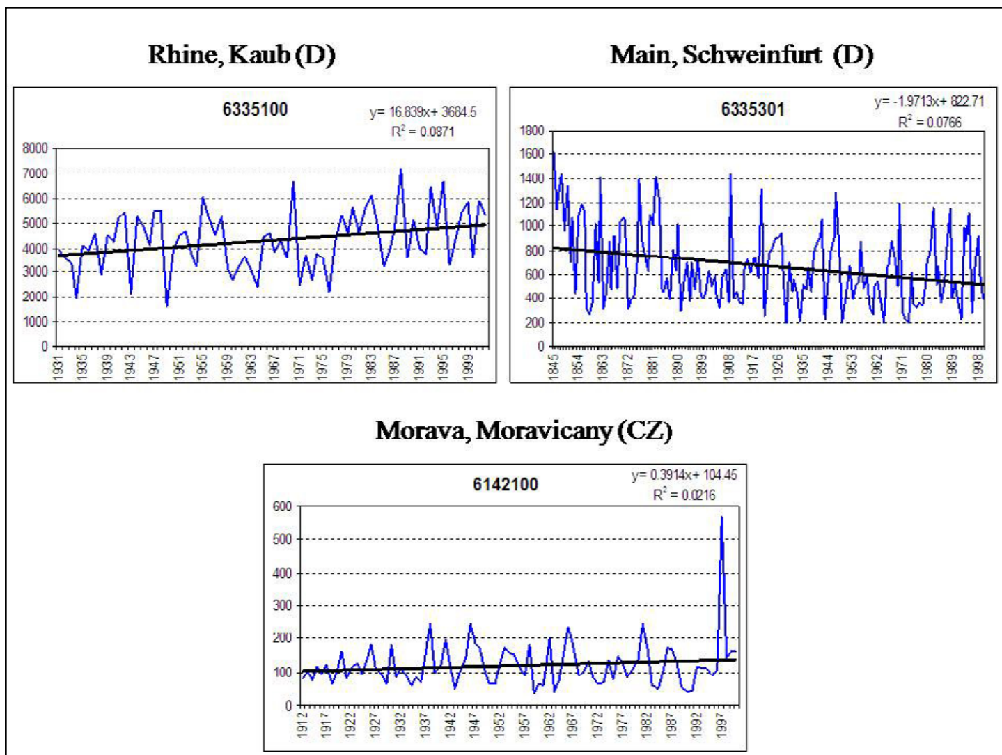
Figure 3. Examples of time series of annual maximum discharge of European rivers.
