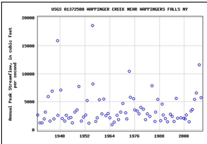
Figure 1a. Annual Peak Flow on Wappinger Creek
