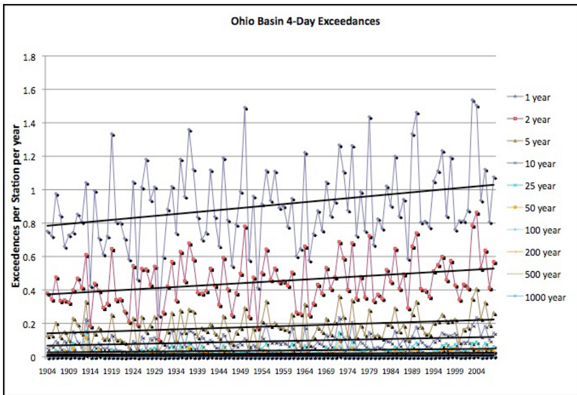
Figure 12. Ohio Basin 4-Day Exceedances.
