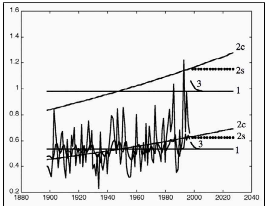
Figure 2. Mean and 50-year flood levels over historical record and planning period, for Hannibal record using three flood risk models. (1) LN-iid; (2) LN-Trend, continues [C] or stops [S]; (3) LN-ARMA(2, 1) one-step ahead forecast over historical period and forecast for beyond historical record (flood flows in million cfs).
