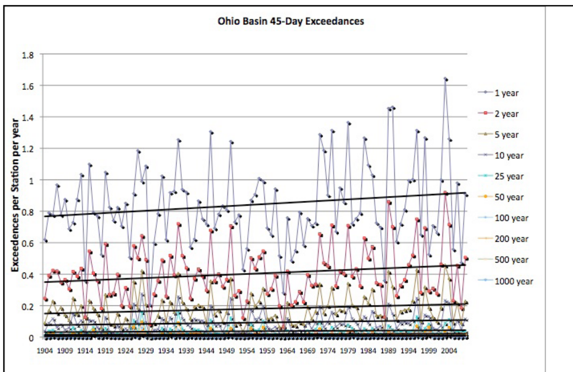
Figure 15. Ohio Basin 45-Day Exceedances.
