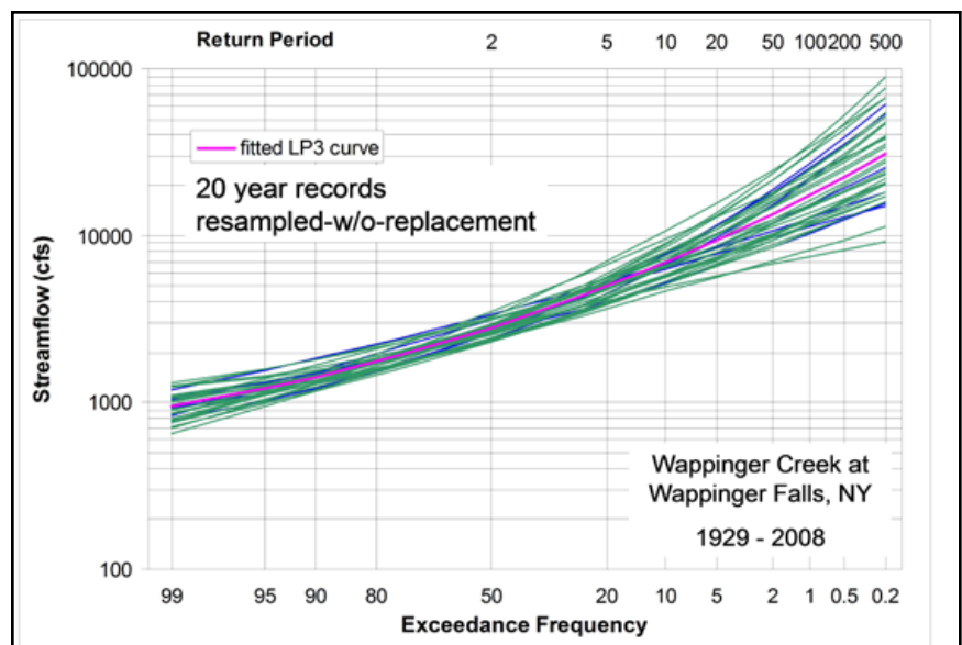
Figure 5b. Frequency curves fit to re-sampled 20-year sets from an 80-year flow record
