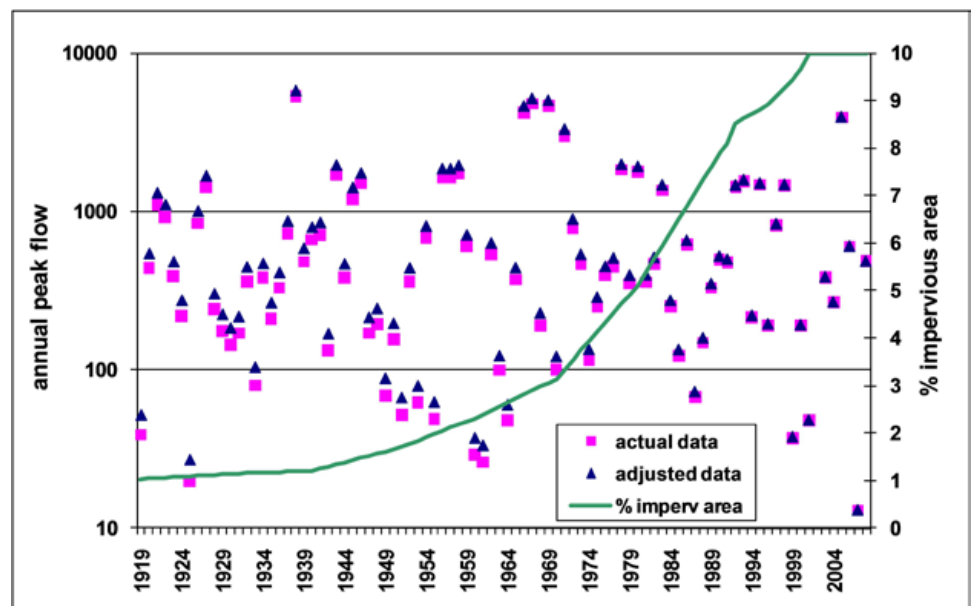
Figure 2a. Peak flows adjusted to current urbanization
