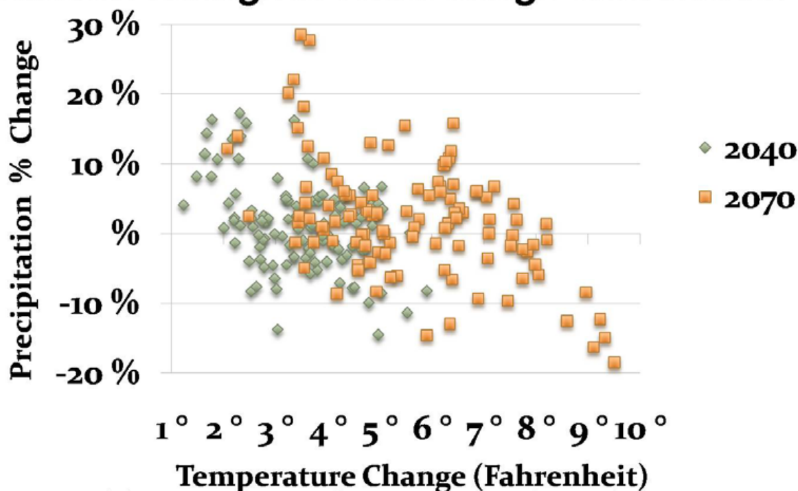
Figure 1. Presented changes are comparisons of 30 year averages around 2040 and 2070 to 1950-1999 averages based on 112 statistically downscaled projections from 16 climate models used to simulate low, medium and high emission paths. Information courtesy of the Joint Front Range Climate Change Vulnerability Study.
