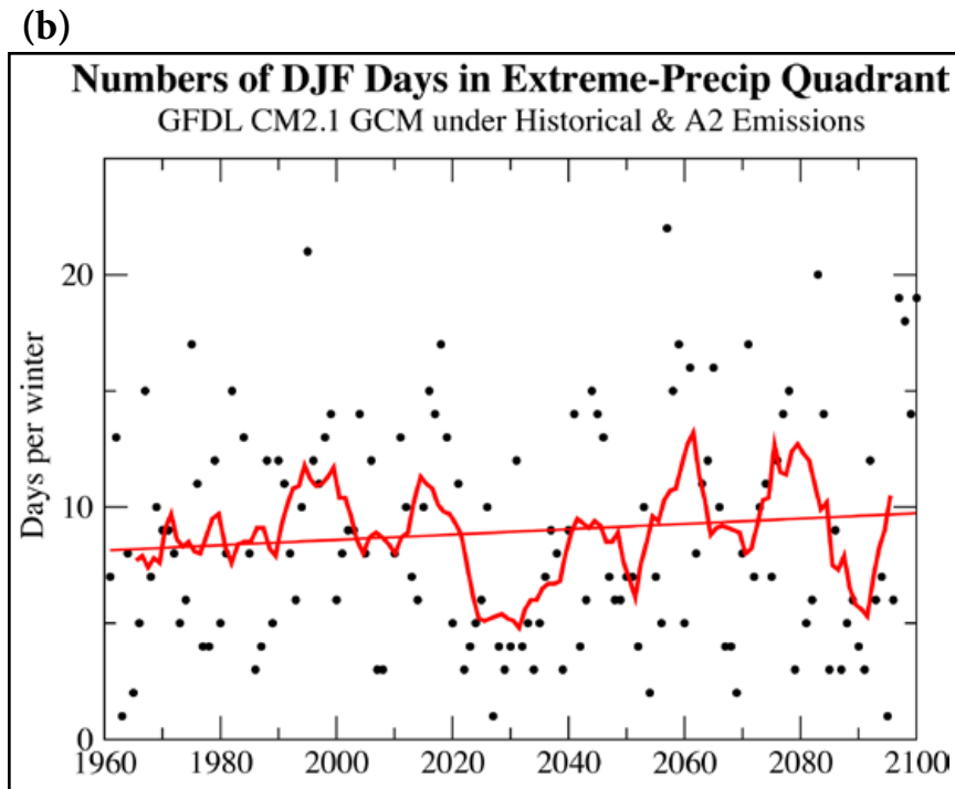
Figure 2. Plot of daily December-February integrated water vapor (IWV) and upslope wind values from GFDL CM2.1 climate model (a) and numbers of days per winter falling into the upper right quadrant of that plot (b), under evolving 20th and 21st century climate changes with A2 greenhouse-gas emissions. Thin red line in panel (b) is a linear fit to data; thicker red curve is a 7-yr moving average of data.
