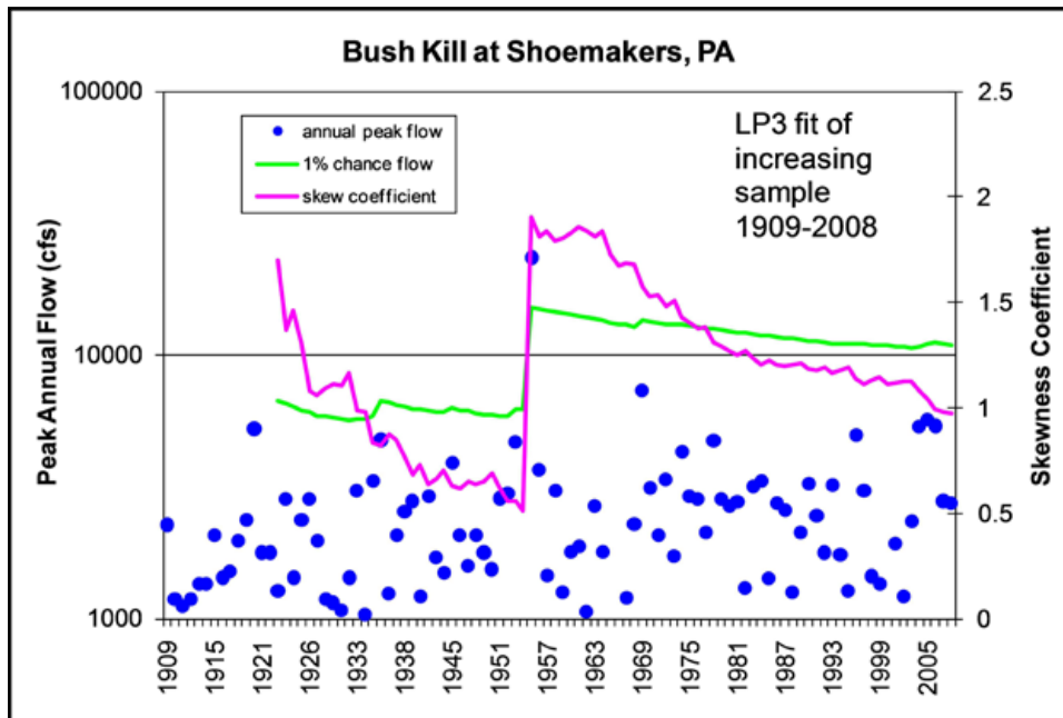
Figure 3. Skew coefficient and 1% LP3 quantile for increasing record
