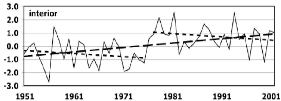
Figure 3. Annual departures from the period of record mean temperature in degrees C for Alaska's Interior climate region from 1951 to 2001. The least squares linear regression lines for 1951–2001, 1951–75, and 1977–2001 are included. From Hartmann and Wendler, 2005.
