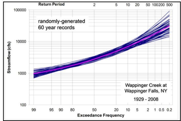
Figure 5d. Frequency curves fit to random 60-member samples from assumed frequency curve
