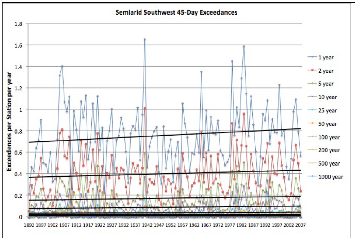
Figure 8. Semiarid Southwest 45-Day Exceedances.
