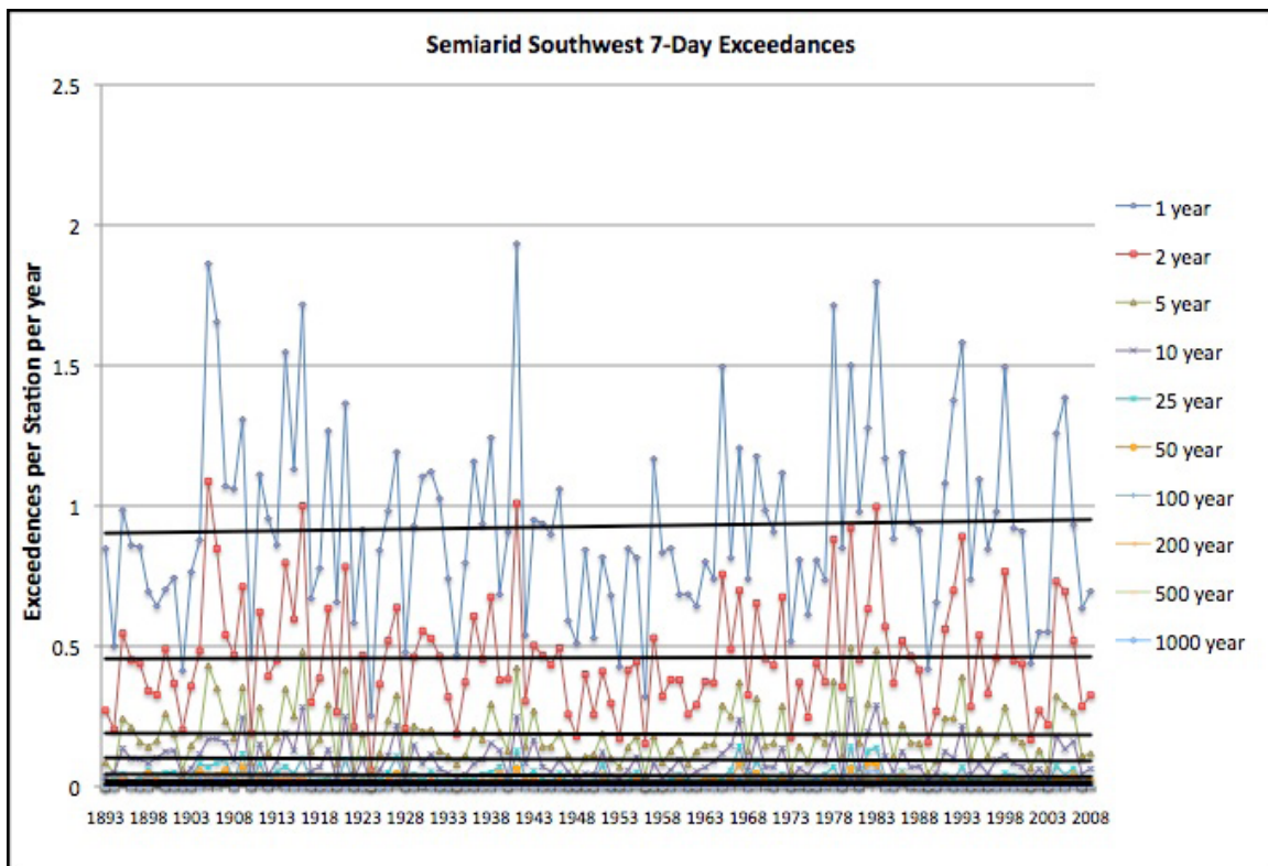
Figure 6. Semiarid Southwest 7-Day Exceedances.
