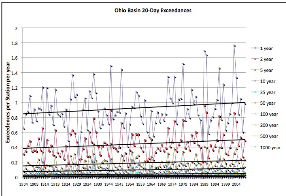
Figure 14. Ohio Basin 20-Day Exceedances.
