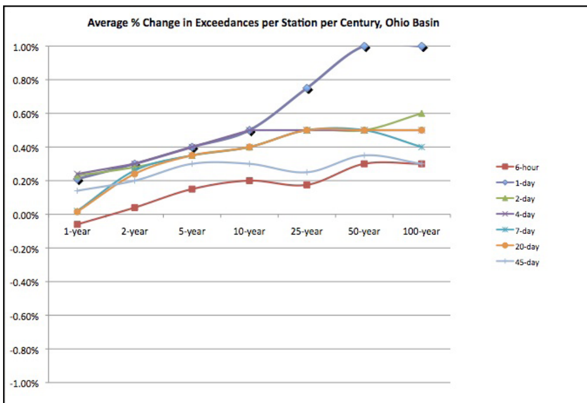
Figure 17. Average Percentage Change in Exceedances per Station per Century for the Ohio River Basin and Surrounding States Study Area.
