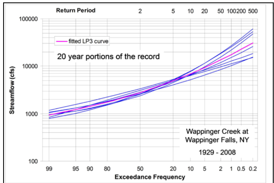
Figure 5a. Frequency curves fit to 20-year portions of an 80-year flow record
