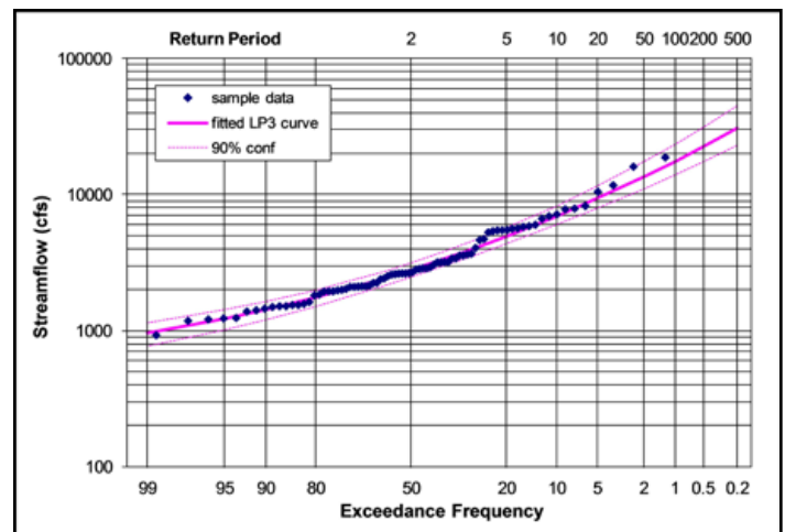
Figure 1d. Cumulative frequency curve and plotted data
