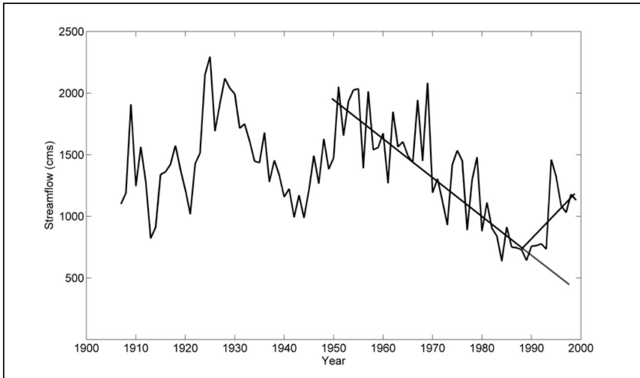
Figure 6. Streamflows at the Koulikoro station on the Niger River Basin, Africa, and errors resulting from direct extrapolation of observed records.
