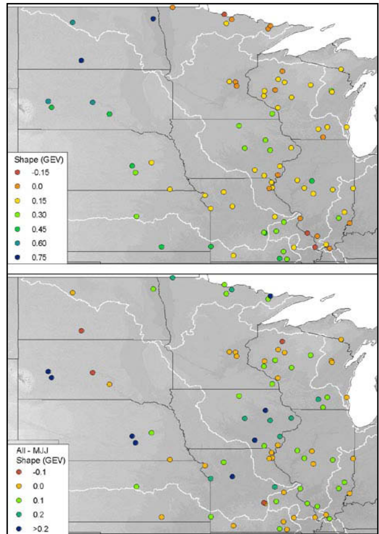
Figure 12. Map of the shape parameters of the GEV distribution for the series without change-points (in mean and variance) or linear trends (upper panel) and map with the differences in the shape parameter between the entire record and the record after removing peaks during the May-June-July period.
