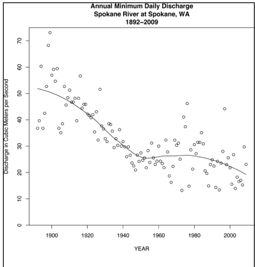
Figure 2. Annual Minimum Daily Discharge, Spokane River at Spokane, WA, 1892-2009. Solid line is a local polynomial regression fit.
