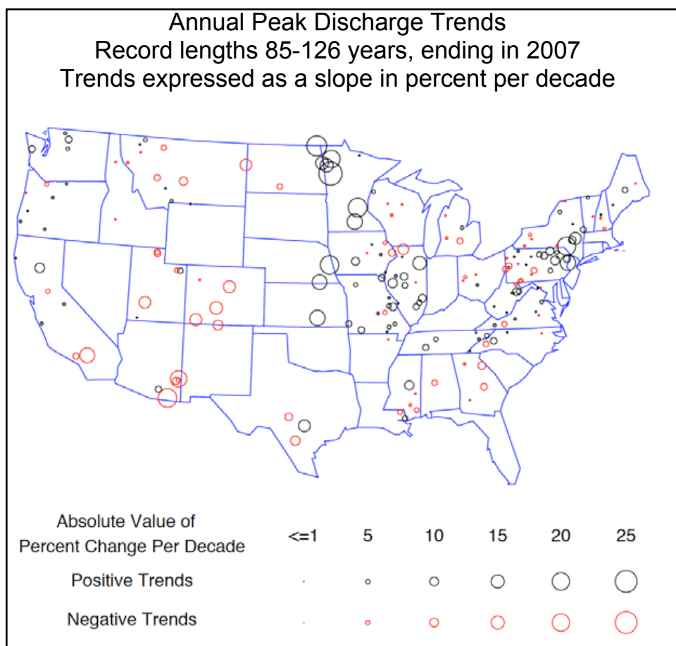
Figure 6. Annual Peak Discharge Trends. Record lengths range from 85-126 years, all ending in Water Year 2007. Trend slopes are expressed as percentage change per decade, based on a linear regression of the log of the annual peak discharge versus Water Year. The black circles indicate upwards trends, and red circles indicate downward trends. Circle diameters are proportional to trend magnitude.
