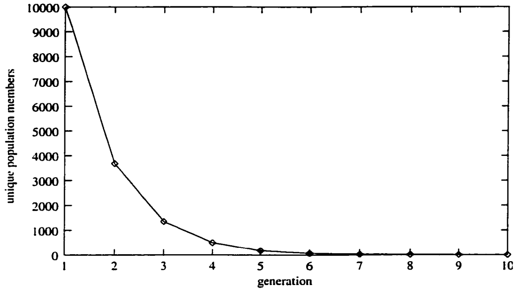
Figure 3.20: The expected number of unique population members in each generation given a population of 10,000 unique population members and a uniform distribution. Only the resampling operation is applied for each next generation.
