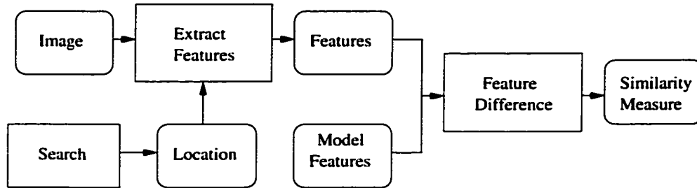
Figure 1.2: Adding Location to Classification by Transforming Image Features to Match the Model
