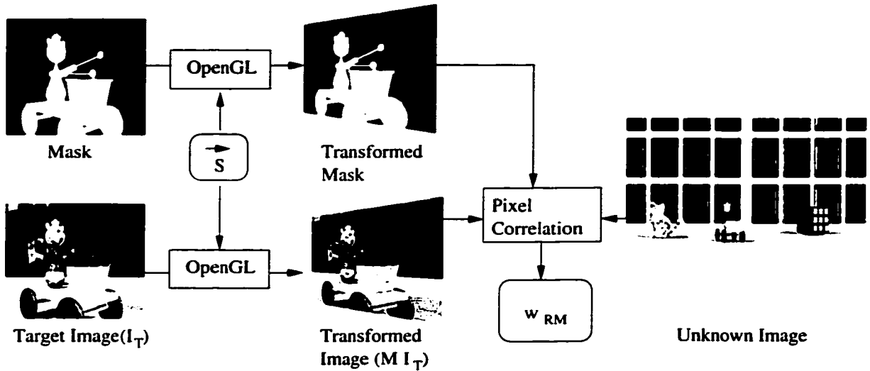
Figure 4.11: Implementation of the render-match algorithm using OpenGL. Note, the same process is used to implement the color index algorithm, except “Pixel Correlation” is replaced with “Color Index.”
