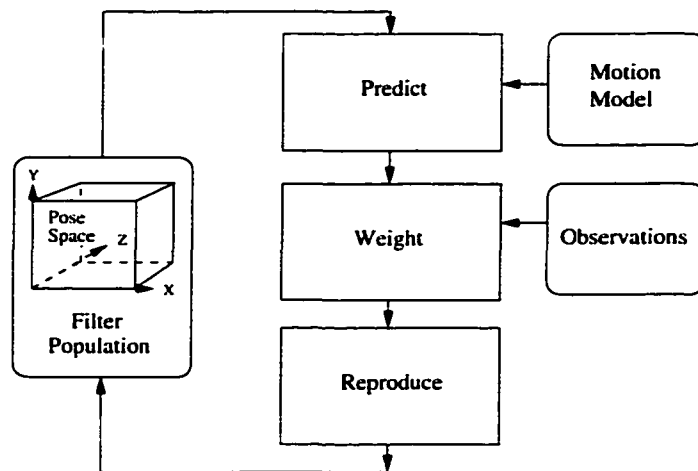
Figure 1.6: Top-level architecture of the canonical Condensation Filter
