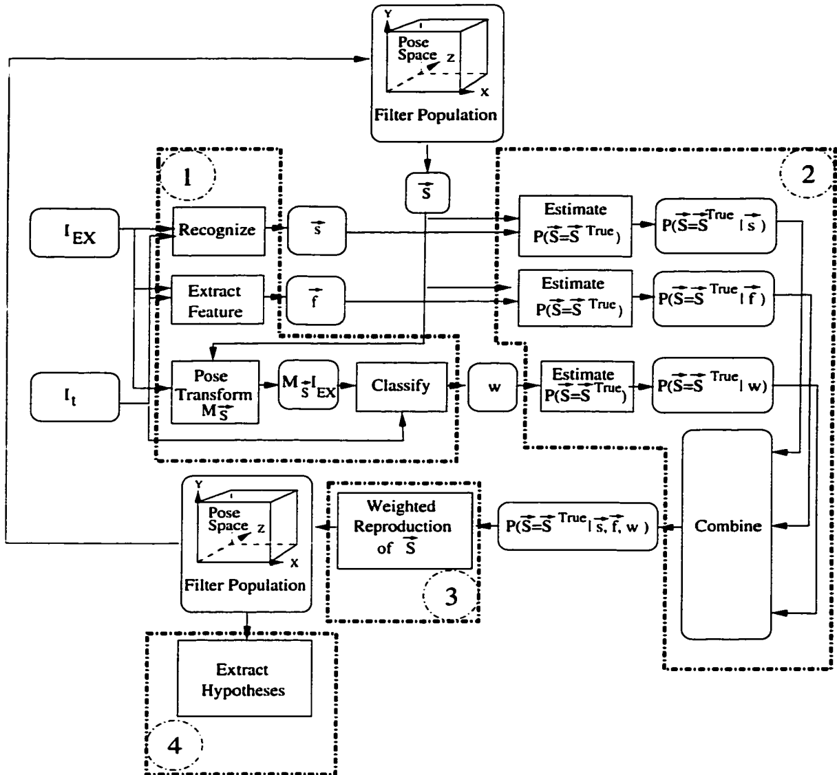
Figure 1.9: Fundamental stages within the Condensation Filter extensions: 1 - Independent Expert Estimates, 2 - Combining Independent Estimates, 3 - Weighted Reproduction, 4 - Extract Hypotheses.
