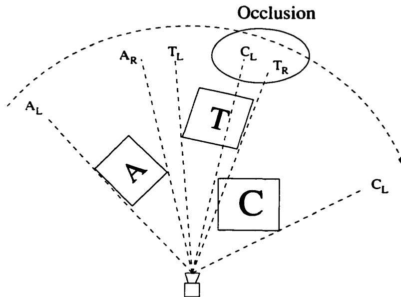
Figure 4.4: Testing for Occlusion. If camera-relative viewing angles for any of the objects overlap, as indicated with the middle “T” and right object “C”, the set of target object poses is discarded.
