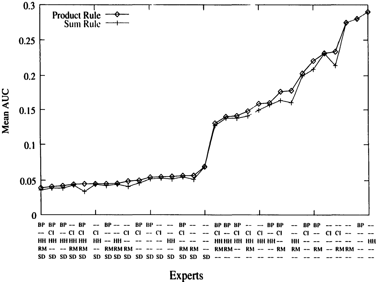
Figure 5.8: Comparing the discrimination provided by the Bayesian product and mean sum rules.
