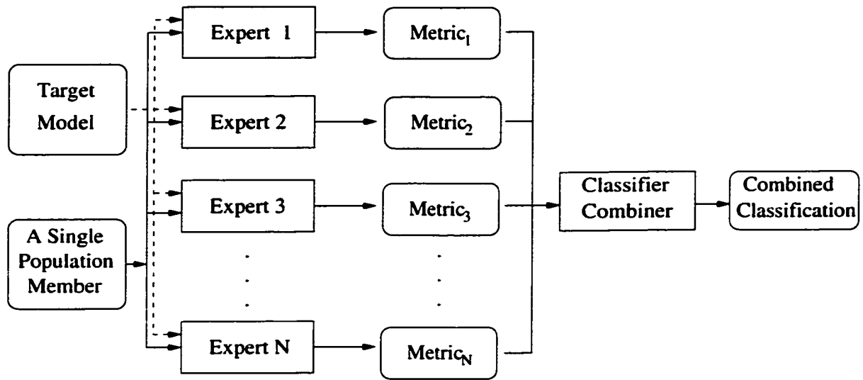
Figure 2.10: Combining classification data from multiple experts
