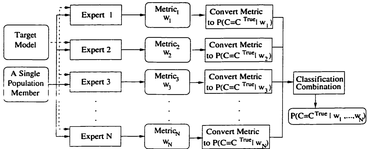
Figure 2.12: Combining classification data using a probabilistic algorithm and a single target model
