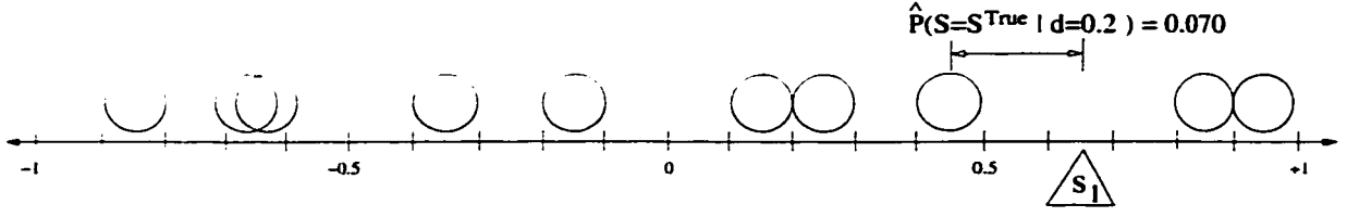
Figure 3.14: Step One - Measurements. Computing the weight P(S = S^{True}|d) for one particle using the distance between the particle and the estimate s_1 is shown.
