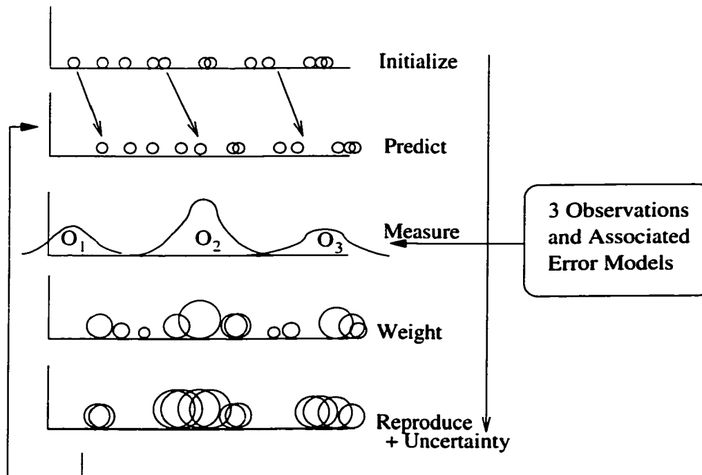
Figure 2.19: Condensation Filter process steps: 1) a filter update begins with an equally weighted set of particles, 2) the predicted motion model and a model of uncertainty are applied to every particle, 3) measurements are acquired, 4) each particle is weighted as a function of the distance between the particle and the measurements, 5) the particles are reproduced as a function of their weight
