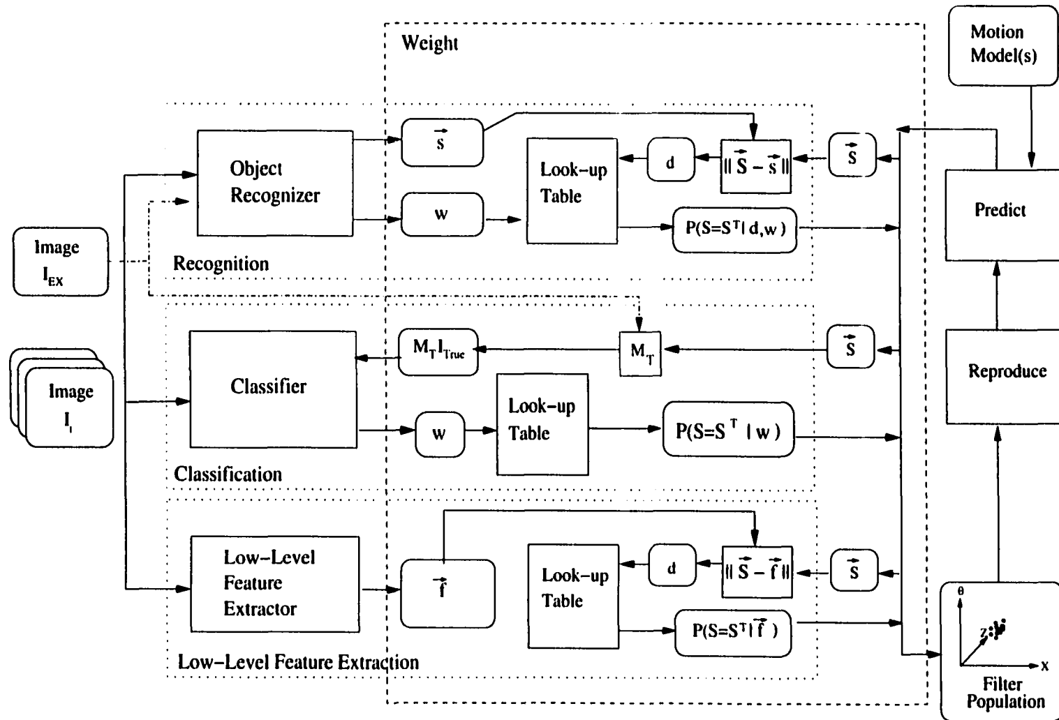
Figure 3.3: The Extended Condensation Filter
