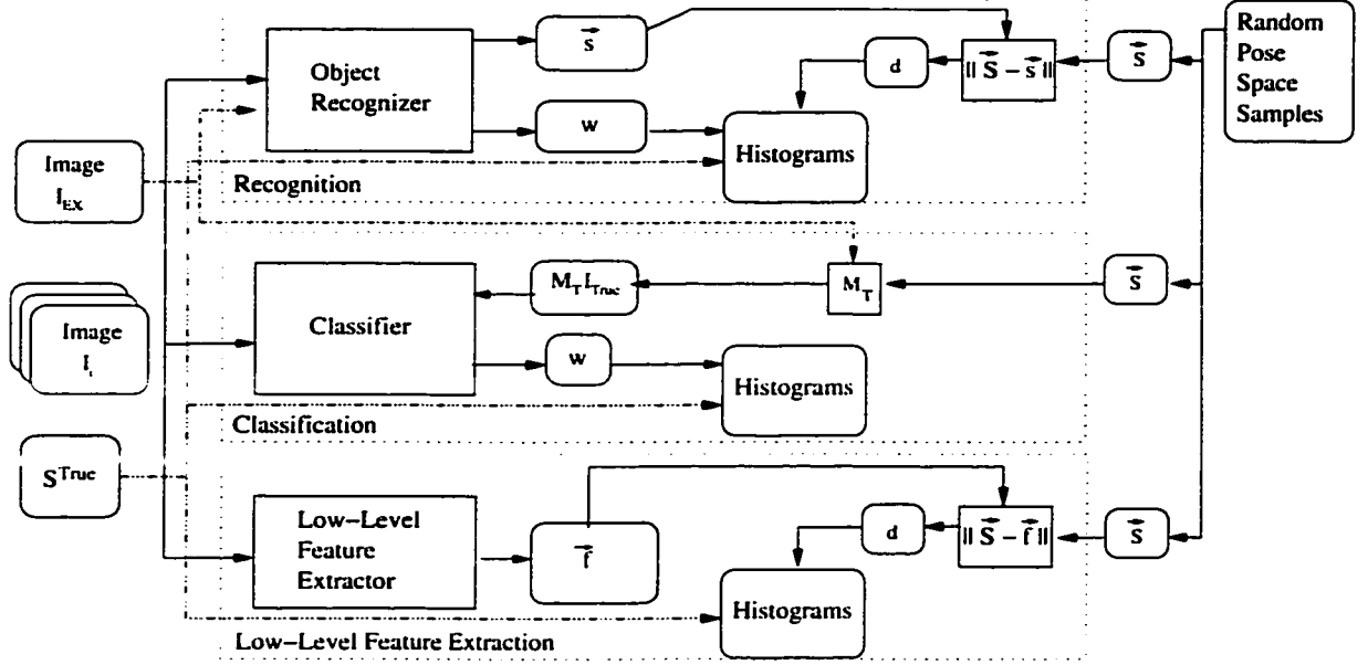
Figure 3.4: Training the Extended Condensation Filter
