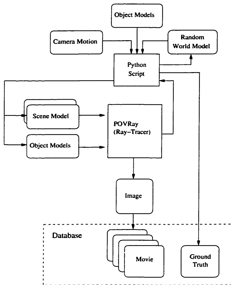
Figure B.1: Creation of movies (sequential images) and target object ground truth.
