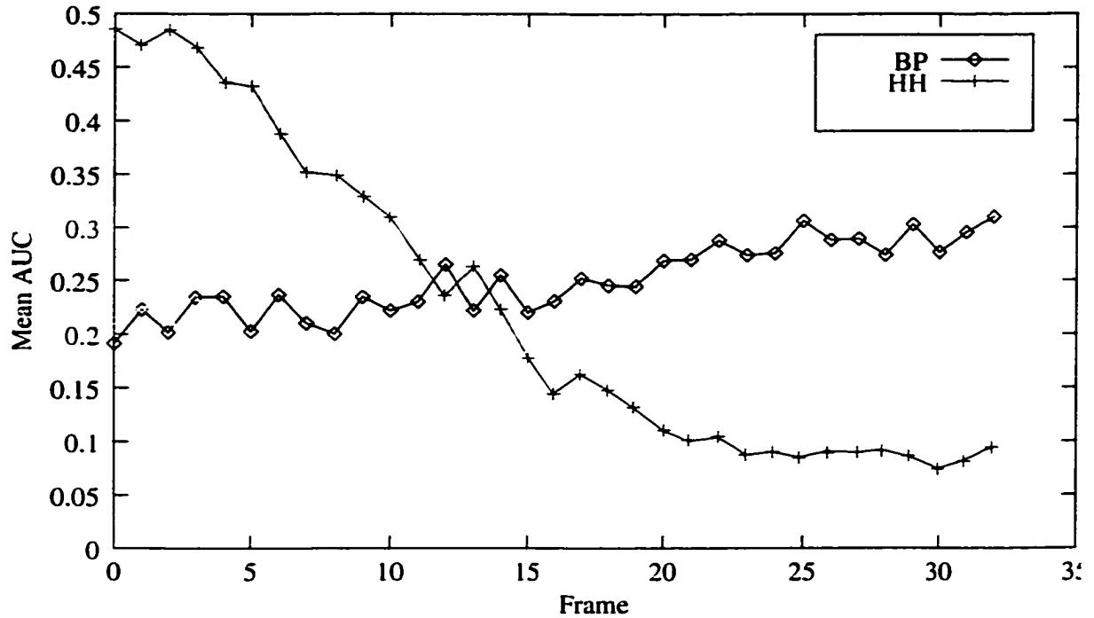
Figure 5.3: Comparing back-projection (BP) and Hausdorff-Huttenlocher (HH) discrimination. Thirty untrained tracking problems in Block World One are used to make the comparison.
