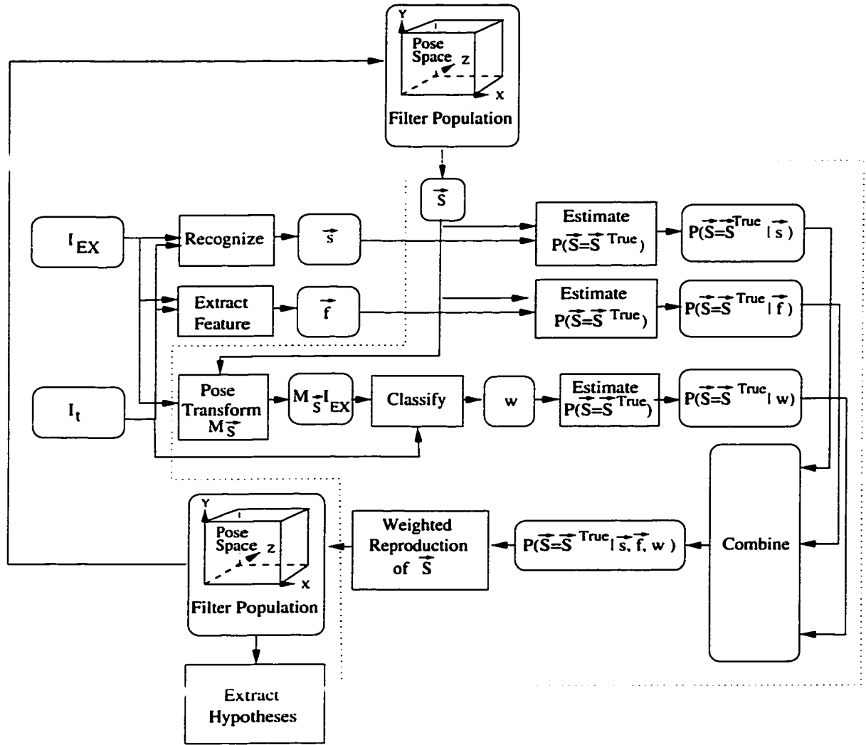
Figure 1.8: Operations performed by the Extended Condensation Filter to weight a single particle based on the particle's pose estimate. The operations inside the dotted line are repeated for each particle in the filter. I_{EX} is the target object example image. I_t is an unknown image acquired at time t . \vec{s} is a target pose estimate provided by a recognition algorithm. \vec{f} is a feature provided by a low-level feature extractor. \vec{S} is a pose assigned to a single particle in the filter's population of particles. M_{\vec{S}}I_{EX} is the target image transformed on the basis of the pose \vec{S} . w is the classification algorithm's measurement of similarity between the transformed target image M_{\vec{S}}I_{EX} and the acquired image I_t . \vec{S}^{True} is the true target pose, and P(\vec{S} = \vec{S}^{True}) is the probability that \vec{S} is the true target pose.
