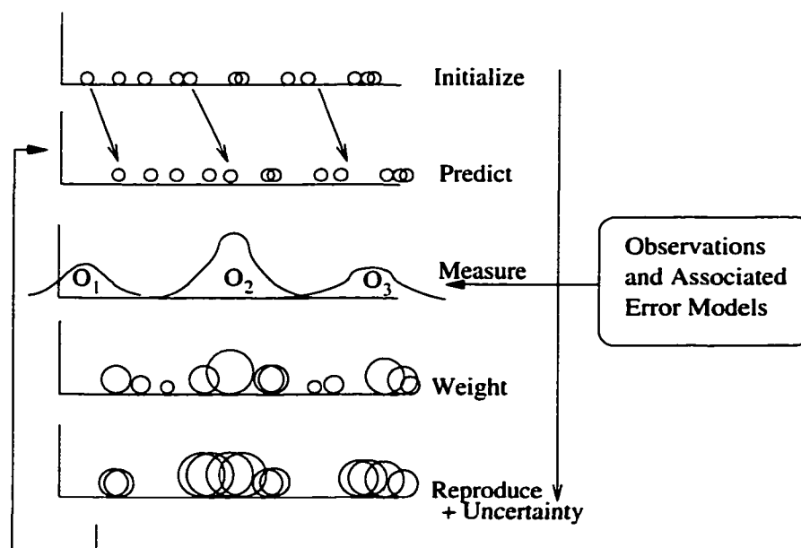
Figure 1.7: Top-level architecture of the canonical Condensation Filter showing a small population of particles
