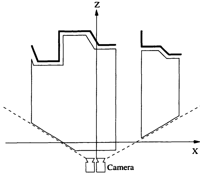
Figure 1.4: The range features are shown as a bold line. The pose space eliminated by low-level range features is shown in gray.
