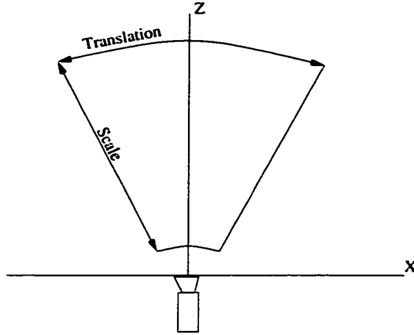
Figure 4.10: The Hausdorff scale and translation parameters correspond to a wedge of camera-relative pose space. The range of scale parameters define the wedge depth. The range of translation parameters define the wedge angle.
