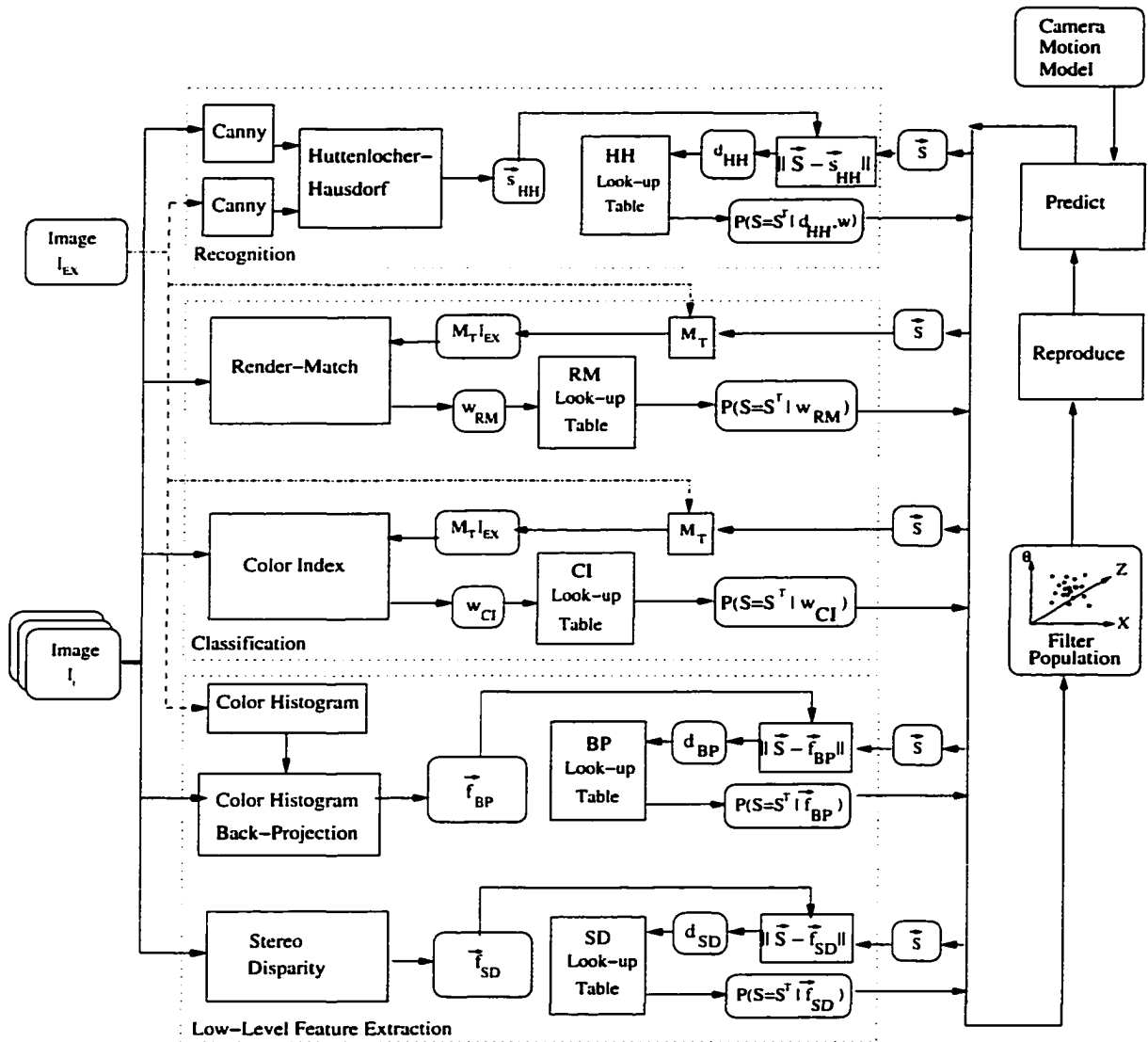
Figure 4.9: Implementation of the Extended Condensation Filter
