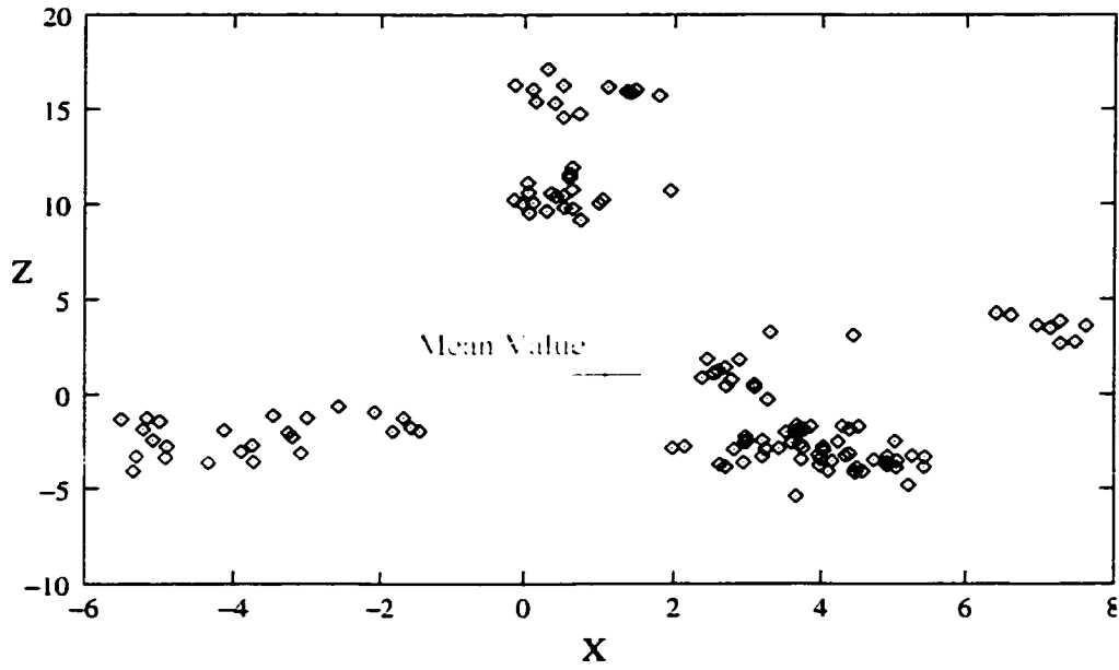
Figure 5.10: Example of multiple clusters in the x and z portion of pose space. This is the state of the filter after frame 32 for movie 1, target block A, Block World One training data.
