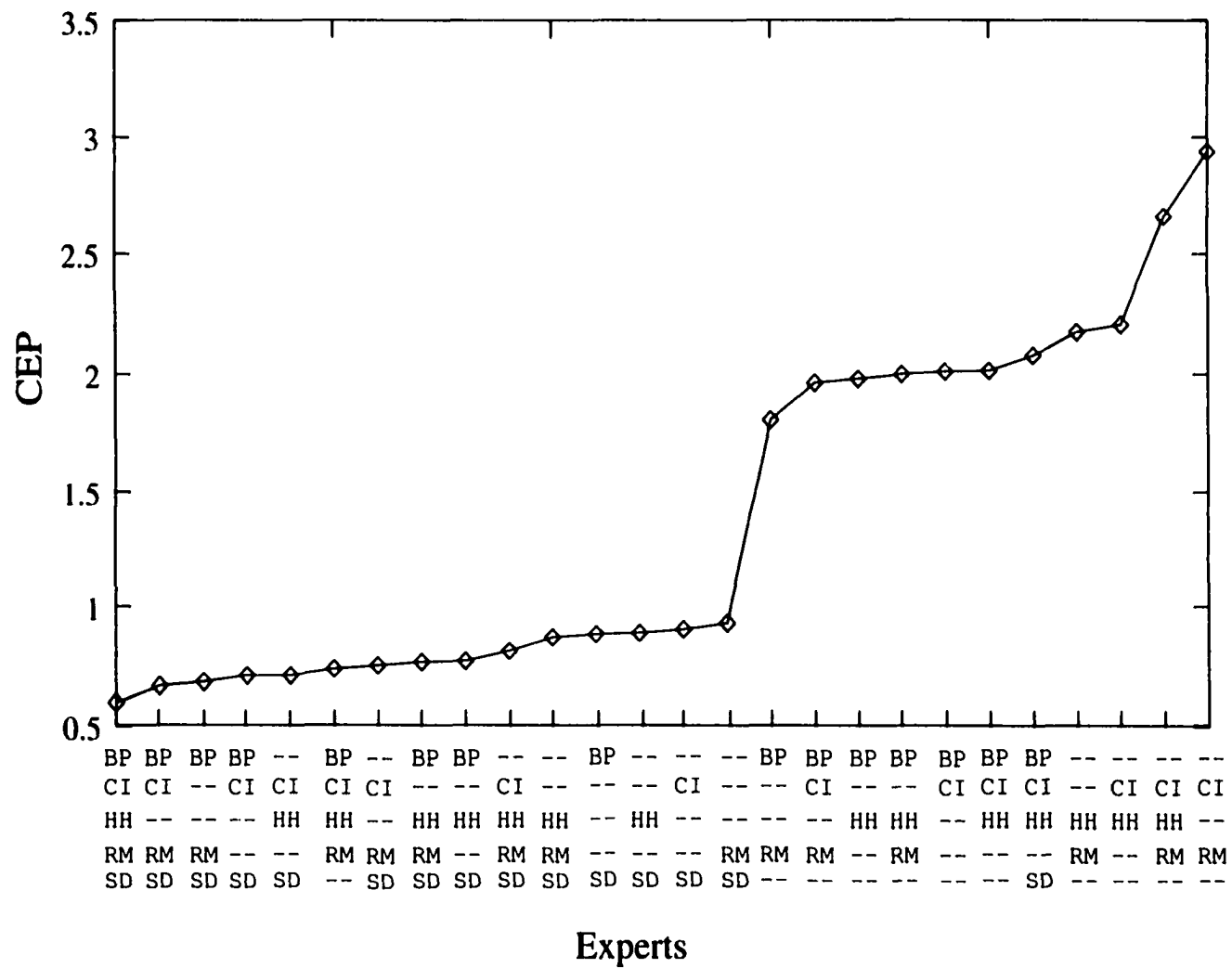
Figure 5.7: Accuracy and precision provided by the Bayesian product rule. Combinations of two or more experts are shown on the independent axis and sorted from smallest to largest CEP.
