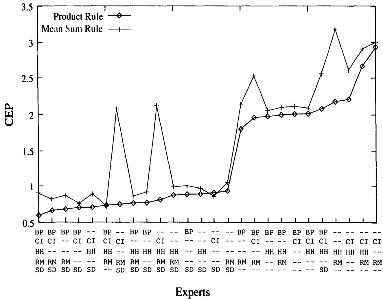
Figure 5.9: Comparing the accuracy and precision provided by the Bayesian product rule and mean sum rules. Each value is the mean scaled CEP using x and z only. The 31 combinations of experts, where each combination is shown on the independent axis, are sorted from lowest to highest CEP.
