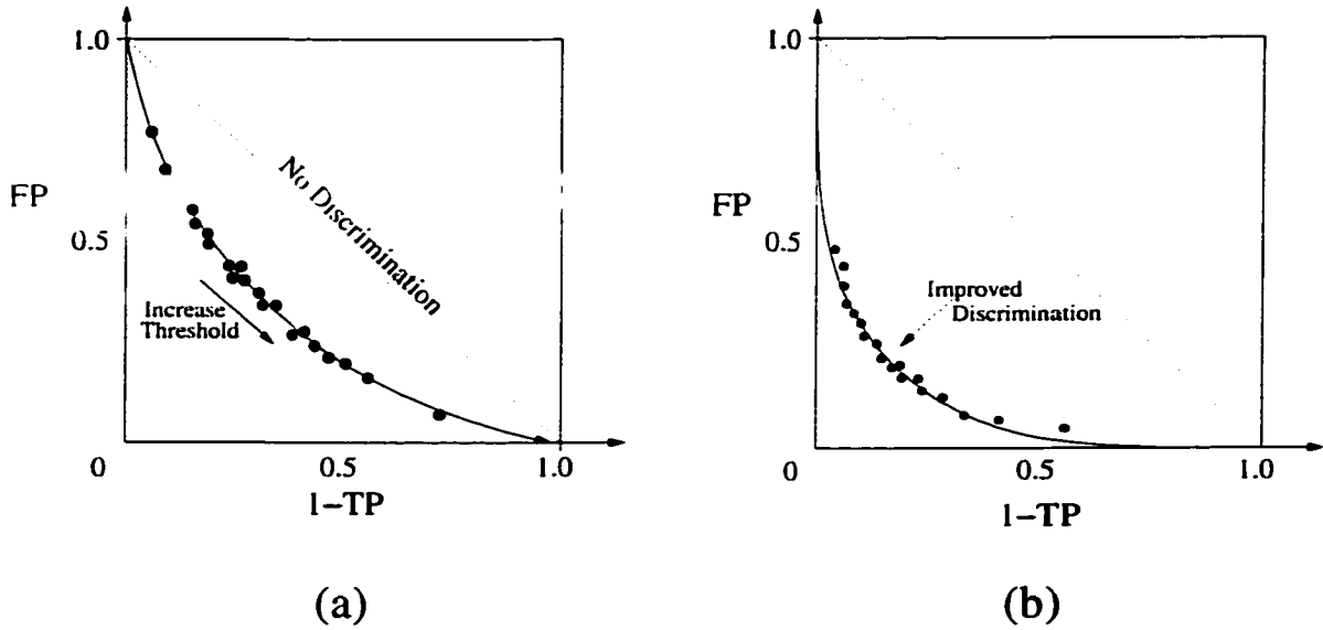
Figure 2.9: Typical ROC Curves. Figure (a) indicates less discrimination than (b).
