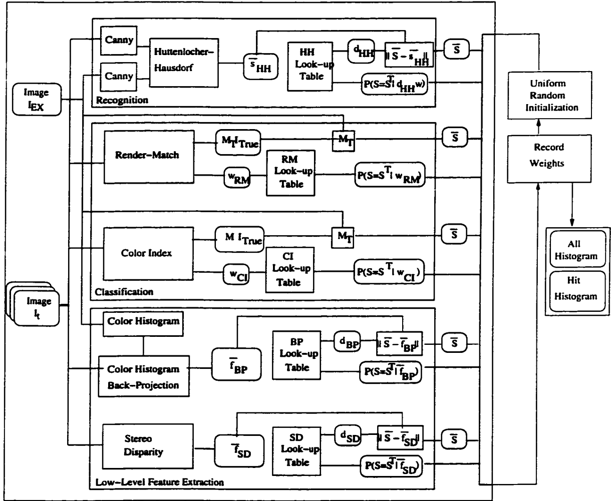
Figure 4.16: Implementation of the learning algorithm. The portion of the implementation shown in gray (light blue in the on-line version) is identical to the filter.
