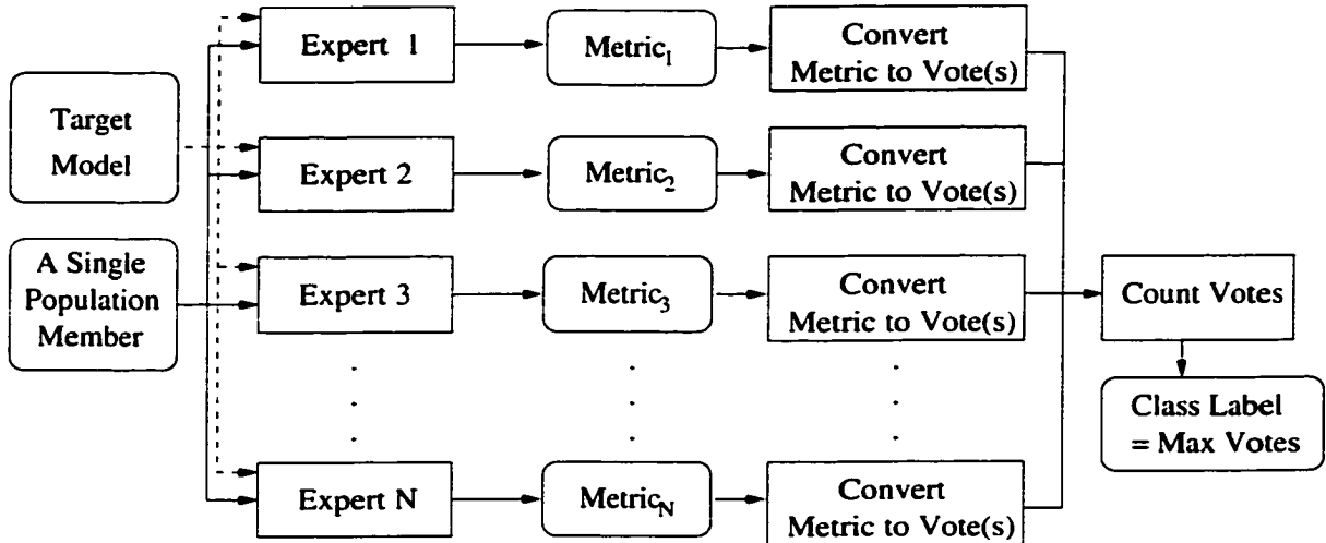
Figure 2.11: Combining classification data using a deterministic voting algorithm and a single target model
