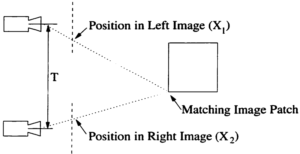
Figure 2.3: Inferring depth information using the stereo disparity from two cameras
