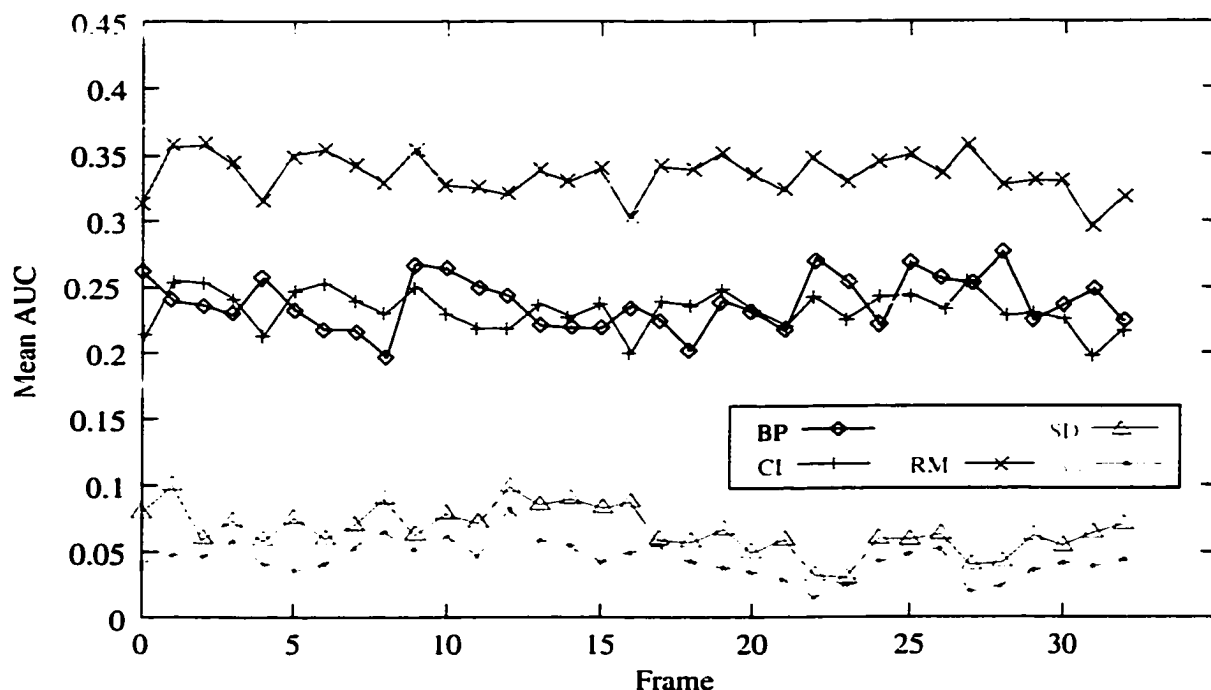
Figure 5.2: Comparing the discrimination using each expert individually (BP, CI, HH, RM, SD) to all the experts combined (All). Thirty tracking problems in Block World Two are used to make the comparison.
