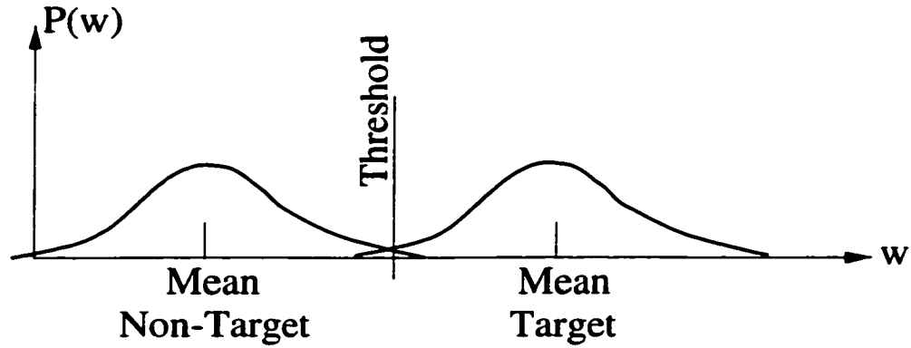
Figure 2.7: Example Gaussian distributions for a two-class classification problem. w is a similarity metric and P(w) is the probability of the metric w occurring for each distribution. The threshold is used to discriminate between target and non-target images.
