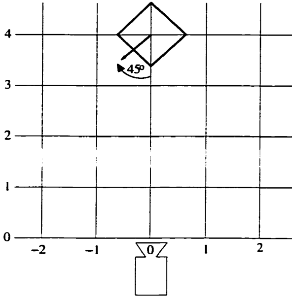
Figure 2.15: Transformed target image based on the pose shown in Figure 2.14
