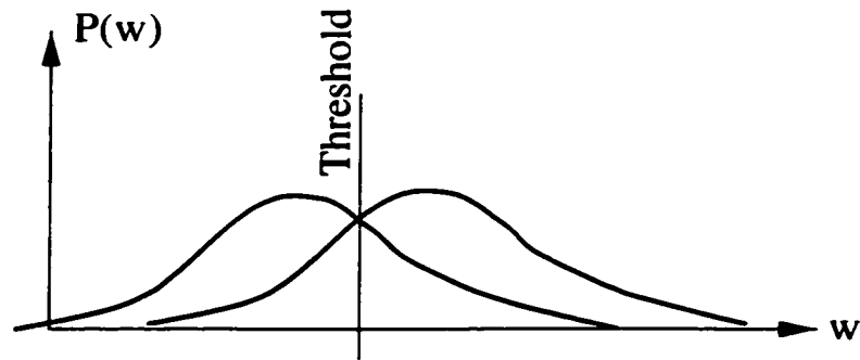
Figure 2.8: Example Gaussian distributions for a two-class classification problem where the classifier has relatively poor discrimination, when compared to Figure 2.7.
