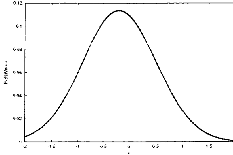
Figure 3.7: Object recognition (Hausdorff-Huttenlocher) uncertainty model, where the uncertainty \hat{P}(\vec{S} = \vec{S}^{True} | d_{\vec{S}}, w) is modeled by a Gaussian. For this example \vec{s} is simply the horizontal translation x .
