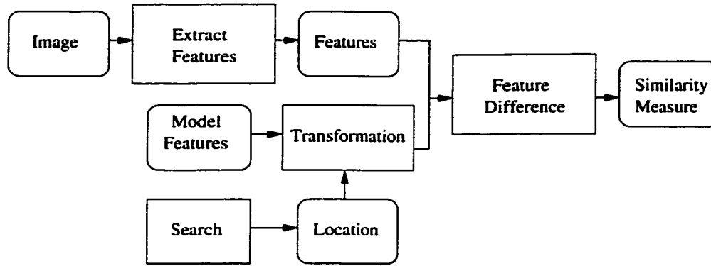
Figure 1.3: Adding Location to Classification by Transforming the Model Features to Match the Image
