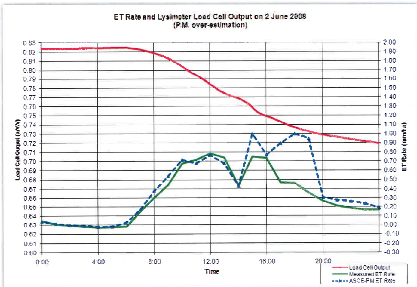
Figure 6. Example of over-estimation of afternoon hourly ET rates by the ASCE standardized reference ET equation (dashed line), compared to measured alfalfa ET from the lysimeter (solid line). In the afternoon of June 2, 2008, dry, warm wind originating from a nearby prairie blew from the southwest.
