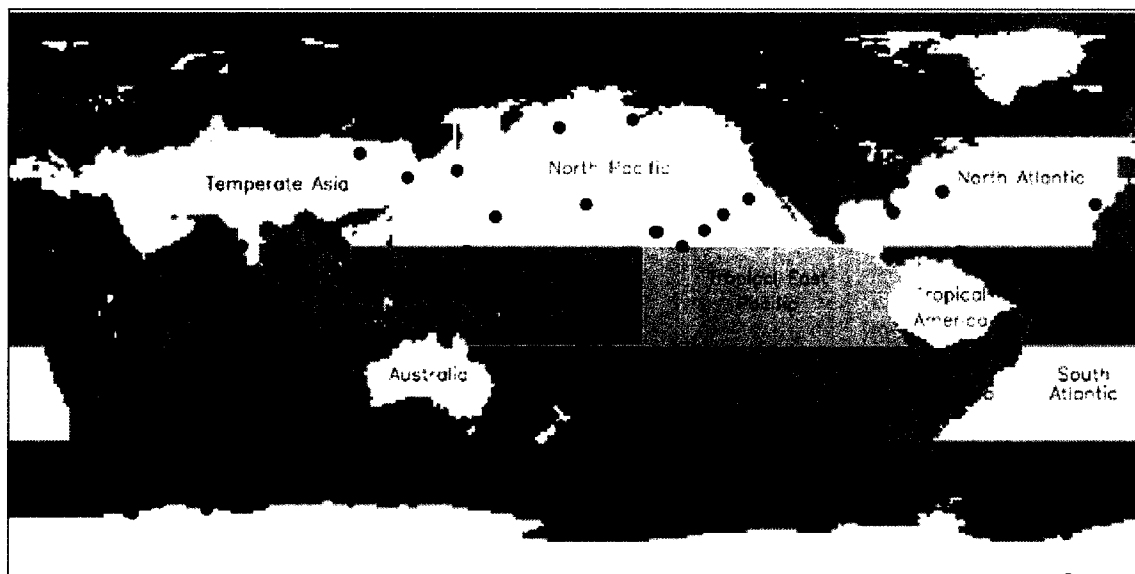
Figure 1: Regions used in the inversion and the locations of the 76 CO 2 observational records used. Multiple records exist at some locations.
