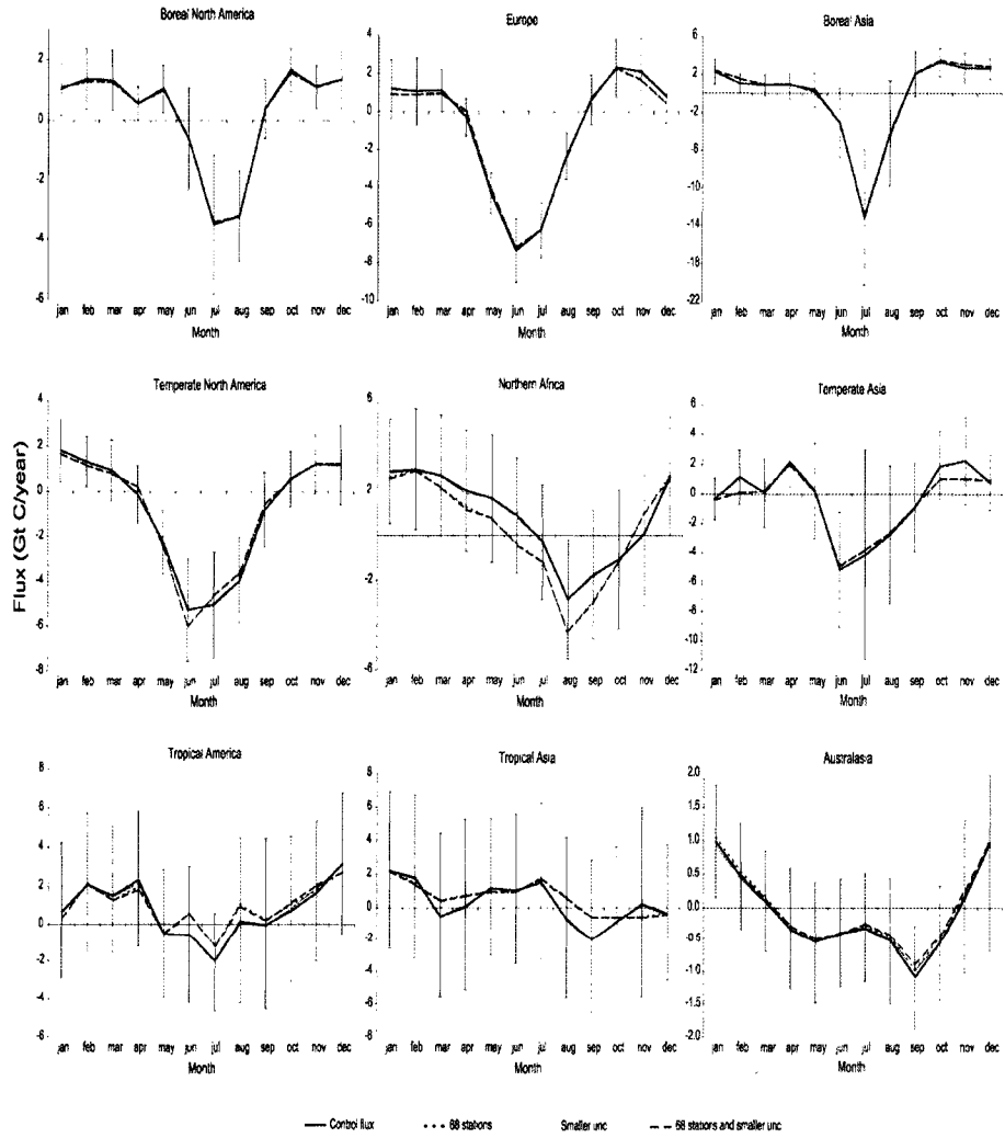
Figure 8a. Station sensitivity for selected land regions. Estimated flux for the control inversion (75 stations), an inversion with 68 stations (removed CRI, GMI, IZO, UTA, Carr 5000m, PRS, and IUUN), the control inversion with halved uncertainty on six southern stations (Bass Strait, SPO, HBA, SYO, MAA, and PSA), and an inversion with the combination of these two station adjustments. Note that the vertical scale varies. The fluxes do not include fossil fuel emissions.
