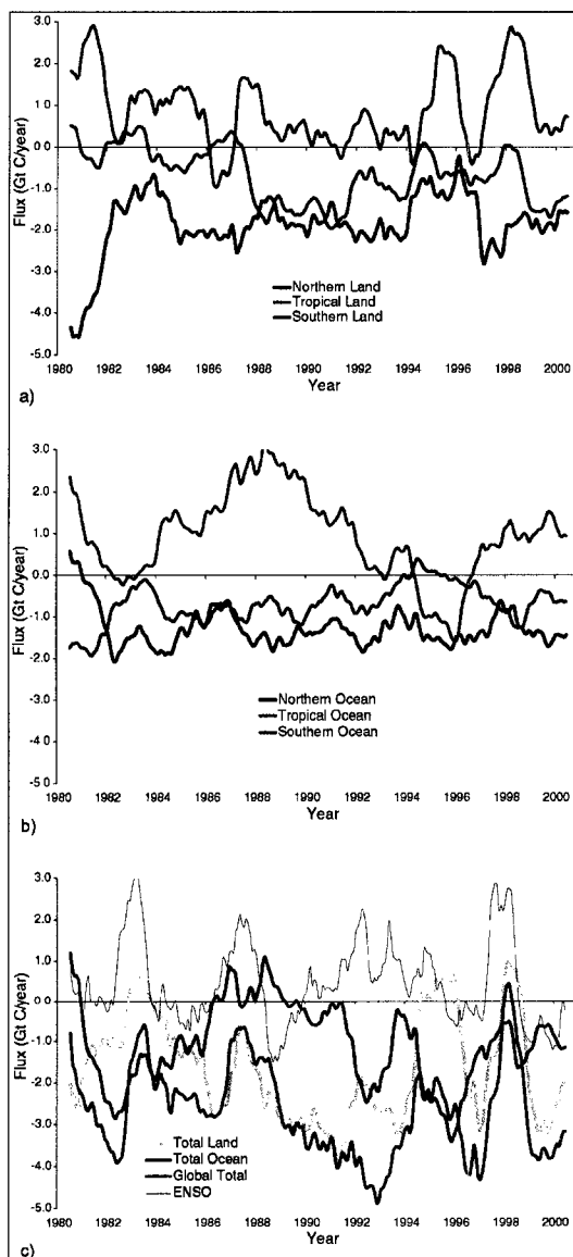
Figure 4.6. Regionally aggregated, deseasonalized carbon fluxes from the inversion using the 23 station network. a) Land, b) ocean, c) totals.
