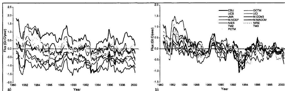
Figure 4.4. Deseasonalized, individual model fluxes for the Boreal Asia region. a) Original, unadjusted fluxes. b) Fluxes with offset from model mean removed.
