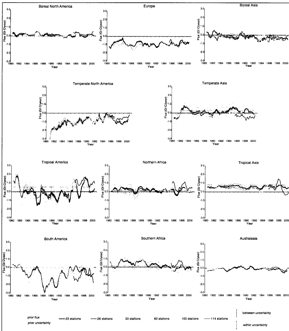
Figure 4.2a. Model mean, deseasonalized, land-based interannual flux estimates (Gt C/year) for the six CO 2 observation networks. The 1 \sigma within and between uncertainty estimates are based on the 23 station network only. Note that all the vertical scales are identical.
