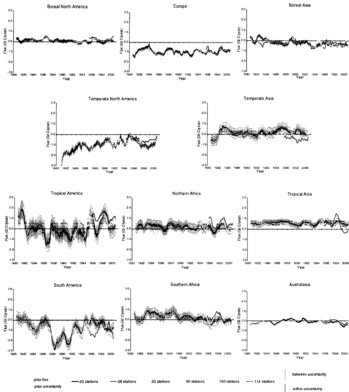
Figure 4.5a. As in figure 4.2a except the individual model long-term mean offsets around the model mean has been removed.
