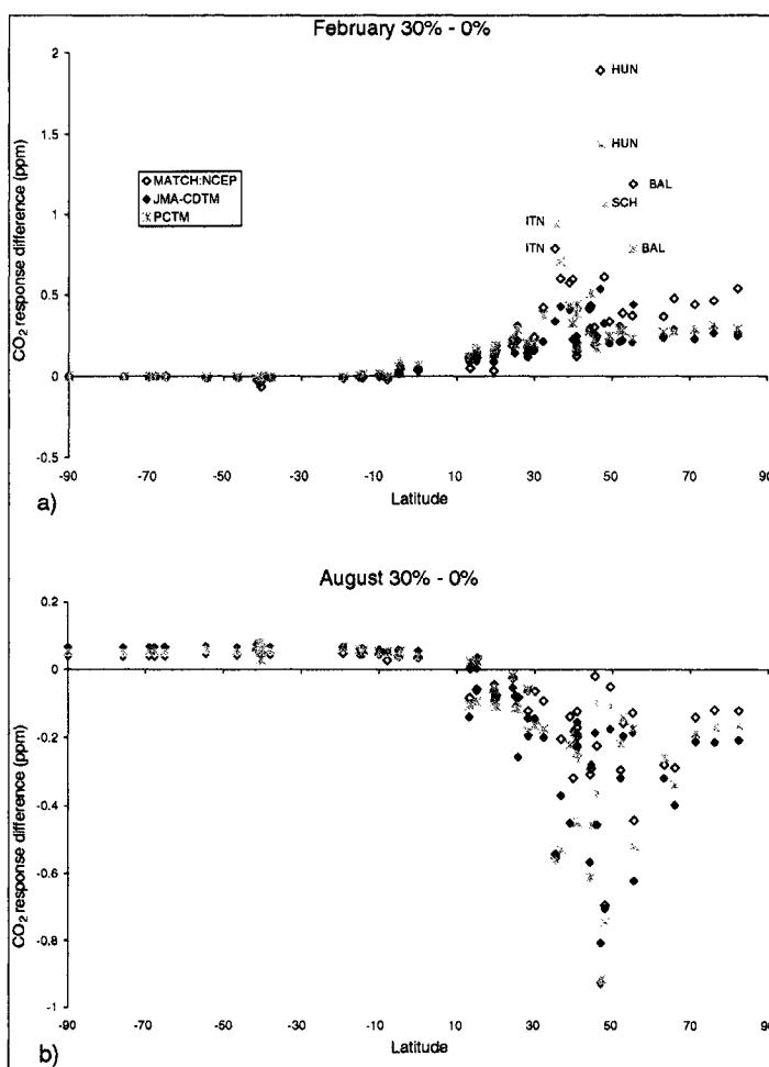
Figure 5.9. CO 2 concentration response difference at all of the observation stations for the month of a) February and b) August. The values represent the difference between the 30% and base AF fossil fuel emissions cases.
