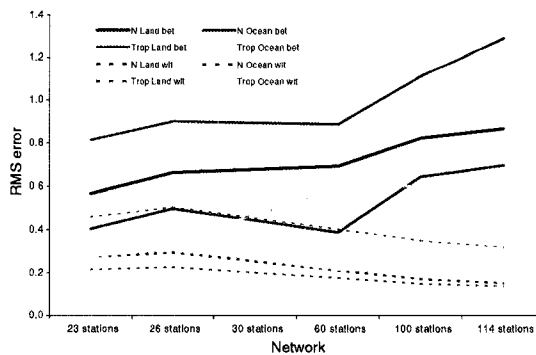
Figure 4.3. Error as a function of aggregated region and station network size.
