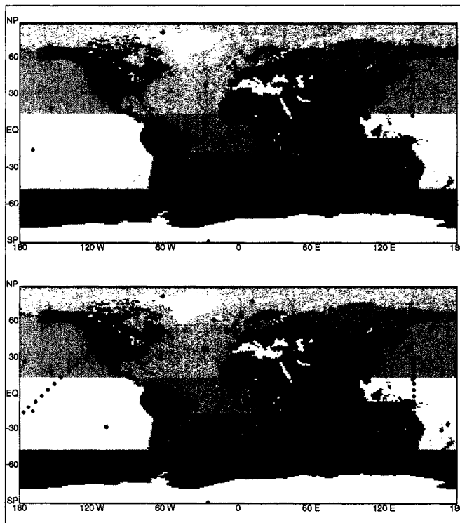
Figure 4.1. Locations of the stations for the a) smallest (23) and b) largest (114) CO 2 observational networks.
