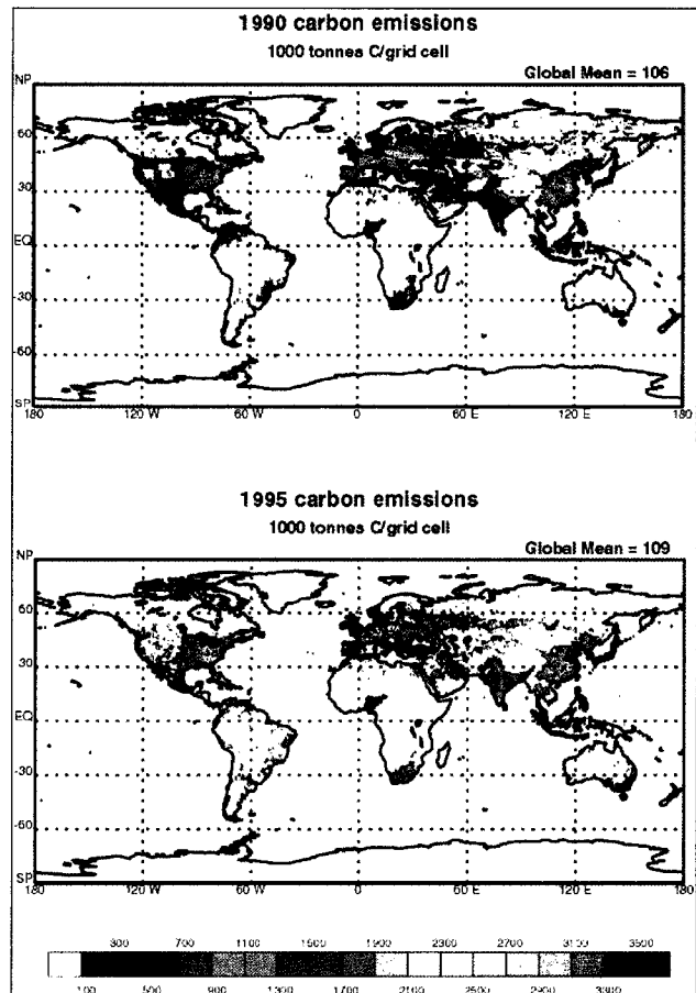
Figure 5.1. Fossil fuel emissions for a) 1990 and b) 1995. Units are 1000 tonnes C/grid cell and the grid cells are dimensioned 1° x 1°.
