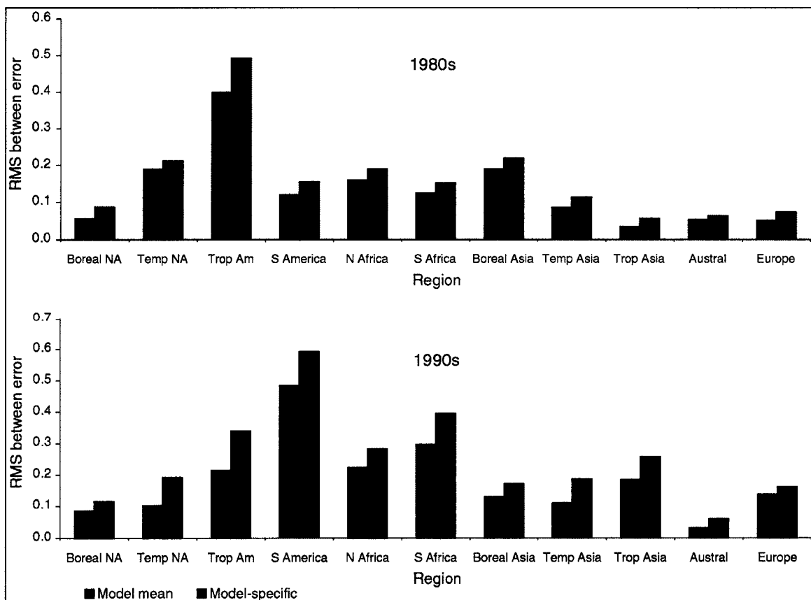
Figure 4.10. Comparison of the RMS between uncertainty due to network composition for two different time periods. The different color bars represent the model mean sensitivity and the model-specific sensitivity.
