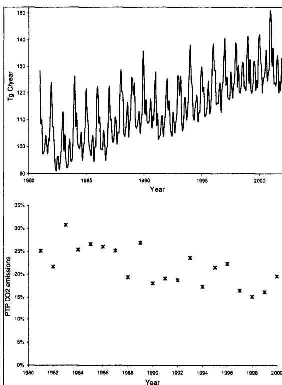
Figure 5.2. a) Total fossil fuel CO 2 emissions for the United States (Tg C/year). B) Peak to peak fossil fuel emissions for the United States.
