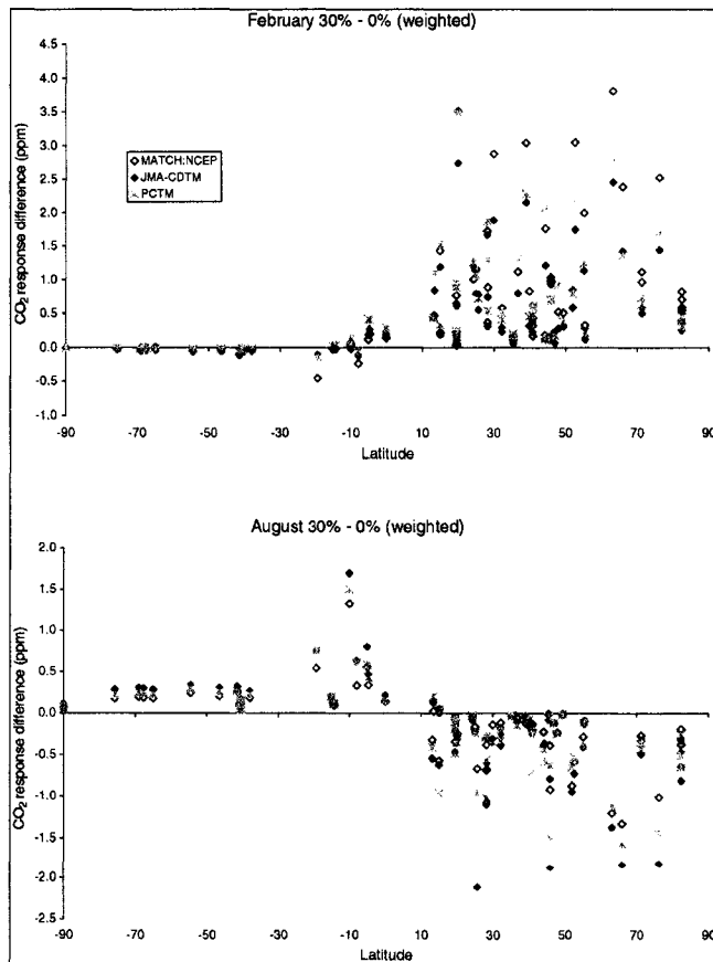
Figure 5.12. As in figure 5.9 except the response values have been weighted by the inverse square of the “data uncertainty”.
