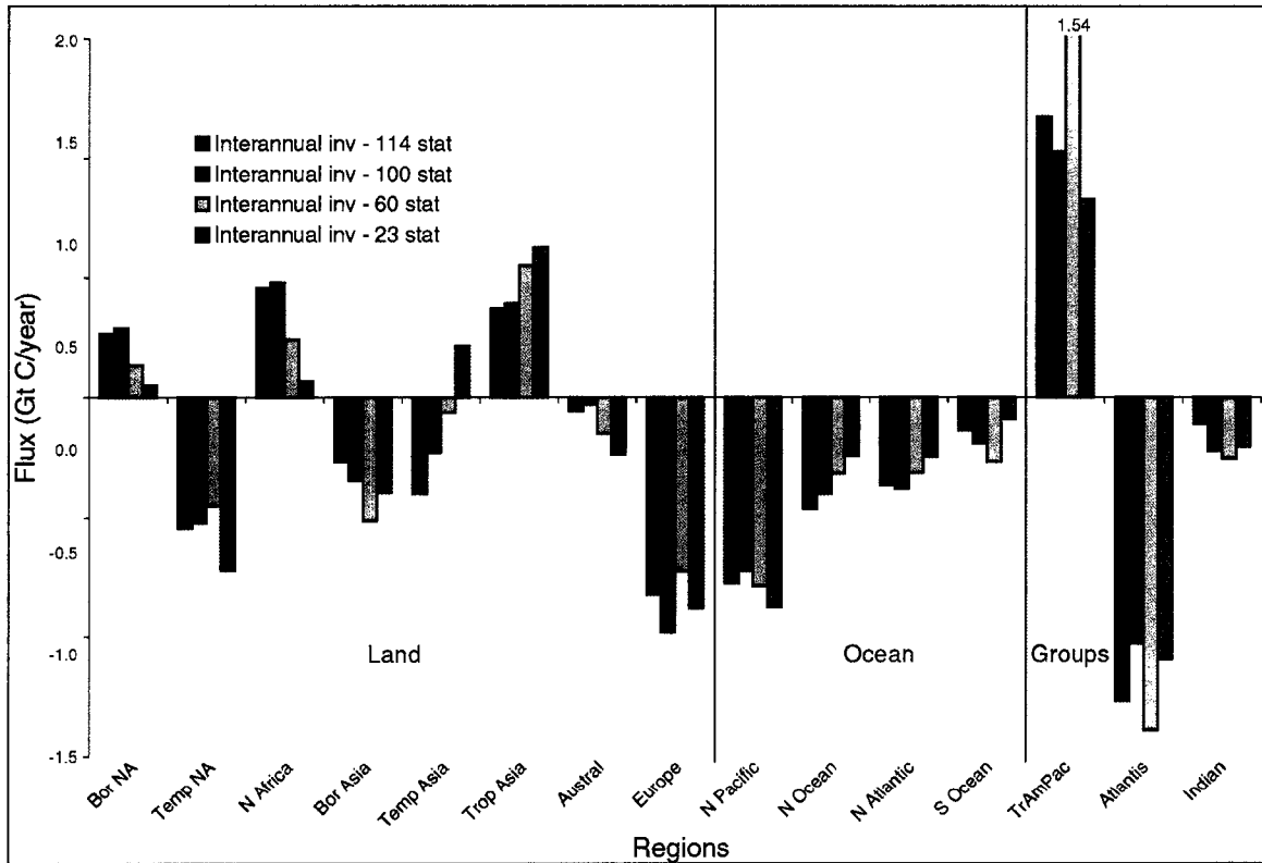
Figure 4.12. Model mean, time-averaged carbon exchange for the 1995 to 2000 time period across different CO 2 observation station networks.
