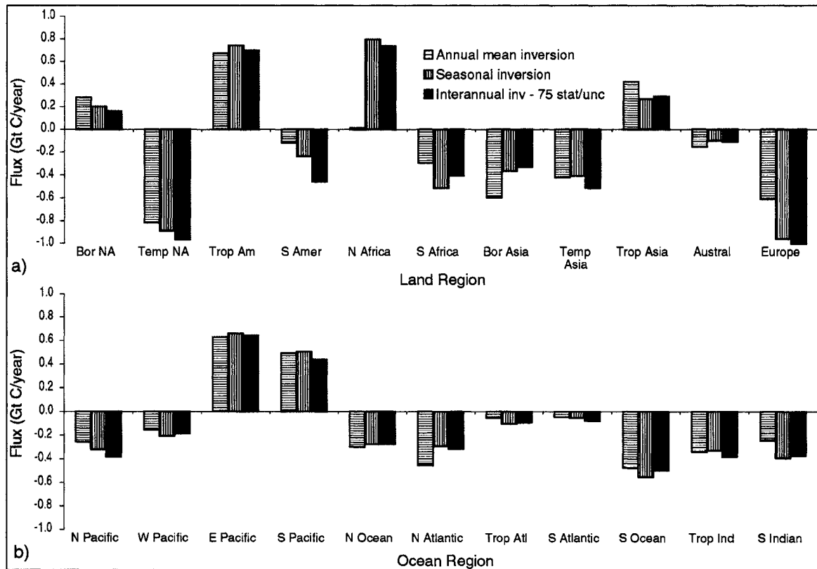
Figure 4.11. Model mean carbon exchange for the 1992 to 1996 time period across different inversion methods. a) land regions, b) ocean regions.
