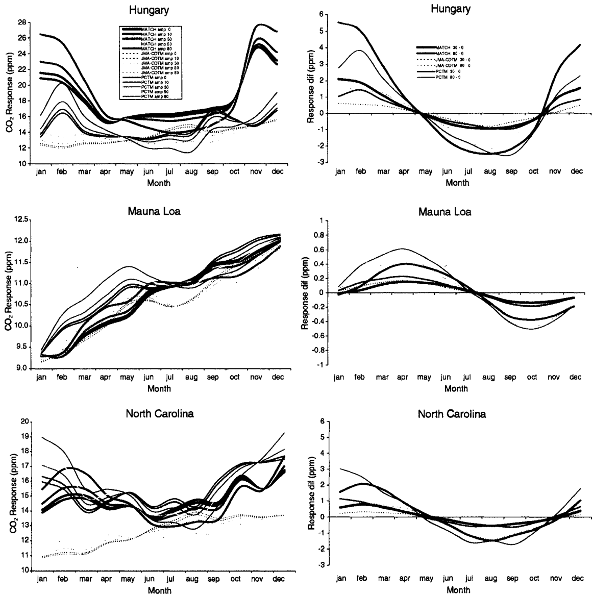
Figure 5.7. a) CO 2 concentration response at three stations reflecting seasonal fossil fuel emissions. Five AFs for each of the three models are shown. b) CO 2 concentration response difference between the 80% AF and the base case and the 30% AF and the base case.
