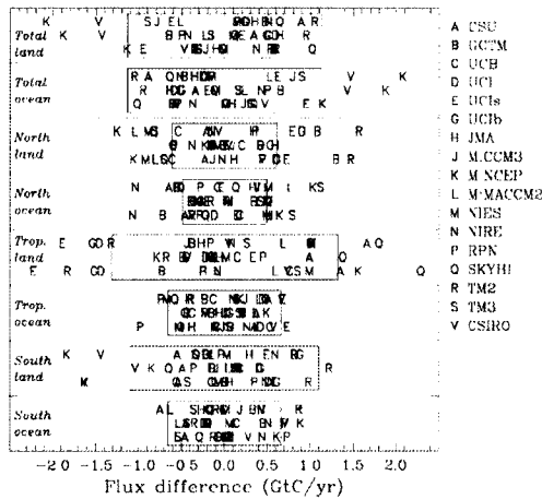
Fig. 7. Aggregated posterior flux differences from the model mean for the control inversion (top row in each box), the No Rect. case (sensitivity test 3, middle row in each box) and the Zero Ocean. case (sensitivity test 5, bottom row in each box). The box represents the within-model uncertainty ( 1\sigma ). Regional aggregation is as follows: North land (Boreal N America, Temperate N America, Europe, Boreal Asia, Temperate Asia), North ocean (N Pacific, Northern Ocean, N Atlantic), Tropical land (Northern Africa, Tropical Asia, Tropical America), Tropical ocean (W Pacific, E Pacific, Tropical Atlantic, Tropical Indian), South land (Southern Africa, Australia, S America), South ocean (S Pacific, S Atlantic, S Indian, Southern Ocean).
