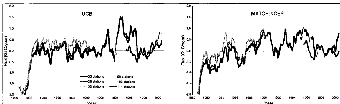
Figure 4.9. Deseasonalized interannual flux estimates for all six networks and for model a) UCB, and b) MATCH:NCEP.
