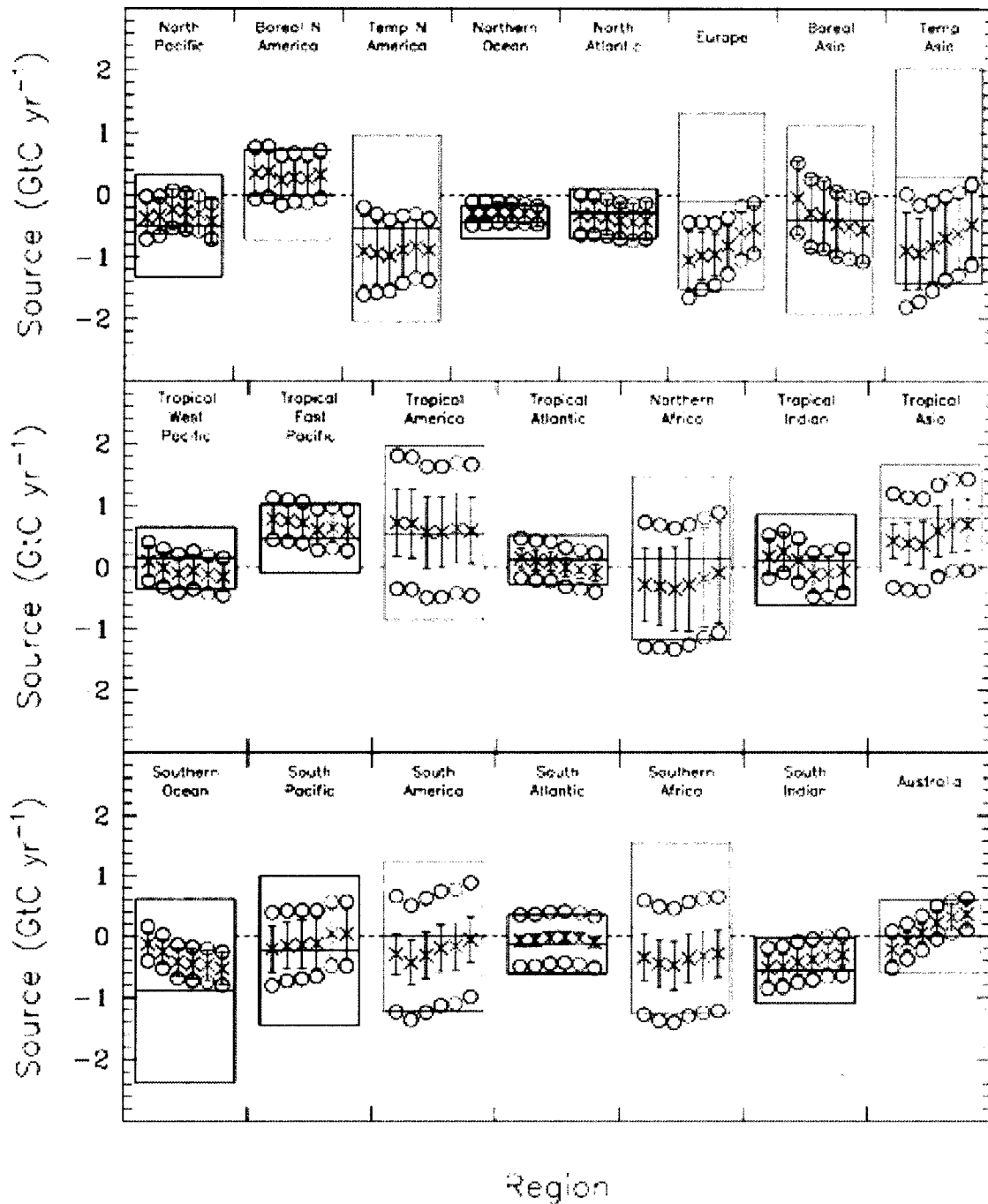
Figure 3: Prior sources and uncertainties (boxes), mean estimated sources (x), 'within-model' uncertainties (o) and 'between-model' uncertainties (error bars) for six 5-year periods. Only the CO 2 observational data is changed in each of these six periods. The time periods are displayed from left to right as: 1988-1992, 1989-1993, 1990-1994, 1991-1995, 1992-1996 (control, red symbols), and 1993-1997. The same 76 sites are used for all inversions even though this means that some sites have more than 30% extrapolated data. Growth rates and fossil emissions are adjusted to be appropriate to each period. For most regions, the change in time period does not move the mean estimated source outside the control uncertainty range.
