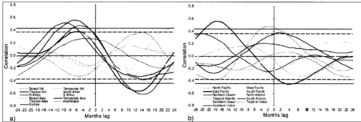
Figure 4.15. Lagged correlation between the MEI ENSO index and the regional carbon exchange for the 23 station network. a) land regions, b) ocean regions. Two-tailed significance (95%) is denoted by the solid horizontal lines. The one-tailed significance level (95%) is denoted by the horizontal dashed line.
