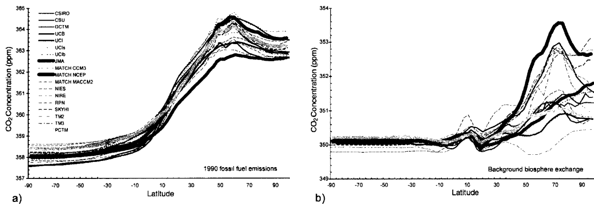
Figure 5.3. a) Annual/zonal mean surface CO 2 concentration (ppm) resulting from 4 years constant emissions of 1990 fossil fuel CO 2 and b) neutral biosphere exchange. The models used in the current study are denoted in bold.
