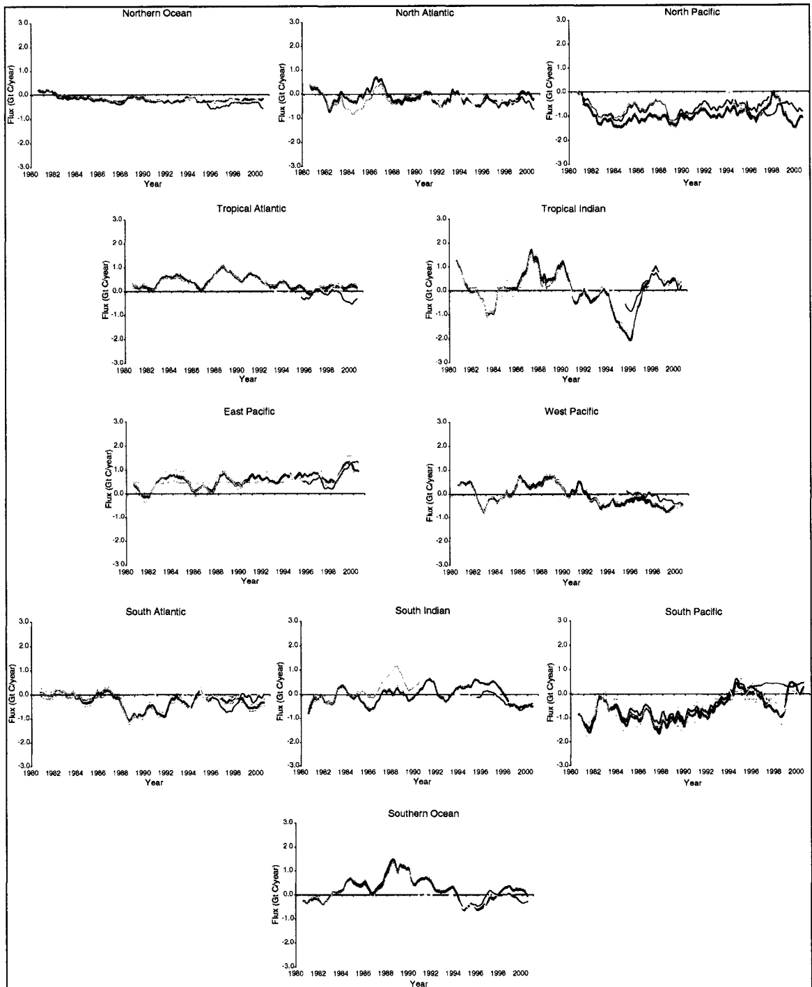
Figure 4.5b. As in figure 4.5a but for the ocean regions.
