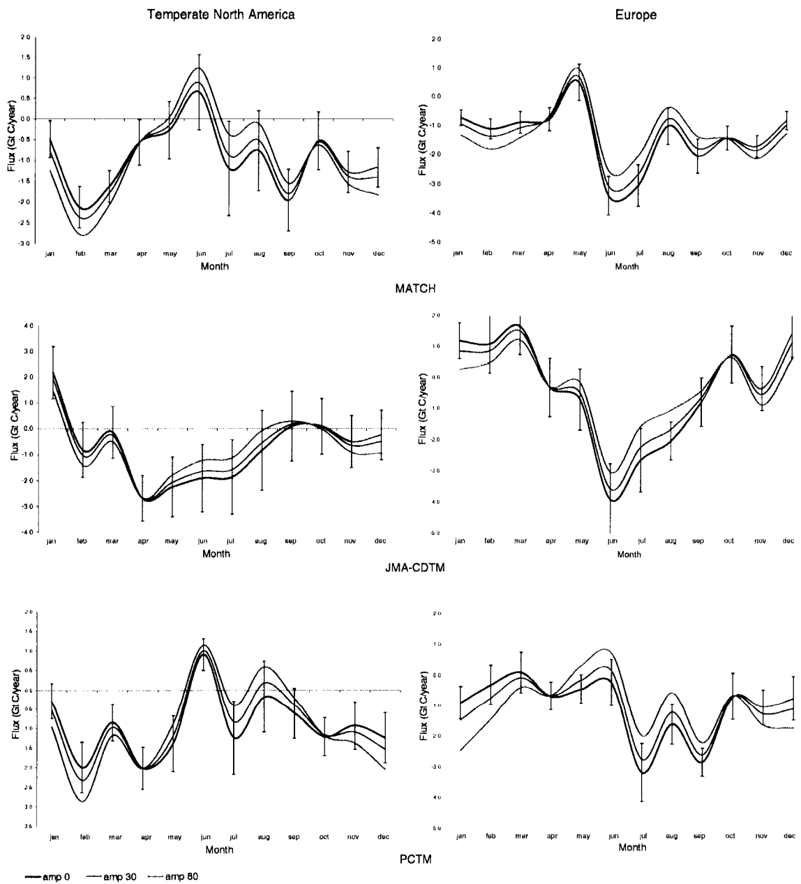
Figure 5.10. Monthly mean inverse flux estimates for the Temperate North American and European land regions. Inverse flux estimates are shown for three fossil fuel AF cases (base, 30%, and 80%) and all three transport models.
