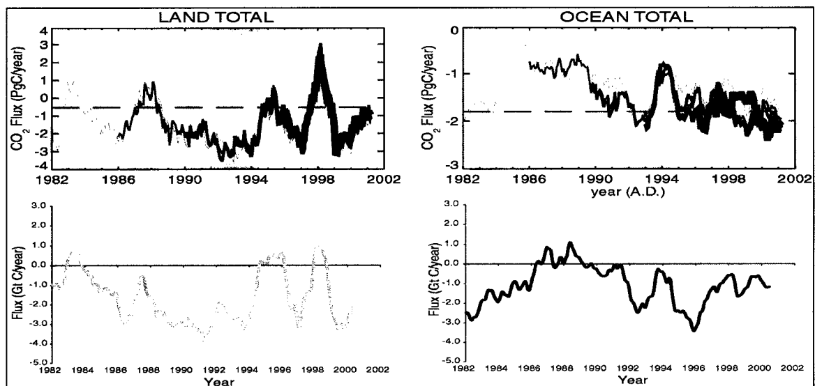
Figure 4.14. Comparison of total land and total ocean fluxes from this study (bottom panels) and Rödenbeck et al. , 2003.
