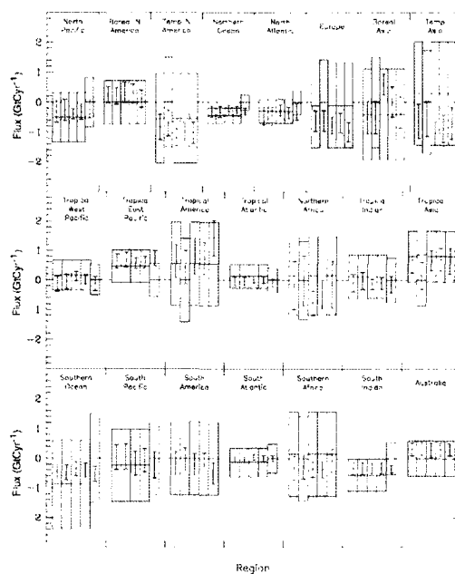
Fig. 6. Results of sensitivity tests 2-5. The control inversion is denoted by the leftmost set of symbols (as in Fig. 5). The Zero Land Priors case (sensitivity test 2), No Rect case (sensitivity test 3), Adjust Rect case (sensitivity test 4), and Zero Ocean case (sensitivity test 5) are denoted progressively to the right. Mean does not include CSIRO.
