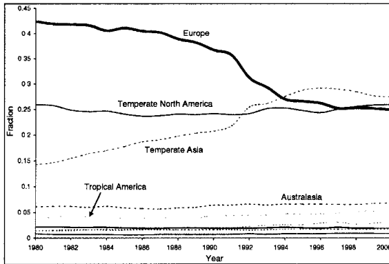
Figure 5.5. Regional fossil fuel emissions as a fraction of the yearly global total.
