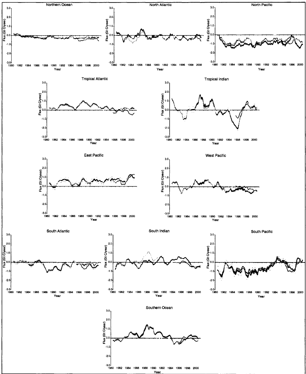
Figure 4.2b. As in figure 4.2a but for the ocean regions.
