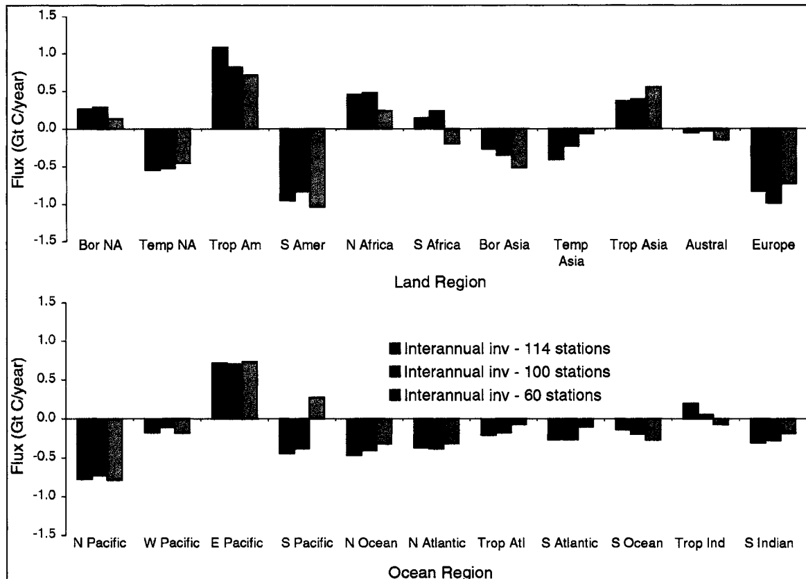
Figure 4.13. Model mean, time-averaged carbon exchange for the 1995 to 2000 time period across different CO 2 observation station networks. All 11 land and 11 ocean regions are separately estimated.
