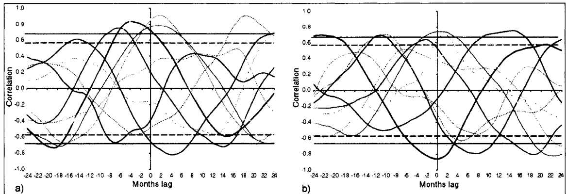
Figure 4.16. Lagged correlation between the MEI ENSO index and the regional carbon exchange for the 114 station network. Legend is identical to figure 4.15. The vertical scale is larger than found in figure 4.15.
