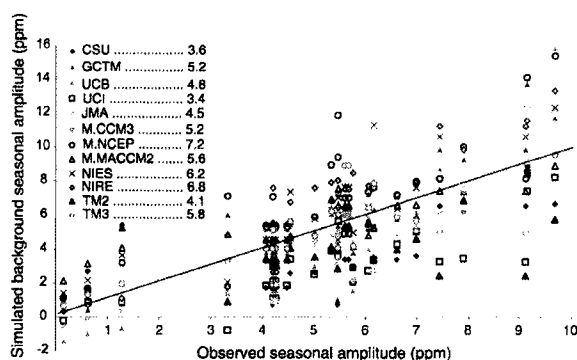
Figure 2. Simulated background seasonal amplitude versus the observed amplitude at stations north of 35°N. Amplitude is defined as the mean October–March concentration minus the mean June–August concentration. The station average simulated values are provided in the legend. The observed station average is 5.6 ppm. A one-to-one line is included. See color version of this figure at back of this issue.
