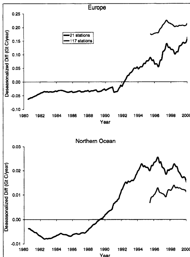
Figure 5.14. The deseasonalized flux difference (Gt C/year) between the base interannual run and the perturbation run for a) Europe and b) the Northern Ocean. Both the 21 and 117 station network results are shown.
