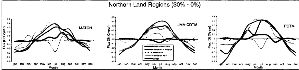
Figure 5.11. Estimated regional fluxes for each month and each model represented as the difference between the 30% and the base AF cases. All northern extratropical regions are shown.
