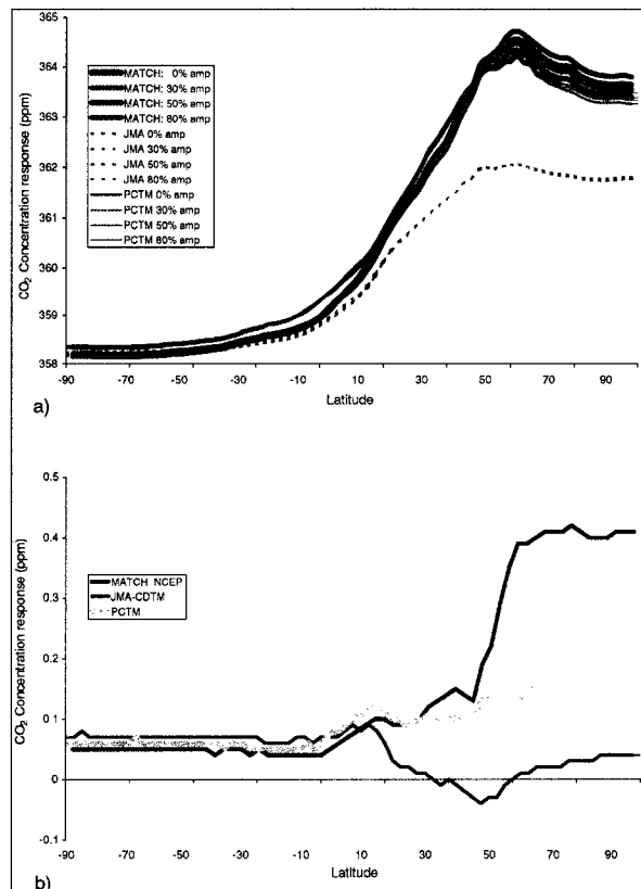
Figure 5.6. a) Annual/zonal mean surface CO 2 concentration resulting from seasonal fossil fuel emissions for four of the nine AFs (including the base case). b) CO 2 concentration difference between the 80% and base AF cases.
