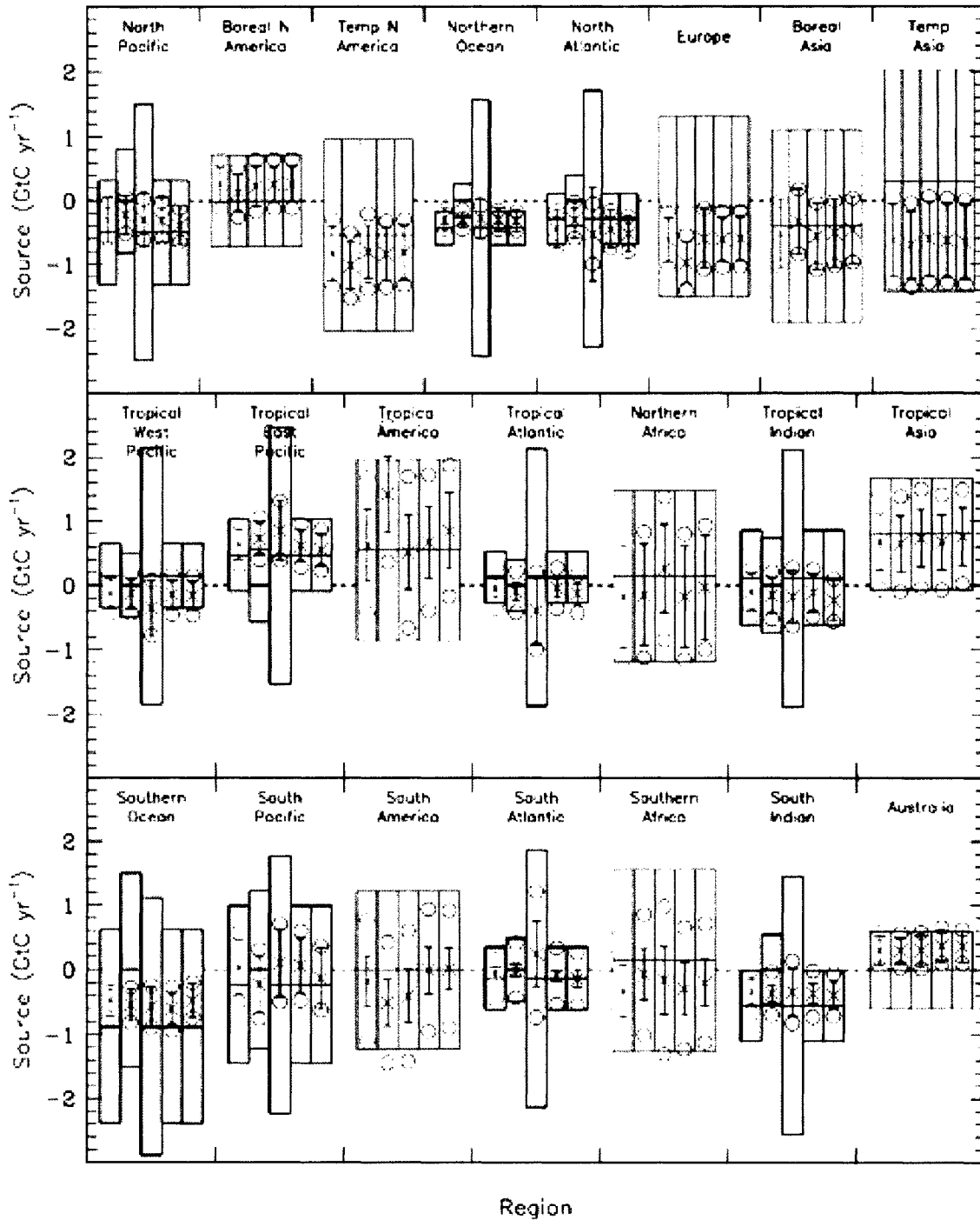
Figure 2: Prior sources and uncertainties (boxes), mean estimated sources (x), 'within-model' uncertainties (o) and 'between-model' uncertainties (error bars) for 4 example sensitivity tests. The results from the control experiment (lefthand symbols in Figure 1, main text) are repeated in the leftmost set of symbols. Second from the left is an inversion run without the background ocean fluxes. Second from the right is an inversion run with prior source uncertainties on all ocean regions of \pm 2 \text{ GtC yr}^{-1} . Third from the left is an inversion run using only half the data records south of 45^\circ\text{S} (HBA_00D0, MQA_02D0, SPO_00C0, SPO_02D0). Far right is an inversion in which the total global oceanic uptake is constrained to -2.5 \pm 0.5 \text{ GtC yr}^{-1} . In each inversion there is little change to the southern ocean estimated flux.
