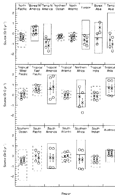
Figure 1 Mean estimated sources and uncertainties for two inversions. Left-hand symbols in each box are for the control inversion, right-hand symbols are for an inversion without the background seasonal biosphere flux. Mean estimated fluxes are shown by crosses, and include all background fluxes except fossil fuel. Positive values indicate a source to the atmosphere. The prior flux estimates and their uncertainties are indicated by the boxes (solid for land, dashed for ocean); the central horizontal bar indicates the prior flux estimate, and the top and bottom of the box give the prior flux uncertainty range. The mean estimated uncertainty across all models (the ‘within-model’ uncertainty) is indicated by the circles. The standard deviation of the models’ estimated fluxes (the ‘between-model’ uncertainty) is indicated by the ‘error bars’. Regions are shown in their approximate north–south and east–west relationship.
