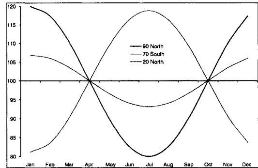
Figure 5.4. Seasonal fossil fuel emissions example with an amplitude factor of 20% and a base level of 100 units.
