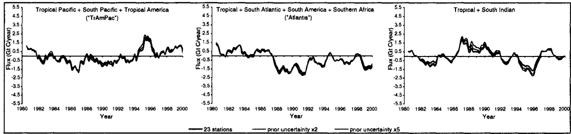
Figure 4.8. Estimated deseasonalized fluxes for three groupings of land and ocean regions as the prior uncertainty is loosened by 2x and 5x, respectively.
