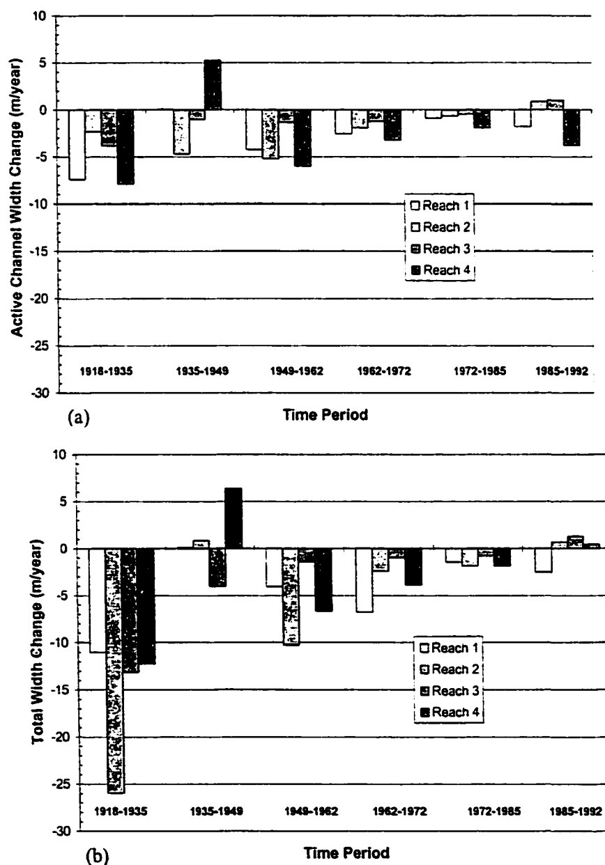
Figure 5-14 - Reach averaged change in channel width (a) change in non-vegetated active channel width, (b) change in total channel width between outer bank lines, including mid-channel bars and islands.
