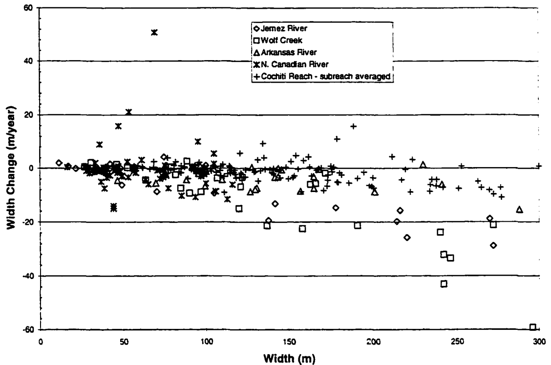
Figure 7-20 - Comparison of width vs. width change rate relationship between Cochiti reach and other published data. Non-Rio Grande river data are from Williams and Wolman (1984) and represent narrowing associated with dam closure.
