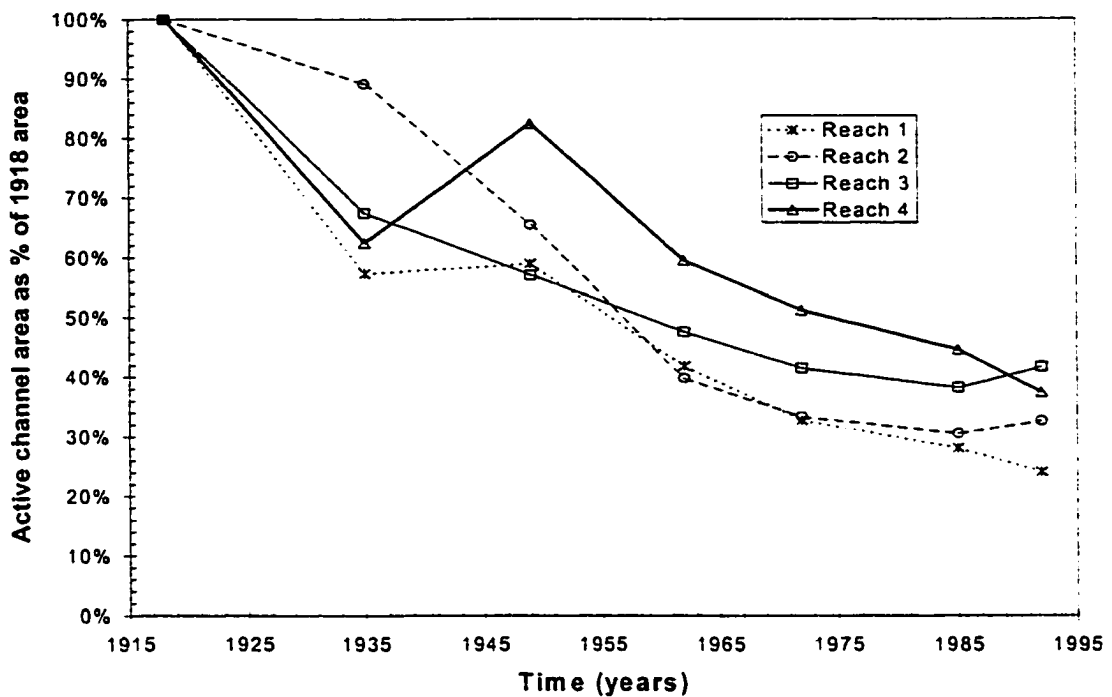
Figure 5-19 - Active channel area normalized by the active channel area in 1918.
