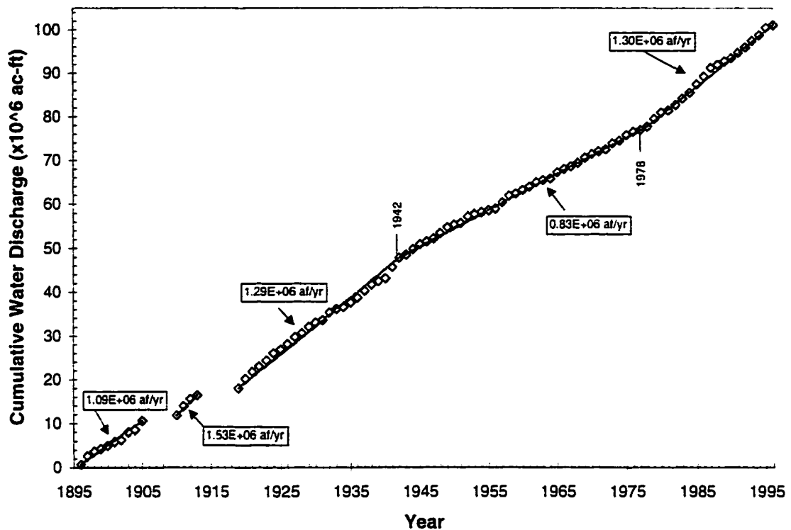
Figure 4-4 - Cumulative discharge for Otowi gage (1895-1996). (1ac-ft = 1,233 m 3 )
