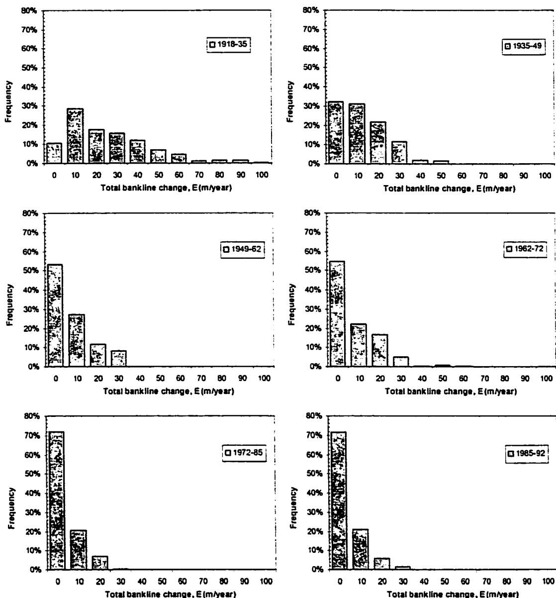
Figure 5-4 - Histograms of frequency of the total bankline change at all agg/deg lines.
