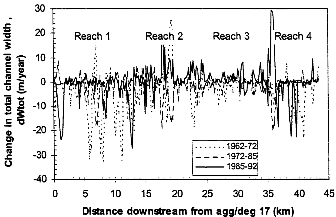
Figure 5-12 - Downstream plots of change in total channel width at each agg/deg line.
