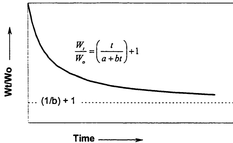
Figure 4-20 - Hyperbolic model of width change with time.
