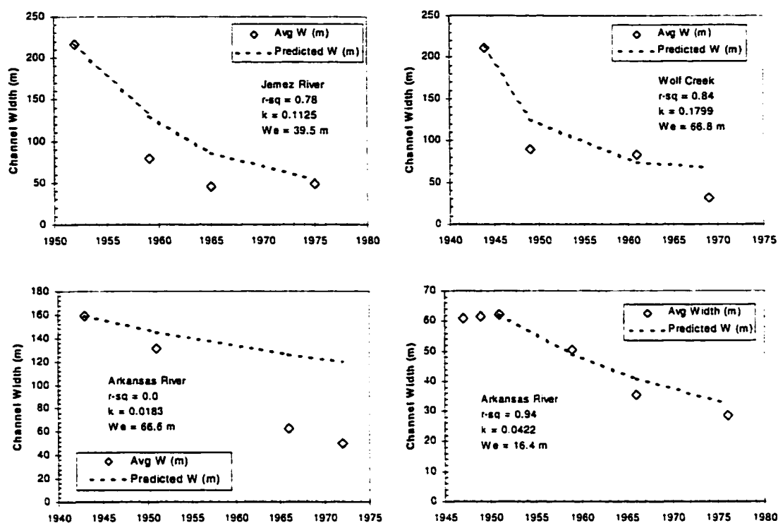
Figure 7-22 - Application of exponential model to width change data from Williams and Wolman (1984).
