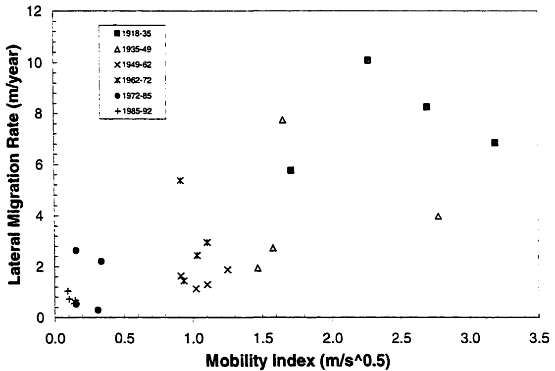
Figure 6-16 - Mobility index vs. lateral migration rate
