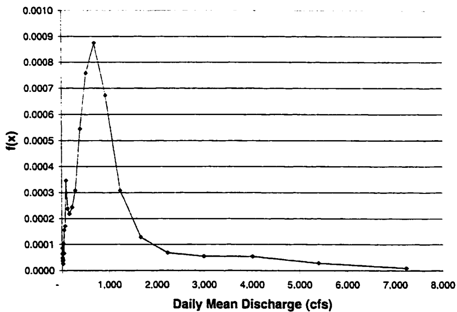
Figure 4-8 - Probability distribution function of daily mean discharge data (1 cfs = 0.0283 m 3 /sec) from Rio Grande at Cochiti (1974-1997)
