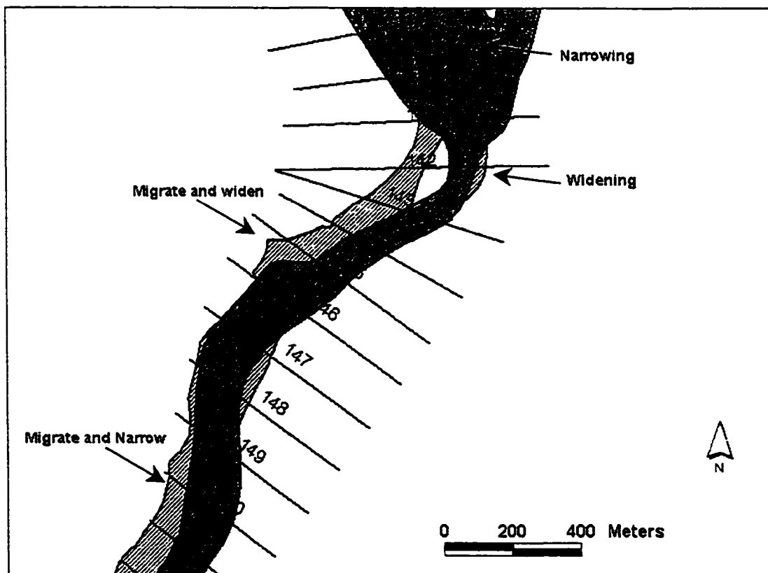
Figure 5-1 - River planform changes from 1918 to 1935. Rio Grande, NM.
