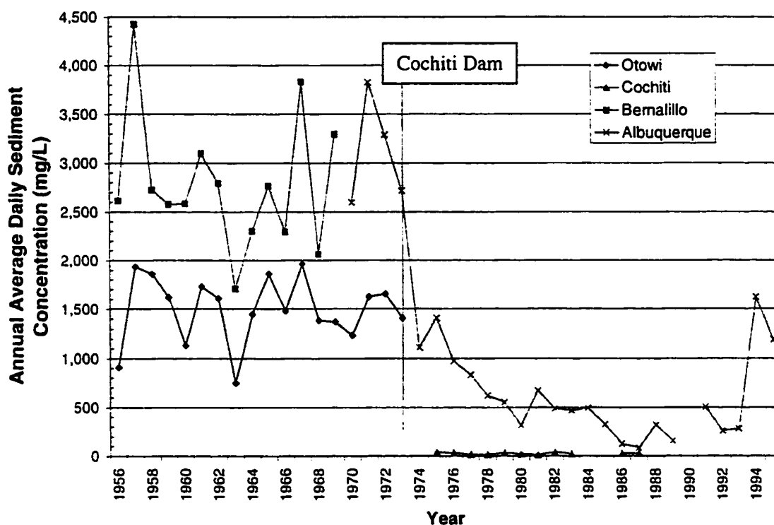
Figure 4-10 - Annual average suspended sediment concentration Rio Grande at Cochiti and Albuquerque (1975-1987).
