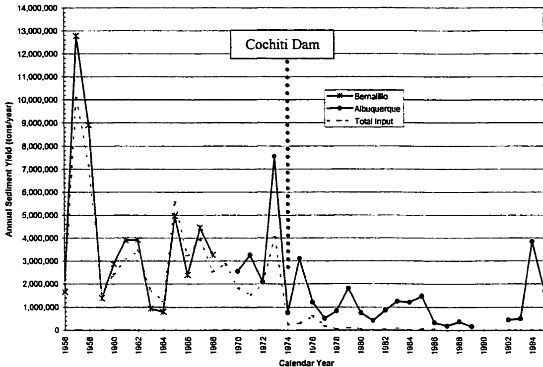
Figure 4-13 - Annual suspended sediment yield – Rio Grande, Cochiti reach
