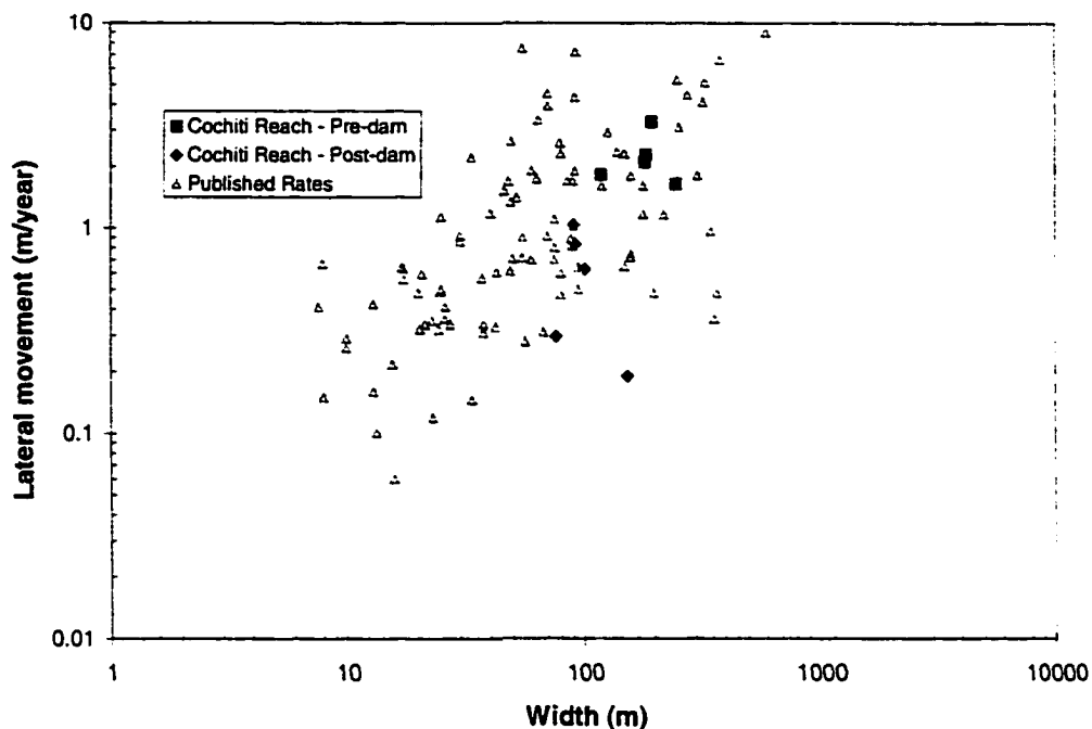
Figure 7-11 - Cochiti reach pre and post dam width and lateral movement data plotted with other published results.
