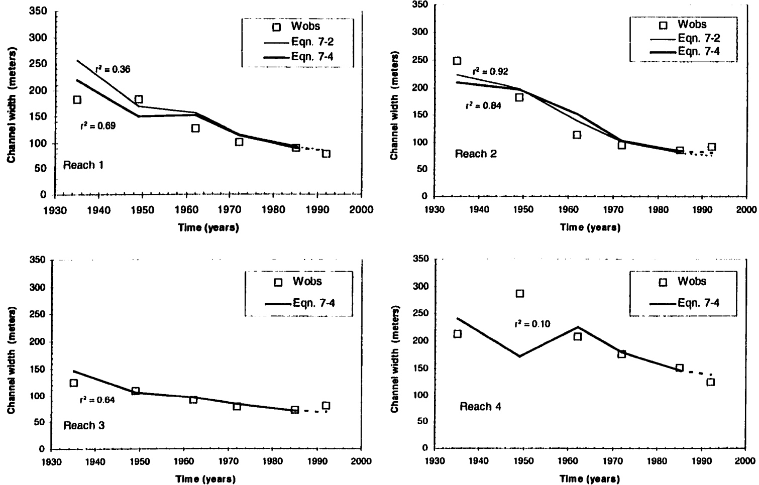
Figure 7-18 - Regression equations 7-2 and 7-4 applied to the reaches 1 through 4 of the Cochiti reach for active channel width estimation. The solid line represents calibration with 1918-1985 data, and the dashed line represents the validation with 1985-1992 data. The r^2 -values are computed for the entire time period.
