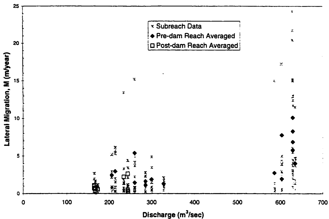
Figure 6-13 - Discharge vs. lateral migration rate.
