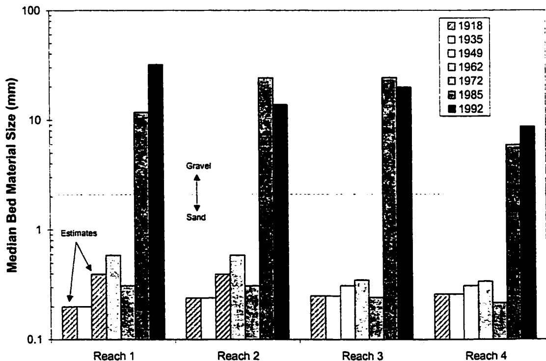
Figure 4-15 - Reach averaged median bed material size.
