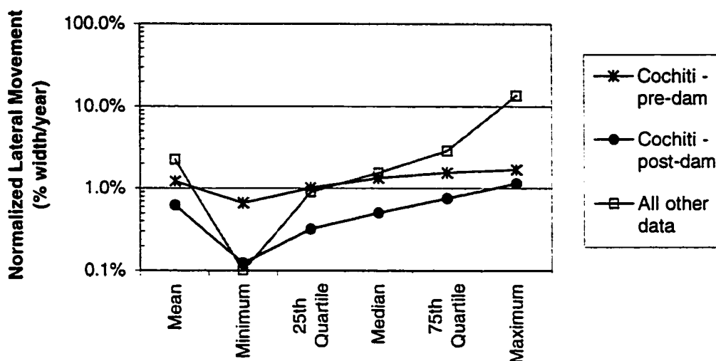
Figure 7-13 - Comparison of Rio Grande normalized lateral movement rates with other published rates.
