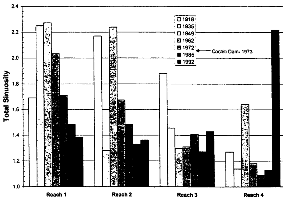
Figure 4-27 - Time series of total sinuosity.
