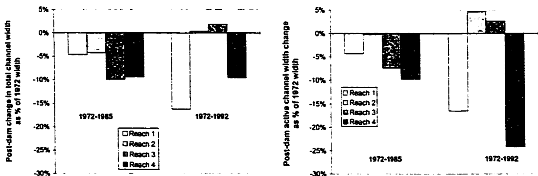
Figure 4-19 - Post-dam change in channel width as % of 1972 width.
