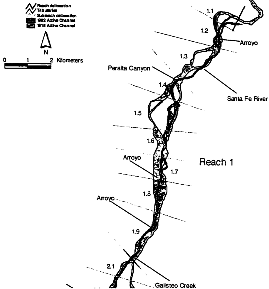
Figure 3-6 - Reach 1 - subreach delineation
