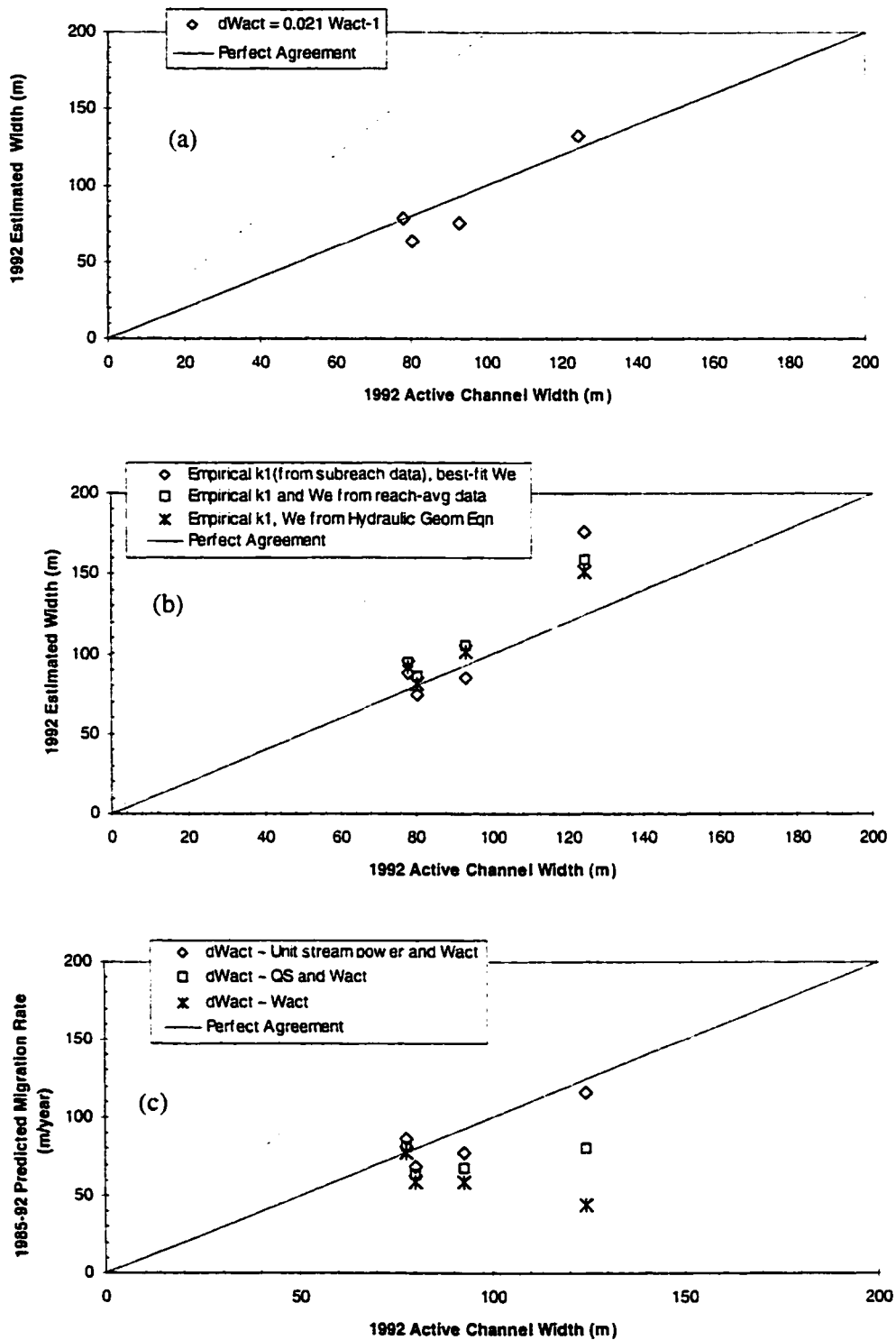
Figure 7-17 - Validation results for 1992 active channel width of reaches 1-4 of the Cochiti reach, Rio Grande, NM. (a) Simplified model, (b) Exponential models, (c) Regression models.
