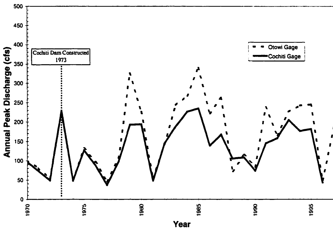
Figure 4-5 - Post-dam annual peak flows at Otowi and Cochiti gages
