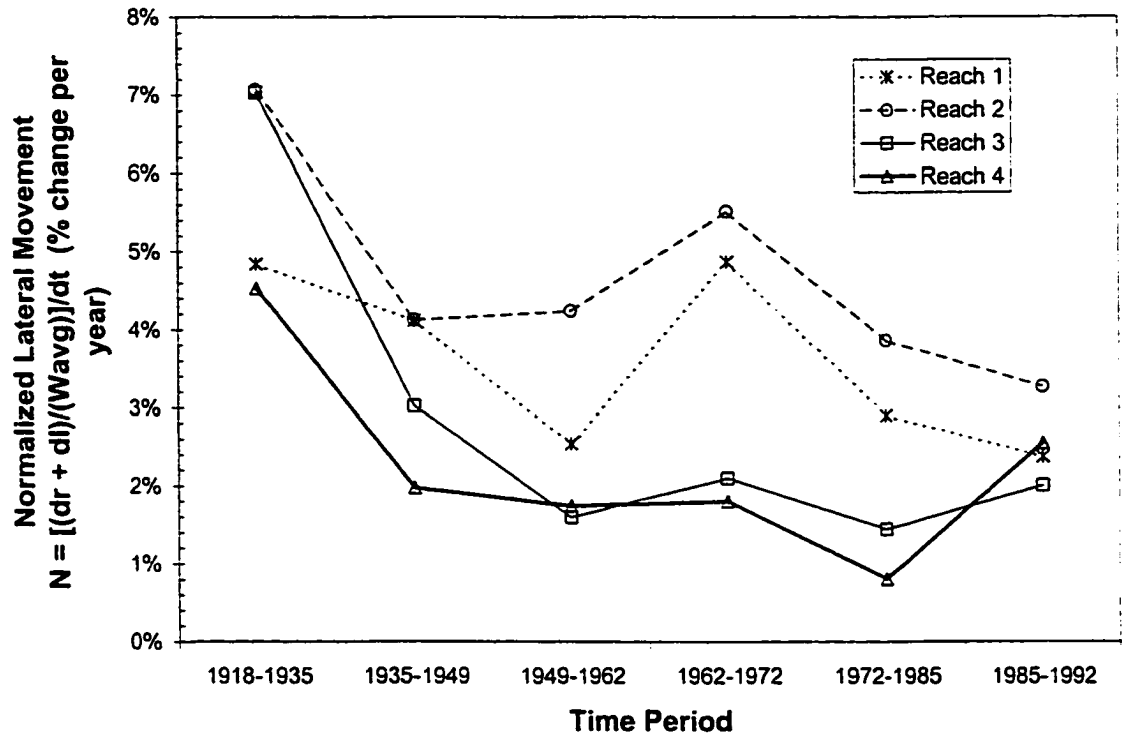
Figure 5-9 - Normalized lateral movement, N
