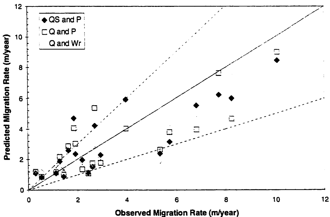
Figure 6-20 - Results of \log_{10} -transformed equations using reach averaged data from 1918 to 1985.
