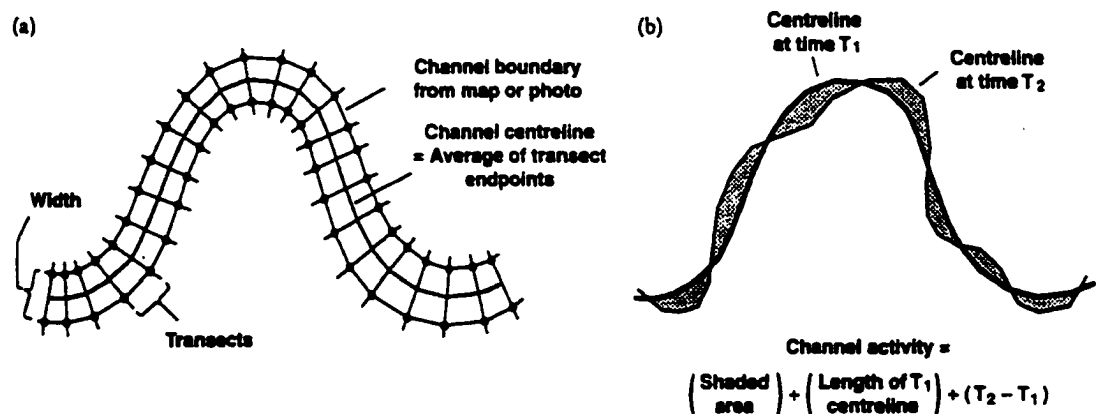
Figure 2-8 - Methods for measuring channel geometry and activity (a) Determination of channel centerline location and channel width, (b) Determination of channel activity (after Shields et al. 2000)
