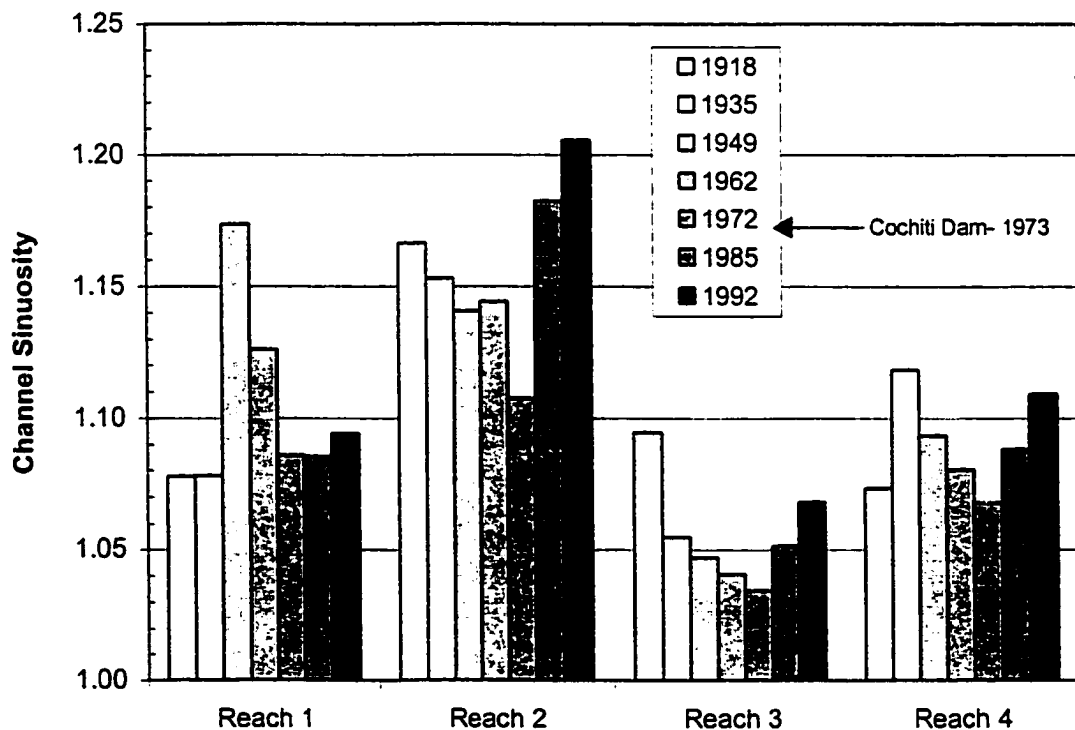
Figure 4-25 - Sinuosity of the reaches
