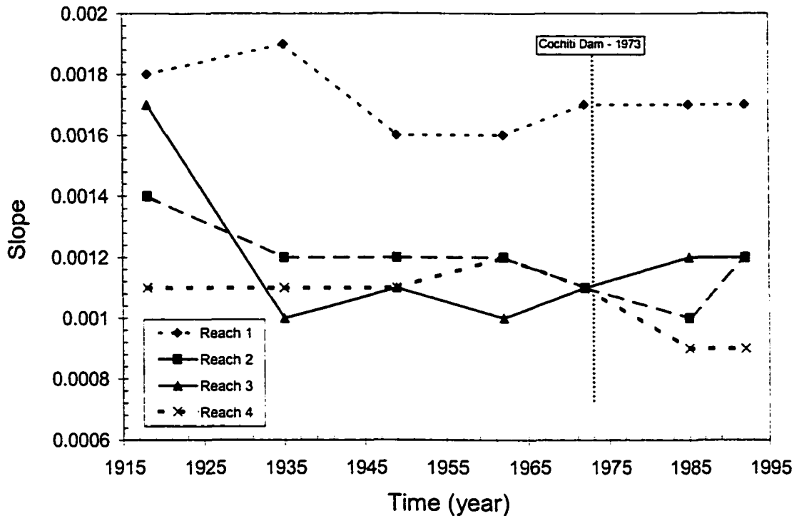
Figure 4-14 - Time series of slope for reach 1 through 4 of the Cochiti study reach.
