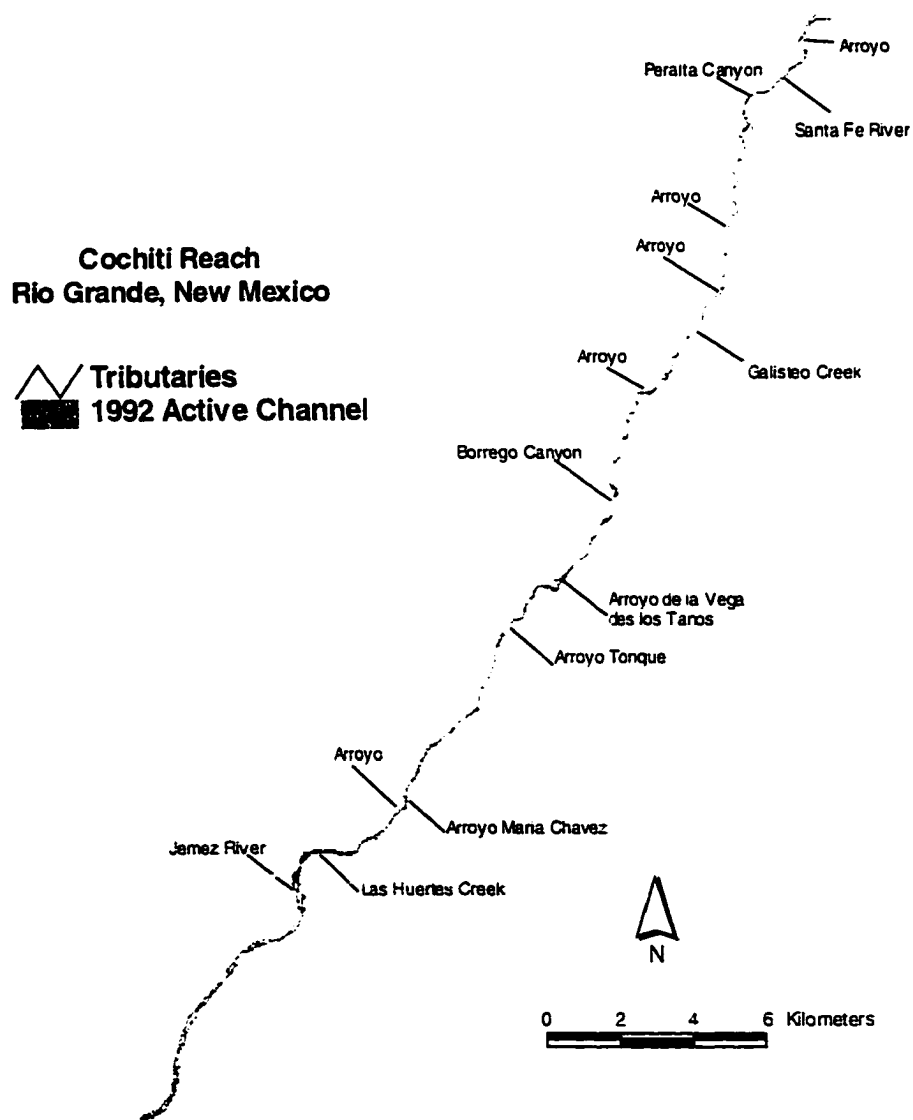
Figure 3-2 - Map of study reach with locations of tributaries.
