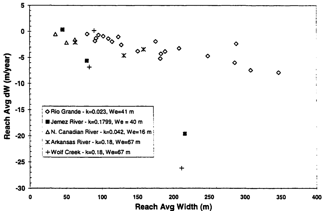
Figure 7-21 - Reach averaged channel width versus reach averaged annual change in width (m/year) for time periods where narrowing occurred ( dW < 0 ) except for last time period for the Jemez River, which widened 0.4 m/year. Non-Rio Grande data are from Williams and Wolman (1984) and represent narrowing associated with dam closure.
