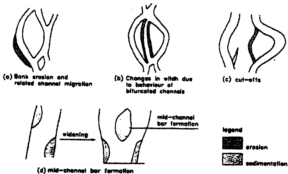
Figure 2-7 - Aggregated mechanisms of planform change in a braided river (after Mosselman 1995)
