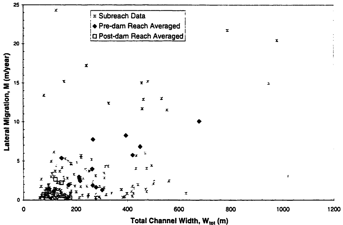
Figure 6-12 - Total channel width vs. lateral migration rate
