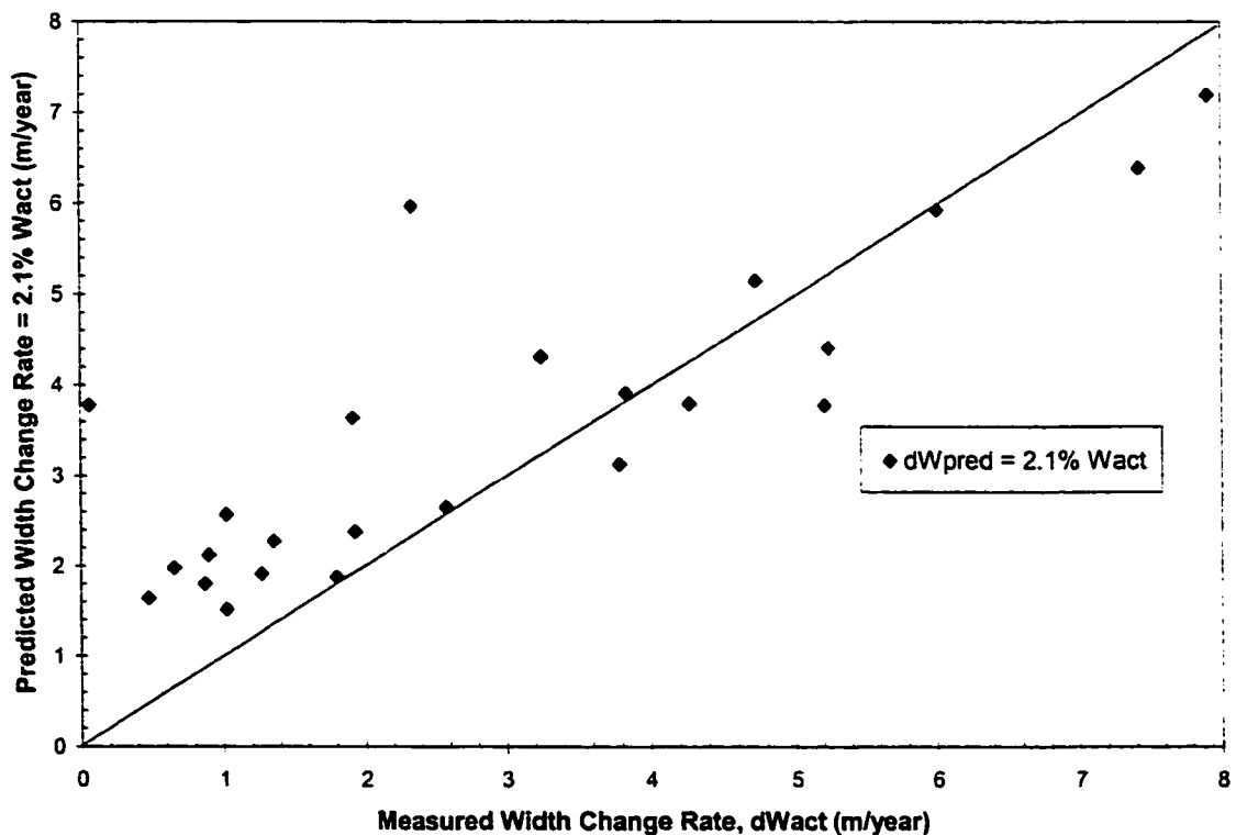
Figure 6-3 - Comparison of predicted vs. measured width change rates. The line indicates perfect agreement.
