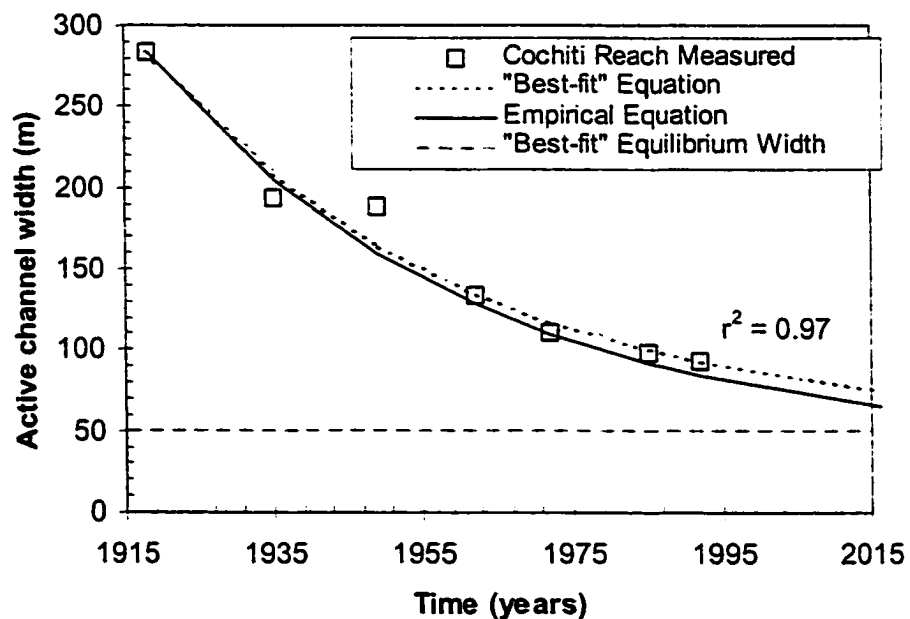
Figure 6-7 - Exponential model of width change applied to the entire Cochiti reach.
