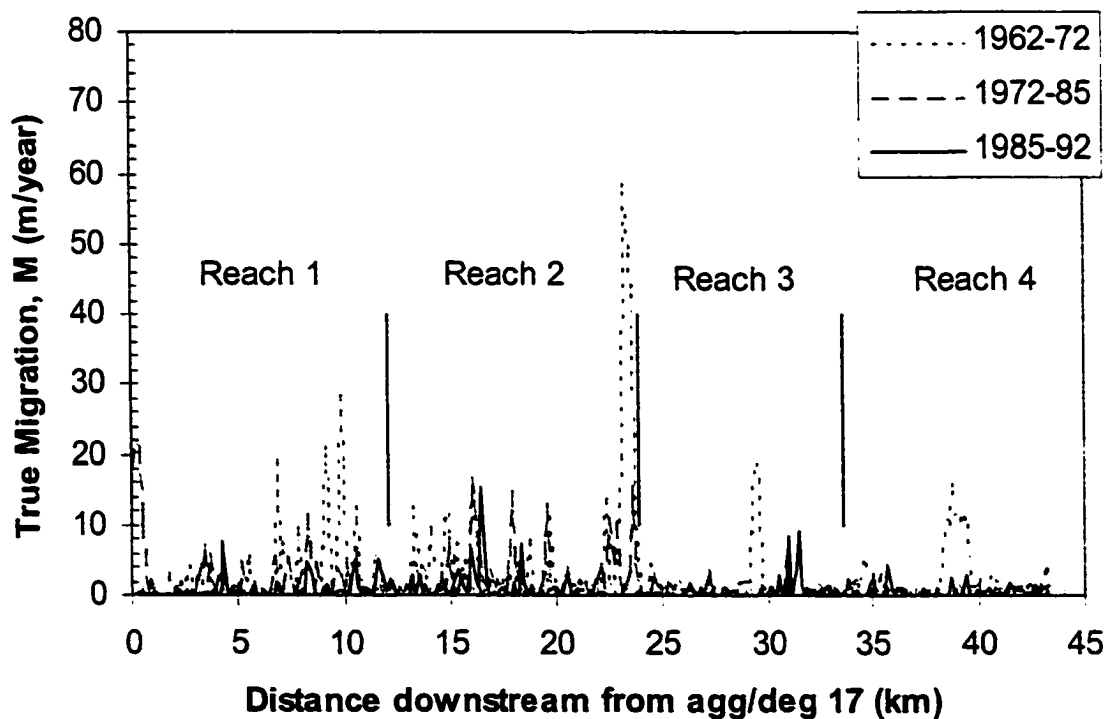
Figure 5-15 - True migration rate, M measured at each agg/deg line.
