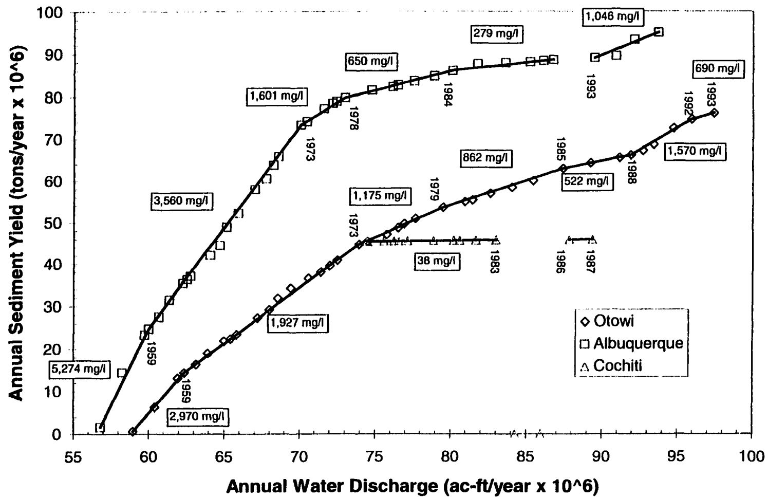
Figure 4-12 - Double-mass curve of annual water and sediment discharge at the Otowi, Cochiti and Albuquerque gages. The slope of the curve indicates the average suspended sediment concentration for the time period.
