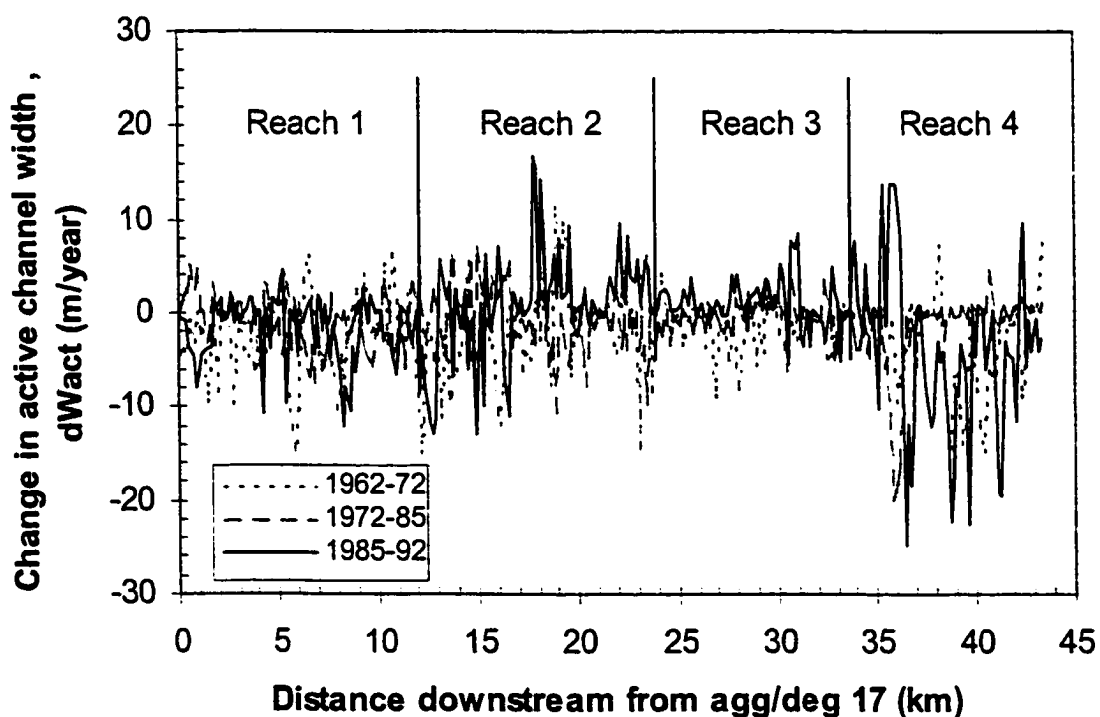
Figure 5-10 - Downstream plots of change in active channel width at the agg/deg lines for each.
