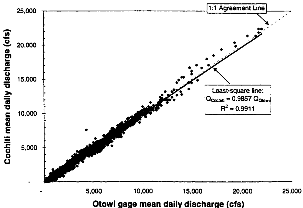
Figure 4-1 - Comparison of daily mean discharge measured at the Otowi and Cochiti gages (1927 to 1996).
