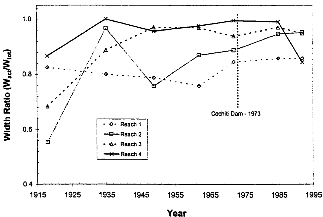
Figure 4-28 - Time series of width ratio for reaches 1 through 4
