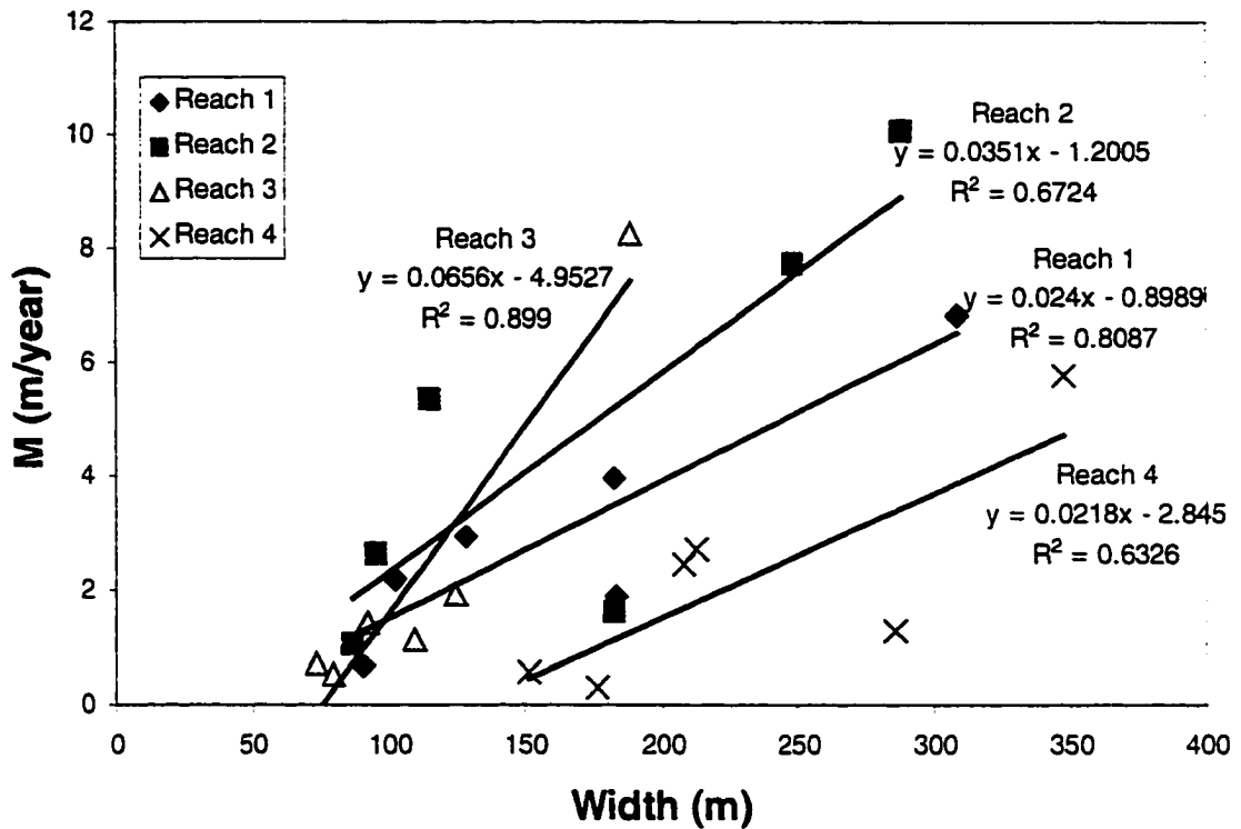
Figure 6-9 - Lateral migration, M (m/year) plotted against the active channel width (m) for estimation of the parameter k , the slope of the regression line.
