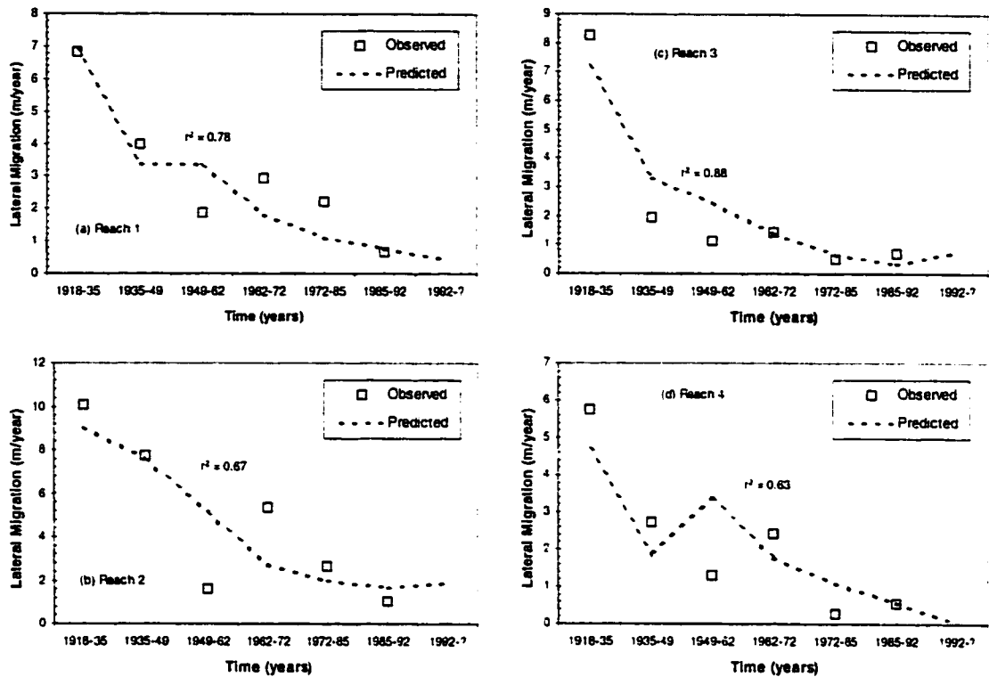
Figure 6-10 - Predicted M using W_e predicted from dW-W relationship and "best-fit" k -values.
