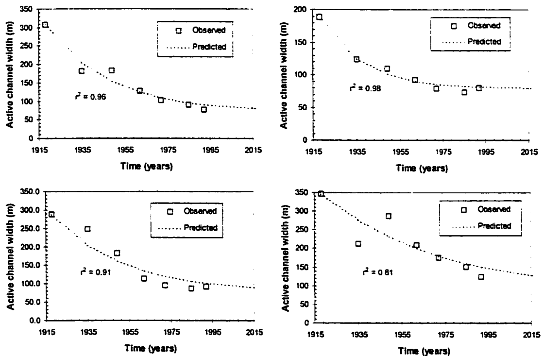
Figure 6-8 - Application of exponential model of width change using Julien and Wargalam's (1995) predicted equilibrium width and empirically derived k .
