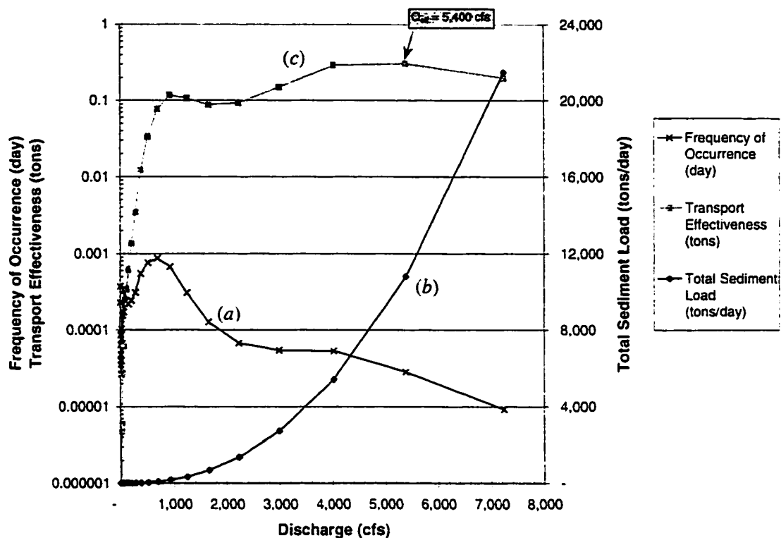
Figure 4-9 - (a) Daily mean discharge frequency (Rio Grande at Cochiti, 1974 - 1997), (b) Total sediment transport rate as a power function of discharge (Bernalillo Island total sediment load data, 1992-1996), and, (c) The product of a and b , transport effectiveness. The maximum of the transport effectiveness curve is the effective discharge, Q_{eff} . (1 cfs = 0.0283 m 3 /sec)
