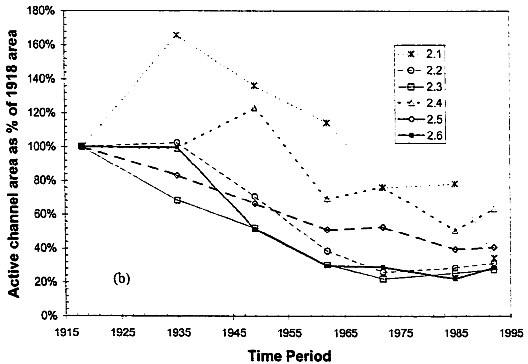
Figure 5-20 - Active channel area of subreaches normalized by the area in 1918 (a) Reach 1, (b) Reach 2.
