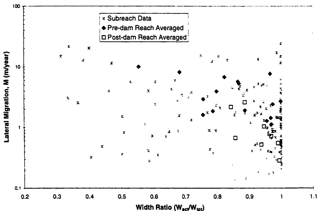
Figure 6-17 - Width ratio vs. lateral migration rate.
