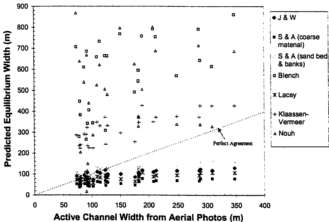
Figure 4-22 - Results of equilibrium width prediction by hydraulic geometry equations.
