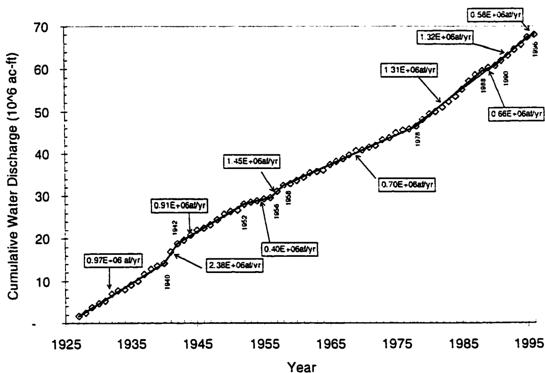
Figure 4-3 - Cumulative discharge for Cochiti Gage (1927-1996) (1ac-ft = 1,233 m 3 )
