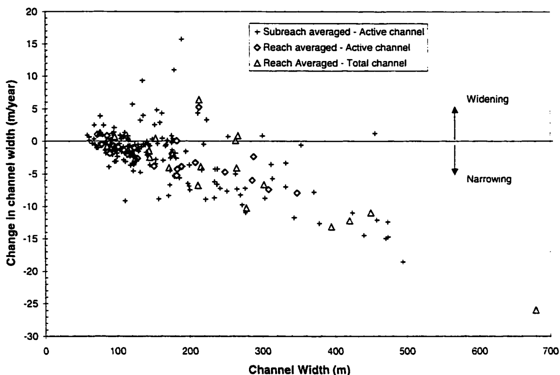
Figure 6-18 - Channel width vs. change in active channel width
