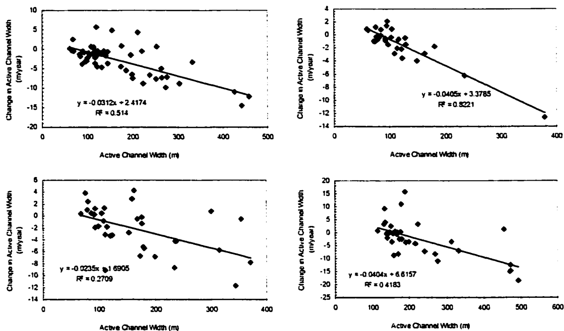
Figure 6-5 - Linear regression results of subreach-averaged data - observed width change (m/year) with observed active channel width (m).
