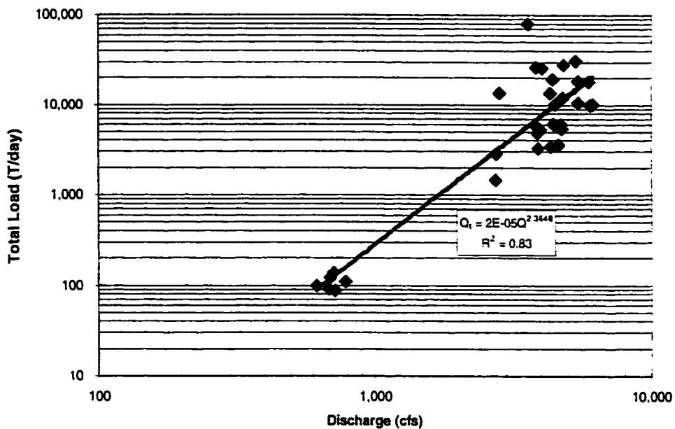
Figure 4-7 - Total sediment load rating curve developed from Bernalillo Island total sediment data (1992-1996) estimated using Modified Einstein Procedure.
