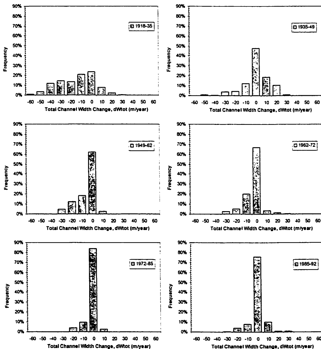
Figure 5-13 - Probability density functions of change in total channel width at agg/deg lines.
