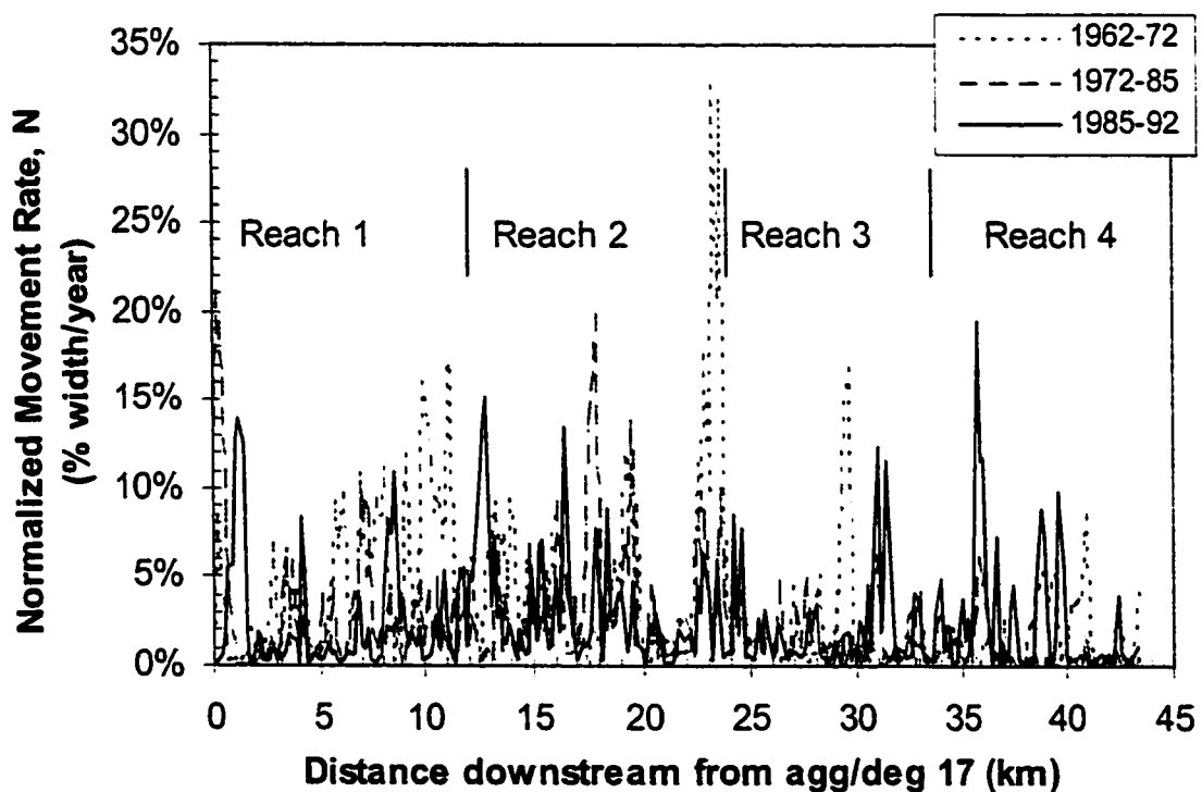
Figure 5-7 - Normalized lateral movement rates, N , expressed as % of width per year measured at each agg/deg line.
