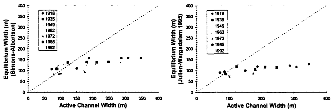
Figure 4-23 - Equilibrium width prediction using Simons and Alberston (1963) and Julien and Wargadalam (1995).
