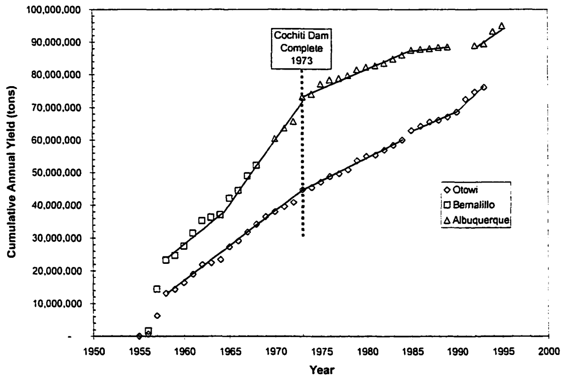
Figure 4-11 - Cumulative mass curve of annual suspended sediment yield.
