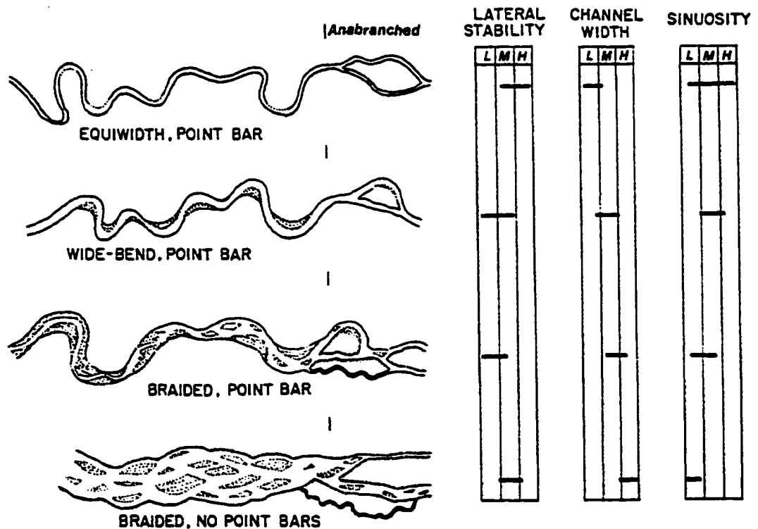
Figure 2-5 - Alluvial stream types (after Brice 1982)
