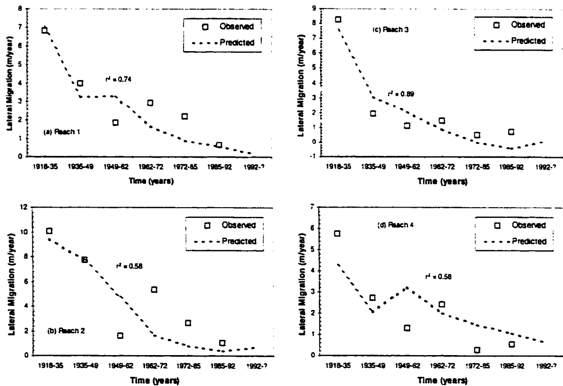
Figure 6-11 - Predicted M using W_e from hydraulic geometry equations.
