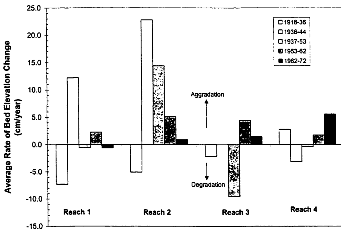
Figure 4-16 - Pre-dam average rate of bed elevation change (cm/year).
