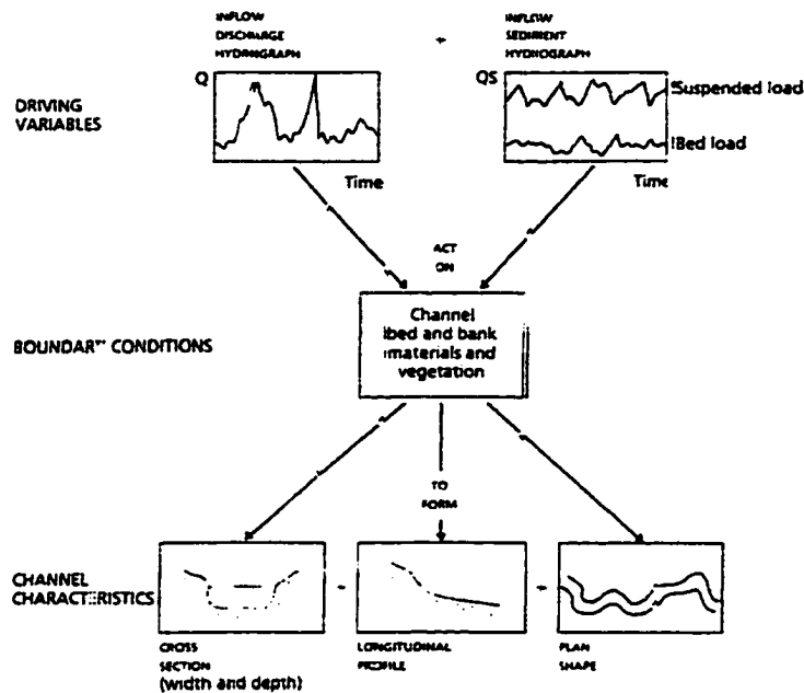
Figure 2-1 - Equilibrium concept for erodible channels (after Brookes 1992)
