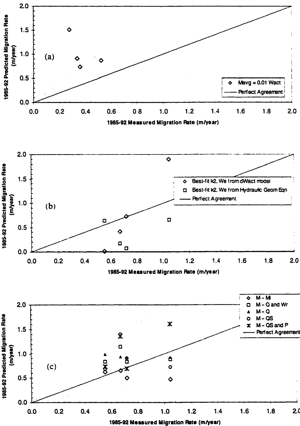
Figure 7-14 - Validation results for 1985-92 lateral migration rate of reaches 1-4 of the Cochiti reach, Rio Grande, NM. (a) Simplified model. (b) Exponential models, (c) Regression models.
