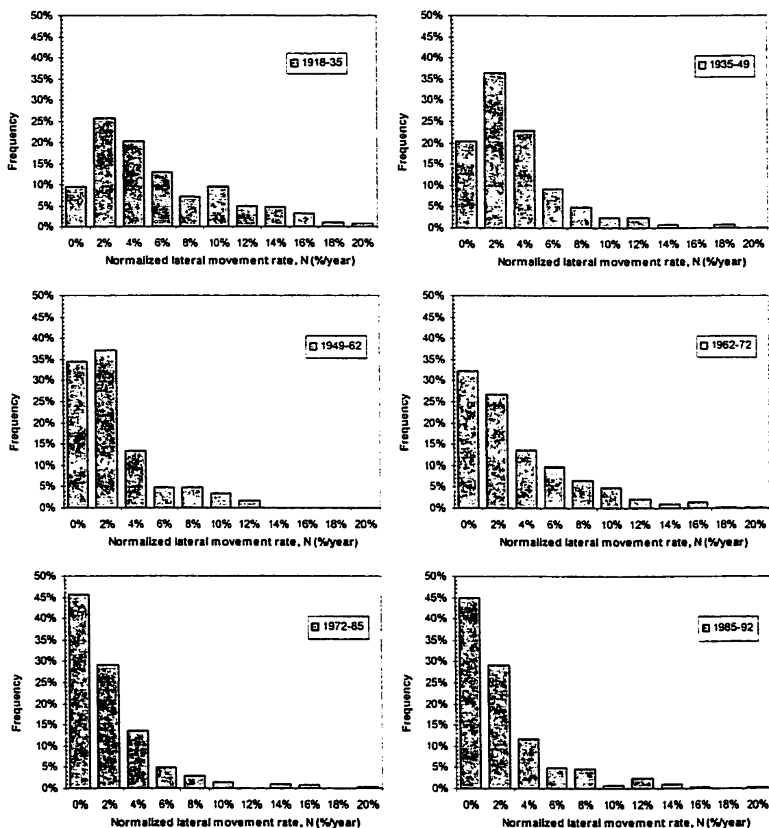
Figure 5-8 - Histograms of the frequency of the normalized lateral movement rate measured at each agg/deg line.
