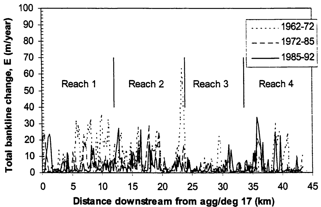
Figure 5-3 - Total bankline change, E, for each agg/deg line
