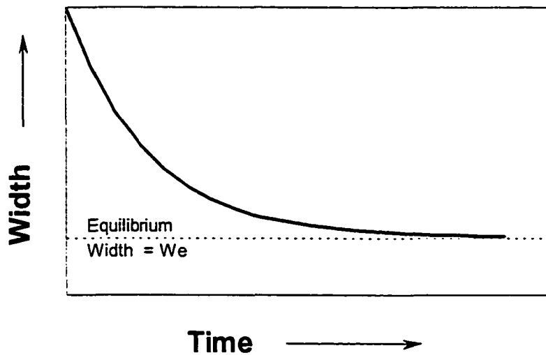
Figure 6-4 - Schematic of exponential channel width changes with time.
