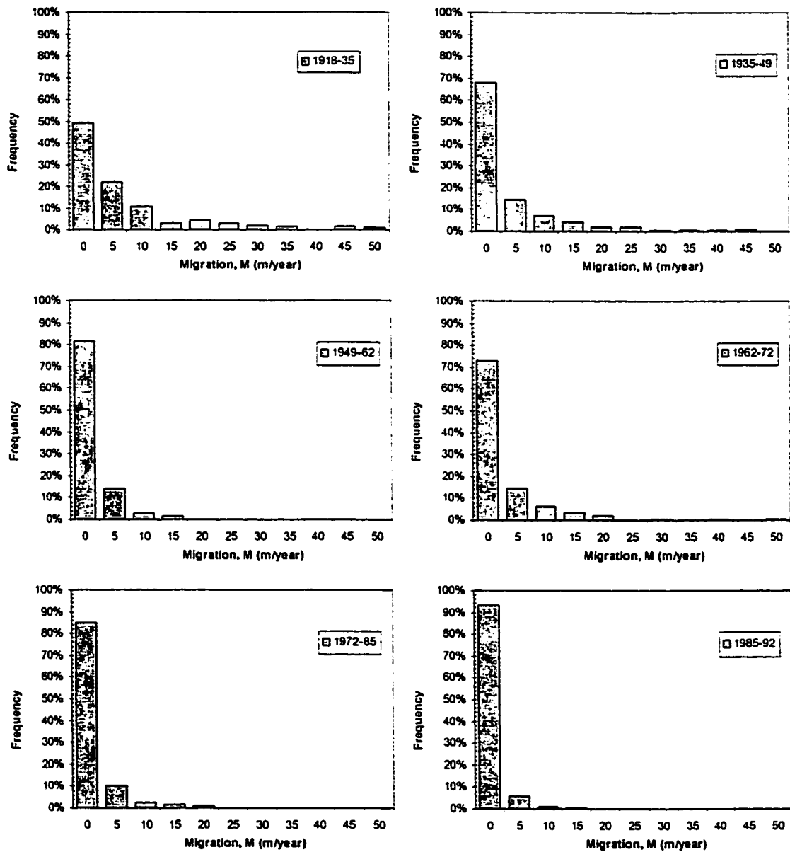
Figure 5-16 - Histograms of frequency of occurrence of migration rate at all the agg/deg lines.
