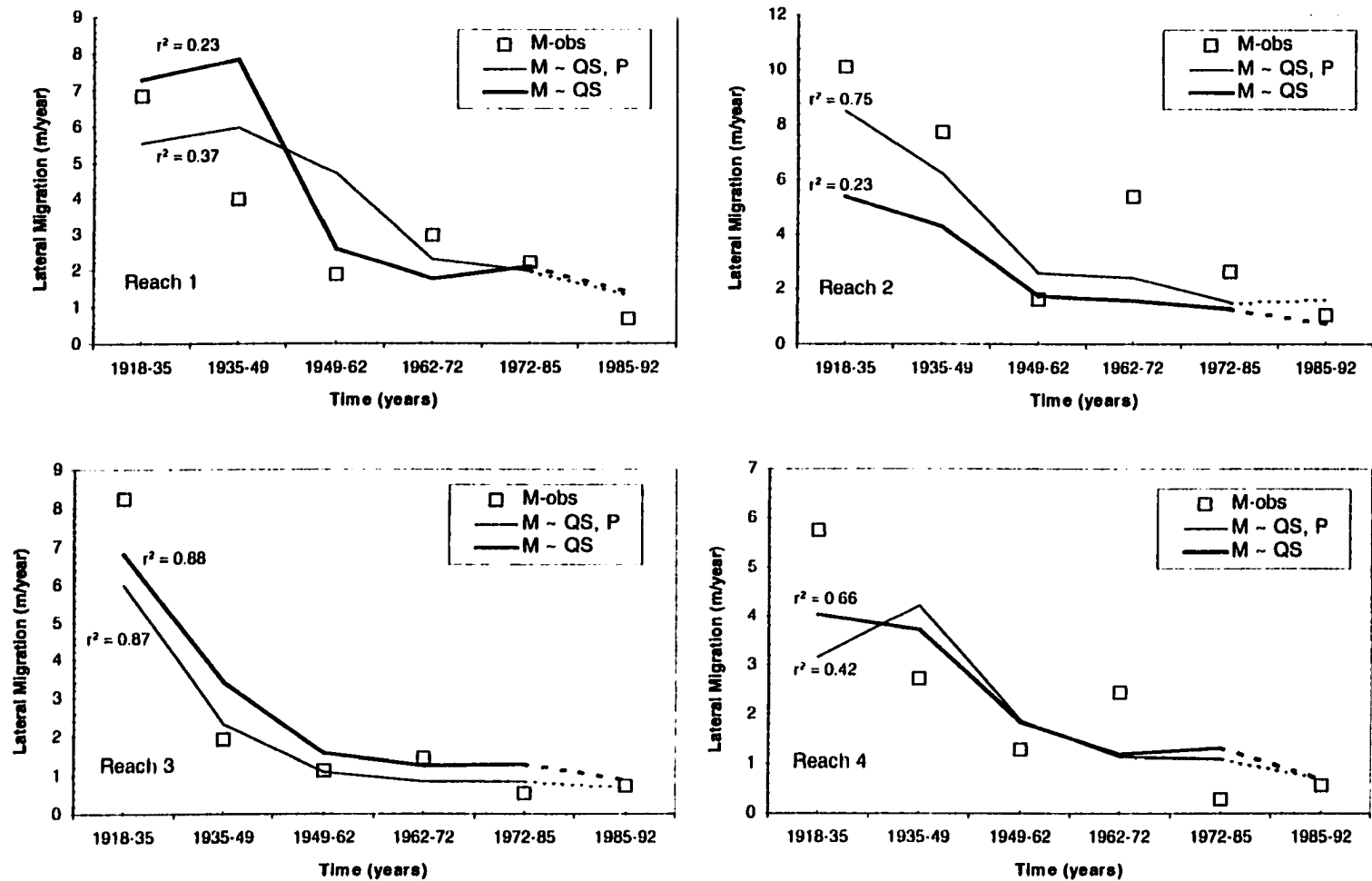
Figure 7-16 - Regression equations applied to the reaches 1 through 4 of the Cochiti reach. The solid line represents calibration with 1918-1985 data, and the dashed line represents the validation with 1985-1992 data. The r^2 -values are computed for the entire time period.
