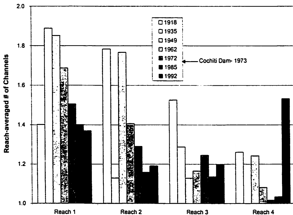
Figure 4-26 - Time Series of Average Number of Channels – Cochiti reach.
