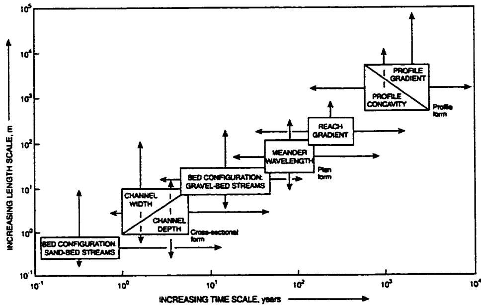
Figure 2-3 - Time-scales of adjustment (after Knighton 1998)
