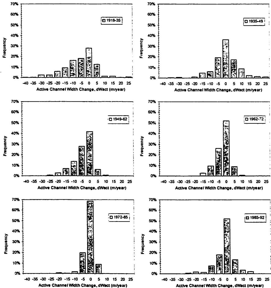
Figure 5-11 - Probability density functions of change in active channel width at agg/deg lines.
