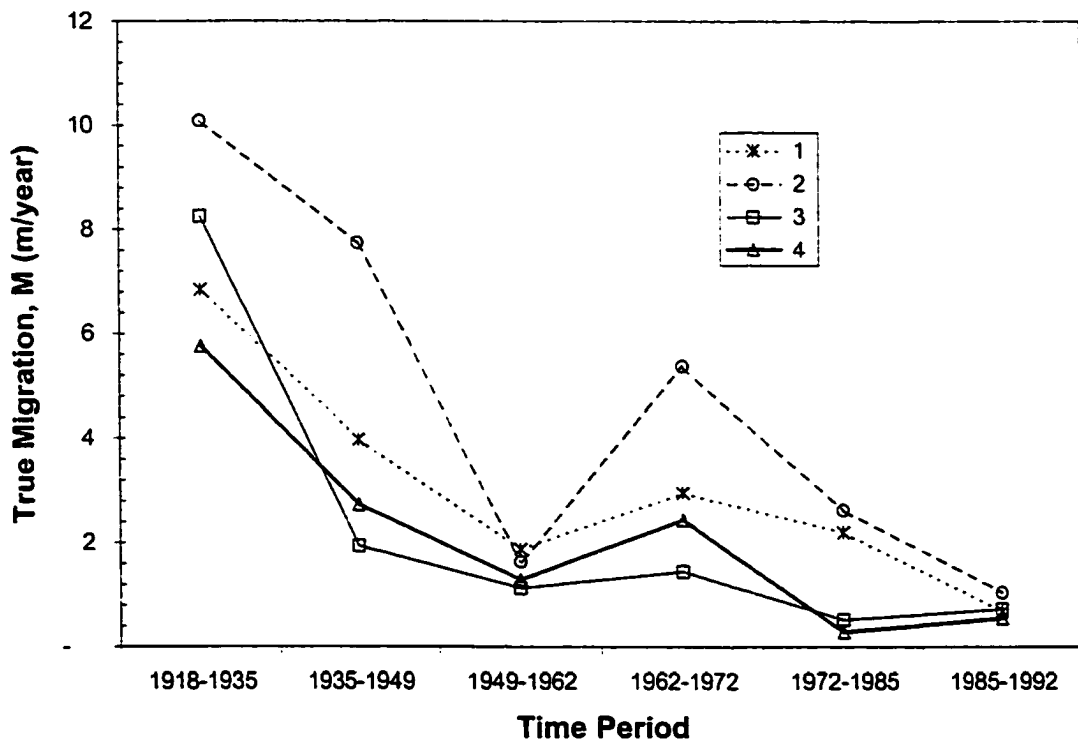
Figure 5-17 - Time series of true migration rate, M
