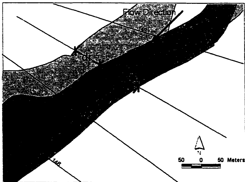
Figure 5-2 - Measurement of bankline change at agg/deg 144 between 1918 and 1935.
