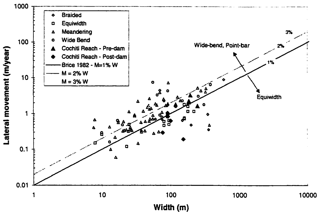
Figure 7-19 - Lateral movement rate in relation to channel width for different types of streams.
