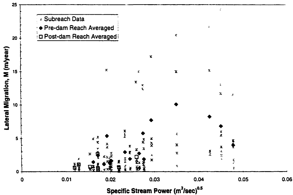
Figure 6-14 - Specific stream power vs. lateral migration rate.
