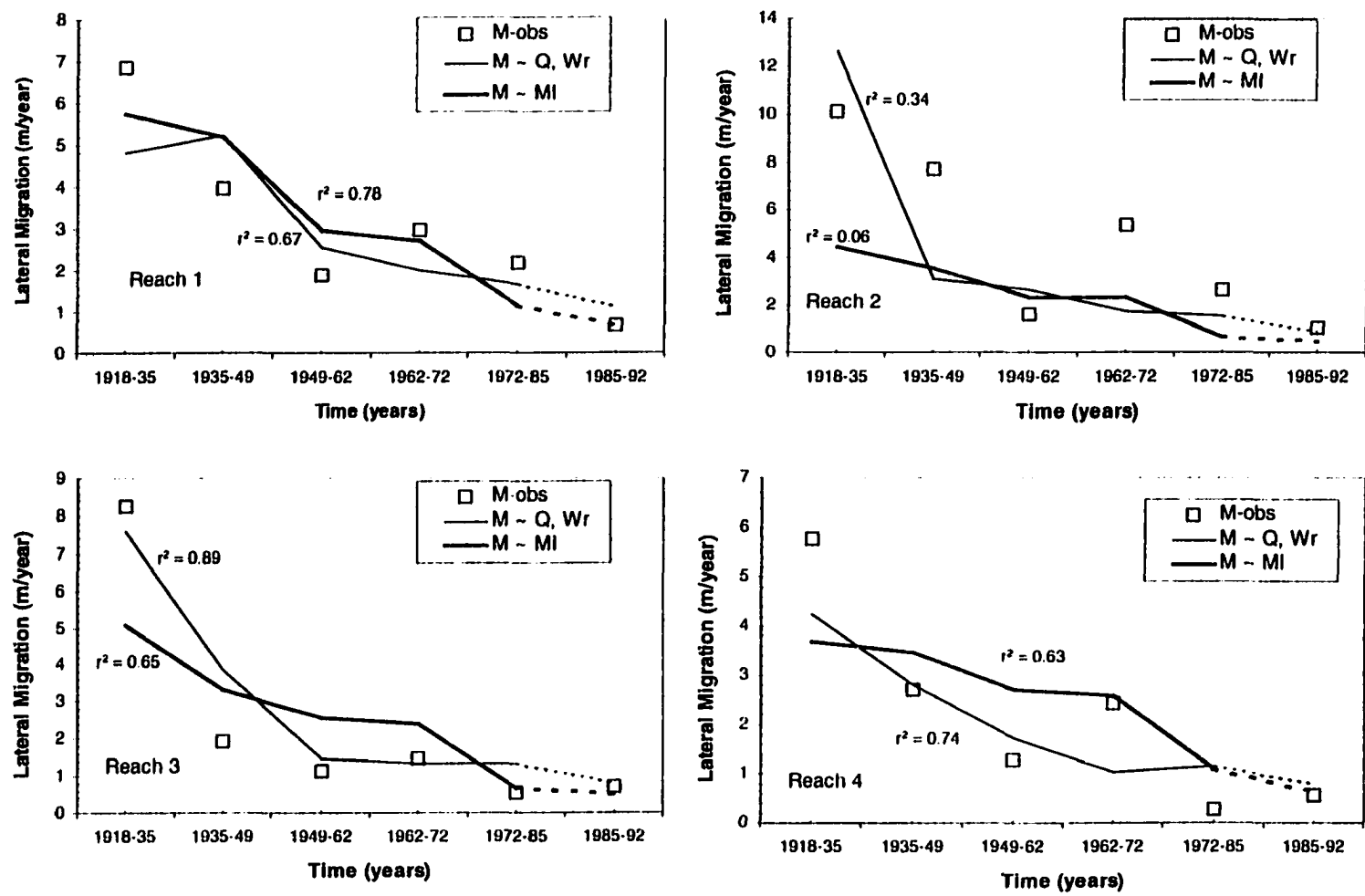
Figure 7-15 - Regression equations applied to the reaches 1 through 4 of the Cochiti reach. The solid line represents calibration with 1918-1985 data, and the dashed line represents the validation with 1985-1992 data. The r^2 -values are computed for the entire time period.
