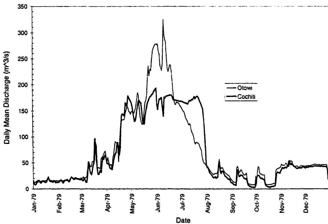
Figure 4-6 - 1979 Discharge hydrograph at Otowi and Cochiti gaging stations.
