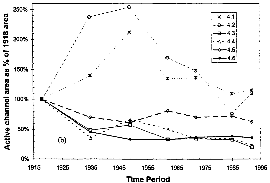
Figure 5-21 - Active channel area of subreaches normalized by the area in 1918 (a) Reach 3, (b) Reach 4.
