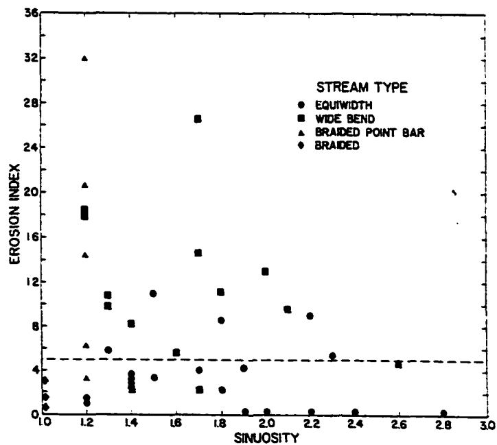
Figure 2-10 - Relationship between erosion index and channel planform (after Brice 1982)
