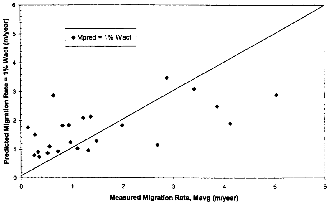
Figure 6-1 - Comparison of predicted migration rates vs. measured. The line represents perfect agreement.
