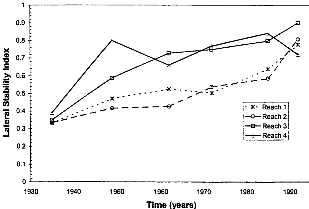
Figure 5-23 - Lateral stability index - Time series of the area of active channel that remained unchanged since the last aerial photo. It is expressed as a percentage of the previous total active channel area.
