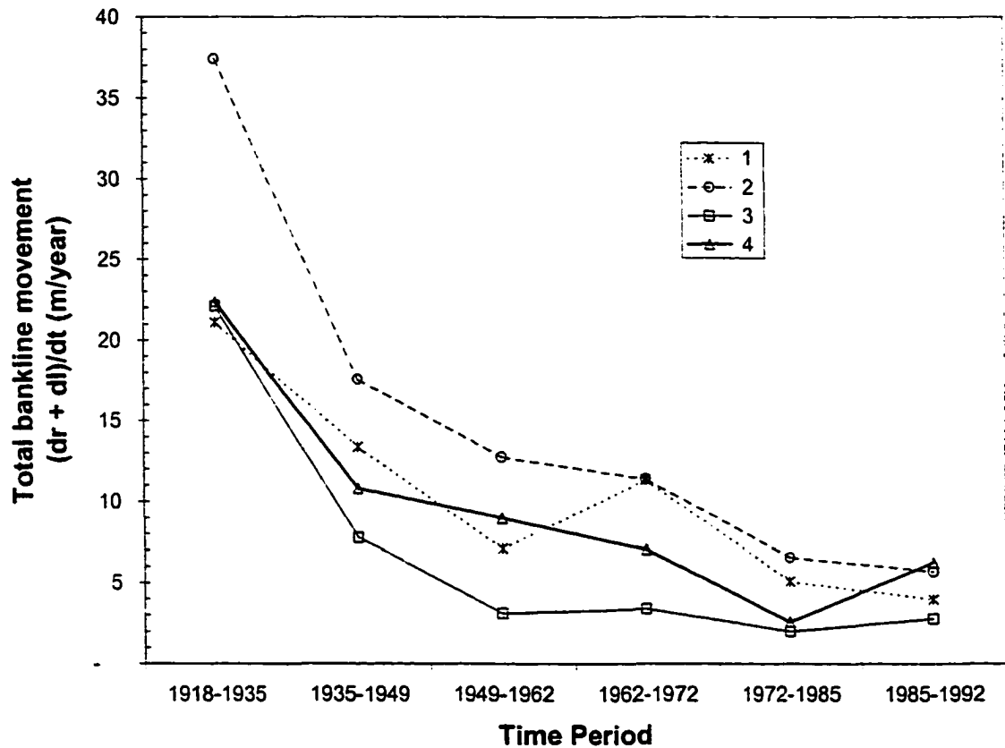
Figure 5-5 - Reach-averaged - Total bankline change per year. Erosion rate, E
