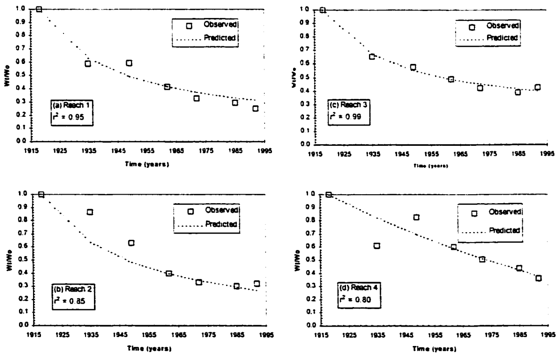
Figure 4-21 - Application of Williams and Wolman (1984) hyperbolic width change model to reaches 1-4 of the study reach.
