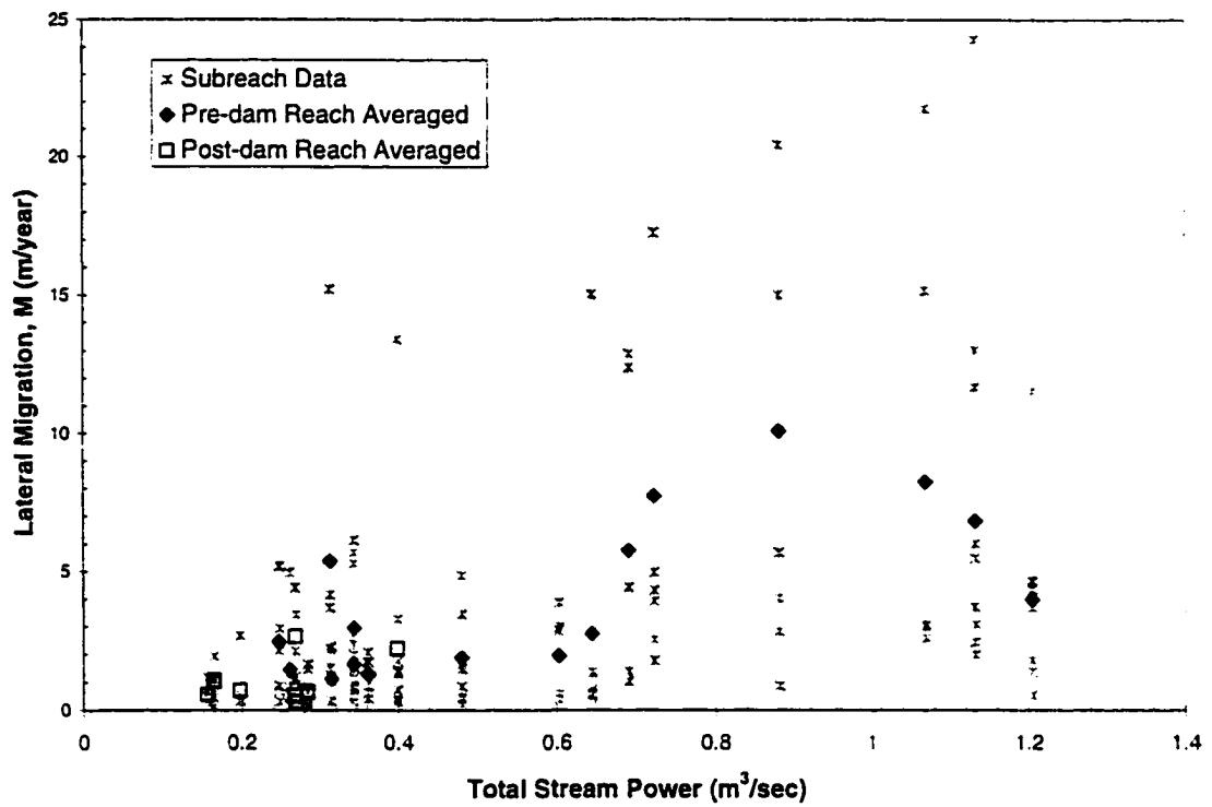
Figure 6-15 - Total stream power vs. lateral migration rate
