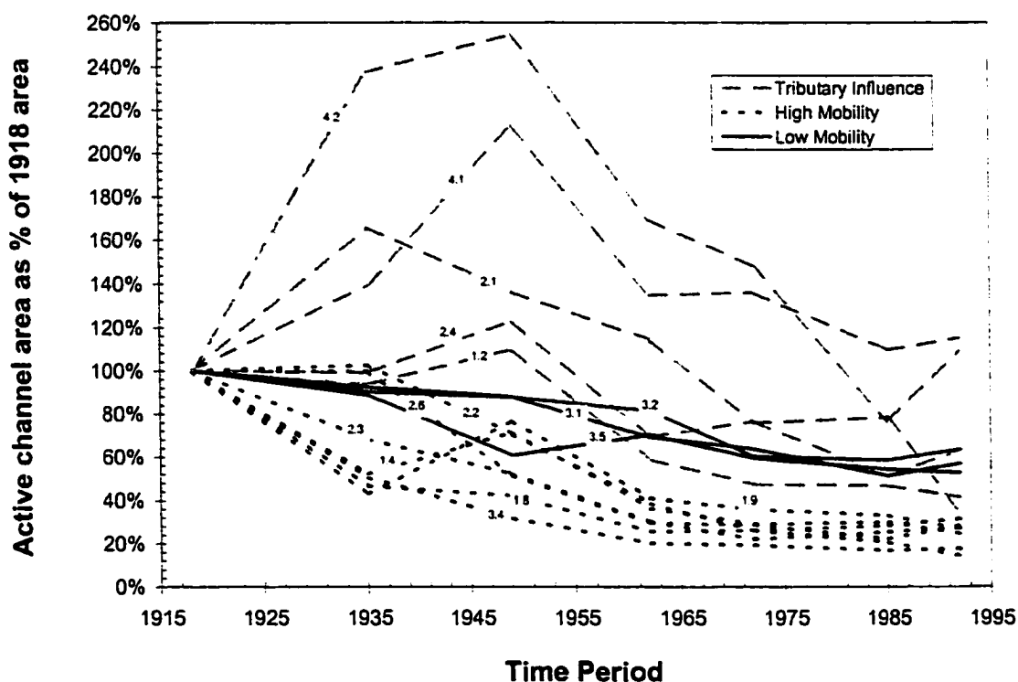
Figure 5-24 - Change in active channel area of the subreaches that exhibit either high or low mobility or tributary influence. The subreach number is given on the line.
