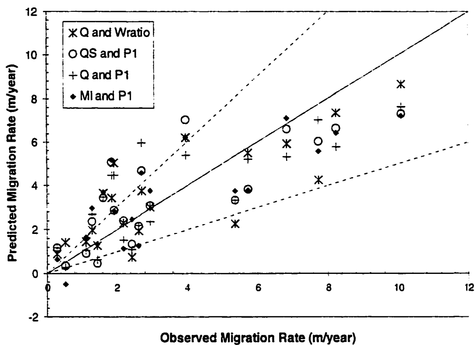
Figure 6-19 - Results of arithmetic regression models using reach-averaged data from 1918 to 1985.
