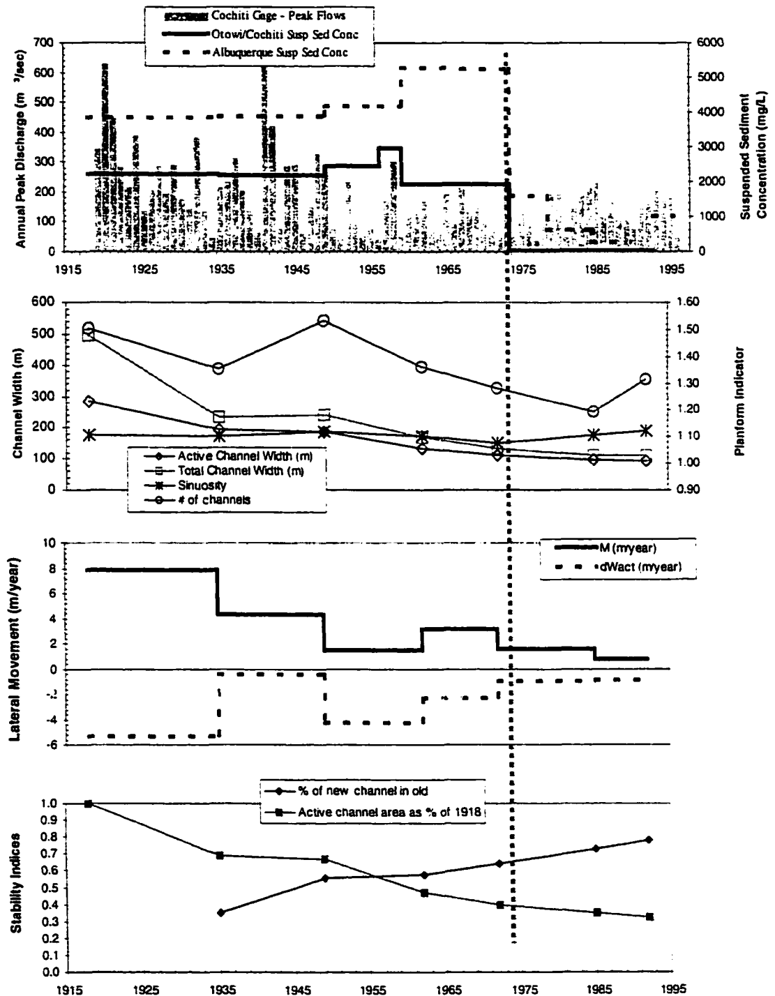
Figure 7-1 - Changes in Cochiti reach from 1918 to 1992.
