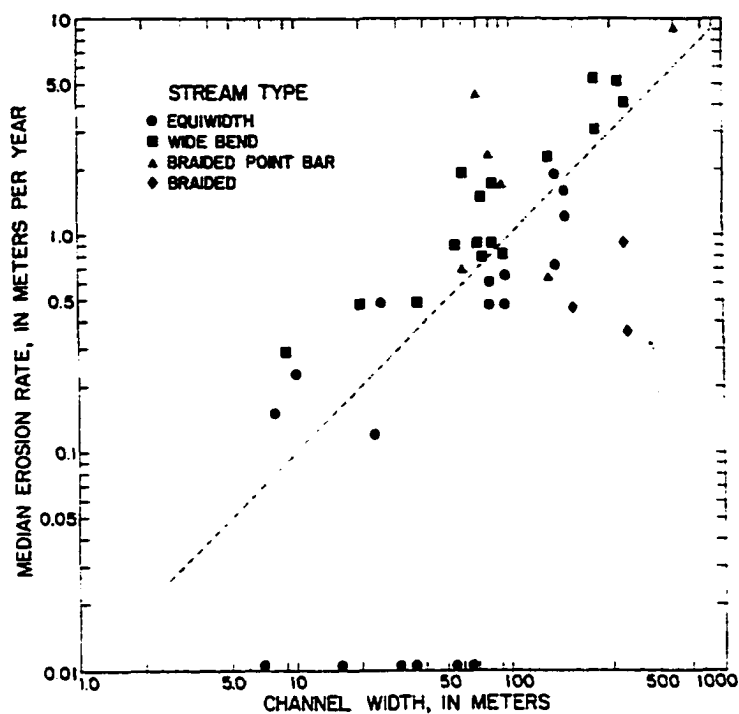
Figure 2-9 - Relationship between lateral channel movement and channel width (after Brice 1982)
