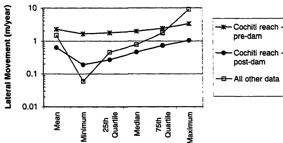
Figure 7-12 - Comparison of Rio Grande lateral movement rates with other published rates.
