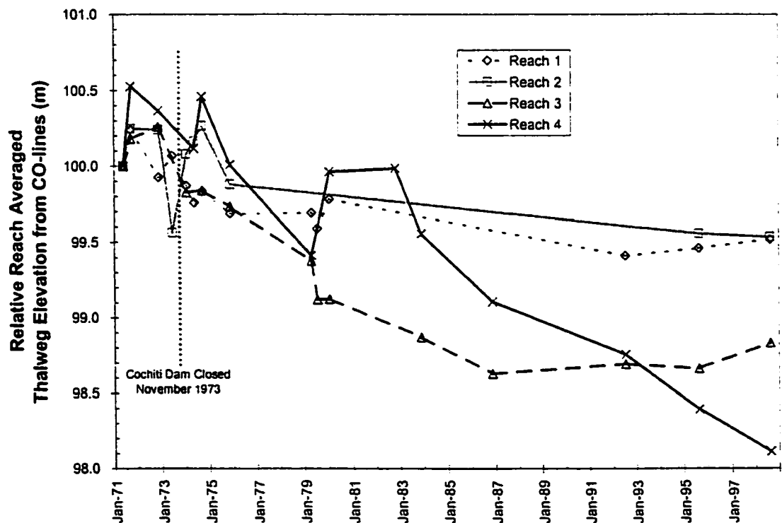
Figure 4-17 - Post-dam thalweg elevation changes using CO-line surveys from 1971 to 1998.
