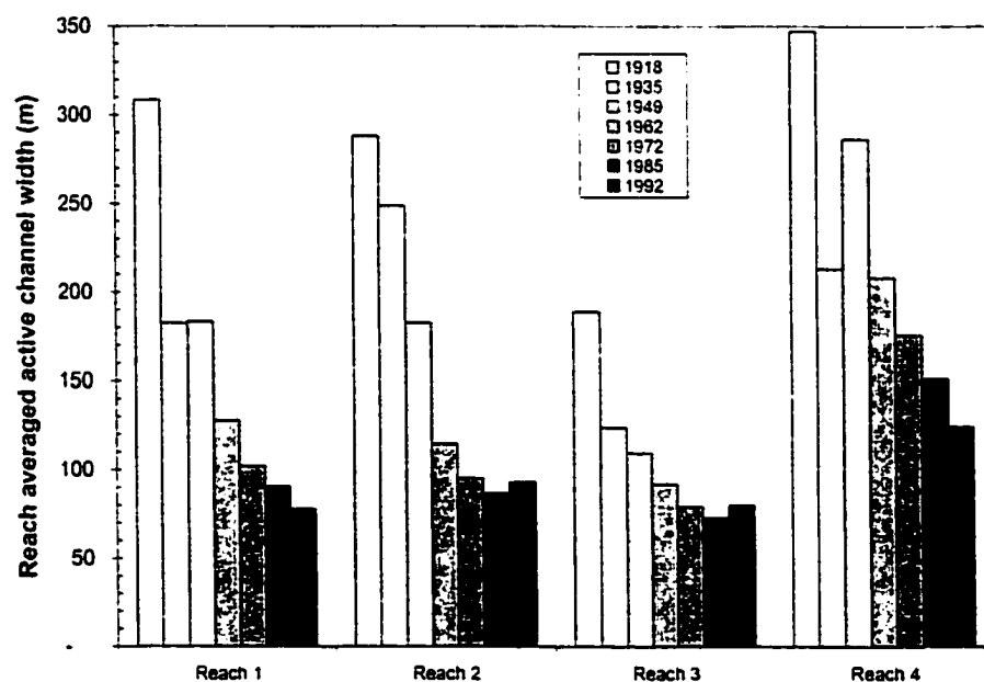
Figure 4-18 - Reach averaged active channel width.
