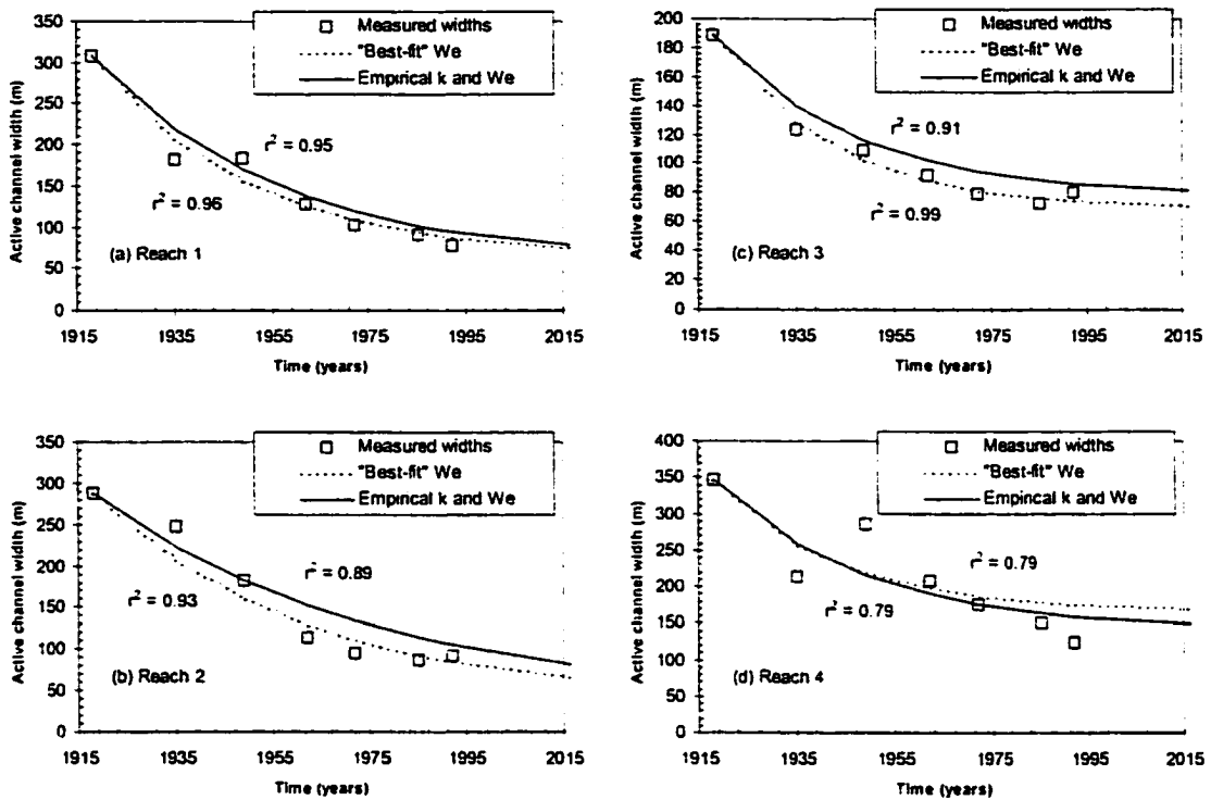
Figure 6-6 - Exponential models of width change applied to the reaches.
