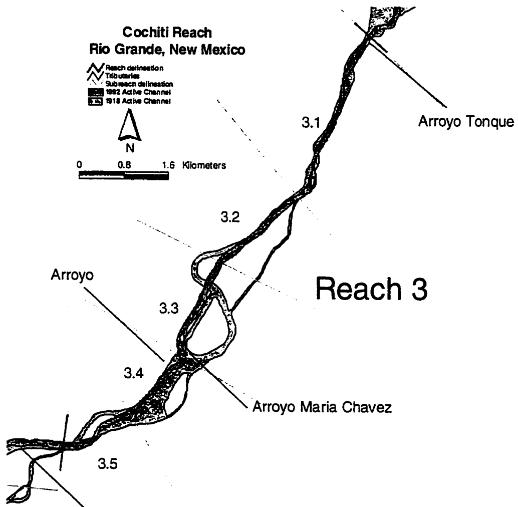
Figure 3-8 - Reach 3 - subreach delineation
