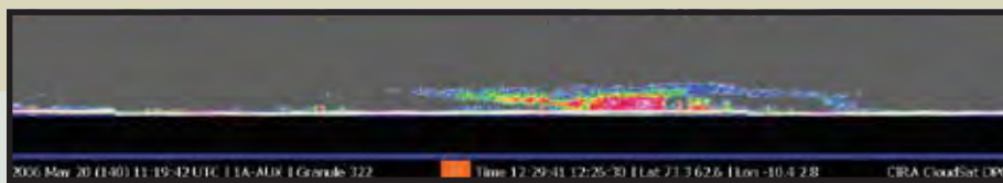
Figure 1. “QuickLook” image of first minutes of CloudSat data, collected at 12:26-12:29 UTC on May 20, 2006. The “data window” (see Figure 2) is approximately 30-km high, and the colors represent radar return echo power (reflectivity), with red being the strongest return (precipitation) and blue the weakest (thin cirrus clouds).
