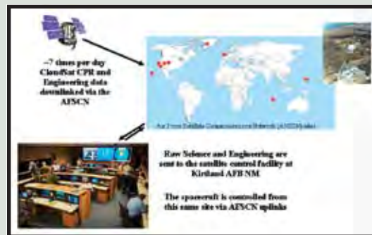
Figure 4. CloudSat data flow – satellite to USAF site at Kirtland AFB.
