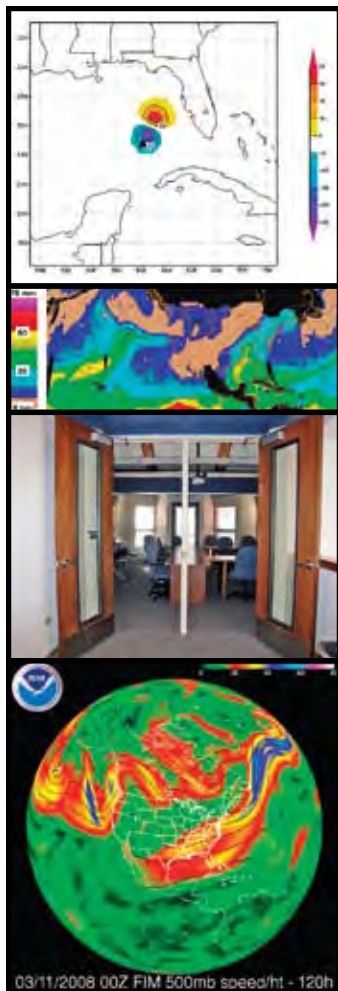
Photos above, from top: Figure 1. Surface pressure forecast difference (hPa) between the experiments with and without data assimilation. Figure 2. The blended TPW AMSU and SSM/I product augmented with GPS data over the CONUS on March 4, 2008. Figure 3. CIRA's Director's Conference Room after the remodel. Figure 4. Wind speed (meter/sec.) at 500mb and geopotential height at 500mb.
