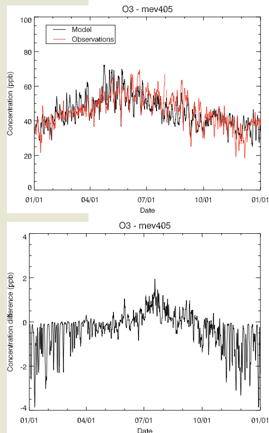
Figure 2a-b. Ozone time series for (a) simulated (black) and observed (red) ozone [ppb, 24 hour average] at Mesa Verde National Park during the 2002 base case simulation, and (b) the change in ozone concentration [ppb, 24 hour average] at this site due solely to VOC and NO x emissions from oil and gas development.
