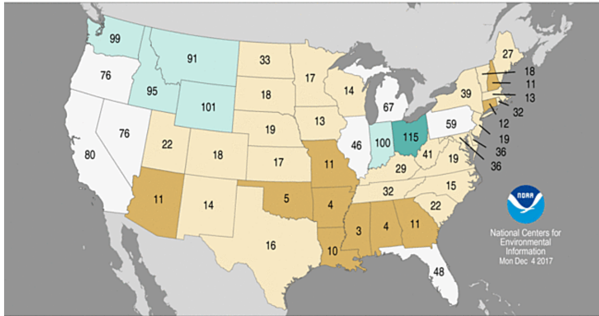
Statewide Precipitation Ranks November 2017 Period: 1895–2017
