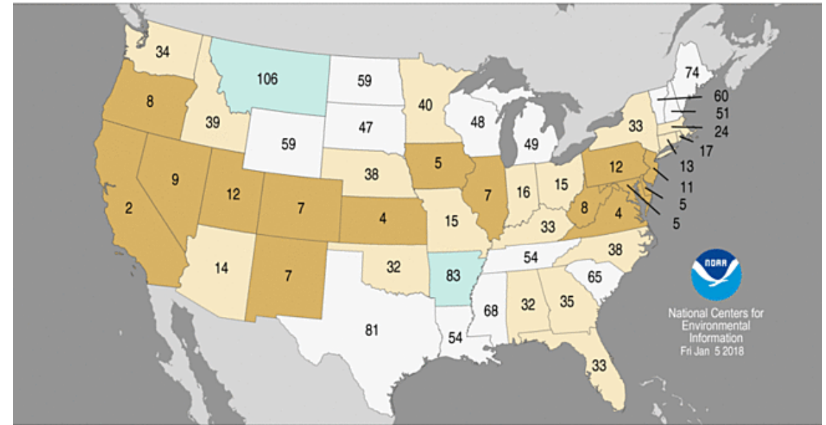
Statewide Precipitation Ranks December 2017 Period: 1895–2017
