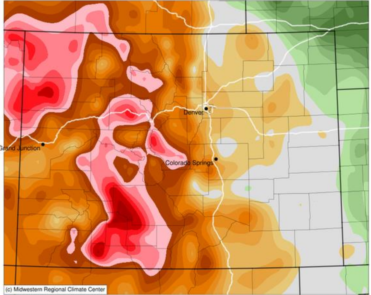
Average Temperature (°F): Departure from 1981-2010 Normals January 01, 2018 to January 16, 2018
