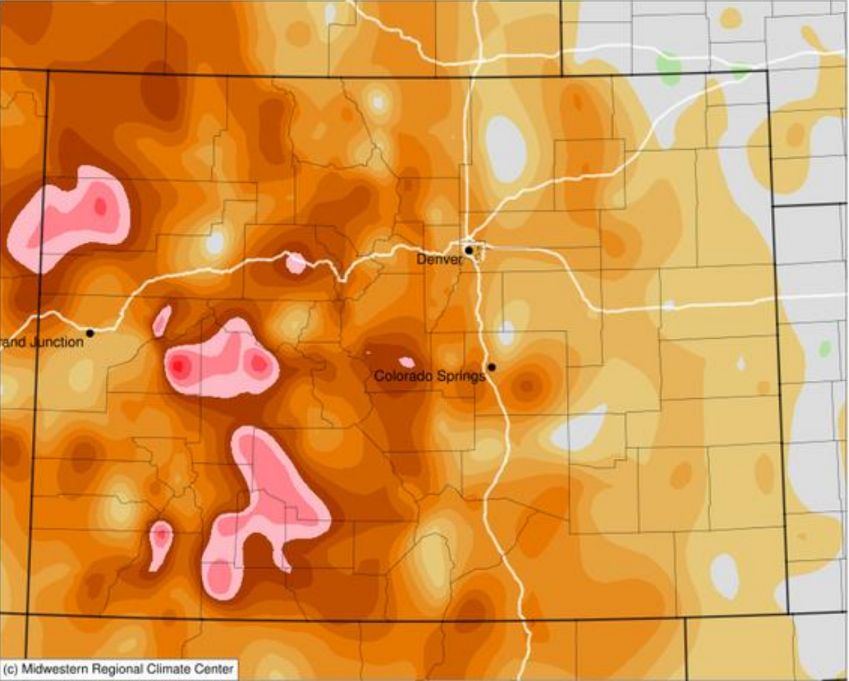
Average Temperature (°F): Departure from 1981-2010 Normals December 01, 2017 to December 31, 2017
