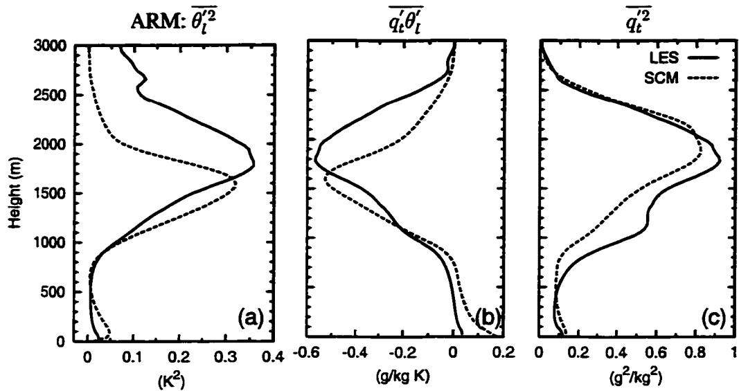
Figure 4.10: Profiles of \overline{\theta_t'^2} (a), \overline{q_t'\theta_t'} (b), and \overline{q_t'^2} (c) averaged between 1900 and 2000 UTC of the ARM simulation. Solid lines are LES results and dashed lines SCM outputs.
