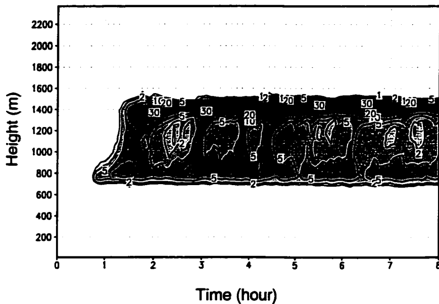
Figure 2.12: Time evolution of the LES cloud fraction (%) for ATEX.
