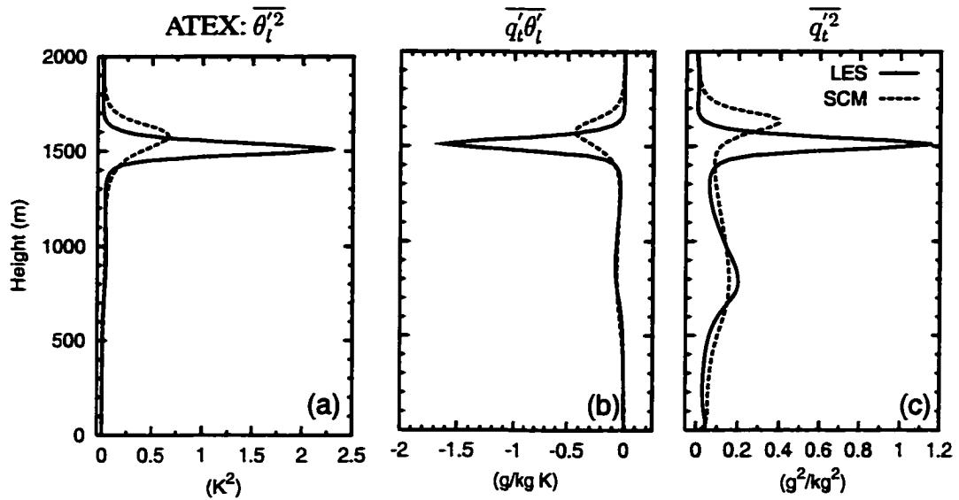
Figure 4.19: Profiles of \overline{\theta_t'^2} (a), \overline{q_t' \theta_t'} (b), and \overline{q_t'^2} (c) averaged over the last five hours of the ATEX simulation. Solid lines are LES results and dashed lines SCM outputs.
