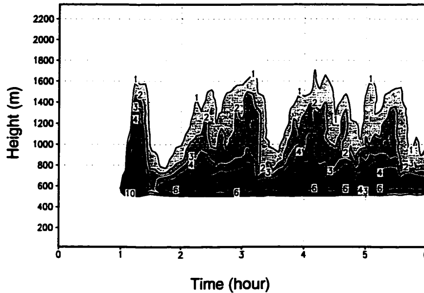
Figure 2.5: Time evolution of the LES cloud fraction (%) for BOMEX.
