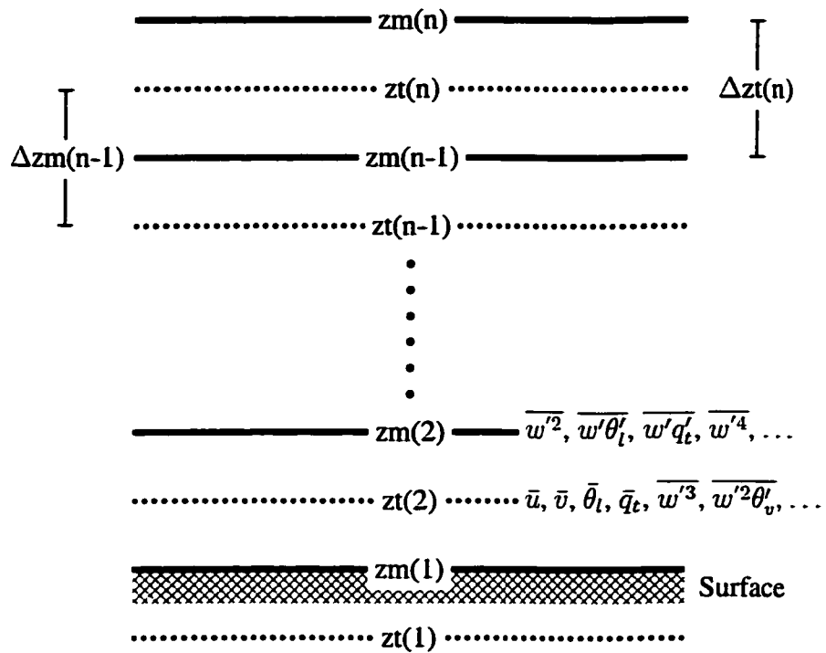
Figure 3.5: Model grid setup. The surface is located at the z_m(1) level. First- and third-order moments reside on z_t levels, and second- and fourth-order moments on z_m levels.
