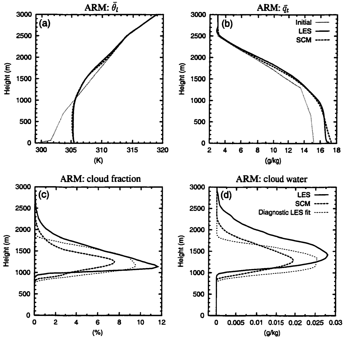
Figure 4.8: Mean profiles of liquid water potential temperature (a), total water specific humidity (b), cloud fraction (c), and liquid water (d) for the ARM case. Thick solid lines LES results and thick dashed line SCM results, both averaged between 1900 and 2000 UTC. Thin dotted lines in panels (a) and (b) represent initial profiles; thin dashed lines in (c) and (d) show cloud properties obtained using a diagnostic PDF fit to the LES data.
