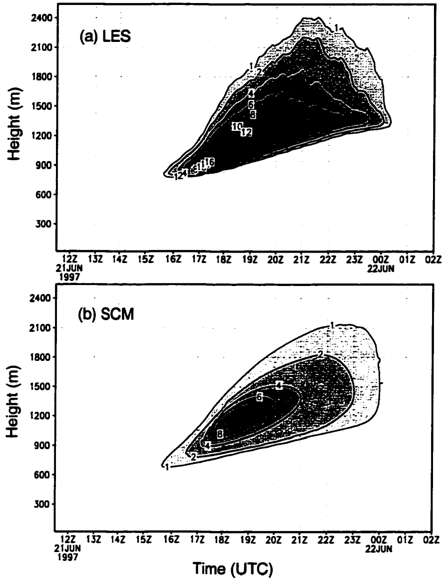
Figure 4.7: Time evolution of the cloud fraction (%) produced by the LES (a) and the SCM (b) for the ARM case. A 60 minutes running average has been applied to the LES cloud fraction to smooth out intermittency.
