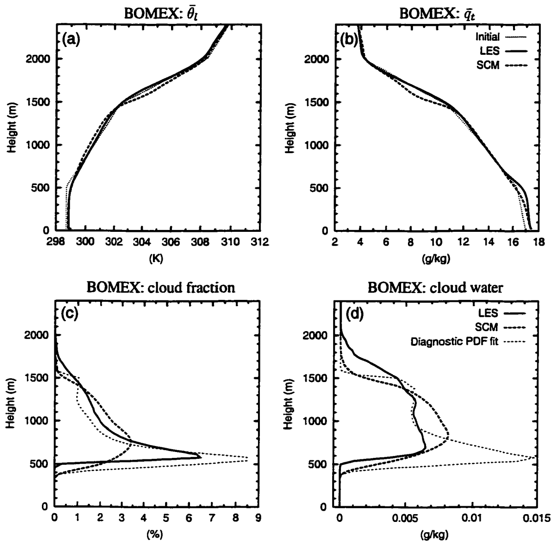
Figure 4.3: Mean profiles of liquid water potential temperature (a), total water specific humidity (b), cloud fraction (c), and liquid water (d) for BOMEX. Thick solid lines represent LES results and thick dashed line SCM results, both averaged over the last three hours of the simulation. Thin dotted lines in panels (a) and (b) represent initial profiles; thin dashed lines in (c) and (d) show cloud properties obtained using a diagnostic PDF fit to the LES data.
