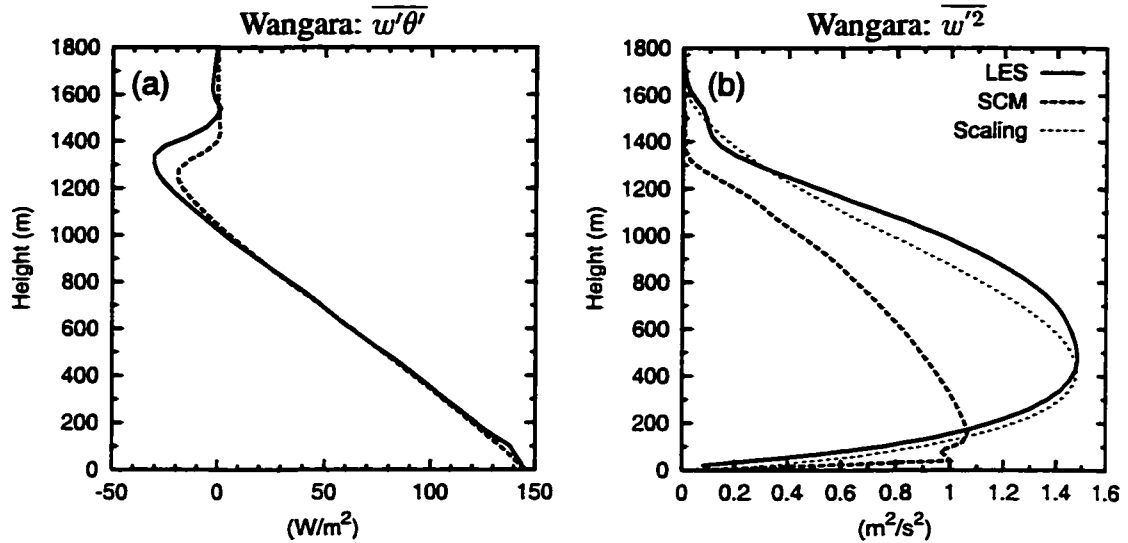
Figure 4.2: Comparison of heat flux (a) and vertical velocity variance (b) between the LES and the SCM; averaged between 1400 and 1500 LST of the Wangara day 33 experiment. LES results are shown in thick solid lines, and SCM in thick dashed lines. The thin dashed line in (b) is the mixed layer scaling proposed by Lenschow et al. (1980).
