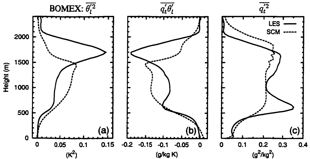
Figure 4.5: Profiles of \overline{\theta_i'^2} (a), \overline{q_i'\theta_i'} (b) and \overline{q_i'^2} (c) averaged over the last three hours of the BOMEX simulation. Solid lines are LES results and dashed lines SCM outputs.
