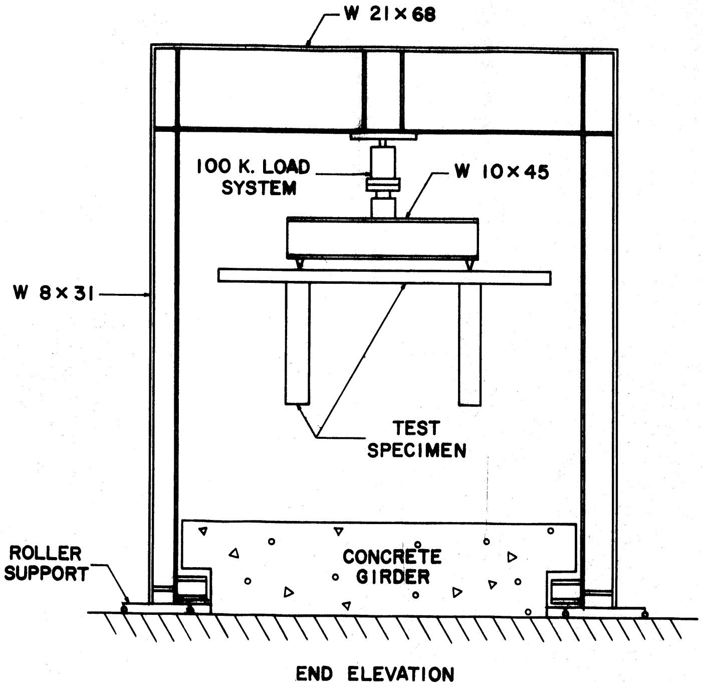
Figure 4. End View of Test Frame Arrangement
