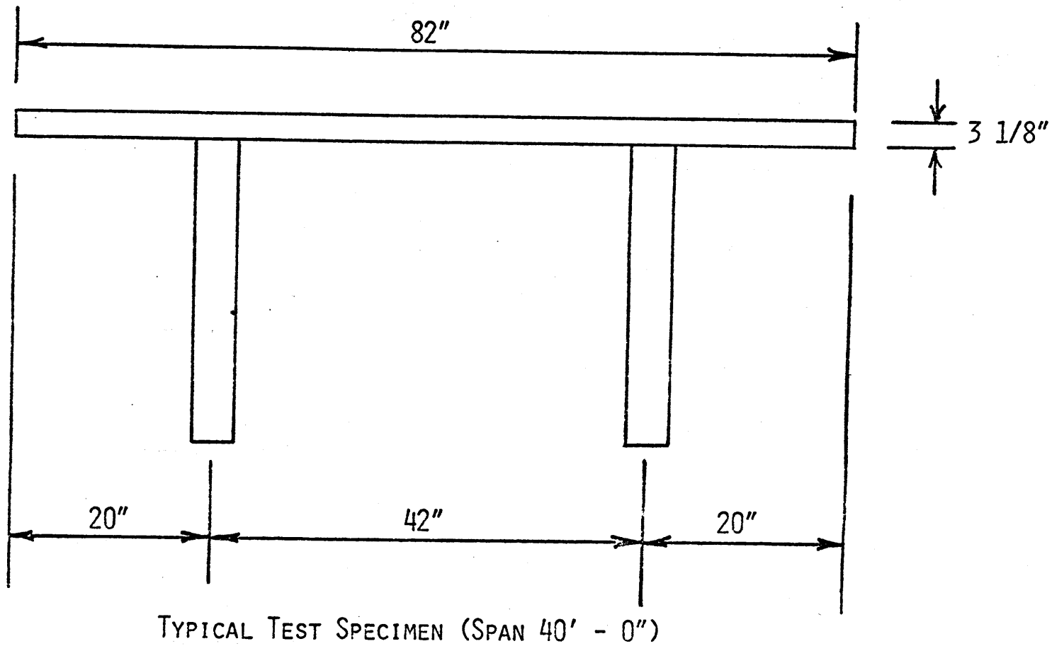
Figure 2. Twin T-Beam Cross-Section
