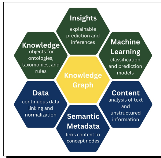
Figure 2.41: KG concepts.
