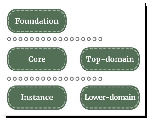
Figure 2.13: Ontological layers [57].
