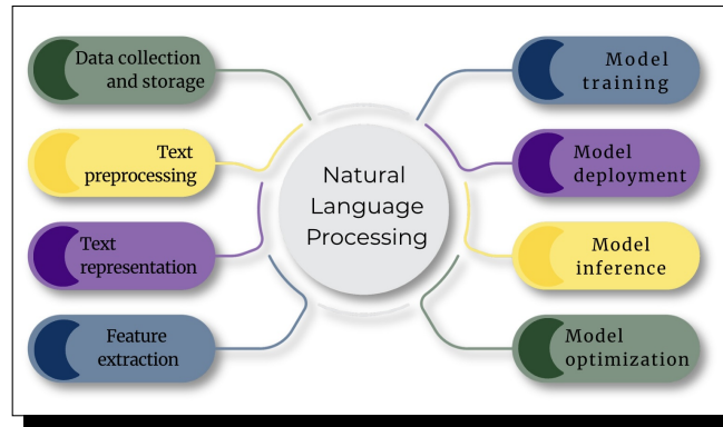
Figure 2.30: NLP processes.
