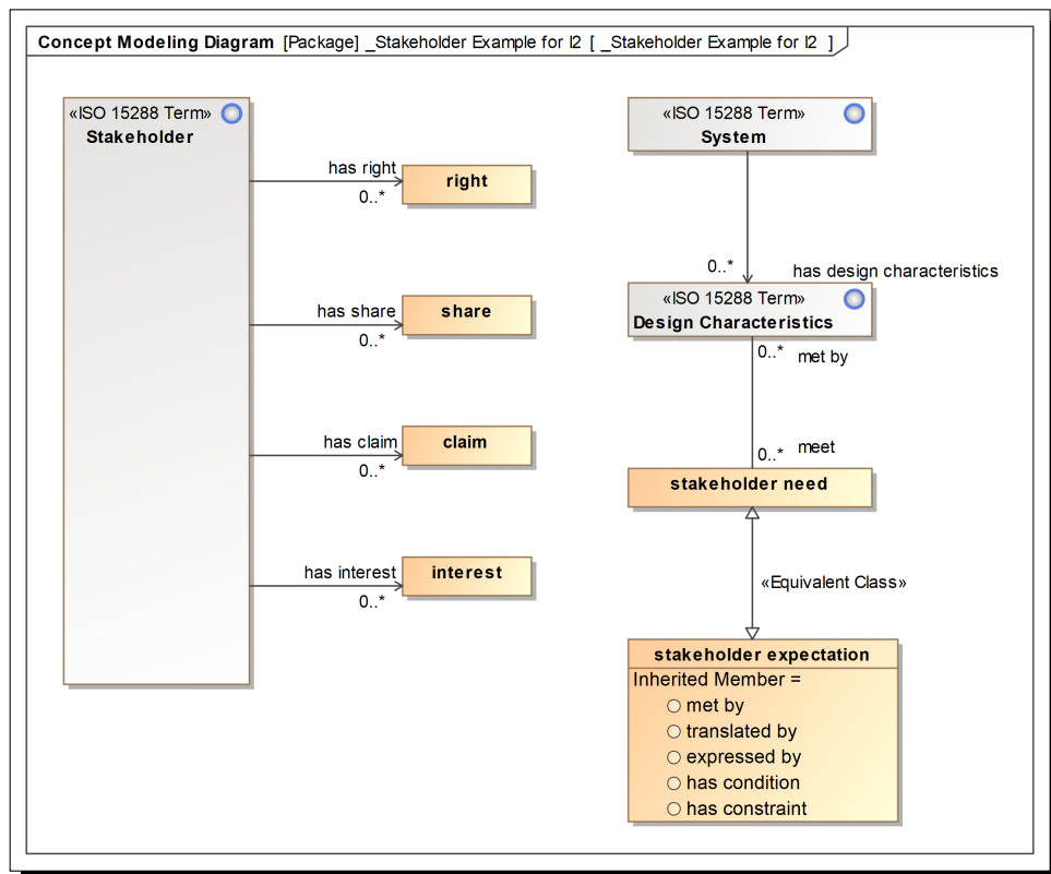
Figure 4.9: ISO 15288 ontology “Stakeholder” class within a concept modeling diagram.
