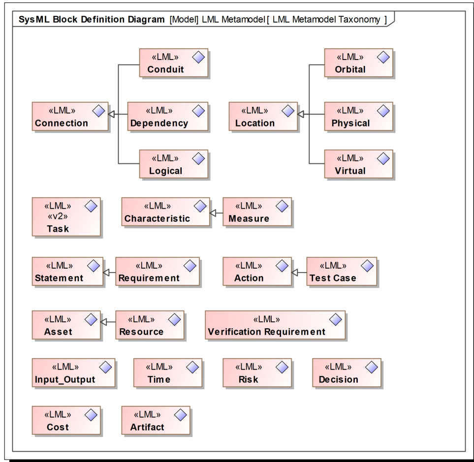
Figure 3.34: LML v2.0 metamodel taxonomy leveraging the generalization relationship.
