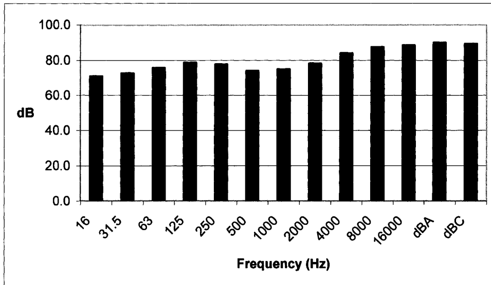
Figure 8: Graph of Gas Metal Arc Welding (GMAW) Octave Band Spectrum.
