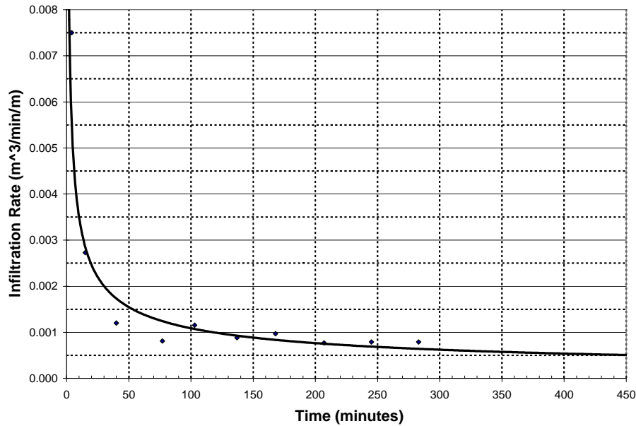
Figure 2: Time vs. Infiltration Rate
