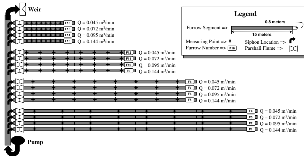
Figure 1. Schematic of the Experimental Area
