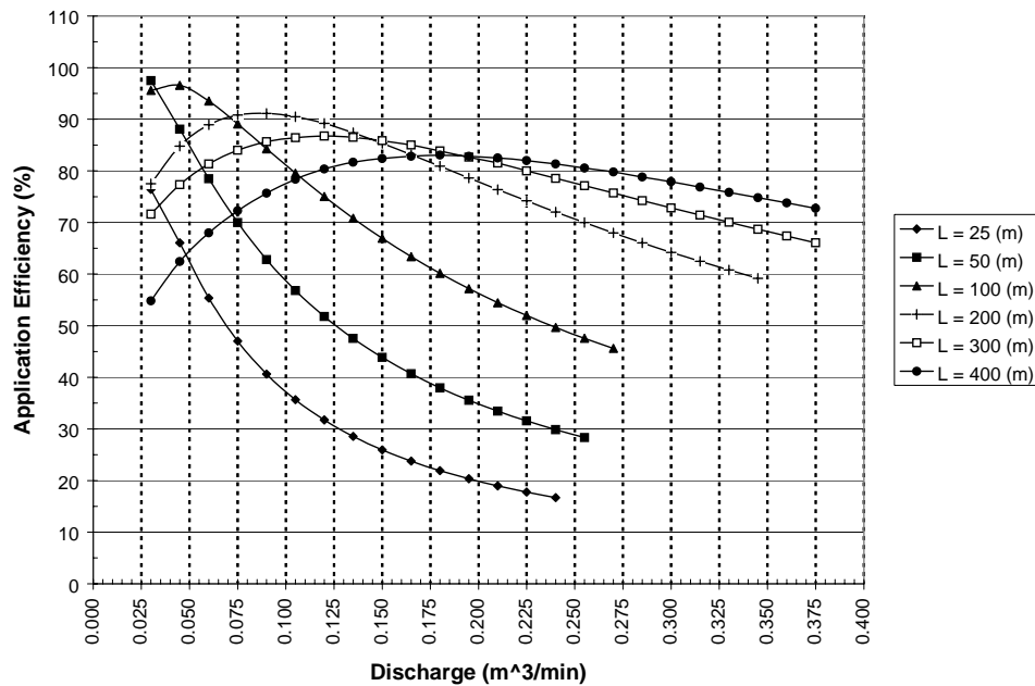
Figure 4: Furrow Discharge vs. Application Efficiency for Modeled Lengths
