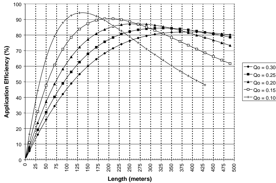
Figure 3: Furrow Lengths vs. Application Efficiency for Modeled Discharges
