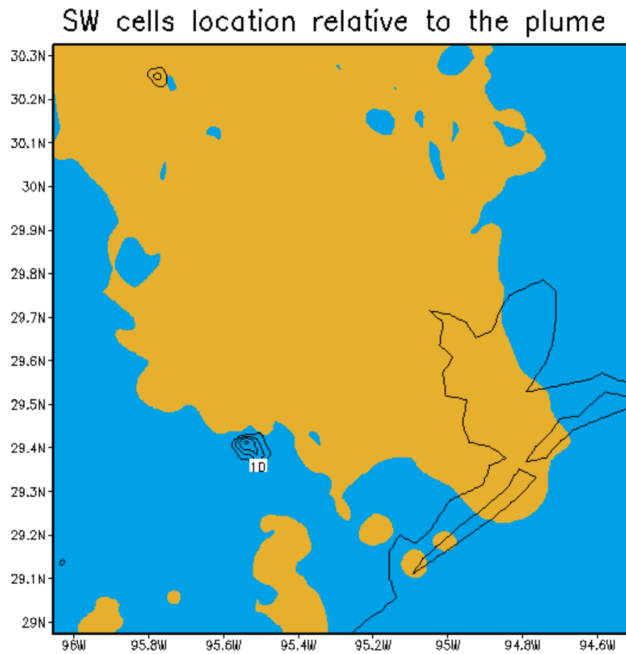
Figure 3. Shaded area Represents the Aerosol Plume One Hour Before the Convective Activity. The Contours Indicate the Position of the SW Cells.
