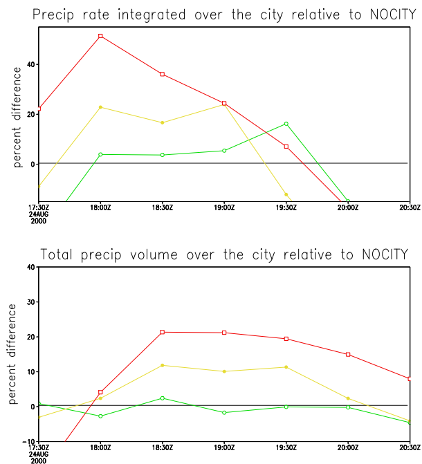
Figure 5. Idem Figure 4 but for Urban Cells.
