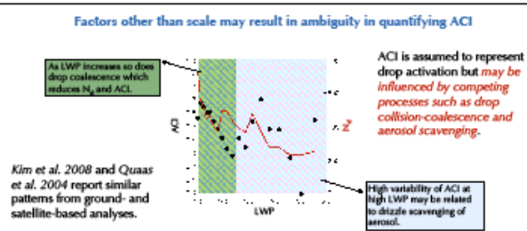
Fig. 1. DOE/ARM Conference Poster Presentation on an Improved Understanding of the Cloud Albedo Effect
