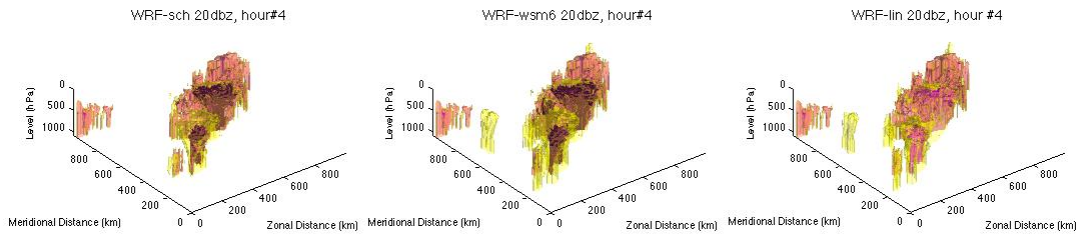
Figure 1: 3D contingency tables (model/observation “yes” or “no” occurrence in each spatial point ) in radar reflectivity field for threshold of 20 dbz, for three model simulations using different cloud microphysics parameterizations at verification time 04 UTC June 13 2004 within model domain (model domain is depicted in next figures). White color indicates no/no (model/observation), black yes/yes, yellow (no/yes) and pink yes/no. Version of the precipitation microphysical parameterization is indicated in the panel title.
