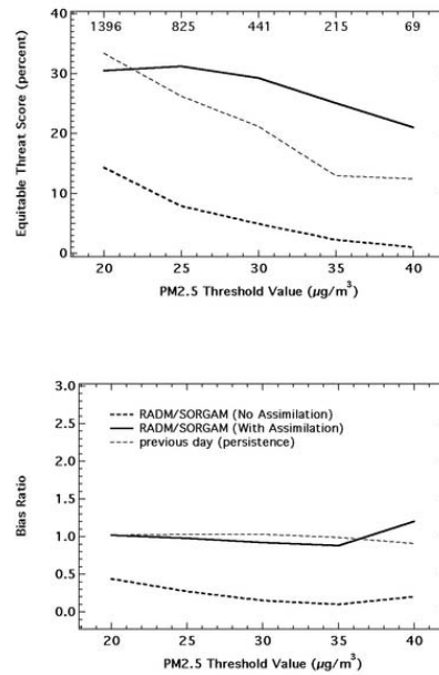
Fig. 7. Equitable Threat Score and Bias Ratio for Different Thresholds of the 24-hour Average PM 2.5 Concentration for Non-assimilated and Assimilated Forecasts.
