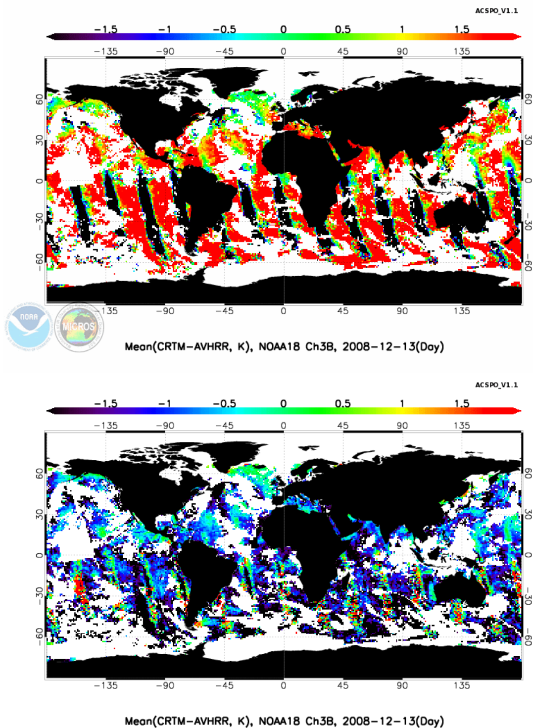
Figure 1. Global geophysical distribution of M-O bias in NOAA18 Ch3B in daytime of Dec. 13, 2008. Upper panel: solar reflectance model used in current CRTM version; bottom panel: Cox-Munk model was used in CRTM.
