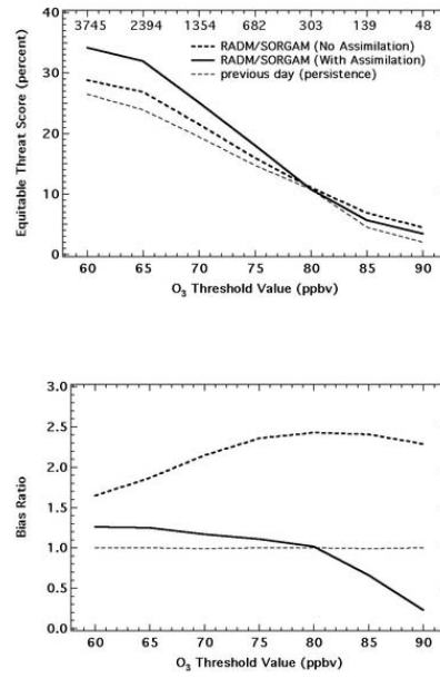
Fig. 6. Equitable Threat Score and Bias Ratio for Different Thresholds of the Next-day 8-hour Average Maximum Ozone Concentration for Non-assimilated and Assimilated Forecasts.
