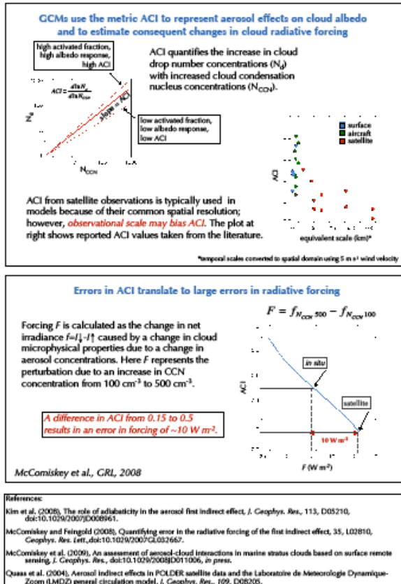
Fig. 1. DOE/ARM Conference Poster Presentation on an Improved Understanding of the Cloud Albedo Effect
