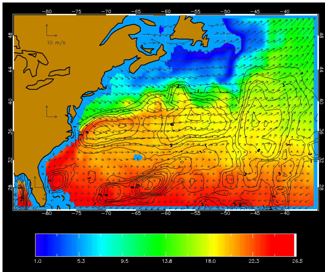
Figure 1. January 2007 monthly mean of sea surface temperature (color fill, deg C), lightning density (strikes/km 2 -year, black contours), and ocean surface winds (vectors) from QuikSCAT.
