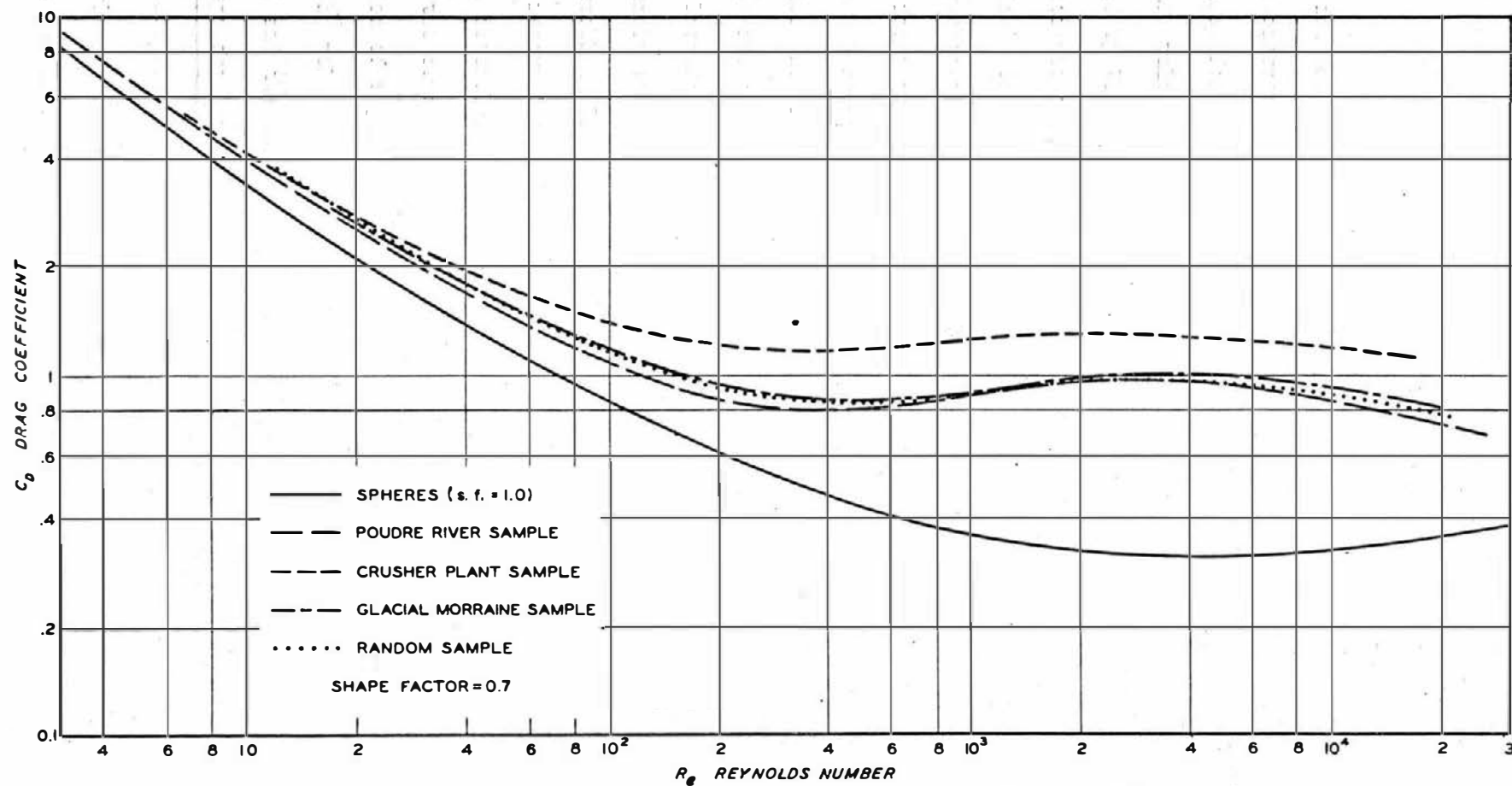
COMPARISON OF RESISTANCE CURVES OF SAMPLES STUDIED BY WILDE (FROM REF. 41)
