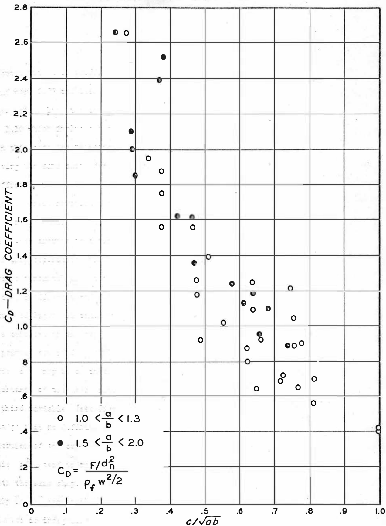
EFFECT OF PARTICLE LENGTH ON C_D FROM REF. 41
