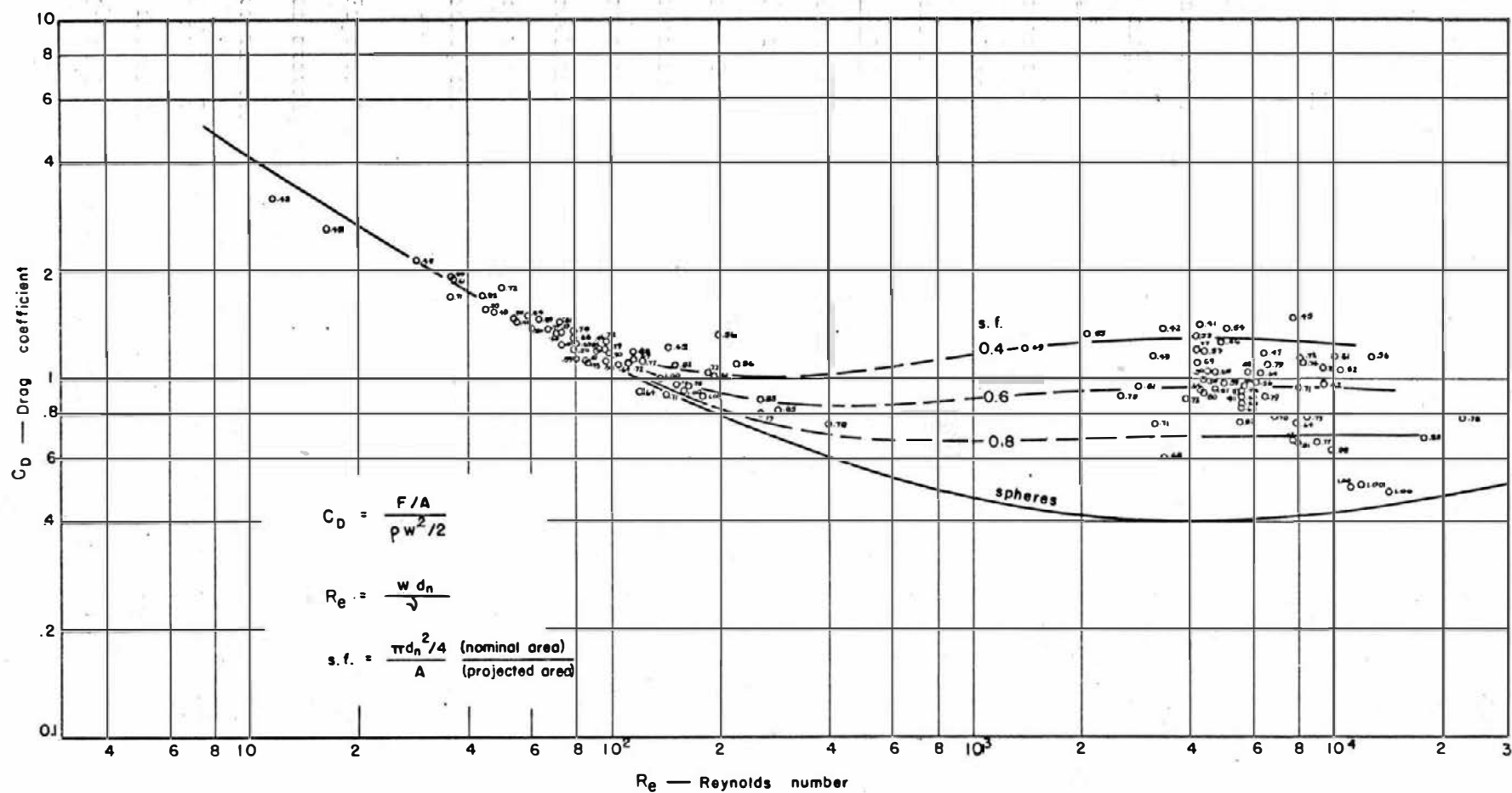
INFLUENCE OF SHAPE ON DRAG COEFFICIENT FOR RANDOM SAMPLE (FROM REF. 41)
