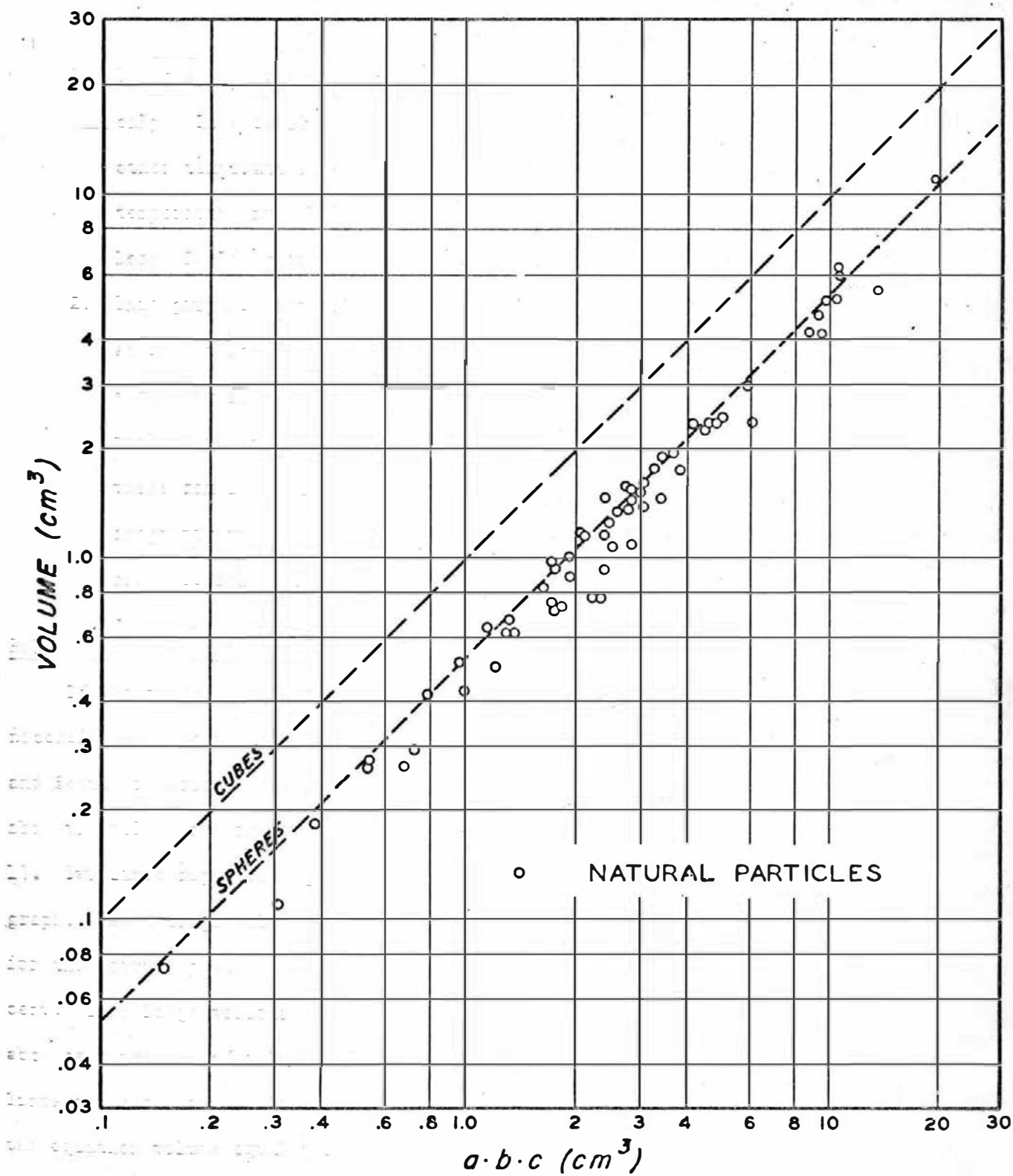
PARTICLE VOLUME AS A FUNCTION OF a \cdot b \cdot c
