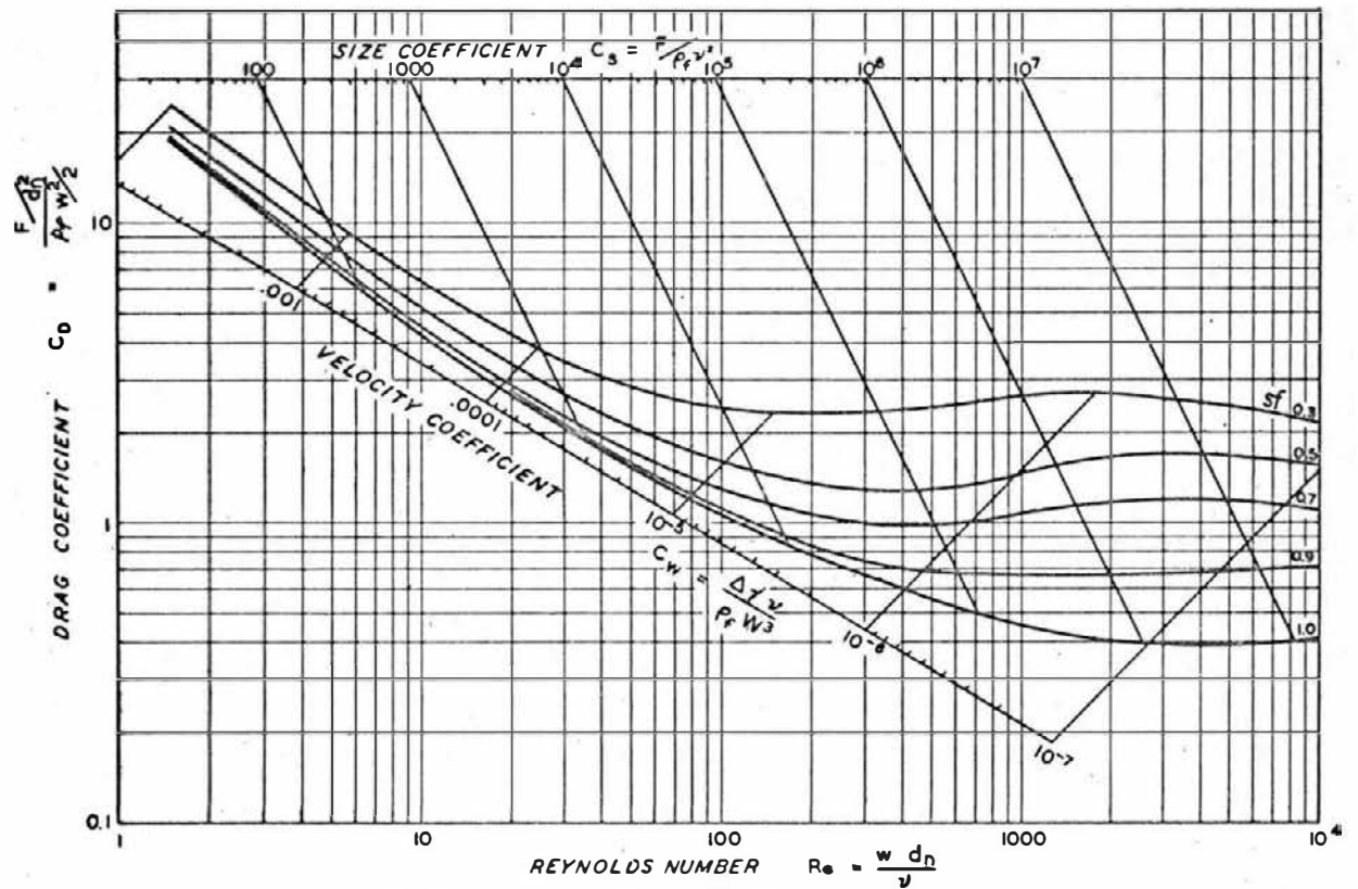
(a) C_D:Re GRAPH FOR NATURALLY WORN SEDIMENTS
