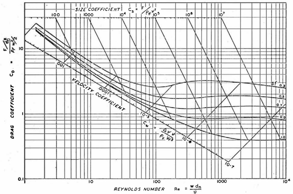
(b) C_D:Re GRAPH FOR CRUSHER FRAGMENTS
