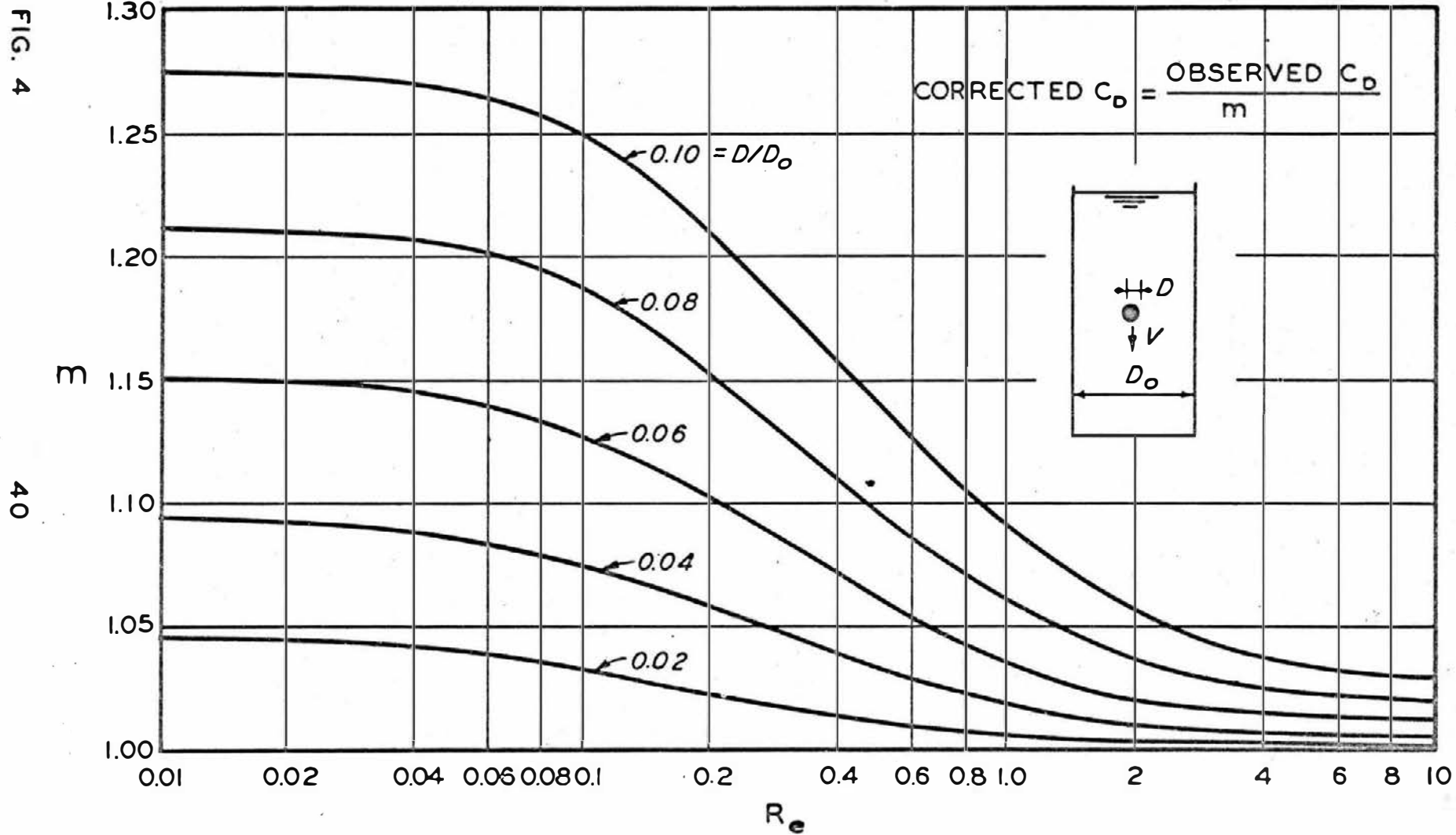
VARIATION OF THE BOUNDARY CORRECTION WITH REYNOLDS NUMBER AFTER McNOWN - REFERENCE 14
