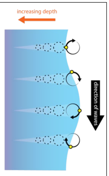
Figure 12. Behavior of water particles in a wave propagating in deep water.
