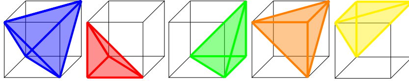
Figure 4: Triangulation of the cube into five tetrahedra. Here, we have the tetrahedra \tau_1, \tau_2, \tau_3, \tau_4 , and \tau_5 , respectively. The lavender tetrahedron, \tau_1 , is the balanced tetrahedron.
