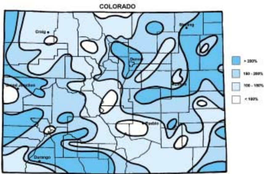
August 1999 precipitation as a percent of 1961-1990 average
