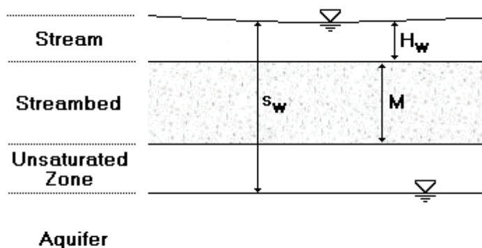
Figure 1. Representation of interaction between a perched stream and underlying alluvial aquifer. H_w =river stage, s_w =drawdown, and M =streambed thickness.
