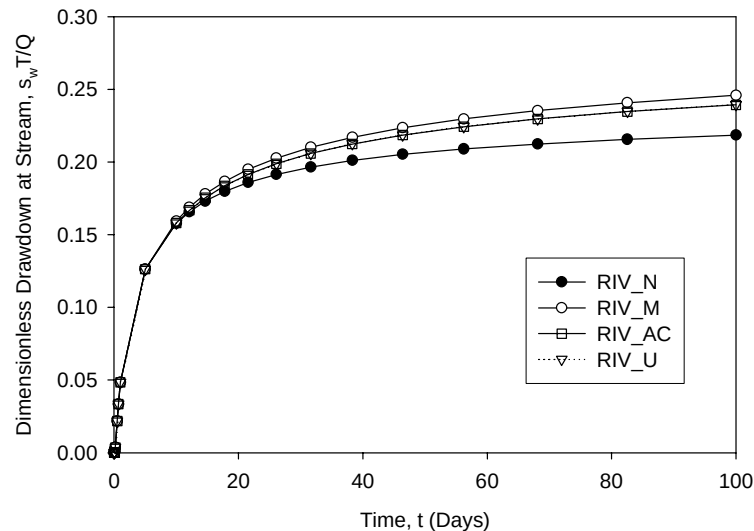
Figure 4. Comparison of dimensionless aquifer drawdown at the stream location nearest the pumping well as predicted by the four different MODFLOW RIVER packages for a fine sand aquifer ( K=50.0 \text{ m-d}^{-1} , h_e=5 \text{ cm} ).
