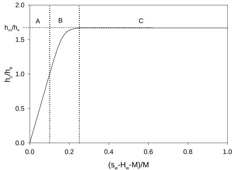
Figure 2. Interface capillary pressure head, h_c , divided by the entry pressure head, h_e , as a functions of water table position for regimes A (saturated flow), B (transition), and C (unsaturated flow). From Fox and Durnford (2003).
