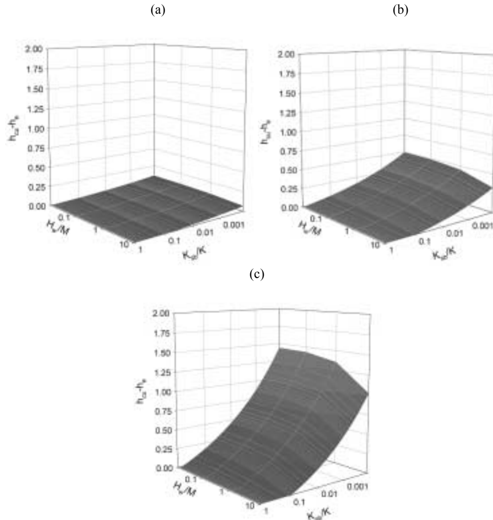
Figure 3. Difference between ultimate, h_{cu} , and entry, h_e , capillary pressure heads as a function of K_{sb}/K and H_w/M for (a) coarse sand ( K=50 \text{ m-d}^{-1} , h_e=5 \text{ cm} ), (b) medium sand ( K=10 \text{ m-d}^{-1} , h_e=20 \text{ cm} ), and (c) fine sand ( K=2.5 \text{ m-d}^{-1} , h_e=50 \text{ cm} ) subsoil with a streambed thickness, M=1 \text{ m} .
