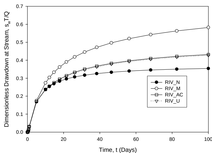
Figure 5. Comparison of dimensionless aquifer drawdown at the stream location nearest the pumping well as predicted by the four different MODFLOW RIVER packages for a fine sand aquifer ( K=5.0 \text{ m-d}^{-1} , h_c=50 \text{ cm} ).
