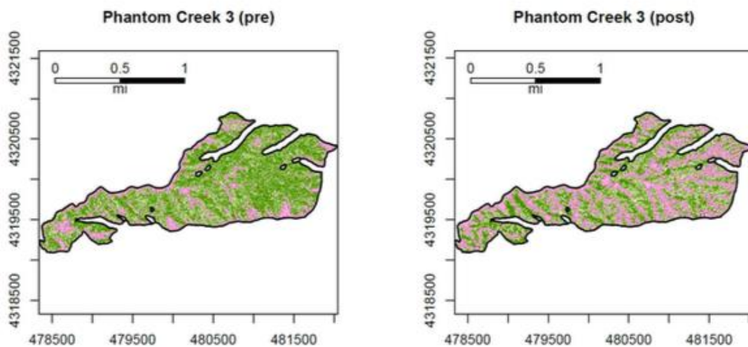
Figure 4. Example of additional spatial heterogeneity monitoring show the increase in large gaps (pink regions) resulting from forest management at Phantom Creek. Literature suggests these types of patterns can increase forest resiliency to disease, insects, wildfire, and climate change, as well as help sustain other ecosystem services such as regeneration, wildlife habitat, and carbon sequestration.
