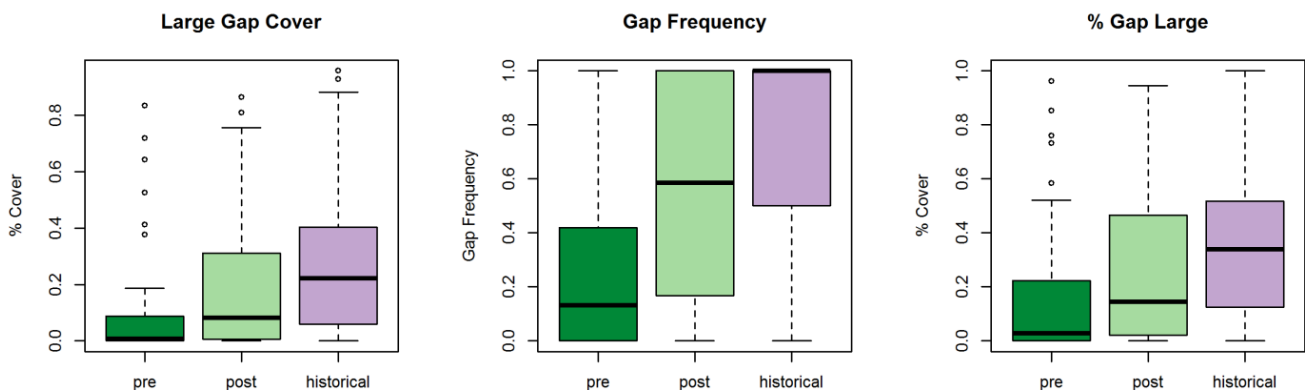
Figure 2. Analysis of 7 early CFLR projects, showing (A) increases in the percent cover of large gaps (>59 ft), (B) the frequency of plots containing large gaps, and (C) the proportion of large gaps relative to the total area of openings following forest management activities relative to reconstructed data. Reconstructed data courtesy of the Front Range Forest Reconstruction Network (Brown, et al. 2015).
