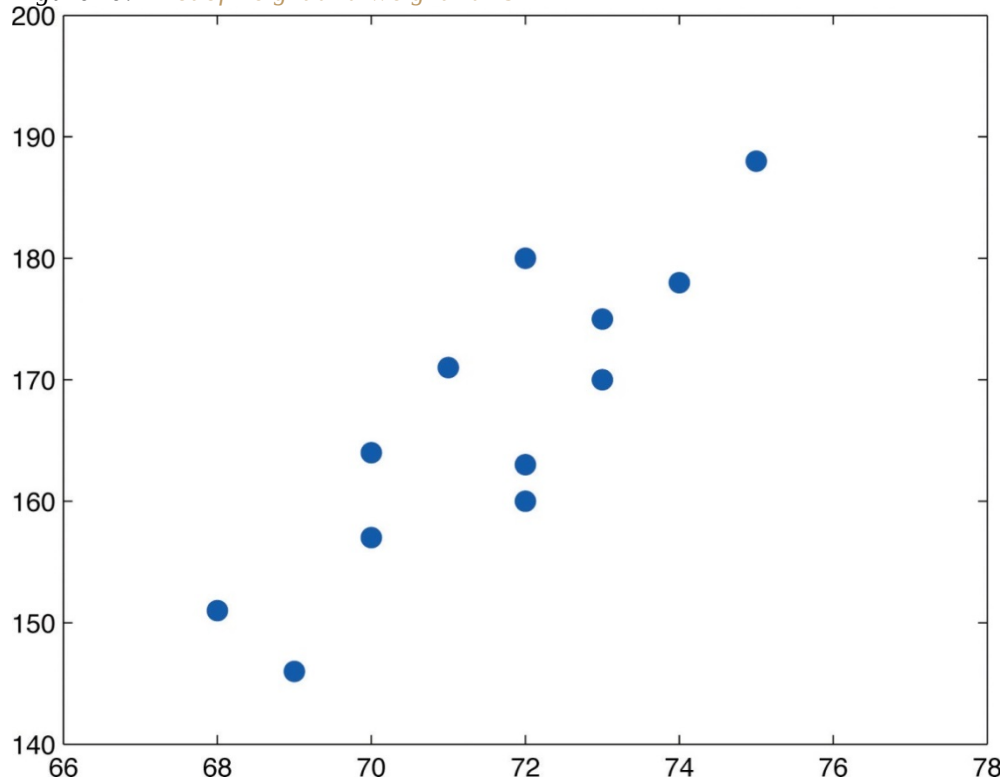
Figure 10.2 Plot of Height and Weight Pairs
