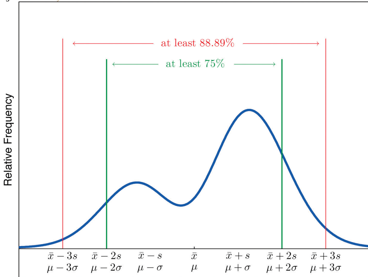
Figure 2.19 Chebyshev's Theorem
