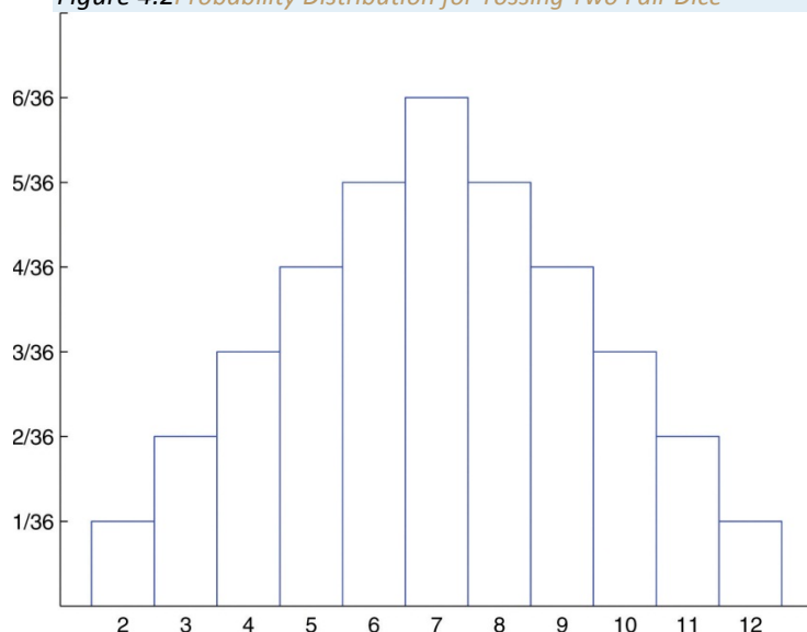
Figure 4.2 Probability Distribution for Tossing Two Fair Dice
