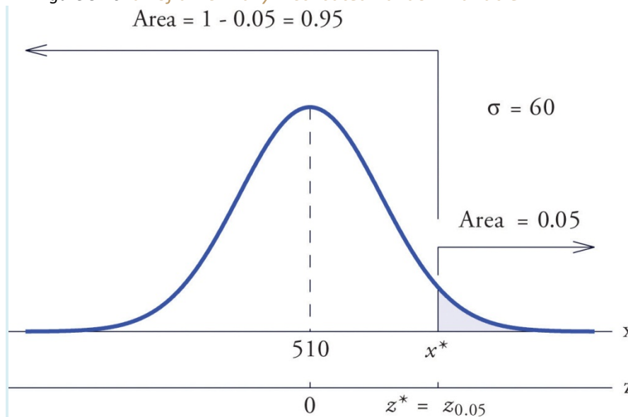
Figure 5.26 Tail of a Normally Distributed Random Variable
