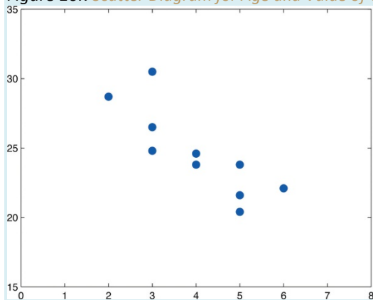
Figure 10.7 Scatter Diagram for Age and Value of Used Automobiles
