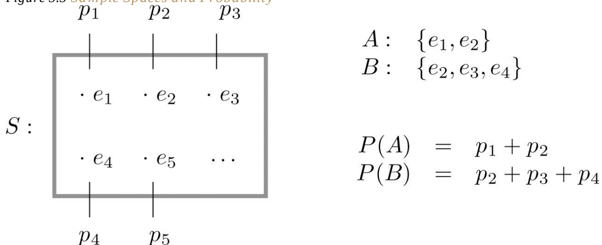
Figure 3.3 Sample Spaces and Probability
