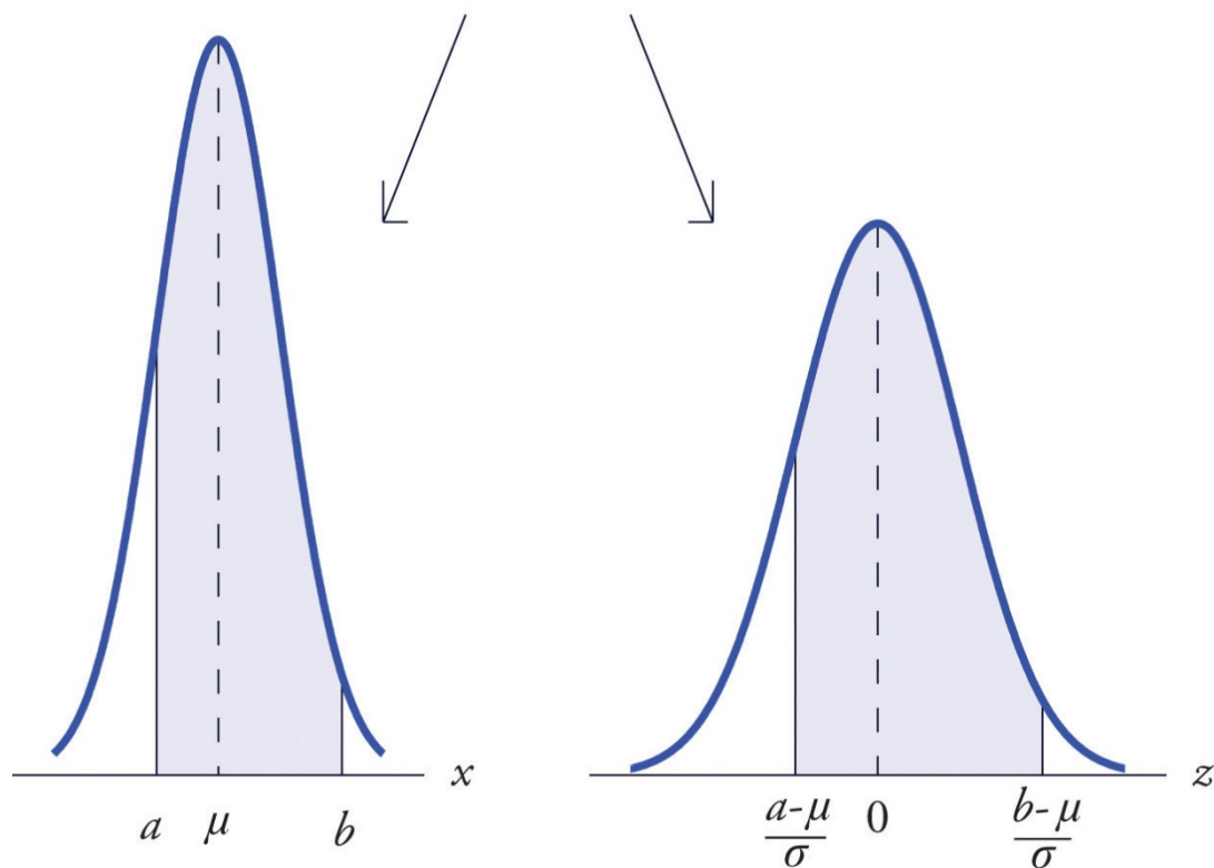
Figure 5.14 Probability for an Interval of Finite Length Same shaded area
