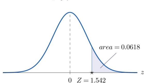
Figure 8.18 P -Value for Note 8.50 "Example 15"
