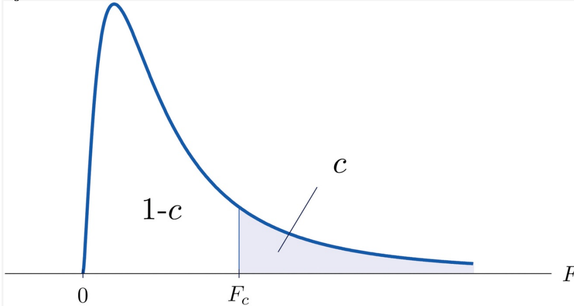
Figure 11.8 F_c Illustrated
