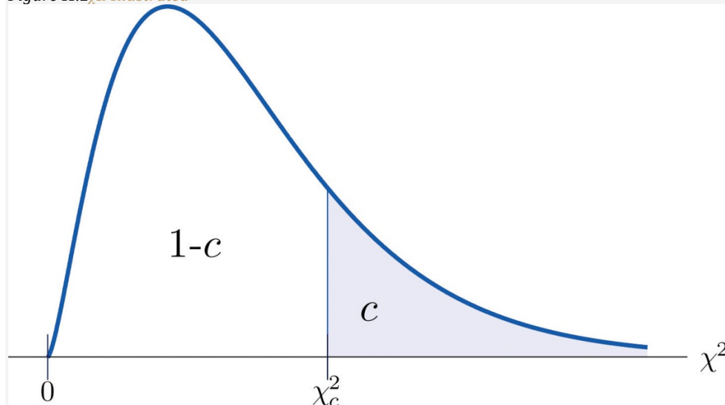
Figure 12.4 "Critical Values of Chi-Square Distributions" gives values of \chi^2_c for various values of c and under several chi-square distributions with various degrees of freedom.
