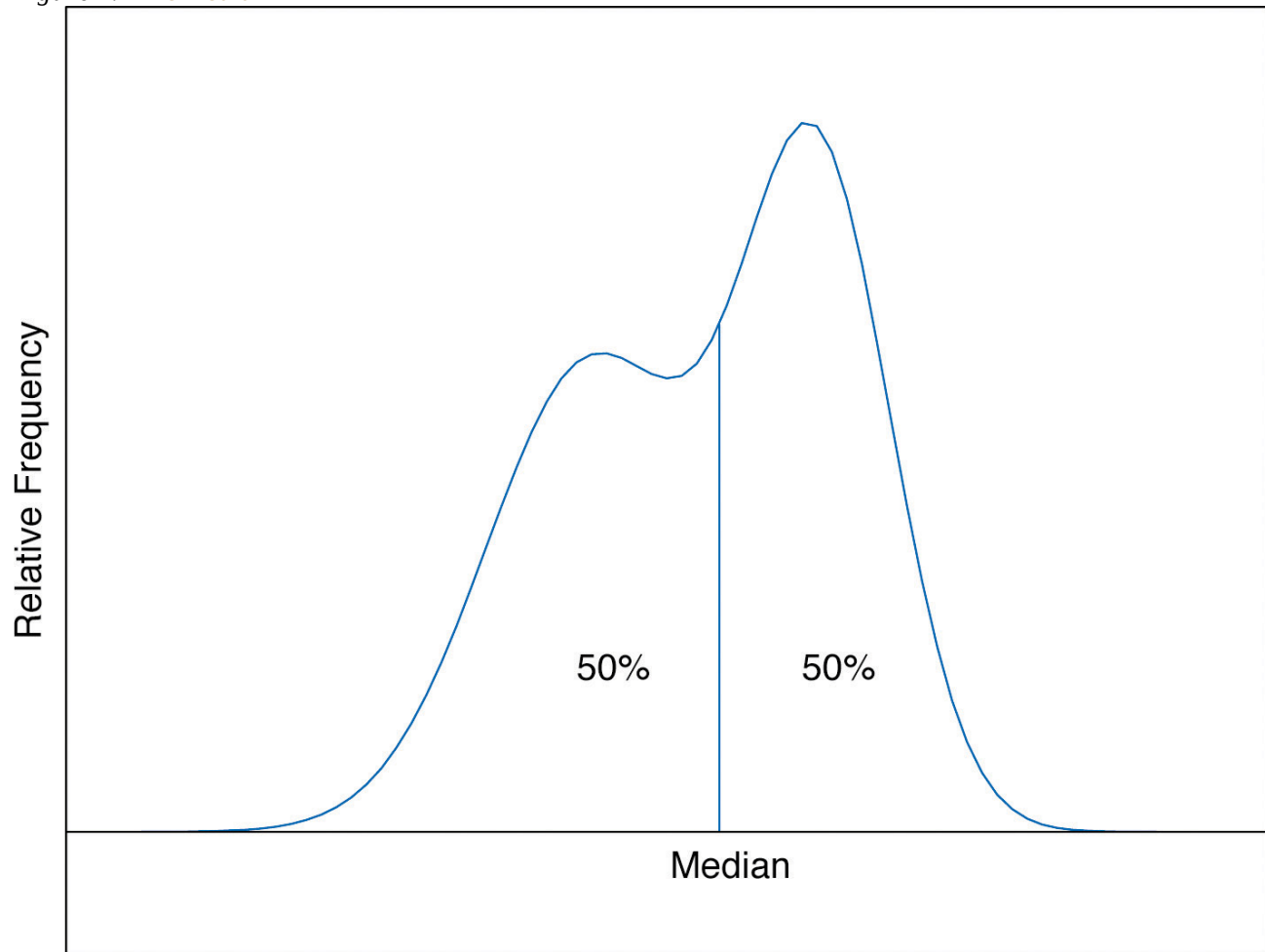
Figure 2.7 The Median
