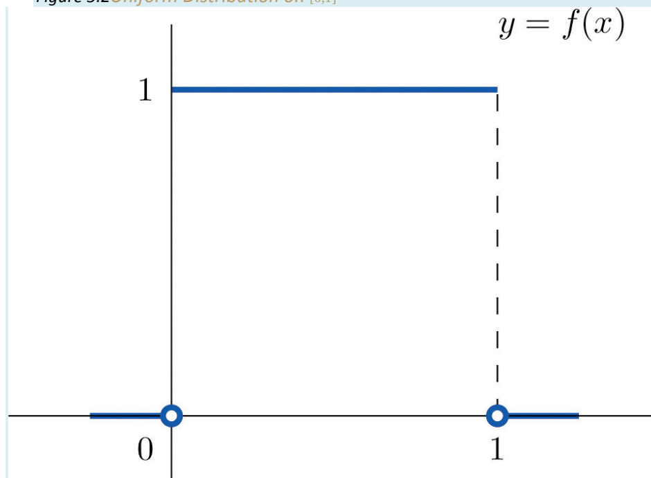
Figure 5.2 Uniform Distribution on [0,1]
