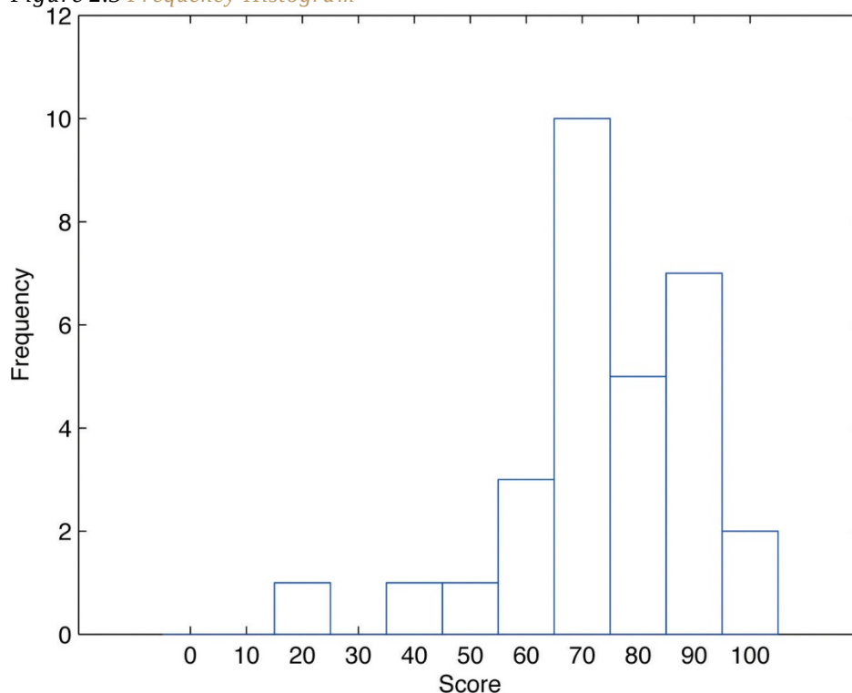
Figure 2.3 Frequency Histogram
