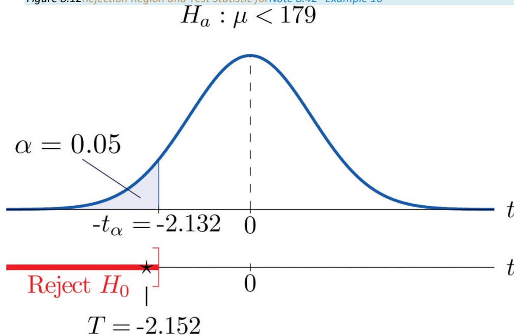
Figure 8.12 Rejection Region and Test Statistic for Note 8.42 "Example 10"
