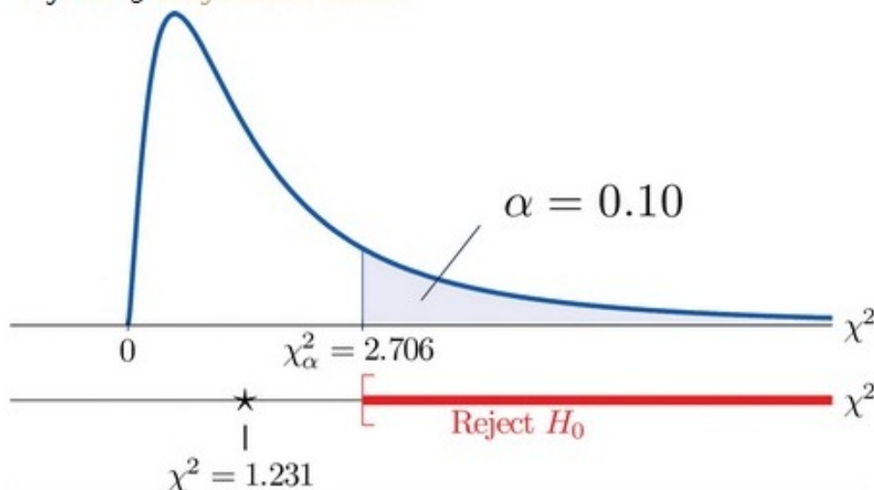
Figure 11.3 Baby Gender Prediction
