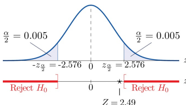
Figure 8.6 Rejection Region and Test Statistic for Note 8.28 "Example 5"
