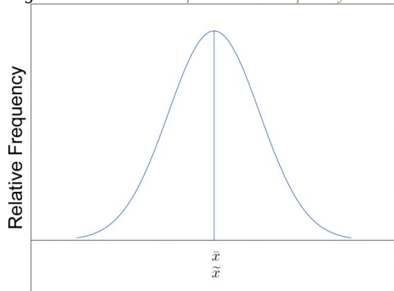
Figure 2.8 Skewness of Relative Frequency Histograms
