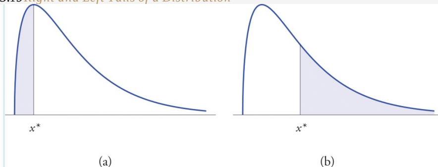
Figure 5.19 Right and Left Tails of a Distribution
