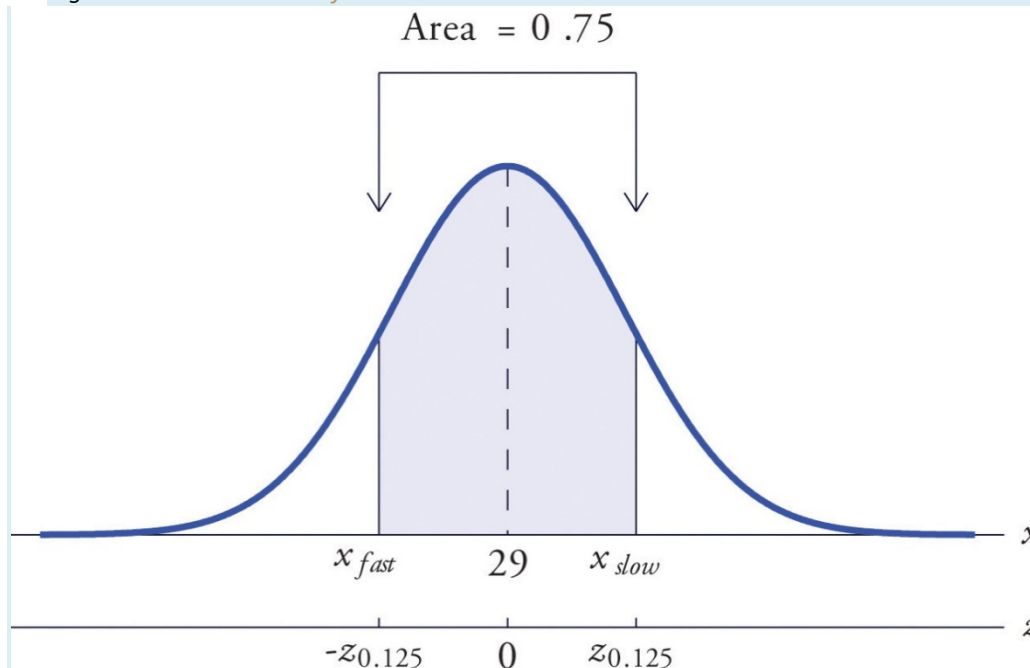
Figure 5.27 Distribution of Times to Run a Course
