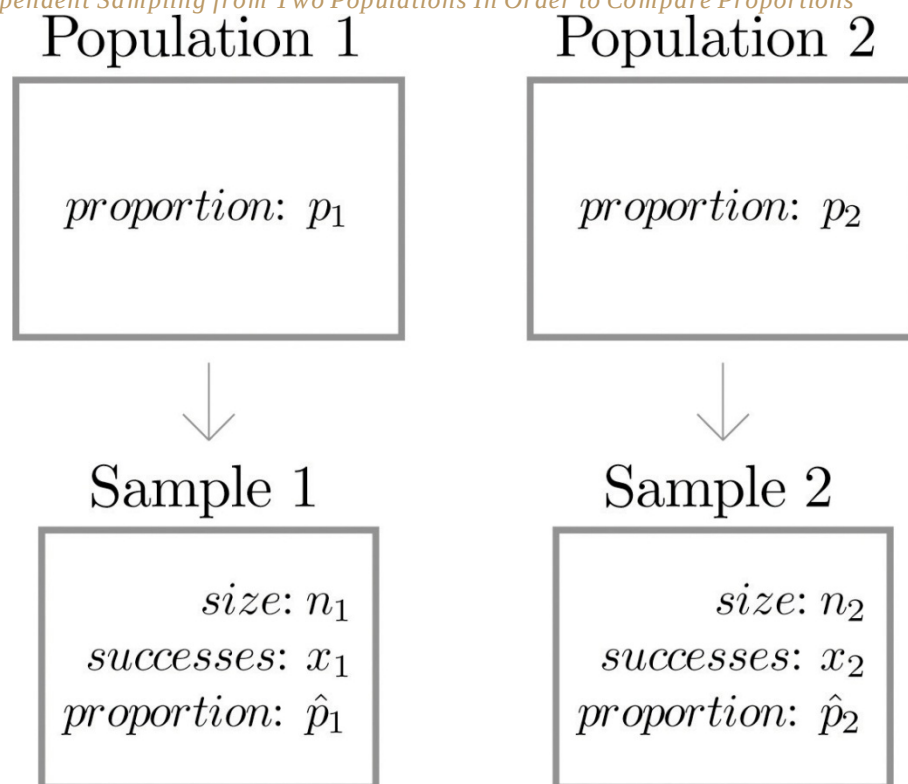
Figure 9.7 Independent Sampling from Two Populations In Order to Compare Proportions
