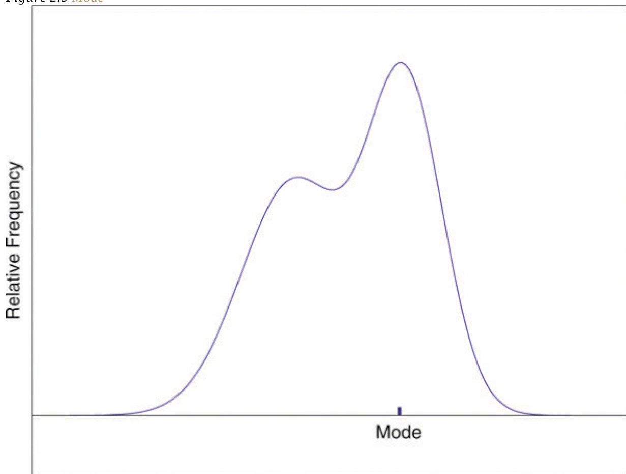
Figure 2.9 Mode
