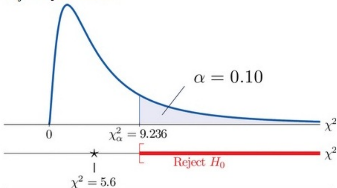
Figure 11.5 Balanced Die
