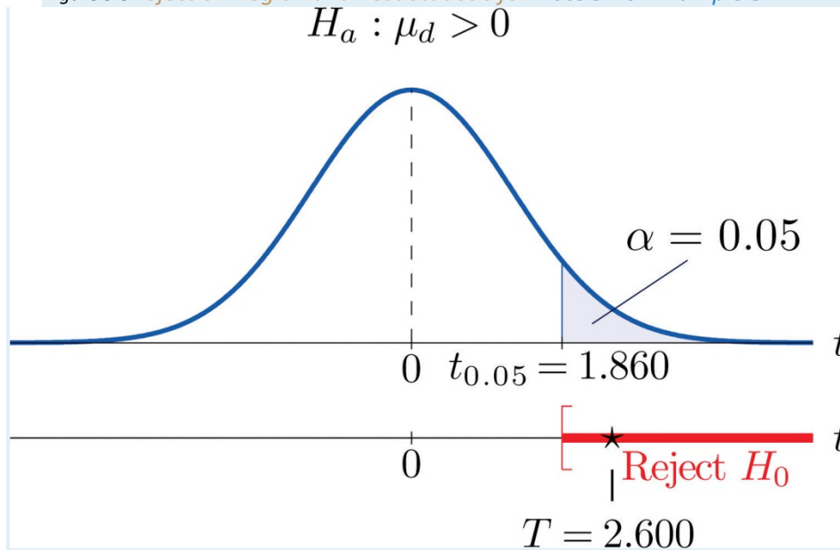
Figure 9.5 Rejection Region and Test Statistic for Note 9.20 "Example 8"
