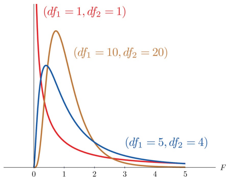
Figure 11.7 Many F -Distributions
