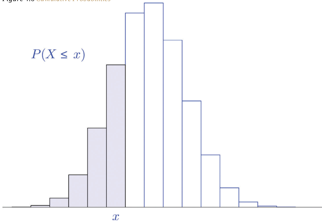
Figure 4.6 Cumulative Probabilities
