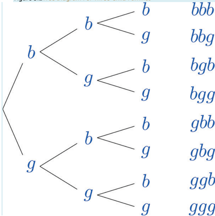
Figure 3.2 Tree Diagram For Three-Child Families
