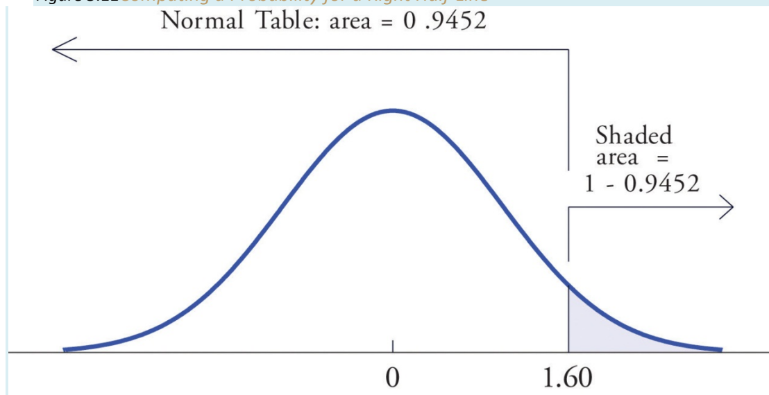
Figure 5.11 Computing a Probability for a Right Half-Line
