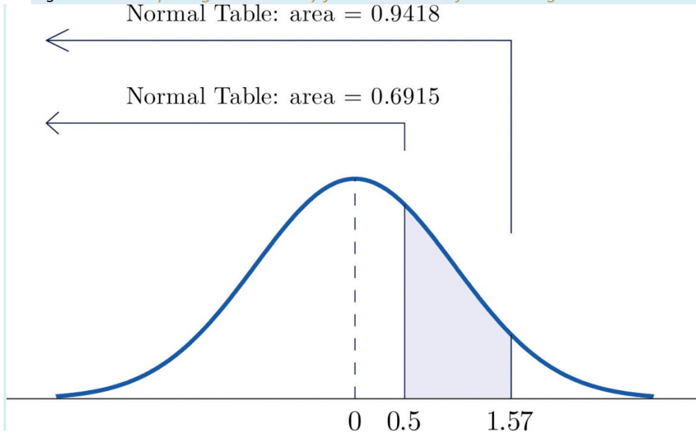
Figure 5.12 Computing a Probability for an Interval of Finite Length
