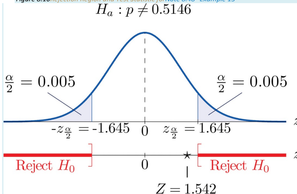
Figure 8.16 Rejection Region and Test Statistic for Note 8.48 "Example 13"
