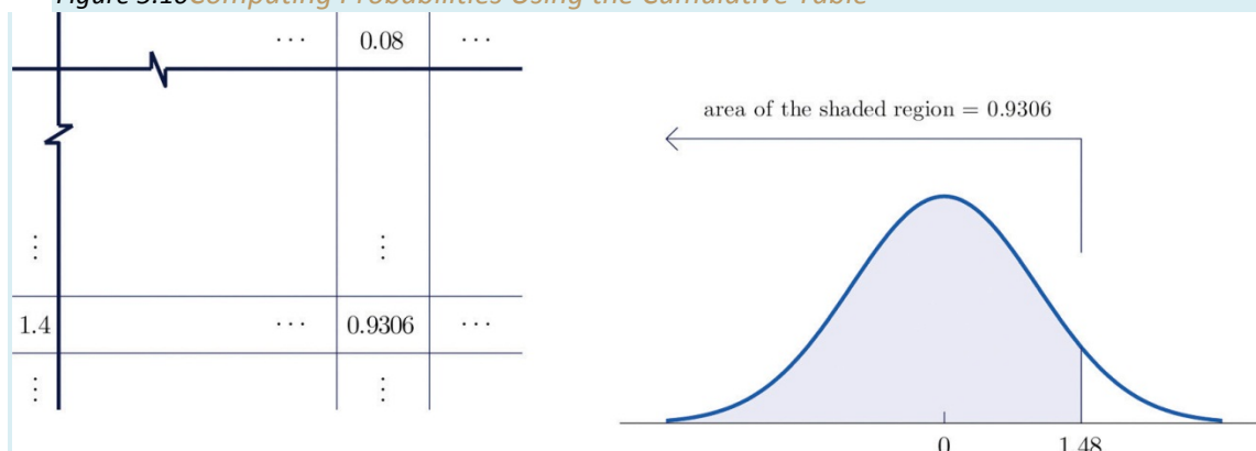
Figure 5.10 Computing Probabilities Using the Cumulative Table
