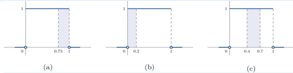
Figure 5.3 Probabilities from the Uniform Distribution on [0,1]
