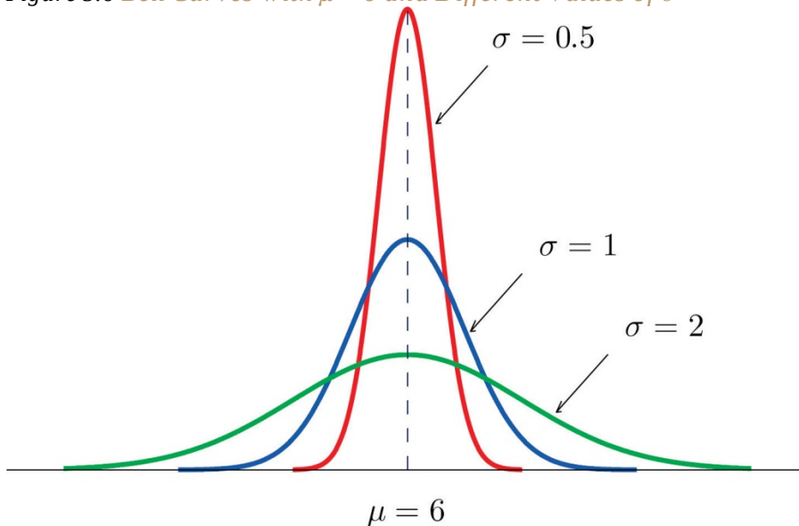
Figure 5.6 Bell Curves with \mu = 6 and Different Values of \sigma
