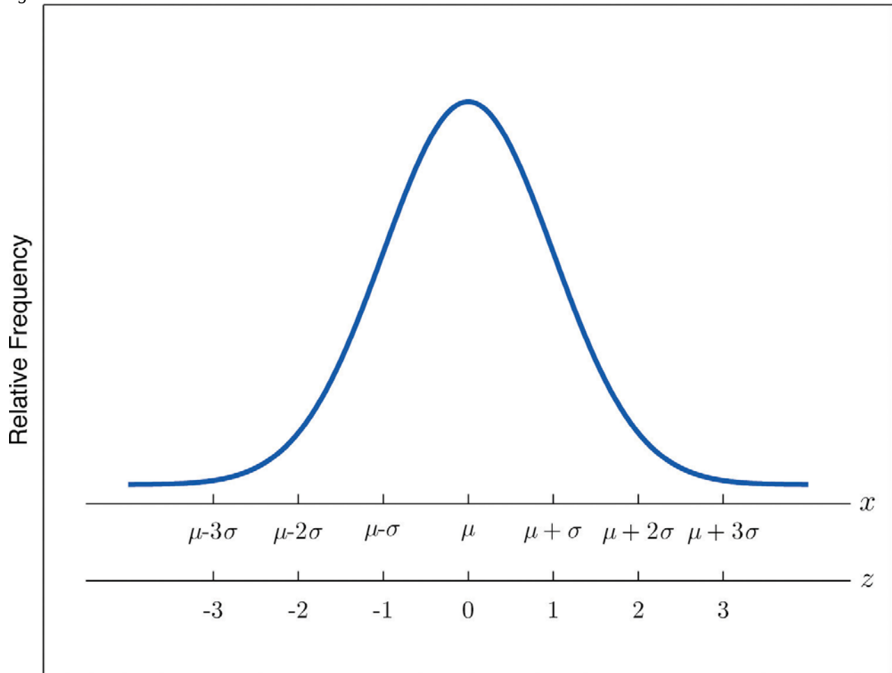
Figure 2.14 x -Scale versus z -Score
