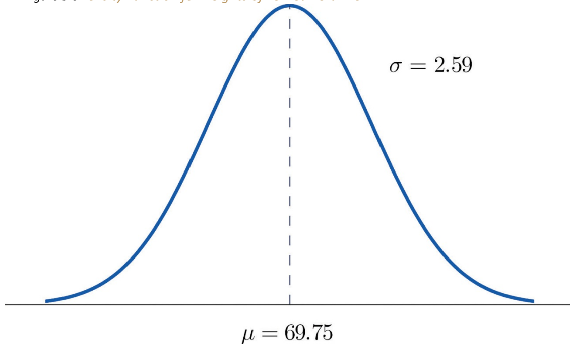
Figure 5.8 Density Function for Heights of 25-Year-Old Men
