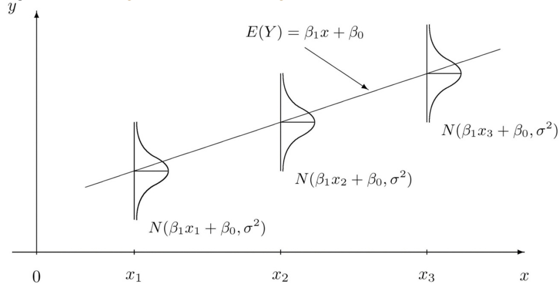
Figure 10.5 The Simple Linear Model Concept
