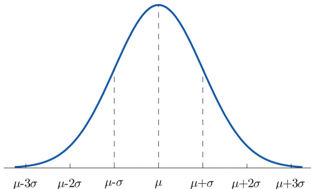
Figure 5.7 Density Function for a Normally Distributed Random Variable with Mean \mu and Standard Deviation \sigma
