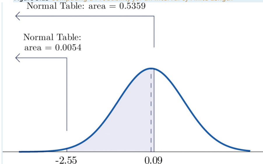
Figure 5.13 Computing a Probability for an Interval of Finite Length
