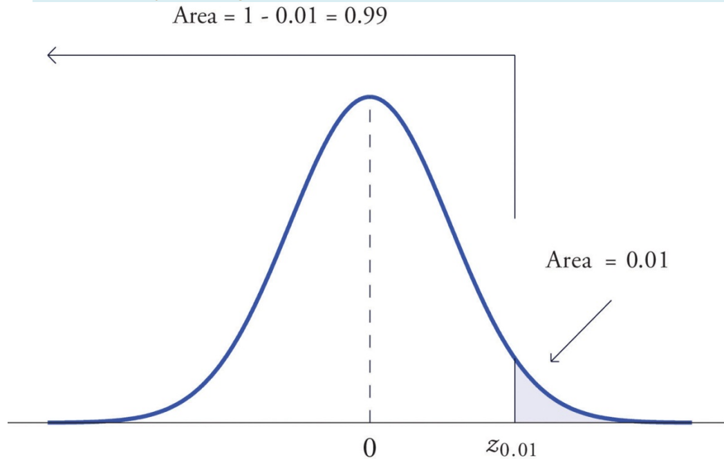
Figure 5.23 Computation of the Number z_{0.01}
