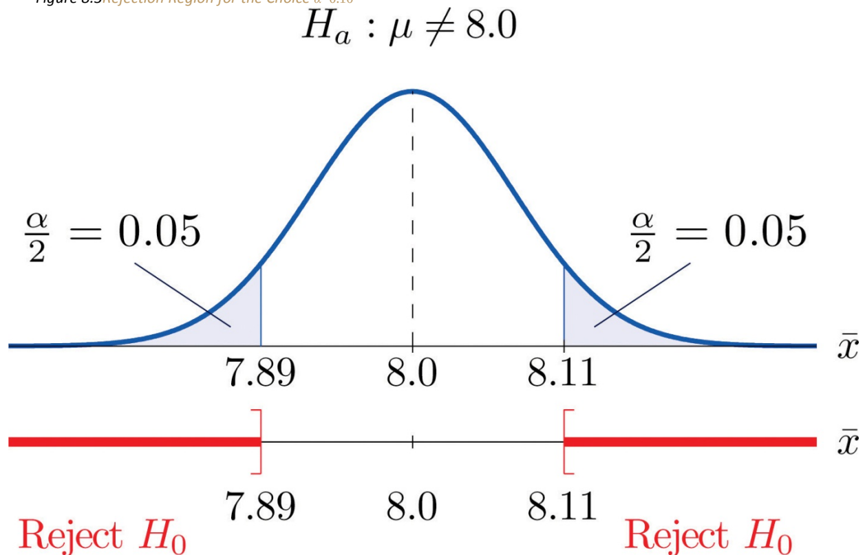
Figure 8.3 Rejection Region for the Choice \alpha=0.10
