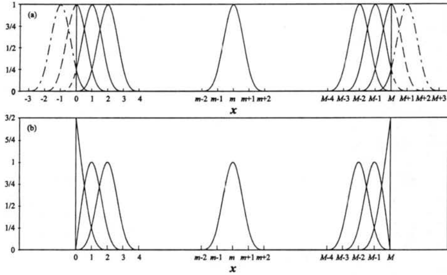
Figure 2.4: Distribution of the a) open bases \psi_m(x) and b) closed bases \phi_m(x) for the boundary condition R1T2 (see appendix D).
