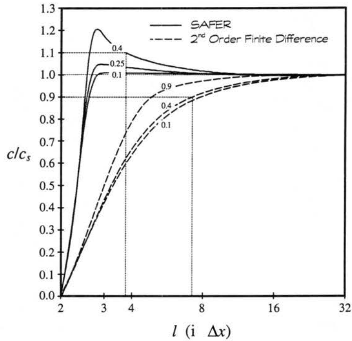
Figure 2.10: Normalized phase speed, c/c_s , as a function of wavelength, l (in units of \Delta x ), for the SAFER (solid) and second-order, centered finite-difference (dashed) methods applied to the one-dimensional advection equation, with constant phase speed, c_s . The numbers along each curve represent the Courant number, \mu = c_s \Delta t / \Delta x . Finally, the dotted lines identify the wavelengths with 10% dispersion errors (redrafted from Ooyama's personal notes).
