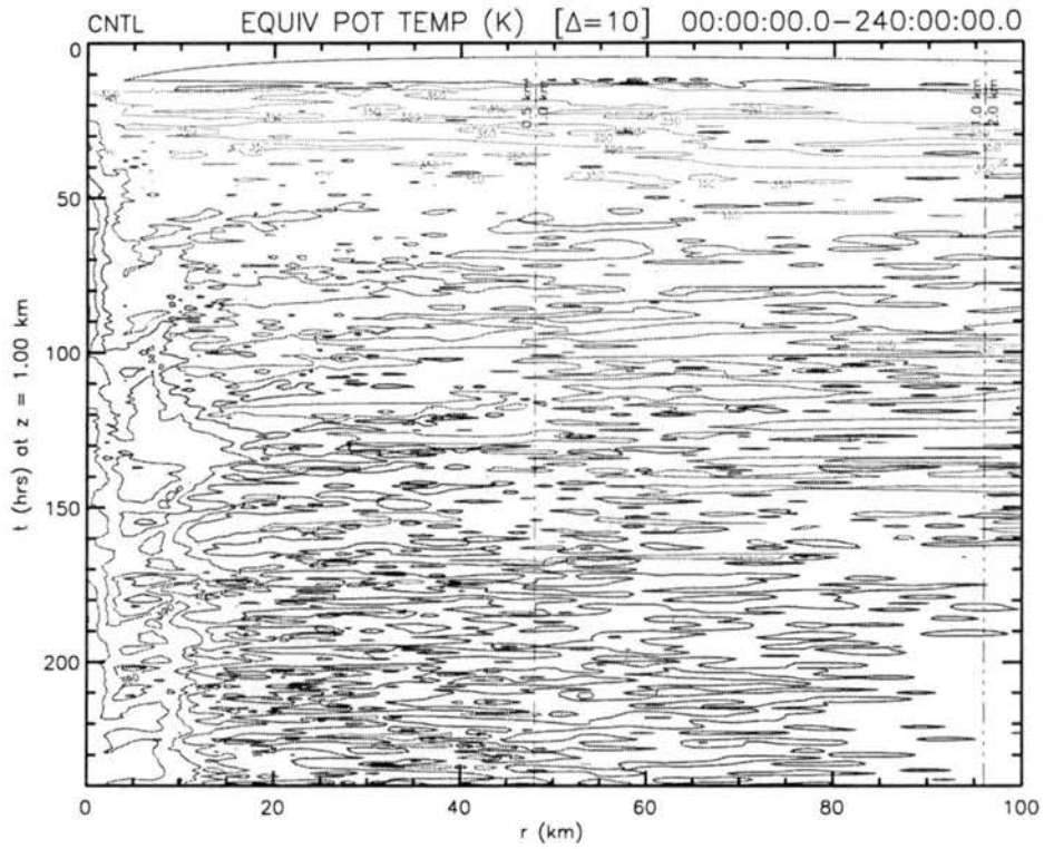
Figure 4.6: CNTL Experiment — Hovmöller diagram of \theta_e at z = 1 km from 0 to 100 km and 0 to 240 hours.
