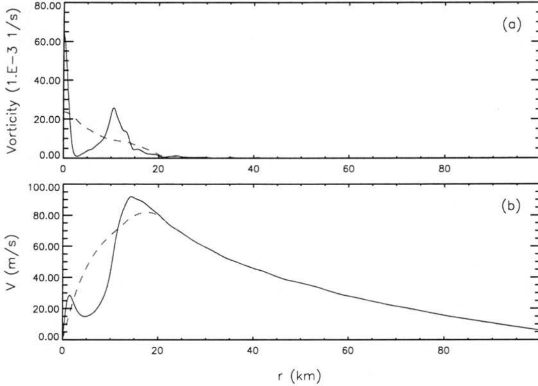
Figure 6.2: Azimuthally-averaged a) vorticity and b) tangential wind profiles for the initial (solid) and final (dashed) states.
