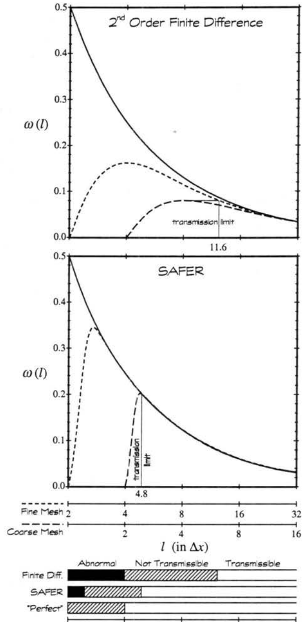
Figure 2.11: Frequency, \omega , as a function of wavelength, l (in units of \Delta x ), for the second-order, centered finite-difference (top) and SAFER (bottom) methods applied to the one-dimensional, linear advection equation, with constant phase speed, c_s = 1 . The solid curve in each represents the exact or "perfect" solution, \omega = c_s/l , while the other curves represent the approximate solution on the fine ( \Delta x_f , dashed) and coarse ( \Delta x_c = 2\Delta x_f , dotted) grids (redrafted from Ooyama's personal notes).
