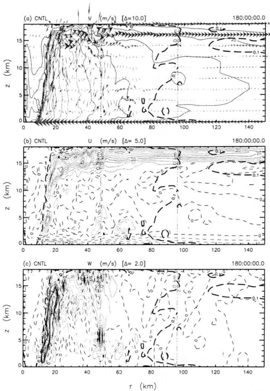
Figure 4.22: CNTL Experiment — 180-hour cross-sections of the a) tangential, b) radial and c) vertical wind speeds ( \text{ms}^{-1} ). For further explanation of the figure markings, see figures 4.2 and 4.13.
