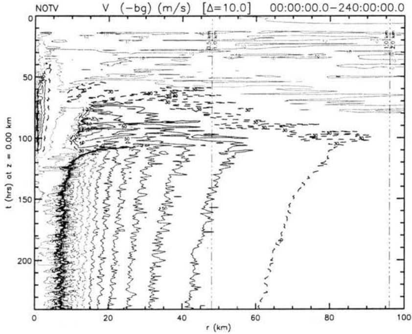
Figure 5.11: NOTV Experiment — Same as figure 4.5.
