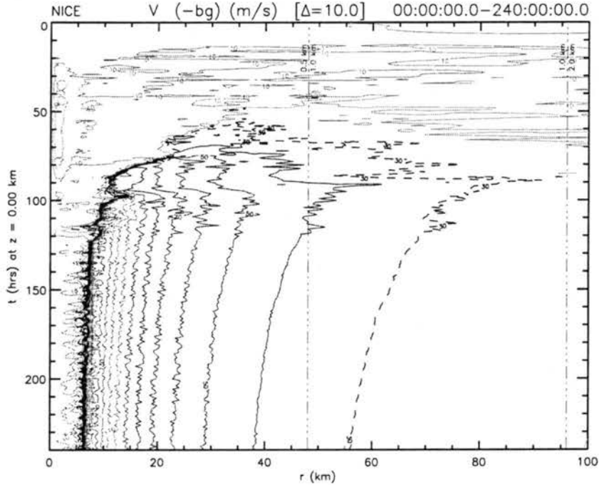
Figure 5.6: NICE Experiment — Same as figure 4.5.
