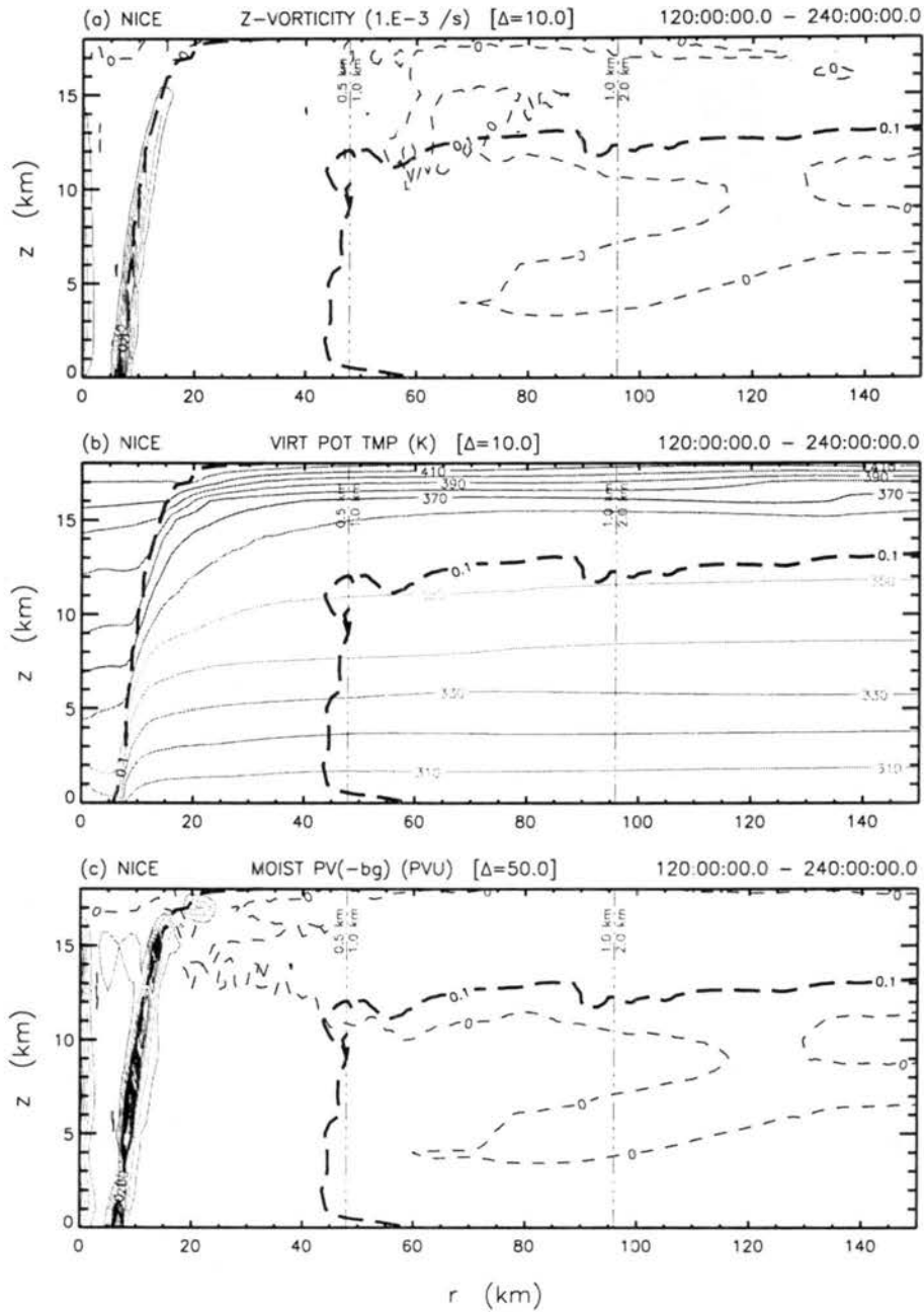
Figure 5.10: NICE Experiment — Same as figure 4.20 but for 120–240 hour time-average.
