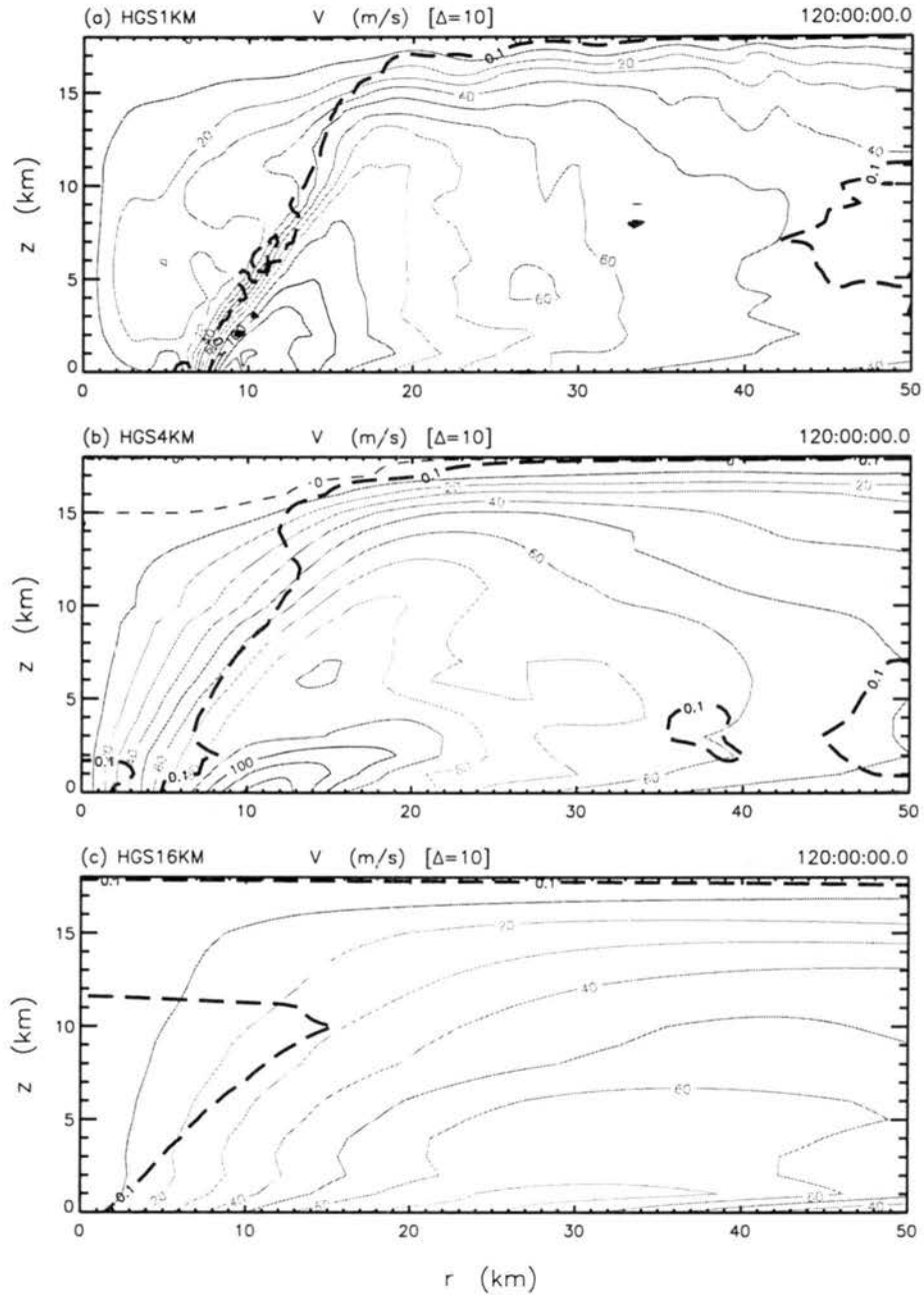
Figure 5.2: HGS[1, 4, 16]KM Experiments — 120-hour (near steady state) cross-sections of the tangential wind speed for a) \Delta r = 1 km, b) \Delta r = 4 km, and c) \Delta r = 16 km. For further explanation of the figure markings, see figures 4.2 and 4.13.
