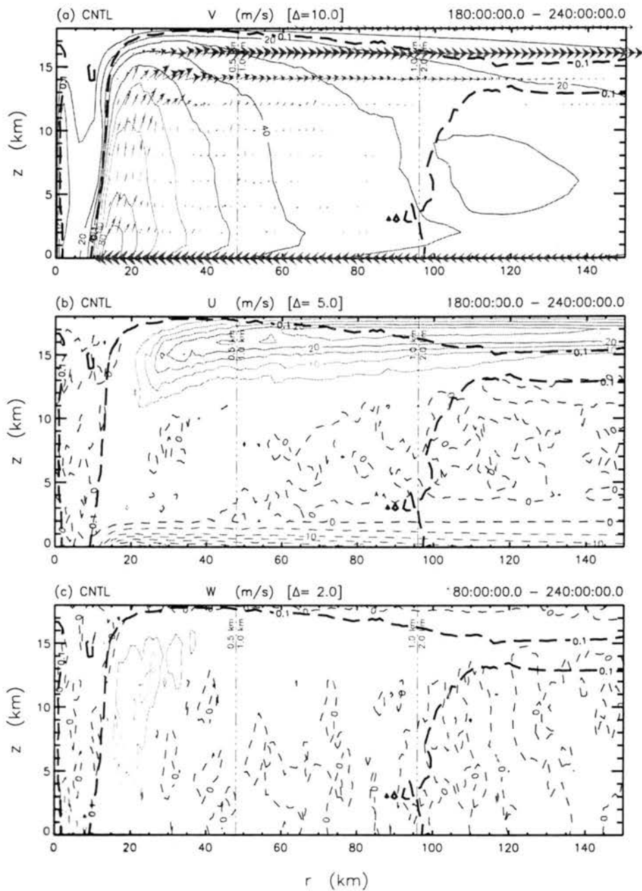
Figure 4.13: CNTL Experiment — time-averaged (180–240 hours) cross-sections of the a) tangential, b) radial and c) vertical wind speeds ( \text{ms}^{-1} ). The heavy dashed line denotes liquid water mixing ratios greater than 0.1 \text{ g kg}^{-1} . For further explanation of the figure markings, see figure 4.2.
