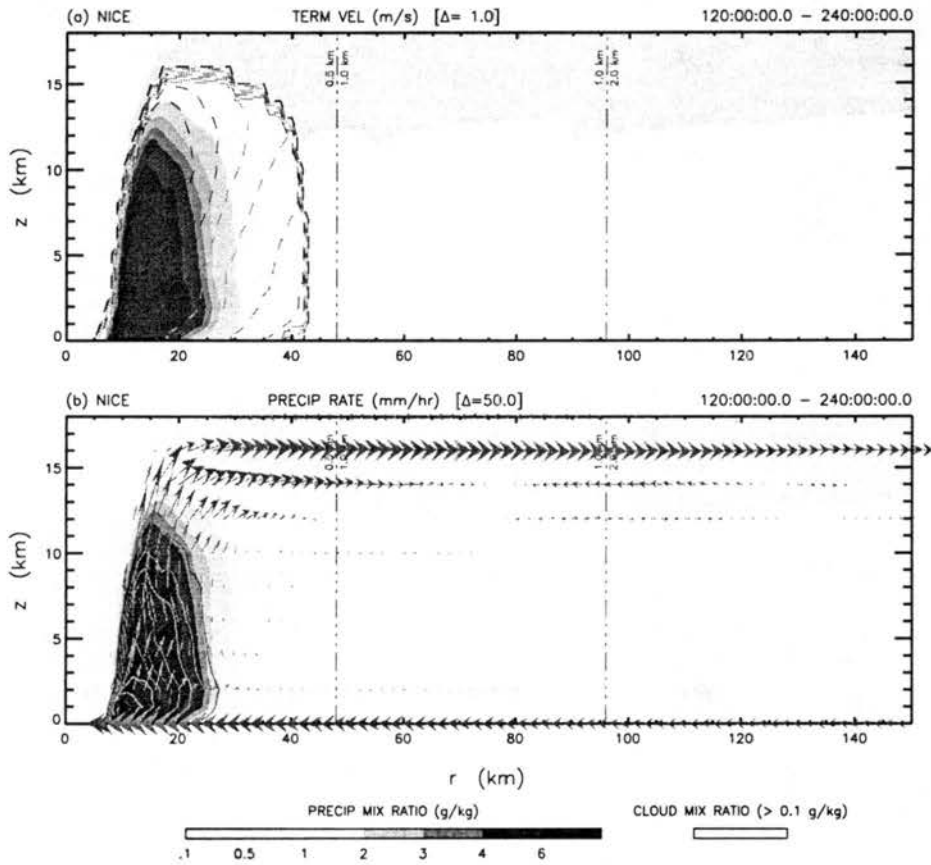
Figure 5.9: NICE Experiment — Same as figure 4.19 but for 120–240 hour time-average.
