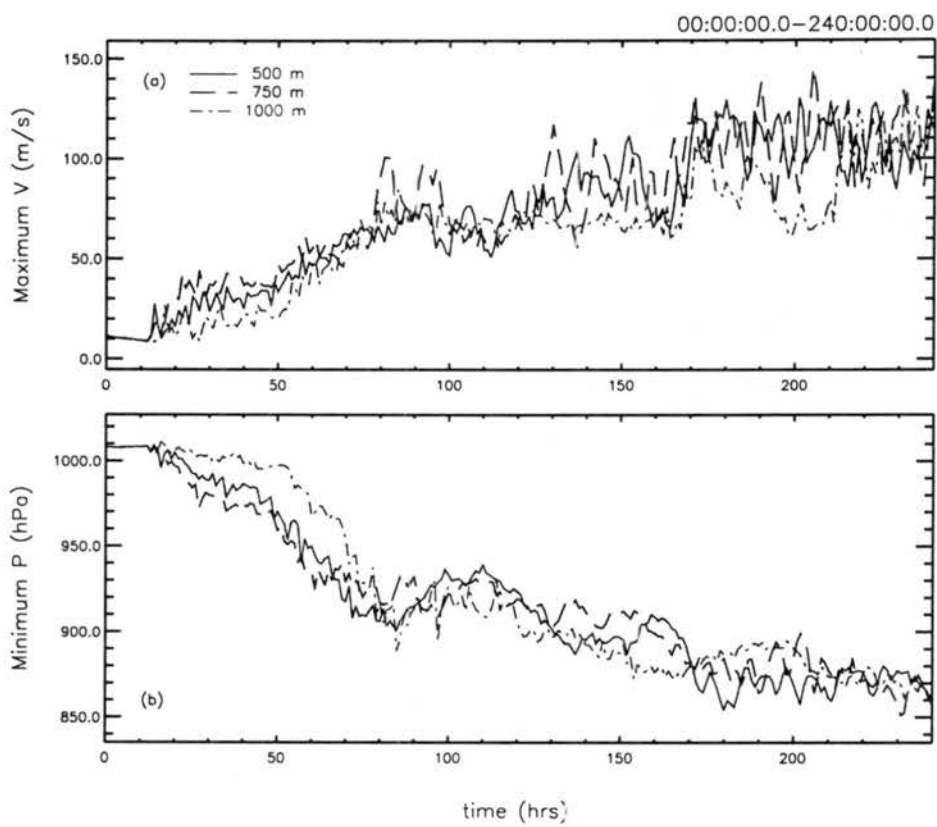
Figure 5.4: VGS[500,750,1000]M Experiments — Same as figure 4.3.
