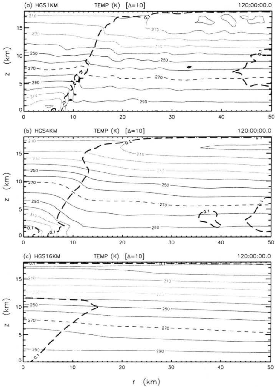
Figure 5.3: HGS[1, 4, 16]KM Experiments — 120-hour (near steady state) cross-sections of the temperature for a) \Delta r = 1 km, b) \Delta r = 4 km, and c) \Delta r = 16 km. For further explanation of the figure markings, see figures 4.2 and 4.13.
