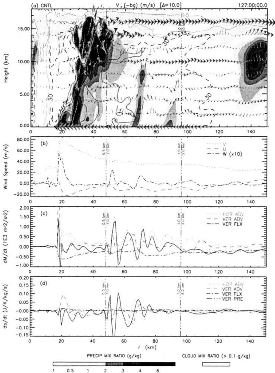
Figure 4.9: CNTL Experiment — Same as figure 4.7 except the time is 127 hours.
