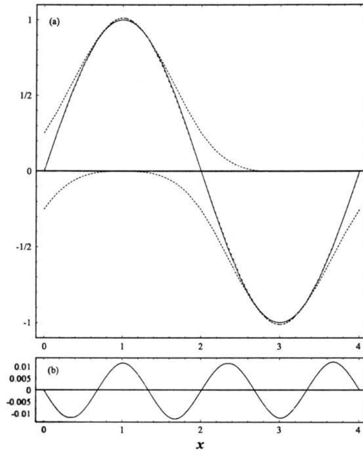
Figure 2.7: Plots of an a) input 4\Delta x sine wave (solid) and its spline representation (large dash), and b) the representational error or "parasite" wave. Included in a) are the individual splines (small dashed) used to obtain the spline representation (redrafted from Ooyama's personal notes).
