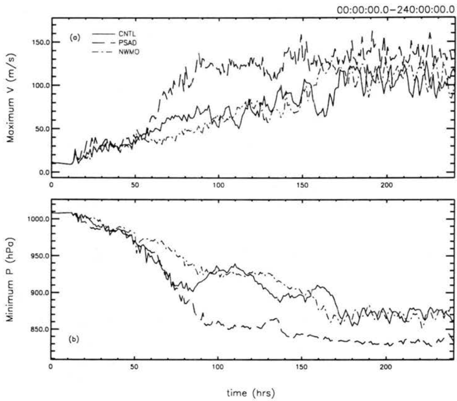
Figure 5.13: PSAD and NWMO Experiments — Same as figure 4.3.
