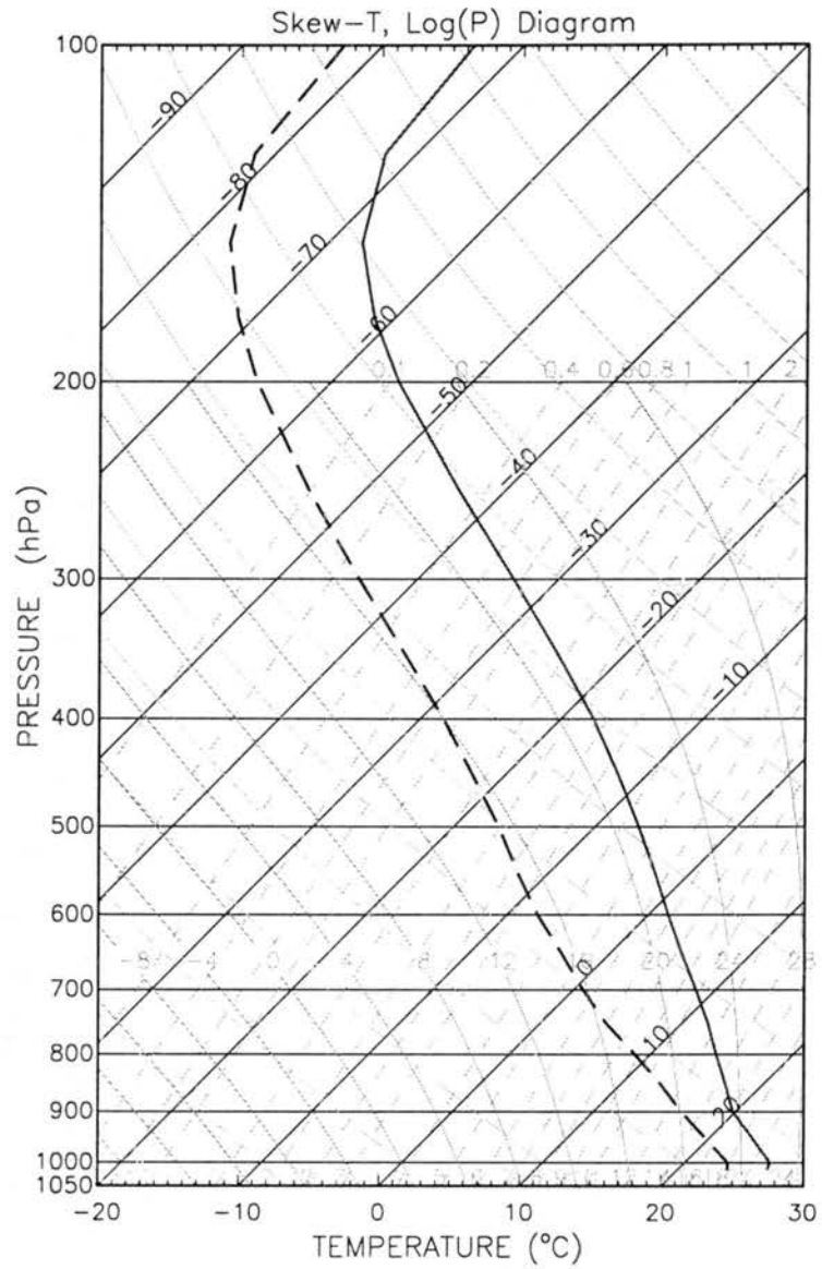
Figure 4.1: Jordan's (1958) mean hurricane season temperature (solid) and dew-point temperature (dashed) soundings.
