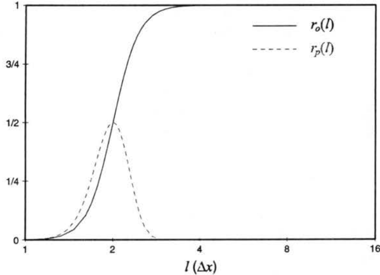
Figure 2.8: Reduced input, r_o(l) , and error, r_p(l') , amplitudes (curves fit to data in Ooyama's personal notes).
