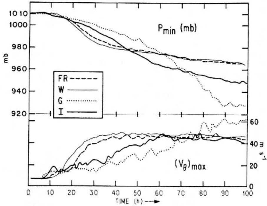
Figure 1.1: W, I, FR, and G Experiments — Evolution of the maximum tangential wind speed [(v_{\theta})_{max}] and minimum surface pressure ( p_{min} ) for Lord and Lord's (1988) frozen rain (FR), water only (W), ice (I), and graupel but no cloud ice or snow (G) experiments. Note that the W and I experiments are identical to the W5A and I7A experiments of Willoughby et al. (1984) [reproduced from Lord and Lord (1988)].
