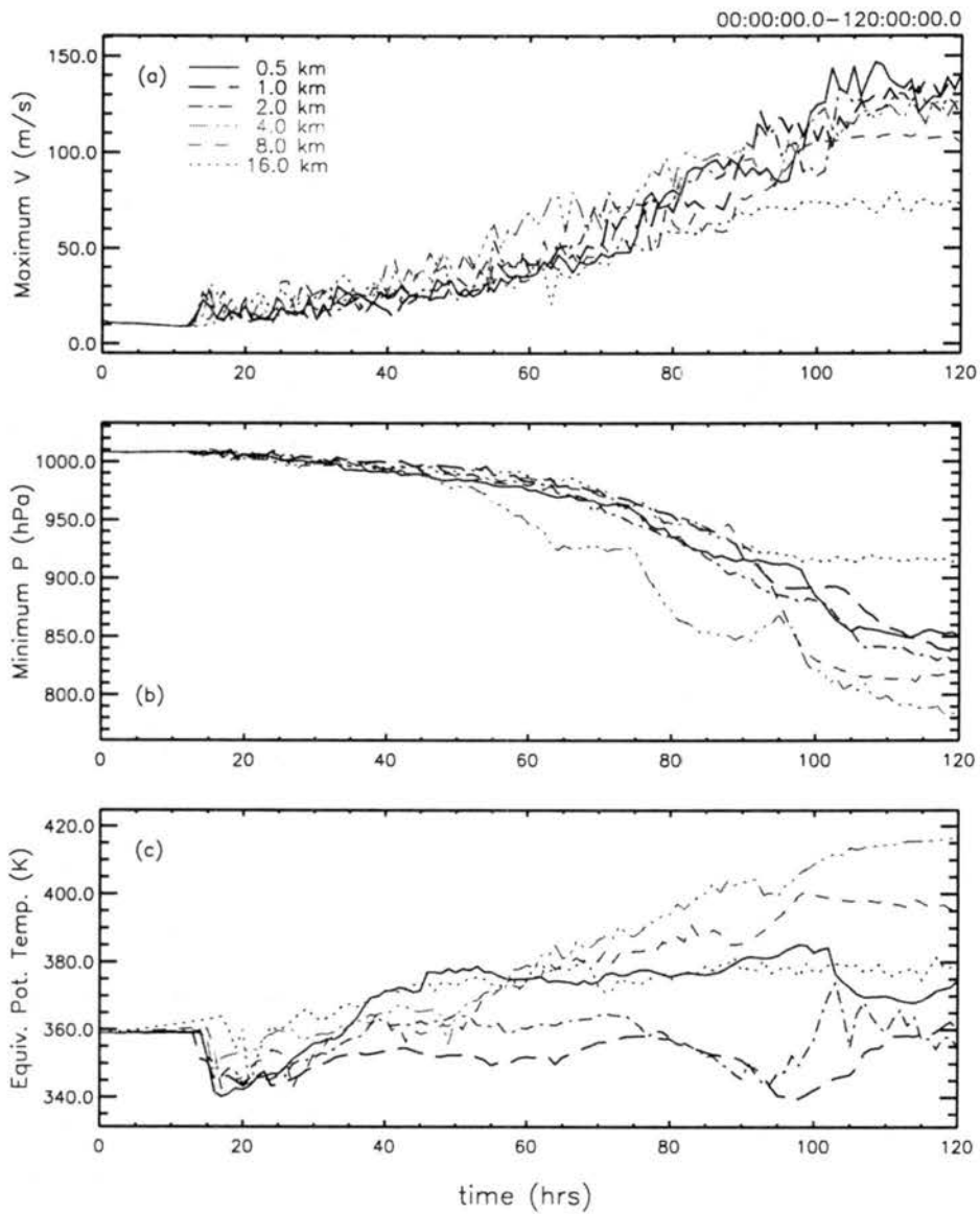
Figure 5.1: HGS[H-16]KM Experiments — Same as figure 4.3, including the c) central surface equivalent potential temperature (K).
