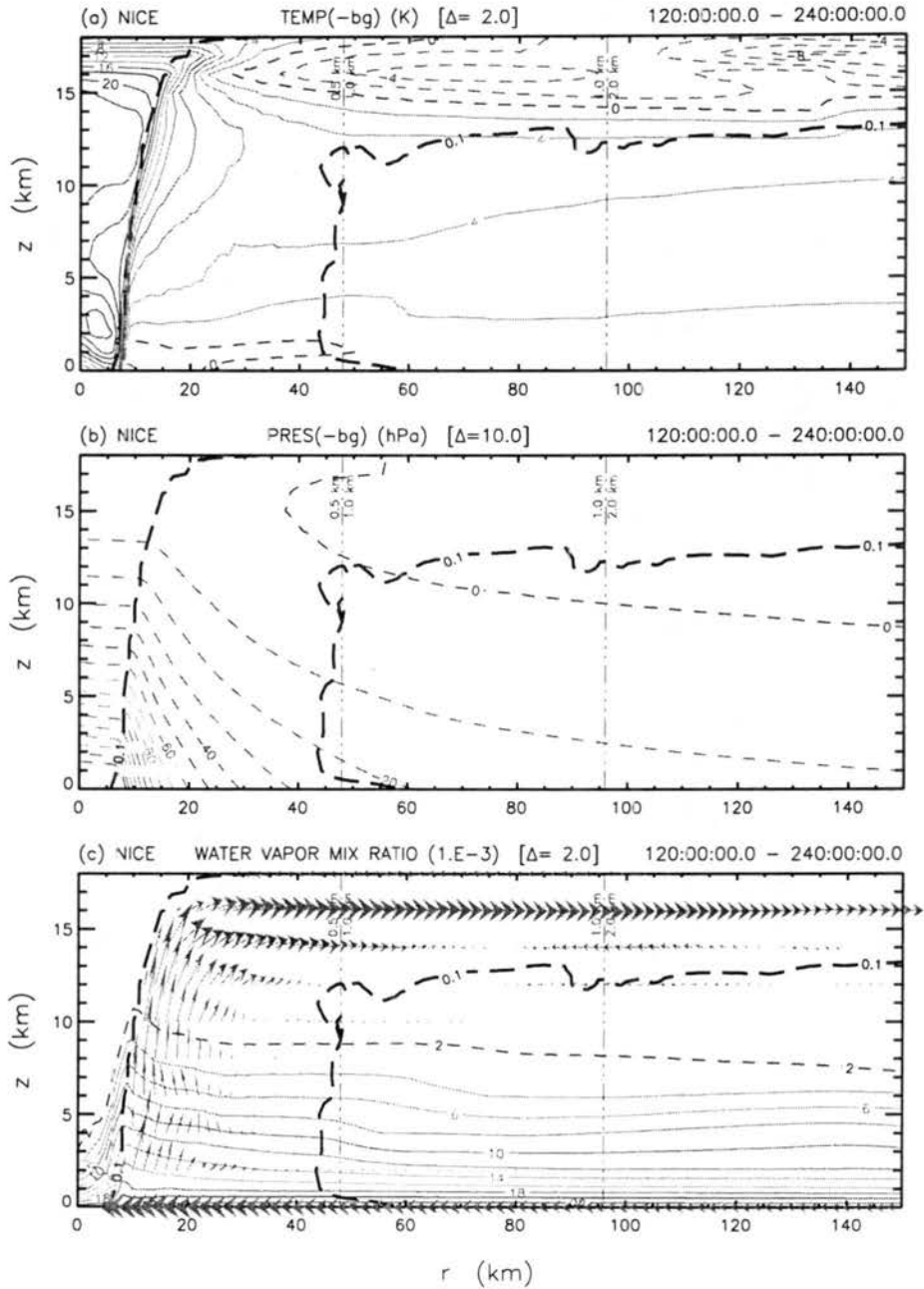
Figure 5.8: NICE Experiment — Same as figure 4.16 but for 120-240 hour time-average.
