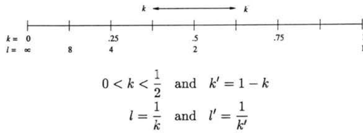
Figure 2.6: Graphical representation of the relationship between the wavenumbers k and k' , or wavelengths l and l' . Notice that a wave with wavelength l is always resolved, whereas a wave with wavelength l' is never resolved. Both k and l are defined in units of \Delta x (adapted from Ooyama's personal notes).
