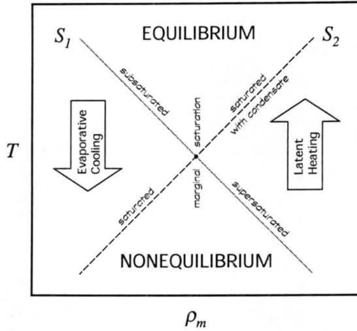
Figure 2.2: Relationship of S_1 and S_2 to T and \rho_m for a given \rho_a , neglecting precipitation. Function S_1 applies when there is no condensate ( \rho_c = 0 ), while S_2 applies when the water vapor is always saturated [ \rho_v = \rho_v^*(T) ]. The function occupying an equilibrium state determines the temperature of the system. Function S_1 is bisected by the marginal saturation, which is the point where \rho_v = \rho_v^*(T) . To the left of this point, the atmosphere is unsaturated. To satisfy the saturation condition on S_2 , condensate is added to the system and evaporated until the wet bulb temperature is reached. Since this addition is physically impossible, S_1 is chosen as the equilibrium state. To the right of the marginal saturation point, the atmosphere is either saturated with condensate or is supersaturated. Since supersaturation typically represents a state of nonequilibrium, S_2 is chosen as the equilibrium state.
