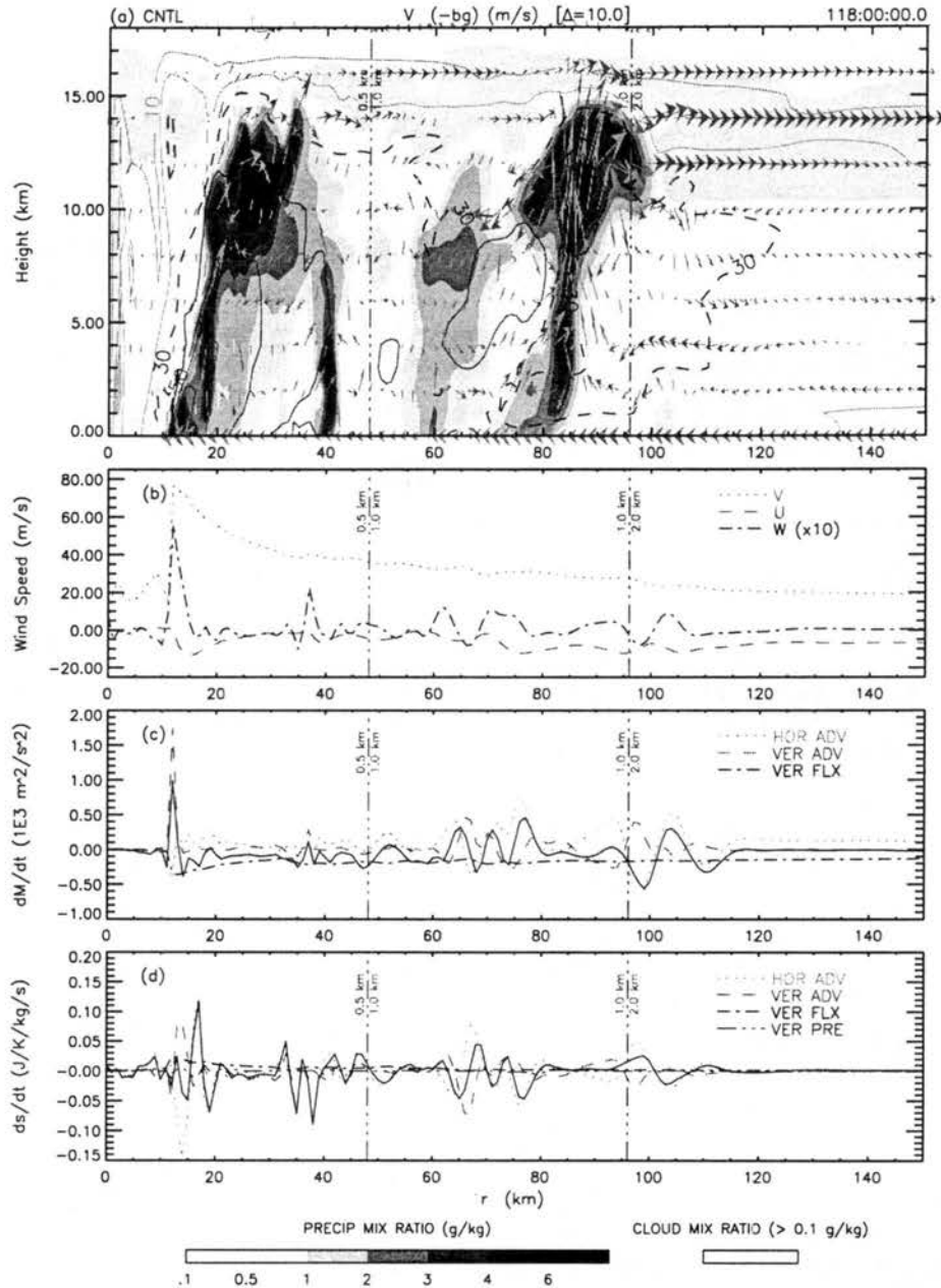
Figure 4.7: CNTL Experiment — Evolution of a concentric eyewall cycle at 118 hours. The panels contain the a) tangential wind (contour), radial and vertical winds (vectors), cloud (gray shading, 0.1 \text{ g kg}^{-1} ), and precipitation (blue shading, .1, .5, 1, 2, 3, 4, 6 \text{ g kg}^{-1} ); b) tangential (dot), radial (dash), and vertical (dash-dot, \times 10 ) wind components (radial profiles); c) equation (4.3) terms (radial profiles), and d) equation (4.4) terms (radial profiles). The terms in (4.3) and (4.4) are the local change (solid), horizontal advection (dot), vertical advection (dash), vertical turbulent flux (dash-dot), and precipitation flux (chain). All of the profiles were computed at a height of 500 m. For further explanation of the figure markings, see figures 4.2 and 4.4.
