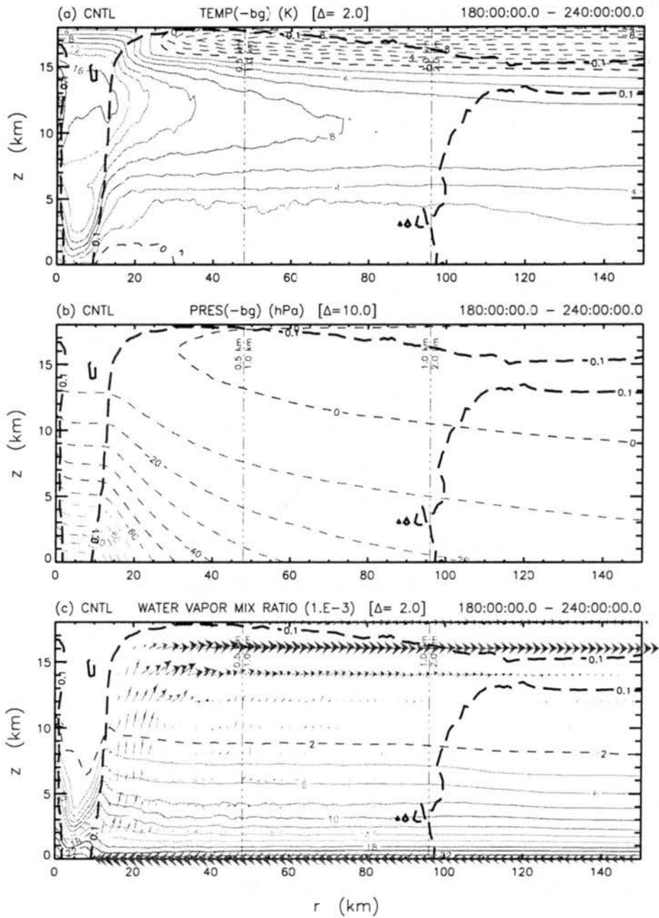
Figure 4.16: CNTL Experiment — time-averaged (180–240 hours) cross-sections of the a) perturbation temperature, b) perturbation pressure and c) water vapor mixing ratio. For further explanation of the figure markings, see figures 4.2 and 4.13.
