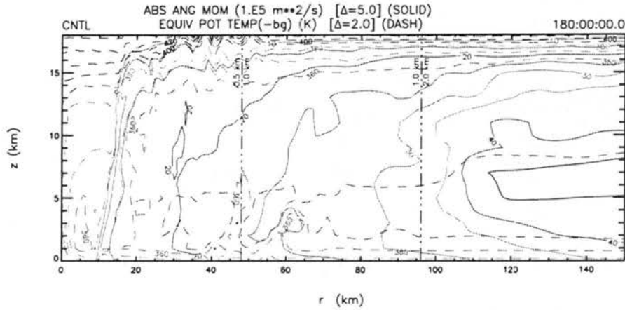
Figure 4.24: CNTL Experiment — 180-hour cross-sections of the absolute angular momentum, M (solid) and the equivalent potential temperature, \theta_e (dashed). For further explanation of the figure markings, see figure 4.2.
