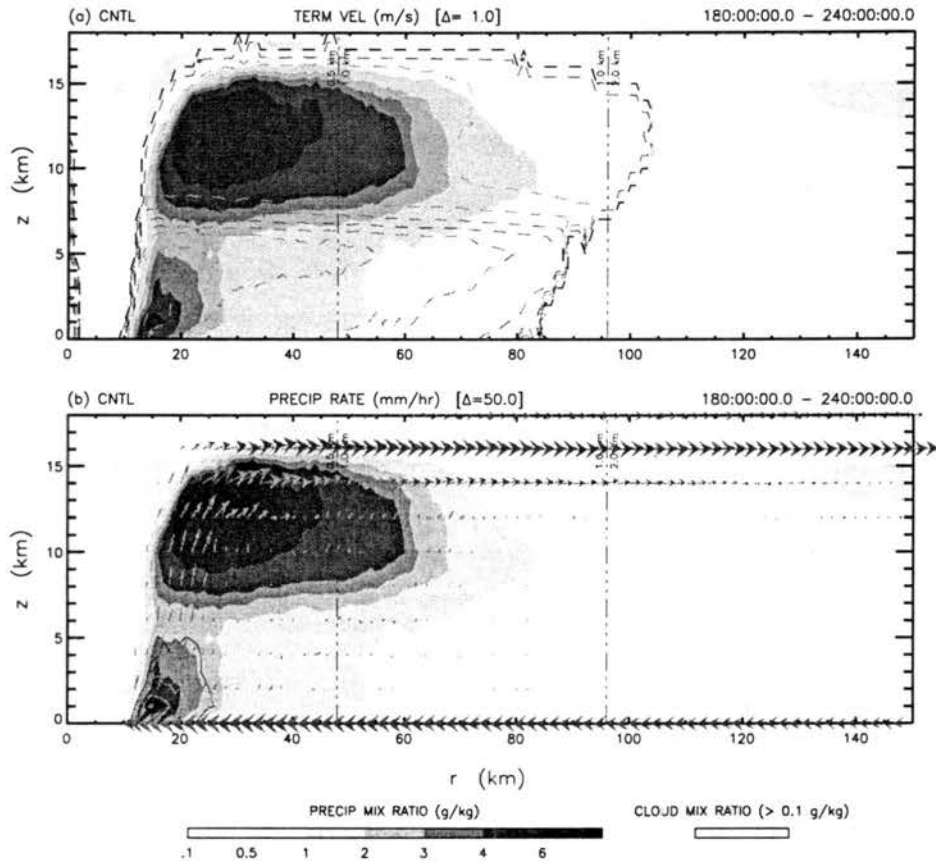
Figure 4.19: CNTL Experiment — time-averaged (180–240 hours) cross-sections of the a) terminal velocity, W and b) the precipitation rate. For further explanation of the figure markings, see figure 4.2.
