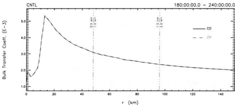
Figure 4.15: CNTL Experiment — time-averaged (180–240 hours) radial profiles of the bulk transfer coefficients for momentum (solid) and energy/mass transfers (dashed). If only a single curve is shown, then the coefficients are identical. For further explanation of the figure markings, see figure 4.2.
