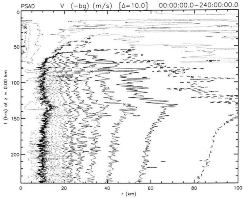
Figure 5.14: PSAD Experiment — Same as figure 4.5.
