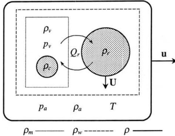
Figure 2.1: Parcel of moist air with total mass density \rho = \rho_a + \rho_w , which is composed of dry air and total water with mass densities \rho_a and \rho_w , respectively. The total water mass density, \rho_w = \rho_v + \rho_c + \rho_r , is further separated into the mass densities of water vapor ( \rho_v ) and of condensate (liquid and/or solid), which includes cloud ( \rho_c ) and precipitation ( \rho_r ). The dry air and airborne water, which has mass density \rho_m = \rho_a + \rho_v , move with velocity \mathbf{u} = (u, v, w) , while the precipitation falls relative to the volume with terminal velocity \mathbf{U} = (0, 0, W) or relative to the Earth with velocity \mathbf{u}_r = \mathbf{u} + \mathbf{U} . Note that the lines of demarcation enclosing the different mass densities illustrate the partition of mass, but not its location; we assume that all mass is distributed uniformly over the parcel volume.
