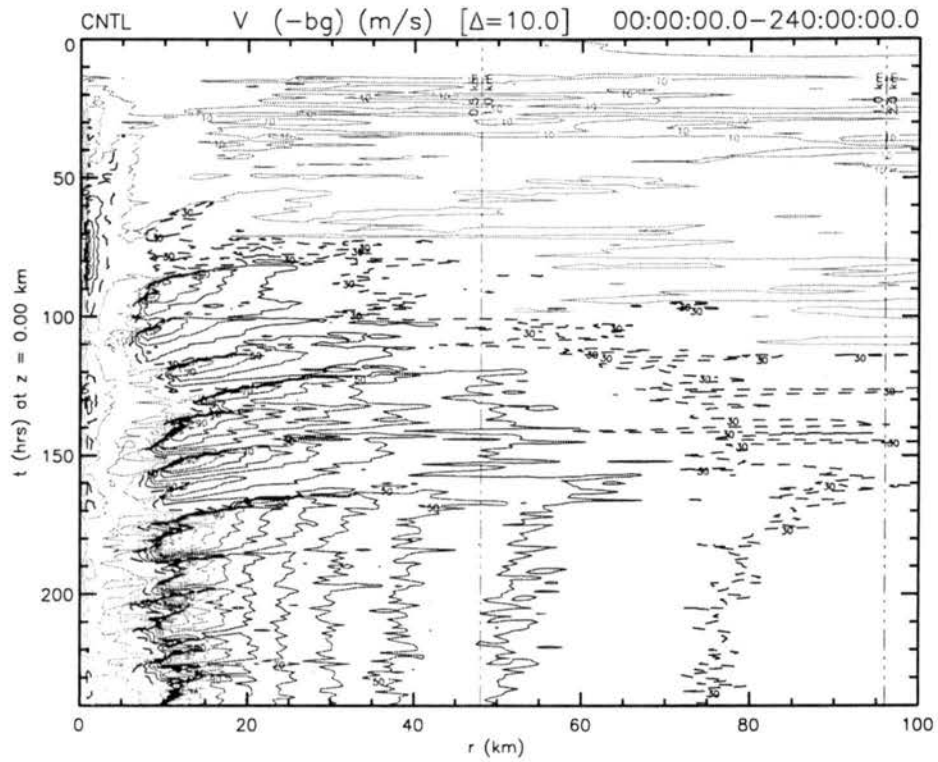
Figure 4.5: CNTL Experiment — Hovmöller diagram of the surface tangential wind speed from 0 to 100 km and 0 to 240 hours. The dashed line marks the 30 \text{ m s}^{-1} contour, which is slightly less than hurricane intensity, 33 \text{ m s}^{-1} .
