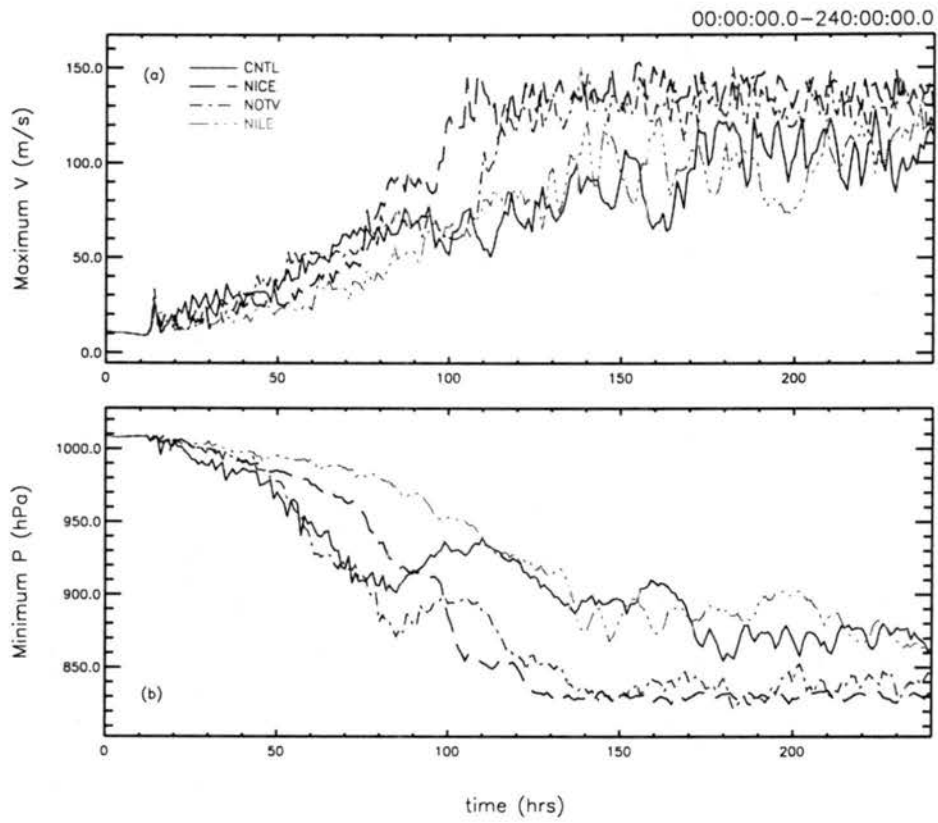
Figure 5.5: NICE, NOTV, and NILE Experiments — Same as figure 4.3.
