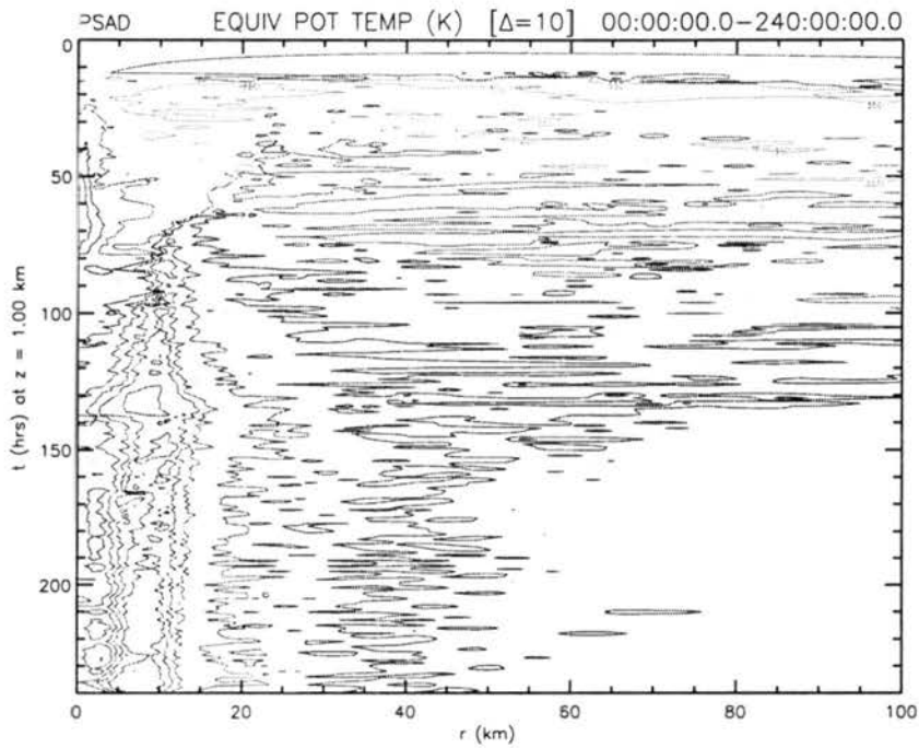
Figure 5.15: PSAD Experiment — Same as figure 4.6.
