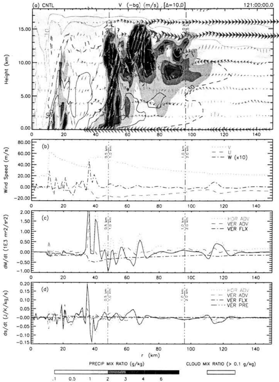
Figure 4.8: CNTL Experiment — Same as figure 4.7 except the time is 121 hours.
