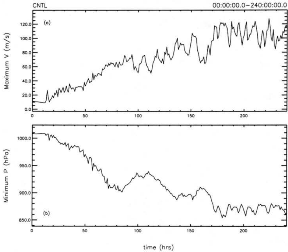
Figure 4.3: CNTL Experiment — Time series from 0–240 hours of the a) maximum tangential wind speed ( \text{m s}^{-1} ) and the b) central surface pressure (hPa).
