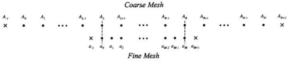
Figure 2.5: Nesting schema of two grids, a fine grid ( a 's) with M nodes and a coarse grid ( A 's) with N nodes, for which the nodal spacing differs by a factor of 2. Both interfaces are identified by the vertical dashed line. Subscripts L and R distinguish the left and right interfaces, respectively. The large filled circles denote the primary nodes and the \times 's the auxiliary nodes. The small filled circles denote gaps in the depiction of the grids [adapted from DeMaria et al. (1992)].
