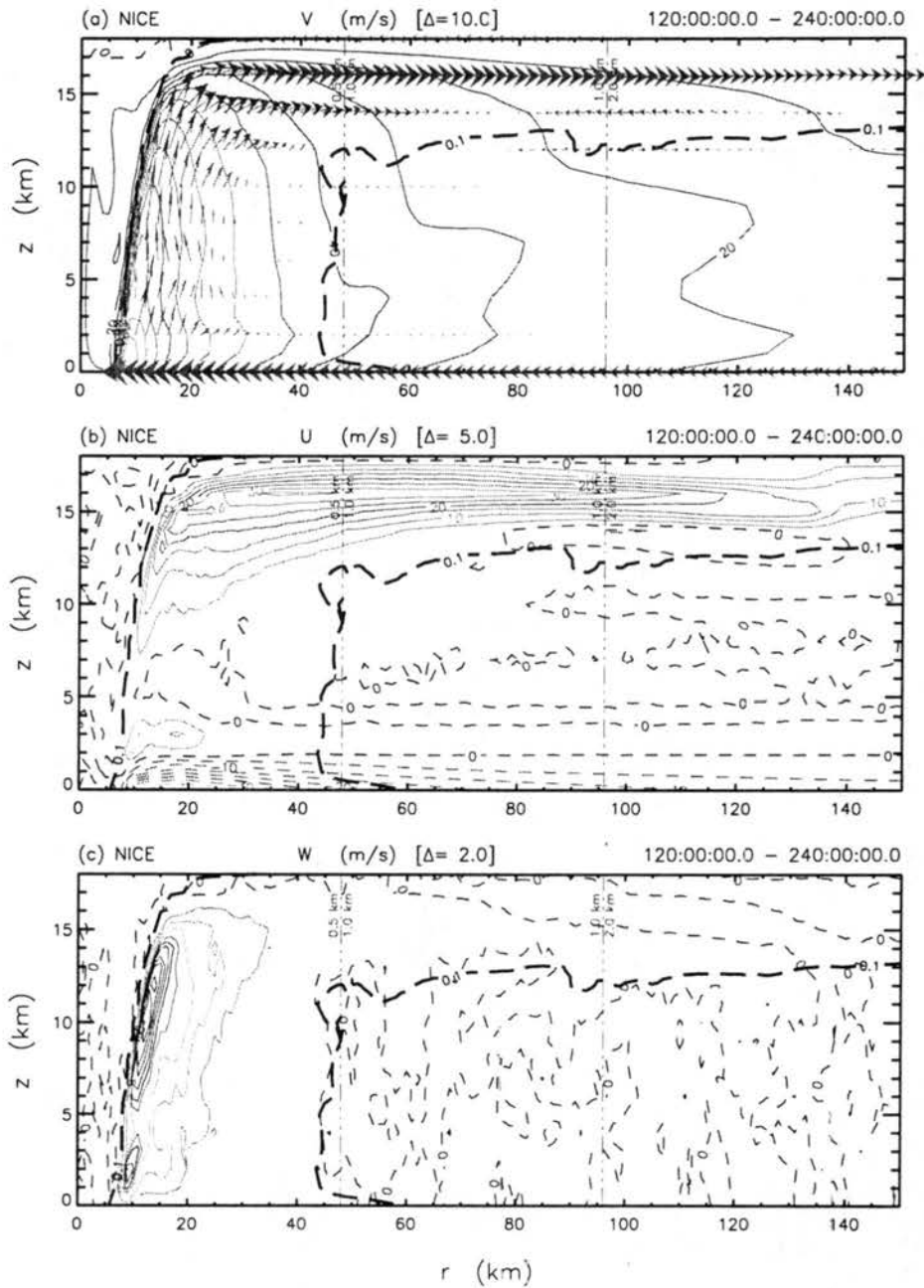
Figure 5.7: NICE Experiment — Same as figure 4.13 but for 120–240 hour time-average.
