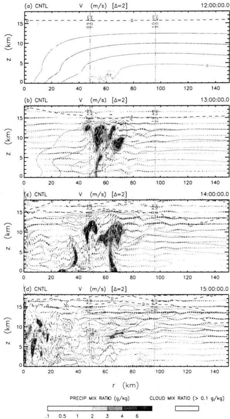
Figure 4.4: CNTL Experiment — Cross-sections depicting the initial formation of convection in terms of the tangential wind (contouring), precipitation mixing ratio (blue shading), and cloud mixing ratio (gray shading) for a) 12, b) 13, c) 14, and d) 15 hours. The wind vectors depict the relative magnitude of the winds in the plane of the cross-section. For further explanation of the figure markings, see figure 4.2.
