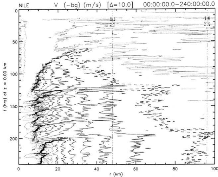
Figure 5.12: NILE Experiment — Same as figure 4.5.
