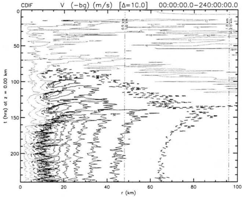
Figure 5.17: CDIF Experiment — Same as figure 4.5.
