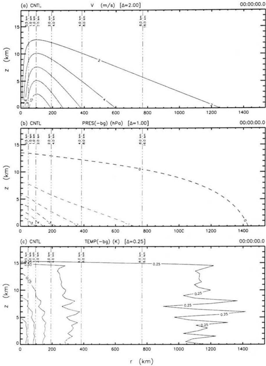
Figure 4.2: Initial vertical cross-sections ( r, z ) of the vortex a) tangential wind speed ( v ), b) pressure perturbation ( p' ), and temperature perturbation ( T' ). Headings above each figure indicate the experiment (left); the contoured variable, including units and contour interval ( \Delta ) (center); and the time in units of hh:mm:ss.s (right). Perturbation variables are identified by the (-bg) to the right of the variable name. The vertically-oriented chained lines mark the interfaces between nested grids, while the distances straddling these lines indicate the grid spacing to either side.
