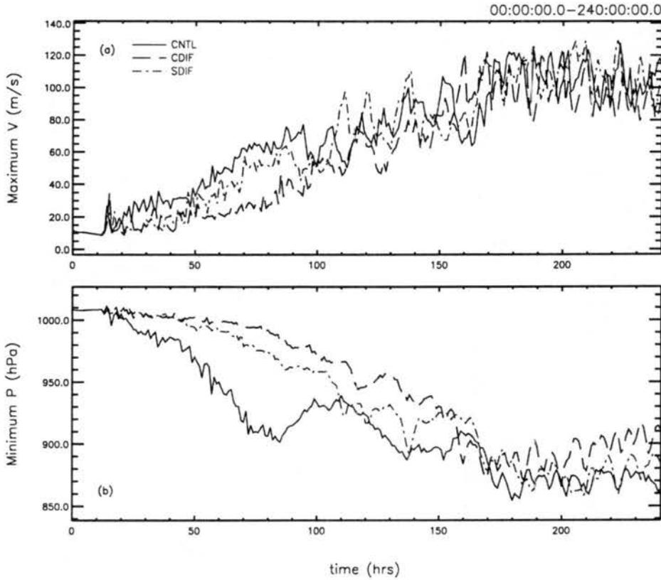
Figure 5.16: CDIF and SDIF Experiments — Same as figure 4.3.
