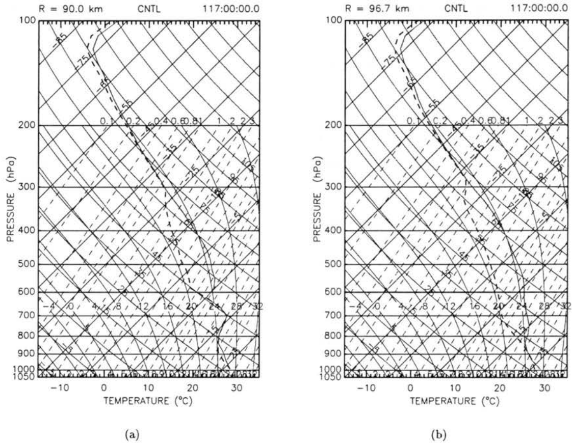
Figure 4.10: CNTL Experiment — Evolution of the developing secondary eyewall at 117.0 hours. The panels contain the vertical profiles of temperature and dewpoint temperature a) through and b) outside of the secondary eyewall, and the contours of c) specific entropy and d) absolute angular momentum, the radial and vertical winds (vectors), cloud (gray shading, 0.1 \text{ g kg}^{-1} ), and precipitation (blue shading, .1, .5, 1, 2, 3, 4, 6 \text{ g kg}^{-1} ). For further explanation of the figure markings, see figures 4.2 and 4.4.
