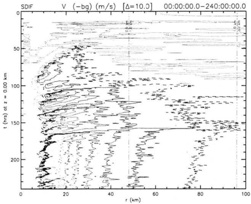
Figure 5.18: SDIF Experiment — Same as figure 4.5.
