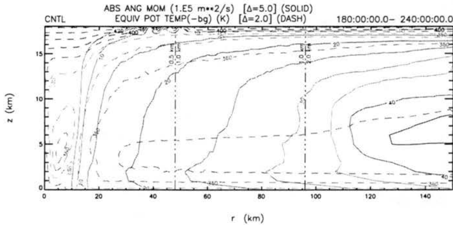
Figure 4.17: CNTL Experiment — time-averaged (180–240 hours) cross-sections of the absolute angular momentum, M (solid) and the equivalent potential temperature, \theta_e (dashed). For further explanation of the figure markings, see figure 4.2.
