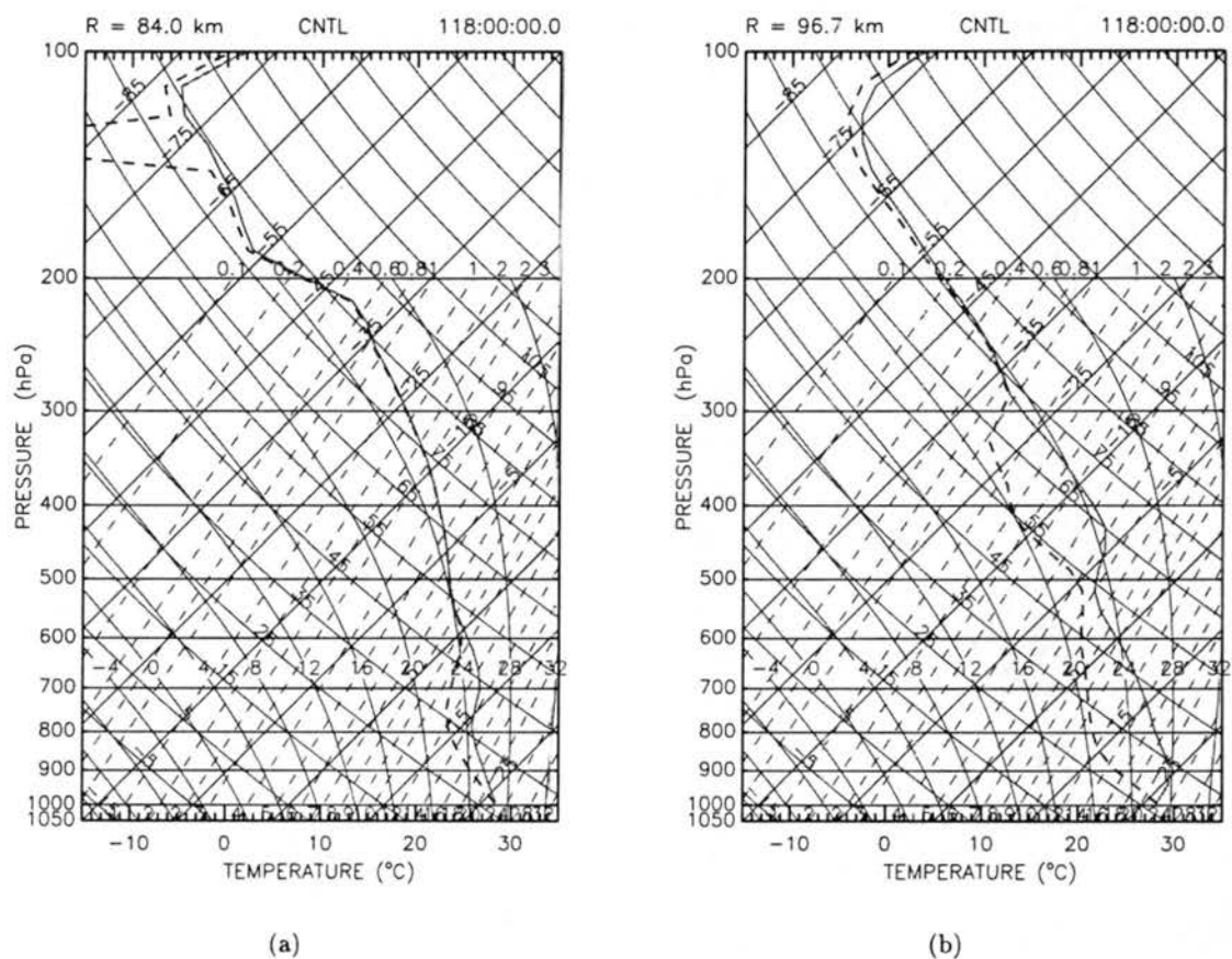
Figure 4.12: CNTL Experiment — Same as figure 4.10 except the time is 118.0 hours.
