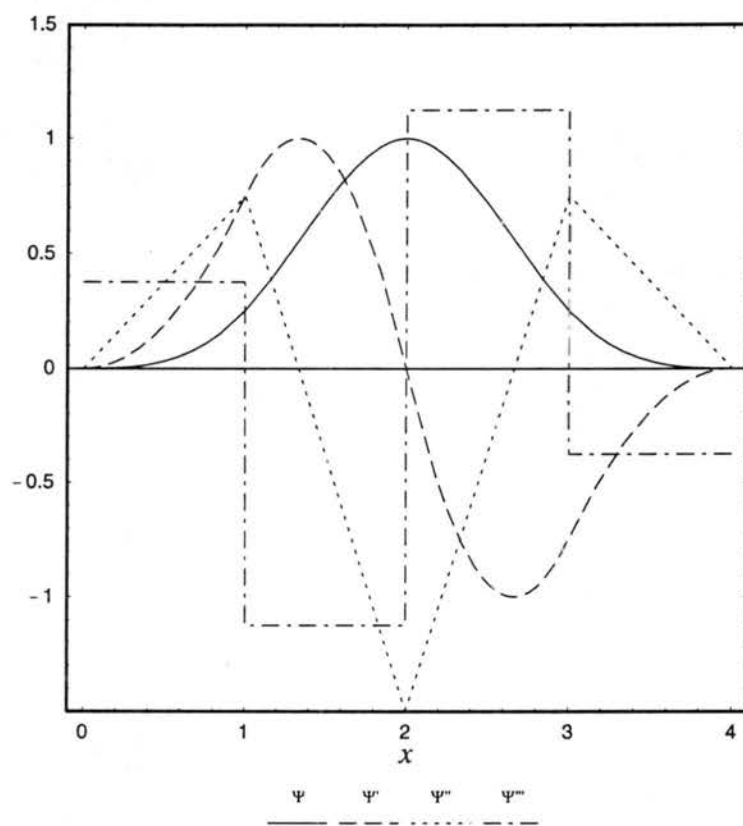
Figure 2.3: The cubic B-spline \Psi(x) and its first three derivatives. Note that the second derivative has been scaled by 1/2 and the third derivative by 1/4 .
