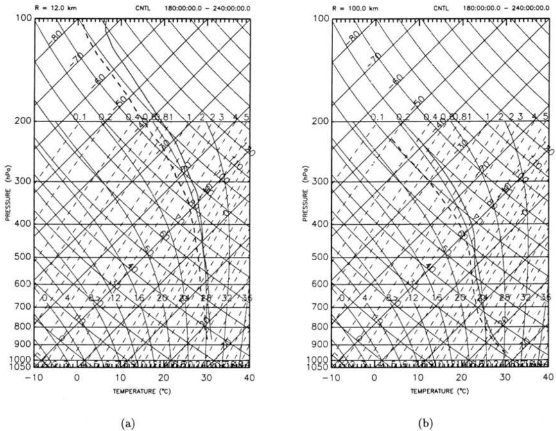
Figure 4.18: CNTL Experiment — time-averaged (180–240 hours) vertical profiles of temperature and dewpoint temperature at a) r = 12 km and b) r = 100 km. Above z = 1 km, both profiles are computed along R = \text{constant} , wherein r and R are related by \frac{1}{2}fR^2 = rv + \frac{1}{2}fr^2 .
