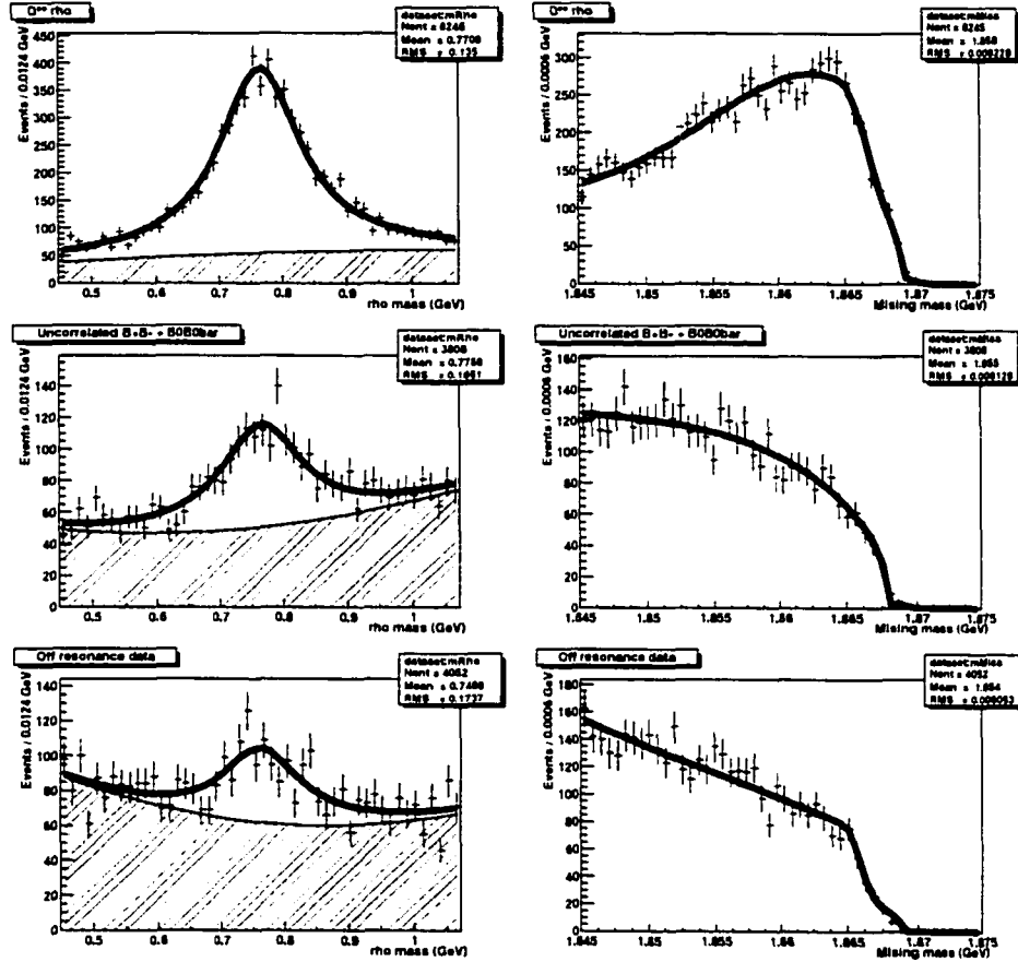
Figure 7.4: m(\rho) and m_{\text{miss}} distributions (from top to bottom) of \bar{B} \rightarrow D^{**}\rho^+ (Monte Carlo), and combinatoric B\bar{B} events (Monte Carlo), and off-resonance data. The shaded region in the m(\rho) plots shows the polynomial component of the fit.
