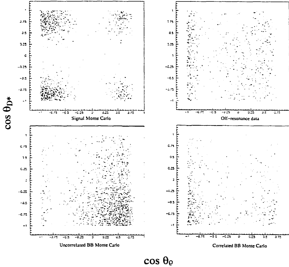
Figure 4.6: \cos \theta_{D^*} vs. \cos \theta_\rho distributions of (clockwise from top left) Monte Carlo signal events, off-resonance data, Monte Carlo correlated backgrounds (see section 6.4) and uncorrelated Monte Carlo generic B\bar{B} events. \cos \theta_\rho < 1 due to the requirement |\vec{p}_{\pi^0}| > 0.4 \text{ GeV}/c . The polarization generated in the signal Monte Carlo is based on the CLEO polarization measurement [35].
