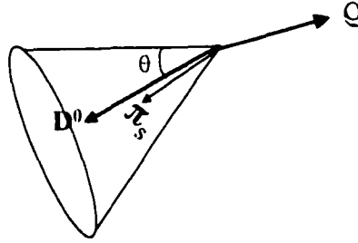
Figure 5.4: A schematic representation of the cone-cut. In this analysis we use \theta = 1 rad.
