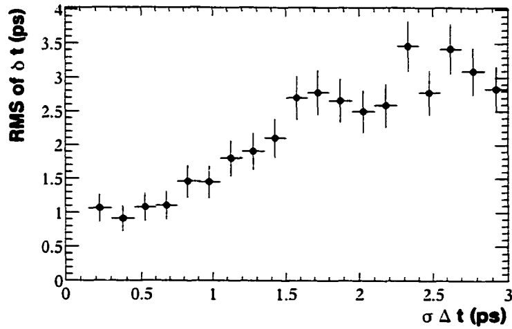
Figure 5.8: RMS of the residual (\Delta t - \Delta t_{true}) distribution plotted for various bins of \sigma_{\Delta t} .
