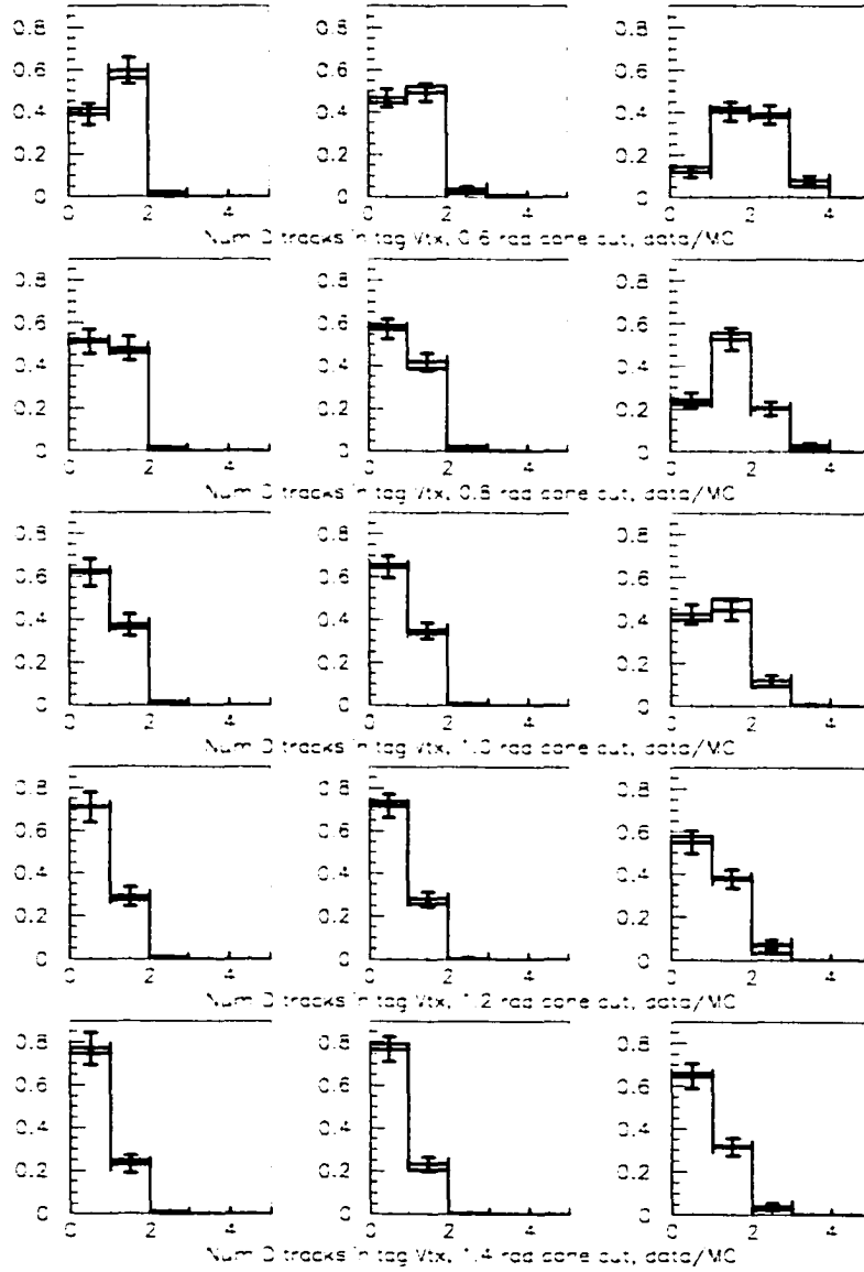
Figure 7.10: The number of D_{\text{miss}} daughter tracks wrongly assigned to the tag B vertex for cone cuts of (from top to bottom) 0.6, 0.8, 1.0, 1.2, and 1.4 rad. The histograms are fully reconstructed Monte Carlo events, and the data points are from fully reconstructed data in the modes (from left to right) K\pi , K\pi\pi^0 , and K3\pi . All distributions are normalized to unit area.
