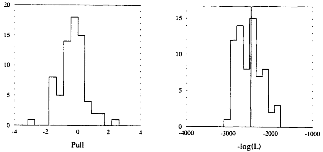
Figure 9.5: Full toy Monte Carlo results when using the GExp resolution function: Left: \tau_B pull distribution. Right: -\log(\text{likelihood}) distribution. The vertical line is the value obtained from the fit to the data.
