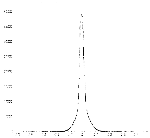
Figure 5.2: Resolution of the z_{rec} vertex obtained from Monte Carlo.
