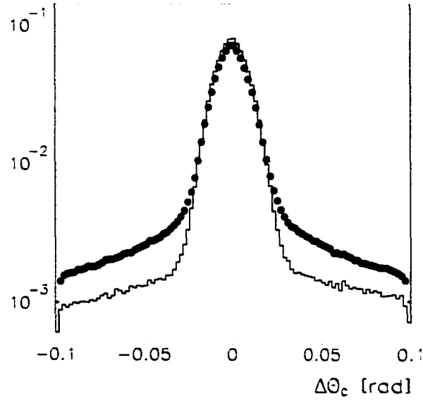
Figure A.7: The single photon Cherenkov angle distribution for the muon track as reconstructed in the DIRC for data(dots) and Monte Carlo(line) overlayed. On the y axis is the probability plotted on a log scale.
