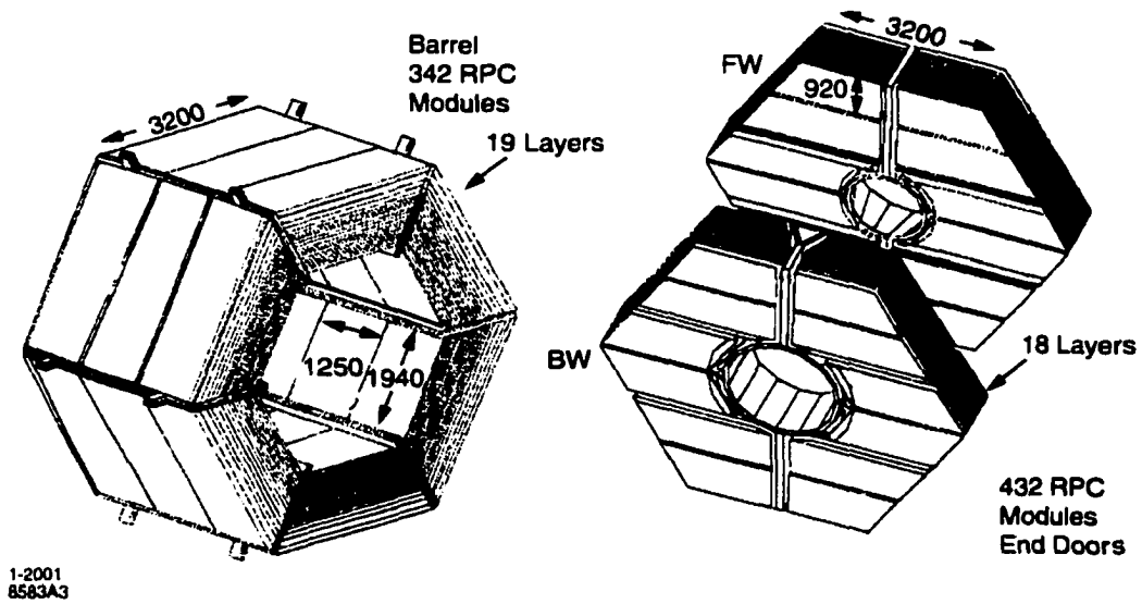
Figure 3.13: The Instrumented Flux Return consists of three sections: the barrel (left), containing 342 RPC modules between 19 layers of steel, and the forward and backward end-doors (right), with a total of 432 RPC modules in 18 layers. 32 more RPCs are placed in the two cylindrical layers (not shown here).
