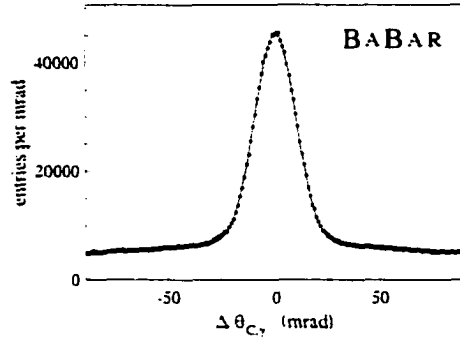
Figure A.6: The difference between the measured and expected Cherenkov angle for single photons, \Delta\theta_{c,\gamma} for single muons in \mu^+\mu^- events. The curve shows the result of a fit of two Gaussians to the data. The width of the narrow Gaussian is 9.6 mrad.
