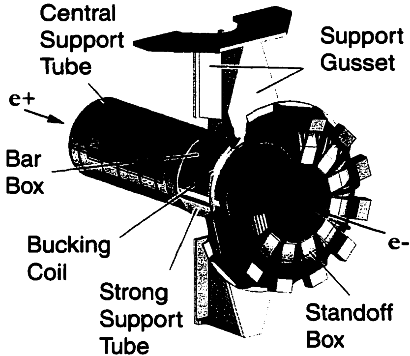
Figure A.2: Schematical view of the DIRC assembly within BABAR .
