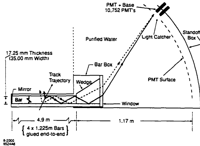
Figure 3.10: Schematic of the DIRC fused silica radiator bar and imaging region.
