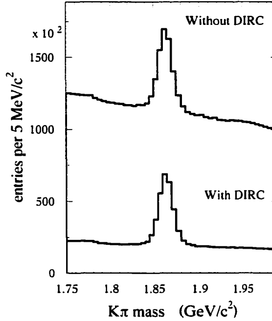
Figure A.10: Invariant K\pi inclusive mass spectrum with and without the use of the DIRC for kaon identification. The mass peak corresponds to the decay of the D^0 particle.
