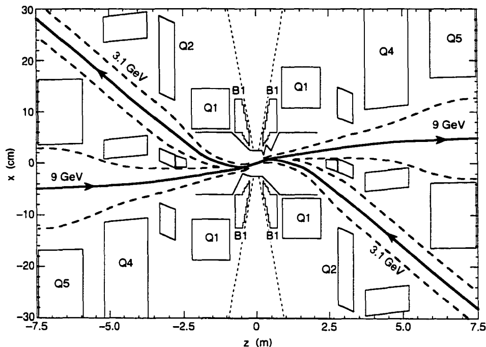
Figure 3.2: A plan view of the interaction region. The vertical scale is exaggerated. The beams collide head-on and are separated magnetically by the B1 dipole magnets. The focusing of the beams is achieved by using the quadrupole magnets, Q1, Q2, Q4 and Q5. The dashed lines indicate the beam stay-clear region and the detector acceptance cutoff at 300 mrad.
