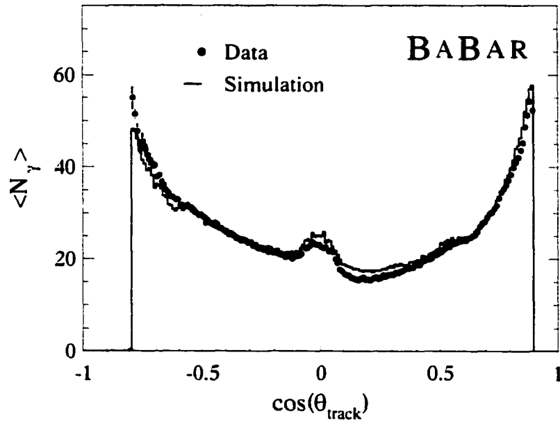
Figure A.9: Number of detected photons versus track polar angle for reconstructed tracks in dimuon events compared to Monte Carlo simulation. The mean number of photons in the simulation has been tuned to match the data.
