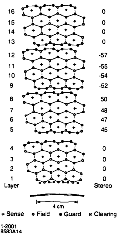
Figure 3.7: Schematic layout of the drift chamber layer arrangement. The layers are arranged into 10 super-layers of 4 layers each.
