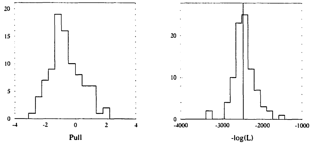
Figure 9.7: Full toy Monte Carlo results when signal events are generated using the 3-Gaussian resolution function, but the GExp resolution function is used in the fit: Left: \tau_B pull distribution. Right: -\log(\text{likelihood}) distribution. The vertical line is the value obtained from the fit to the data.
