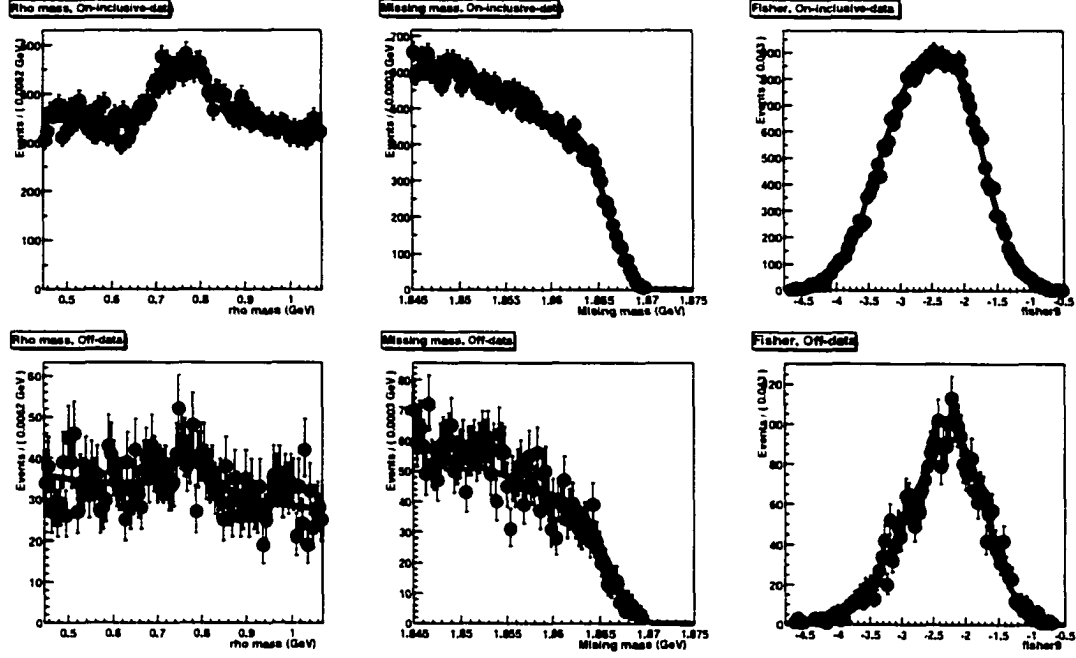
Figure 8.3: Projections of the wrong-sign kinematic variable PDF on the wrong-sign on-resonance (top) and off-resonance (bottom) data. The variables are, from left to right, m(\rho) , m_{\text{miss}} , and the Fisher discriminant.
