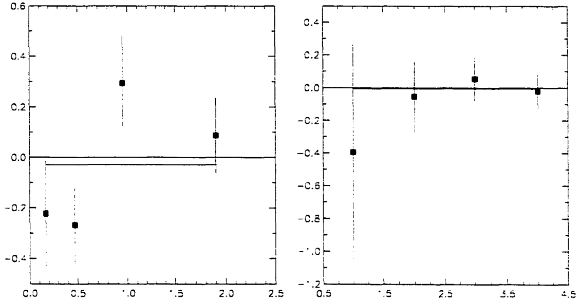
Figure 10.3: Difference from nominal \tau_B obtained when fitting the data in bins of the momentum of the \pi_f in the lab frame (left), or when separating the data by local alignment set (right). The alignment sets are 1 =A, 2 =C, 3 =D, 4 =E.
