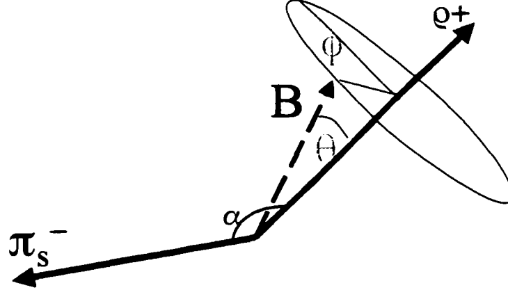
Figure 4.1: A schematic drawing to represent the decay B^0 \rightarrow D^{*-} \rho^+ . \rho is the daughter of the B^0 and the \pi_s is the daughter of the D^* . The momentum of the B^0 is known up-to an angle \theta with respect to the \rho momentum.
