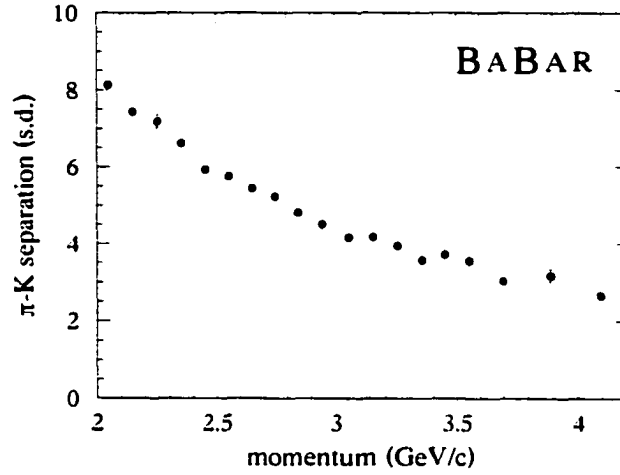
Figure A.11: DIRC \pi -K separation versus track momentum measured in D^0 \rightarrow K^-\pi^+ decays selected kinematically from inclusive D^* production.
