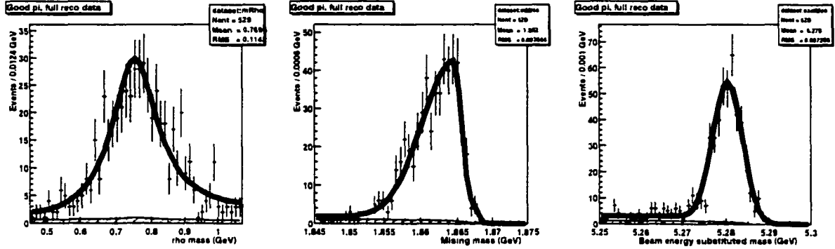
Figure 7.6: A 3-dimensional kinematic fit to fully reconstructed data. The shaded histograms show the continuum contribution. All m(\rho) , m_{\text{miss}} and m_{\text{ES}} parameters of signal events were allowed to float in the fit. m(\rho) and m_{\text{miss}} parameters of the backgrounds were fixed from fits to Monte Carlo or off-resonance data. The parameters of the m_{\text{ES}} distributions of the backgrounds ( A_1(m_{\text{ES}}) and A_2(m_{\text{ES}}) of Eq. (7.2)) were also allowed to float. The fractions of all backgrounds, except the continuum background, were fixed by the Monte Carlo yields (Fig. 7.1). The continuum fraction was allowed to float in the fit.
