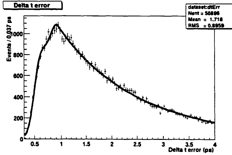
Figure 5.7: Distribution of \sigma_{\Delta t} for data. The solid line is a fit to \sigma_{\Delta t} using the Crystal Ball function plus Gaussian.
