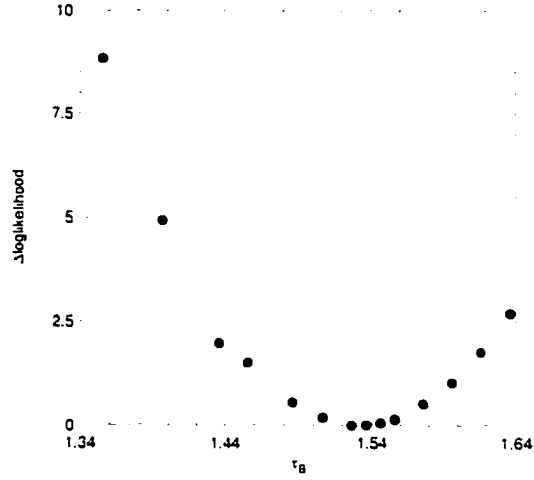
Figure 8.7: Scan of the negative log likelihood obtained from the data, as a function of \tau_B^{\text{raw}} . The minima is at the fitted value of 1.535 ps.
