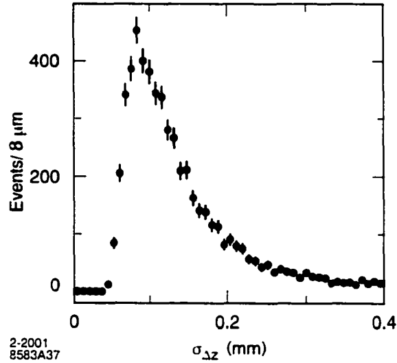
Figure 3.9: Estimated error in the difference \Delta z between the B^0 meson decay vertices for a sample of events in which one B^0 is fully reconstructed.
