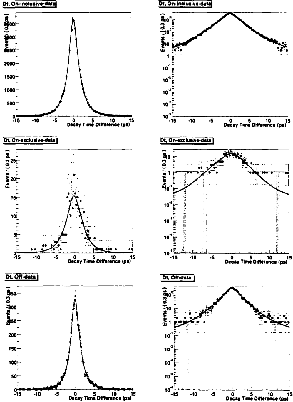
Figure 8.5: Projections of the \Delta t PDF on the partially reconstructed on-resonance data (top), fully reconstructed on-resonance data (middle), and off-resonance data (bottom). Both linear scale and log plots are shown. All events are right-sign, signal region.
