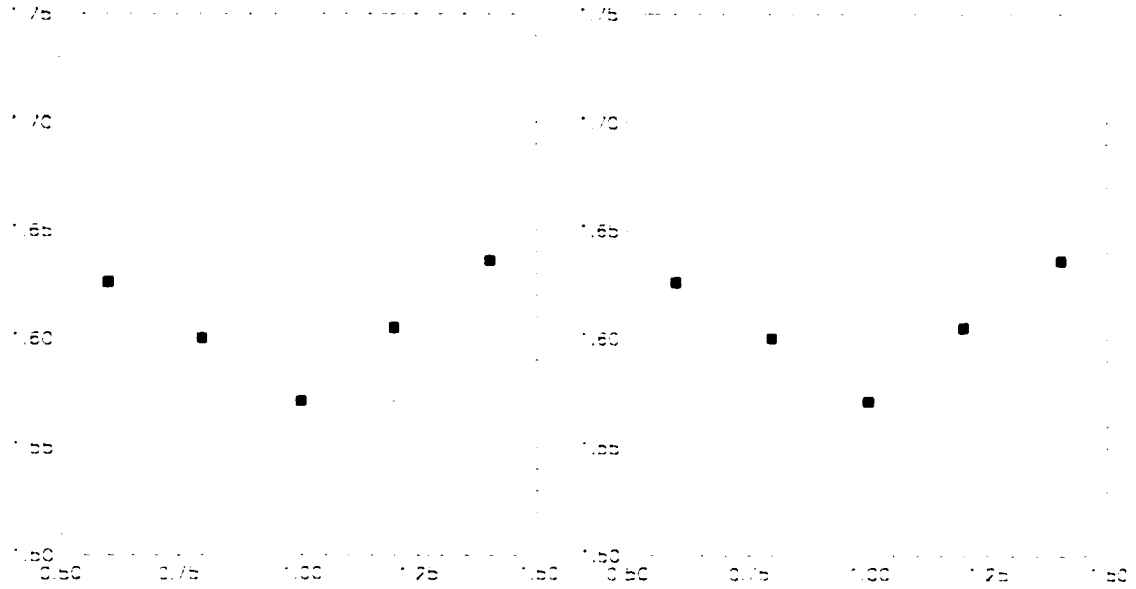
Figure 10.1: \tau_B vs. the cone cut. The errors are the \tau_B errors quoted in Tab. 10.3, subtracted in quadrature from the error of the 1-radian cone cut result. The \chi^2 probability for all the results to be in agreement is 23.3% (left). The probability for just the 0.8- and 1.2-radian cone cut results to be consistent with the 1-radian result is 55% (right).
