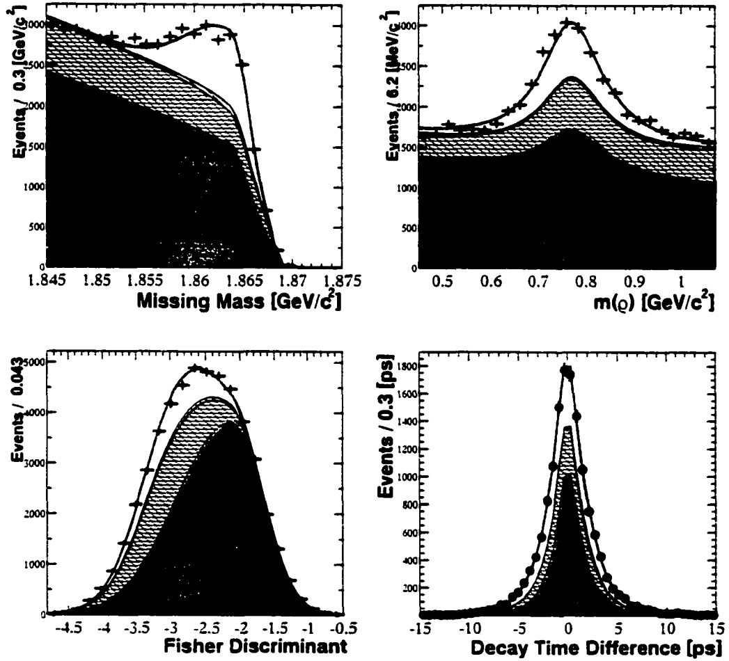
Figure 8.6: The missing mass, \rho mass, Fisher distribution and the \Delta t distribution for the on-resonance right sign events. The result of the fit is superimposed on data. The hatched, cross-hatched and shaded areas are the peaking B\bar{B} , combinatoric B\bar{B} and continuum events respectively.
