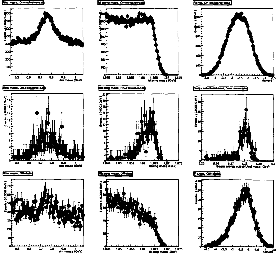
Figure 8.1: Projections of the kinematic variable PDF on the partially reconstructed on-resonance data (top), fully reconstructed on-resonance data (middle), and off-resonance data (bottom). All events are right-sign, signal region. The variables are, from left to right, m(\rho) , m_{\text{miss}} , and Fisher (for partially reconstructed and off-resonance data), or m(\rho) , m_{\text{miss}} , and m_{\text{ES}} (for fully reconstructed data).
