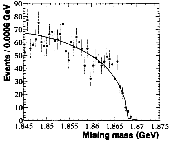
Figure 4.4: m_{\text{miss}} distribution for (combinatoric B\bar{B} ) background Monte Carlo events.
