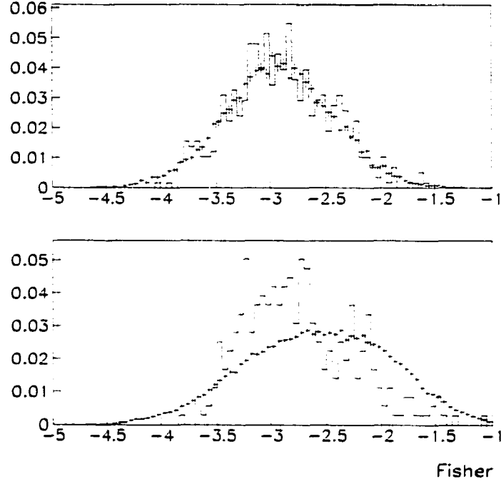
Figure 7.2: A comparison of the normalized distribution of the Fisher discriminant between the partially reconstructed events (error bars) and fully reconstructed events (histogram) in Monte Carlo (top) and data (bottom).
