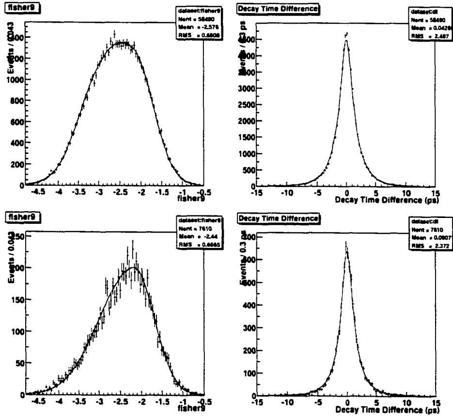
Figure 8.2: Projections of the sideband PDF on the on-resonance (top) and off-resonance (bottom) sideband data. The variables shown are the Fisher (left) and \Delta t (right).
