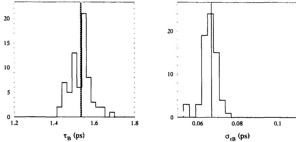
Figure 9.4: Full toy Monte Carlo results when using the GExp resolution function: Left: \tau_B distribution. The solid vertical line shows the value generated (1.534 ps), and the dashed-line indicates the mean measured value (1.531 ps). Right: Error in \tau_B . The vertical line is the value obtained from the fit to the data.
