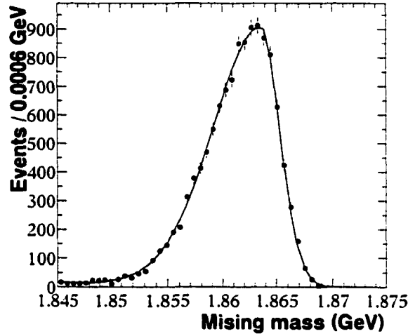
Figure 4.3: m_{\text{miss}} distribution for signal, D^*\rho , Monte Carlo events.
