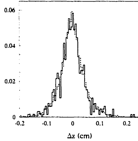
Figure 7.7: The \Delta z distribution of fully reconstructed signal Monte Carlo events (histogram) and inclusively reconstructed signal Monte Carlo events (dotted line).
