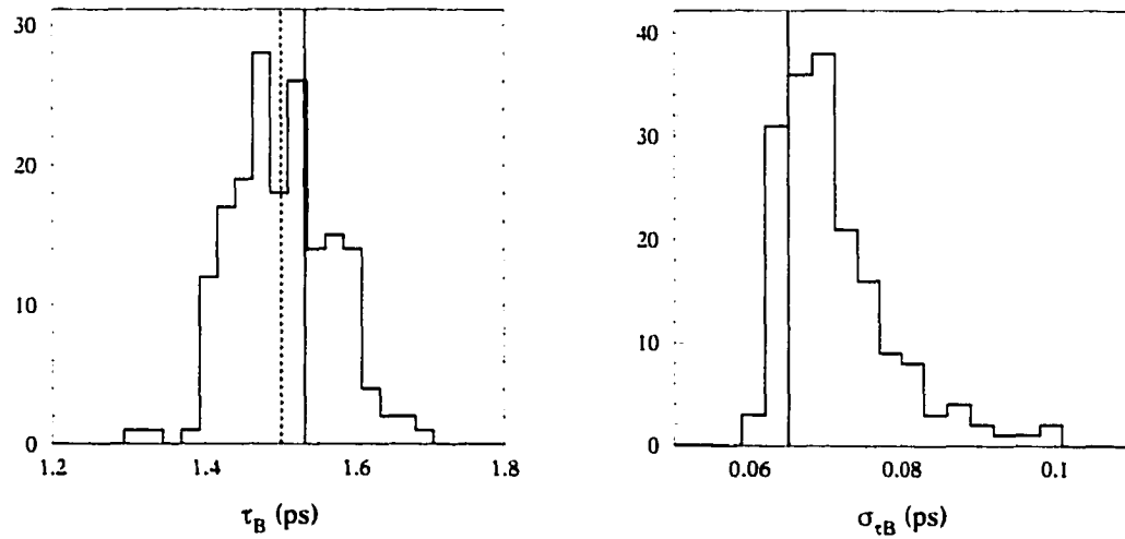
Figure 9.2: Full toy Monte Carlo results: Left: \tau_B distribution. The solid vertical line shows the value generated (1.534 ps), and the dashed-line indicates the mean measured value (1.503 ps). Right: Error in \tau_B . The vertical line is the value obtained from the fit to the data.
