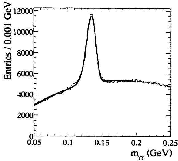
Figure 3.12: Invariant mass of two photons in a B\bar{B} events. The energies of the photons and the \pi^0 are required to be between 30 MeV and 300 MeV. The solid line is the fit to data.
