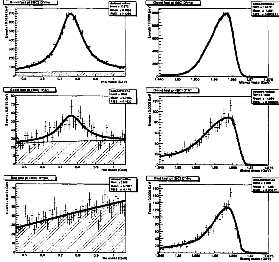
Figure 7.3: m(\rho) and m_{\text{miss}} distributions (from top to bottom) of Monte Carlo signal, B^0 \rightarrow D^{*-} a_1^+ , peaking B^0 \bar{B}^0 . The shaded region in the m(\rho) plots shows the polynomial component of the fit.
