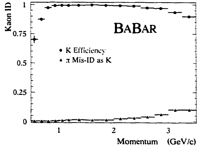
Figure A.12: Efficiency and misidentification probability for the selection of charged kaons as a function of track momentum, for a particular choice of particle selection criteria. The data use D^0 \rightarrow K^-\pi^+ decays selected kinematically from inclusive D^* production.
