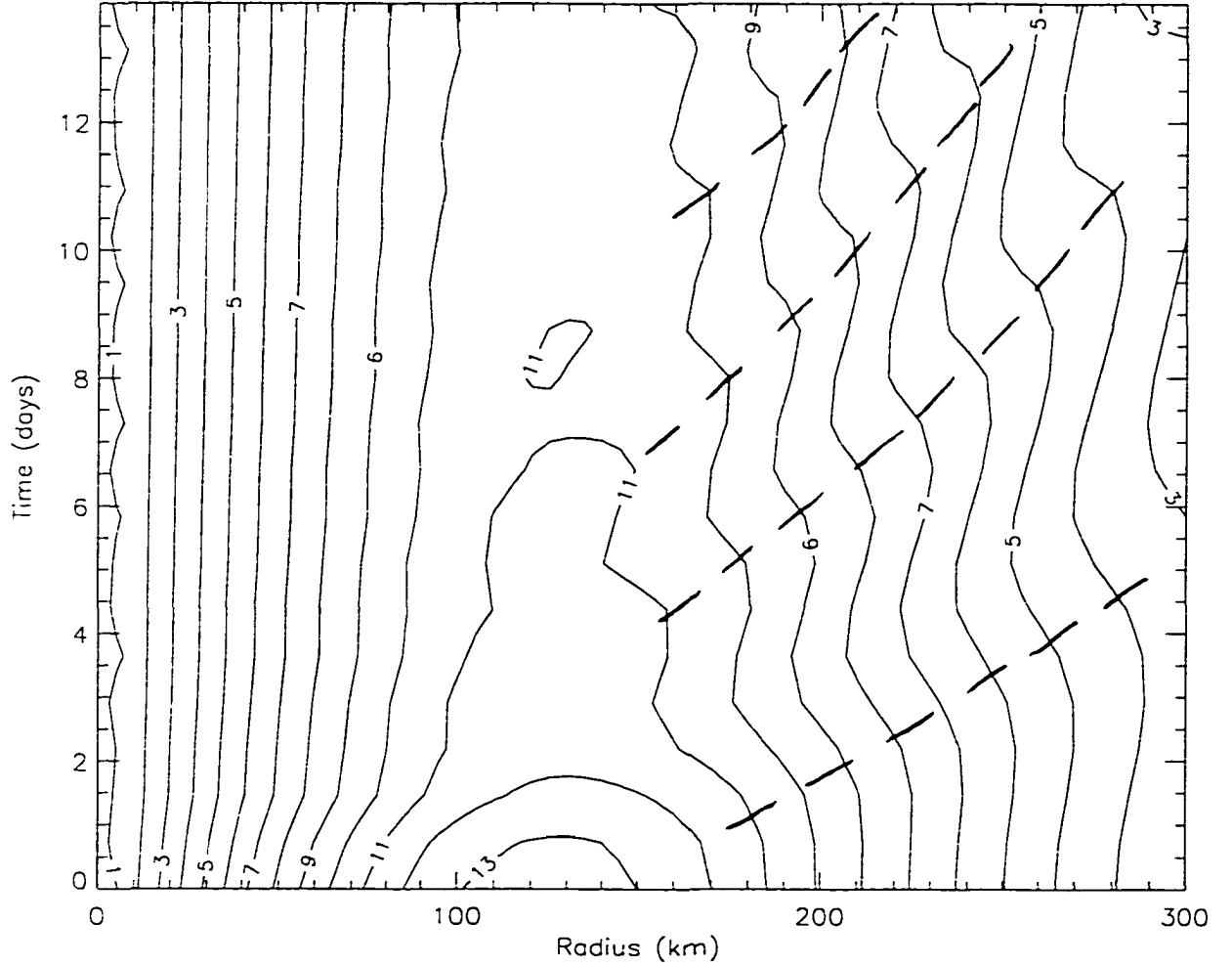
Figure 5.6: Radius-time plot of the wavenumber one PV amplitude at z = 0 over a 5\tau_e period for the benchmark run. The dashed lines denote the crest of the wave packets as they propagate radially outward in time. The quasi-discrete vortex Rossby wave persists near 130 km radius. Contour interval is 1.0 \times 10^{-6} \text{ s}^{-1} .
