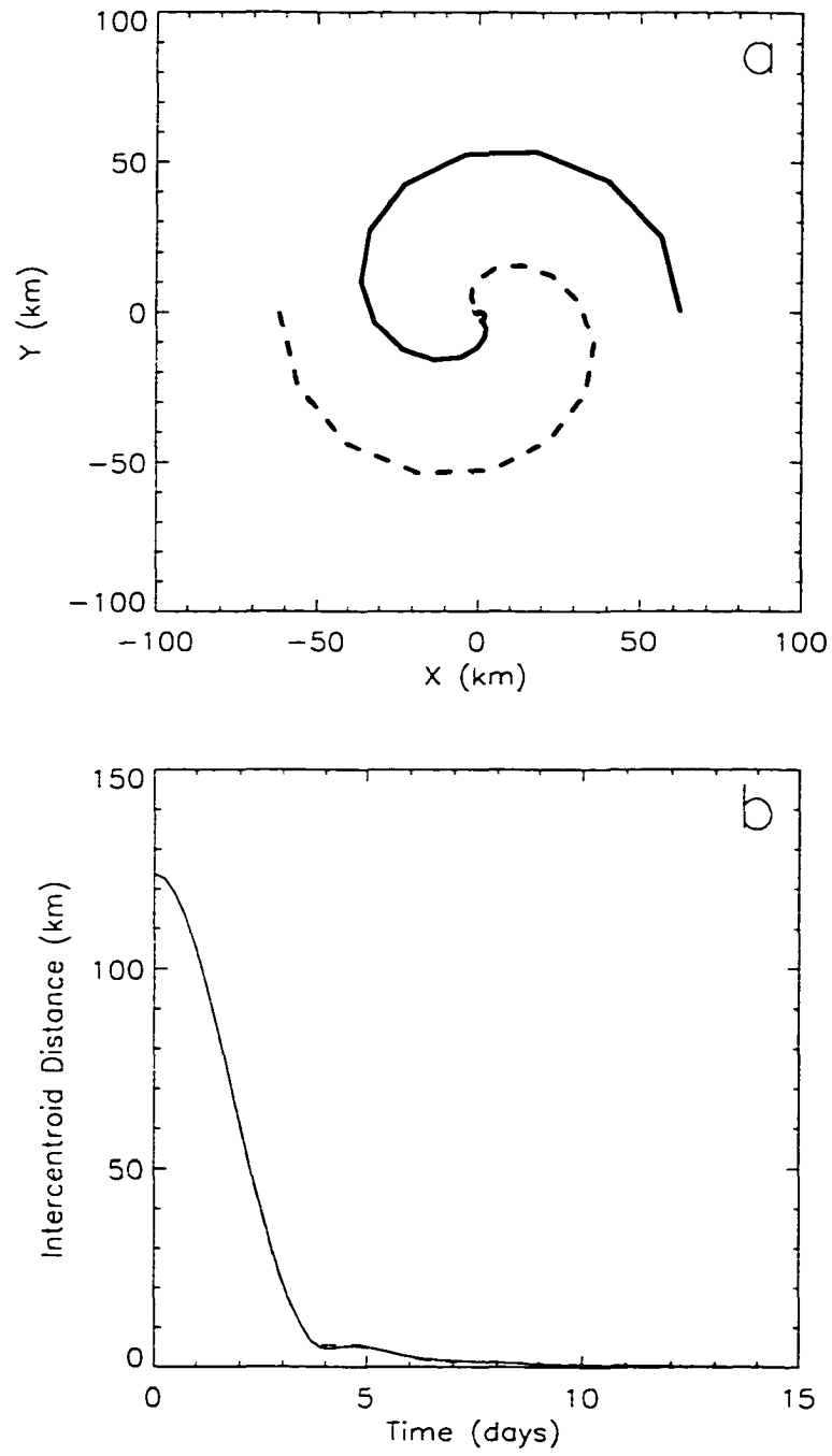
Figure 5.15: As in Fig. 5.5 but for \gamma_l = 20.0 \times 10^{-6} \text{ m}^{-1} .
