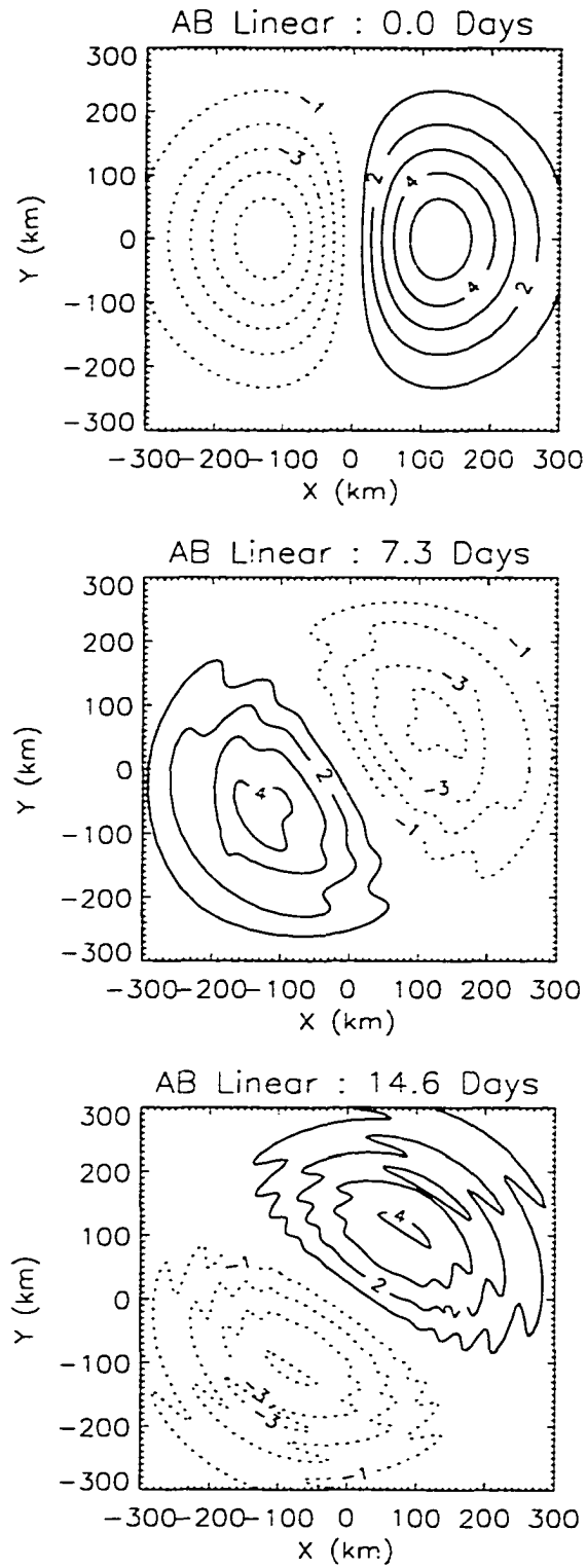
Figure 6.2: Linear equivalent barotropic AB simulation of the wavenumber one component of pseudo-PV (contour interval 1 \times 10^{-9} \text{ s}^{-3} with negative values dashed) at z = 0 over a 5\tau_e period for the benchmark run (compare with Fig. 5.5).
