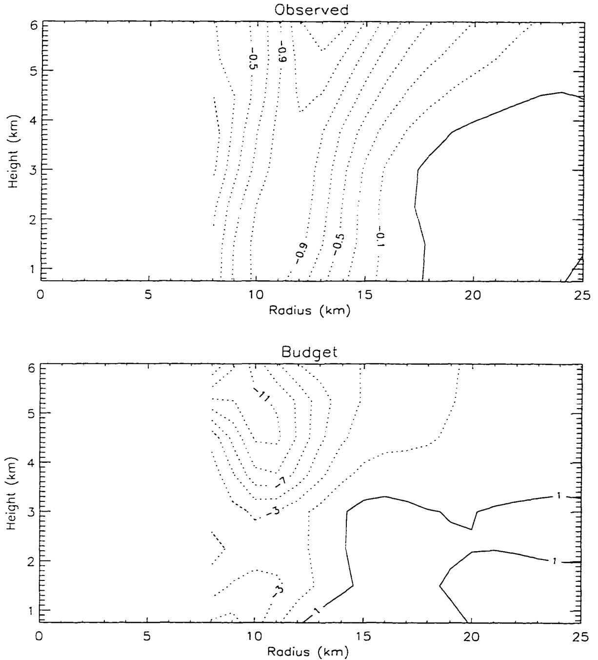
Figure 3.3: A comparison between the observed and budget tendencies of symmetric tangential wind for the transition from leg 1 to 7. Only the symmetric radial vorticity flux and vertical advection terms of Equation 3.1 are used in the budget tendency calculation. The average of the leg 1 and leg 7 wind fields are used in the budget calculation. Contour intervals for the observed and budget tendencies are 0.2 \times 10^{-3} \text{ m s}^{-2} and 2 \times 10^{-3} \text{ m s}^{-2} , respectively. Negative values are depicted by the dashed curves.
