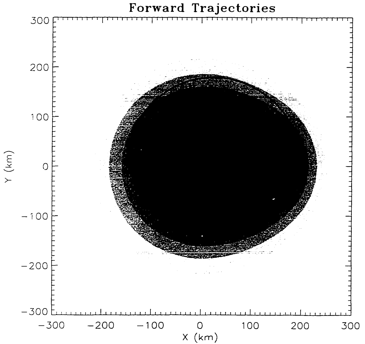
Figure 5.27: Forward Lagrangian trajectories of parcels originating within the isolated anomaly at z = 0 computed using winds simulated by the linear EQB model over 2.5\tau_e . Note that high PV is transported in towards the vortex centroid.
