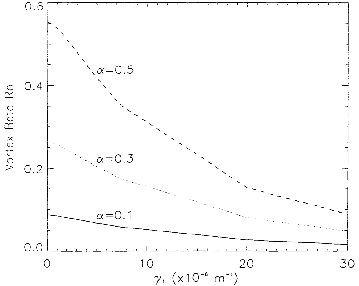
Figure 5.16: Dependence of vortex beta Rossby number at z = 0 on tilt ( \alpha ) and \gamma_1 . For consistency only (m, n) = (1, 1) is used to define the perturbation. The simulation for \alpha \approx 0.5 does contain a small barotropic wavenumber two component which will elevate R_3 slightly for all \gamma_1 .
