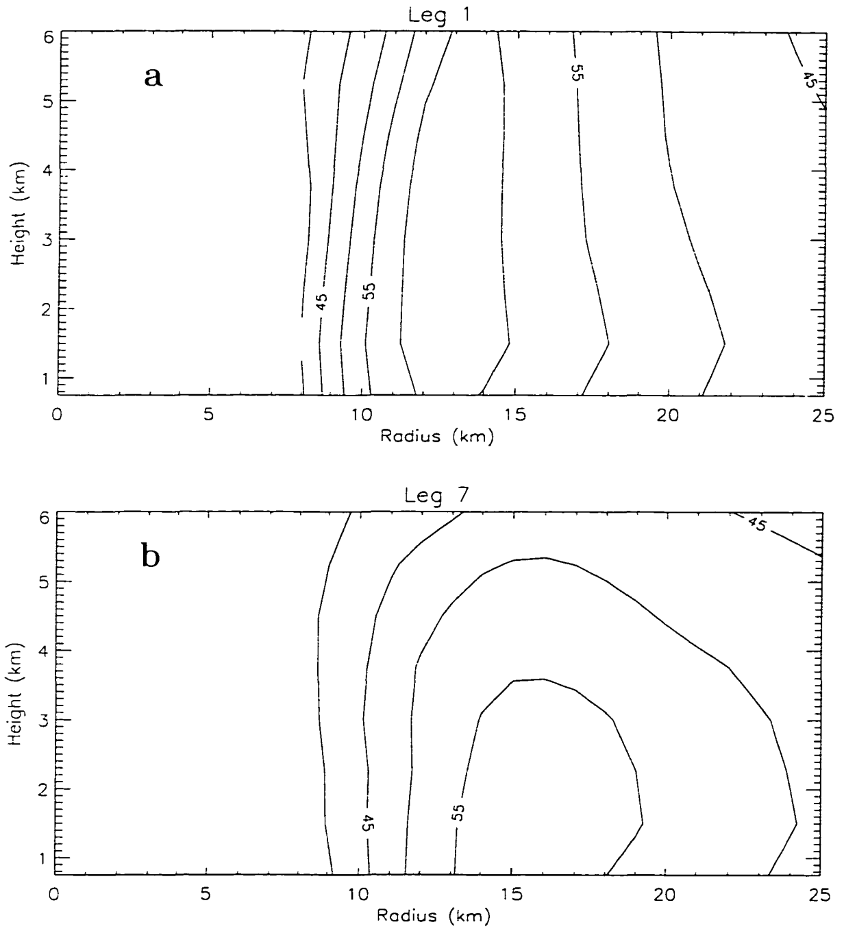
Figure 3.1: Radius-height structure of the symmetric tangential winds during (a) leg 1 and (b) leg 7. Contour interval is 5 m s -1 .
