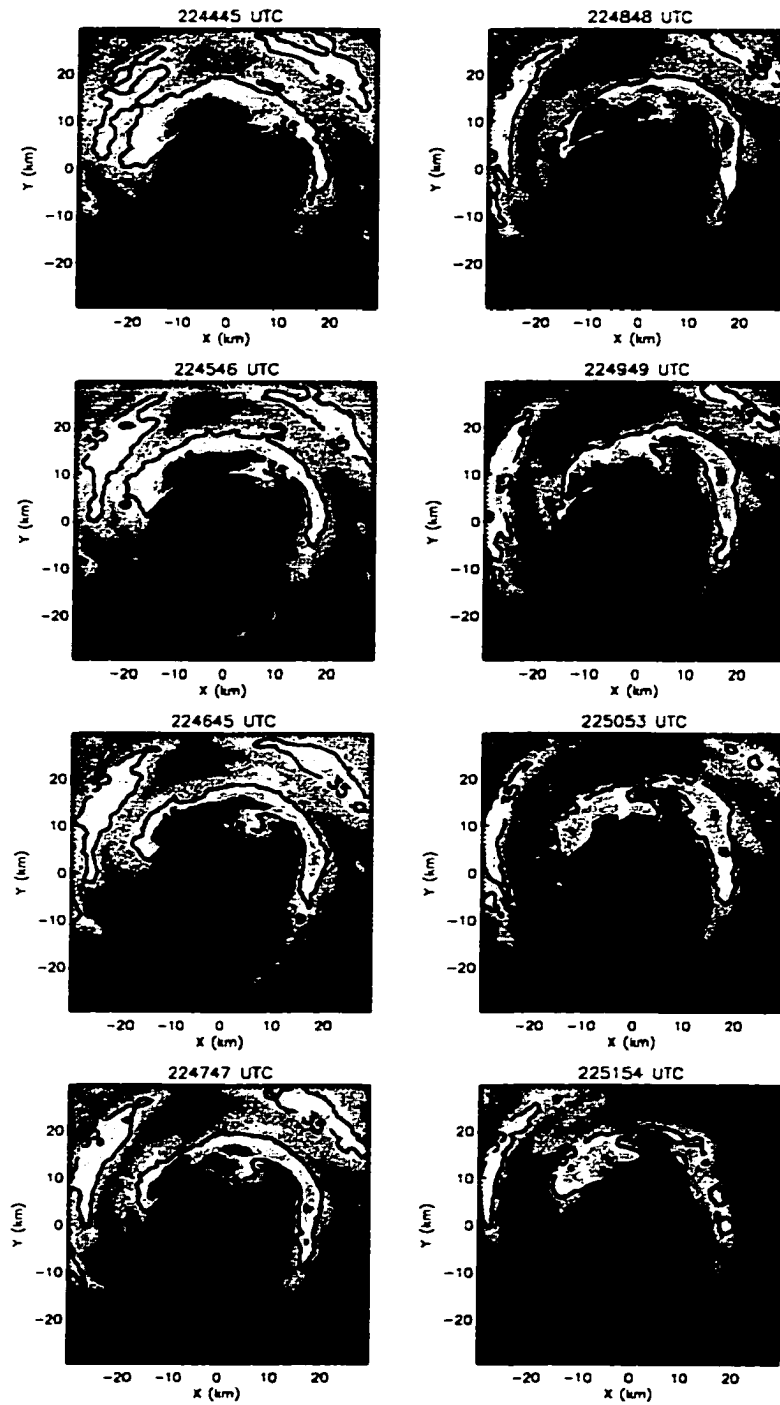
Figure 3.10: Olivia inner-core LF reflectivity composites at 3 km height. Period spanned is 2244-2251 UTC at 1 min time intervals. Contour interval is 10 dBZ.
