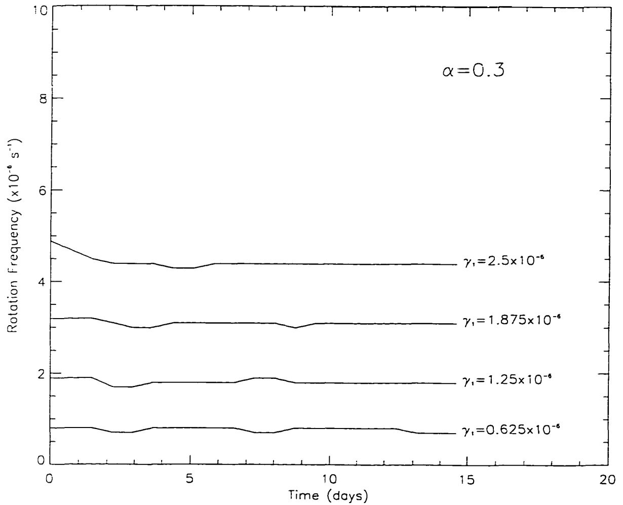
Figure 5.20: Instantaneous wavenumber one asymmetry rotation rate ( \omega ) at z = 0 for small values of \gamma_1 .
