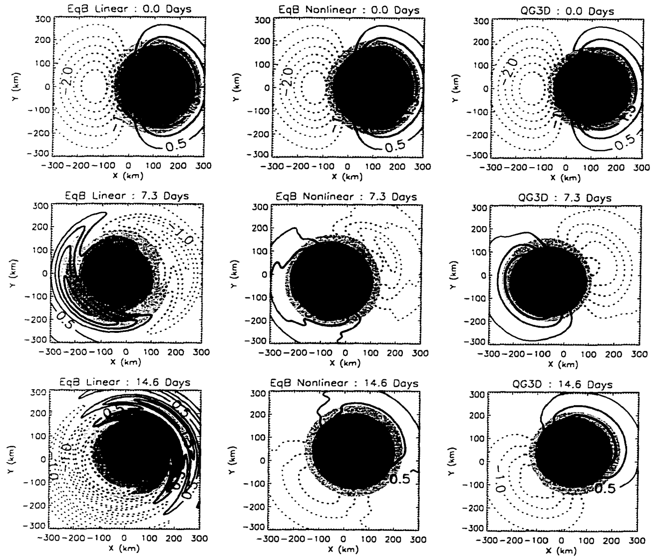
Figure 5.10: As in Fig. 5.5 but for \alpha \approx 0.5 . See text for details on the initial conditions.
