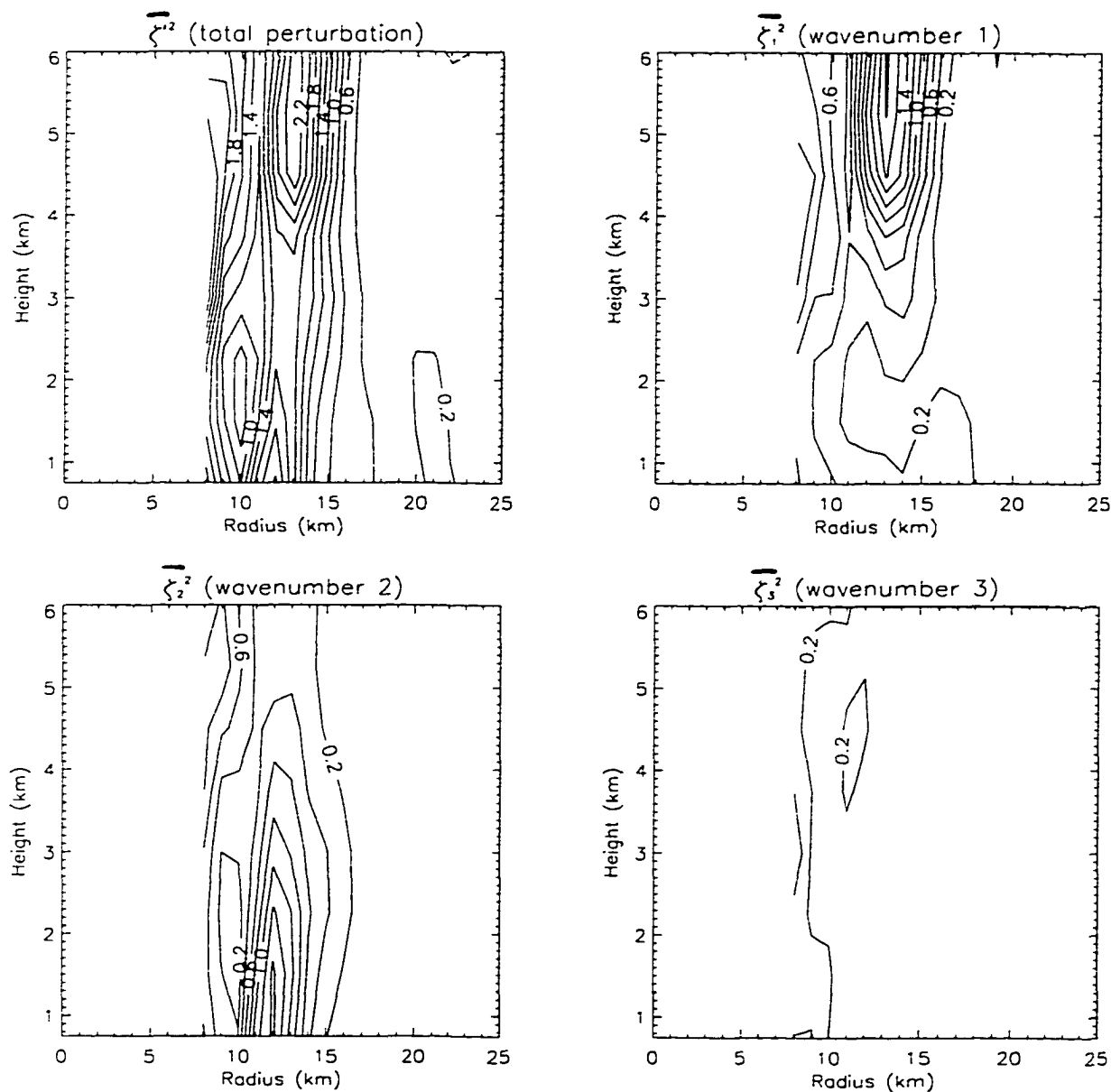
Figure 3.6: Radius-height structure of the azimuthal variance of vorticity averaged over the period 2027–2355 UTC. Also shown are individual wavenumber contributions to the azimuthal variance (i.e., wavenumber components of vorticity squared and azimuthally averaged). Contour interval is 0.2 \times 10^{-6} \text{ s}^{-2} .
