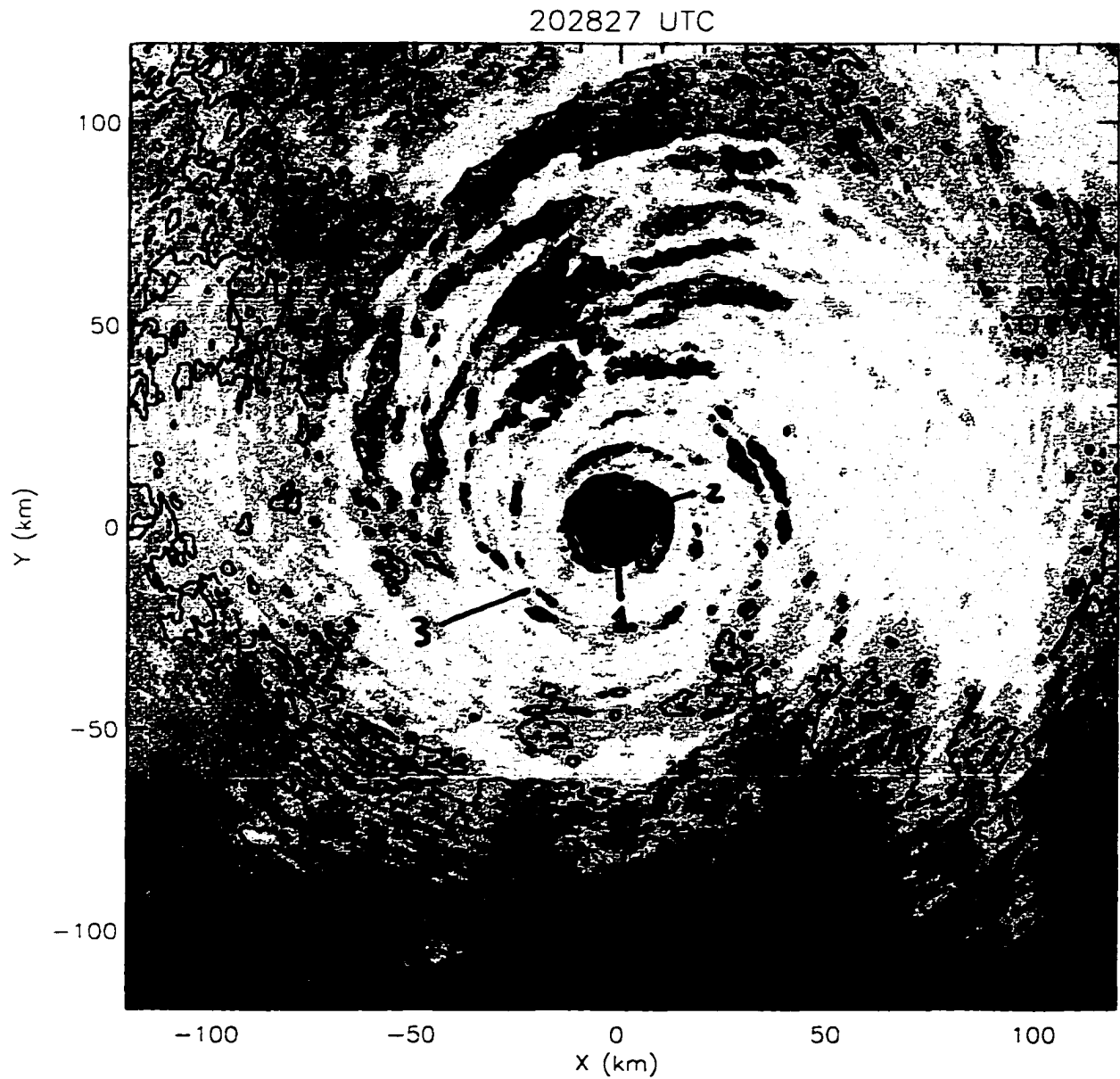
Figure 2.1: Composite of lower fuselage reflectivity from Hurricane Olivia at 2028 UTC, 25 September 1994. Contour interval is 10 dBZ. (1) The precipitation-free eye. (2) The convective eyewall. (3) The stratiform spiral rainband region.
