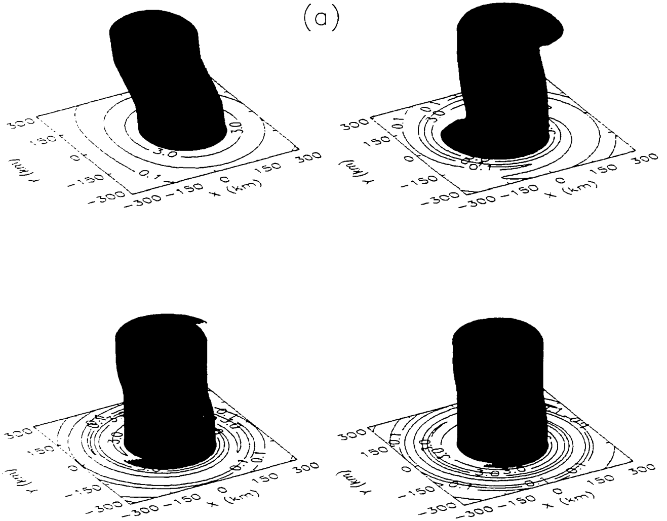
Figure 5.13: Evolution of vortex PV (from left to right) at t = 0, 1.5\tau_e, 2.5\tau_e , and 4\tau_e for \alpha = 0.3 and \gamma_1 = 20.0 \times 10^{-6} \text{ m}^{-1} . Only the inner 600 \text{ km} \times 600 \text{ km} is shown to emphasize the vortex tilt. Results from (a) the nonlinear EQB model with PV isosurface 5.0 \times 10^{-5} \text{ s}^{-1} and (b) the linear EQB model with PV isosurface 5.0 \times 10^{-5} \text{ s}^{-1} are shown. The contours shown are (0.1, 1, 3, 5) \times 10^{-5} \text{ s}^{-1} .
