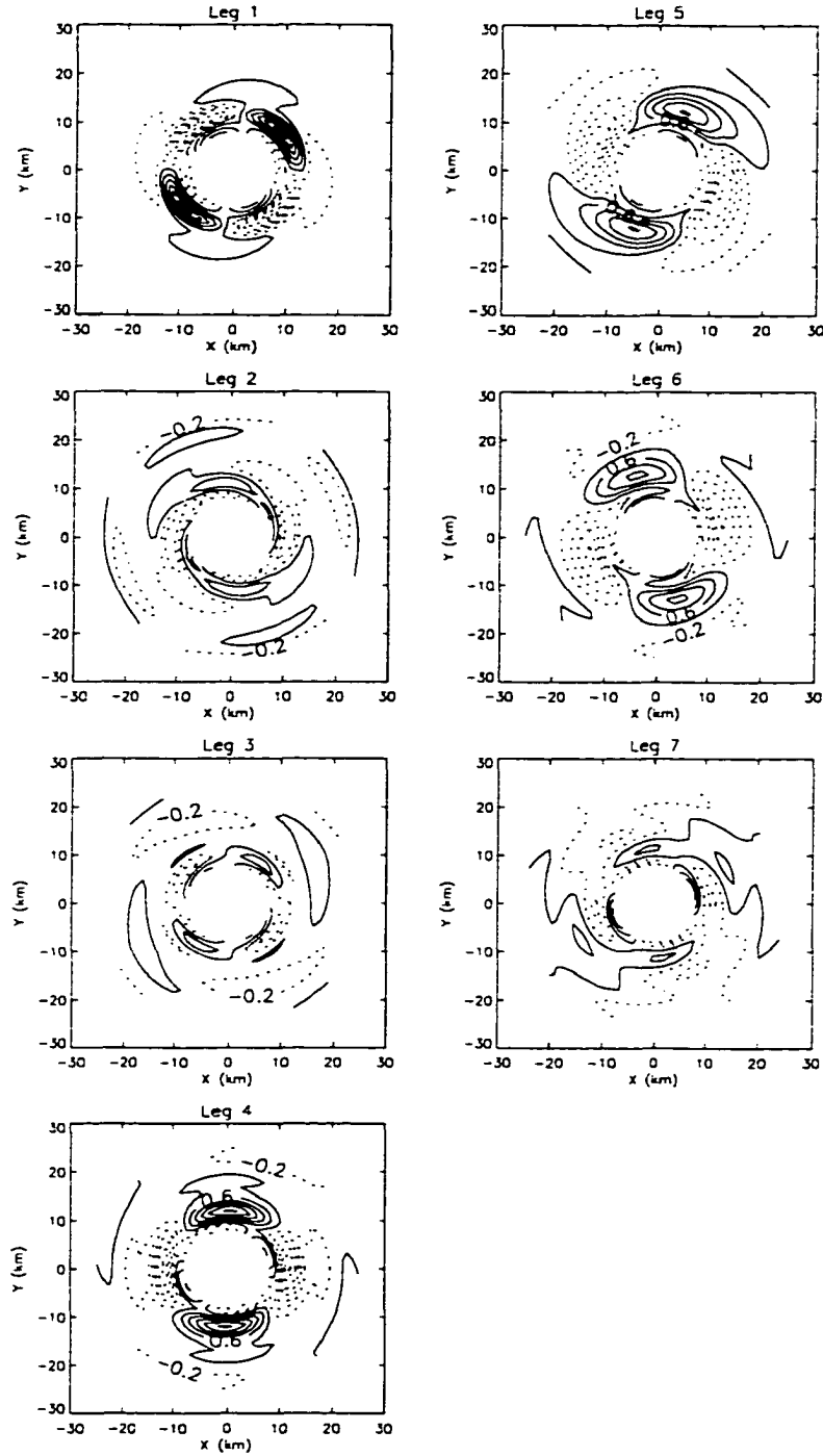
Figure 3.9: Azimuthal wavenumber 2 component of vorticity vertically averaged over the lowest 3 km for each flight leg. Contour interval is 0.4 \times 10^{-3} \text{ s}^{-1} . Negative values are depicted by the dashed curves.
