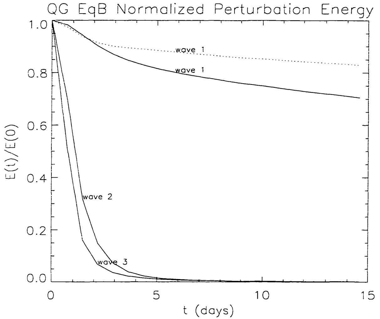
Figure 5.7: QG equivalent barotropic volume-integrated energy contained in wavenumber one from the nonlinear (dashed) and linear (solid) EQB benchmark runs as a function of time. Also shown is the linear energy evolution for initial conditions with the pseudo-mode radial structure, but azimuthal structure of wavenumbers two and three. The energy is normalized by its initial value in all cases.
