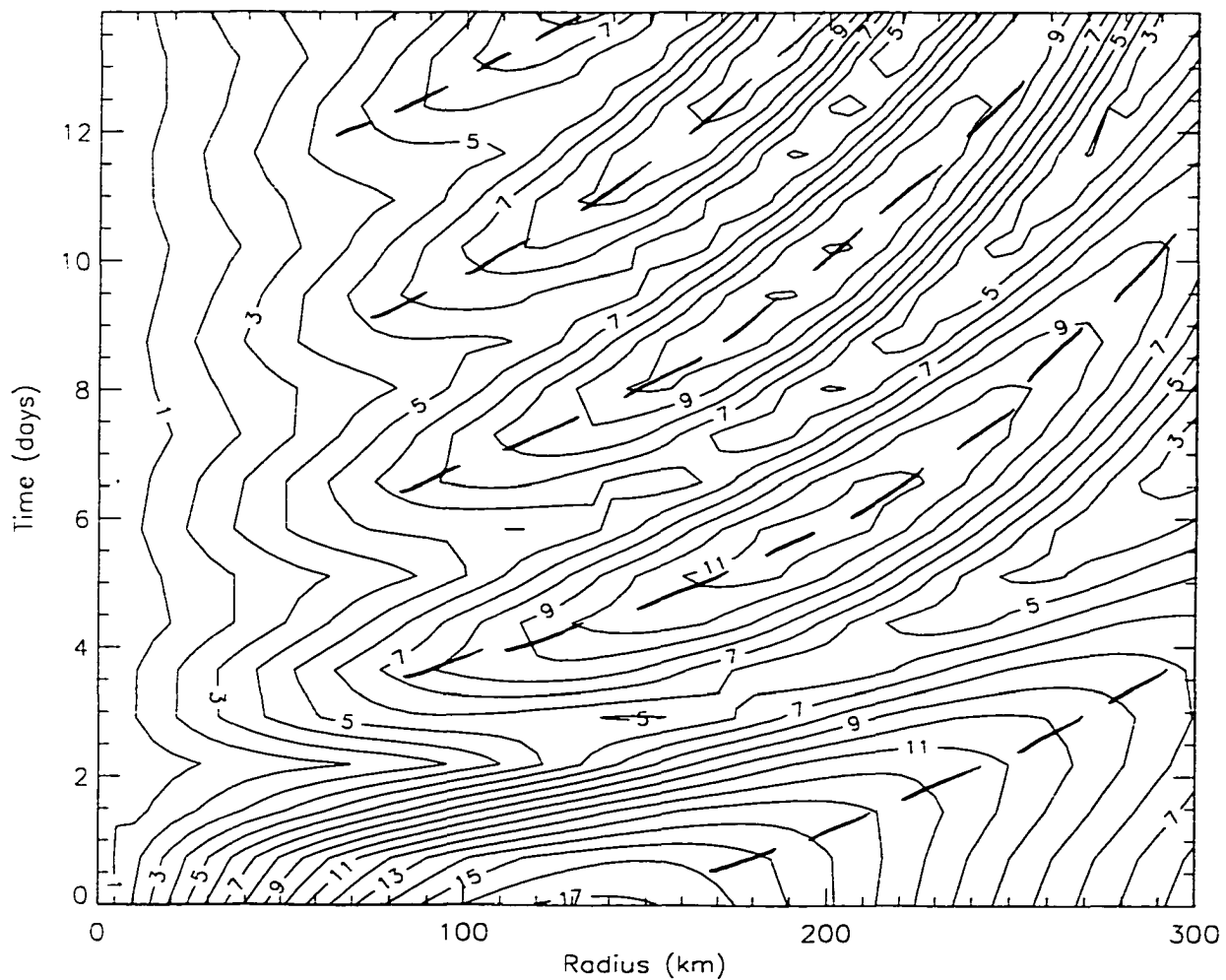
Figure 5.11: As in Fig. 5.6 but for \alpha \approx 0.5 . The radially propagating sheared vortex Rossby waves mask the quasi-discrete wavenumber one structure at early times.
