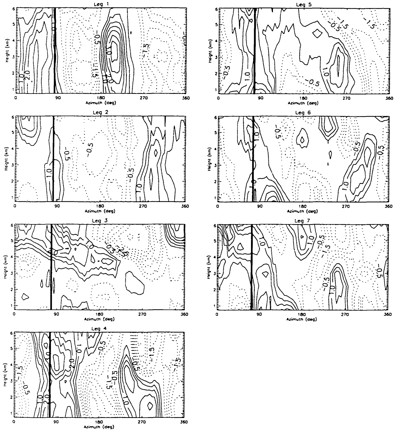
Figure 3.8: Azimuth-height cross-section of perturbation vorticity at 12 km radius from the storm center for each flight leg. North is located at 90^\circ and west is located at 180^\circ . Contour interval is 0.5 \times 10^{-3} \text{ s}^{-1} . Negative values are depicted by the dashed curves. The heavy, solid vertical line denotes the direction of storm motion.
