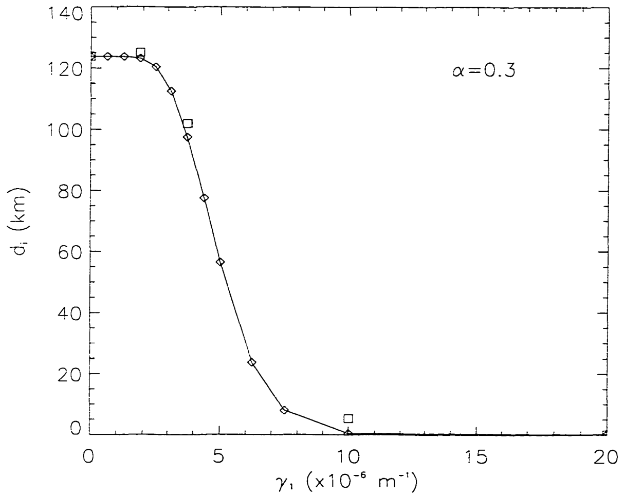
Figure 5.19: As in Fig. 5.18 but for \alpha = 0.3 .
