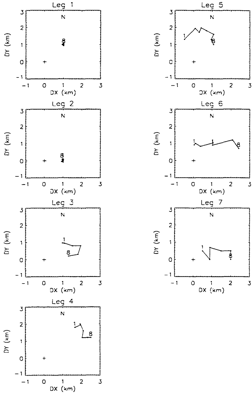
Figure 6.10: Departures of the simplex-algorithm center (●) from the flight-level center (+) as a function of height from 0.75 km to 6 km for each flight leg.
