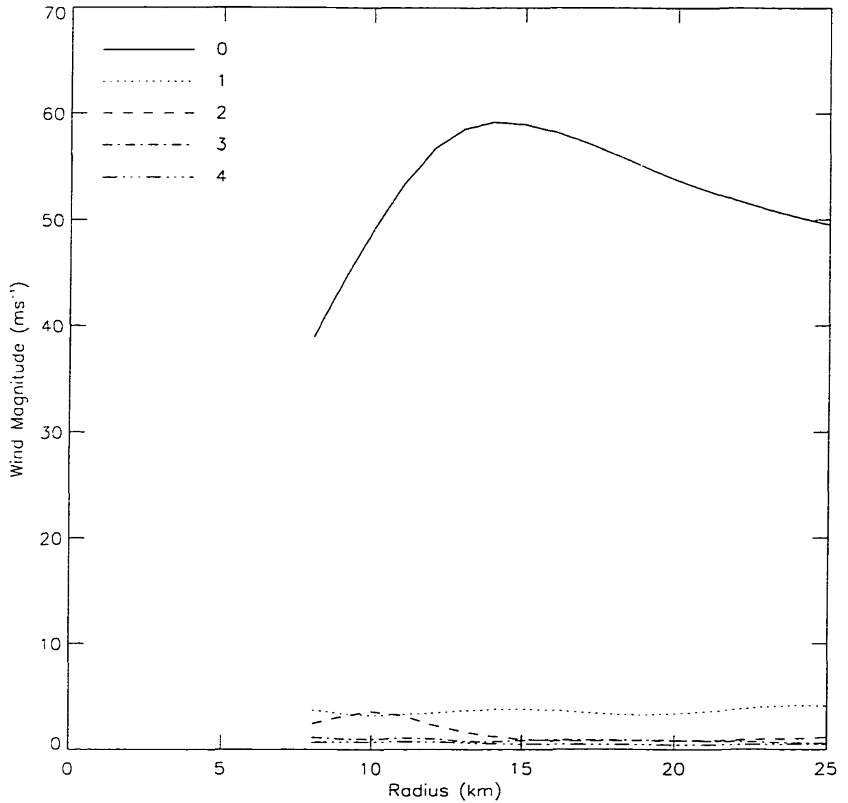
Figure 1.1: Olivia dual-Doppler derived wind magnitude ( \text{m s}^{-1} ) at 1.5 km height averaged over the observation period. Shown are the symmetric, wavenumber one, wavenumber two, wavenumber three, and wavenumber four components. The “no-scatter” region of the eye (i.e., within approximately 8 km radius) is blocked out here and in subsequent plots.
