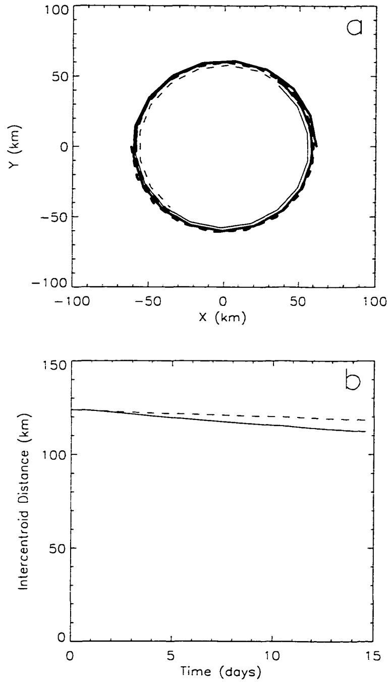
Figure 5.8: Evolution of the EQB PV intercentroid separation between z = 0 and H over 5\tau_e for the benchmark run. (a) Trajectory of the PV centroid at upper (solid) and lower (dashed) levels. The heavy lines show the nonlinear evolution, while the fine lines show the linear evolution. (b) Timeseries of intercentroid separation distance from the linear (solid) and nonlinear (dashed) models.
