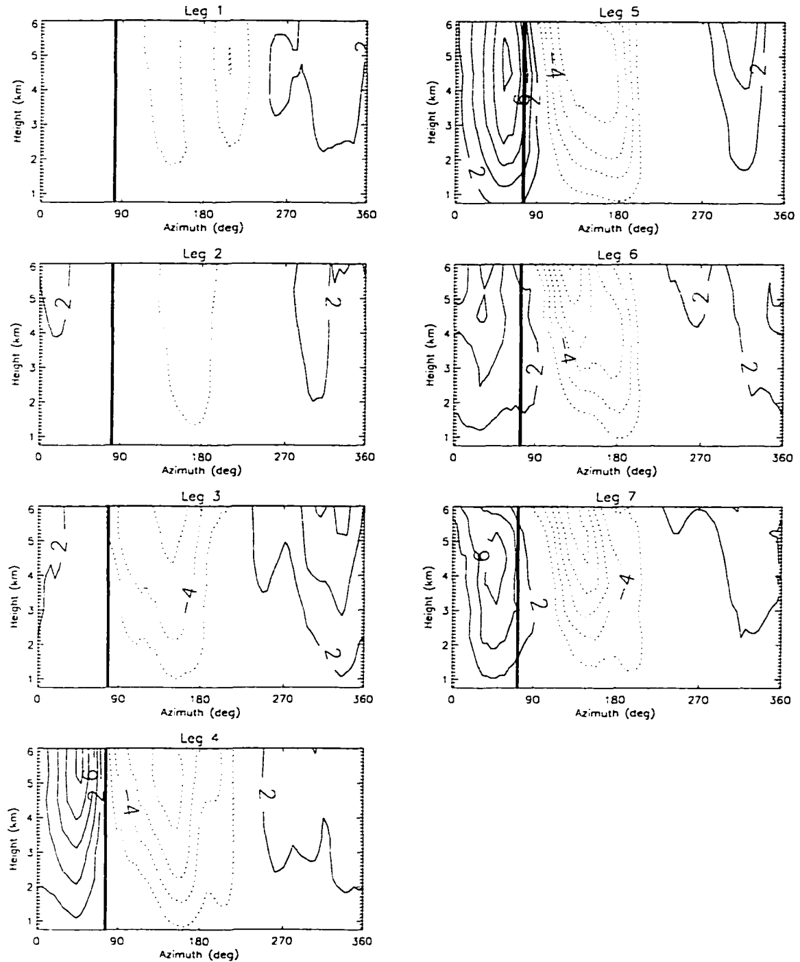
Figure 6.11: Azimuth-height cross-section of vertical velocity at 14 km radius from the storm center for each flight leg. North is located at 90^\circ and West is located at 180^\circ . Contour interval is 2 \text{ m s}^{-1} . Negative values are depicted by the dashed curves. The heavy, solid vertical line denotes the direction of storm motion.
