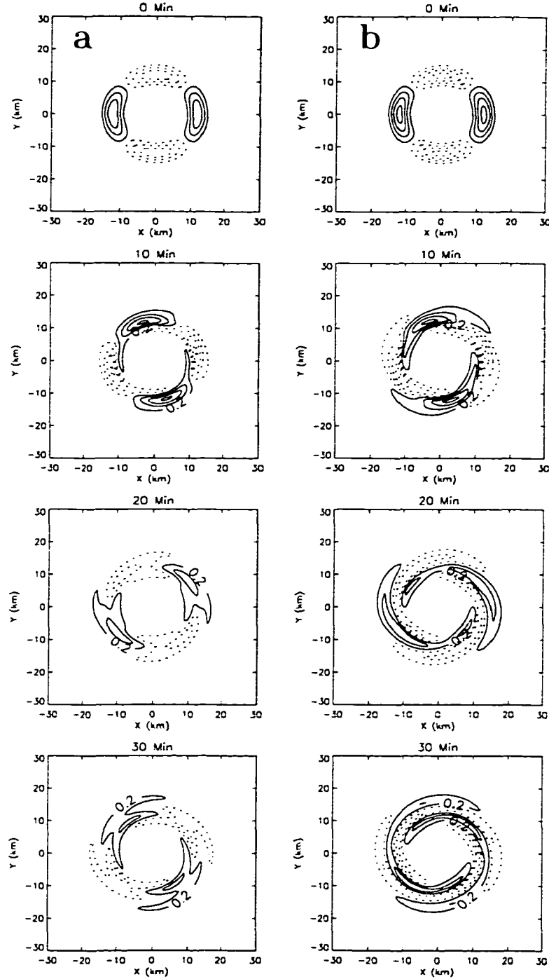
Figure 3.12: Numerical simulation of the wavenumber 2 component of vorticity for (a) Case A and (b) Case B. Contour interval is 0.4 \times 10^{-3} \text{ s}^{-1} . Initial condition is followed by snapshots of the evolution every 10 min. Negative values are depicted by the dashed curves. Also shown are numerical simulations of the total (mean plus perturbation) vorticity for (c) Case C and (d) Case D'. Contour interval is 2 \times 10^{-3} \text{ s}^{-1} . The initial condition derived from (3.6) is followed by snapshots of the evolution every 2 h, except for the last plot in the sequence which depicts the well-mixed state at 10 h.
