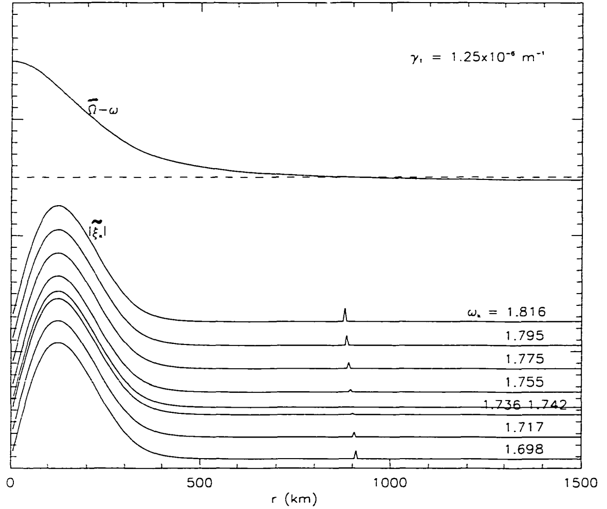
Figure 5.21: PV eigenvector solutions to Eq. 5.9 for the benchmark mean vortex and (m, n) = (1, 1) . Eigenfrequencies centered on the numerically-simulated rotation frequency are shown as well as \bar{\Omega} - \omega for the central frequency. The units of \omega are 10^{-6} \text{ s}^{-1} .
