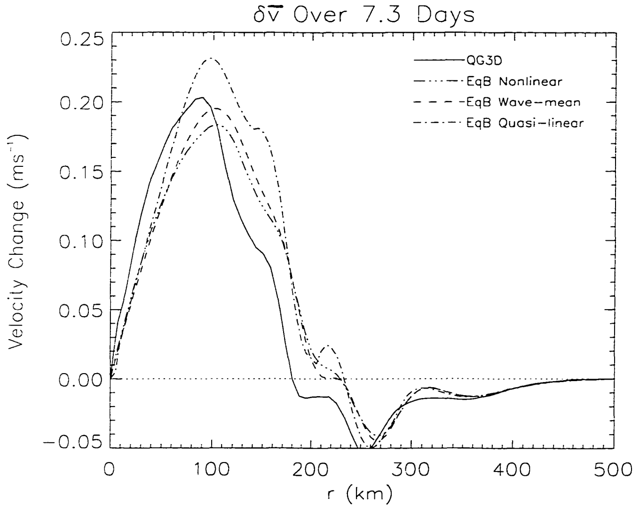
Figure 5.28: Change in azimuthal-mean tangential velocity at z = 0 over 2.5\tau_e as a function of radius for the isolated anomaly experiment. Shown are results from the QG3D and EQB models illustrating the quasi-linear nature of the low-level intensification of the mean flow by vortex Rossby waves.
