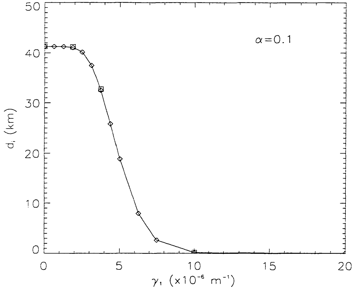
Figure 5.18: PV intercentroid separation between z = 0 and H after 5\tau_e as a function of \gamma_1 for \alpha = 0.1 . The diamonds represent linear EQB simulations and the squares nonlinear EQB simulations.
