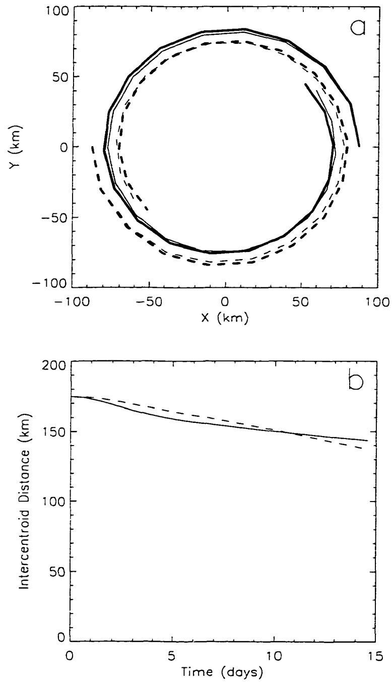
Figure 5.12: As in Fig. 5.8 but for \alpha \approx 0.5 .
