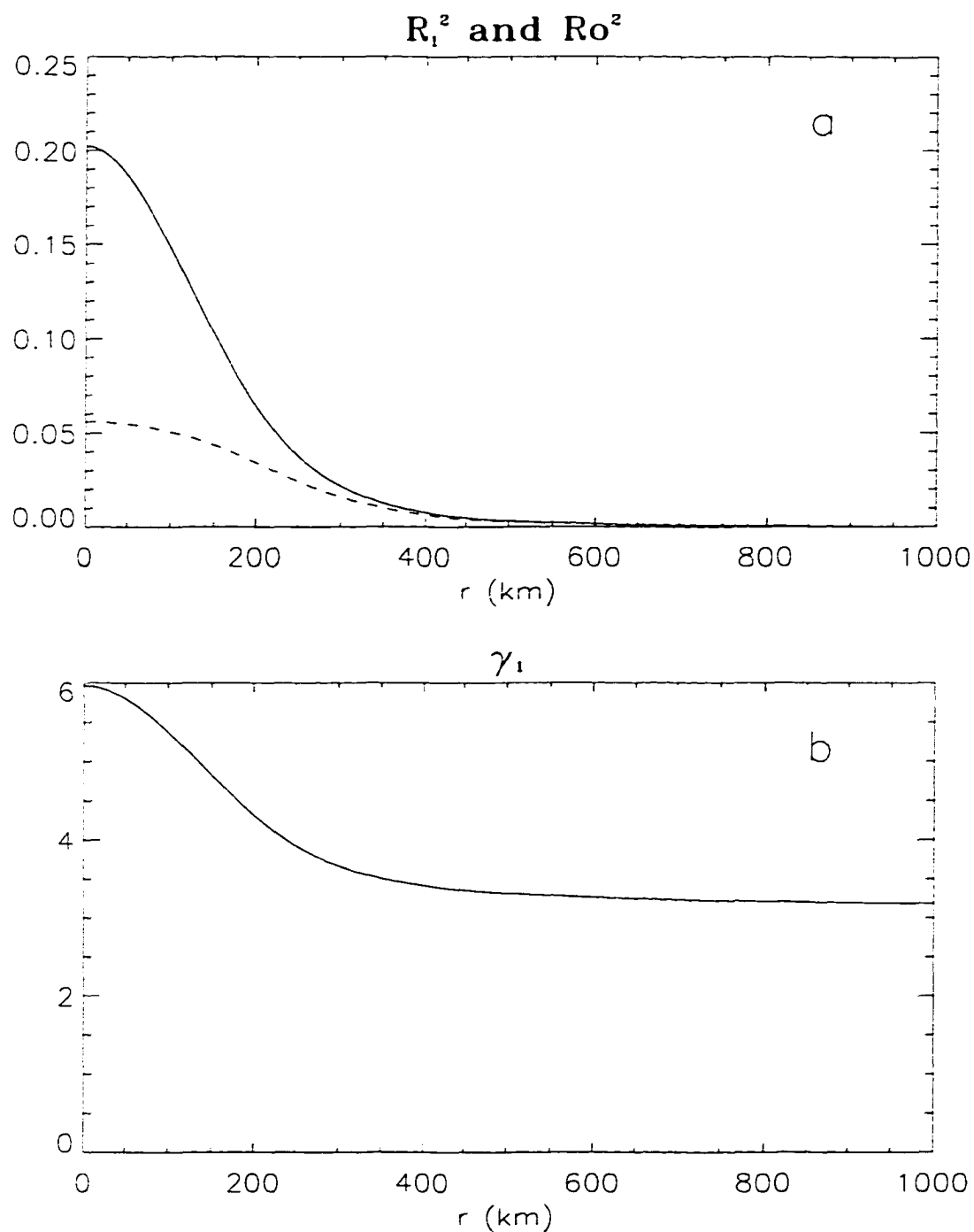
Figure 6.1: Benchmark vortex (a) Local Rossby number squared for azimuthal wavenumber one (dashed) and standard Rossby number squared (solid), and (b) inverse internal Rossby deformation radius for vertical wavenumber one (units 10^{-6} \text{ m}^{-1} ).
