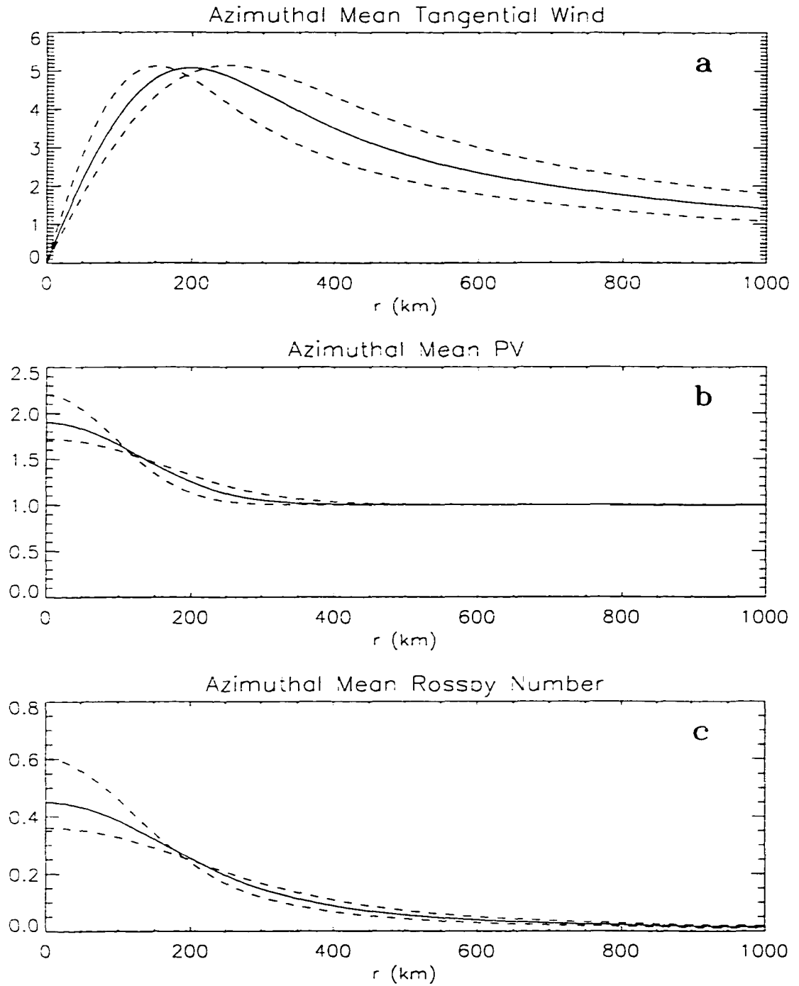
Figure 5.1: The azimuthal-mean vortex (solid) used in all simulations unless stated otherwise in the text. The vortices depicted by the dashed curves are described in Section 5.1.4. The (a) tangential wind is in units of \text{ms}^{-1} and the (b) PV is in units of 10^{-5} \text{ s}^{-1} . The (c) Rossby number is defined as \bar{\Omega}/f , where \bar{\Omega} is the azimuthal-mean angular velocity.
