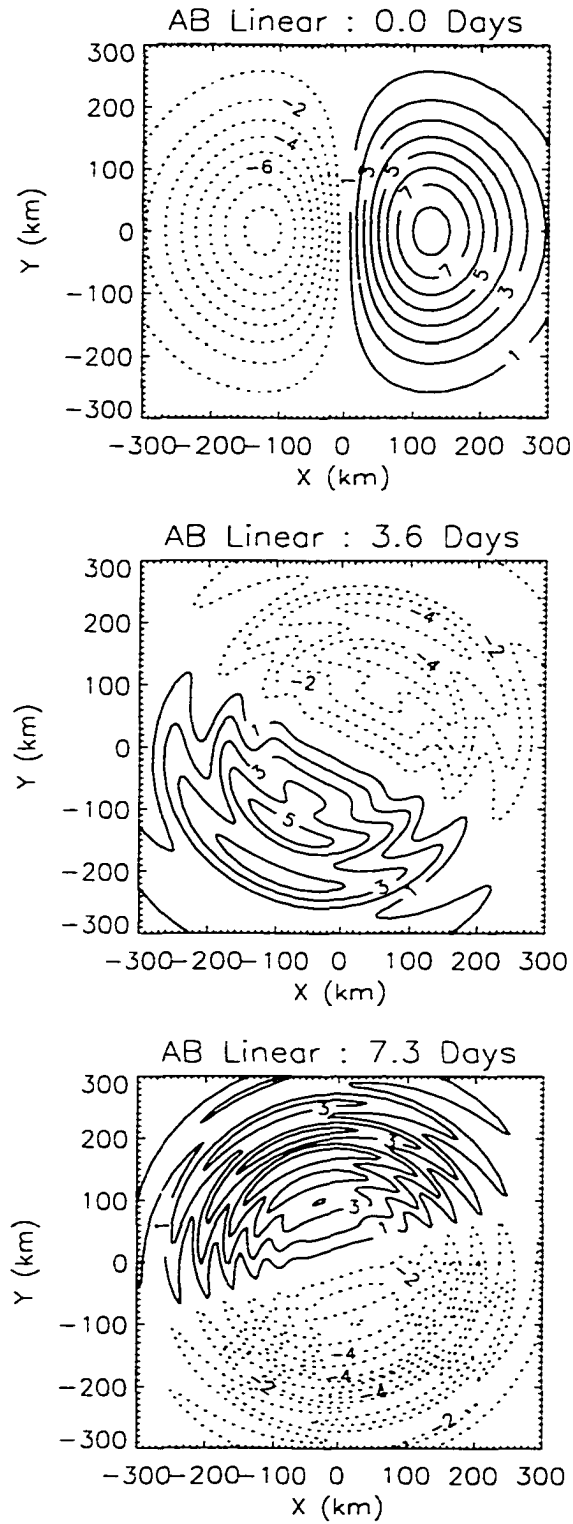
Figure 6.6: As in Fig. 6.2, but for a vortex with maximum mean tangential wind of 10 \text{ ms}^{-1} . Note that the time period considered has been reduced due to the shorter circulation period. Contour interval 1 \times 10^{-9} \text{ s}^{-3} .
