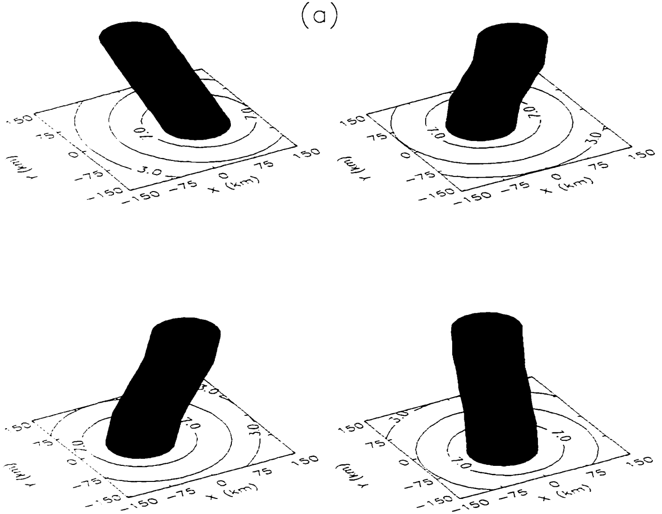
Figure 5.2: Evolution of vortex PV (from left to right) at t = 0, 1.5\tau_e, 2.5\tau_e , and 4\tau_e for the benchmark run with \alpha = 0.3 and \gamma_1 = 3.14 \times 10^{-6} \text{ m}^{-1} . Only the inner 300 \text{ km} \times 300 \text{ km} is shown to emphasize the vortex tilt. The vertical depth is 10 \text{ km} . Results from (a) the QG3D model with PV isosurface 8.0 \times 10^{-5} \text{ s}^{-1} and (b) the nonlinear EQB model with PV isosurface 8.5 \times 10^{-5} \text{ s}^{-1} are shown. The different initial conditions are described in the text. Contour interval is 2.0 \times 10^{-5} \text{ s}^{-1} .
