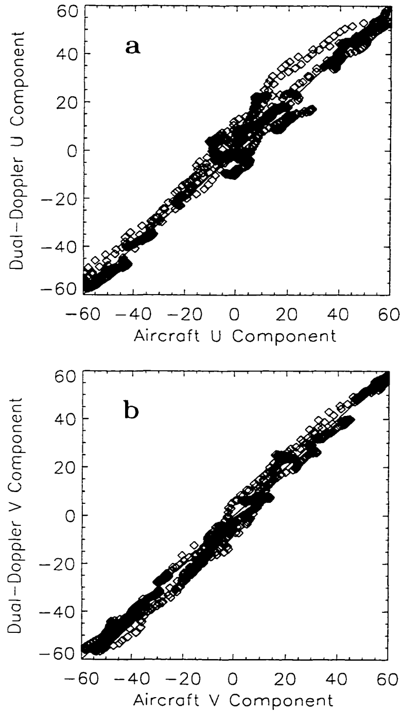
Figure 2.3: Point-by-point comparison between aircraft wind measurements at 3 km height during the period 2027–2355 UTC and the Doppler-derived wind estimates nearest in space. The (a) zonal and (b) meridional components of the wind ( \text{m s}^{-1} ) are shown separately. Interpolated data within Olivia’s eye are included in the comparison.
