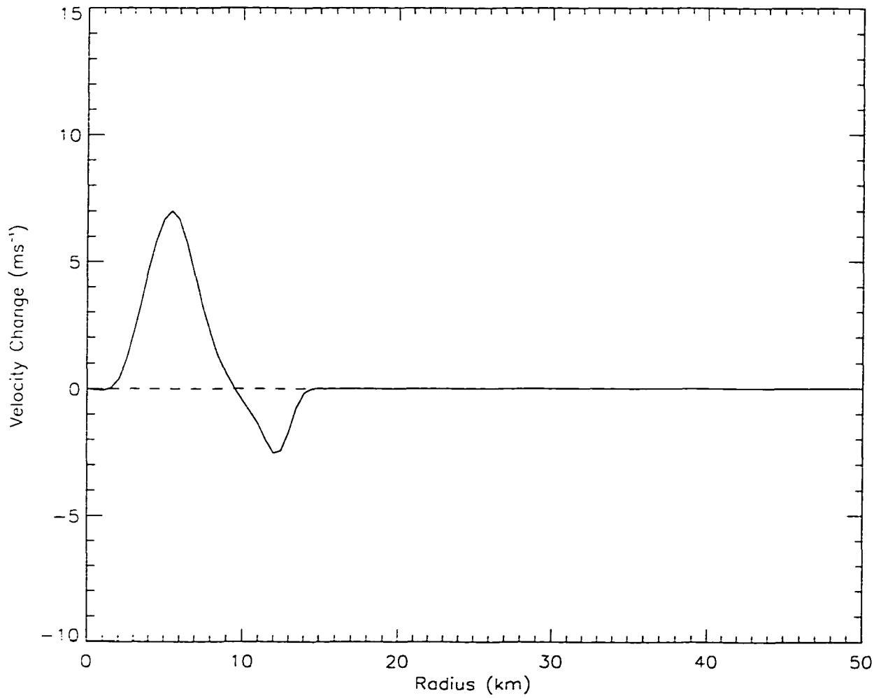
Figure 3.14: Symmetric tangential wind change ( \text{ms}^{-1} ) over the first four hours of the Case C simulation.
