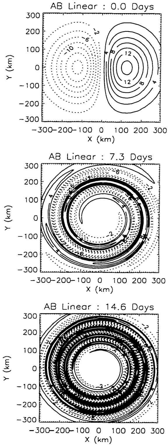
Figure 6.3: As in Fig. 6.2, but for a larger value of f = 4.0 \times 10^{-4} \text{ s}^{-1} . Contour interval 2 \times 10^{-9} \text{ s}^{-3} .
