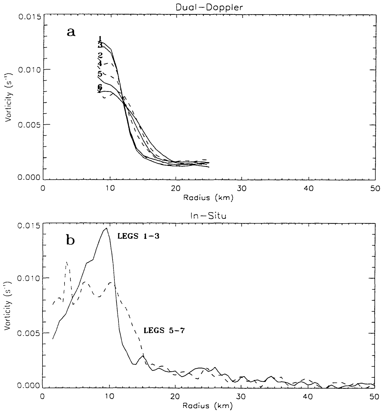
Figure 3.5: Symmetric vorticity ( s^{-1} ) profiles at 3 km height (a) derived from the dual-Doppler analysis (legs 1-7) and (b) computed from aircraft wind measurements averaged over the first three legs (1-3) and last three legs (5-7). For the latter profile, only leg 7 data is used inside 6 km, resulting in a somewhat noisier vorticity distribution.
