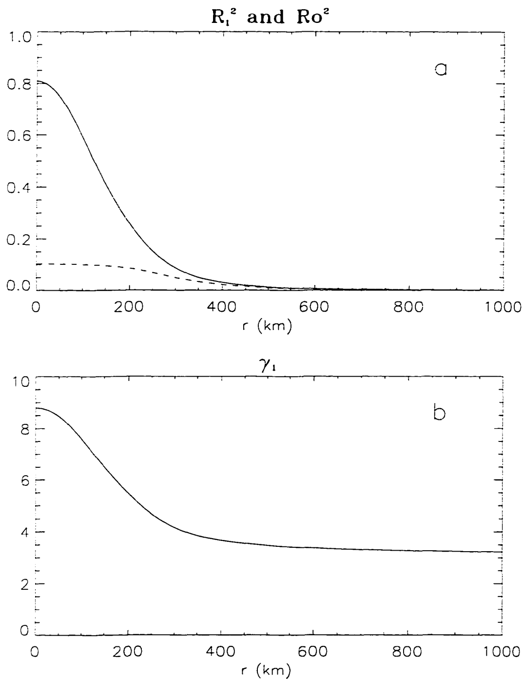
Figure 6.5: As in Fig. 6.1, but for a stronger vortex with maximum tangential wind of 10 \text{ ms}^{-1} .
