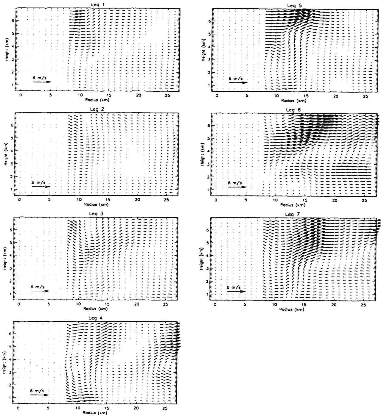
Figure 3.2: Radius-height structure of the symmetric transverse flow (u, w) for each flight leg. Wind vectors of the same length, pointing horizontally or vertically, represent the same speed. Maximum wind vector is 6 \text{ m s}^{-1} .
