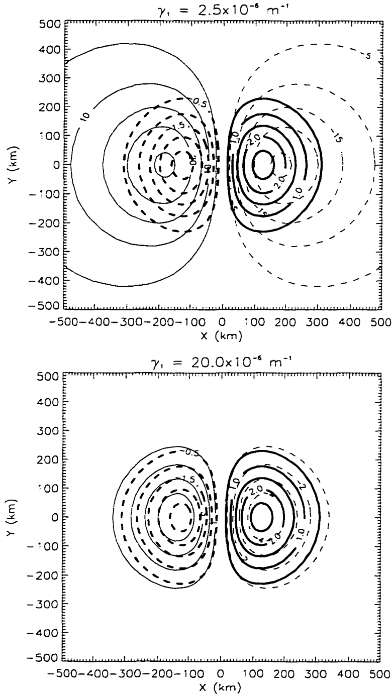
Figure 5.17: Comparison of the initial perturbation PV (heavy) and streamfunction (light) for the benchmark run. Negative values are dashed. (a) \gamma_1 = 2.5 \times 10^{-6} \text{ m}^{-1} (b) \gamma_1 = 20.0 \times 10^{-6} \text{ m}^{-1} . The perturbation PV and streamfunction isolines become more parallel with increasing \gamma_1 . Note also that the perturbation streamfunction amplitude decreases with increasing \gamma_1 . PV contour interval is 0.5 \times 10^{-5} \text{ s}^{-1} . Streamfunction contour interval is 5 \times 10^4 \text{ m}^2 \text{ s}^{-1} in (a) and 1 \times 10^4 \text{ m}^2 \text{ s}^{-1} in (b).
