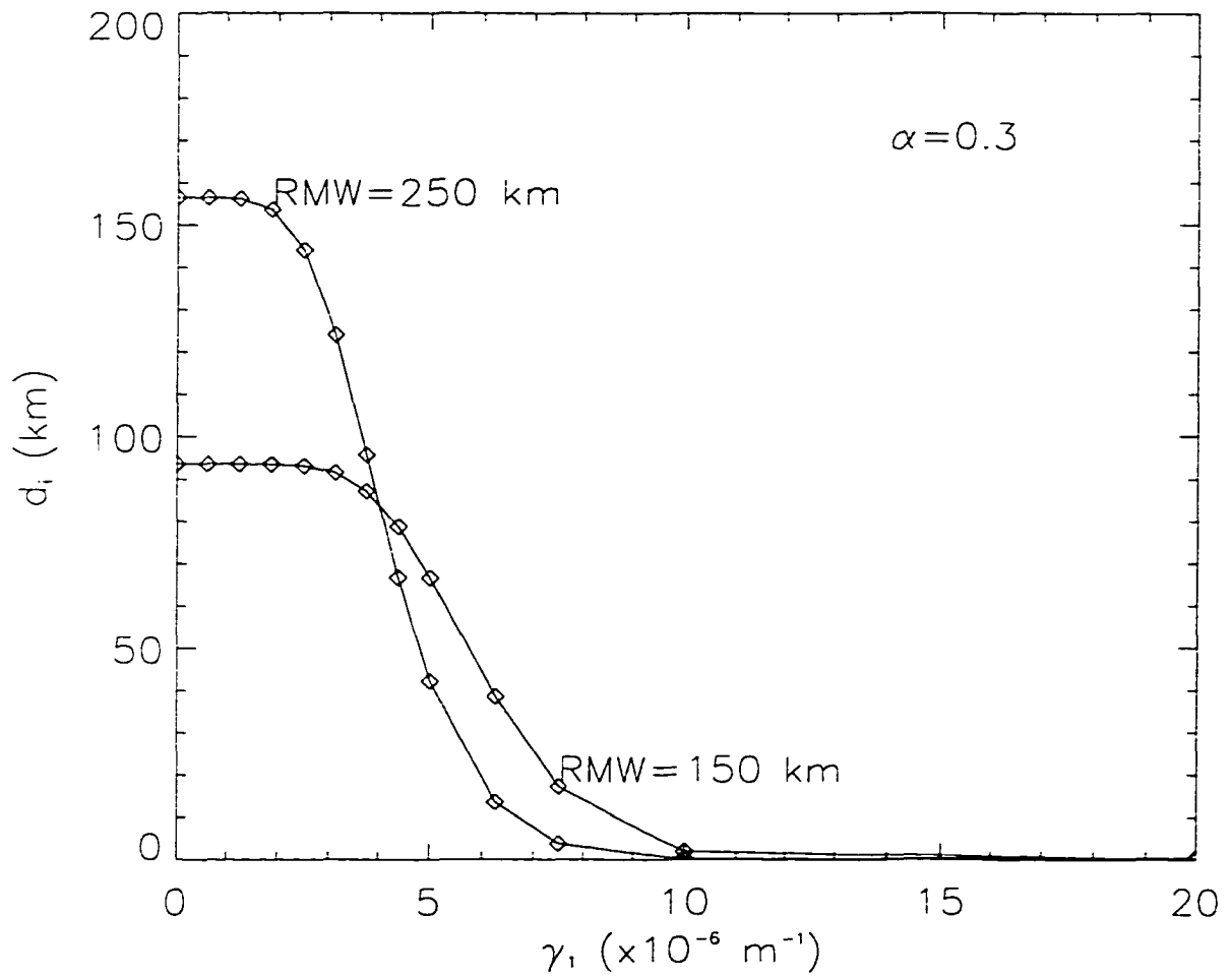
Figure 5.23: As in Fig. 5.19 but for mean vortices smaller and larger than the benchmark vortex.
