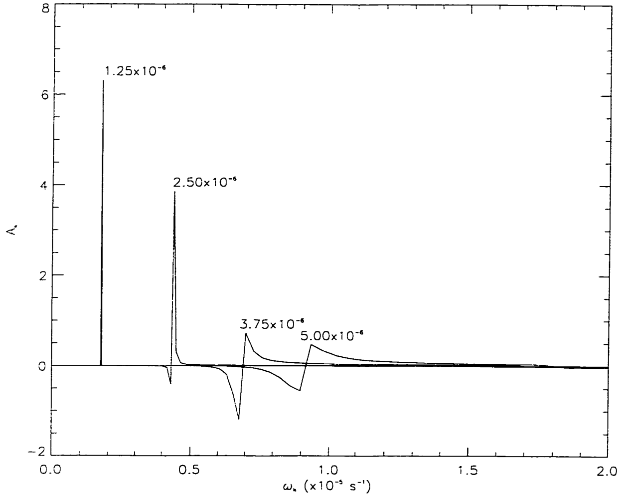
Figure 5.22: Expansion coefficient A_k as a function of eigenfrequency \omega_k for values of \gamma_1 in the quasi-mode and transition regimes. The wave one asymmetry given by Eq. 5.3 and eigenvectors shown in Fig. 5.21 were used to obtain A_k .
