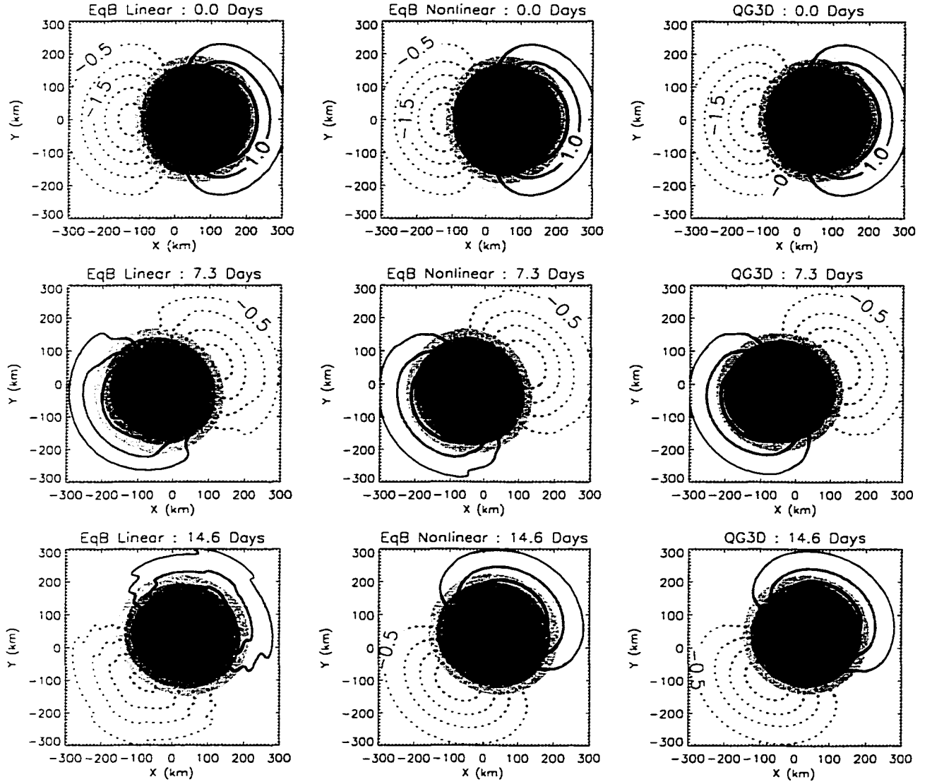
Figure 5.5: Evolution of total vortex PV (shaded) and wavenumber one component of PV (contour interval 0.5 \times 10^{-5} \text{ s}^{-1} with negative values dashed) at z = 0 over a 5\tau_e period for the benchmark run (see Fig. 5.2). From left to right are shown the results from the linear EQB, non-linear EQB, and QG3D models, respectively. Aside from the PV correction in the QG3D model, the initial conditions are identical.
