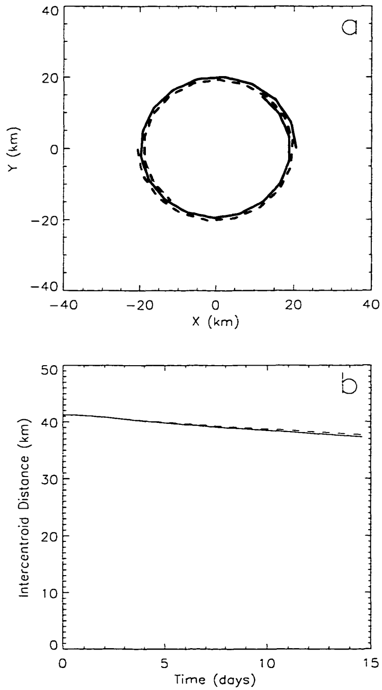
Figure 5.9: As in Fig. 5.8 but for \alpha = 0.1 .
