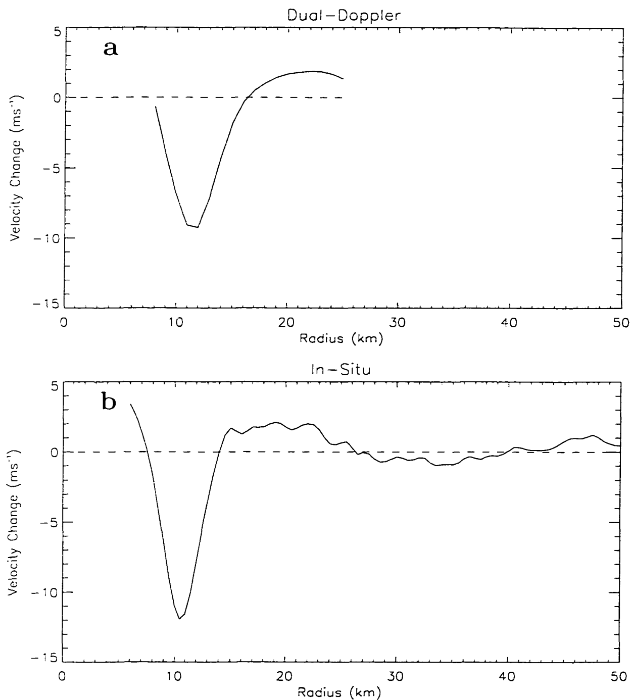
Figure 3.15: Symmetric tangential wind change ( \text{ms}^{-1} ) over the 3.5 h observation period at 3 km height (a) derived from the dual-Doppler analysis and (b) computed from aircraft wind measurements.
