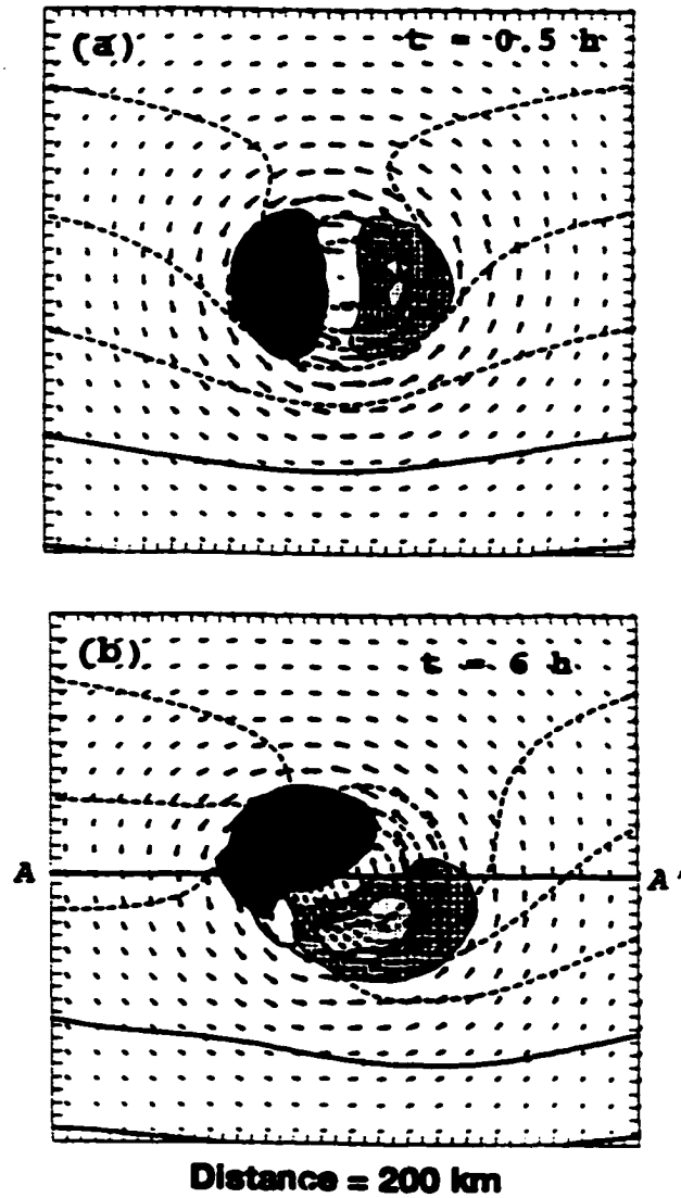
Figure 6.7: Vertical velocity at 2 km height resulting from the interaction of the vortex and vertical shear described by Trier et al. (1998). The results at (a) 0.5 hr and (b) 6 hr are shown. Dark shading denotes values from -1 to -3 \text{ cm s}^{-1} and light shading values from 1 to 3 \text{ cm s}^{-1} . From Trier et al. (1998), used with permission.
