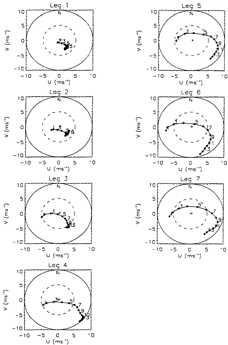
Figure 6.9: Hodographs of the area-averaged storm-relative wind ( \mathbf{V}_e - \mathbf{V}_s ) from 0.75 km to 10.5 km height for each flight leg. The vertical distance between points is 0.75 km.
