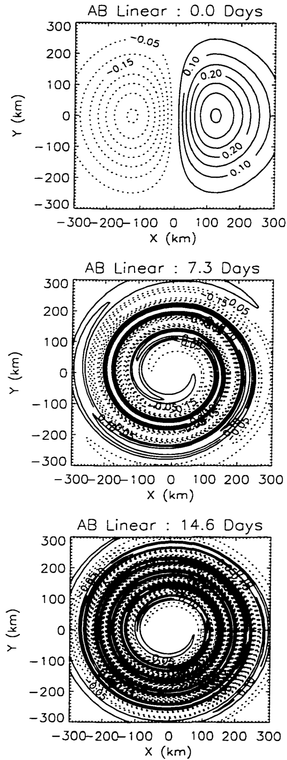
Figure 6.4: As in Fig. 6.2, but for a smaller value of N = 2.5 \times 10^{-3} \text{ s}^{-1} . Contour interval 0.05 \times 10^{-9} \text{ s}^{-3} .
