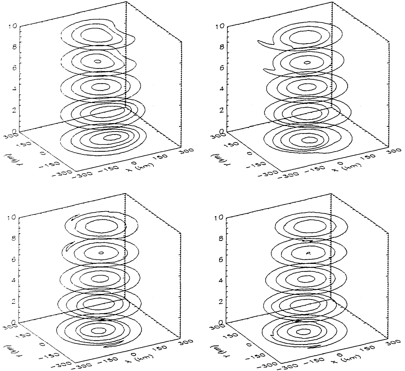
Figure 5.24: Evolution of vortex PV (from left to right) at t = 0, 0.5\tau_e, 1.5\tau_e , and 2.5\tau_e for the case of a barotropic mean vortex perturbed with an isolated baroclinic anomaly. Only the inner 600 \text{ km} \times 600 \text{ km} is shown. The vertical depth is 10 km. The contour interval is 2.0 \times 10^{-5} \text{ s}^{-1} . (a) QG3D model (b) linear EQB model.
