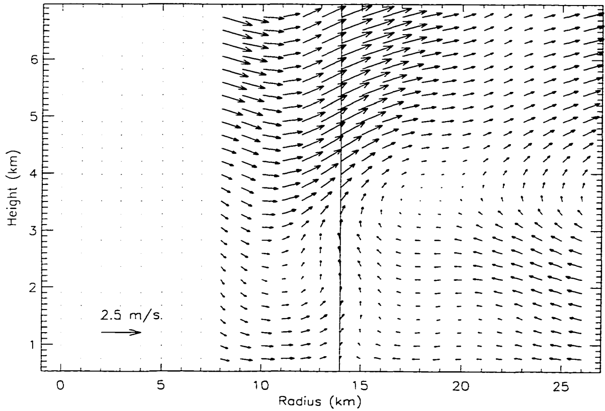
Figure 3.4: As in Fig. 3.2, but averaged over the period 2027–2355 UTC. Maximum wind vector is 2.5 \text{ m s}^{-1} . The solid line denotes the time-average location of the RMW as a function of height.
