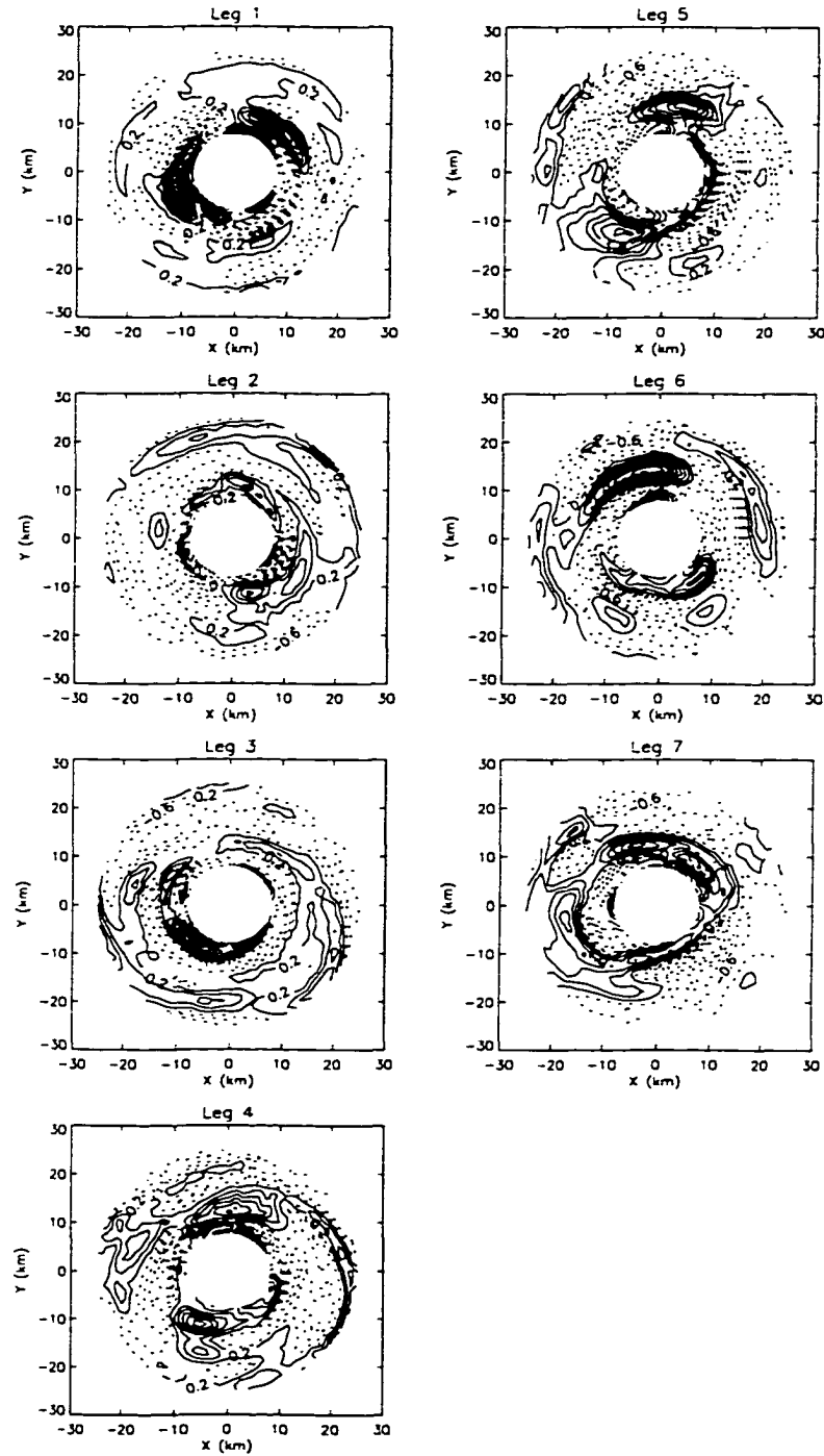
Figure 3.7: Perturbation vorticity, \zeta' , at 3 km height for each flight leg. Contour interval is 0.4 \times 10^{-3} \text{ s}^{-1} . Negative values are depicted by the dashed curves.
