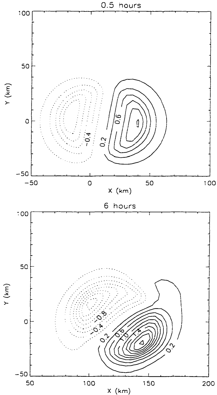
Figure 6.8: Vertical velocity derived from the omega-equation at 2 km height resulting from the interaction of the vortex and vertical shear described by Trier et al. (1998). The results at (a) 0.5 hr and (b) 6 hr agree with the PE simulations of Trier et al. The grid is shifted to the east to account for the eastward translation and increased vertical tilt of the vortex with time. Contour interval is 0.2 \text{ cm s}^{-1} with dashed contours representing downward motion.
