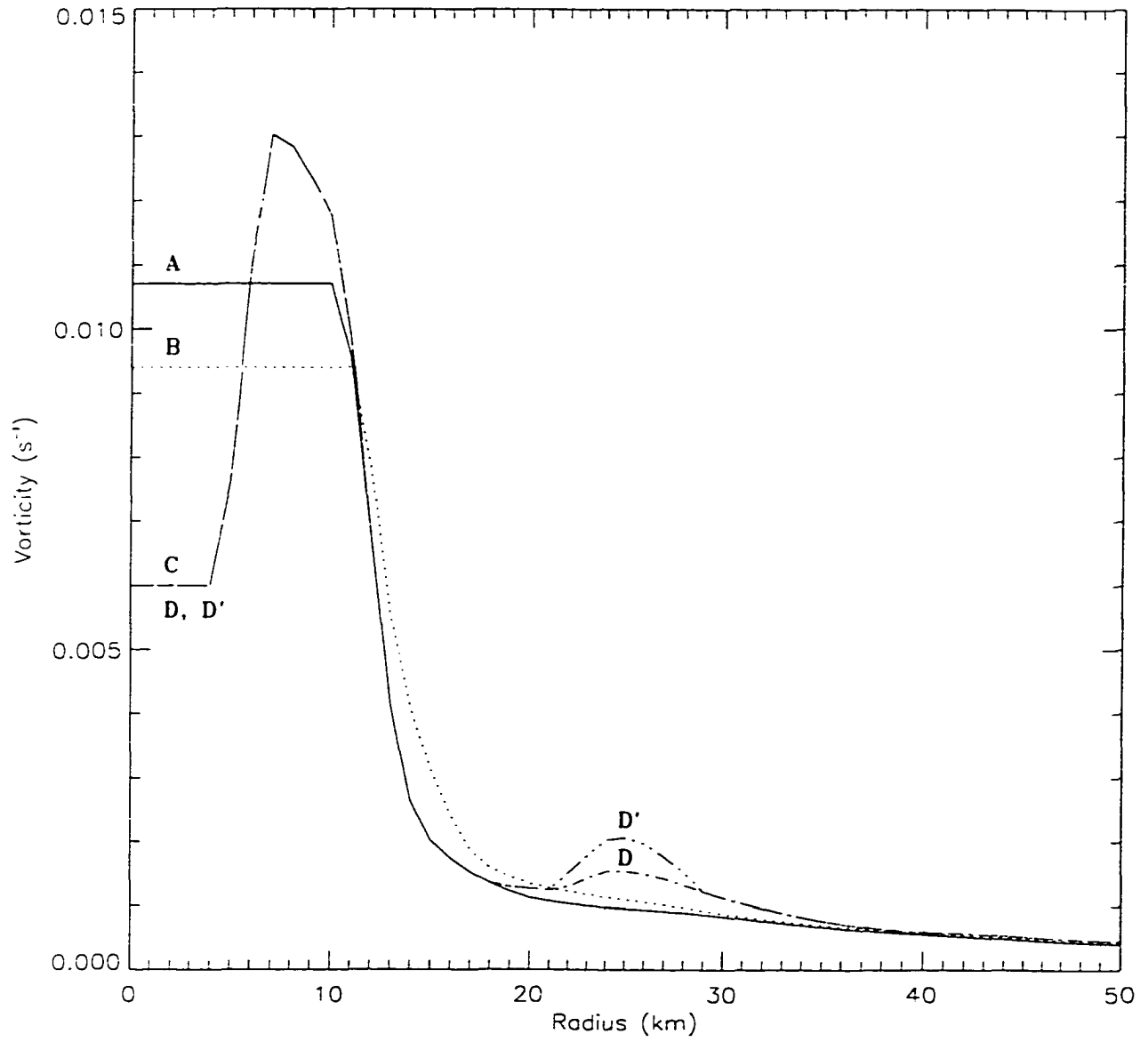
Figure 3.11: Initial profiles of symmetric vorticity ( \text{s}^{-1} ) used in the nondivergent, barotropic numerical simulations. Shown are Case A (solid), Case B (short dash), Case C (long dash), Case D (dash dot), and Case D' (dash dot dot dot).
