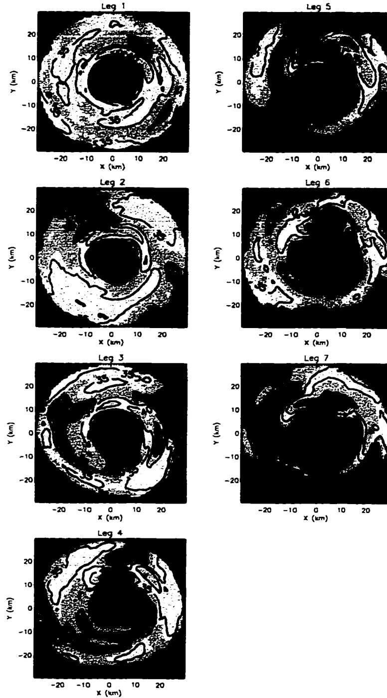
Figure 2.2: Composites of Olivia's inner-core reflectivity near 5 km height derived from the TA radars for each flight leg. See Table 2.1 for the compositing times associated with each leg. Contour interval is 5 dBZ. In this and all subsequent horizontal contour plots, geographical north is located at the top of the plot. Note regions of attenuation radially outside the reflectivity maximum in the northern quadrant of the storm.
