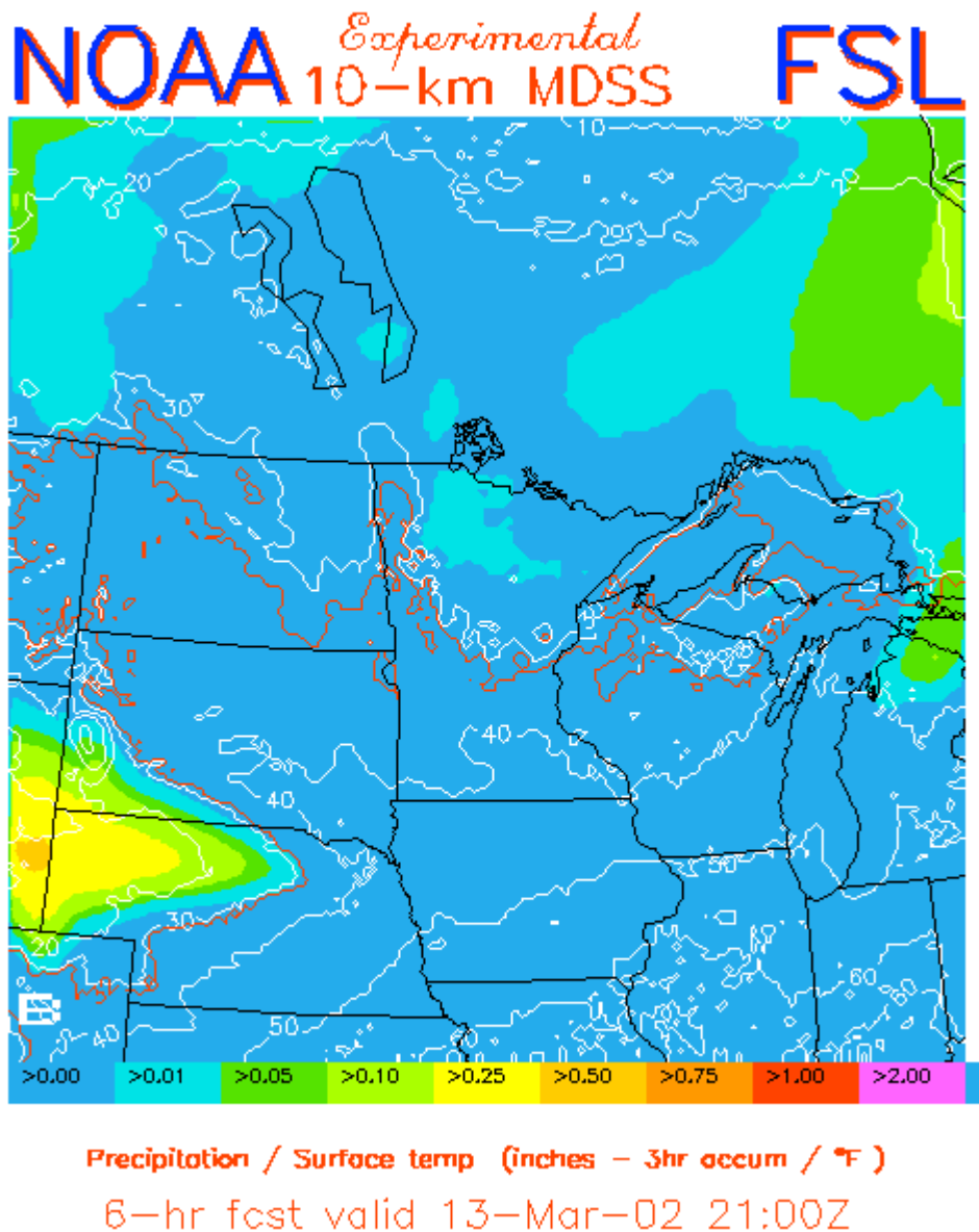
Figure 9. A 6-hr forecast using RAMS over the Minnesota domain (MDSS project). Excellent correlation is found between the radar reflectivity, located at the intersection of the -100 longitude line and the Nebraska-South Dakota border, and the corresponding precipitation pattern depicted in Figure 9.
