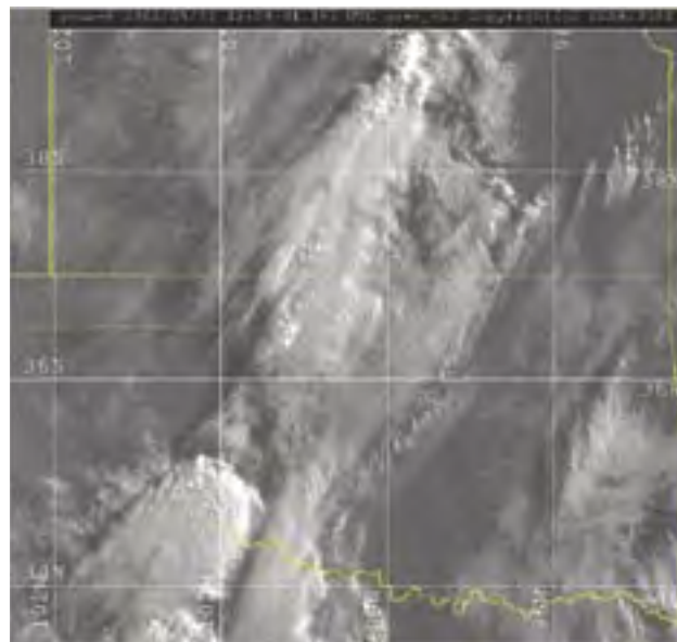
Figure 3. Visible satellite image over OK/KS showing early morning elevated convection.
