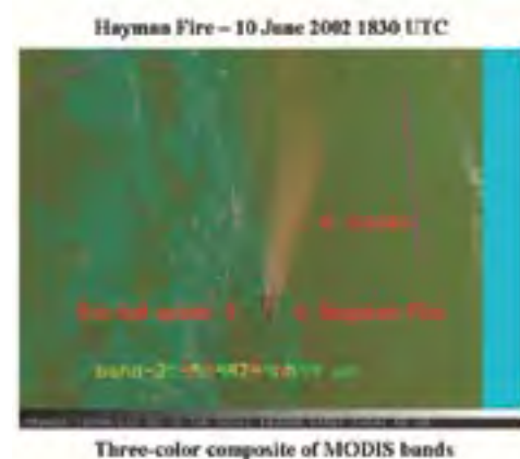
Figure 2: Same as Figure 1, but a false-color red-green-blue (shortwave IR, longwave IR, and visible) composite image of MODIS (bands 25, 31, and 1). The fire hot spots are dark-red to purple and the smoke is light-red to orange. Clouds are white.
