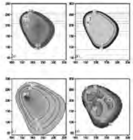
Figure 1. Shaded and contoured plots of (a) synthesized brightness temperatures ( ^{\circ}\text{K} ), (b) monochromatic radiance ( \text{W m}^{-2}\text{sr}^{-1}\text{cm}^{-1} ), (c) column integrated pristine ice ( \text{kg m}^{-2} ) multiplied by 100, and (d) effective mean diameter ( \mu\text{m} ) multiplied by 10^6 at 2 hours into the simulation. In this and subsequent figures, darker shades represent greater values while coordinate values have units of kilometers.
