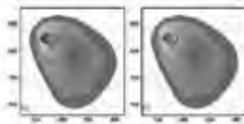
Figure 2. Shaded and contoured plots of synthesized brightness temperatures ( ^\circ\text{K} ) along with (a) total simulated surface condensate (contoured from 0.2 to 2 \text{ g kg}^{-1} ) and (b) simulated precipitation rate (contoured from 20 to 80 \text{ mm hr}^{-1} ).
