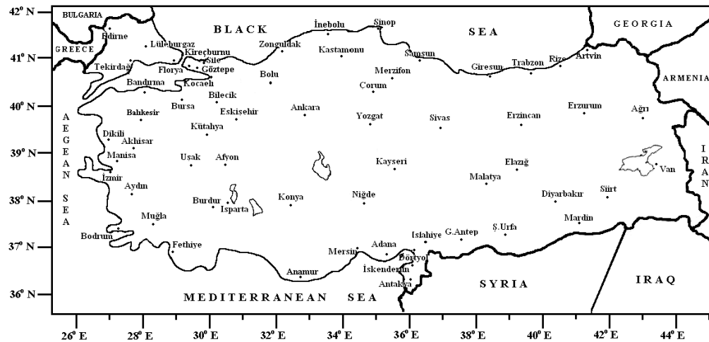
Figure 1. The distribution of temperature observation stations used in the study.
