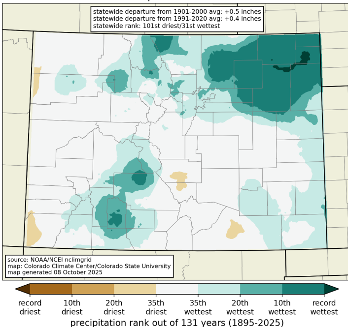
precipitation rank September 2025
