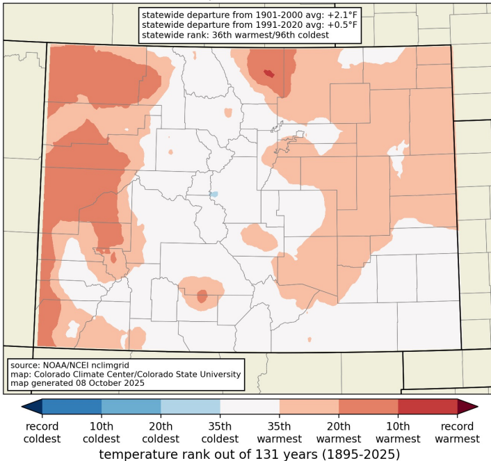
average temperature rank September 2025
