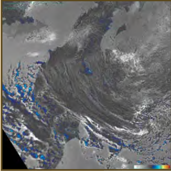
Fig. 3. September 22, 2005, eruption of Mt. Sheveluch, Kamchatka, Russia. AVO satellite image captured ash cloud with AVHRR IR 4/5 enhanced.
