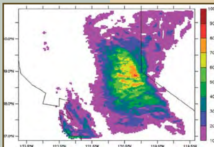
Fig 5b. Ensemble probability of 6-hr. accumulation of precipitation exceeding 0.5" ending at the 18-hr. lead time.
