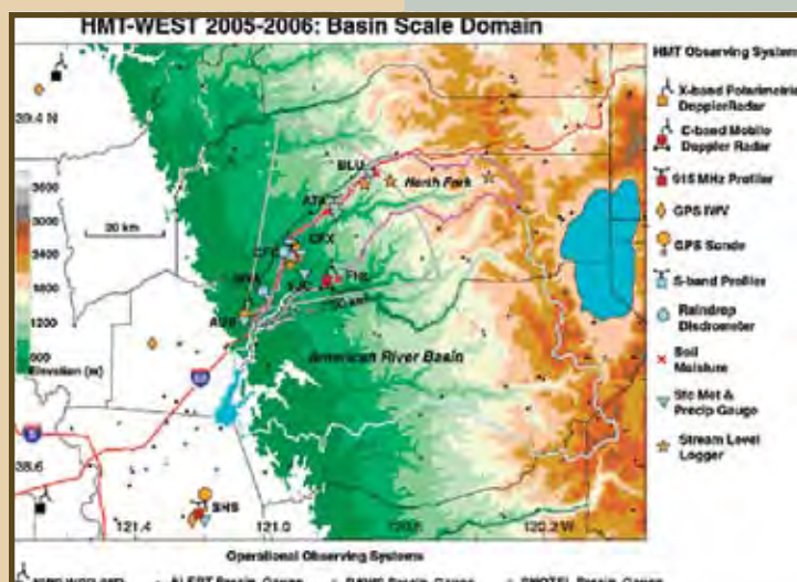
Fig 1. Basin-scale map of the first full-scale deployment of HMT-West 2005-2006 successfully conducted December 2005 - March 2006.
