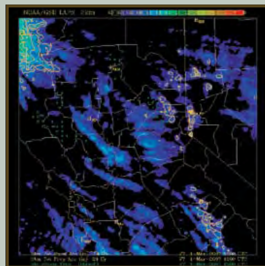
Fig 2b. LAPS analysis of 24-hr. accumulated precipitation (shaded colors), current surface precipitation type (green icons), and 24-hr. snow accumulation (orange contours).
