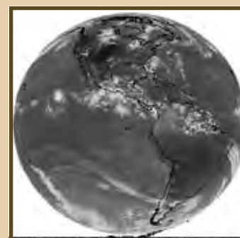
Figure 3: GOES-13 band-4 (10.7 \mu\text{m} ) longwave window image at 1800 UTC on 20 July 2006.
