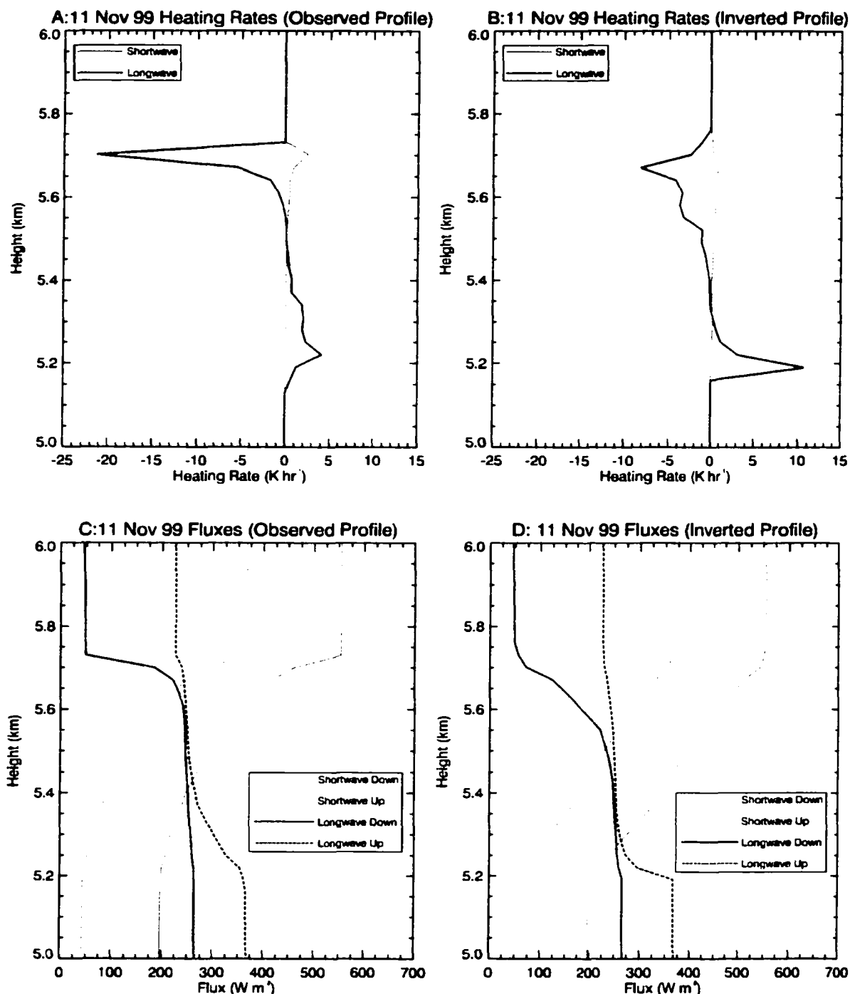
Figure 9.18 Sensitivity of heating rate profiles to model parameterization of cloud phase. (A) and (C) show the observed heating and flux profiles using measured lwc and iwc values for 11 Nov 99; (B) and (D) show the same profile when the cloud lwc and iwc profiles are inverted in the vertical. This is another possible effect of using temperature to determine water phase, as iwc would increase toward cloud top.
