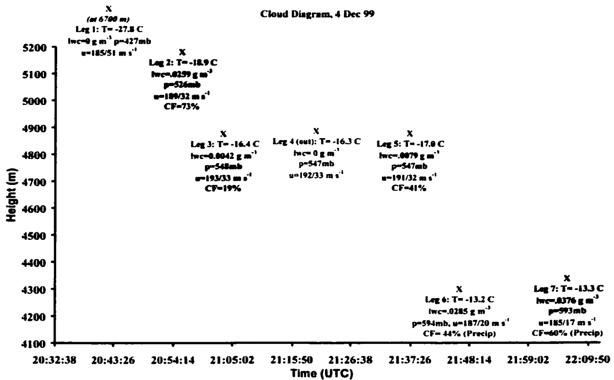
Figure 5.3 Same as the previous figure except for 4 Dec 99. Again, the lighter shading represents lower CF due to inhomogeneous cloud areas, as pockets of drier air were mixed into this cloud. We also had problems moving the aircraft to the cloud on this day due to air traffic control delays when changing flight altitude.
