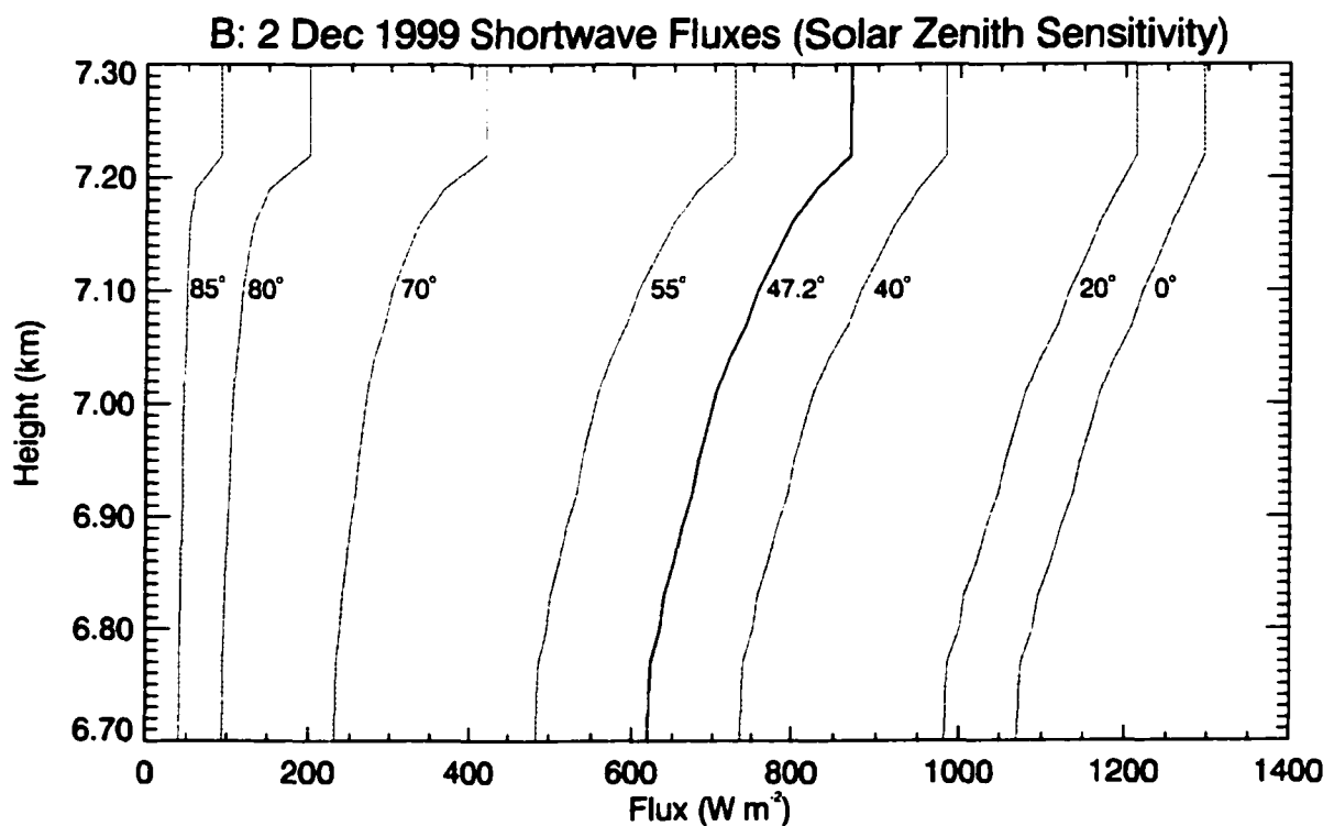
Figure 9.19 Sensitivity of shortwave heating rate to solar zenith angle for 2 Dec 99. The black curve marks the observed heating rate and flux at the observation time; the other curves represent zenith angles as annotated in the diagram. Small angle changes after sunrise may offset nocturnal radiative cooling and cause dissipation.
