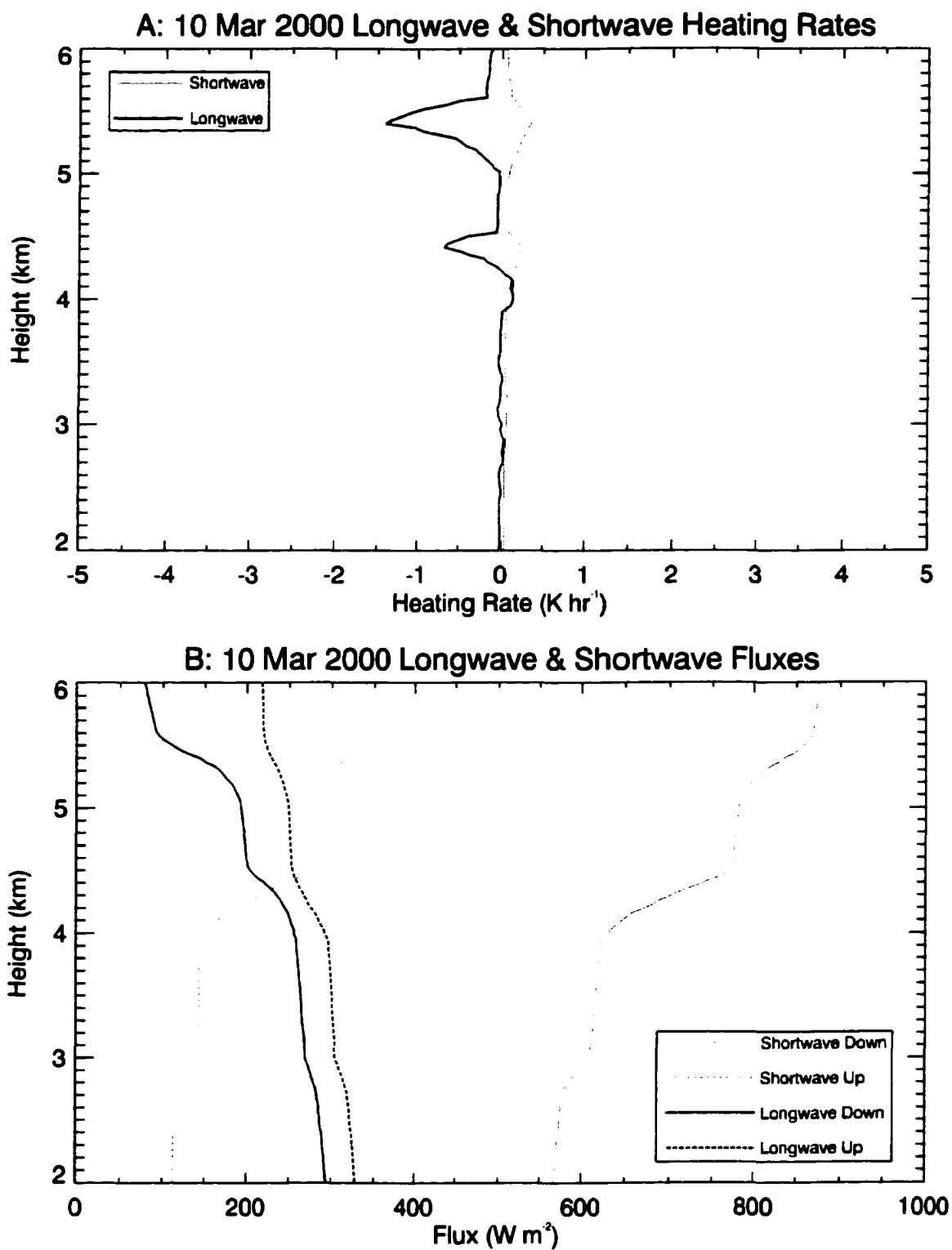
Figure 9.5 Same as the previous three figures except for the multi-layered cloud of 10 Mar 00. Small lwc and iwc values result in small amounts of flux convergence and divergence, which equates to small net heating rates.
