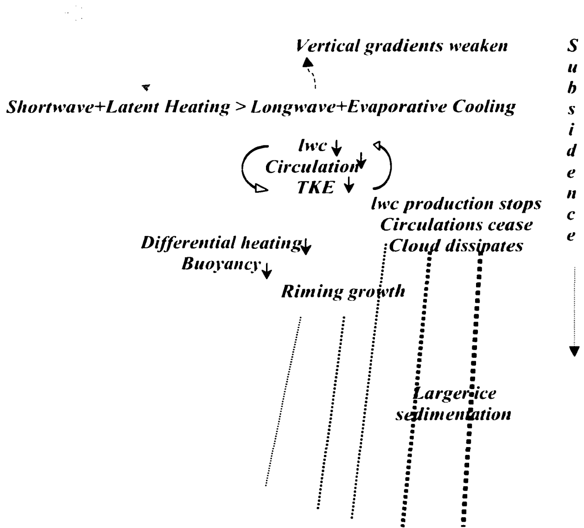
Fig 7.3 Dissipation mechanisms for mid-level, mixed-phase clouds include large-scale subsidence drying, loss of cloud water mass by excessive sedimentation of ice particles from the cloud, excessive dry air entrainment, or a change in the net radiative heating balance of the cloud. Differential vertical radiative heating is critical for maintaining cloud circulations, so if shortwave and latent heating overcome longwave and evaporative cooling at cloud top, the cloud will dissipate.
