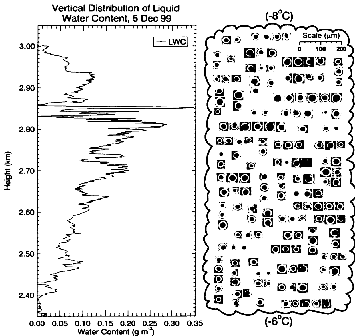
Figure 5.10 Same as previous three figures except for 5 Dec 99. This cloud was composed primarily of supercooled liquid droplets, despite temperatures of only -6 to -8^{\circ}\text{C} . Dry air entrainment near cloud top caused a slight departure from the increase of lwc with height seen in figures 5.7-5.8.
