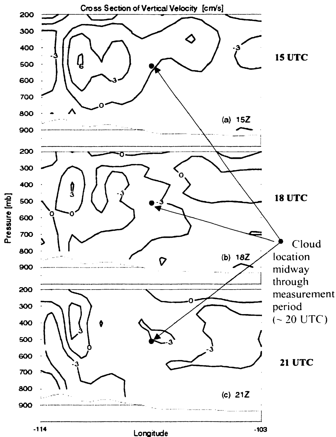
Fig 8.2 Cross-section of MMS forecast vertical velocity ( \text{cm s}^{-1} ) initialized 12 UTC on 11 November 1999. The air motion is upward at several \text{cm s}^{-1} at 1500 UTC, decreases to downward at about -3 \text{ cm s}^{-1} by 1800 UTC as the cloud starts to decay, and remains at -3 \text{ cm s}^{-1} by 2100 UTC, after the cloud dissipates.
