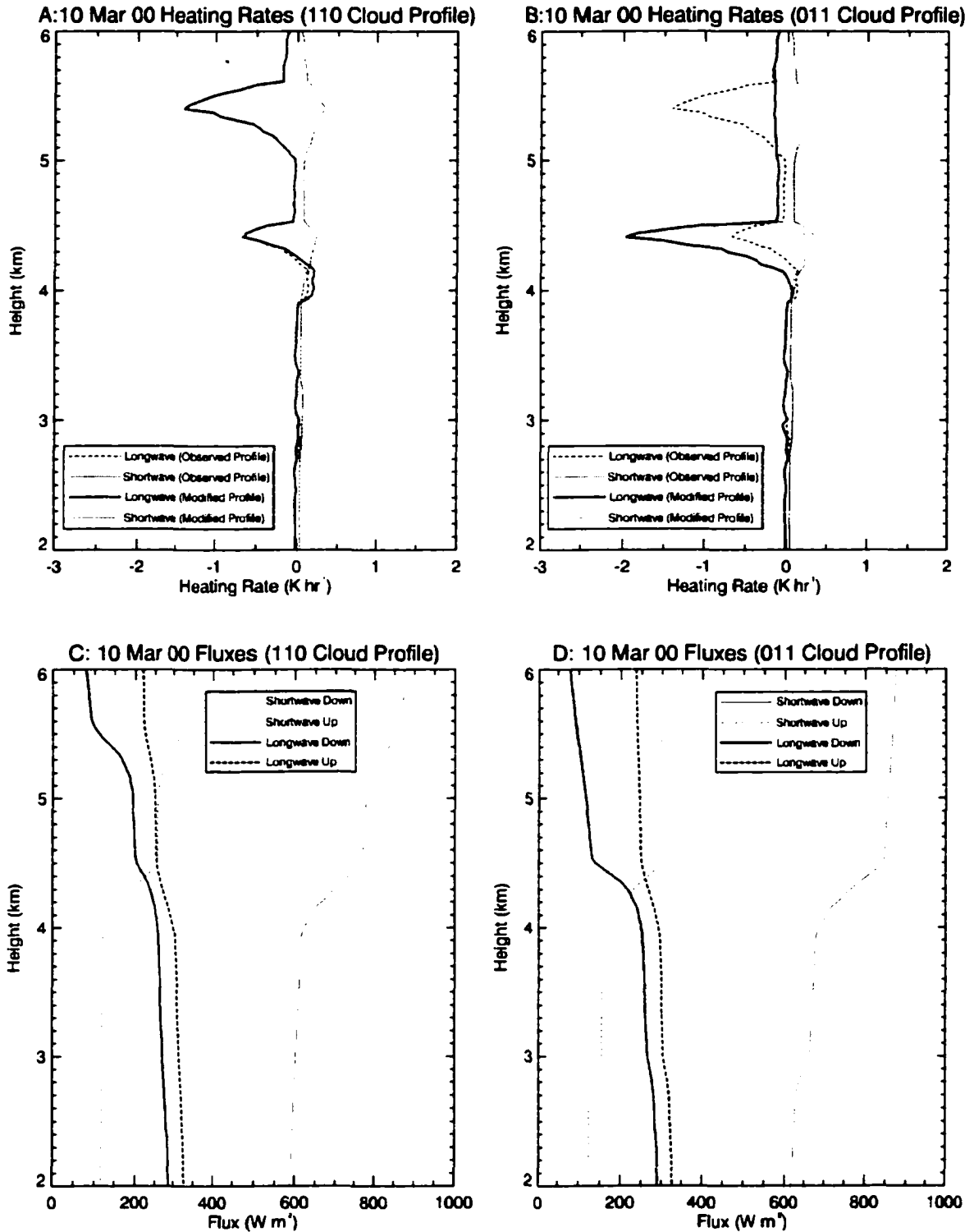
Figure 9.25 Same as the previous two figures except for cases in which only the top two layers (110) and the bottom two layers (011) are included in the profile. The “110” profile in (A) nearly mirrors that of the observed case, while the longwave cooling in the middle layer dominates the “011” profile in (B).
