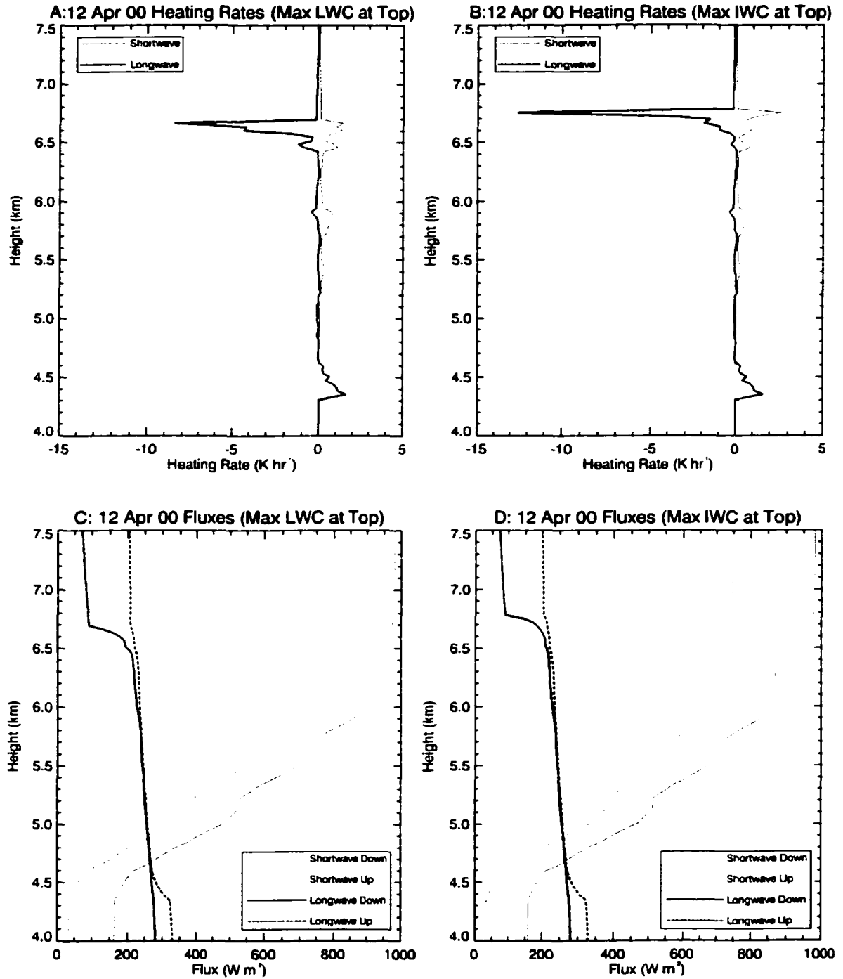
Figure 9.7 Results of a sensitivity study on the 12 Apr 00 case (Fig 9.6) showing the increase in heating rate (top) and flux (bottom) when the maximum lwc is located at cloud top (A,C) or the maximum iwc is located at cloud top (B,D). Note that the maximum longwave cooling approximately triples for A and quadruples for B.
