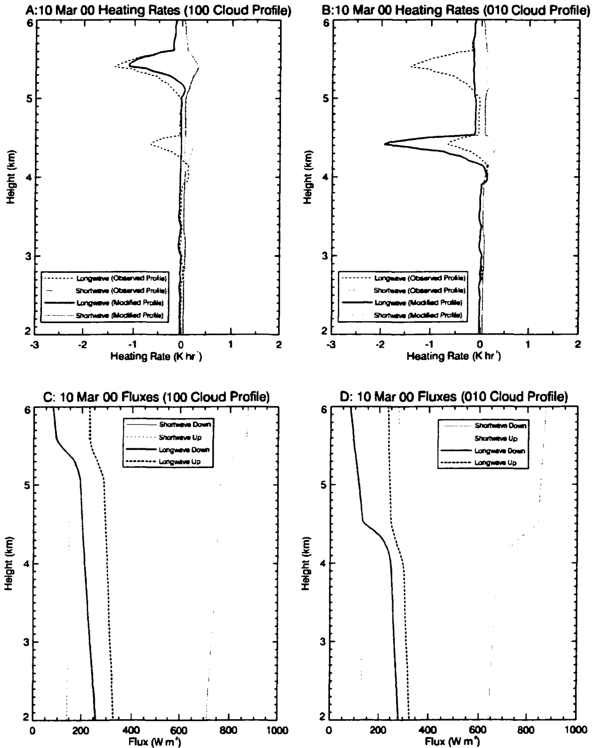
Figure 9.23 Sensitivity of radiative heating rates and fluxes to changes in cloud layering. The three-digit binary code corresponds to the layers included in each plot, i.e., only the top layer is included in “100”. The 10 Mar 00 control case (all three layers) is shown in Figure 9.5 and is represented by a dashed line in each plot.
