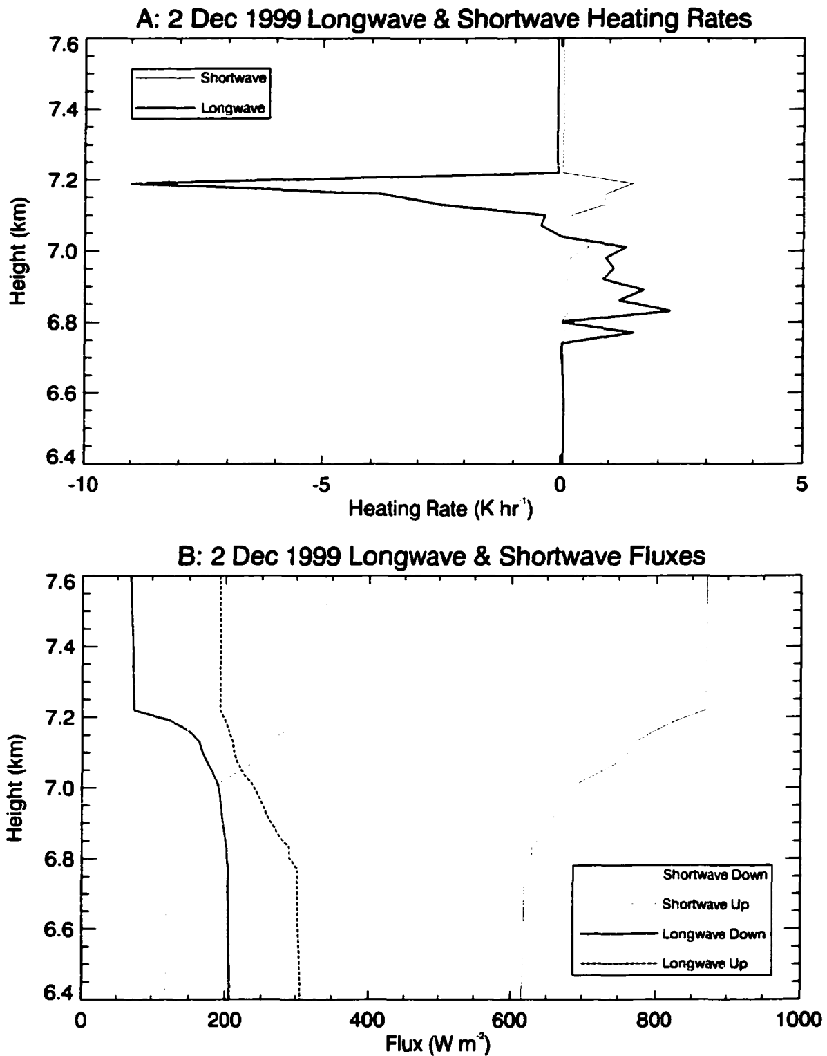
Figure 9.3 Same as Fig 9.2 except for 2 Dec 99 heating rates and fluxes. Note the different scales. The maximum lwc for this case is half that of 11 Nov 99, resulting in smaller longwave and shortwave heating and cooling rates.
