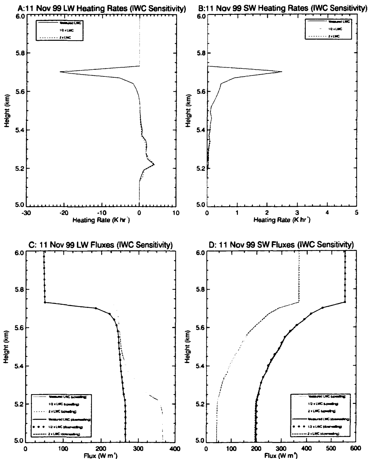
Figure 9.13 Same as Fig 9.8 except for sensitivity to iwc instead of lwc. The heating and cooling rate values and percent changes are shown in parentheses in Tables 9.1 and 9.2. Note the almost indiscernible changes in flux and heating rate when the iwc is doubled and halved, in contrast to the larger radiative interactions with lwc.
