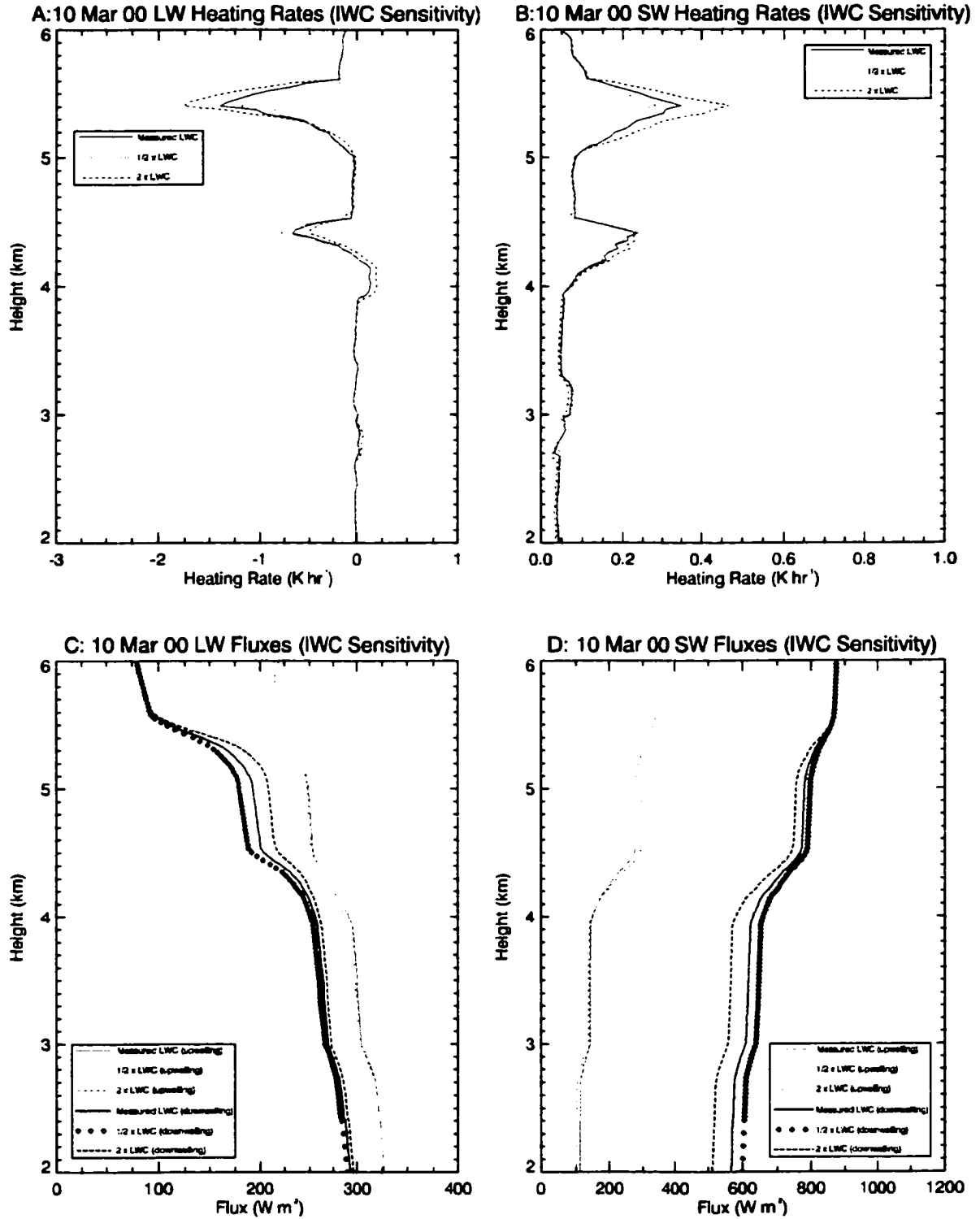
Figure 9.15 Same as previous figure except for the 10 Mar 00 multi-layered case. The effects of doubling and halving the iwc are much more apparent here than in the previous two cases, because the cloud iwc was uniformly distributed and of the same order of magnitude as the lwc. Values are shown in Tables 9.1 and 9.2.
