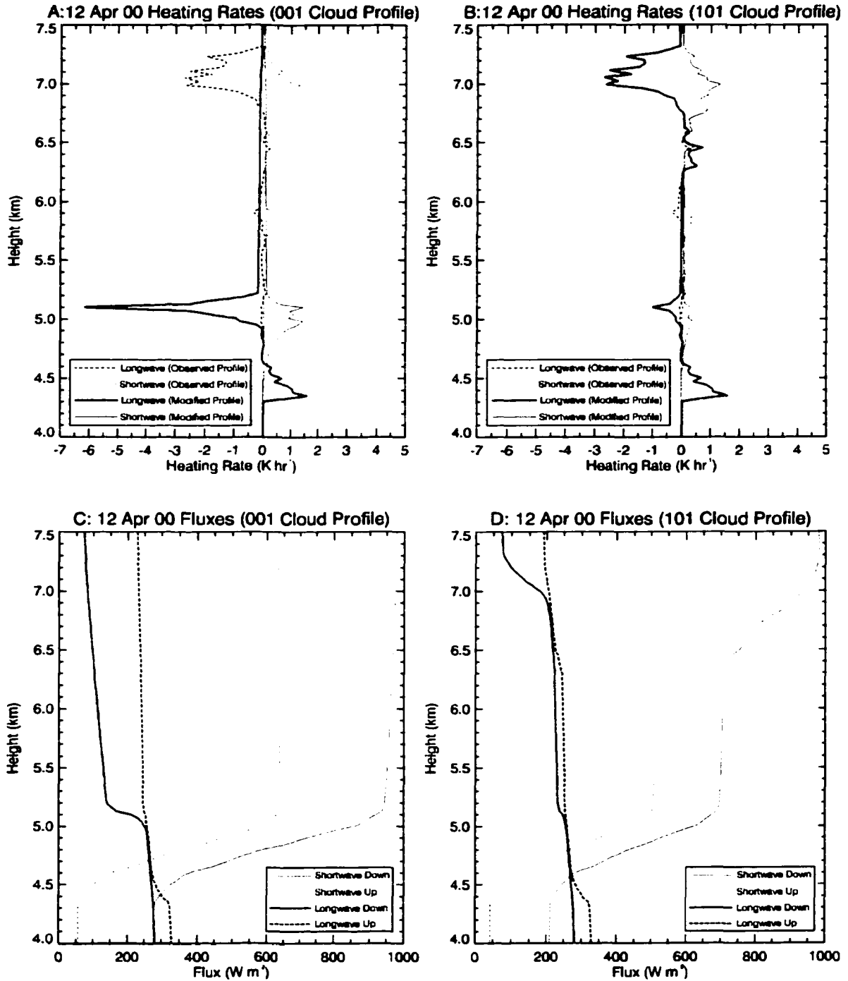
Figure 9.27 Same as Fig 9.24 except for 12 Apr 00. Significant longwave cooling is apparent in (A) when the lowest layer is allowed to radiate without interacting with upper layers; from zero when layers are present to 6 \text{K hr}^{-1} when they are removed. The net radiative profile will change with time as layers develop and dissipate.
