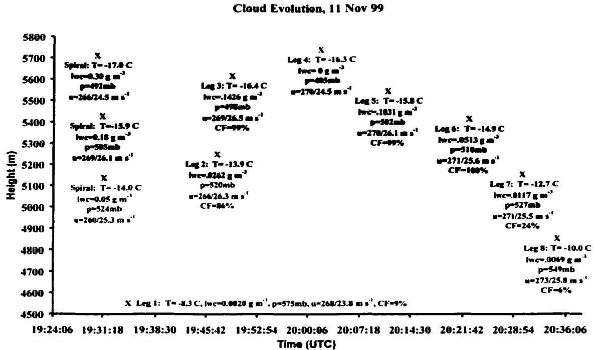
Figure 5.1 Cloud evolution diagram for the 11 Nov 99 case showing the relative time and height of the spiral soundings and subsequent racetracks. Measurements for the spirals are point values, while those for the flight legs are mean values of the diagram are temperature, liquid water content (lwc), pressure, horizontal wind direction and speed, and cloud fraction (CF). Light shading represents lower CF.
