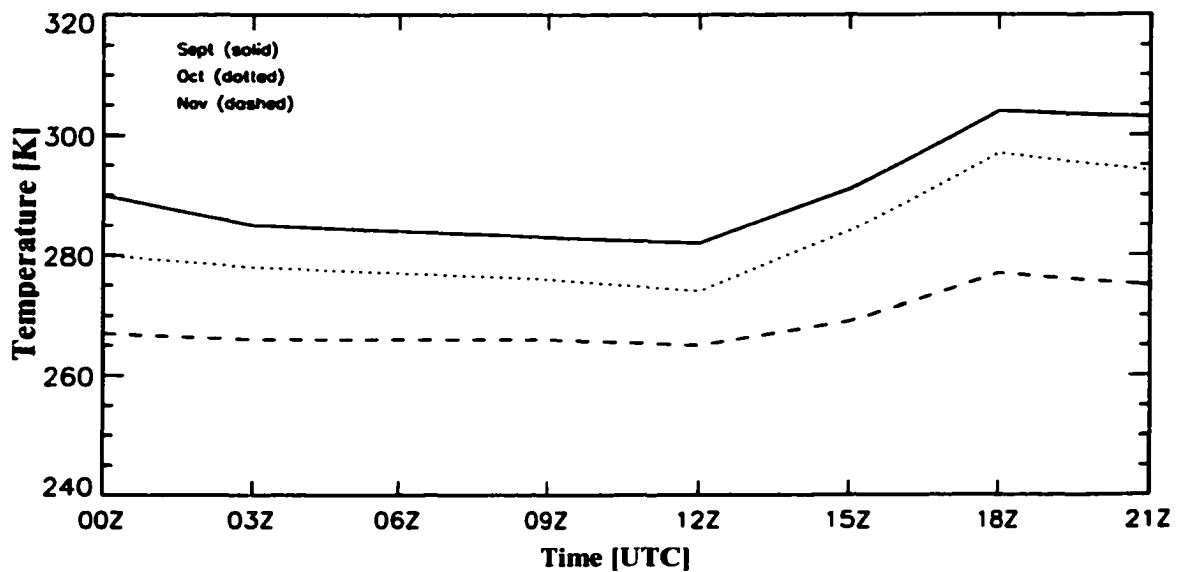
Figure 9.20 Diurnal variation of mid-level clouds over North Dakota. The top panel shows percent frequency of occurrence of mid-level clouds versus time of day for September, October and November. The plots are derived from a three-hourly infrared ISCCP database over a ten-year period of record. The bottom panel shows the satellite-derived surface temperature over the same time period. Clouds increase overnight in response to radiative cooling but decrease after sunset, as net radiational cooling decreases in response to shortwave heating at cloud top.
