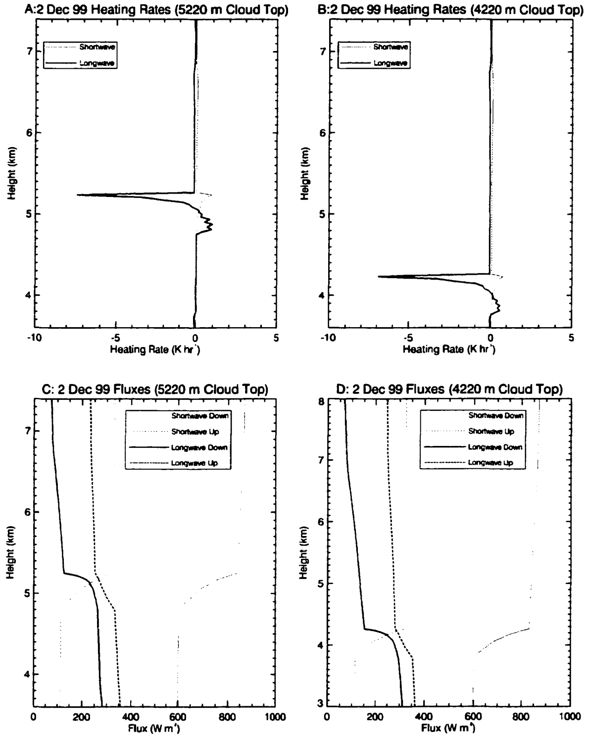
Figure 9.22 Same as Fig 9.21 except at lower heights of 5.2 km (A,C) and 4.2 km (B,D). Note that smaller height differences between cloud base and the Earth's surface result in less heating at cloud base and cooling at cloud top, as forwarded by Stephens (1978). For this reason, cloud height accuracy is important for GCMs.
