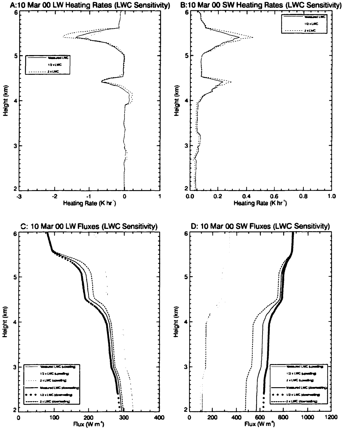
Figure 9.11 Same as previous three figures except for 10 Mar 00. Small lwc amounts ( < 0.04 \text{ g m}^{-3} ) result in small flux changes and a small net heating rate. Note the change in scale from the other figures. Refer to Tables 9.1 and 9.2 for quantitative values of heating rate and the percent changes from the control case.
