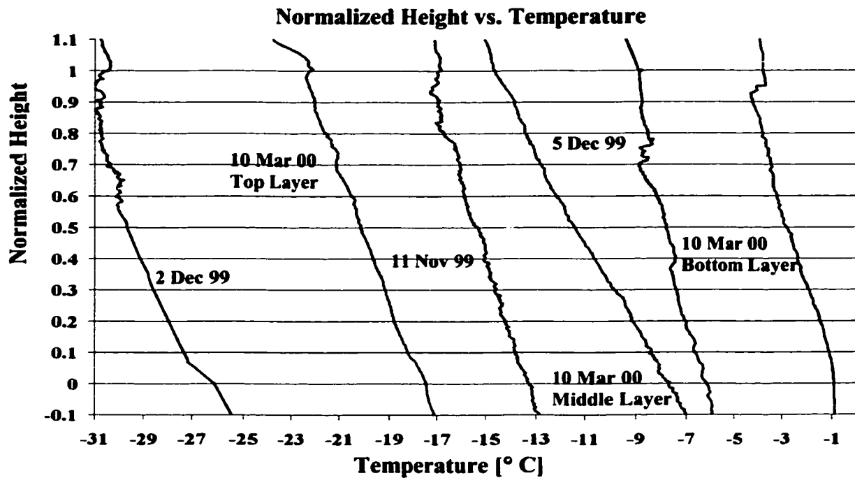
Figure 5.19 Vertical profiles of temperature for four of the cloud cases, including the individual layers of the 10 Mar 00 case. Note the lack of temperature inversions at the cloud boundaries, particularly at cloud top.
