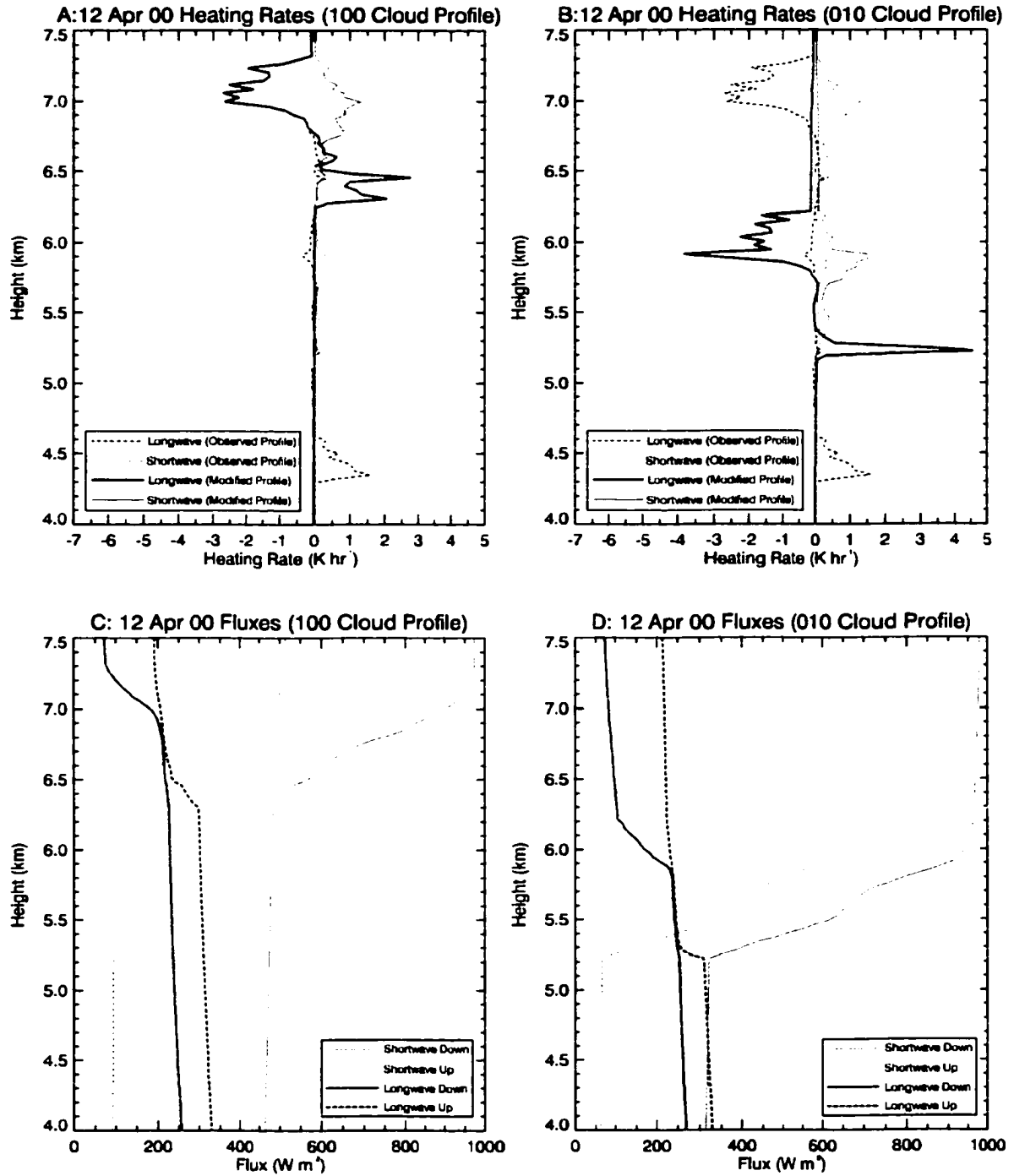
Figure 9.26 Same as Fig 9.23 except for 12 Apr 00. In panel (A), note the longwave heating at the base of the top layer when removing the bottom layers. Likewise, panel (B) shows both radiative heating and cooling in the middle layer that was completely absent when all three layers were present.
