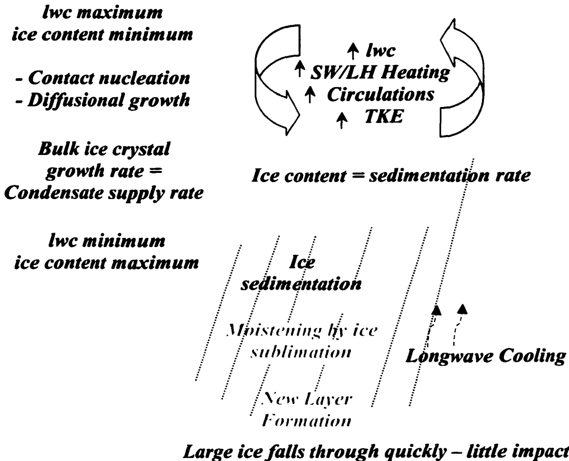
Fig 7.2 Maintenance processes for mid-level, mixed-phase clouds. In this stage, a delicate balance exists between the condensate supply rate, the bulk ice crystal growth rate, the dry air entrainment rate, and the amount of sedimentation. The circulation has to be strong enough to produce more liquid water, but not so strong that dry air is entrained too rapidly. The amount of ice nuclei also appears to be important for maintaining the cloud against rapid glaciation. Sedimentation of large ice from the base of the cloud may moisten the layer beneath by sublimation to the point where a new cloud layer is formed.
