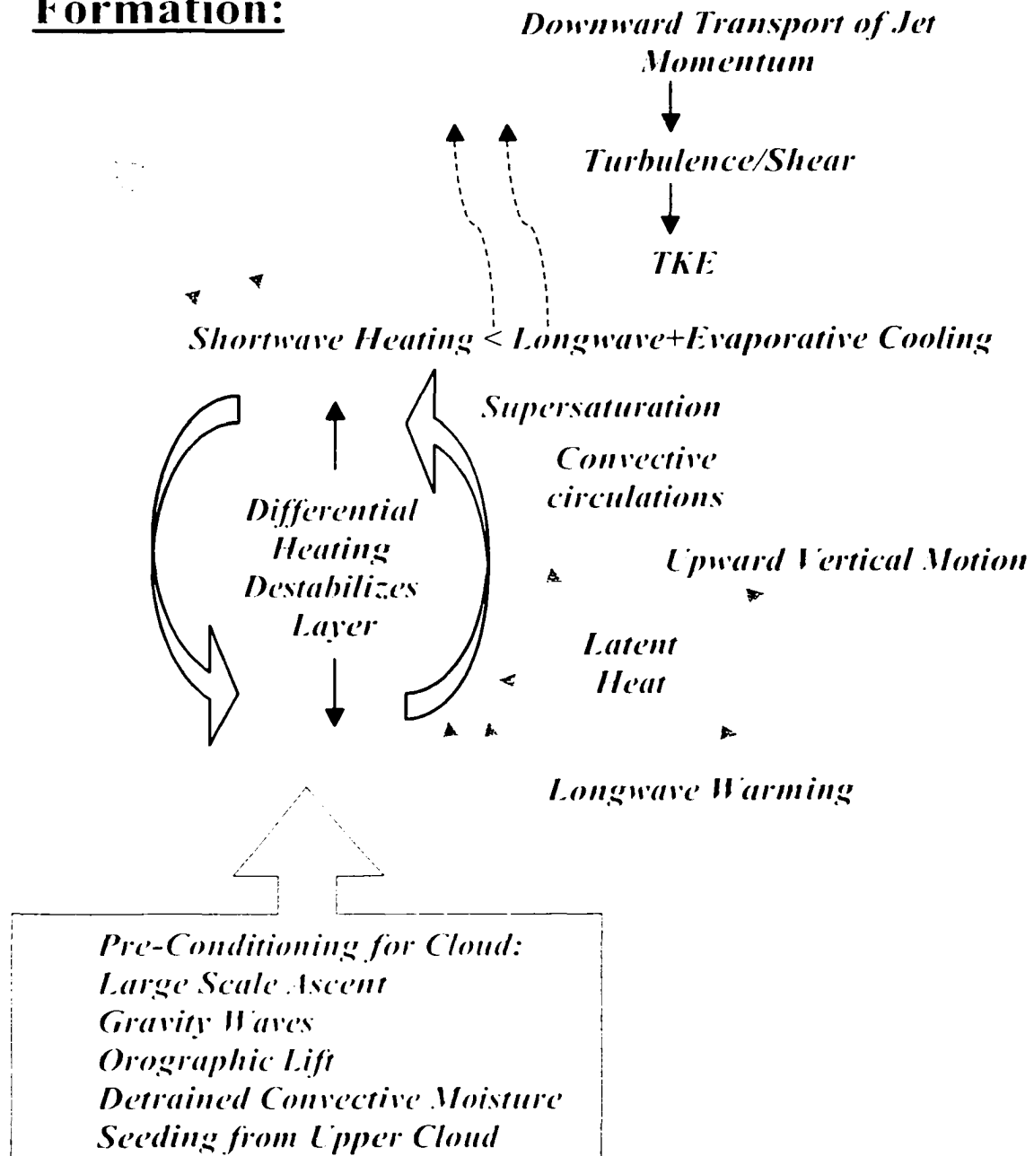
Fig 7.1 Formative mechanisms and processes for mid-level, mixed-phase clouds. In this stage, a cloud is generally first formed by lifting a moist air layer until it cools and condenses, and then destabilized by vertical differential radiative heating and cooling processes. Evaporative cooling at cloud top and the release of latent heat further destabilizes the layer, causing internal circulations to develop. The added lift may increase the condensation supply rate, causing further cooling and more intense cloud circulations, but also increasing the dry air entrainment rate.
