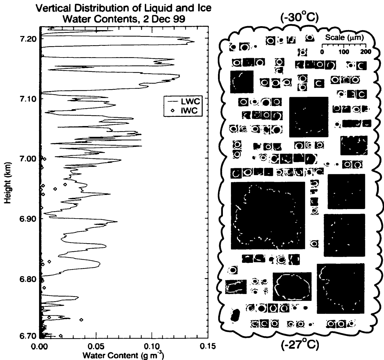
Fig 5.8 Same as previous figure except for 2 Dec 99. Note the change in scale; this cloud has half the lwc as the 11 Nov 99 cloud. Also, despite temperatures in the -27 to -30^{\circ}\text{C} range, this cloud had very low amounts of iwc. This is mainly due to a low concentration of ice particles, as the sizes were generally larger than for 11 Nov 99.
