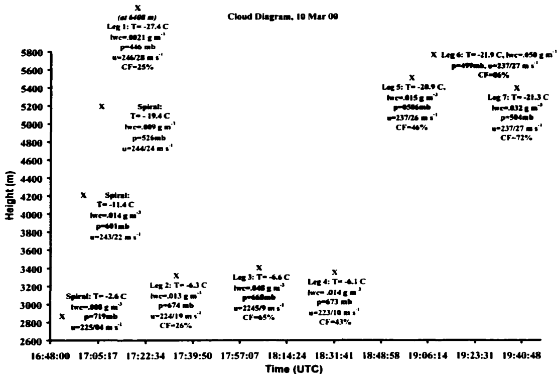
Figure 5.5 Same as the previous figure except for the multi-layered cloud system on 10 Mar 00. Note that the original three layers devolved into two layers after about 18:31 UTC and the bottom layer ascended to a slightly higher height with time.
