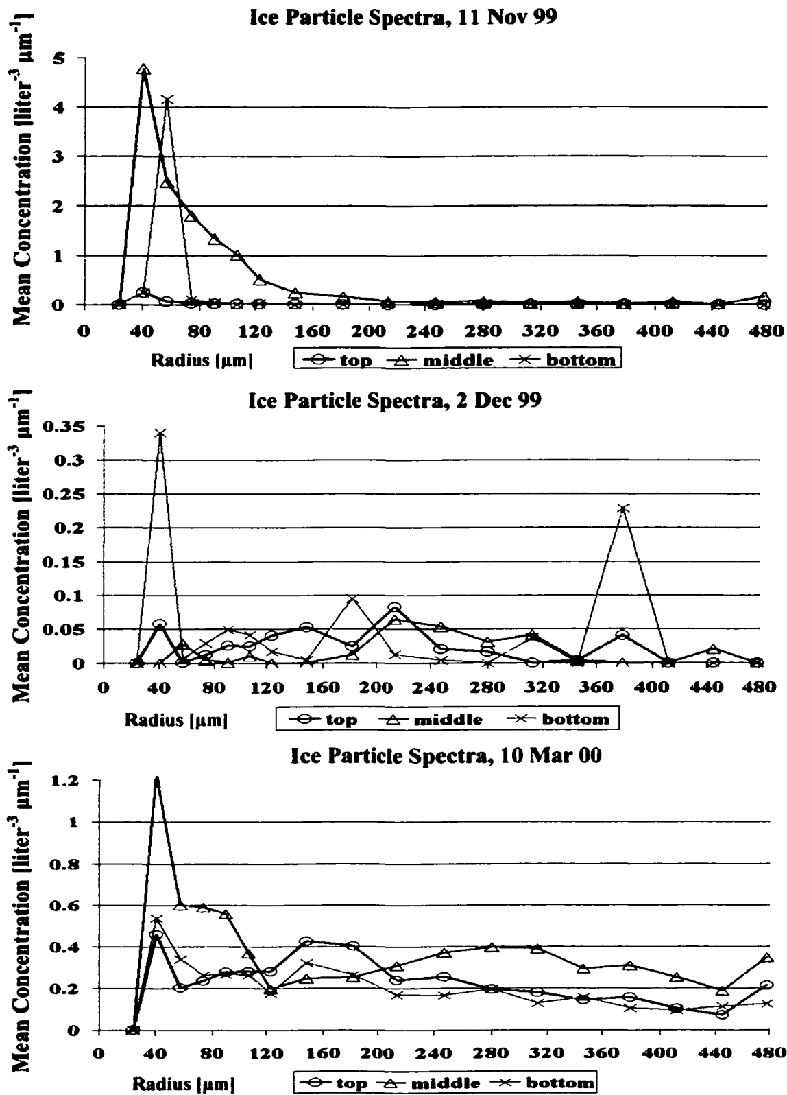
Figure 5.17 Same as the previous four figures, except for ice concentration and size using 2D-C measurements, rather than FSSP liquid droplet spectra. Note the relatively small and rather homogeneous concentrations for all ice particle sizes.
