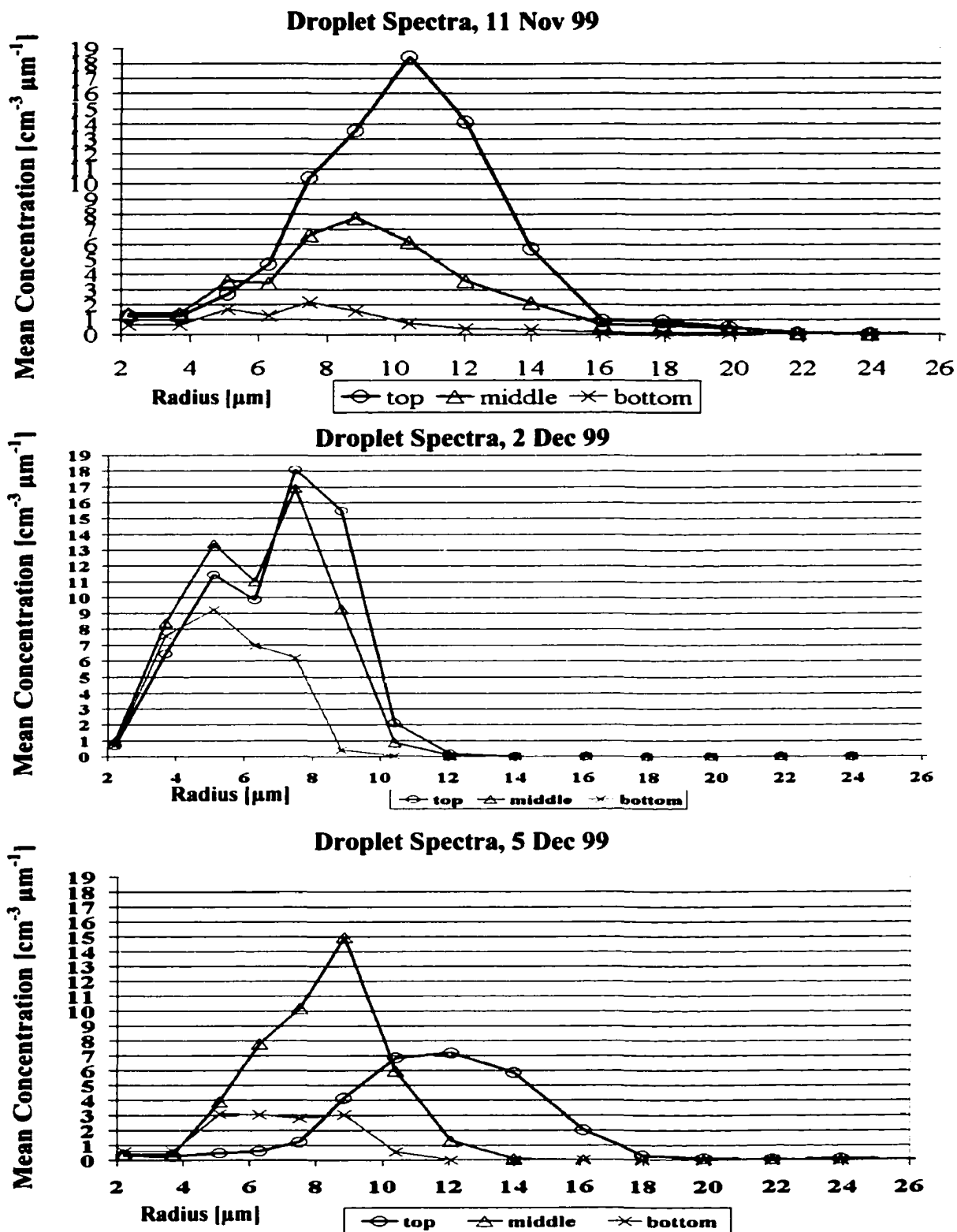
Figure 5.13 Droplet spectra for the single-layer cloud cases on 11 Nov 99 (top), 2 Dec 99 (middle), and 5 Dec 99 (bottom). Notice a shift to larger-sized liquid water droplets with height through each cloud. The concentrations also increase with height in each cloud except 5 Dec 99, when entrainment caused cloud top drying.
