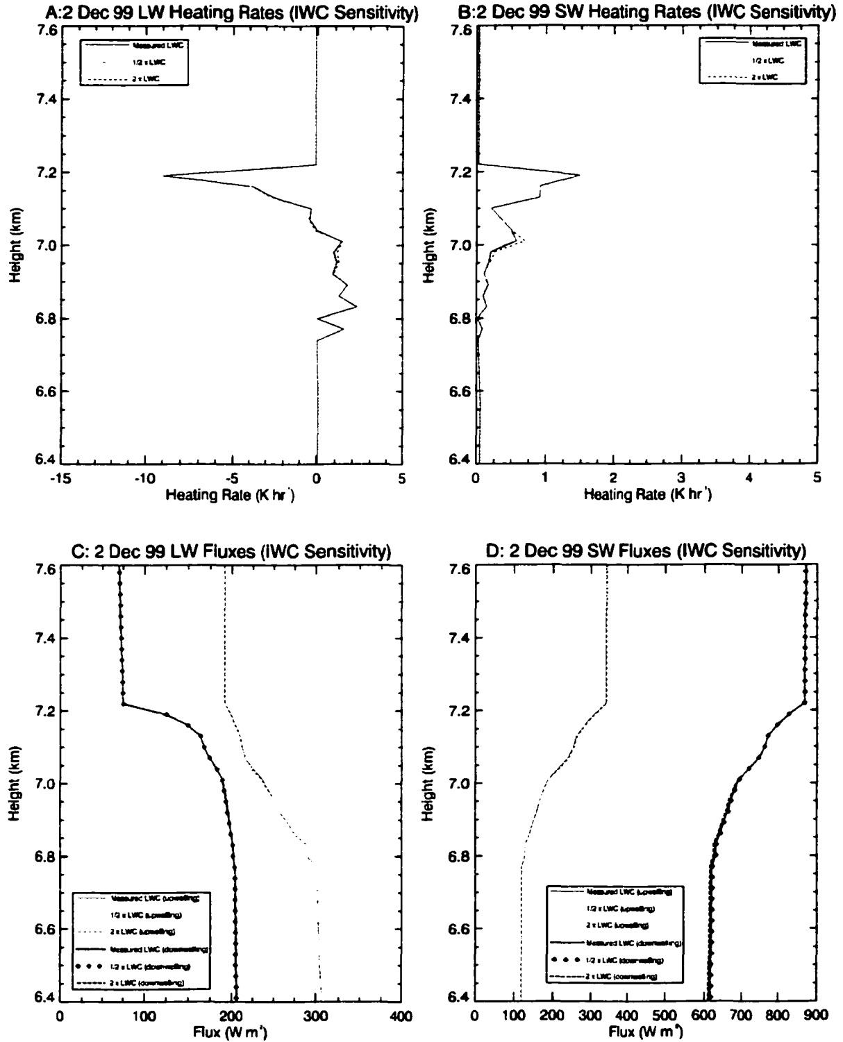
Figure 9.14 Same as previous figure except for 2 Dec 99 sensitivity to iwc. Again, note that there is very little impact to the fluxes and heating rates when doubling and halving the iwc, due to the relatively small amounts of ice in the bottom parts of the single-layer clouds.
