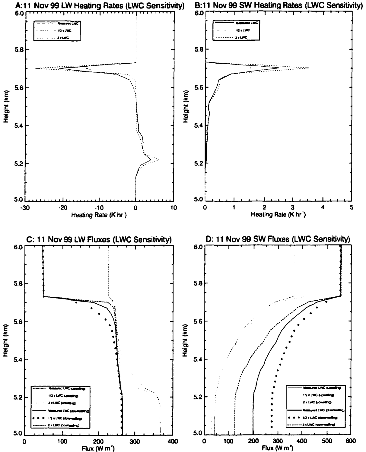
Figure 9.8 Sensitivity of longwave and shortwave radiative heating rate and flux to the amount of lwc for the 11 Nov 99 case. BUGSRAD model results for doubled and halved lwc are compared to the measured lwc value (see legend). Quantitative values and percent changes for the three plots are shown in Tables 9.1 and 9.2.
