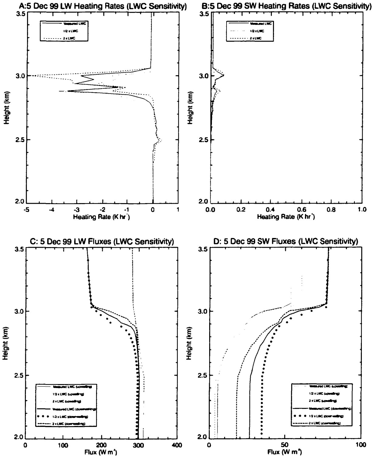
Figure 9.10 Same as previous two figures except for 5 Dec 99. The variation of longwave cooling near the cloud top is due to the effects of dry air entrainment; the cooling rate associated with maximum lwc is at 2880 m, but decreasing amounts of lwc above that level interact with the fluxes to cause reduced cloud top cooling rates.
