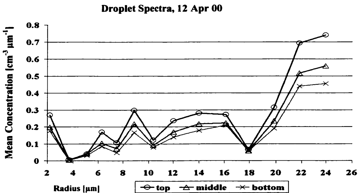
Figure 5.16 Same as the previous two figures, except in this case the droplet spectra is a summation of the earlier plots for the total three cloud system.
