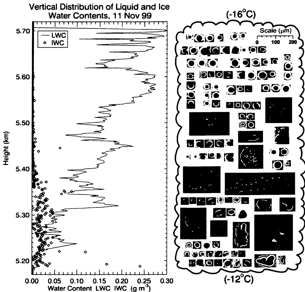
Fig 5.7 Vertical profiles of liquid and ice water content ( \text{g m}^{-3} ) for the 11 Nov 99 single-layer cloud case. To the right is a vertically consistent collage of CPI images, showing representative particles at the relative location they were measured in the cloud.
