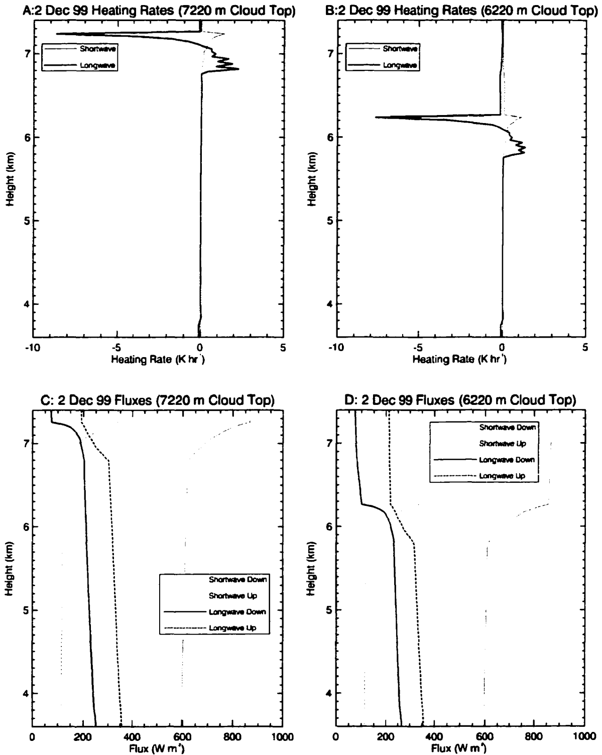
Figure 9.21 Sensitivity of radiative heating rates (A, B) and fluxes (C, D) to changes or errors in cloud height. Plots A and C show the heating rates and fluxes at the actual measurement height, while B and D use the same cloud profile, but at 1 km lower height. The resulting heating rates are about 1 \text{ K hr}^{-1} for the lower cloud.
