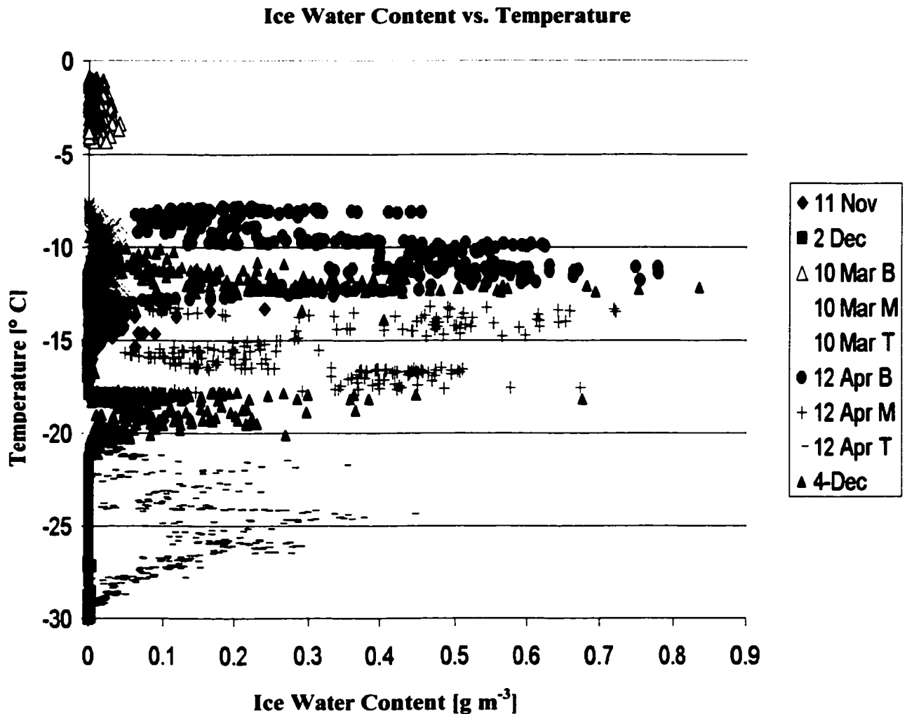
Fig 5.21 Variation of ice water content with temperature for the five mixed-phase cloud cases. Highest values of iwc are between -8 and -20^{\circ}\text{C} , corresponding to the maximum in both ice supersaturation and the growth rate of plate-like crystals centered at -15^{\circ}\text{C} . B, M and T denote bottom, middle and top of cloud, respectively.
