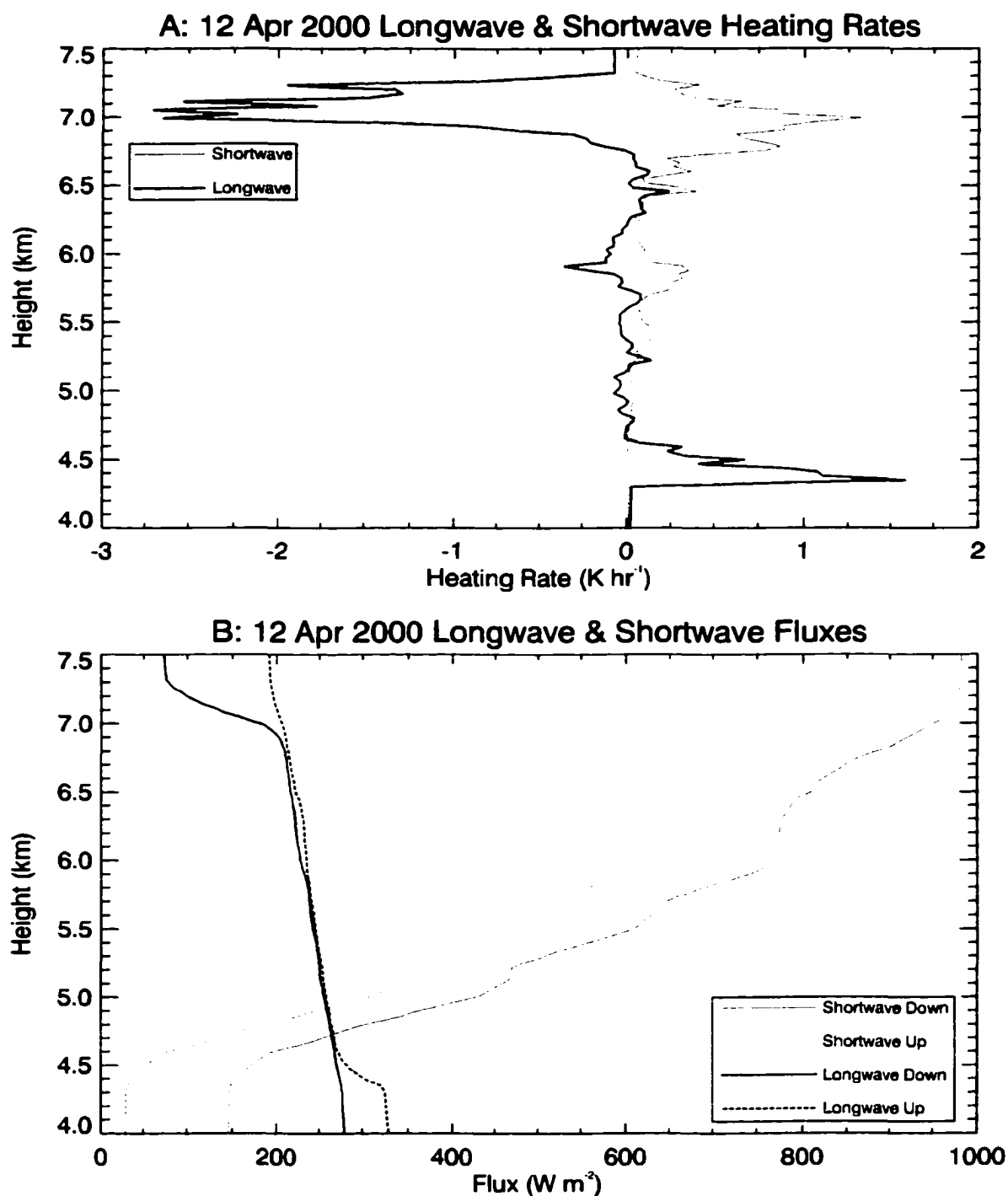
Figure 9.6 Same as previous four figures except for 12 Apr 00. Despite relatively high amounts of lwc and iwc through this system, the maximum longwave cooling and shortwave heating rates are only 2.7 and 1.3 \text{ K hr}^{-1} , respectively. This is due to lwc decreases at the top of the cloud and radiative interactions between the layers.
