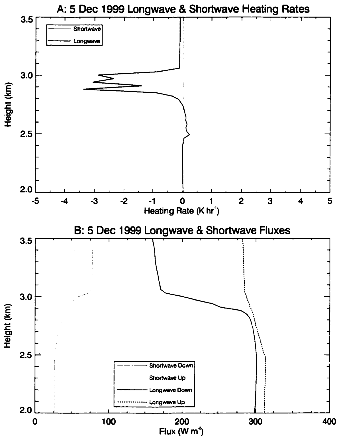
Figure 9.4 Same as previous two figures except for 5 Dec 99. Despite having the largest maximum lwc of any case, the maximum cooling rate is a relatively modest 3.4 \text{ K hr}^{-1} , because of a dry air entrainment-induced reduction in lwc at cloud top.
