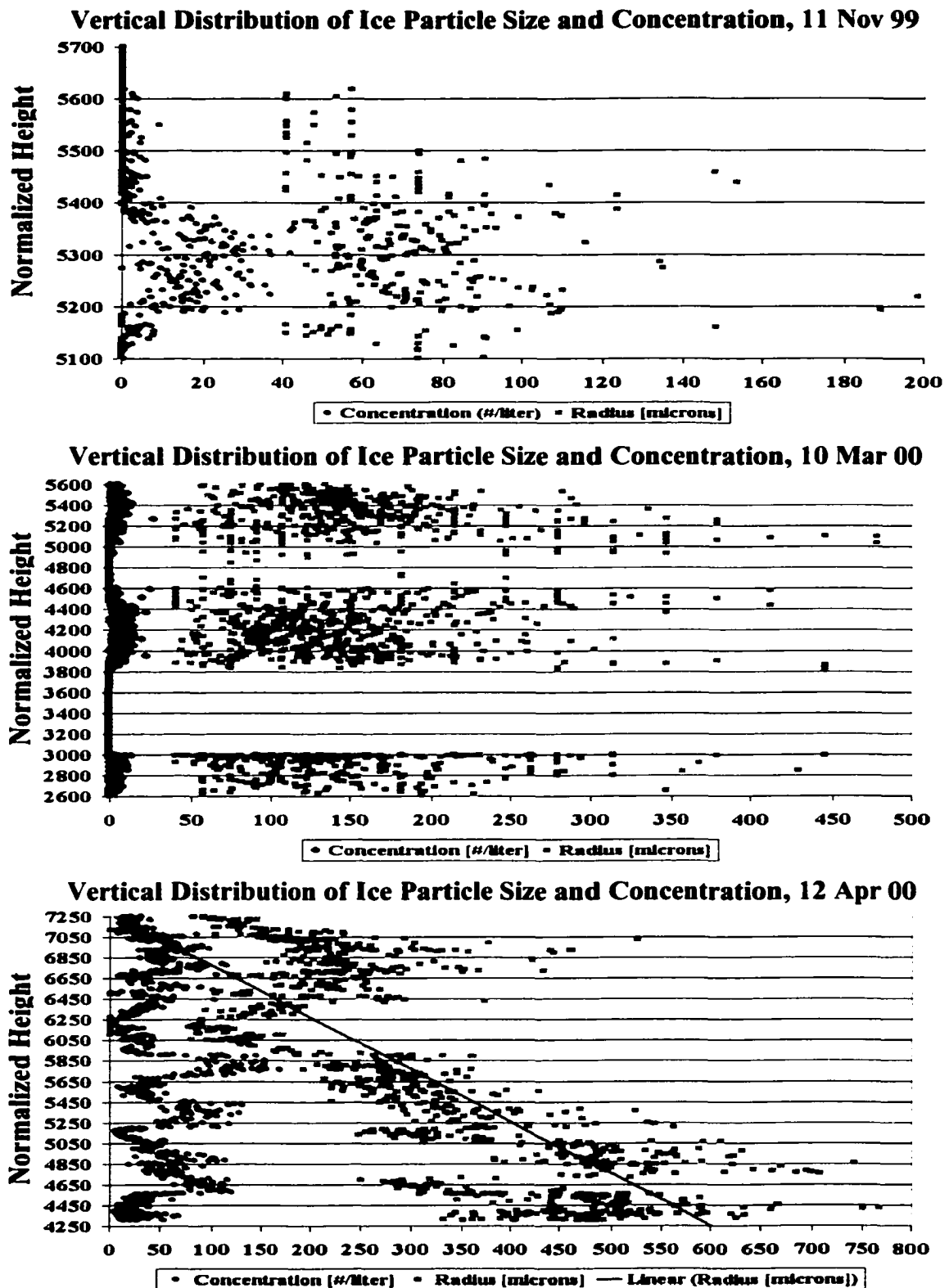
Figure 5.18 Differences in vertical distribution of particle size and concentration between single layers (top) and multiple layers (middle and bottom). Note the increase in particle concentration at the bottom of the single layer cloud, the uniform distribution of both size and concentration in the 10 Mar 00 case, and the increase in size with decreasing altitude on 12 Apr 00.
