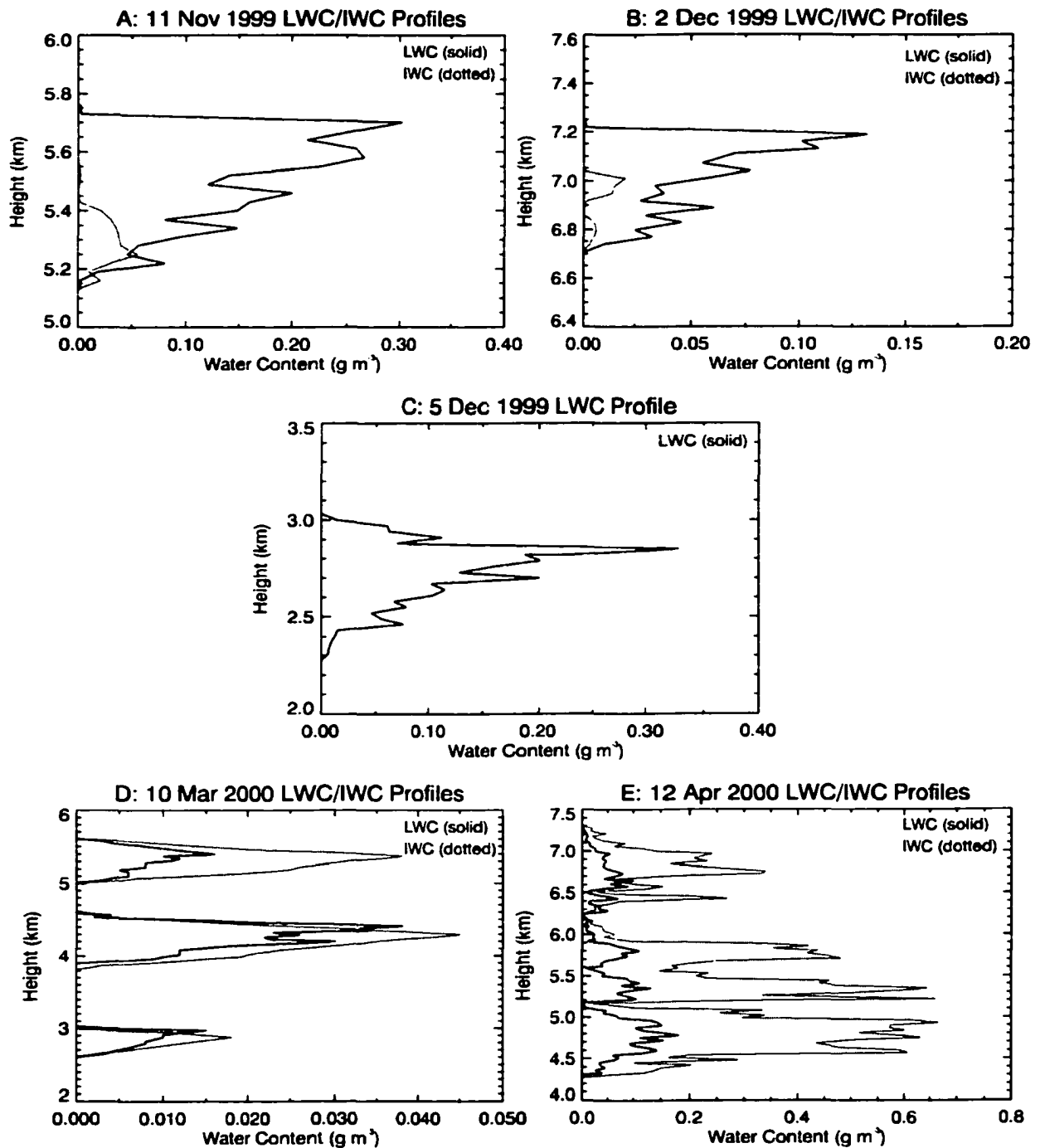
Figure 9.1 BUGSRAD model lwc and iwc input profiles for A) 11 Nov 99, B) 2 Dec 99, C) 5 Dec 99, D) 10 Mar 00 and E) 12 Apr 00. The model profiles use observed lwc and iwc values at 30 m vertical grid spacing and capture the main features of the observed profiles shown in Figures 5.7–5.12.
