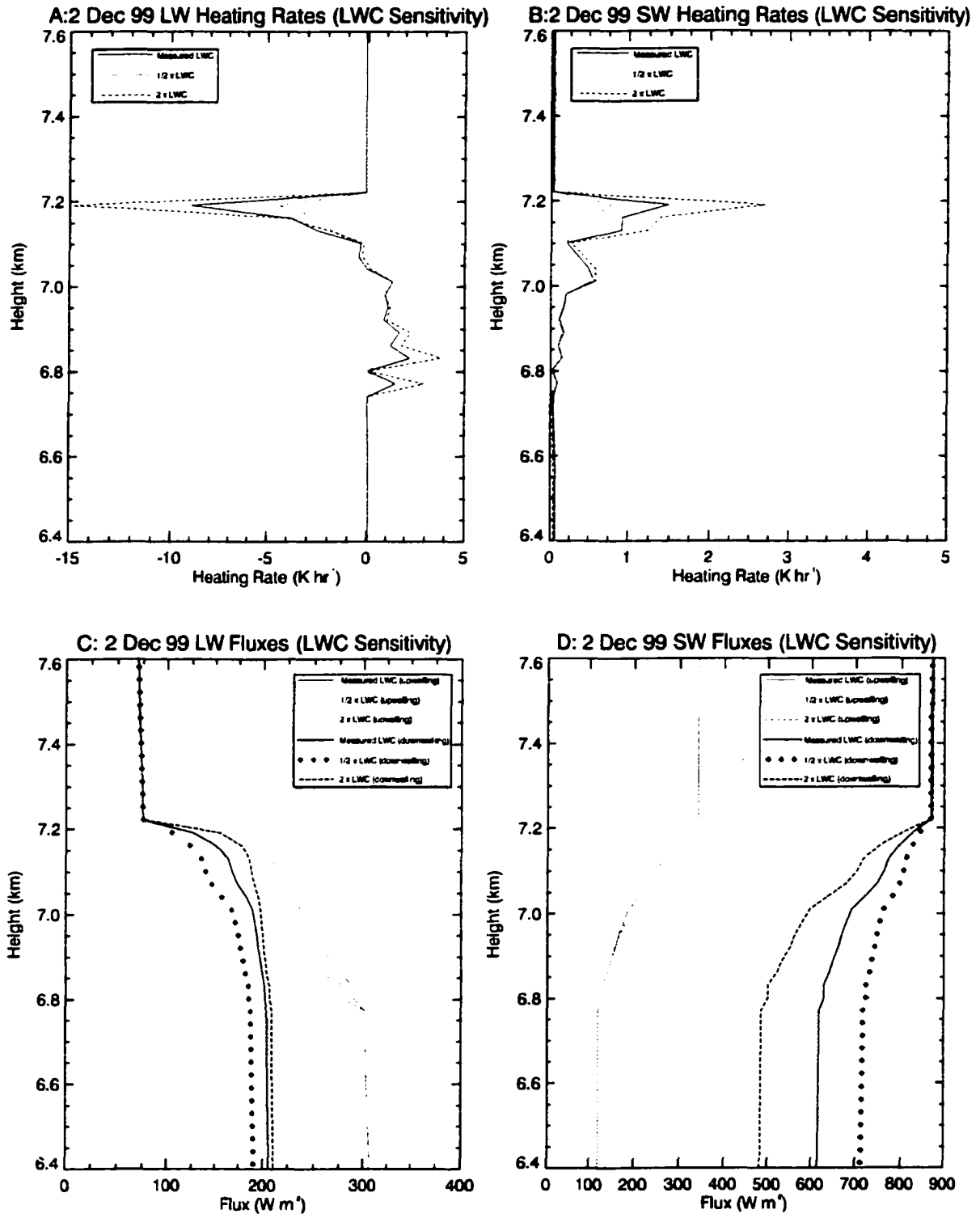
Figure 9.9 Same as previous figure except for 2 Dec 99 case. Longwave cooling and shortwave heating both occur at or near cloud top, while longwave heating occurs near cloud base. Note the change in scale and refer to Tables 9.1 and 9.2 for the values of radiative heating and cooling when the lwc is doubled and halved.
