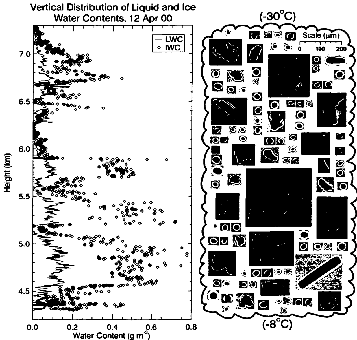
Fig 5.12 Same as previous figure except for 12 Apr 00. Note the relatively high lwc, despite large amounts of ice. The higher total water content leads us to believe this cloud was more strongly forced than the 10 Mar 00 case. A seeder-feeder process is evident, with ice between the layers.
