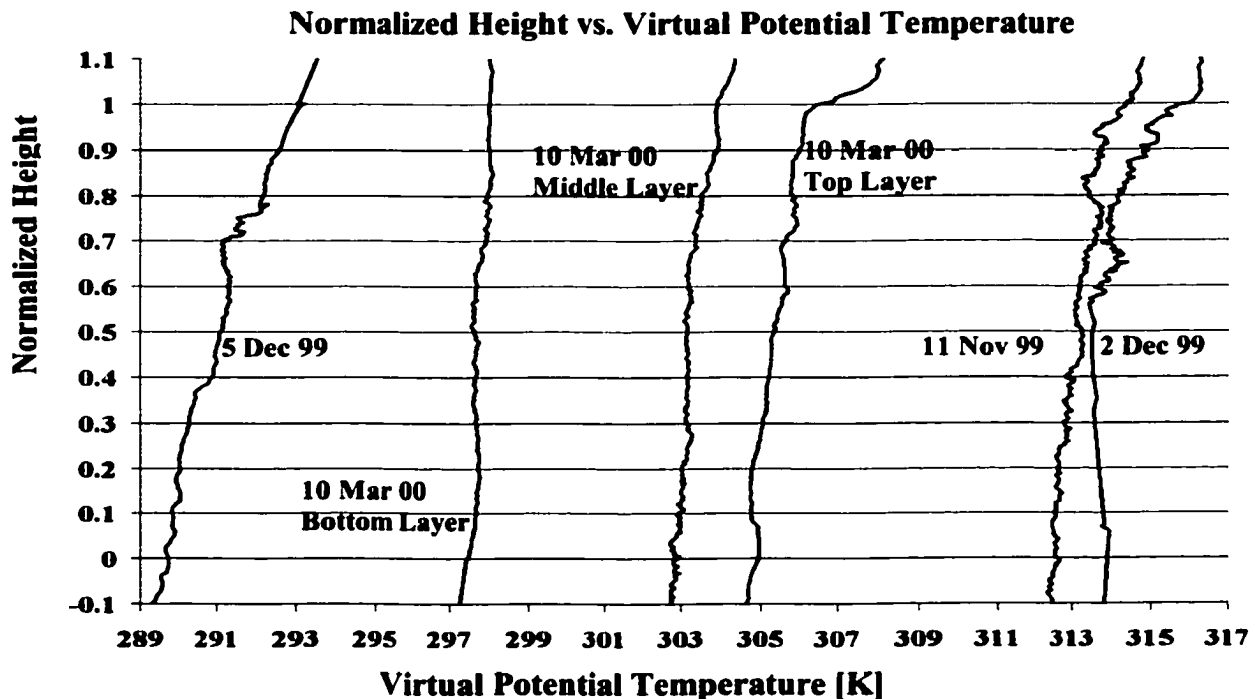
Fig 5.20 Vertical profiles of virtual potential temperature for the same cases as in Figure 5.19. This variable allows for slightly easier determination of mid-level cloud boundaries than temperature inversions, as there is a 1-2 K increase of \theta_v at cloud top (not seen at the top of the bottom and mid layers of 10 Mar 00 case).
