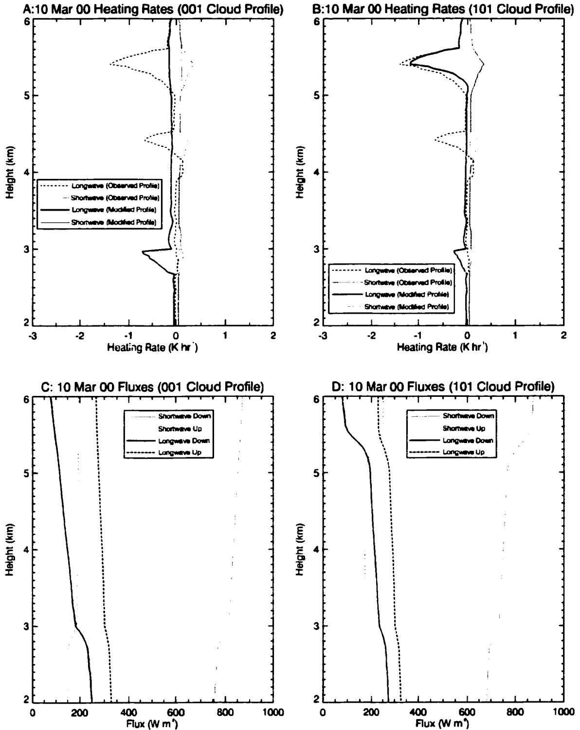
Figure 9.24 Same as Fig 9.23 except for cases in which only the bottom layer is included (001) and only the top and bottom layers are included (101). Note the longwave cooling in the bottom layer in the absence of intervening layers aloft.
