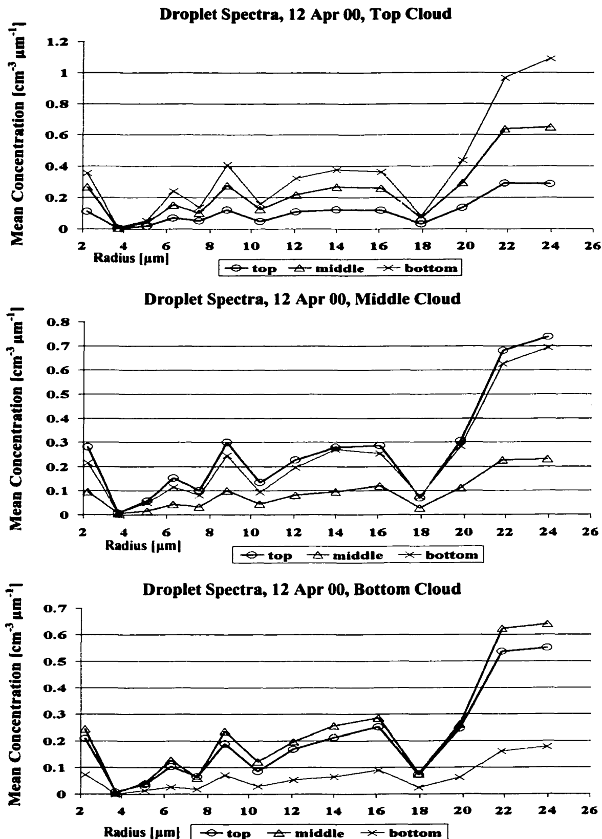
Figure 5.15. Same as figure 5.14, except for 12 Apr 00. The distribution of sizes with concentration is again fairly homogeneous. The increase at sizes greater than 20 μm may be due to some contamination by larger ice particles in those bins.
