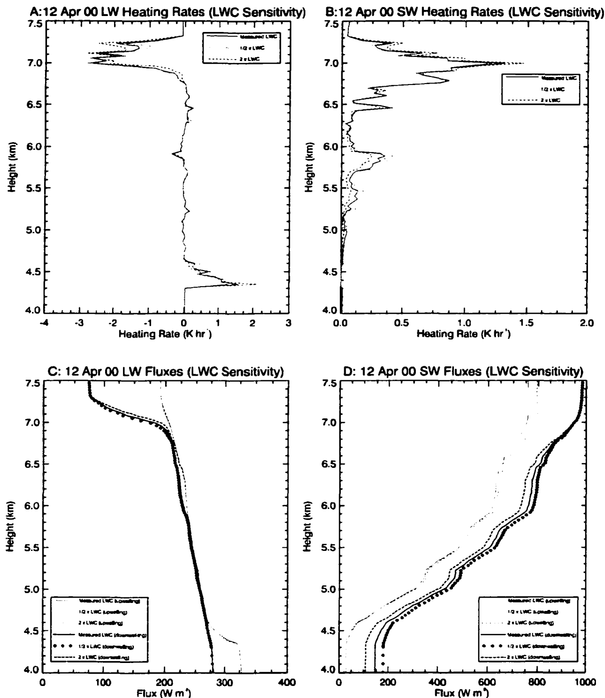
Figure 9.12 Same as previous four figures except for 12 Apr 00. Note the small changes in fluxes and heating rates when the lwc is doubled and halved; this is due both to decreasing lwc with height at the cloud top, similar to that seen in Fig 9.10 for the 5 Dec 99 case, and to the radiative interactions with adjacent cloud layers.
