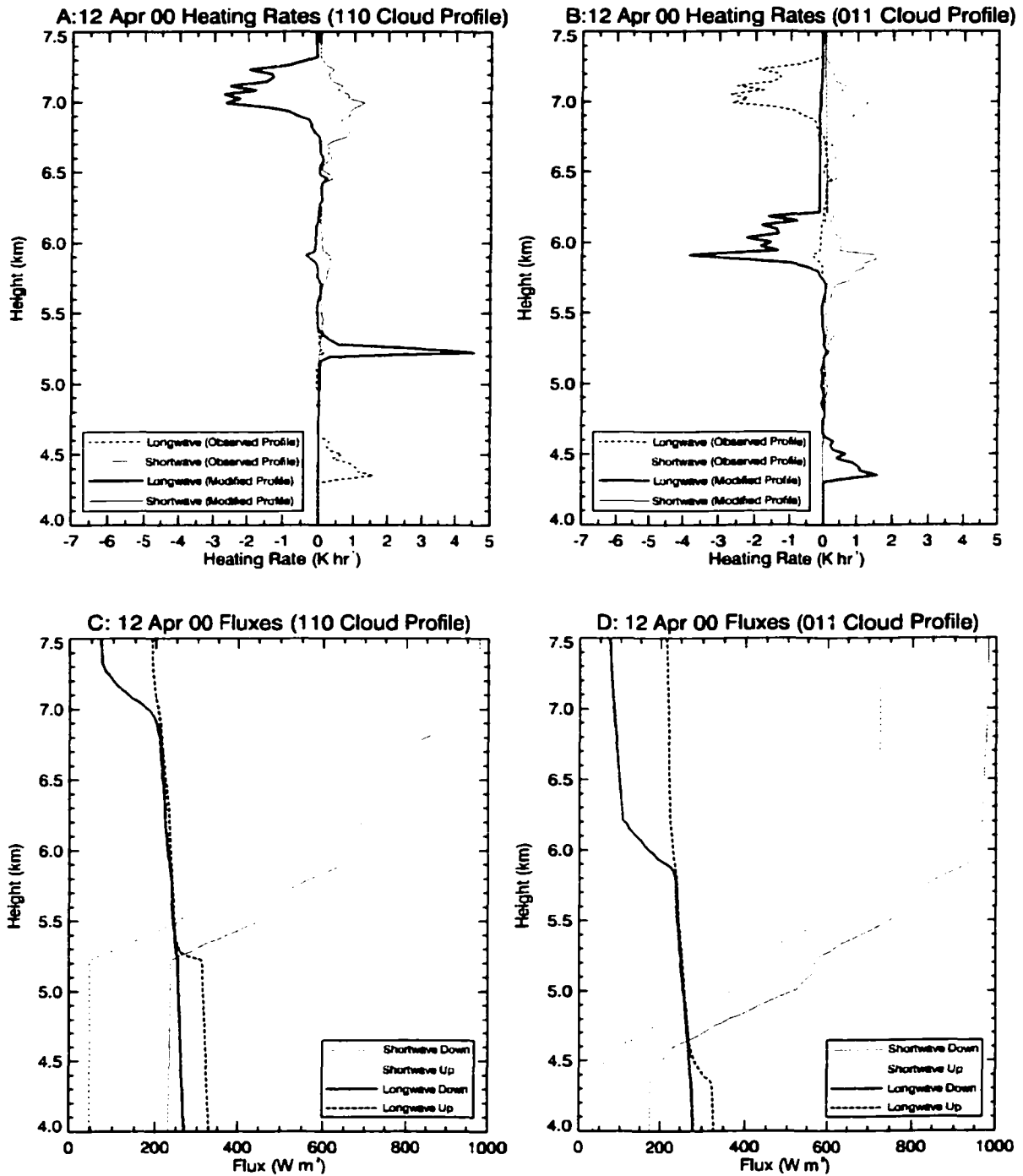
Figure 9.28 Same as Fig 9.25 except for 12 Apr 00. Note that the bottom of the lowest layer and the top of the top layer interact radiatively as if they were a single cloud layer. However, since the differential heating acts over a greater vertical distance with multiple layers, the radiatively driven circulations will be weaker.
