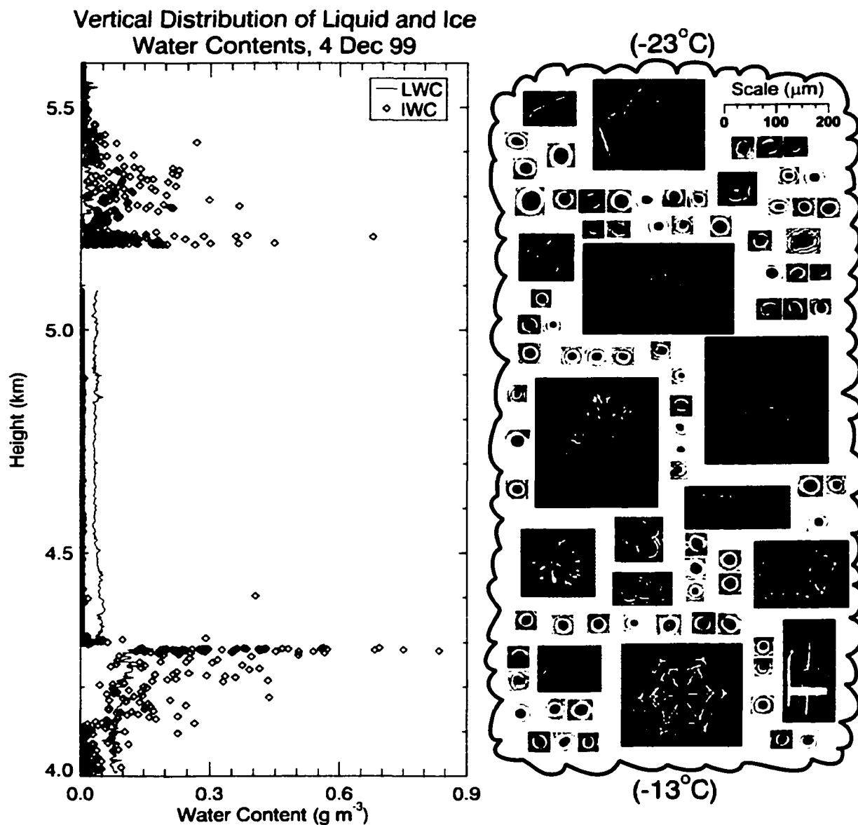
Figure 5.9 Same as the previous two figures except for 4 Dec 99. This cloud was “psuedo-convective”, as it was detrained from convection upstream and then advected over the ARM site. The two discontinuities in lwc and iwc are a result of air traffic control delays of up to 15 minutes.
