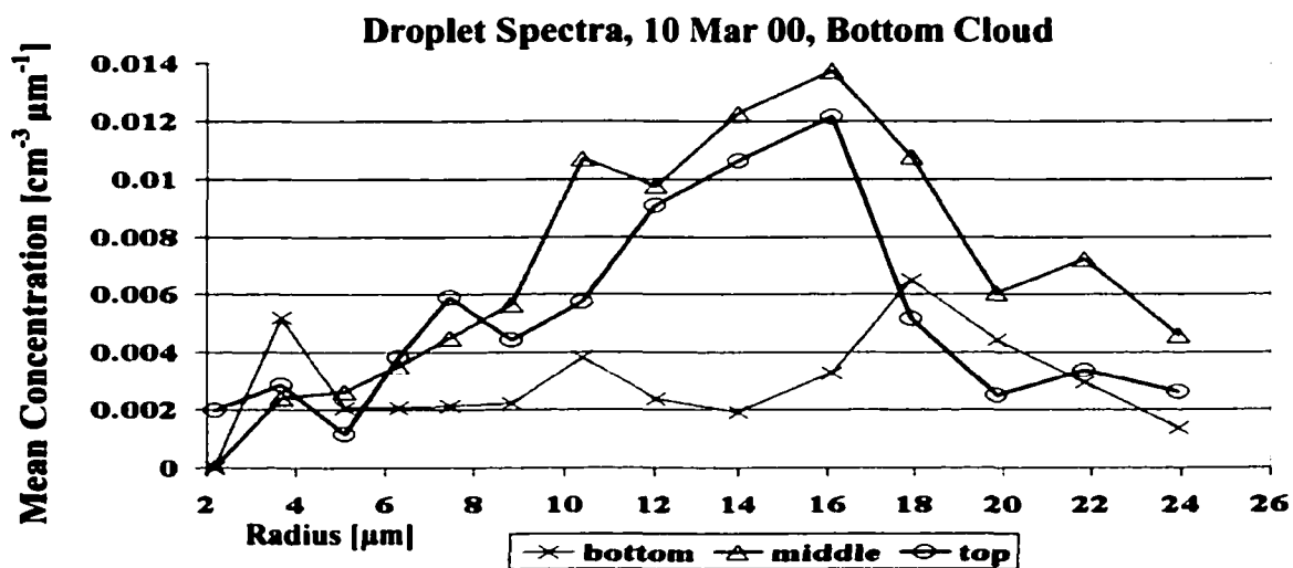
Figure 5.14 Same as figure 5.13, except for the multi-layered system observed on 10 Mar 00. Note the different vertical scales and the absence of droplet size and concentration with height, due to seeder-feeder processes and the presence of more ice particles in this system.
