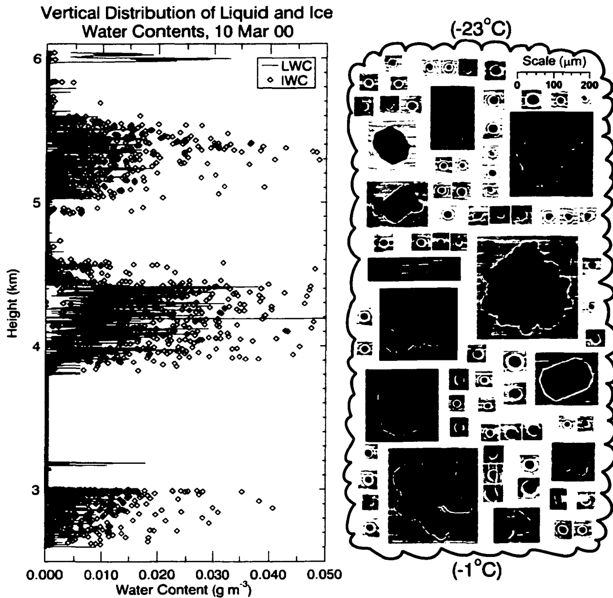
Fig 5.11 Same as previous four figures except for multi-layered cloud on 10 Mar 00. Note the relatively low lwc values and the homogeneous vertical distribution of iwc.
