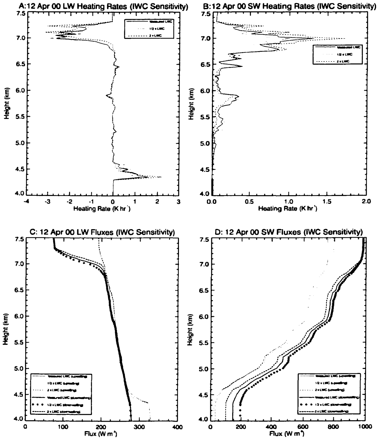
Figure 9.16 Same as previous figure except for 12 Apr 00. The sensitivity to iwc is also evident in this cloud, as the iwc values were relatively large and the ice particles were more evenly distributed with height than in the single-layer cases. For both multi-layer cases, heating rates changed 25-30% when iwc was doubled or halved.
