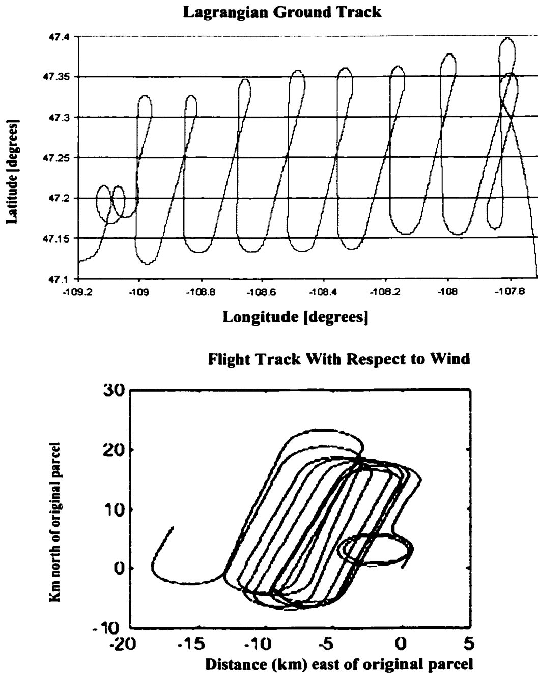
Fig 3.1 Lagrangian racetrack pattern flown on 11 Nov 99. The aircraft drifted with a cloud parcel embedded in westerly flow (top) and the same track with the winds subtracted (bottom).
