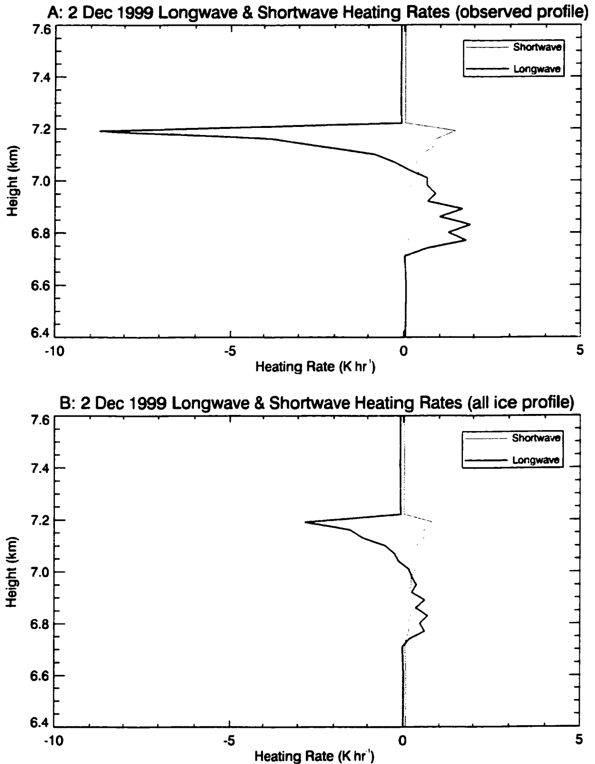
Figure 9.17 Sensitivity of heating rate profiles to model parameterization of cloud phase. (A) shows the heating rate profile using the measured lwc and iwc values; (B) shows the same profile when the cloud is converted completely to ice, as it would be in current models that determine water phase by temperature.
