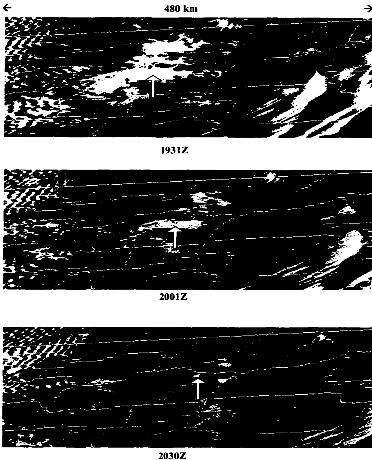
Fig 8.1 Time series of GOES-8 visible satellite images of the 11 Nov 99 cloud that coincides with the time of the CLEX-5 Lagrangian aircraft measurements. The
