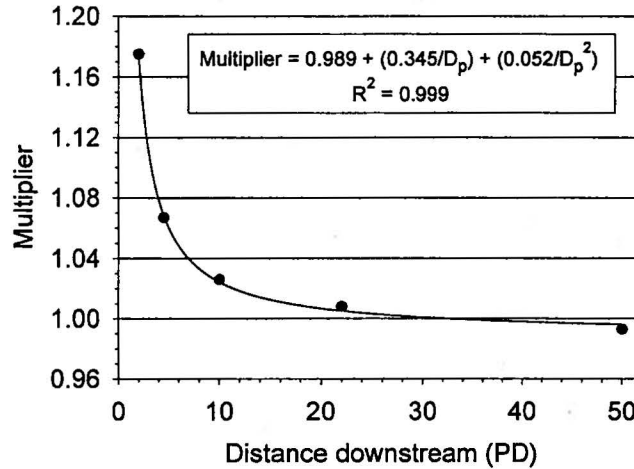
Figure 6. Bias-correcting multiplier.
