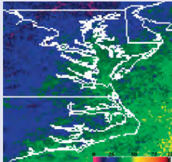
Figure 4. Percent cloud cover for the North wind regime, Aug-Oct, 1998-2000, 1245 UTC.
