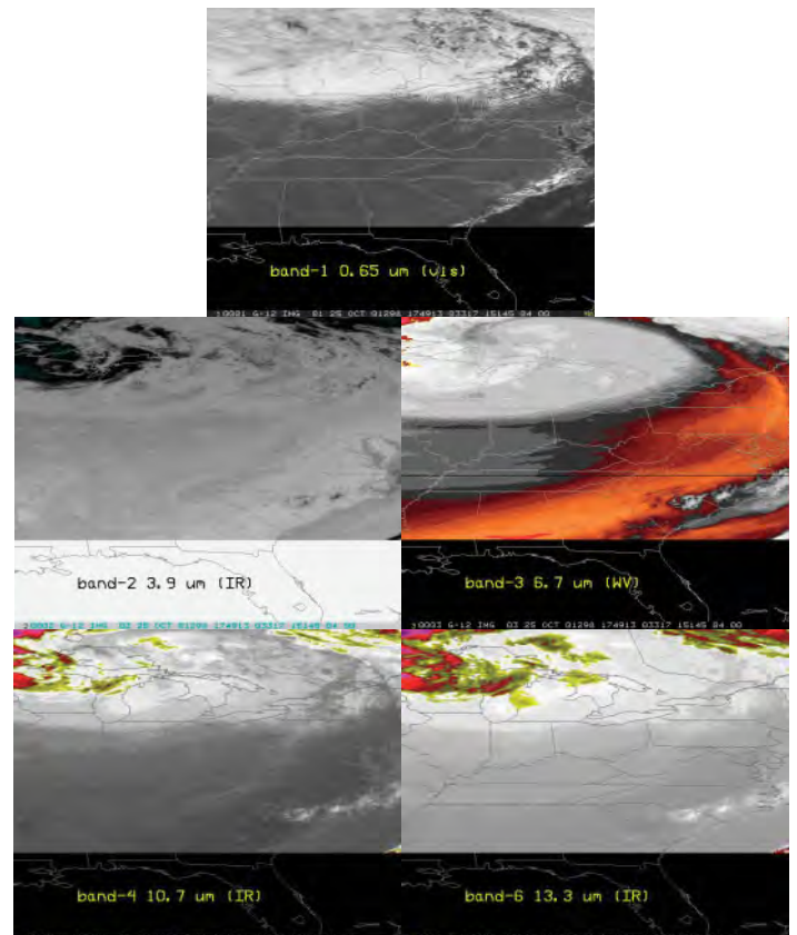
Figure 1: Examples of GOES-12 bands 1 through 4 and 6 with color enhancements applied to the infrared bands.
