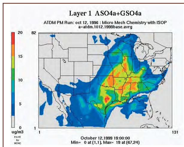
Figure 2. Surface sulfate concentrations predicted by the REMSAD air quality model for the BRAVO study. Total sulfate concentrations are the sum of gas-pathway sulfate (GSO4) and aqueous-pathway sulfate (ASO4). Sulfate particles are a major cause of reduced visibility in many regions of the U.S.
