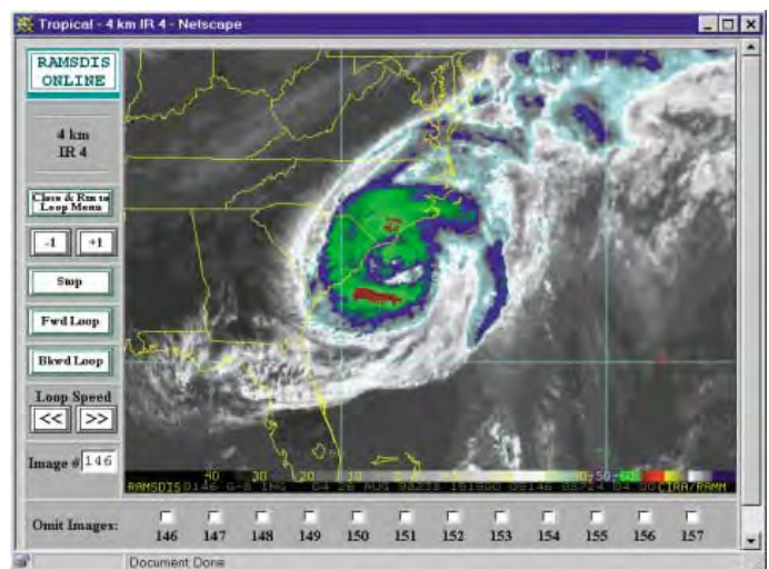
Figure 3: GOES channel-4 (10.7 \mu\text{m} ) infrared image at 4 km spatial resolution showing Hurricane Bonnie.
