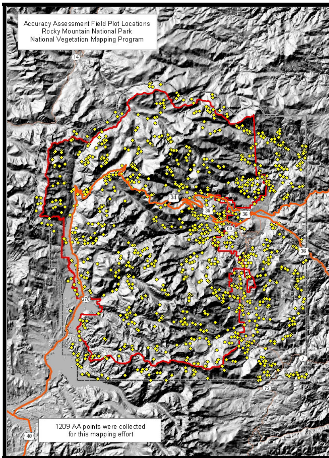
Figure 10. Distribution of accuracy assessment points, ROMO and environs.
