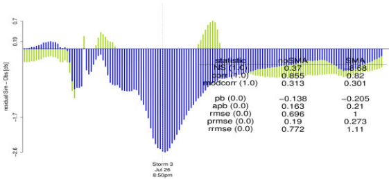
Figure D.2.18: California Gulch at Arkansas—CG-6 gauge from July 26–27, 2006.
