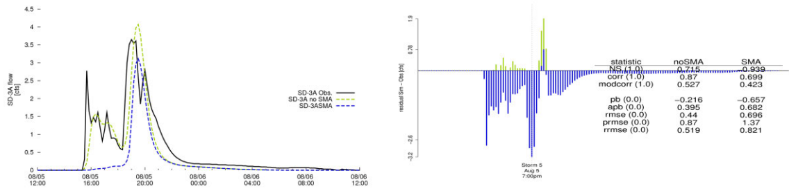
Figure D.2.26: Starr Ditch—SD-3A gauge from August 5–6, 2006.
