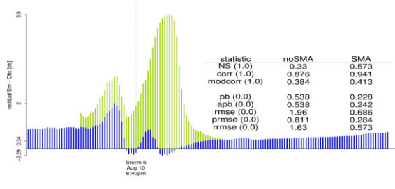
Figure D.2.41: California Gulch above WWTP—CG-5 gauge from August 10–11, 2006.
