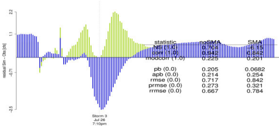
Figure D.2.17: California Gulch above WWTP—CG-5 gauge from July 26–27, 2006.
