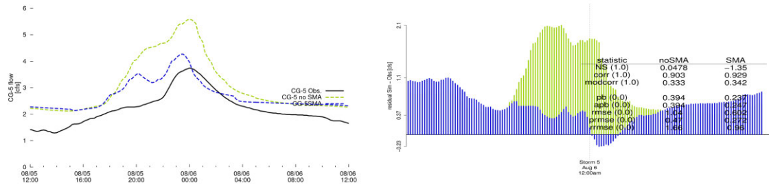
Figure D.2.29: California Gulch above WWTP—CG-5 gauge from August 5–6, 2006.
