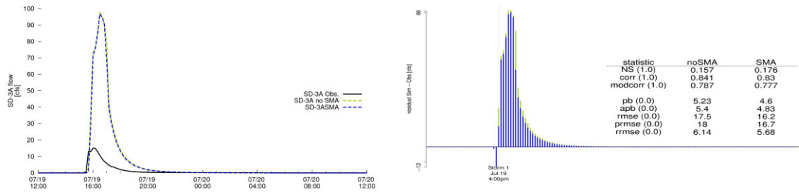
Figure D.2.2: Starr Ditch—SD-3A gauge from July 19–20, 2006.
