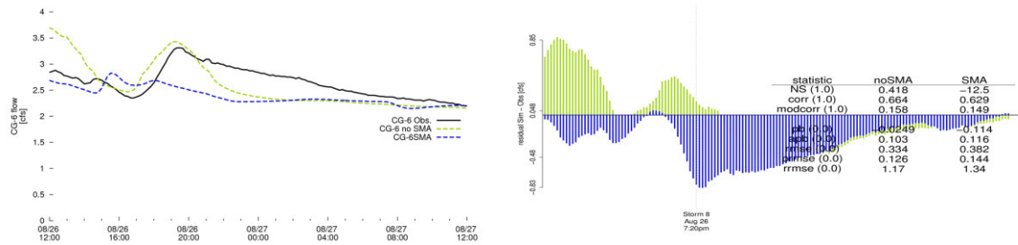
Figure D.2.54: California Gulch at Arkansas—CG-6 gauge from August 26–27, 2006.
