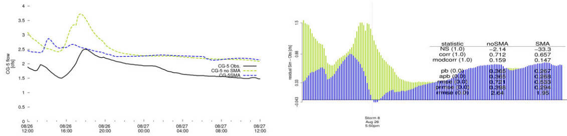
Figure D.2.53: California Gulch above WWTP—CG-5 gauge from August 26–27, 2006.
