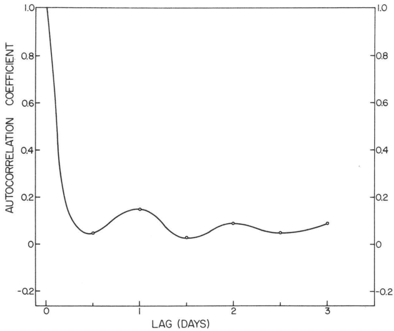
Fig. 30. Correlogram of observed veering at Swan Island in layer from surface to 900 mb. Note lack of persistence of veering. Sample size: 2048 observations.
