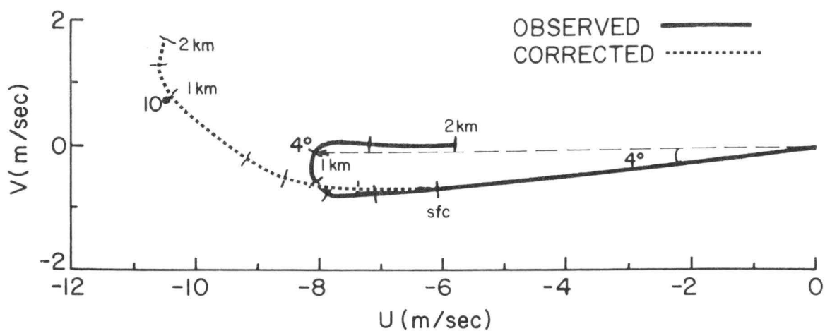
Fig. 7. Observed and geostrophically corrected hodographs at Johnston Island derived from 3667 observations. Elevation marks are shown at the surface, 150, 300, 500, 1000, 1500, and 2000 m. Veering angle between the surface and 1000 m is noted on each hodograph. Observed veering is 4^\circ and corrected veering, 10^\circ .
