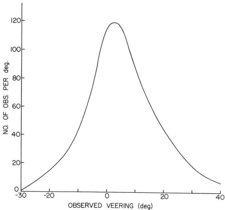
Fig. 31. Smoothed frequency distribution of veering at Johnston Island in the layer from surface to 900 mb. Sample size: 3696 observations.
