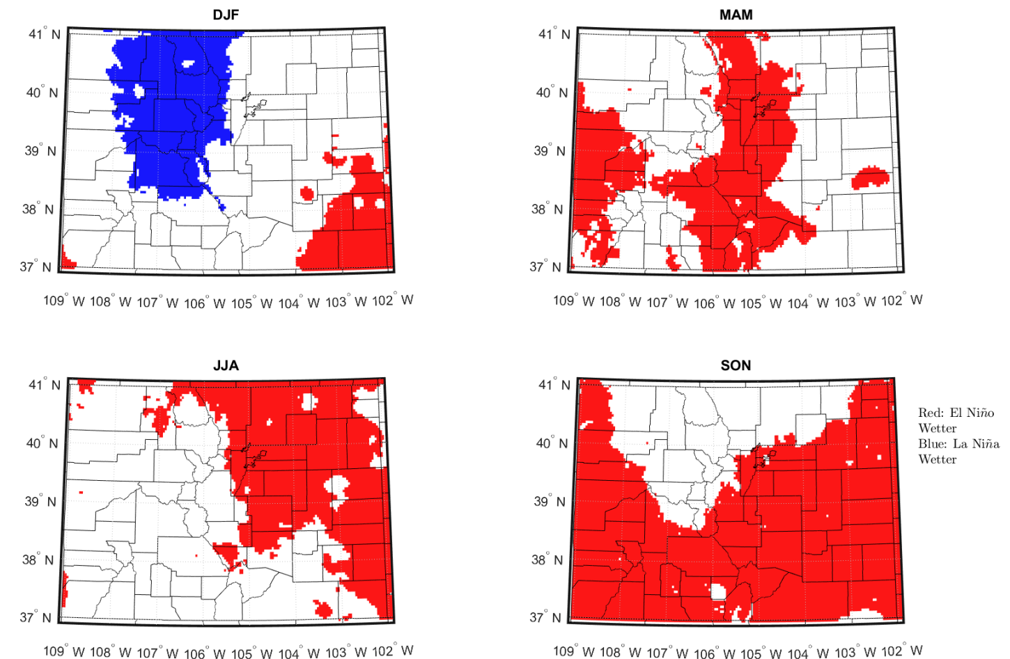
General Relationship Between El Niño Southern Oscillation (ENSO) and Colorado Precipitation
