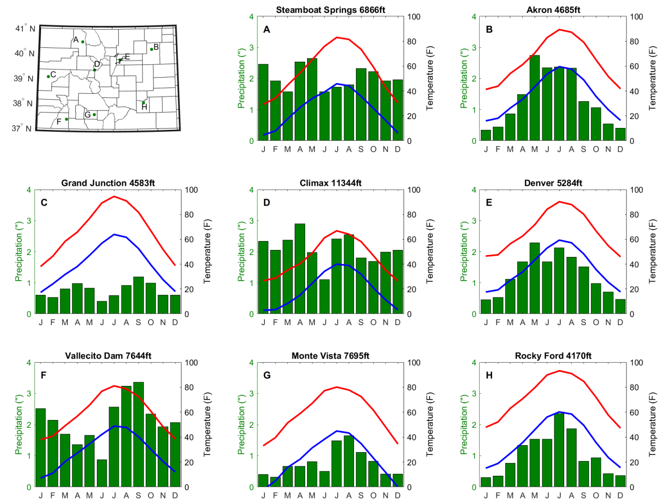
Figure 2.1: 1991-2020 normal monthly precipitation (green bars), daily average maximum (red line) and daily average minimum (blue line) temperatures for eight National Weather Service Cooperative Observer Program (COOP) stations around the state. Precipitation in inches and temperature in degrees Fahrenheit. Locations of the eight stations are labeled on the top left map.
