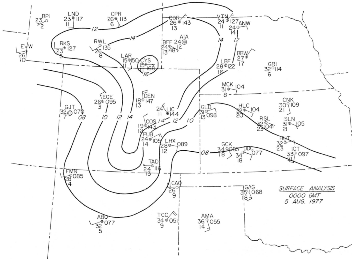
Fig. 4-3. Surface pressure pattern for 0000 GMT, 5 August 1977 for Colorado and portions of Kansas, Wyoming, and Nebraska. (Temperatures in °C.)
