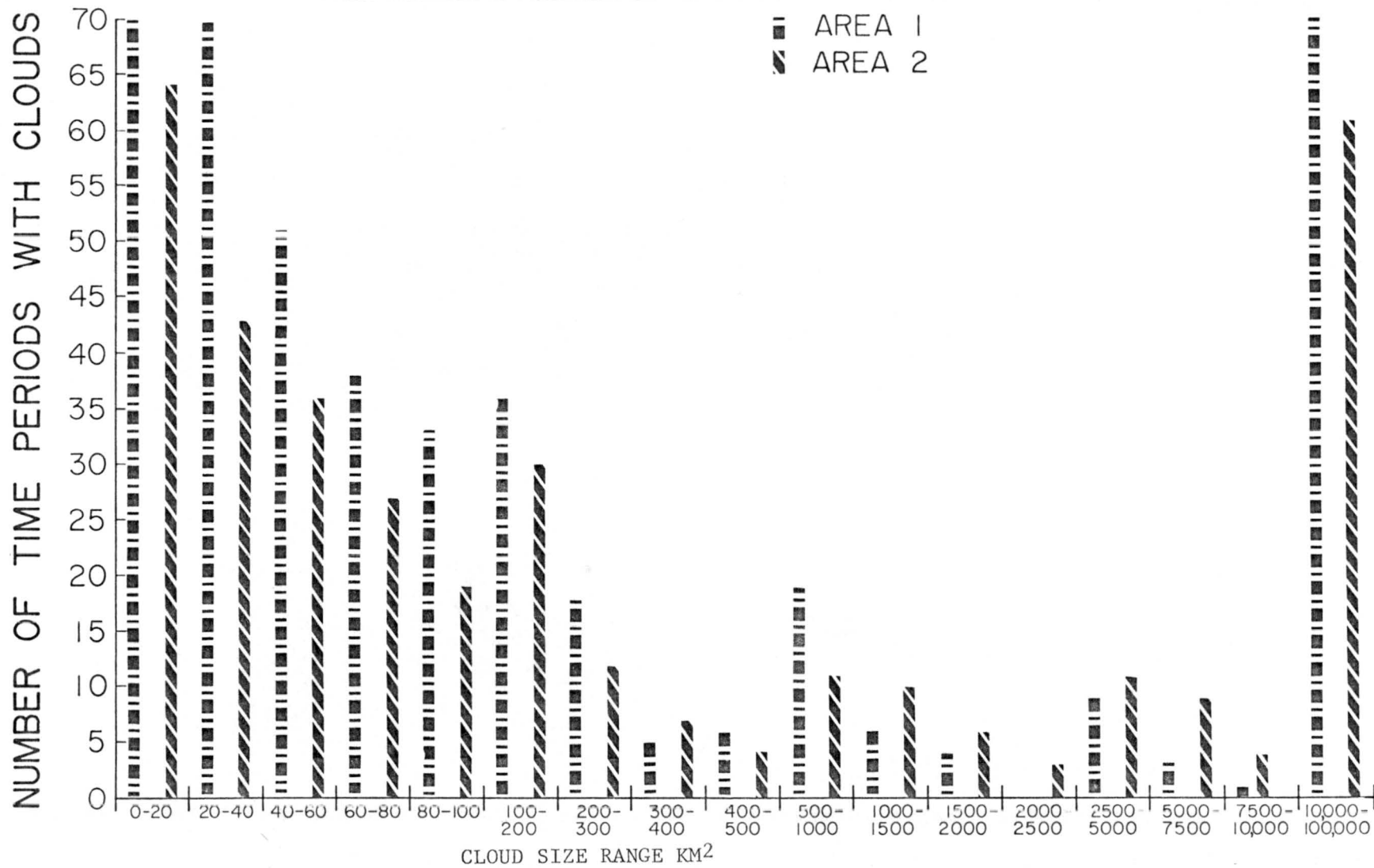
Fig. 4-14 Number of time periods (total out of 70) having clouds by size range and area.
