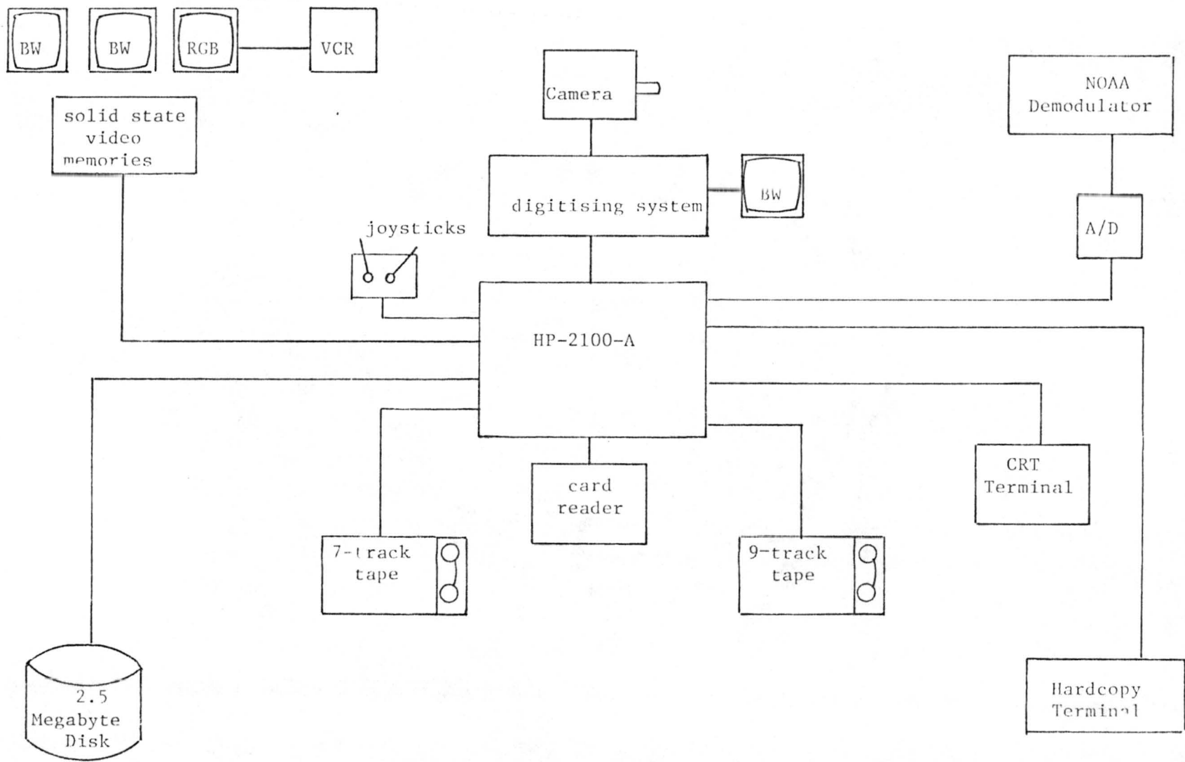
Figure B-1. Schematic illustration of the components of the ADVISAR.
