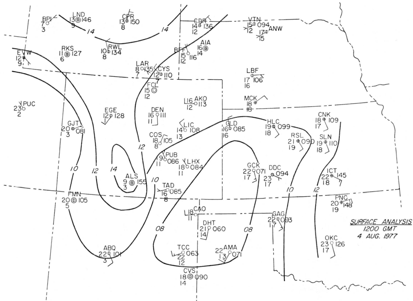
Fig. 4-2. Surface pressure pattern for 1200 GMT, 4 August 1977 for Colorado and portions of Kansas, Wyoming, and Nebraska. (Temperatures in °C.)
