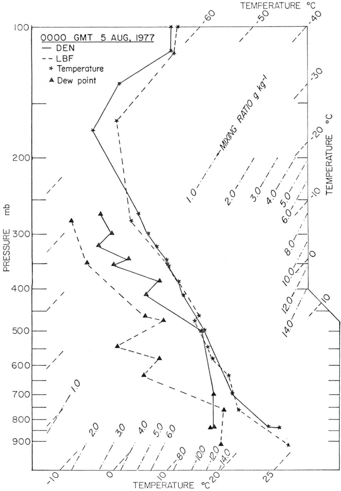
Fig. 4-5. Upper air soundings for DEN and LBF for 0000 GMT, 5 August 1977.
