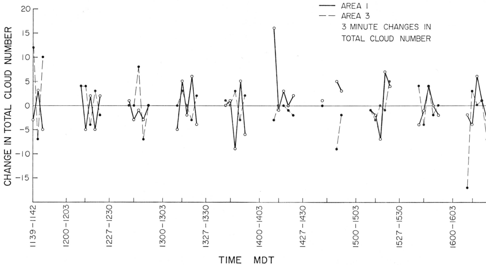
Fig. 4-11 Changes in total cloud number over three-minute intervals from 1100 - 1624 MDT on 4 August 1977 for Areas 1 and 3.
