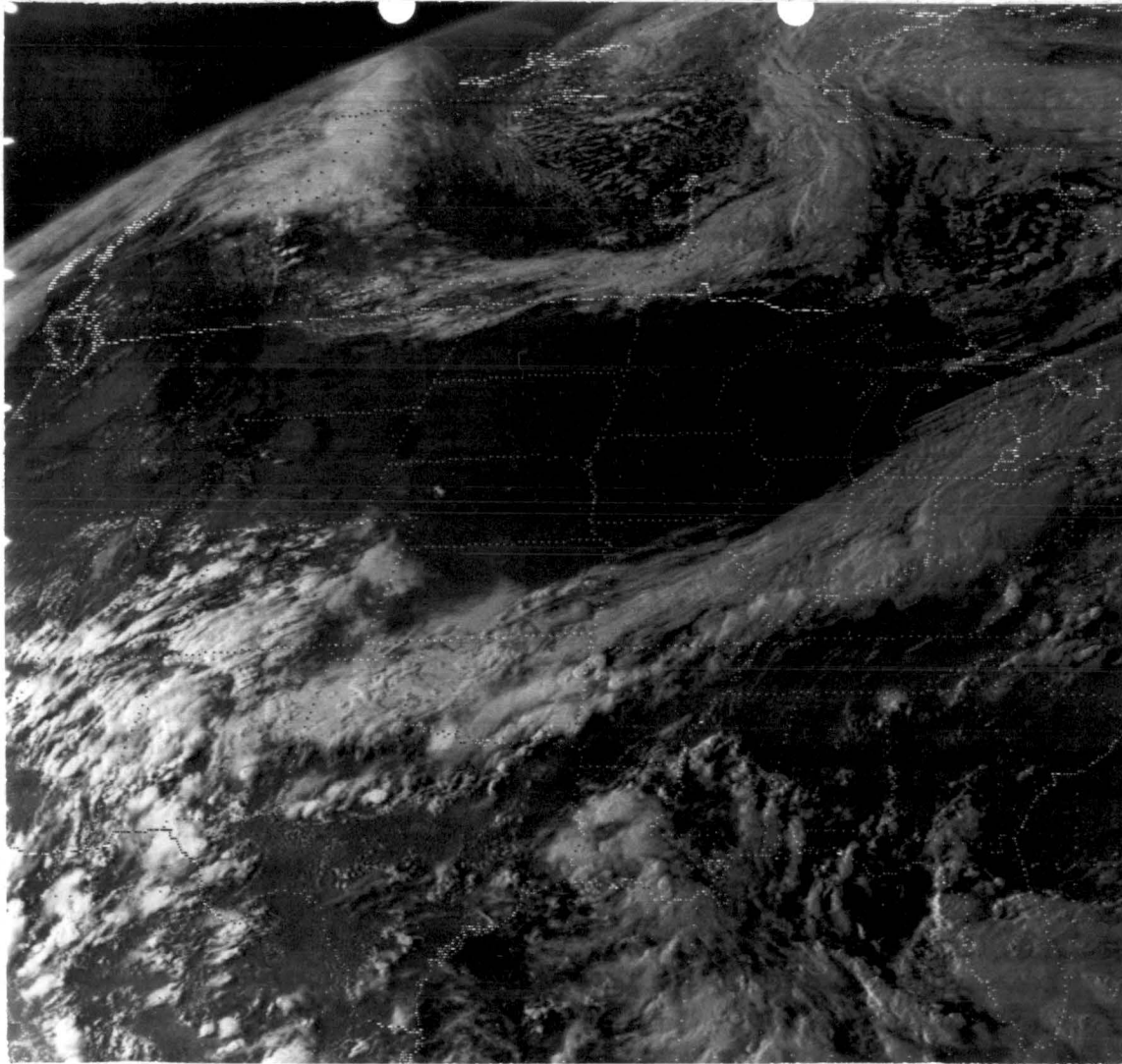
Fig. 3-8 Image for 11 August 1977, 2300 GMT, KB8 sector showing clouds in a patchy developmental pattern.
