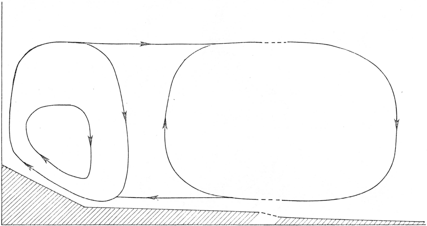
Fig. 2-1 Schematic representation of mountain - plains circulation system (from Dirks, 1969).
