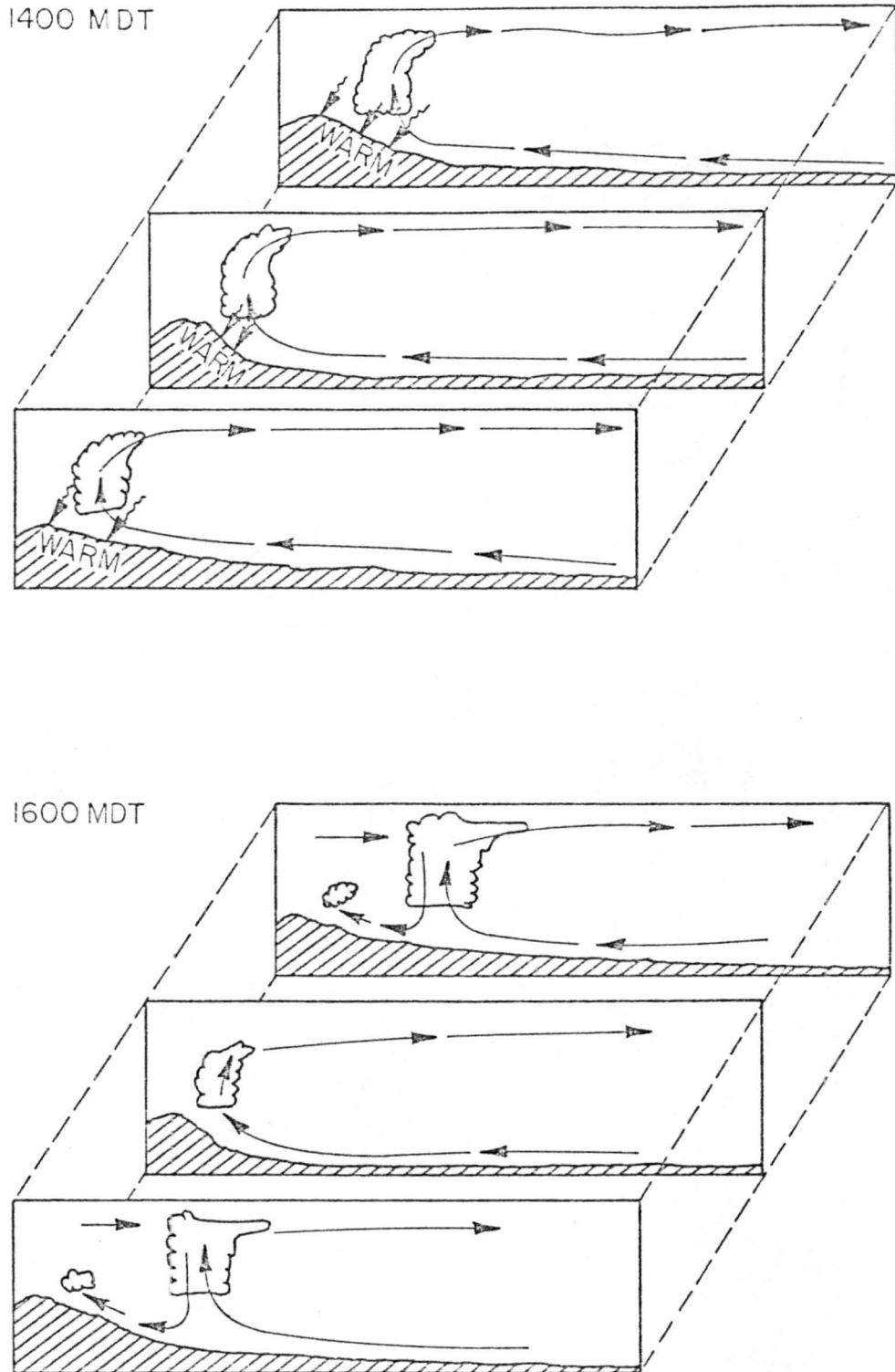
Fig. 2-2 Schematic representation of mountain - plains circulation as it may appear for 1400 and 1600 MDT. The three sections represent the northern, central, and southern portions of the study area (from Wetzel, 1973)
