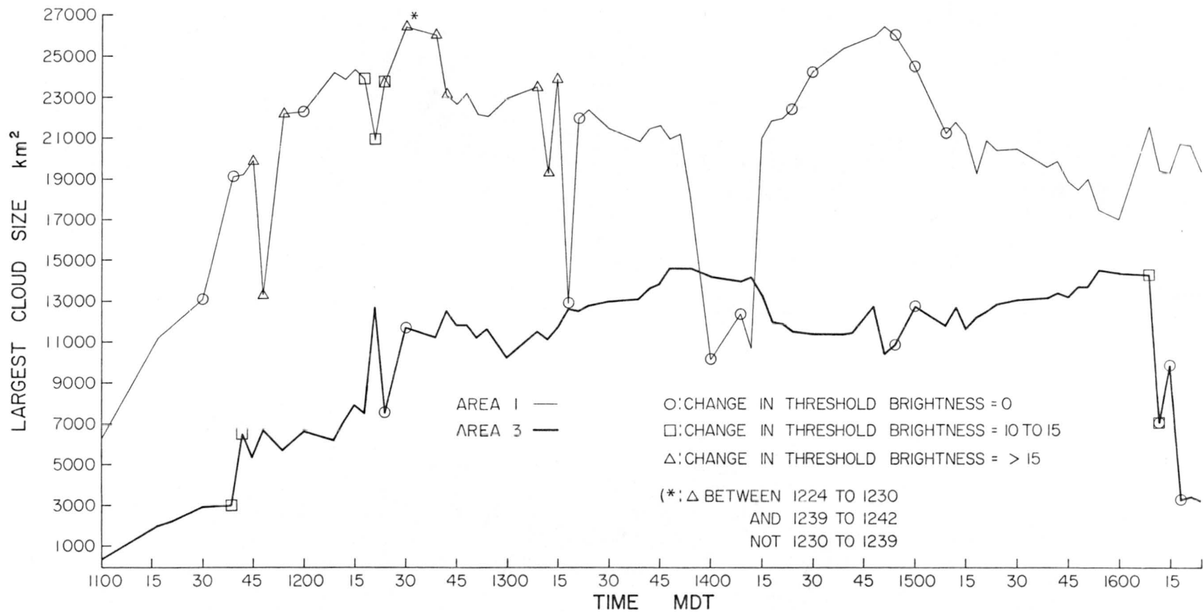
Fig. 4-15 Changes in largest cloud size vs. time for Areas 1 and 3. (Symbols on the graph represent the magnitude of threshold brightness changes occurring between successive times when large changes in largest cloud size occurred.)
