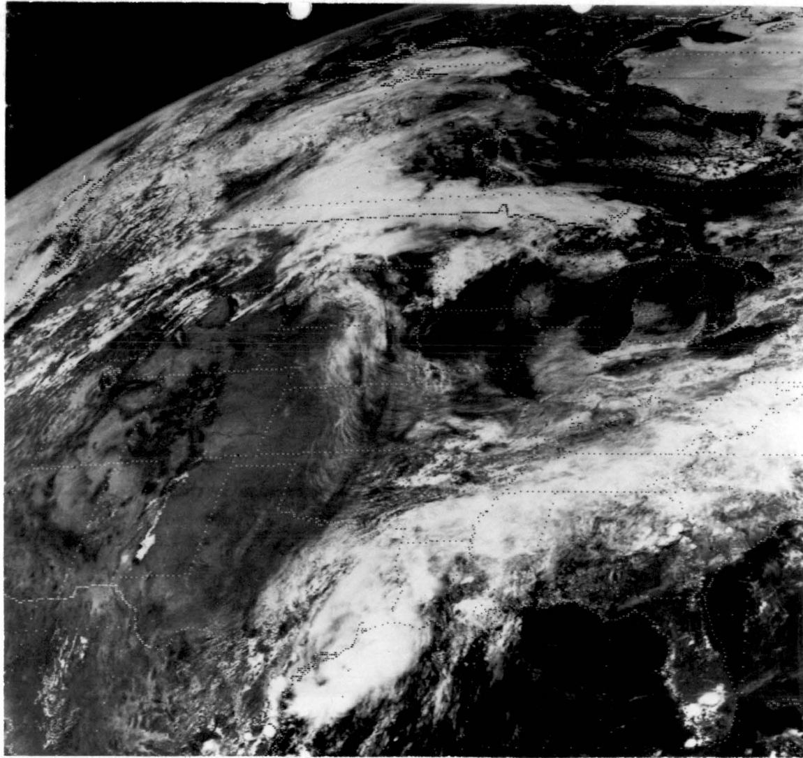
Fig. 3-5 Image for 4 June 1977, 1830 GMT, KB8 sector with some line organization of cloud elements evident.
