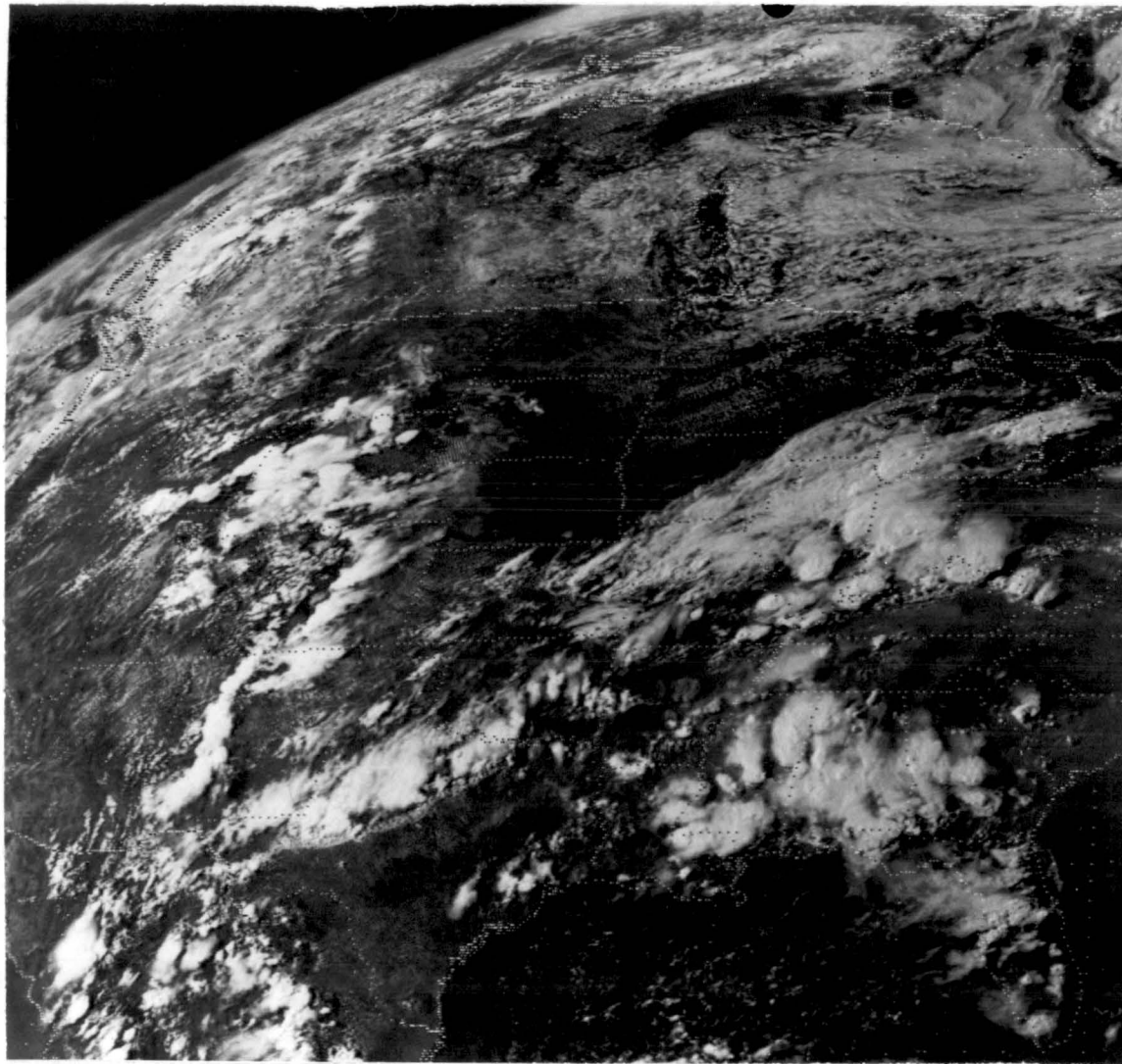
Fig. 3-7 Image for 8 July 1977, 2230 GMT, KB8 sector showing further development of convective cells.
