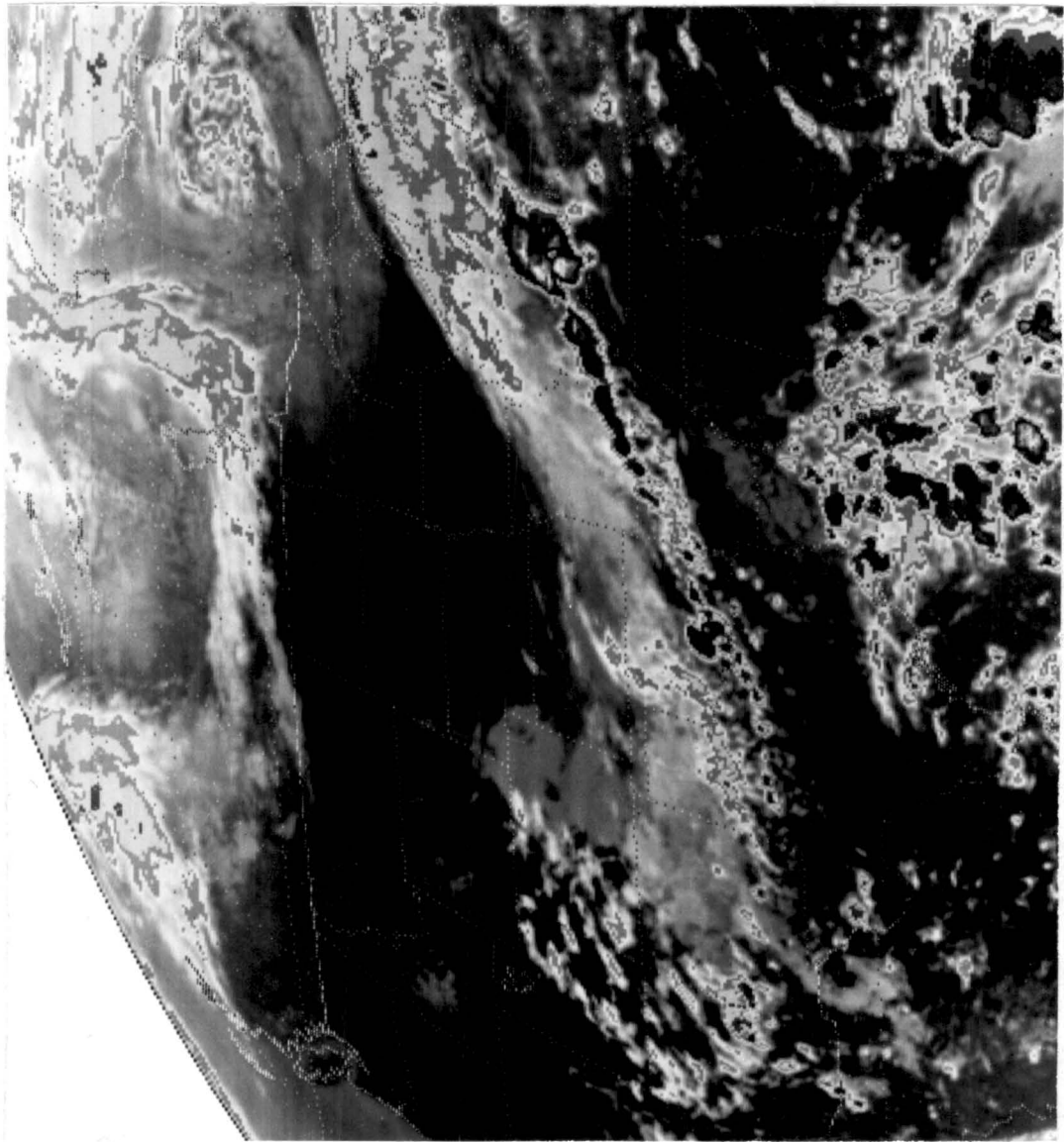
Fig. 3-4 Image for 11 August 1977, 1930 GMT, KB8 sector.
