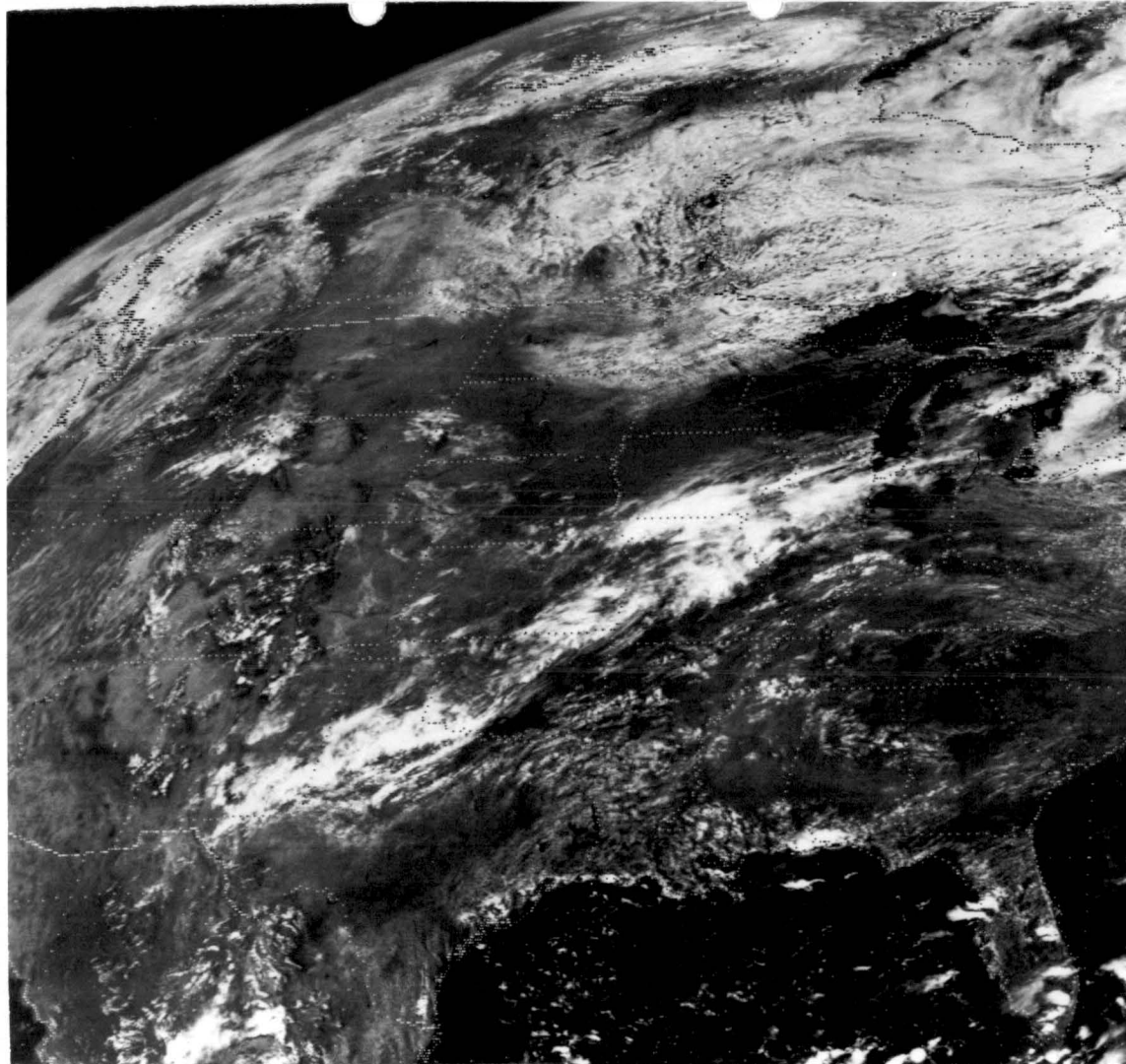
Fig. 3-6 Image for 8 July 1977, 1930 GMT, KB8 sector showing cumulus developing over the mountains.
