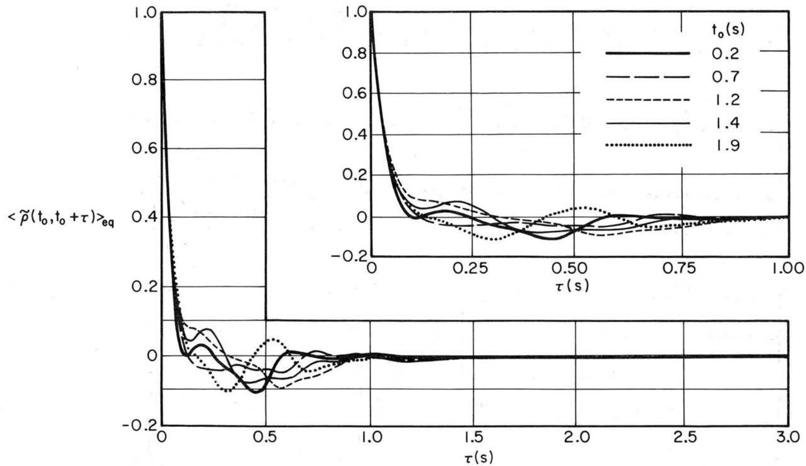
Fig. 6.11 Representative samples of the equivalent ensemble autocorrelation coefficients at five selected starting times t_0 .
