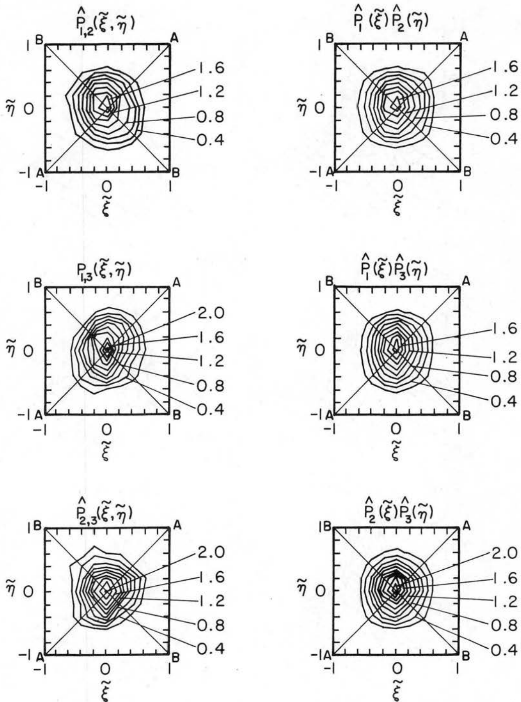
Fig. 6.8 Isoprobability curves of the joint probability density functions and products of individual probability density functions of the equivalent ensemble three sample records.
