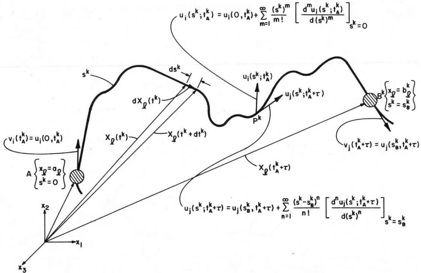
Fig. 3.4 Illustration of the distance s_B^k traveled by a fluid particle along its trajectory and of the Taylor series expansions of the Eulerian velocities at a point p^k on a path line.
