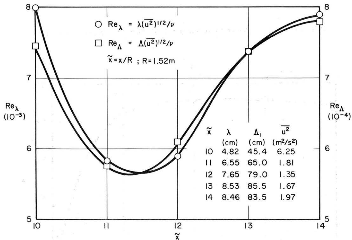
Fig. 6.16 Longitudinal variation of the micro and first integral scale Reynolds numbers along the turbulence line.
