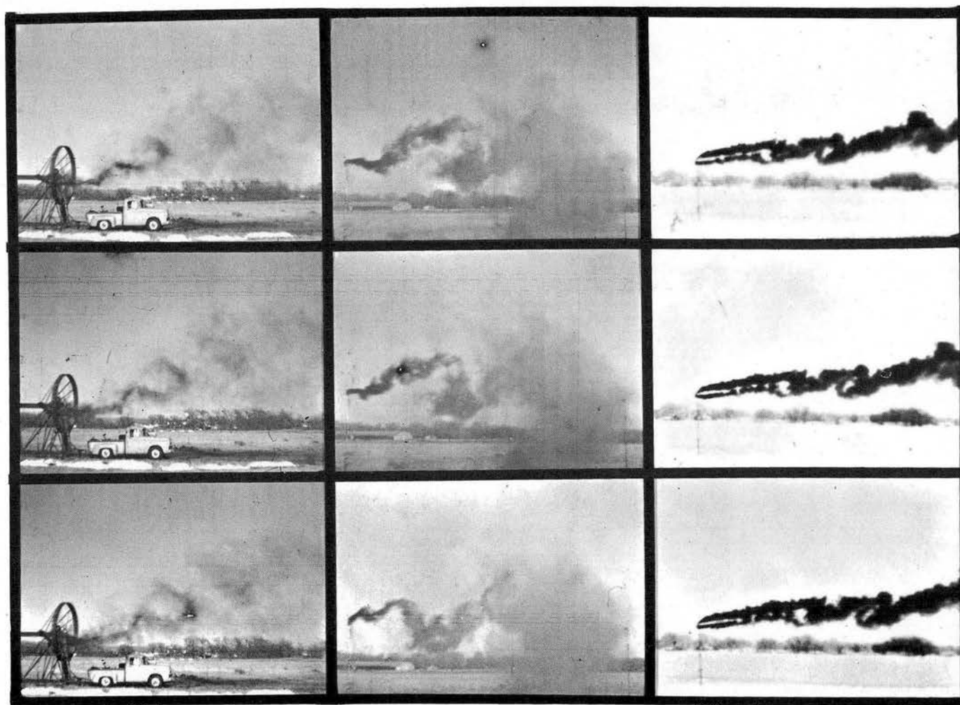
Fig. 6.4 Smoke plume circulation visualization: (1) unstable conditions (a) point source at x = -0.5R and (b) point source at x = 8R ; and, (2) under a temperature inversion (c) point source at x = 30R .
