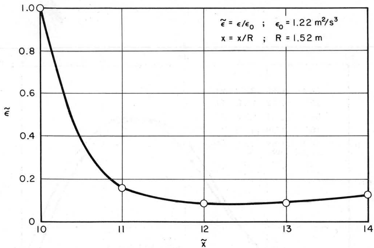
Fig. 6.17 Streamwise change of the dissipation along the turbulence line.
