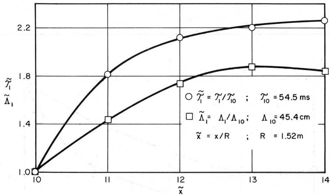
Fig. 6.15 Variation of the Eulerian first integral time and space scales along the turbulence line.
