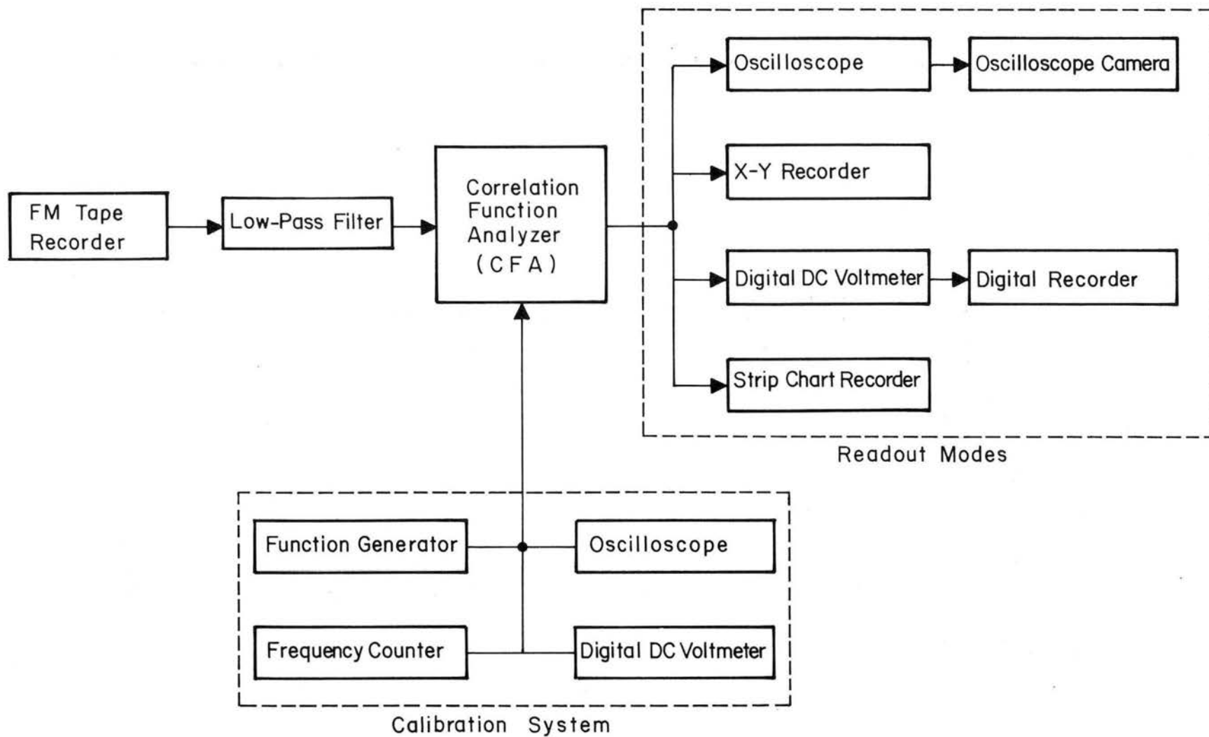
Fig. 5.9 Block diagram of the autocorrelation computation system.
