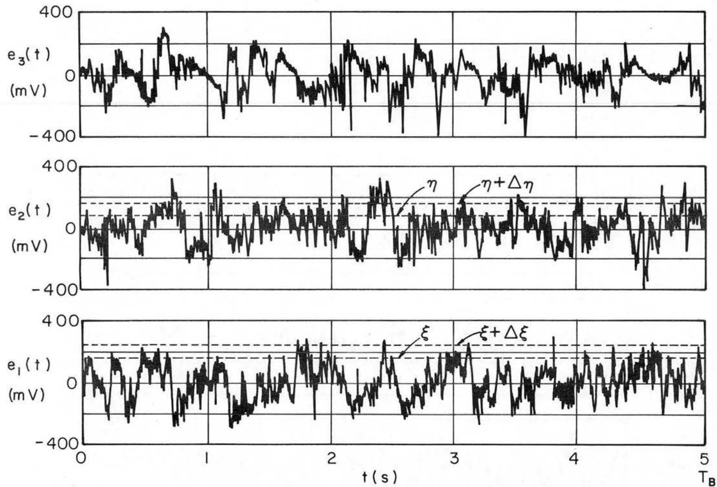
Fig. 6.6 Instantaneous fluctuating voltage during the observation time T_B of three sample records in the equivalent ensemble.
