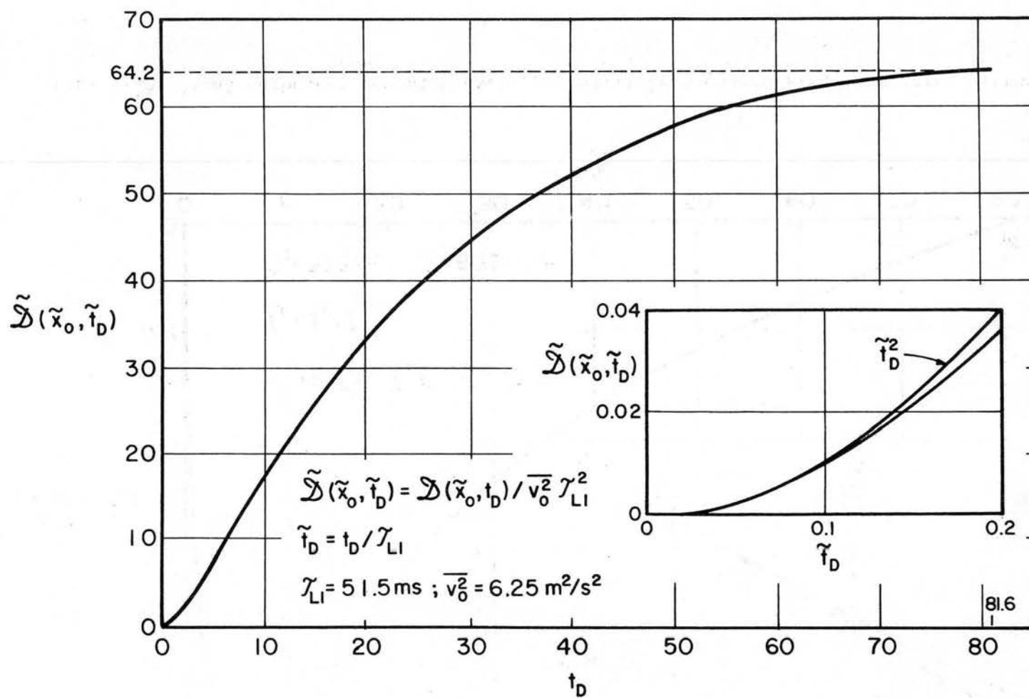
Fig. 6.27 Variation of the longitudinal dispersion coefficient with augmenting diffusion time.
