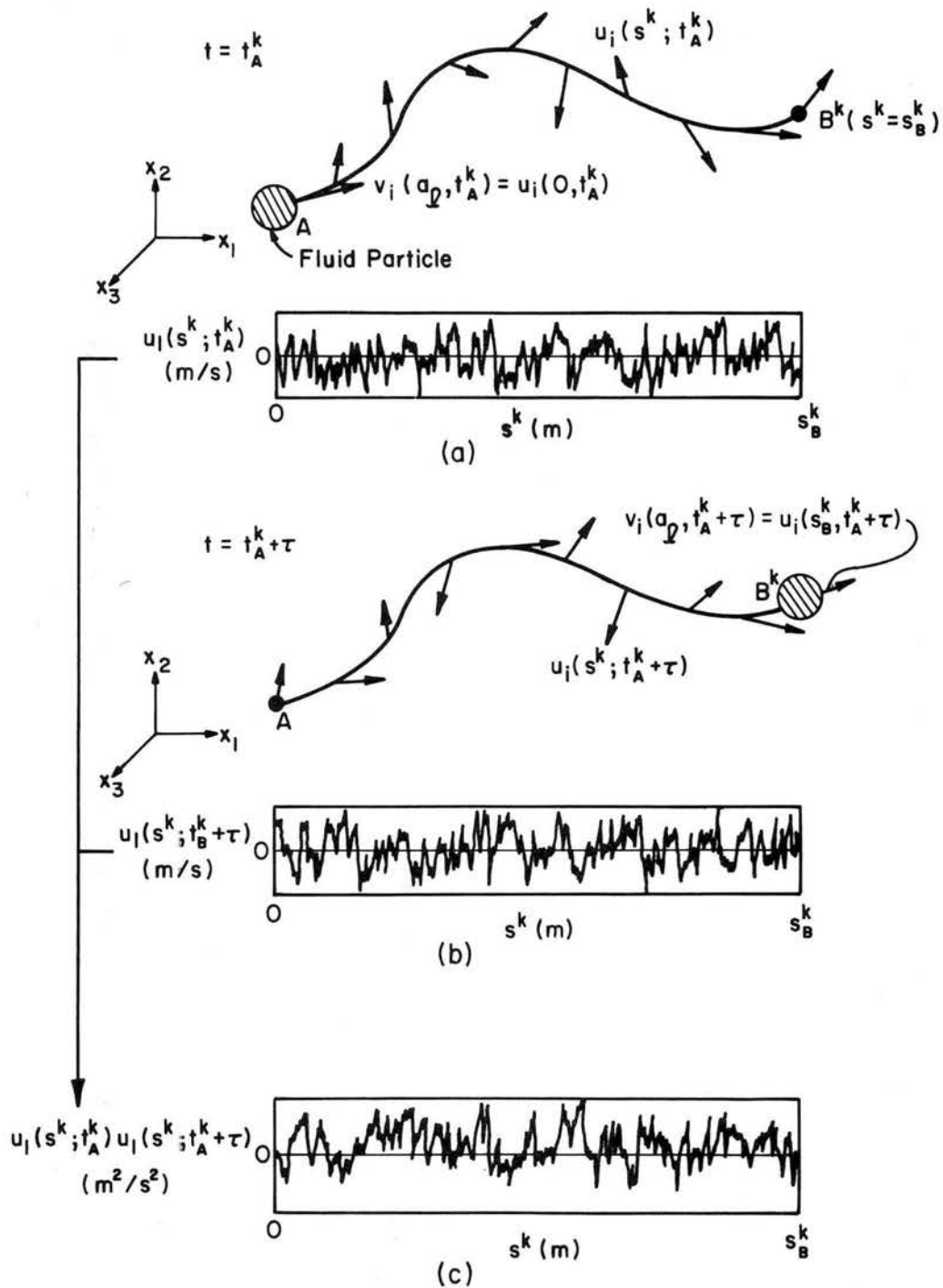
Fig. 3.5 Illustration of the Eulerian velocity product formation for a single velocity component at a point on a trajectory.
