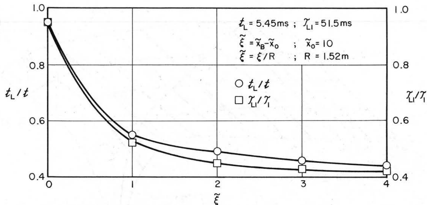
Fig. 6.23 Streamwise changes of the Lagrangian to Eulerian micro time scale and first integral time scale ratios along the turbulence line.
