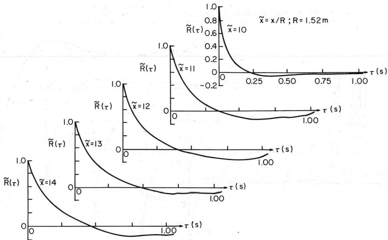
Fig. 6.13(b) - Variation of the five Eulerian turbulent velocity autocorrelation coefficients during the first 1 s lag time.
