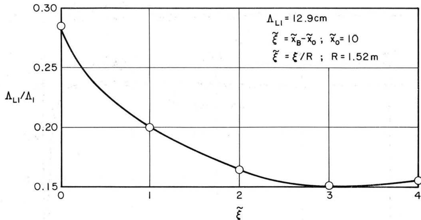
Fig. 6.24 Change of the Lagrangian to Eulerian first integral length scales ratio with increasing axial separation along the turbulence line.
