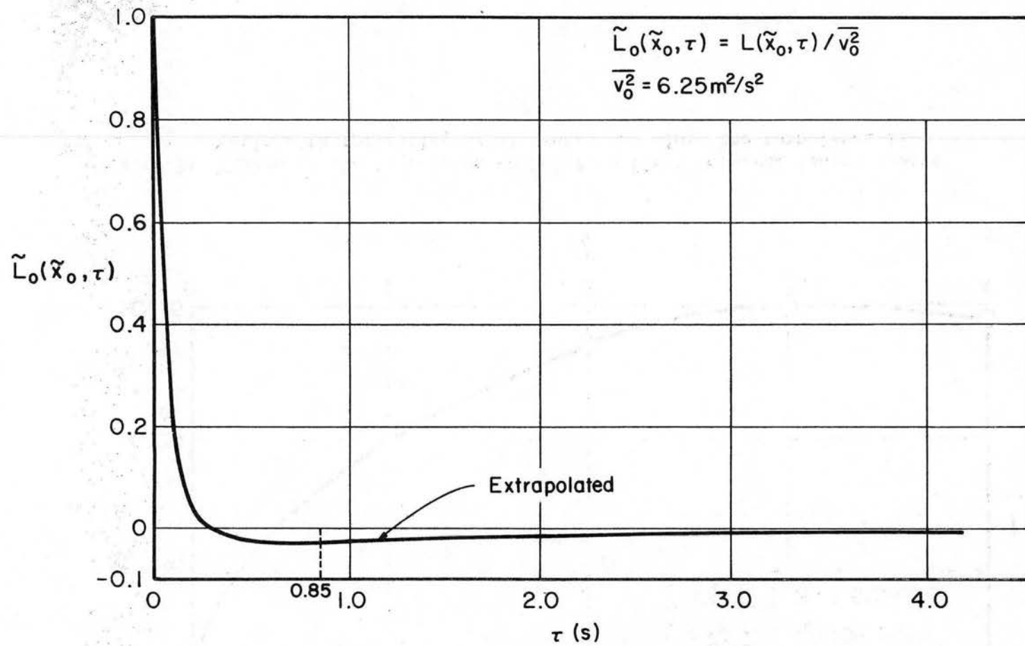
Fig. 6.25 Variation of the extended Lagrangian autocorrelation coefficient with increasing lag time.
