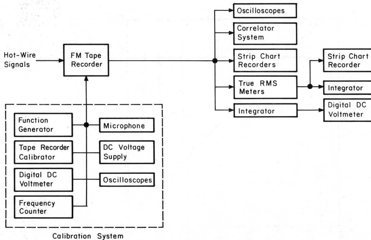
Fig. 5.6 Block diagram of the tape recorder system.
