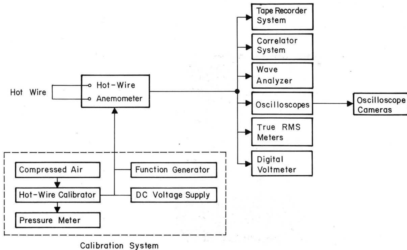
Fig. 5.3 Block diagram of the hot-wire anemometer unit and the Analog Data Acquisition System (ADAS), i.e., the hot-wire anemometer measuring system.
