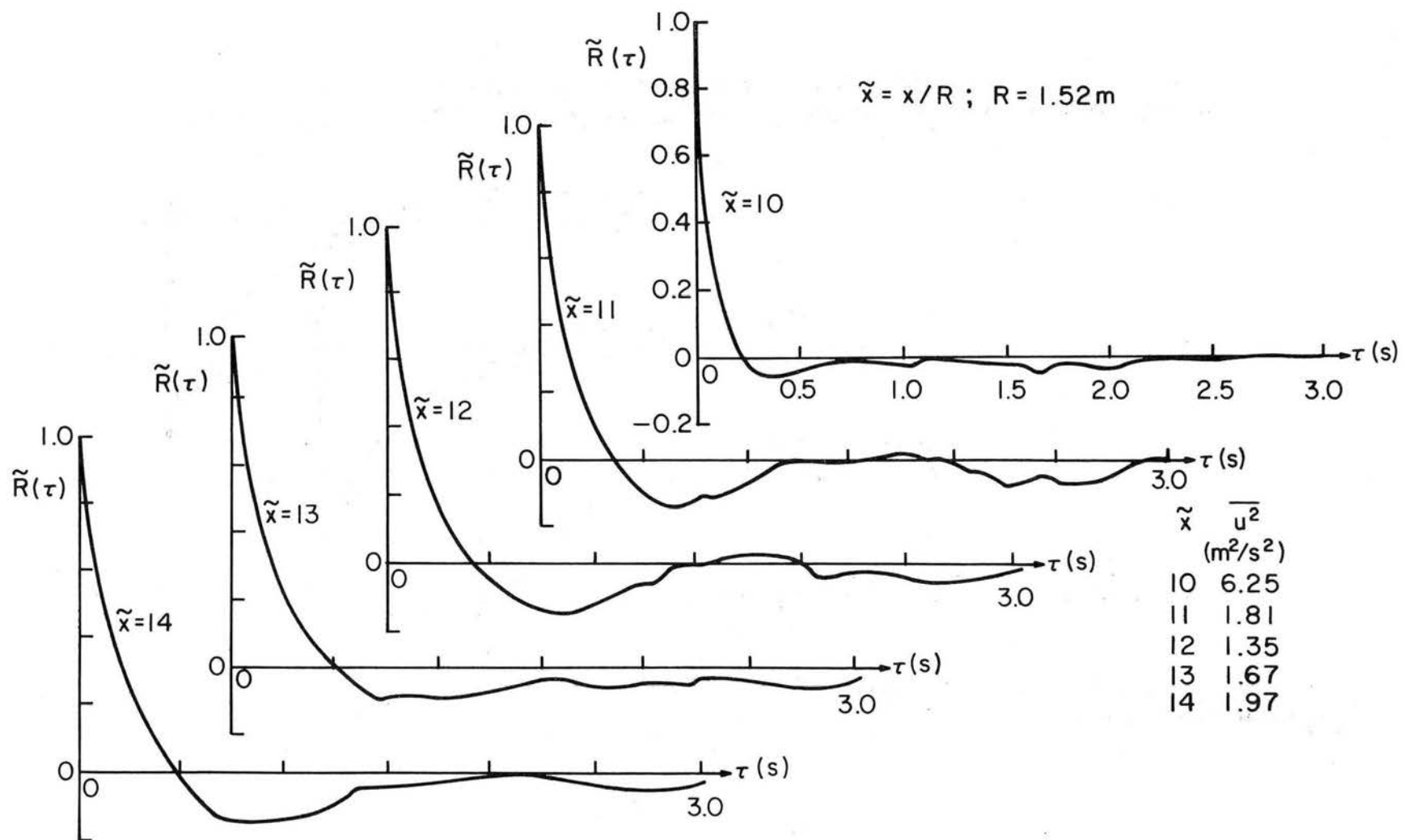
Fig. 6.13(a) Set of five Eulerian turbulent velocity autocorrelation coefficients obtained simultaneously within the turbulence measurement range, i.e., along the turbulence line.
