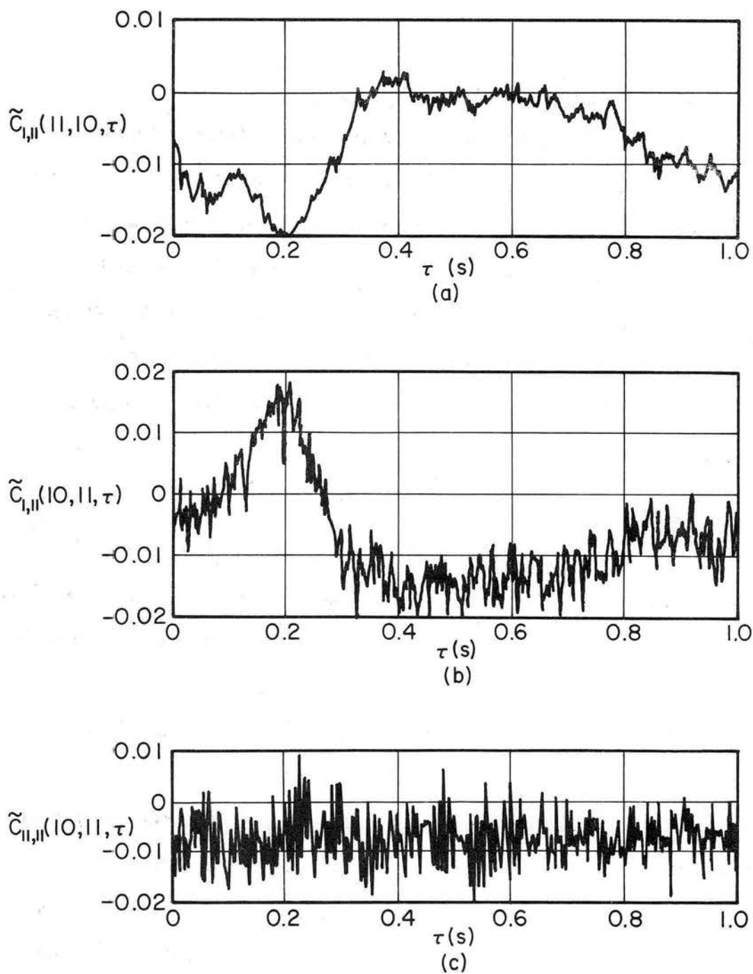
Fig. A.III.1 Variation with increasing time delay for an axial separation \xi = 1 of: (a) and (b) the velocity-velocity derivative cross-correlation coefficients; and, (c) the double velocity derivative cross-correlation coefficient.
