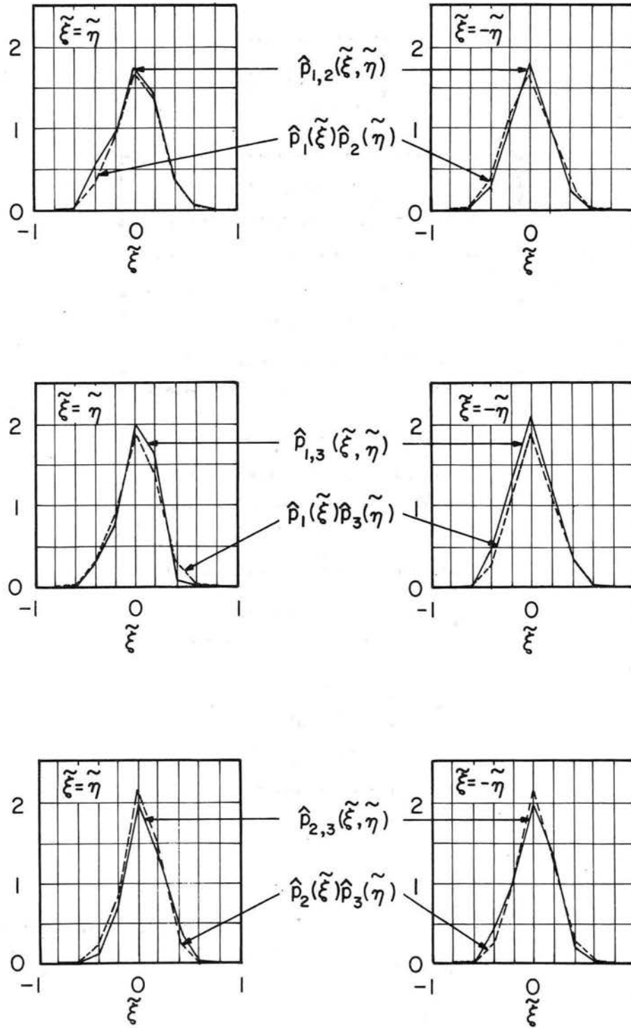
Fig. 6.9 Changes of the joint probability density functions and corresponding products of individual probability density functions for \tilde{\xi} = \tilde{\eta} and -\tilde{\eta} .
