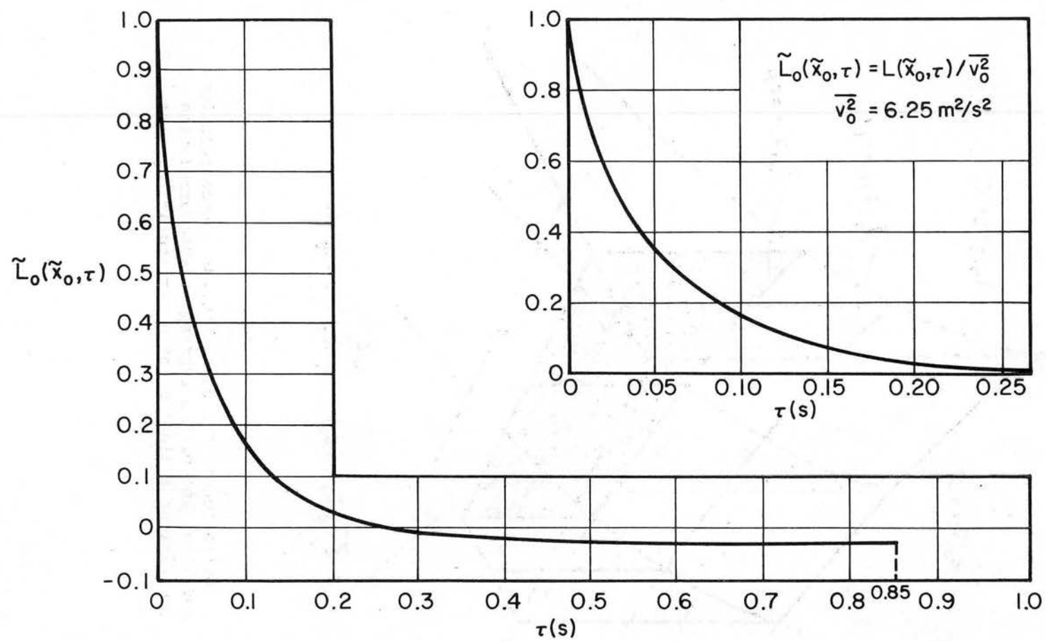
Fig. 6.21 Change of the Lagrangian autocorrelation coefficient with increasing time delay.
