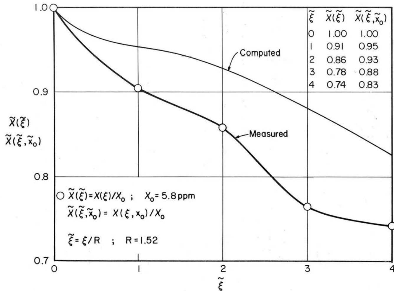
Fig. 6.28 Variation of the measured concentration \tilde{X}(\tilde{\xi}) and computed concentration \tilde{X}(\tilde{\xi}, \tilde{x}_0) along the turbulence line.
