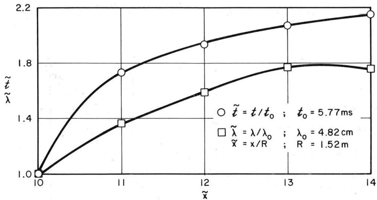
Fig. 6.14 Streamwise variation of the Eulerian micro time and length scales along the turbulence line.
