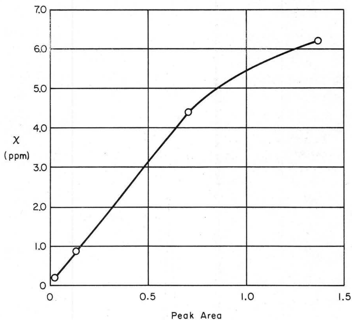
Fig. 5.12 Typical calibration curve of the electron capture detector (ECD) to known \text{SF}_6 concentrations \chi in air mixtures.
