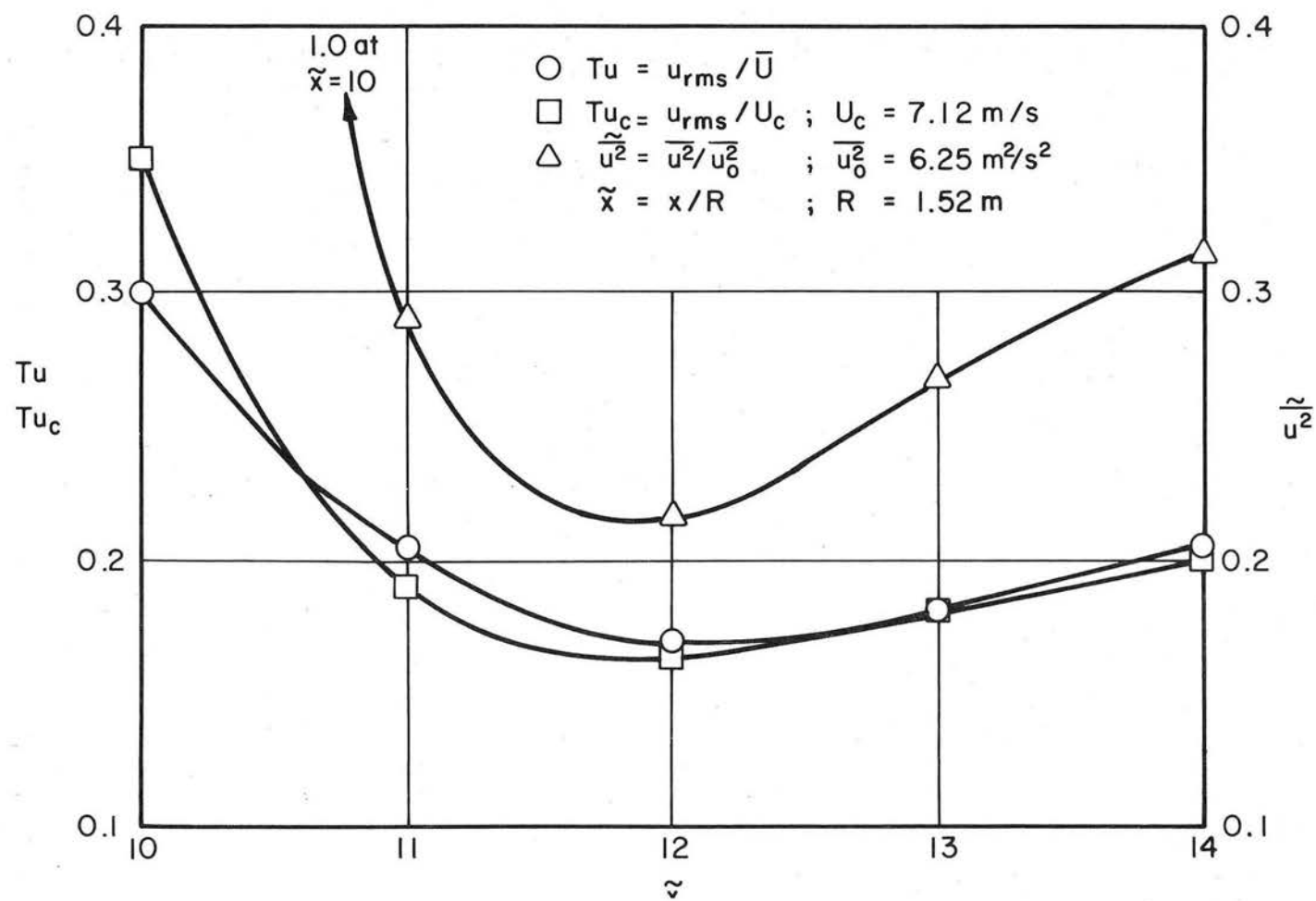
Fig. 6.3 Variation of the longitudinal turbulence intensities and normalized mean-square value of the longitudinal turbulent velocity along the turbulence line.
