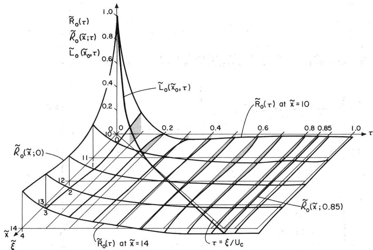
Fig. 6.22 Variations in time and space of the set of five Eulerian reference-point autocorrelation coefficients \tilde{R}_0(\tau) , of several envelopes \tilde{R}_0(\tilde{x}; \tau) and of the Lagrangian autocorrelation coefficient \tilde{L}_0(\tilde{x}, \tau) for the turbulence line.
