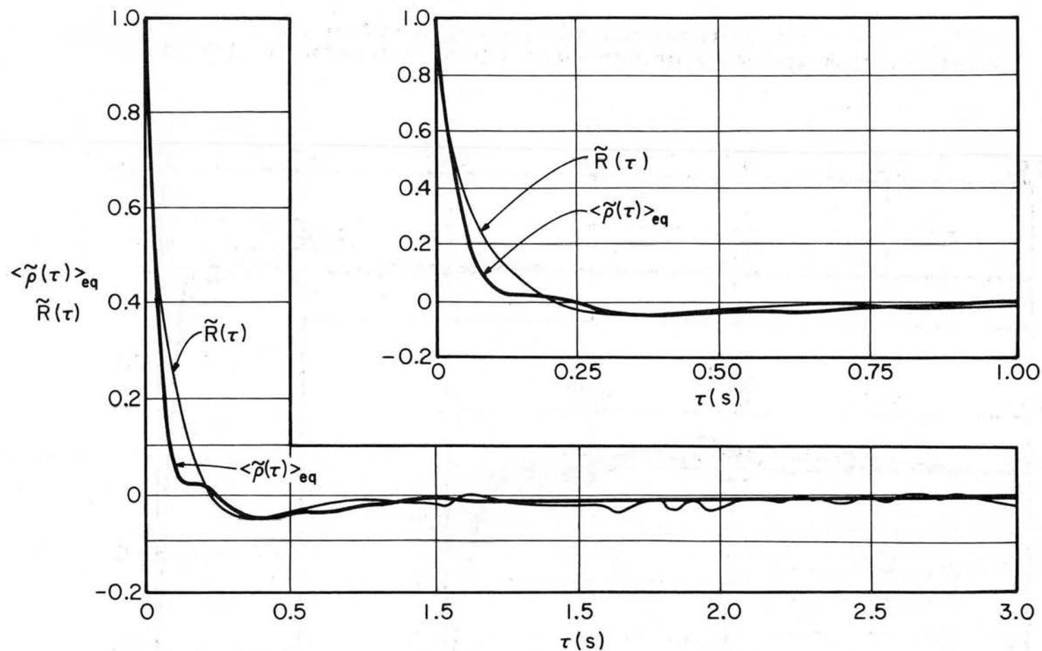
Fig. 6.12 Equivalent ensemble autocorrelation coefficient averaged over all starting times \langle \tilde{\rho}(\tau) \rangle_{eq} and time-averaged autocorrelation coefficient over a single sample record \tilde{R}(\tau) .
