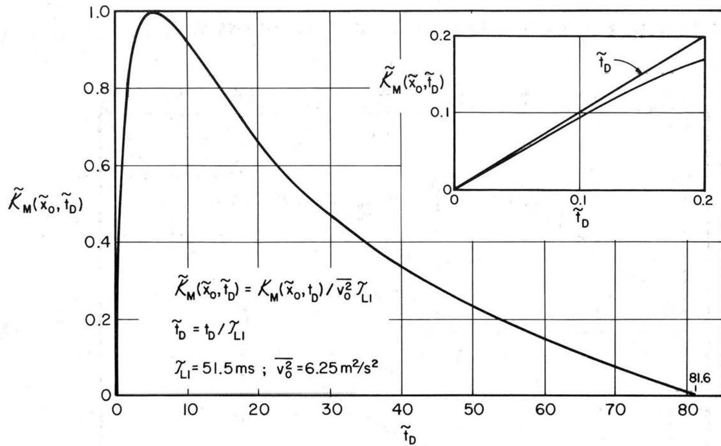
Fig. 6.26 Axial turbulent momentum exchange coefficient change with increasing diffusion time.
