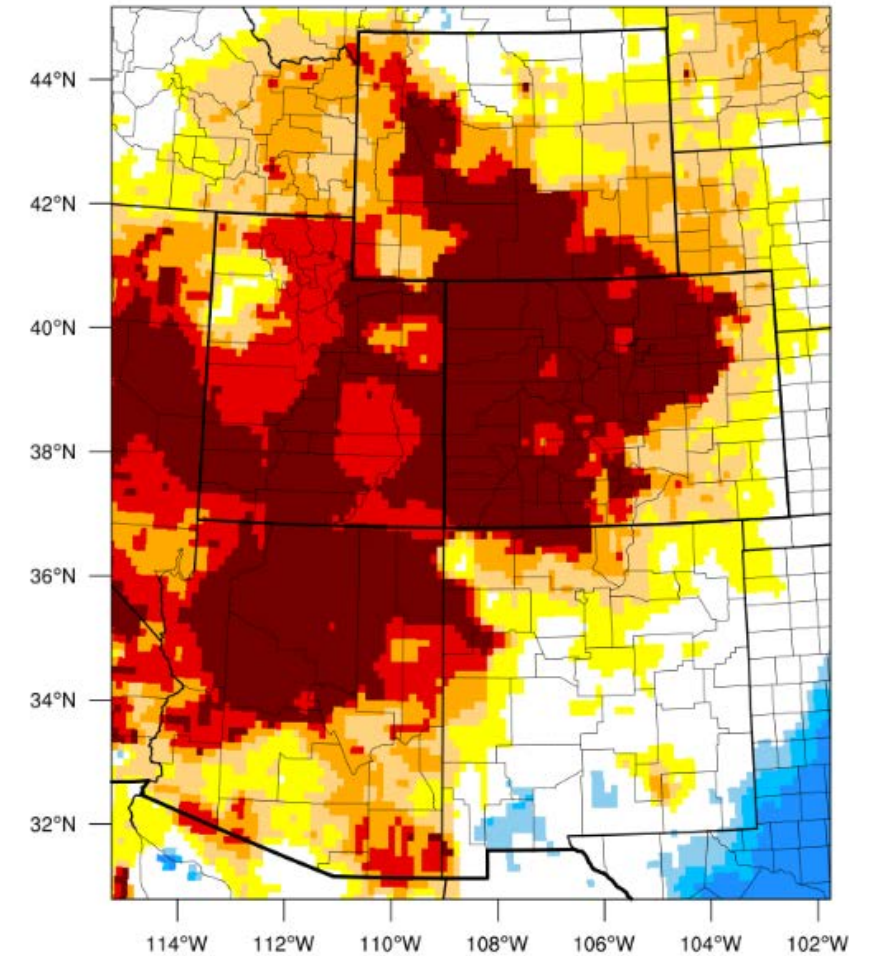
1-week EDDI categories for September 14, 2018
