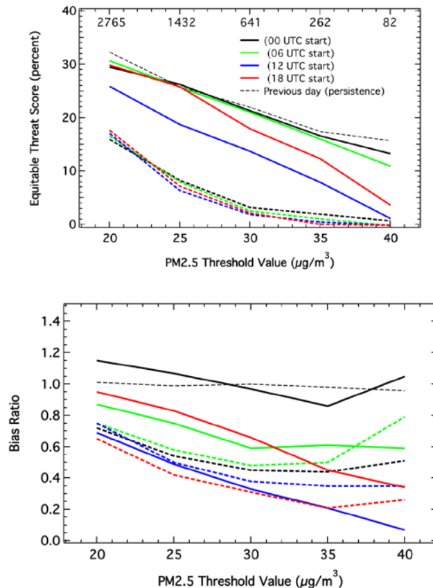
Figures 1 and 2: Equitable threat score and bias ratio for control forecasts (dashed) and with assimilation.
