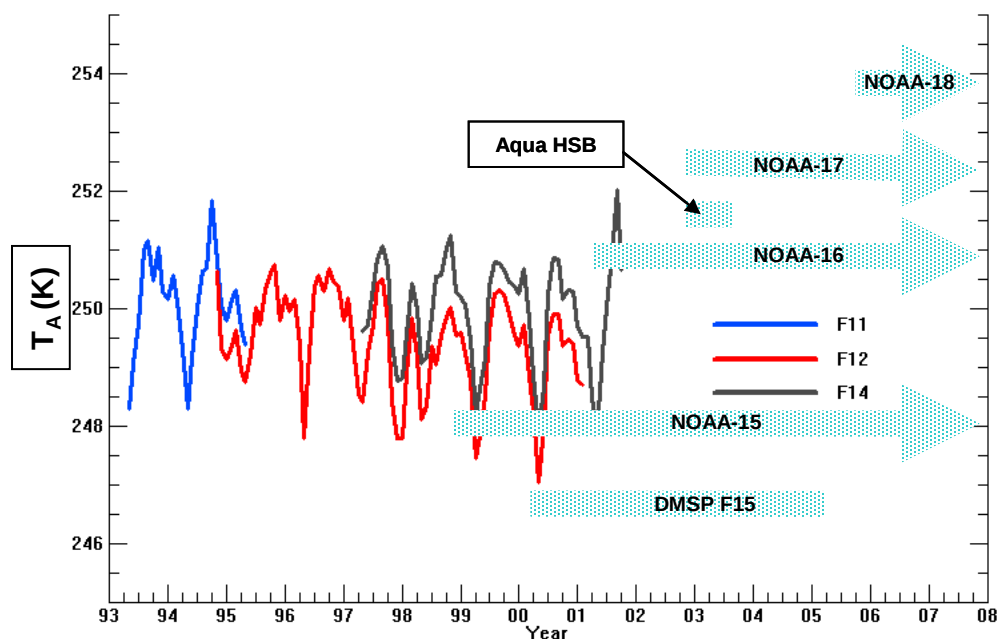
Figure 1: Time series of satellites with 183 GHz measurements. The monthly mean antenna temperature from 10^{\circ} N to 10^{\circ} S for the 183 \pm 1 GHz channel on the SSM/T-2 instrument at near-nadir for the F11, F12 and F14 spacecraft is shown (blue, red, and gray lines). Periods of coverage for the SSM/T-2 on F15 and the AMSU-B sensors, as well as the short-lived but valuable HSB instrument on Aqua are also shown. CIRA rescued the F11 SSM/T-2 data (blue line) and delivered this data to NCDC for future stewardship.
