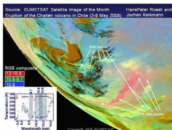
Figure 2: This sample image from the new GOES-R training module demonstrates the use of RGB image combinations and the addition of a new channel near 8.7 \mu\text{m} to aid in the detection of volcanic ash and SO 2 using a EUMETSAT image of the Chaitén Volcano in Chile in May 2008.
