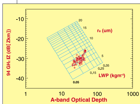
Fig. 2: The relationship between integrated radar reflectivity and cloud optical depth provides independent information about liquid water path and particle size, as indicated by the nearly orthogonal grid.
