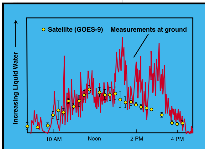
Fig. 2: Verification of GOES-9 imager estimates of cloud liquid water path by comparison to surface microwave radiometer observations over Oklahoma. Differences occurring after 12:30 PM were likely caused by drizzle formation (from Greenwald et al. 1999)
