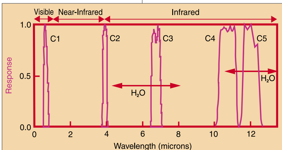
Fig.1: Spectral regions sensed by the five GOES-9 imager channels (C1-C5)
