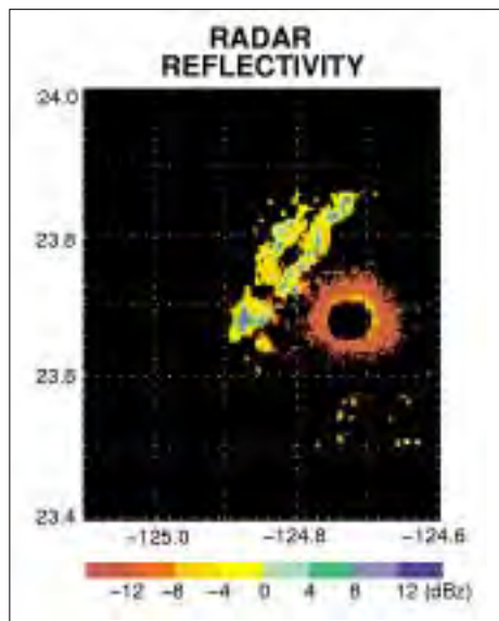
Fig. 4: GOES-9 observed signatures of drizzling marine stratocumulus clouds in the West Pacific for imager channels 1 (left) and 2 (right). Coincident ship-based radar observations are also shown (center). Radar return strength given in units of dBZ (from Greenwald and Christopher 1999b)
