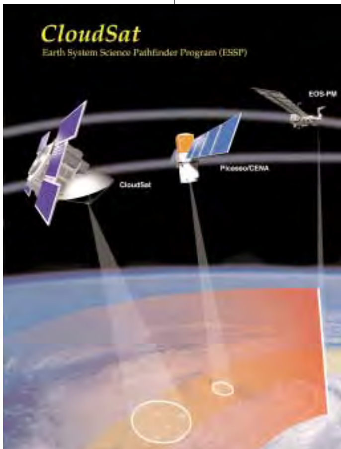
Fig. 1: CloudSat will fly in formation with PICASSO-CENA
