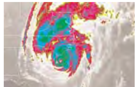
GOES-8 image of Hurricane Floyd as it approaches the North Carolina coast on the evening of September 15, 1999. The colors indicate infrared cloud-top temperatures. The coldest temperatures are near -80 degrees Celsius.
