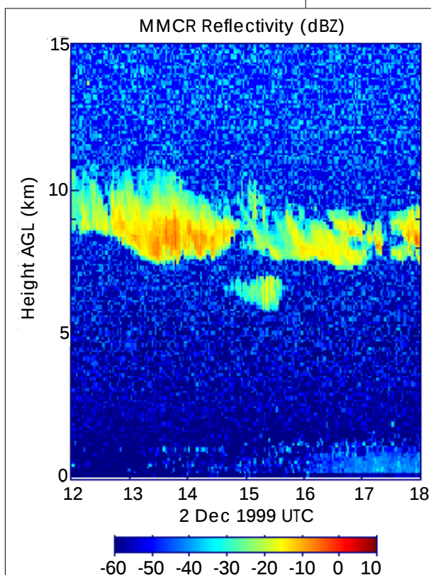
Fig. 4: Millimeter Cloud Radar (MMCR) observations
