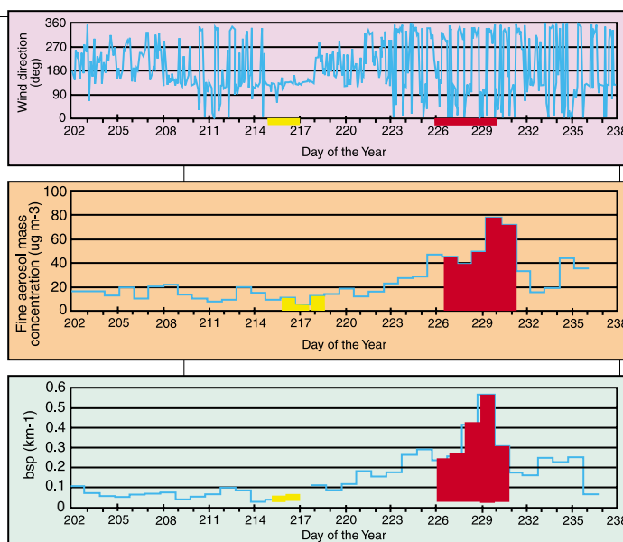
Fig. 1: Timelines of three parameters measured during the 1995 SEAVS study. (Top) Wind direction at the Look Rock Tower site 739 m ASL on the western edge of Great Smoky Mountains National Park. The mountain ridge is oriented SW to NE. The yellow bar marks dates with constant SE flow associated with the passage of the remnants of Hurricane Erin. The red bar marks the calm stagnation (hazy) period, having diurnal wind shifts associated with upslope and downslope flows created by surface heating and cooling. (Middle) Fine aerosol mass concentrations in \mu\text{g m}^{-3} , from filters exposed for 24 hours. Yellow shading marks samples from the hurricane-influenced period; samples shaded red indicate the large increases observed in mass concentrations during the hazy period. (Bottom) Light scattering coefficient, bsp, in \text{km}^{-1} . Bsp is inversely related to the visual range. Note the large increase in bsp, and hence decrease in visual range, associated with the stagnation period (red), relative to the values in the marine air associated with the hurricane-influenced period (yellow).
