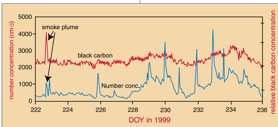
Fig. 3: Timelines of accumulation mode aerosol number concentration and variations in measured black carbon concentrations for two weeks in August 1999 during the BRAVO field project. The spike in black carbon and in number concentration on DOY 222 was associated with transport of smoke from a nearby fire in the Rio Grande river basin. Explanations for other excursions in the two variables have not yet been identified.
