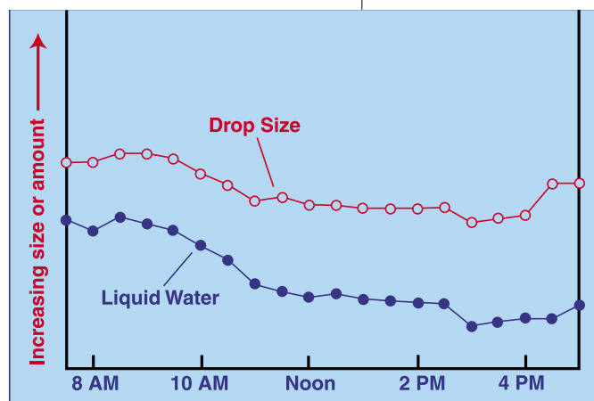
Fig. 3: Daytime cycle of stratocumulus microphysical properties off the coast of Baja California as observed by the GOES-9 imager (from Greenwald and Christopher 1999a)
