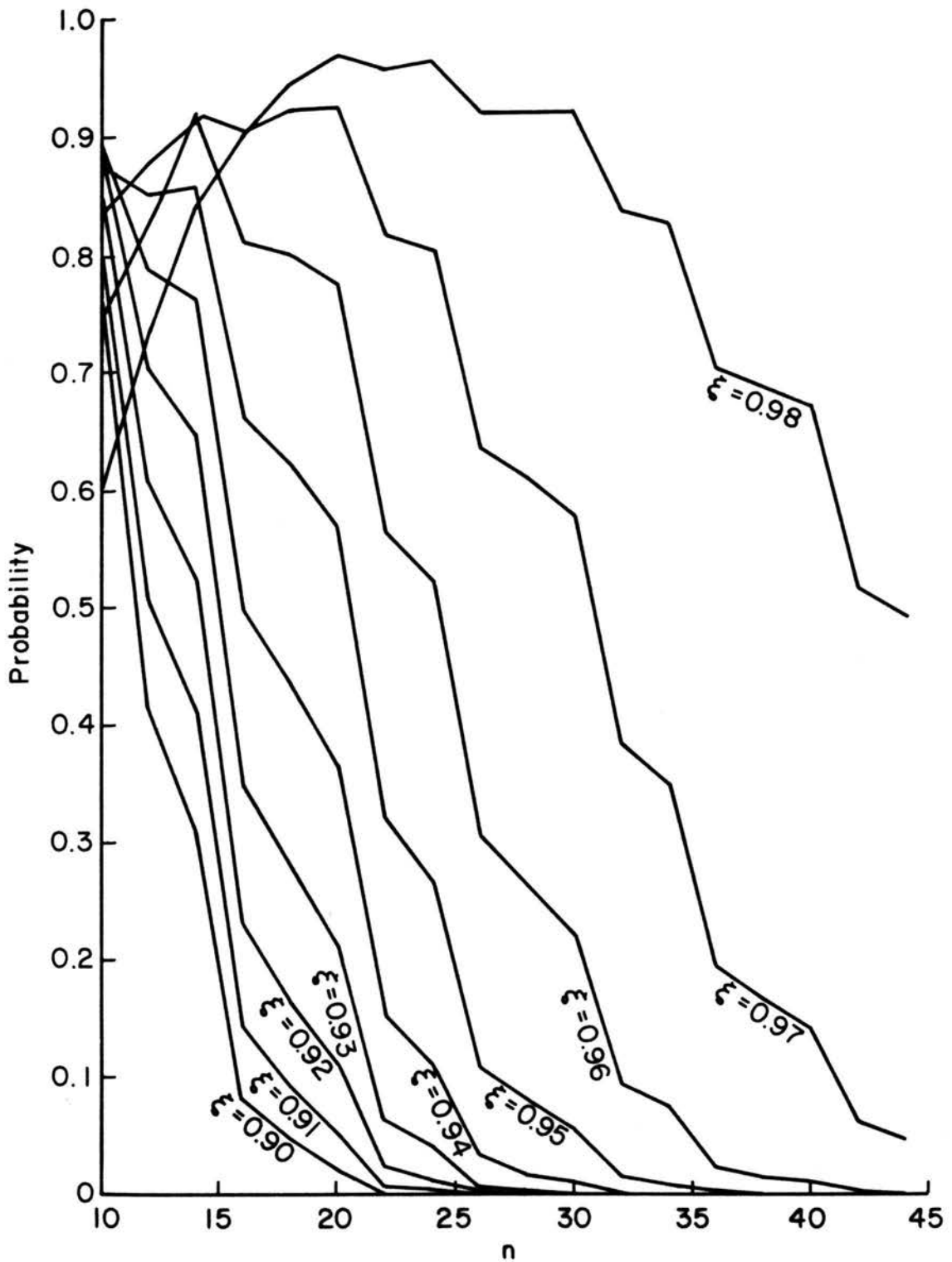
Fig. 3.3.2 Variation of Probability For Percentage (Or More)
