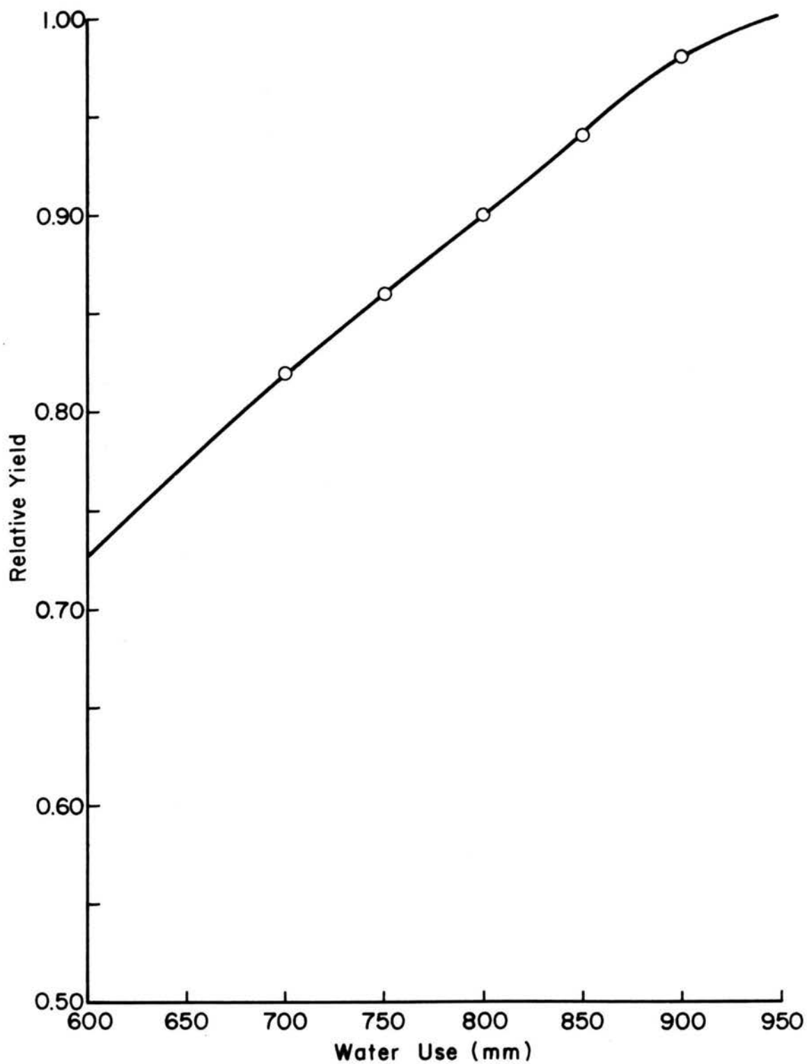
Figure 4.5.3 Yield vs Seasonal Water Use For Corn
