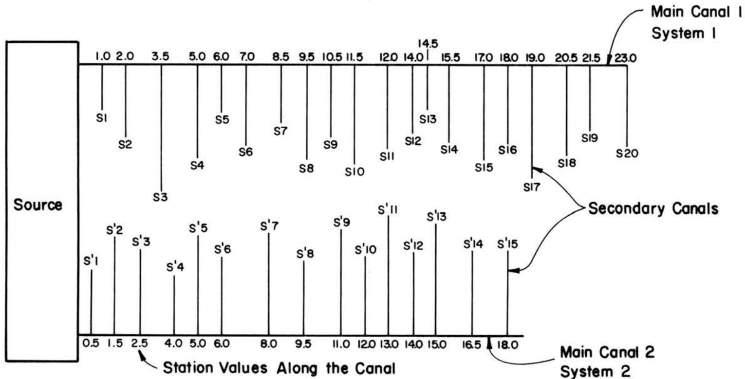
Figure 5.4.1 Idealized View Of The Project System
