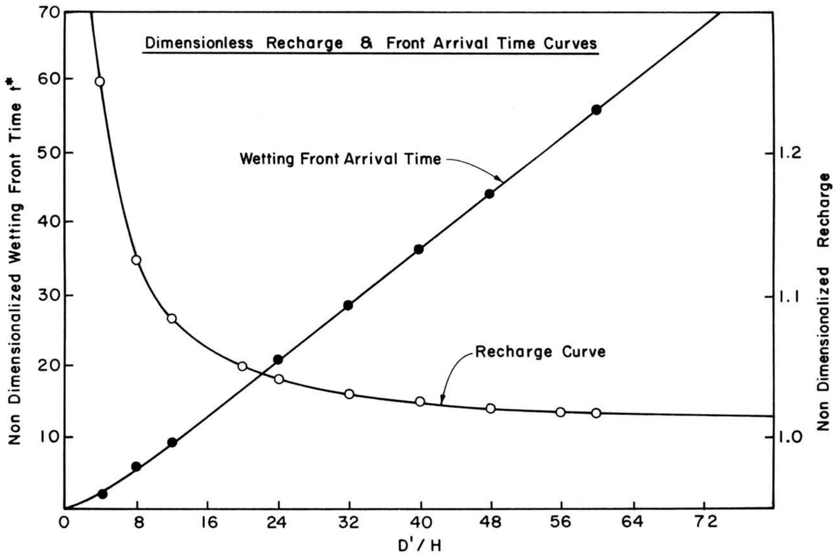
Figure 6.5.1 Dimensionless Recharge And Front Arrival Time Curves
