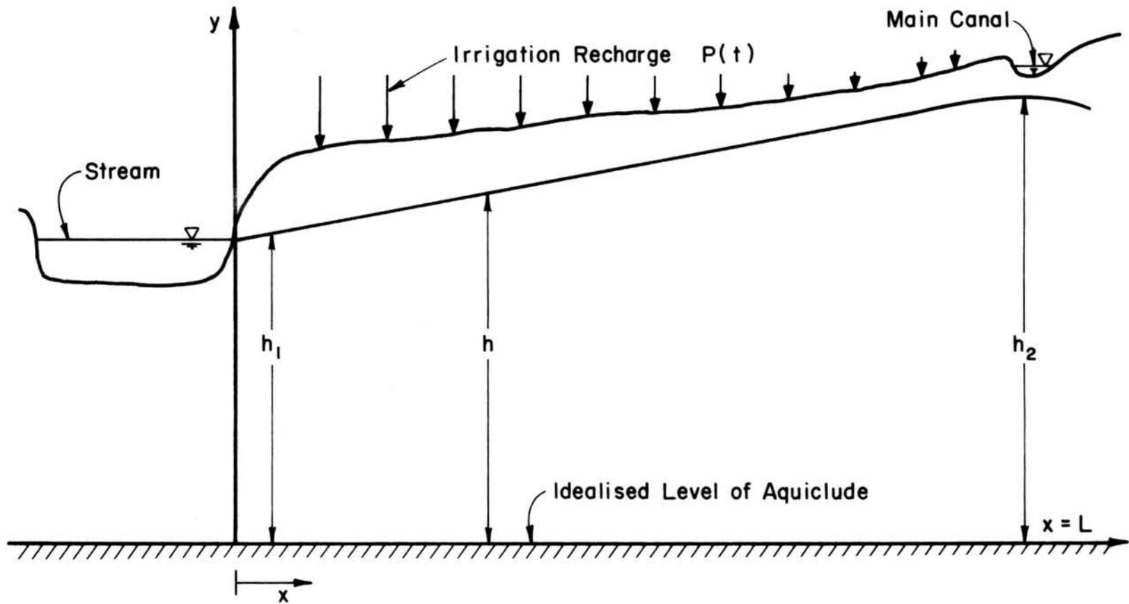
Figure 6.2.2 Cross Sectional View Of Irrigated Area
