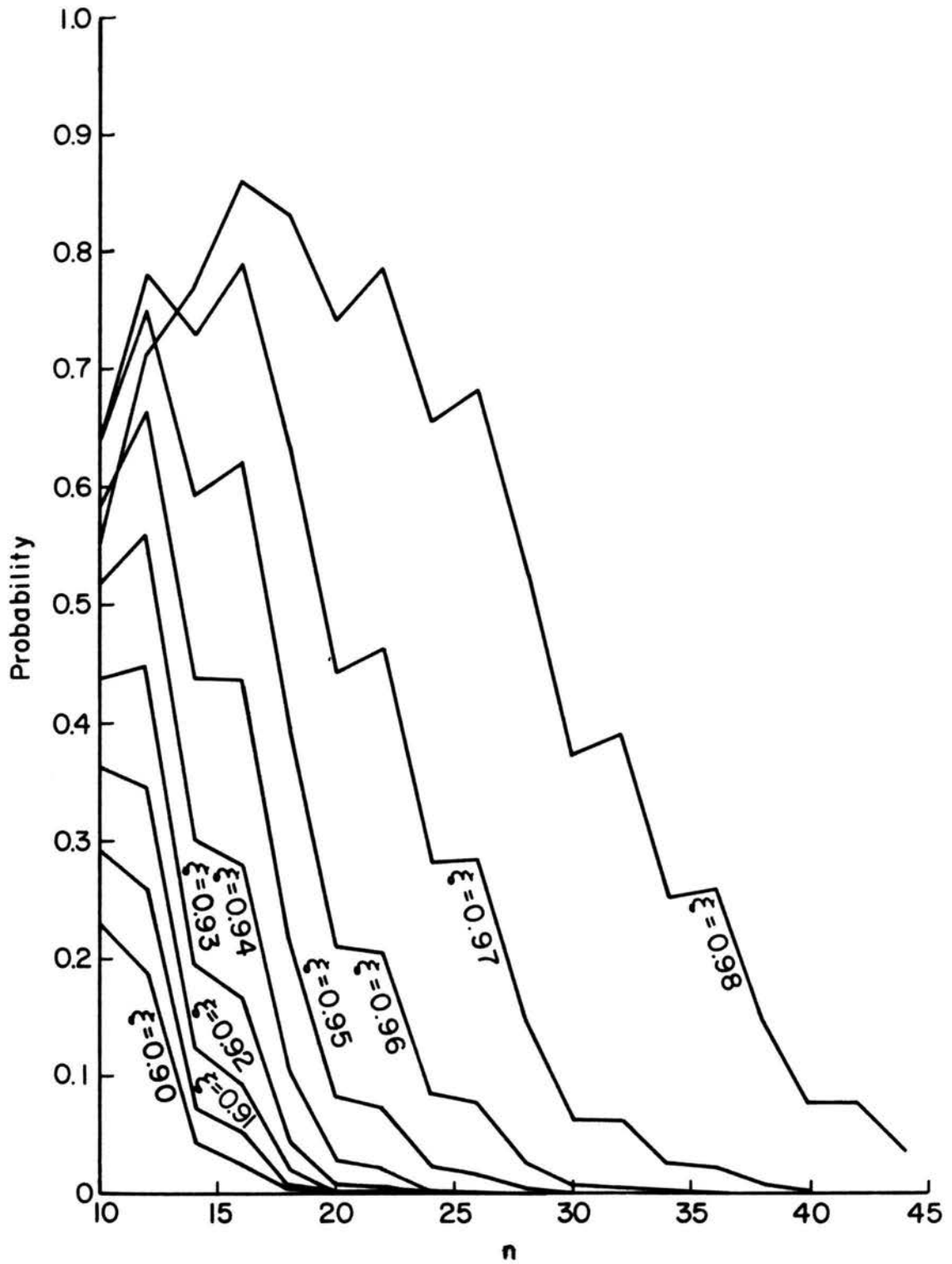
Fig. 3.3.4 Variation of Probability for Percentage
