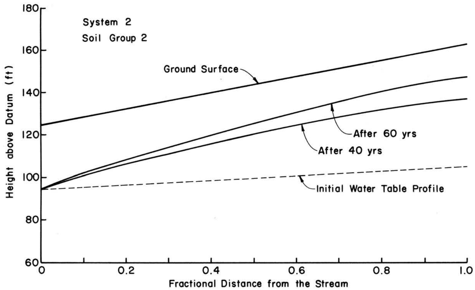
Figure 6.6.6 Water Table Envelope Curves For System 2, Soil Group 2
