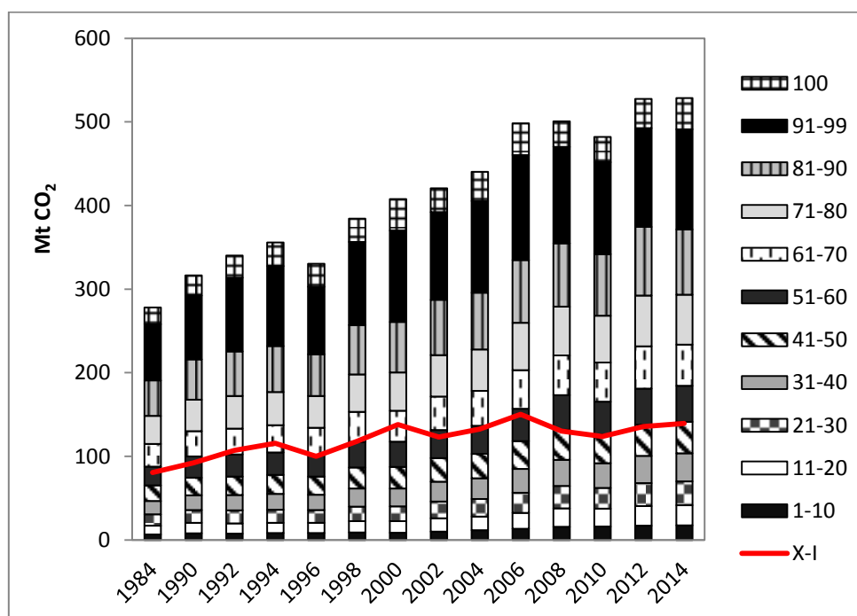
Fig. 2. CO 2 emissions by income group in Mexico 1984-2014 ( \epsilon=0.9 )
