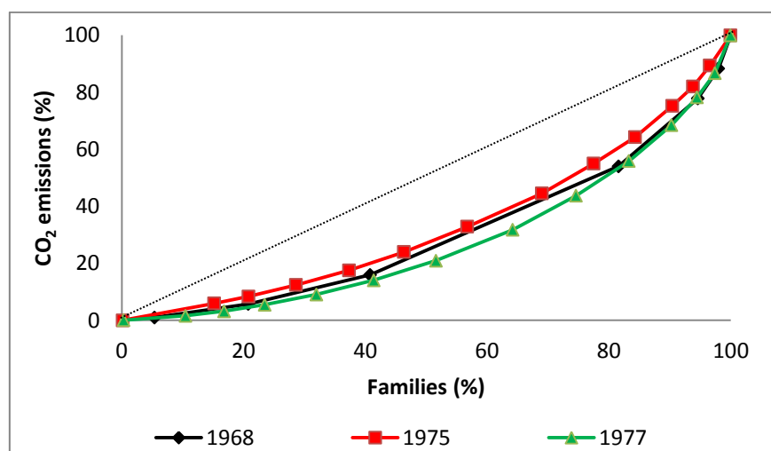
Fig. 1. Lorenz curves for CO 2 emissions in Mexico 1968, 1975, and 1977 ( \epsilon=0.9 ).
