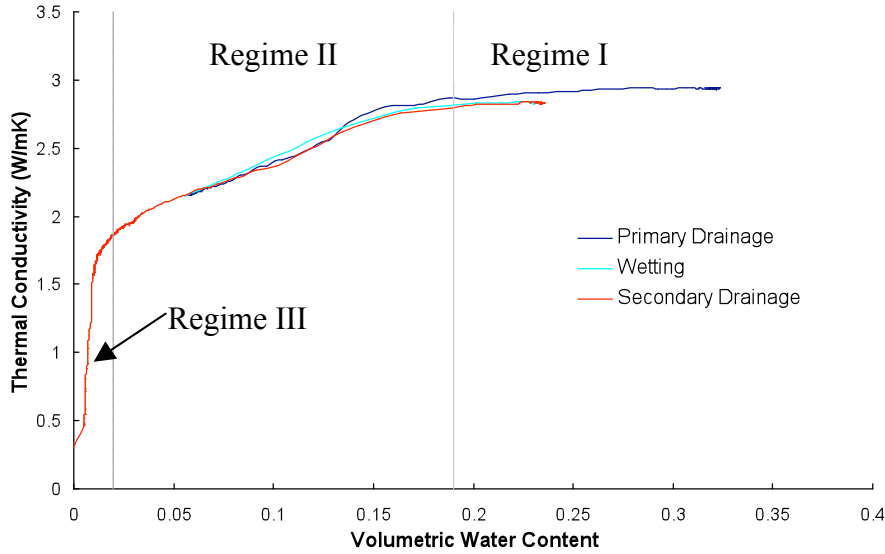
Figure 2: Thermal conductivity as a function of water content for #20/30 sand under tightly packed (porosity = .322, dry bulk density = 1.80 \text{ g/cm}^3 ) conditions for primary drainage, wetting and secondary drainage cycles.
