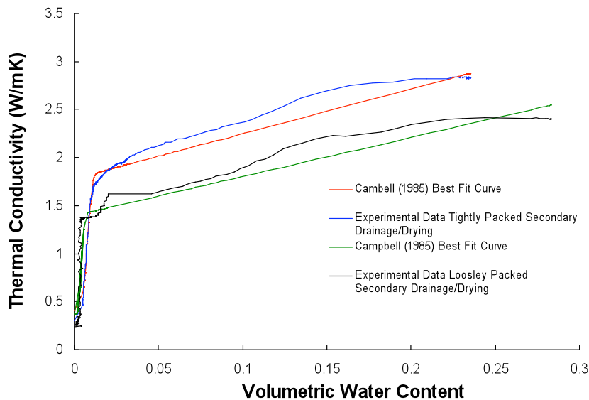
Figure 4: Measured and Campbell model-predicted thermal conductivity values for #20/30 sand under tightly and loosely packed conditions.
