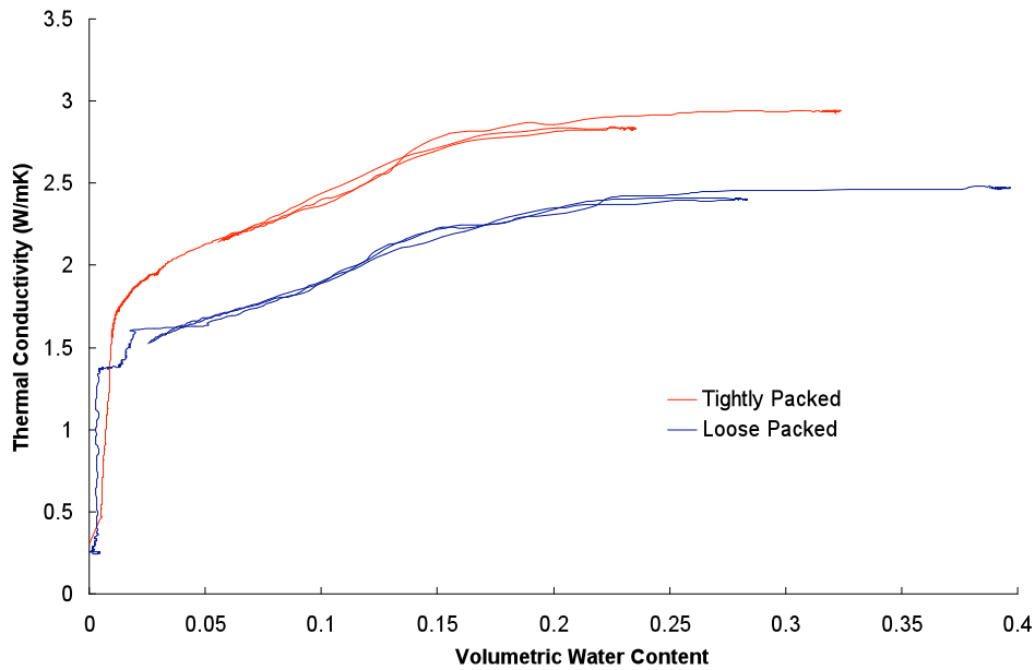
Figure 3: Thermal conductivity as a function of water content for #20/30 sand under tightly packed (porosity = 0.322) and loosely packed (porosity = 0.388) conditions.
